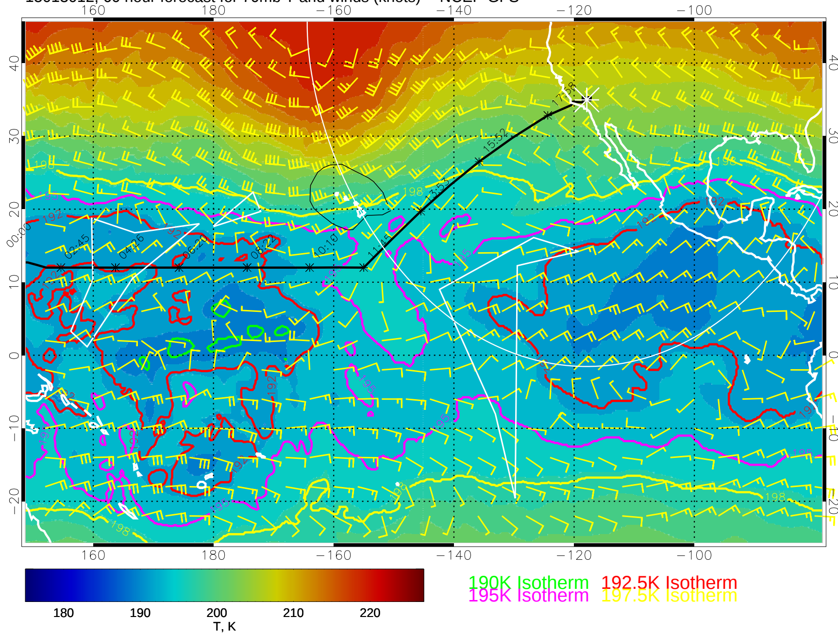
15013012, 60 hour forecast for 70mb T and winds (knots) -- NCEP GFS
