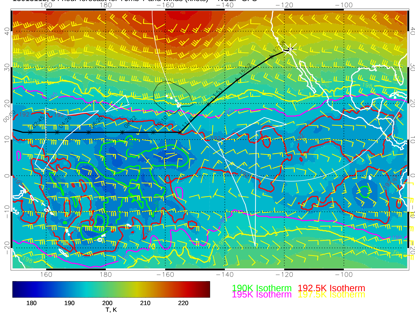
15013112, 84 hour forecast for 70mb T and winds (knots) -- NCEP GFS
