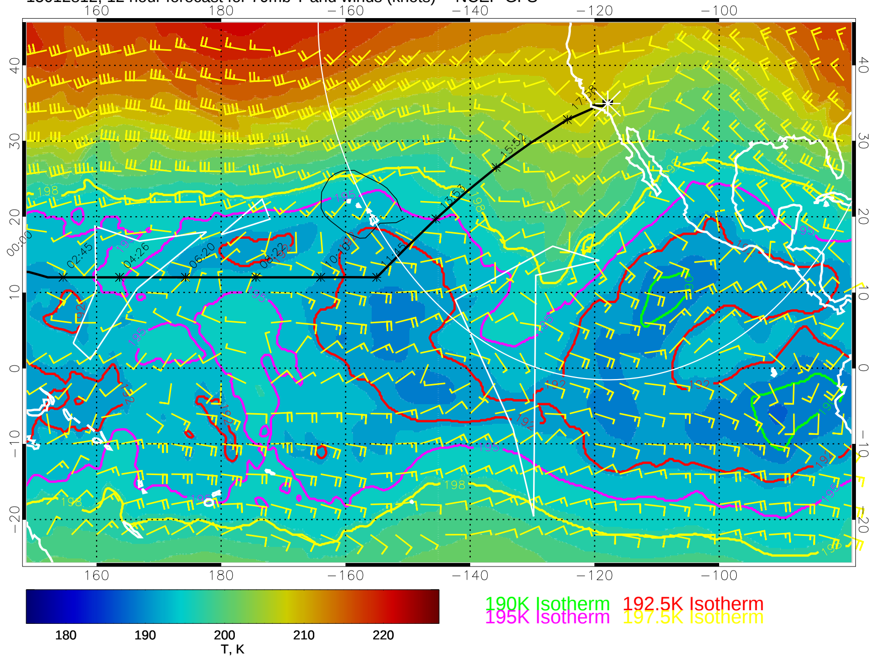
15012812, 12 hour forecast for 70mb T and winds (knots) -- NCEP GFS
