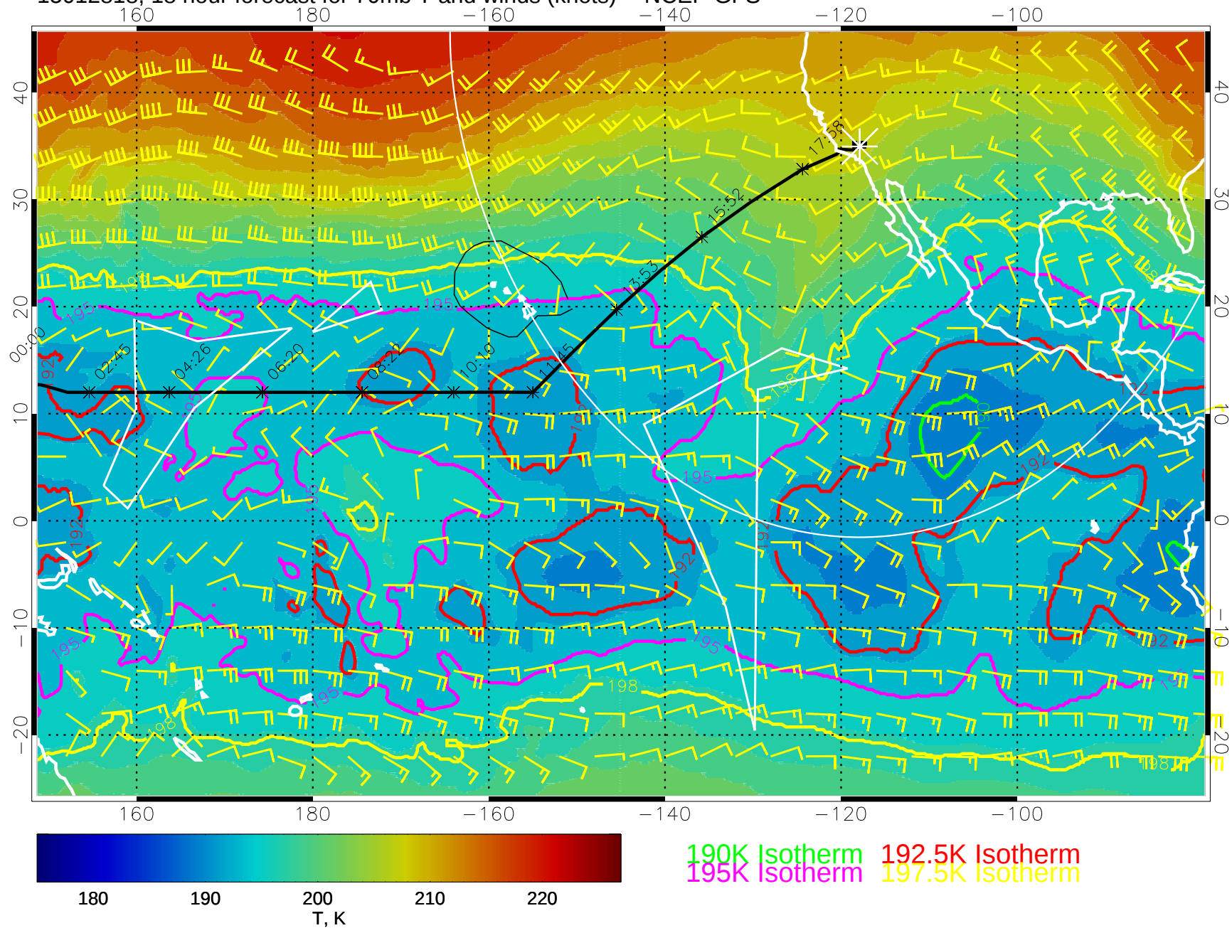
15012818, 18 hour forecast for 70mb T and winds (knots) -- NCEP GFS
