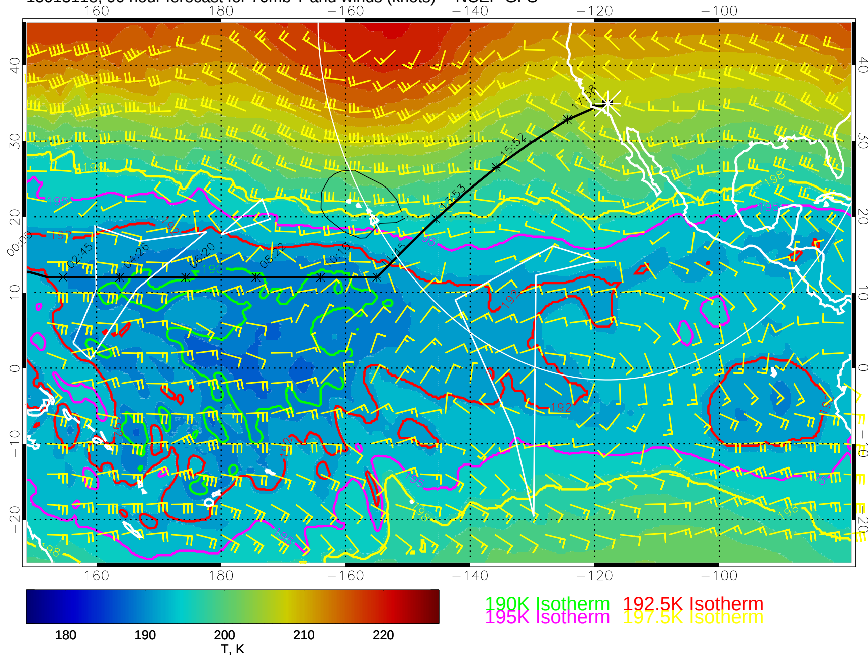
15013118, 90 hour forecast for 70mb T and winds (knots) -- NCEP GFS
