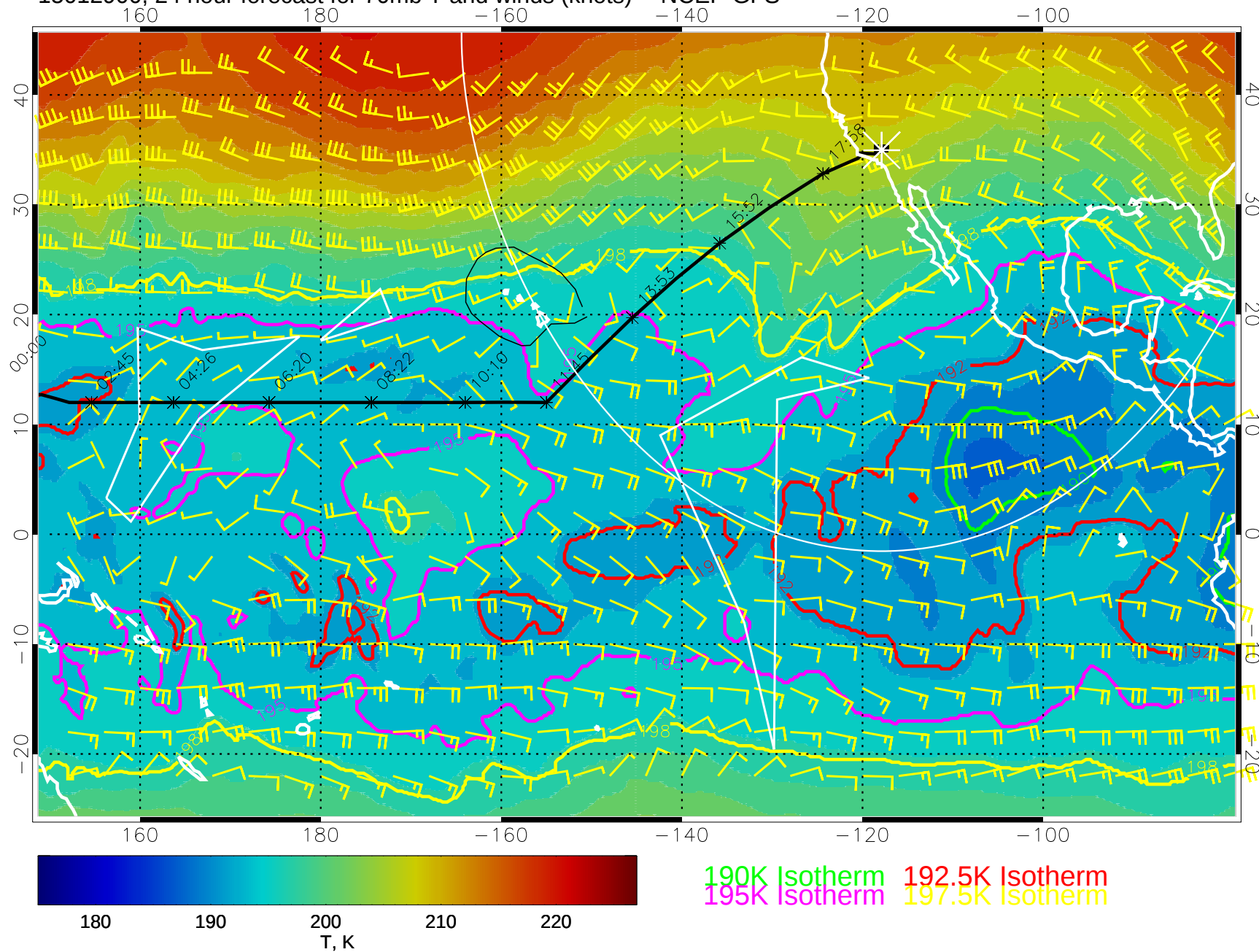
15012900, 24 hour forecast for 70mb T and winds (knots) -- NCEP GFS
