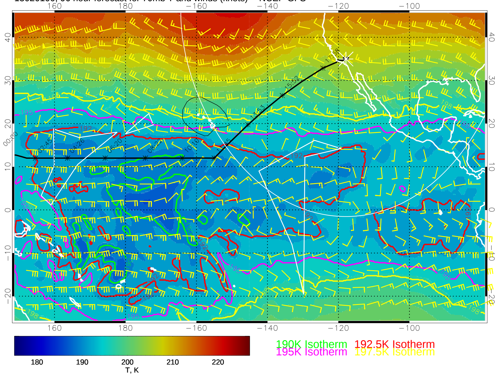
15020100, 96 hour forecast for 70mb T and winds (knots) -- NCEP GFS
