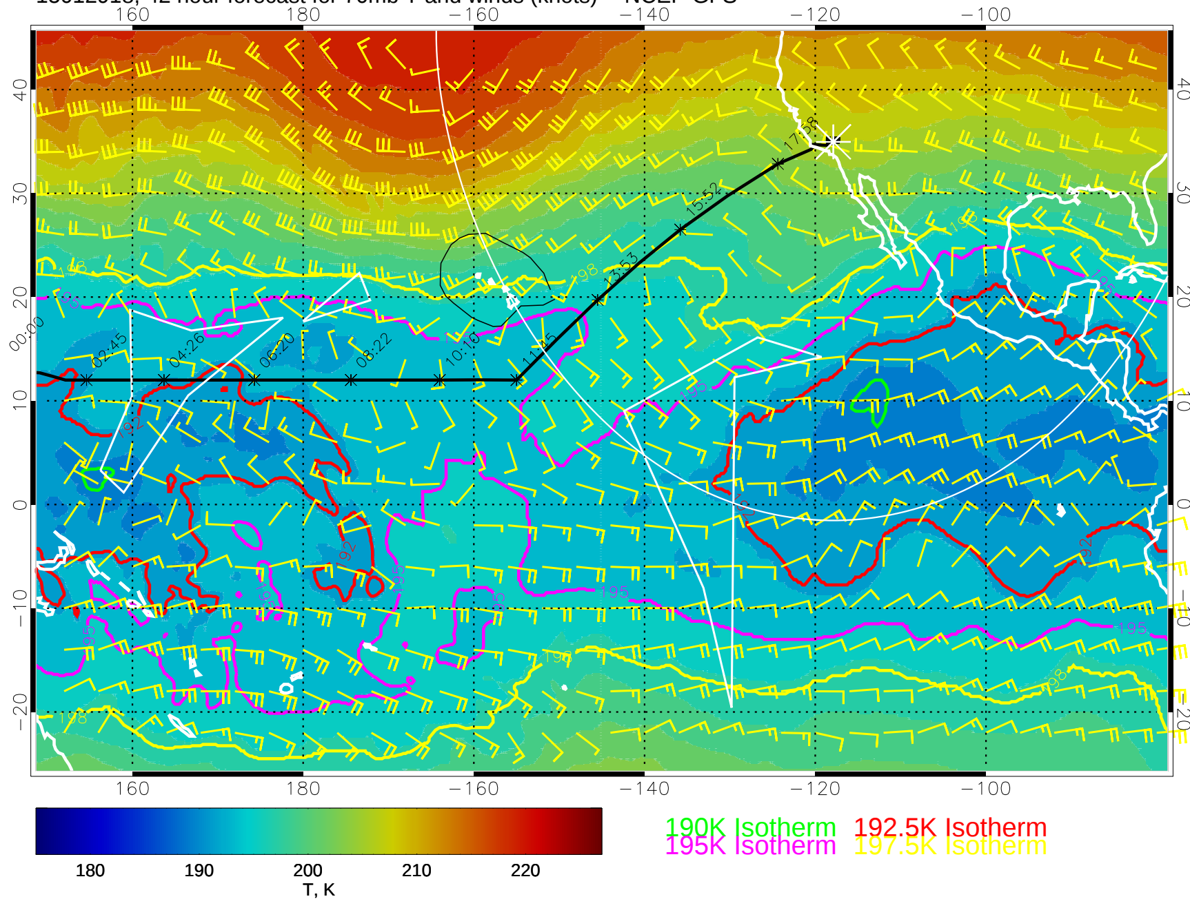
15012918, 42 hour forecast for 70mb T and winds (knots) -- NCEP GFS
