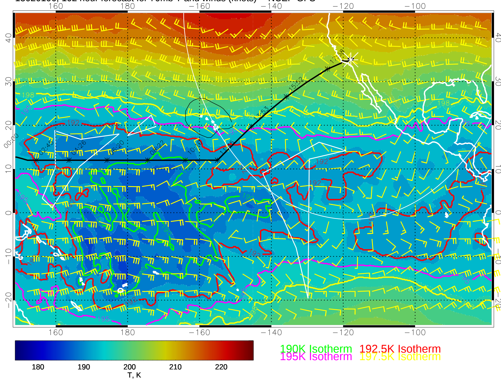
15020106, 102 hour forecast for 70mb T and winds (knots) -- NCEP GFS
