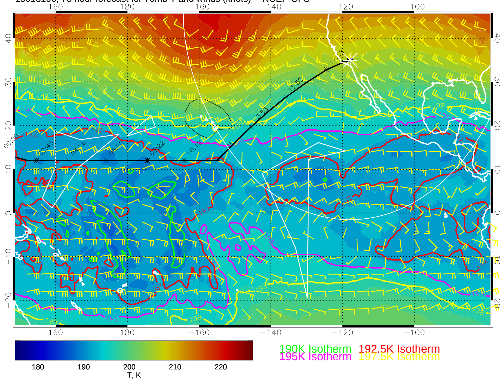
15013106, 78 hour forecast for 70mb T and winds (knots) -- NCEP GFS
