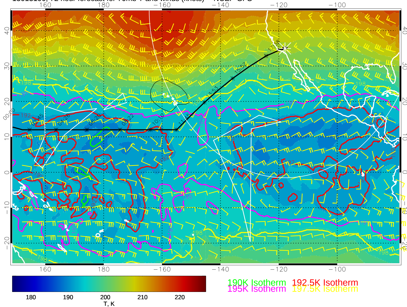
15013100, 72 hour forecast for 70mb T and winds (knots) -- NCEP GFS
