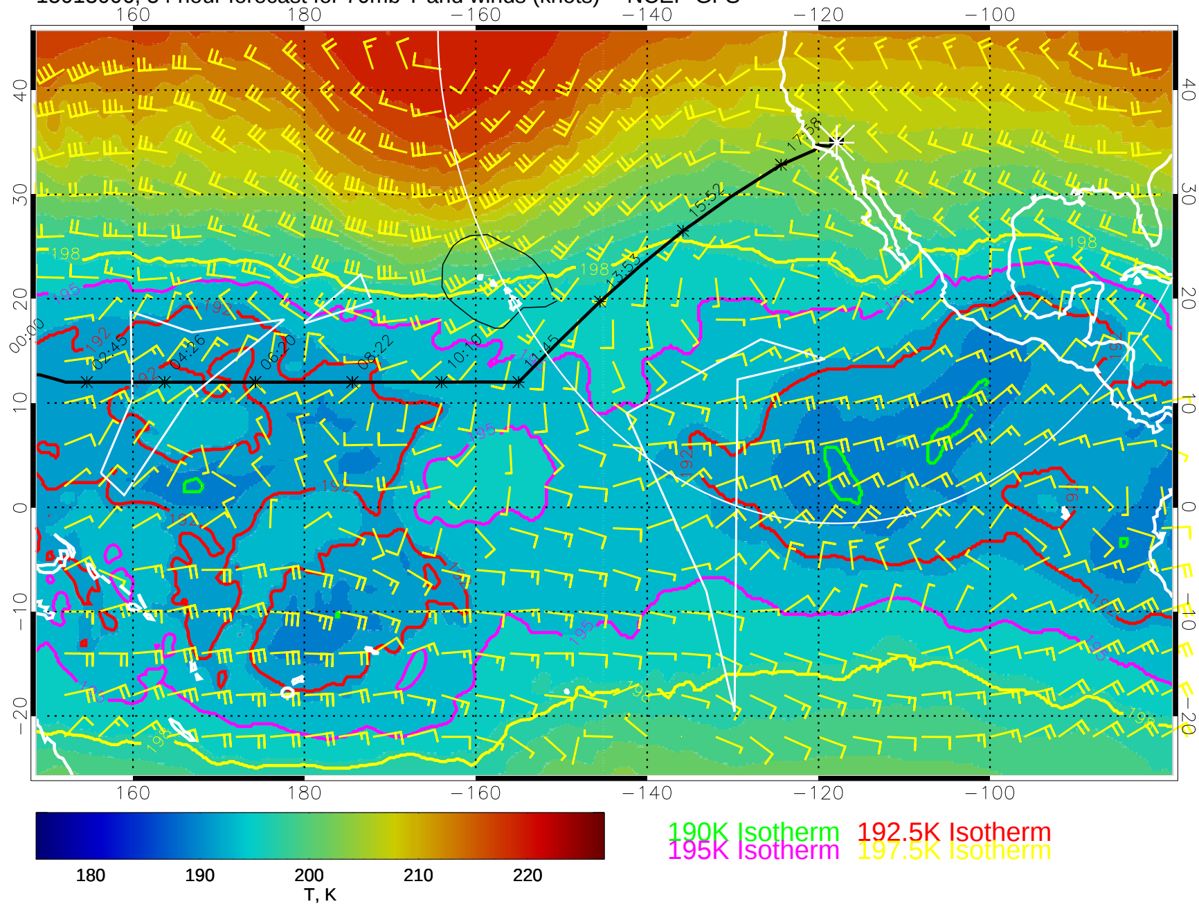
15013006, 54 hour forecast for 70mb T and winds (knots) -- NCEP GFS
