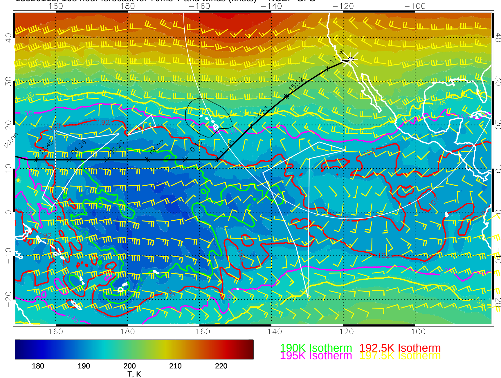
15020112, 108 hour forecast for 70mb T and winds (knots) -- NCEP GFS
