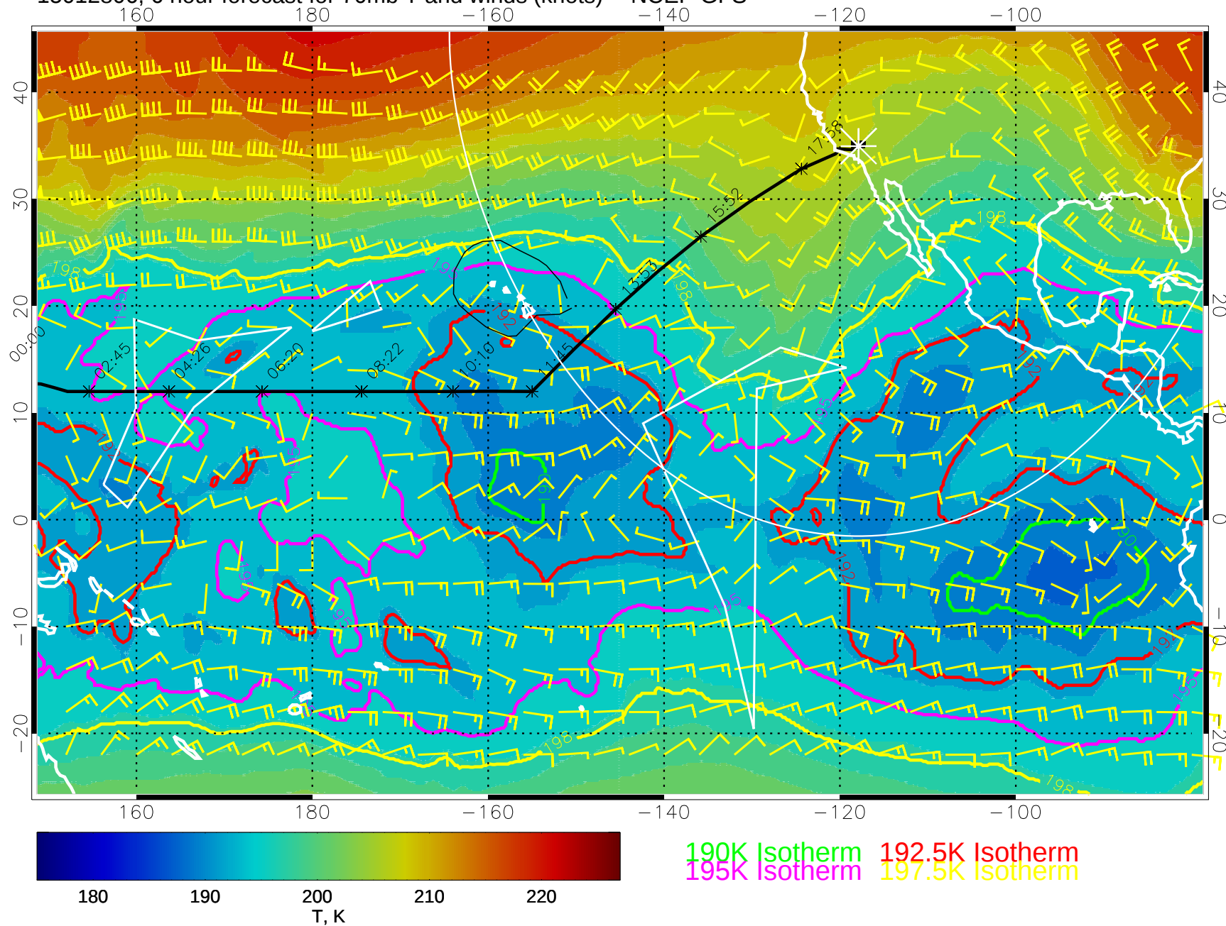
15012806, 6 hour forecast for 70mb T and winds (knots) -- NCEP GFS
