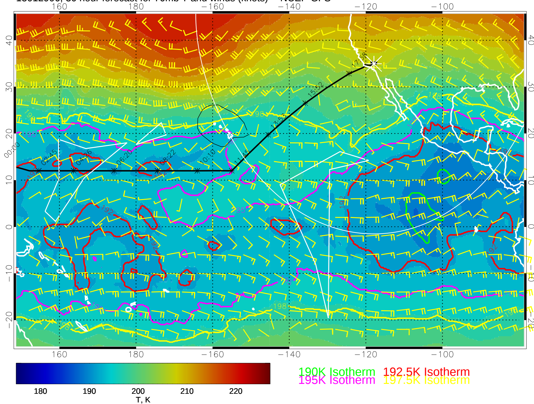
15012906, 30 hour forecast for 70mb T and winds (knots) -- NCEP GFS
