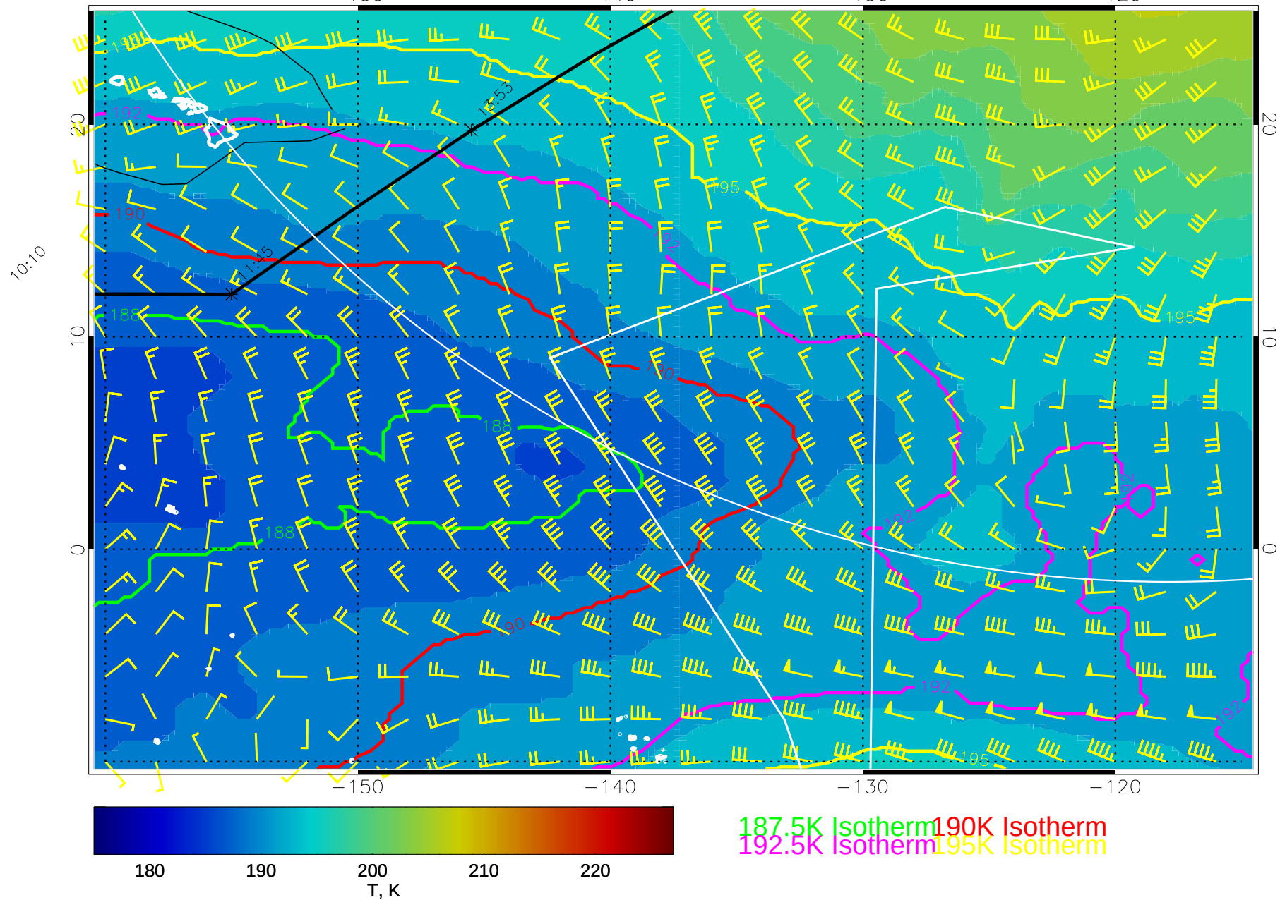
15012818, 18 hour forecast for 100mb T and winds (knots) -- NCEP GFS
