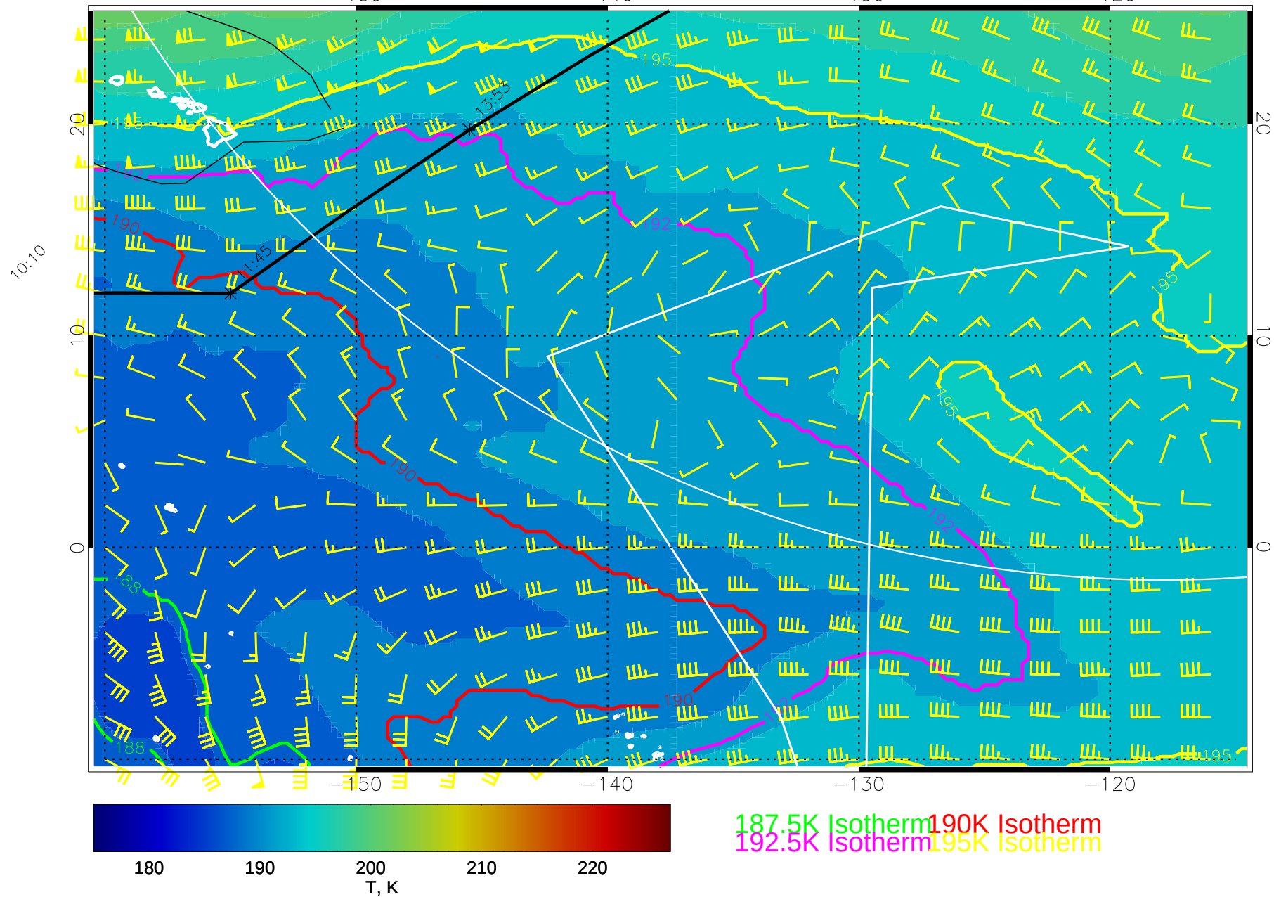
15013100, 72 hour forecast for 100mb T and winds (knots) -- NCEP GFS
