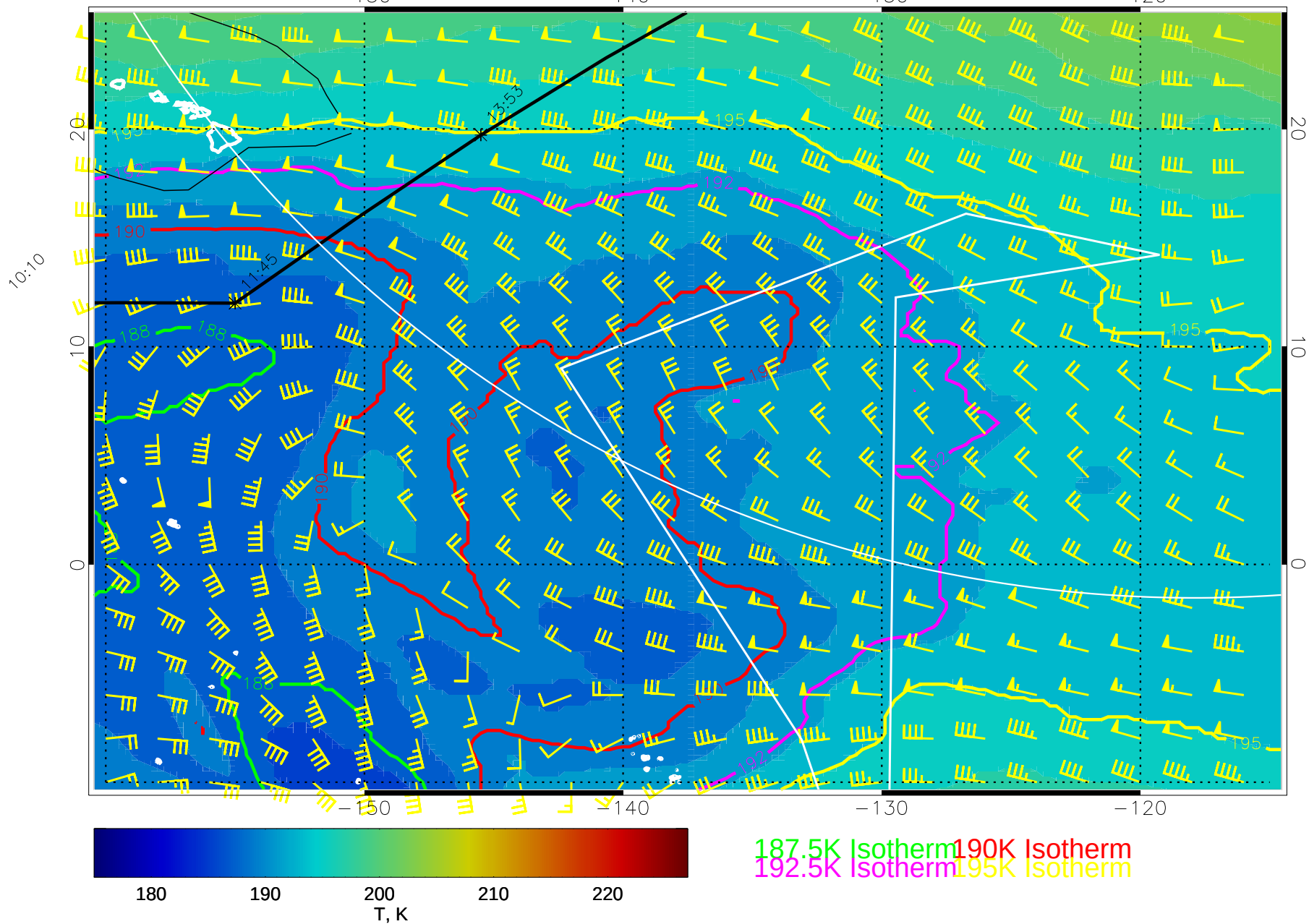
15020112, 108 hour forecast for 100mb T and winds (knots) -- NCEP GFS
