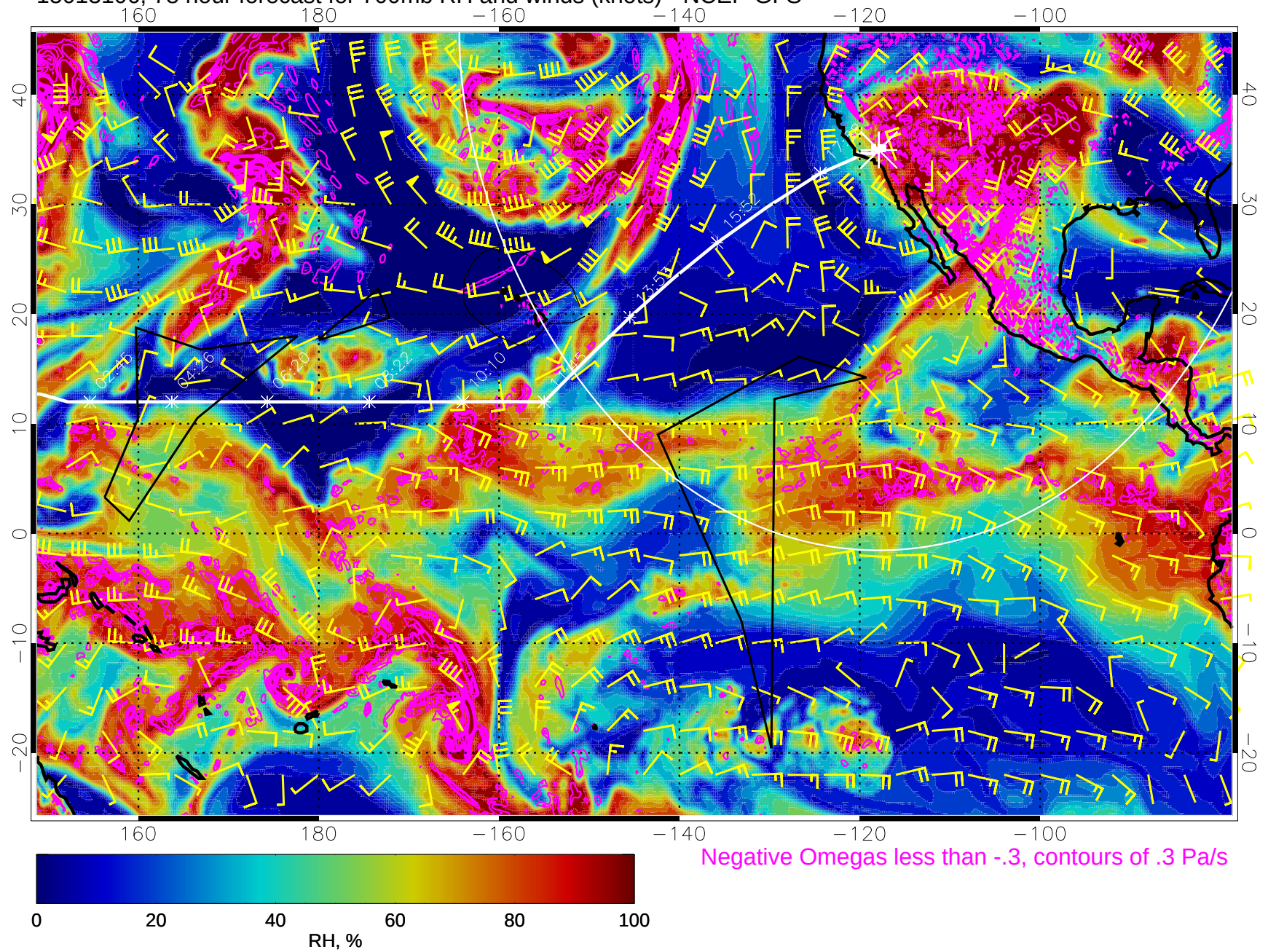
15013106, 78 hour forecast for 700mb RH and winds (knots) - NCEP GFS
