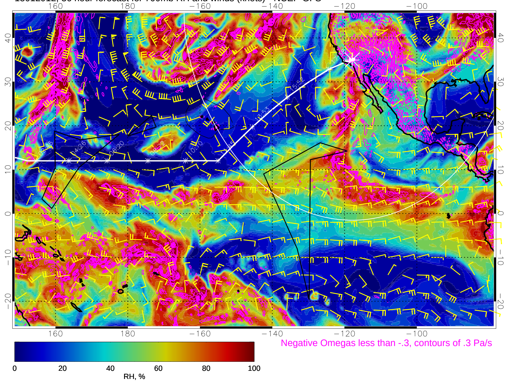
15012912, 36 hour forecast for 700mb RH and winds (knots) - NCEP GFS
