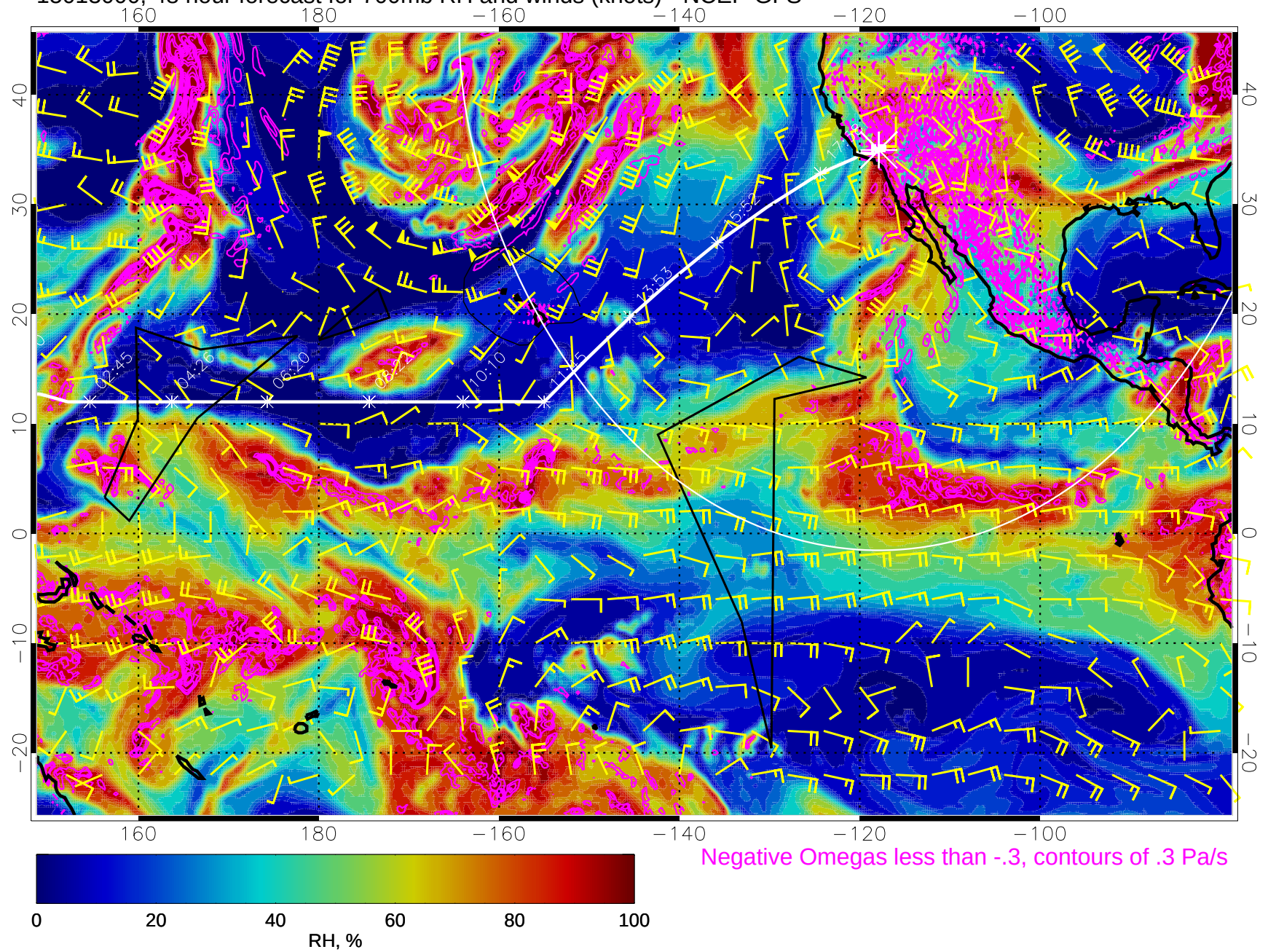
15013000, 48 hour forecast for 700mb RH and winds (knots) - NCEP GFS
