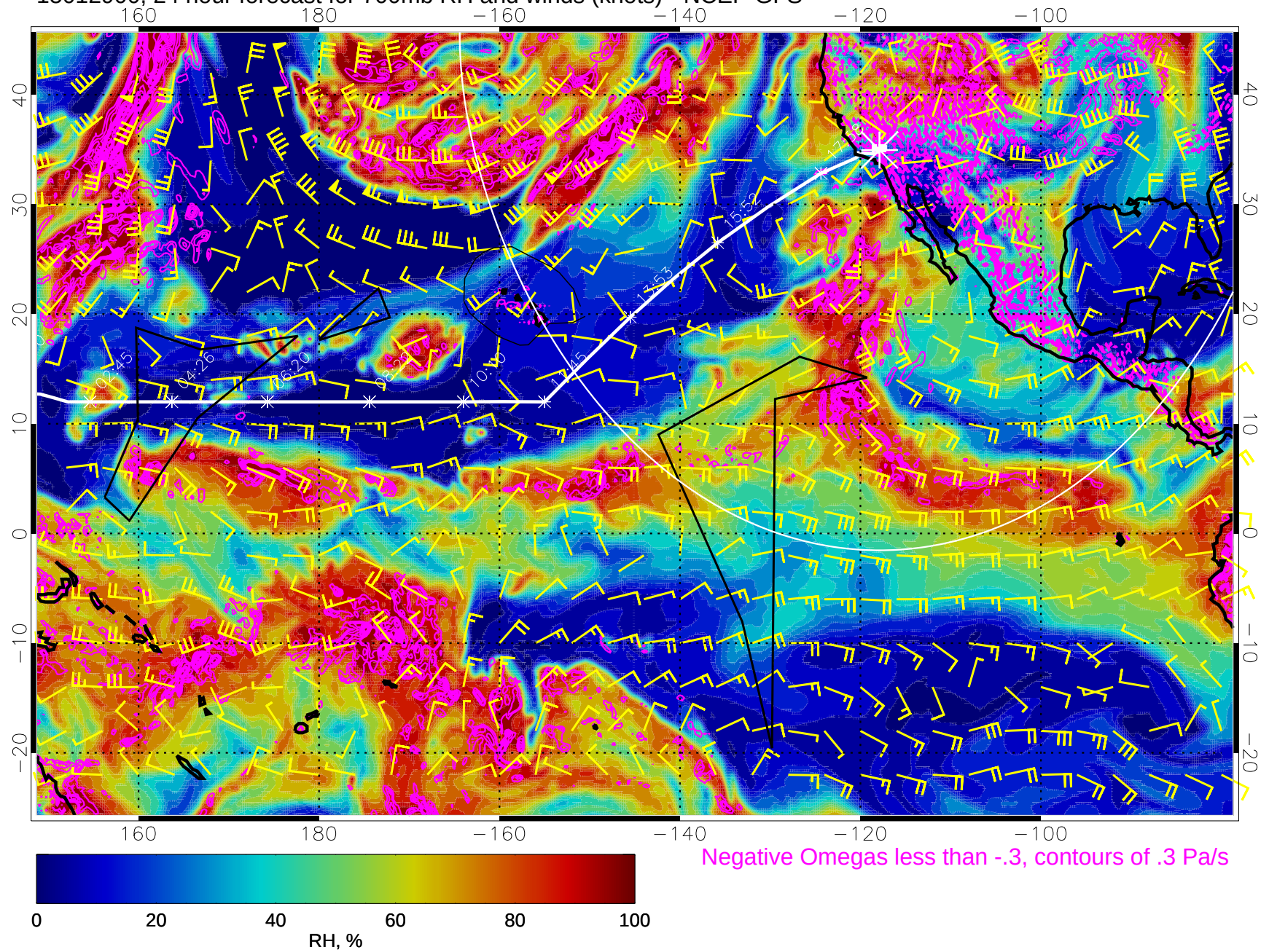
15012900, 24 hour forecast for 700mb RH and winds (knots) - NCEP GFS
