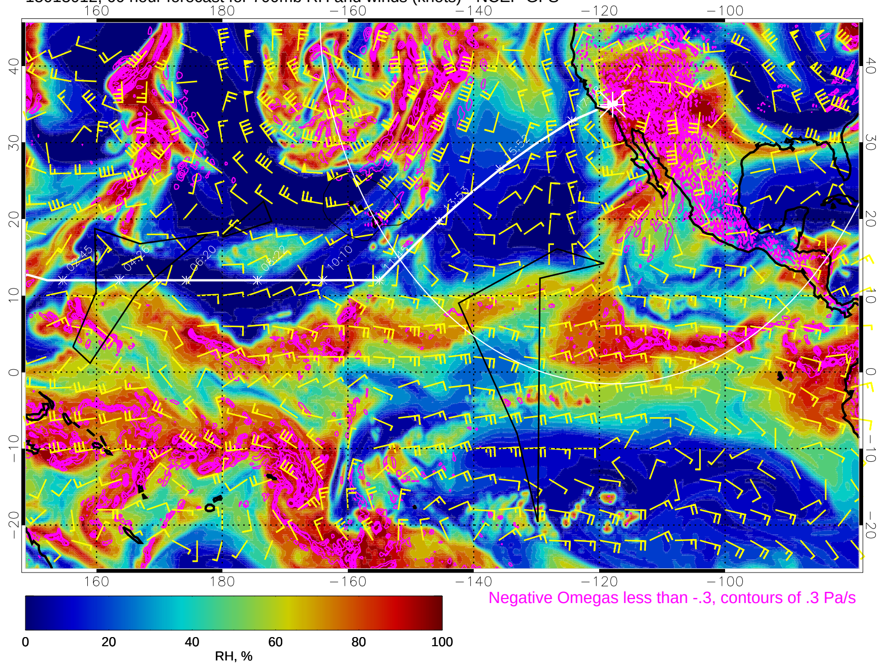
15013012, 60 hour forecast for 700mb RH and winds (knots) - NCEP GFS
