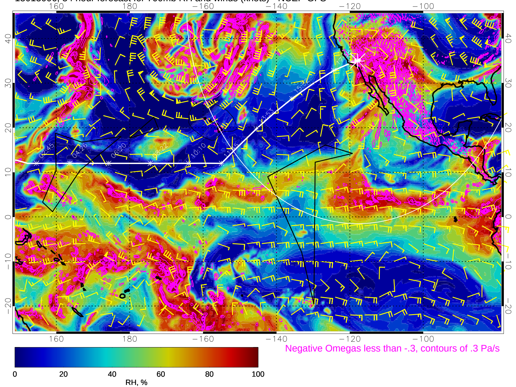
15013006, 54 hour forecast for 700mb RH and winds (knots) - NCEP GFS
