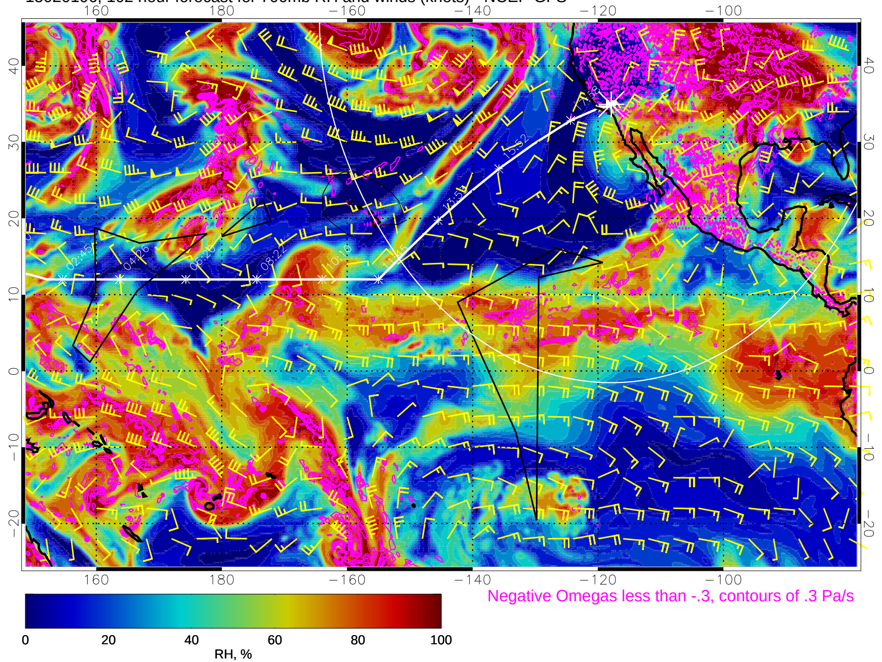
15020106, 102 hour forecast for 700mb RH and winds (knots) - NCEP GFS
