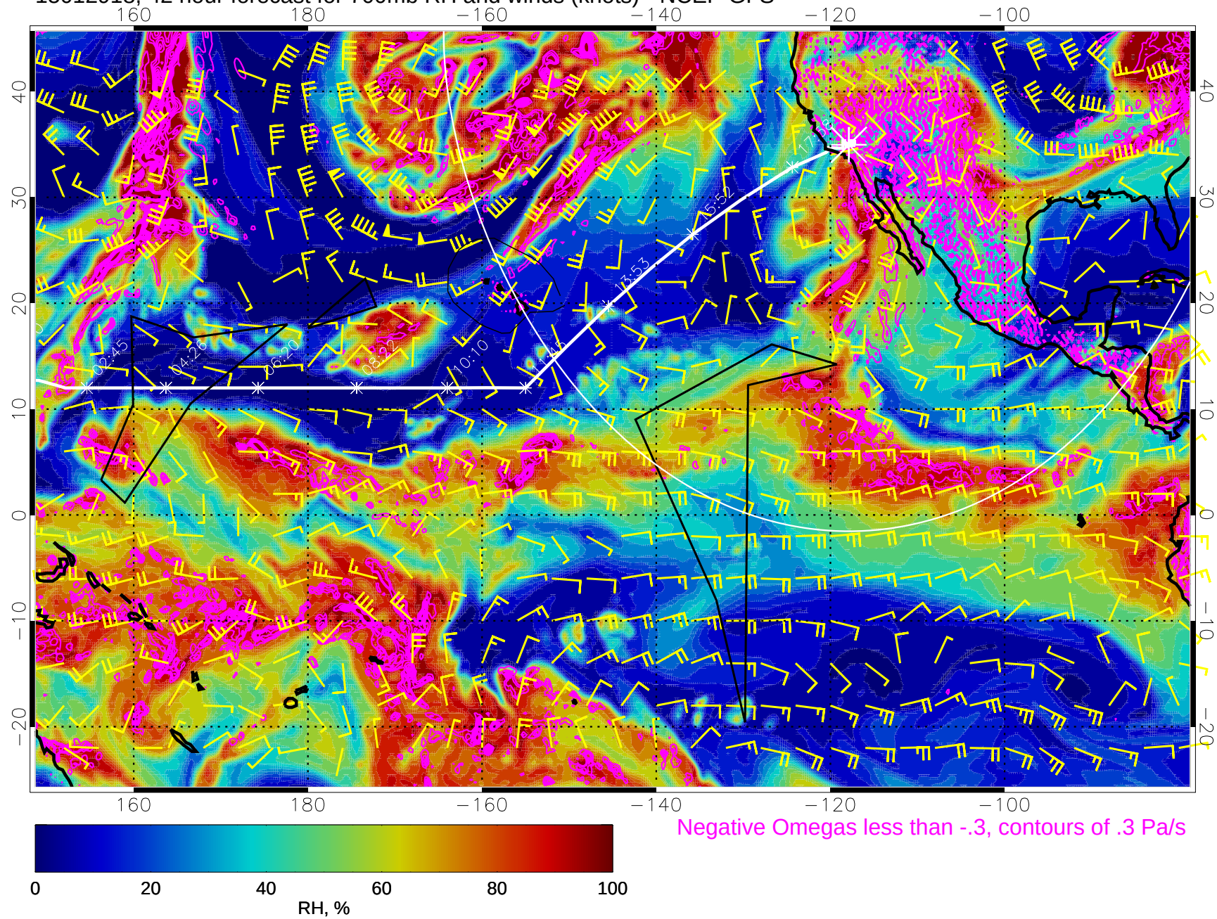
15012918, 42 hour forecast for 700mb RH and winds (knots) - NCEP GFS
