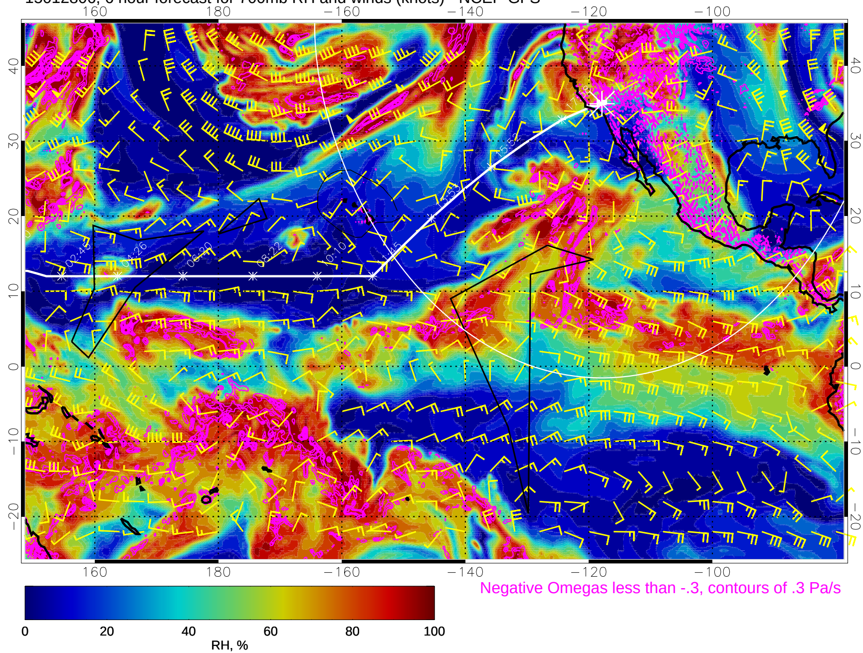
15012806, 6 hour forecast for 700mb RH and winds (knots) - NCEP GFS
