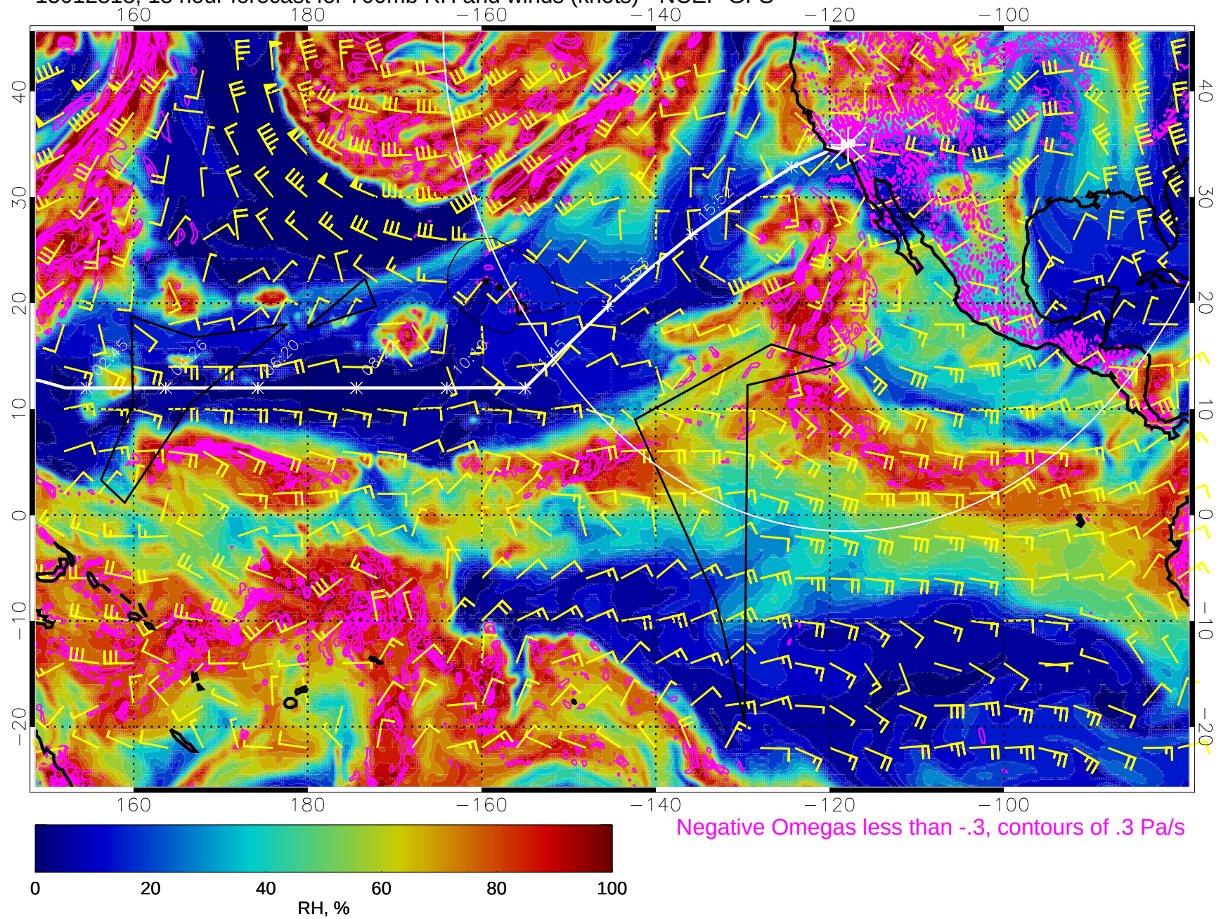
15012818, 18 hour forecast for 700mb RH and winds (knots) - NCEP GFS
