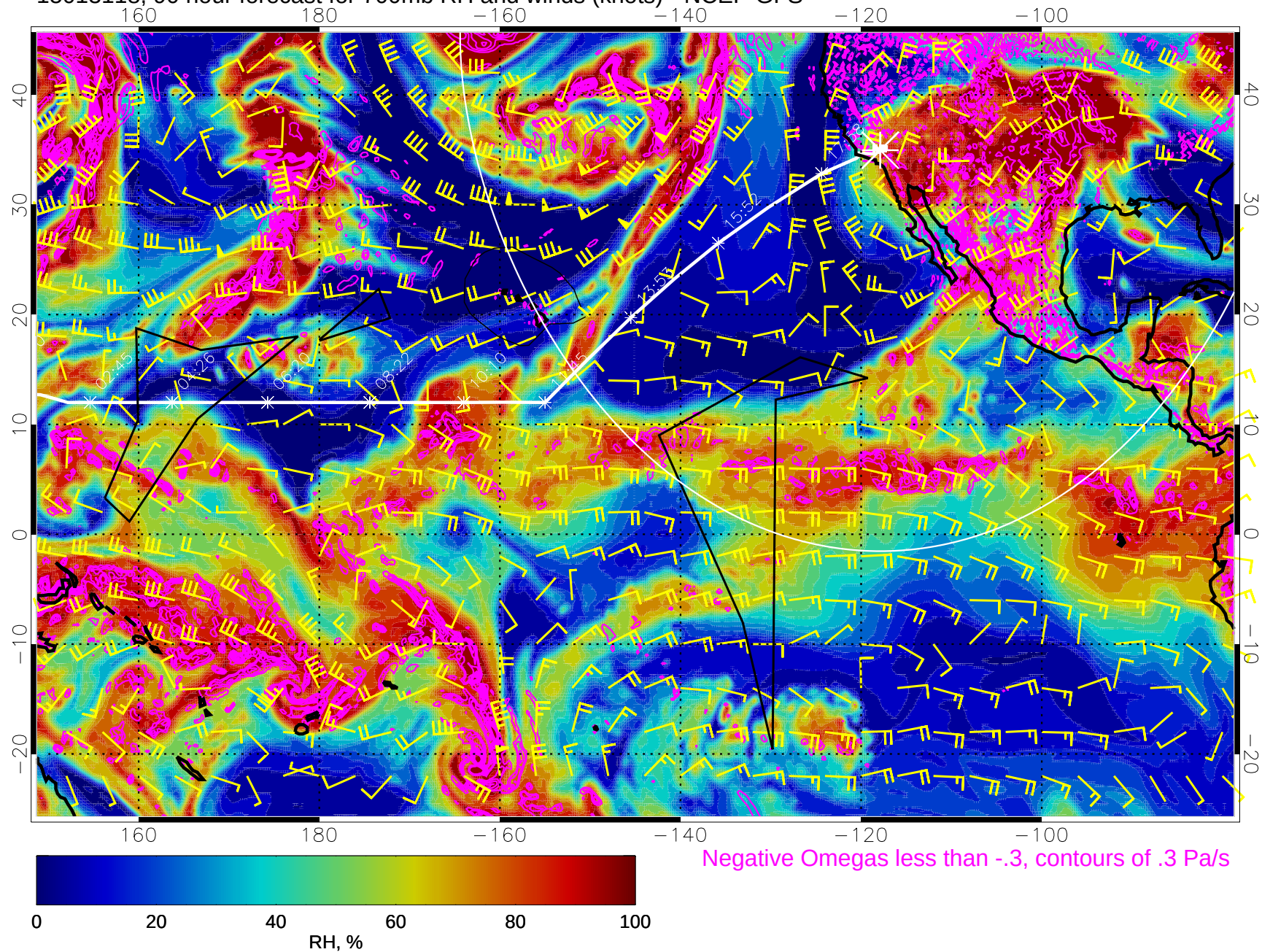
15013118, 90 hour forecast for 700mb RH and winds (knots) - NCEP GFS
