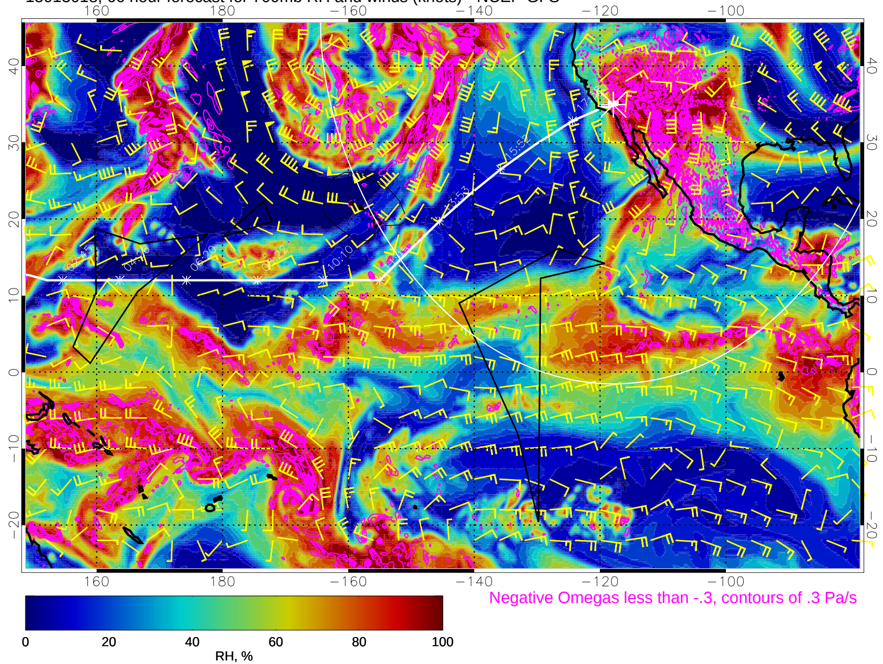
15013018, 66 hour forecast for 700mb RH and winds (knots) - NCEP GFS
