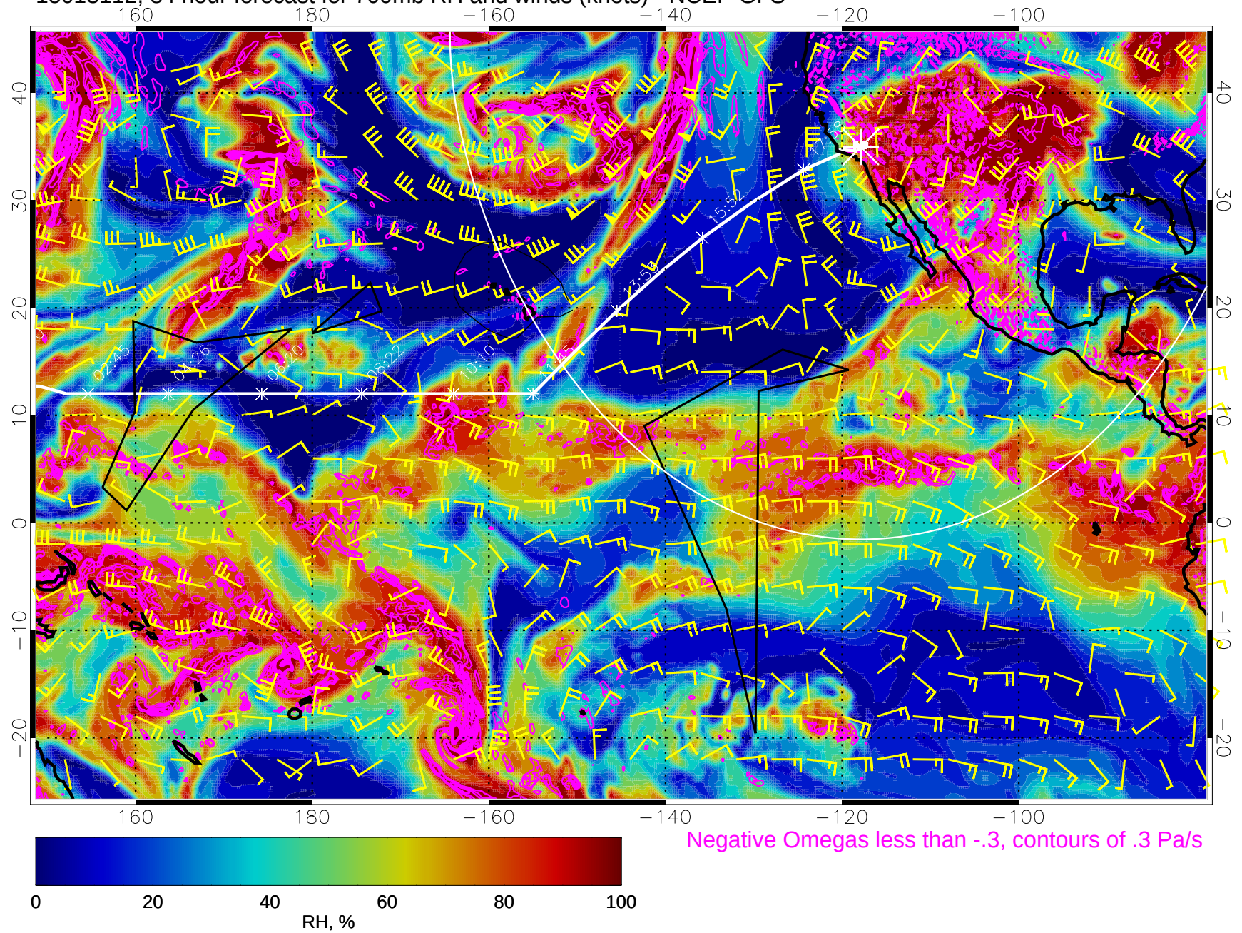
15013112, 84 hour forecast for 700mb RH and winds (knots) - NCEP GFS
