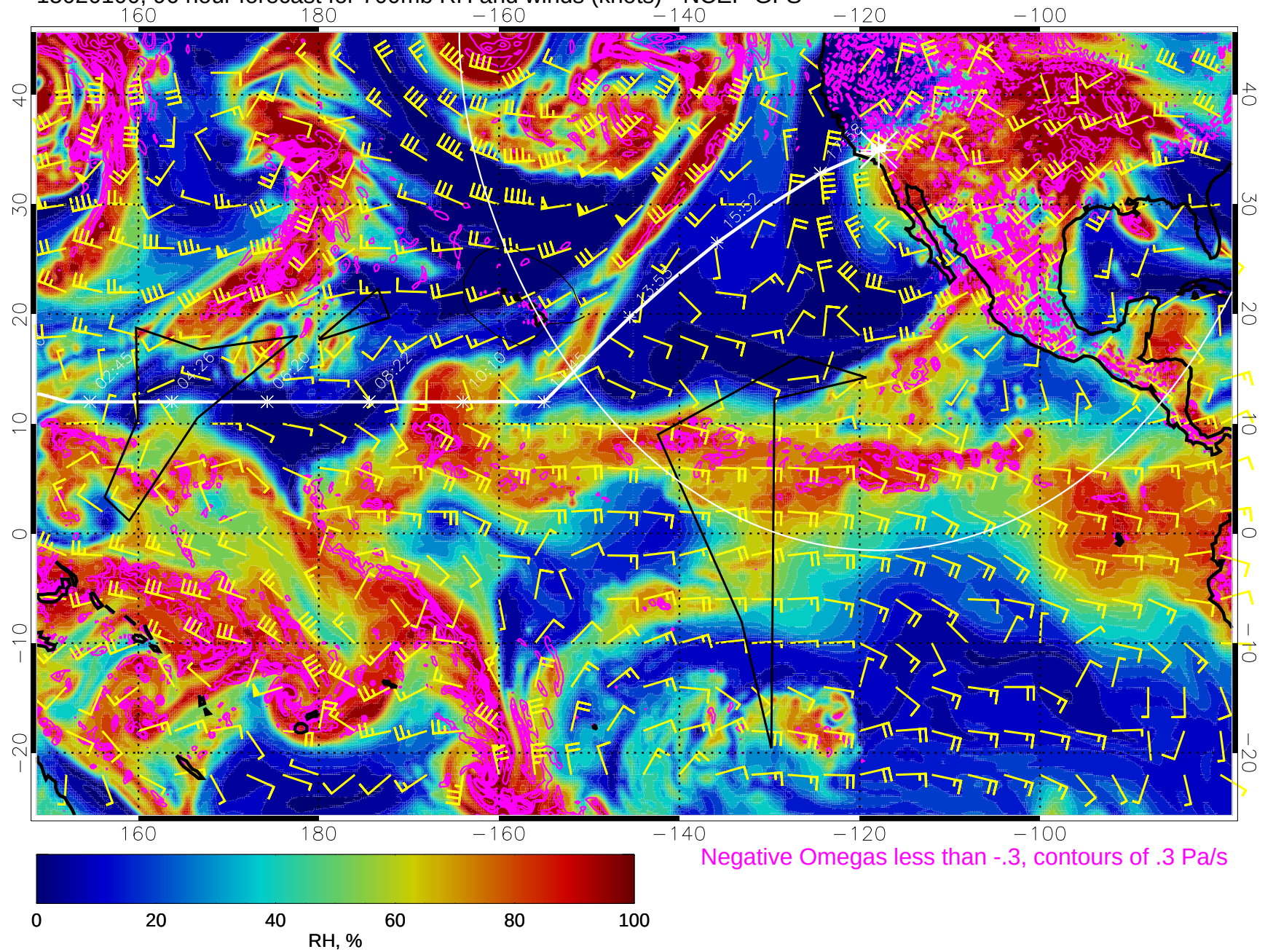
15020100, 96 hour forecast for 700mb RH and winds (knots) - NCEP GFS
