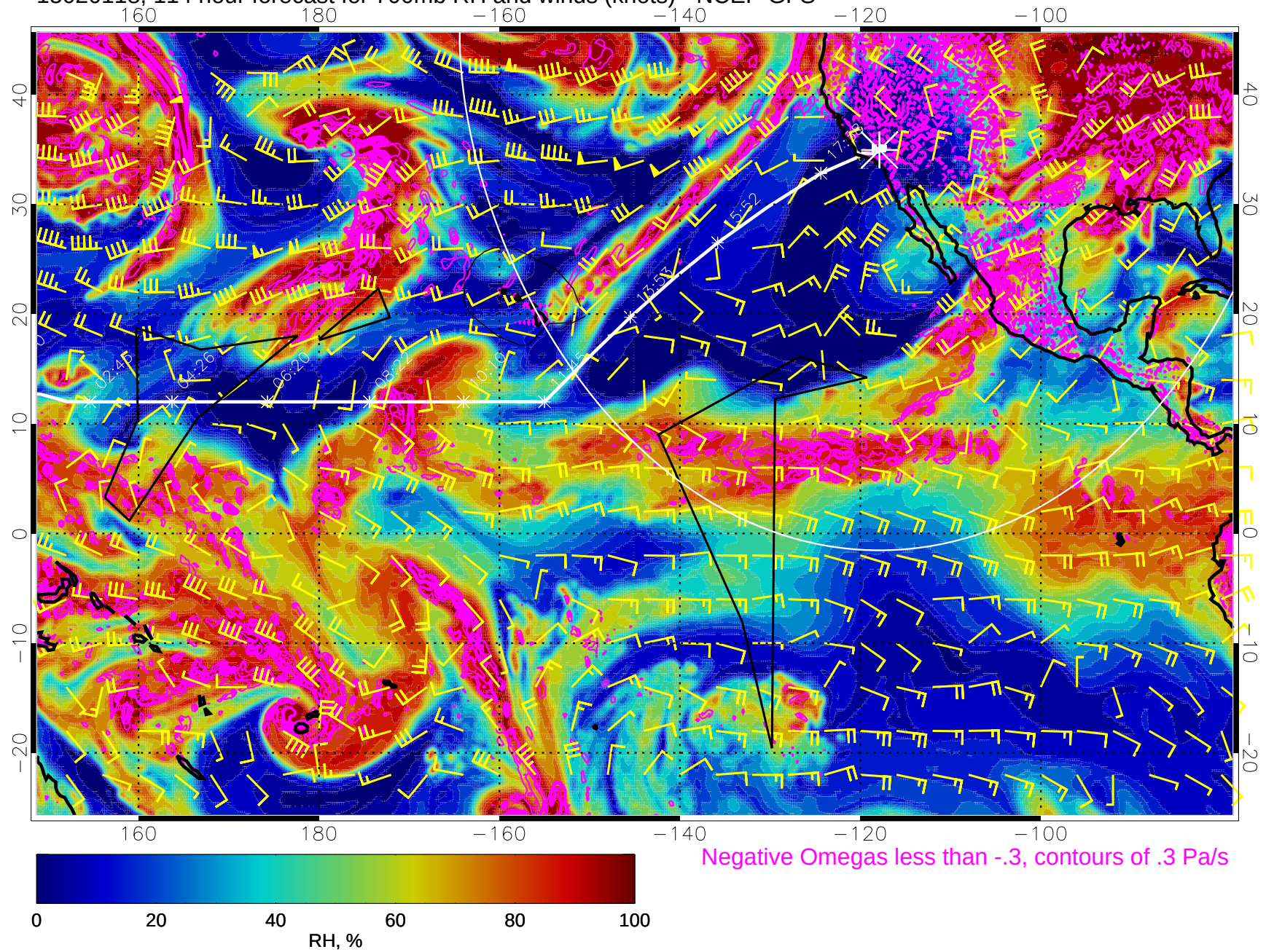
15020118, 114 hour forecast for 700mb RH and winds (knots) - NCEP GFS
