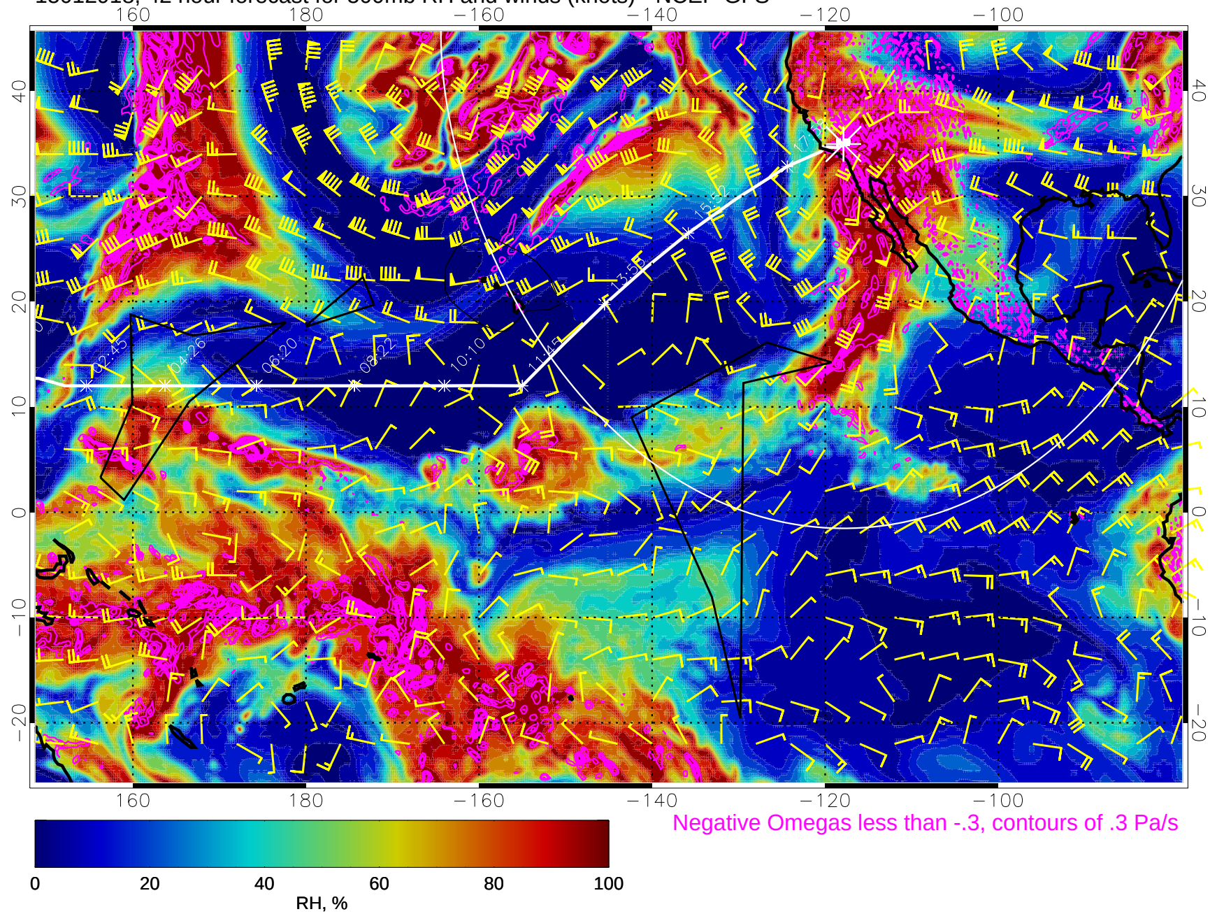
15012918, 42 hour forecast for 500mb RH and winds (knots) - NCEP GFS
