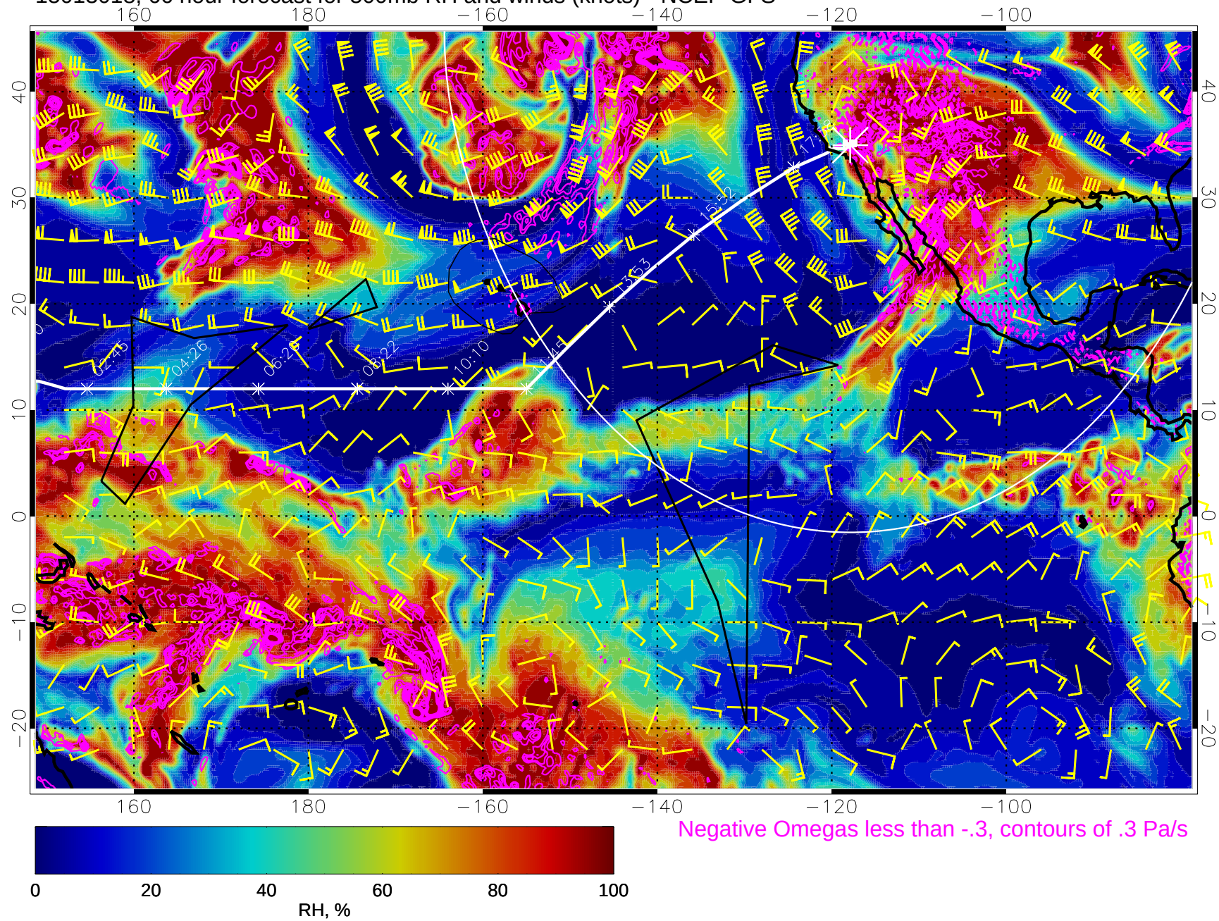
15013018, 66 hour forecast for 500mb RH and winds (knots) - NCEP GFS
