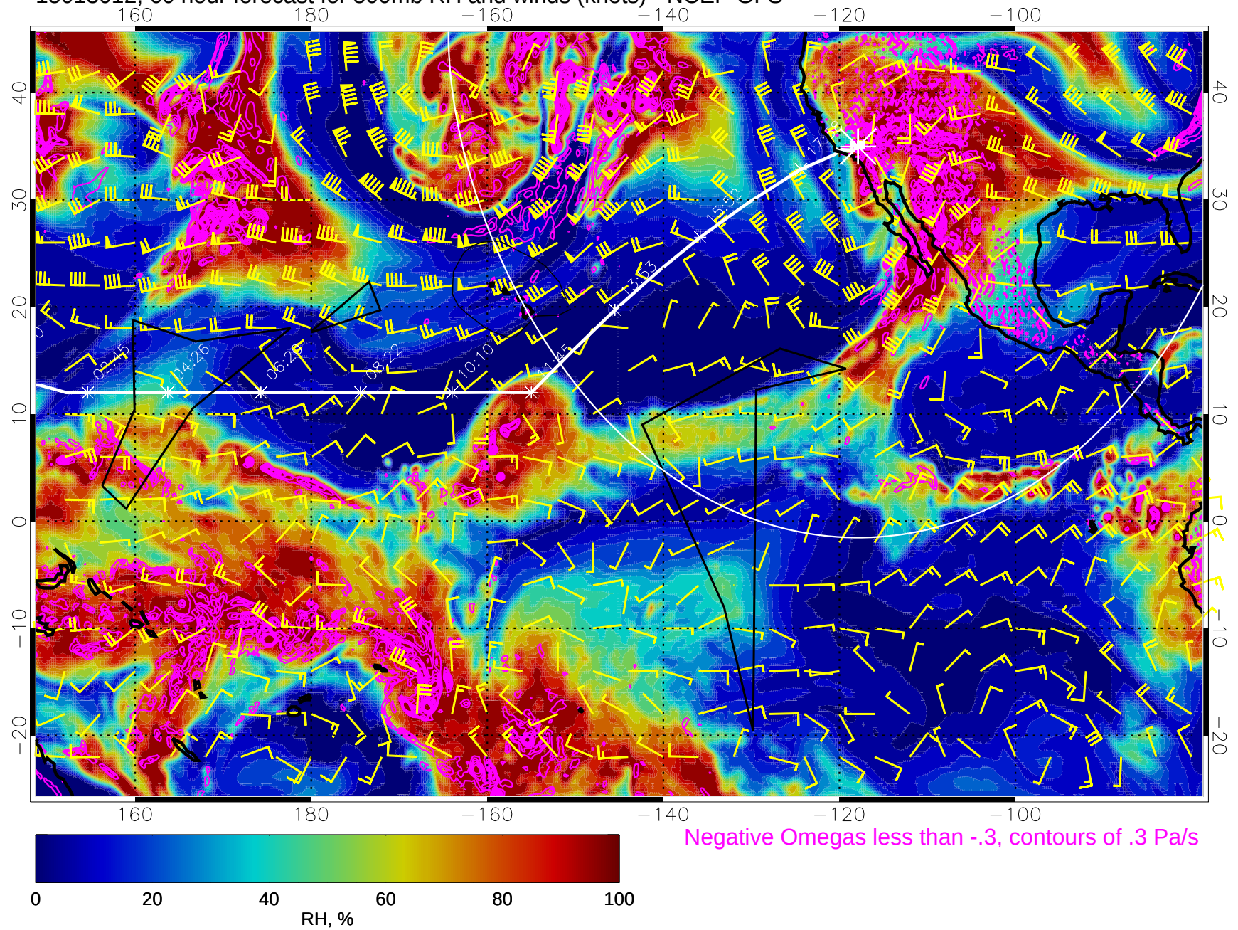
15013012, 60 hour forecast for 500mb RH and winds (knots) - NCEP GFS
