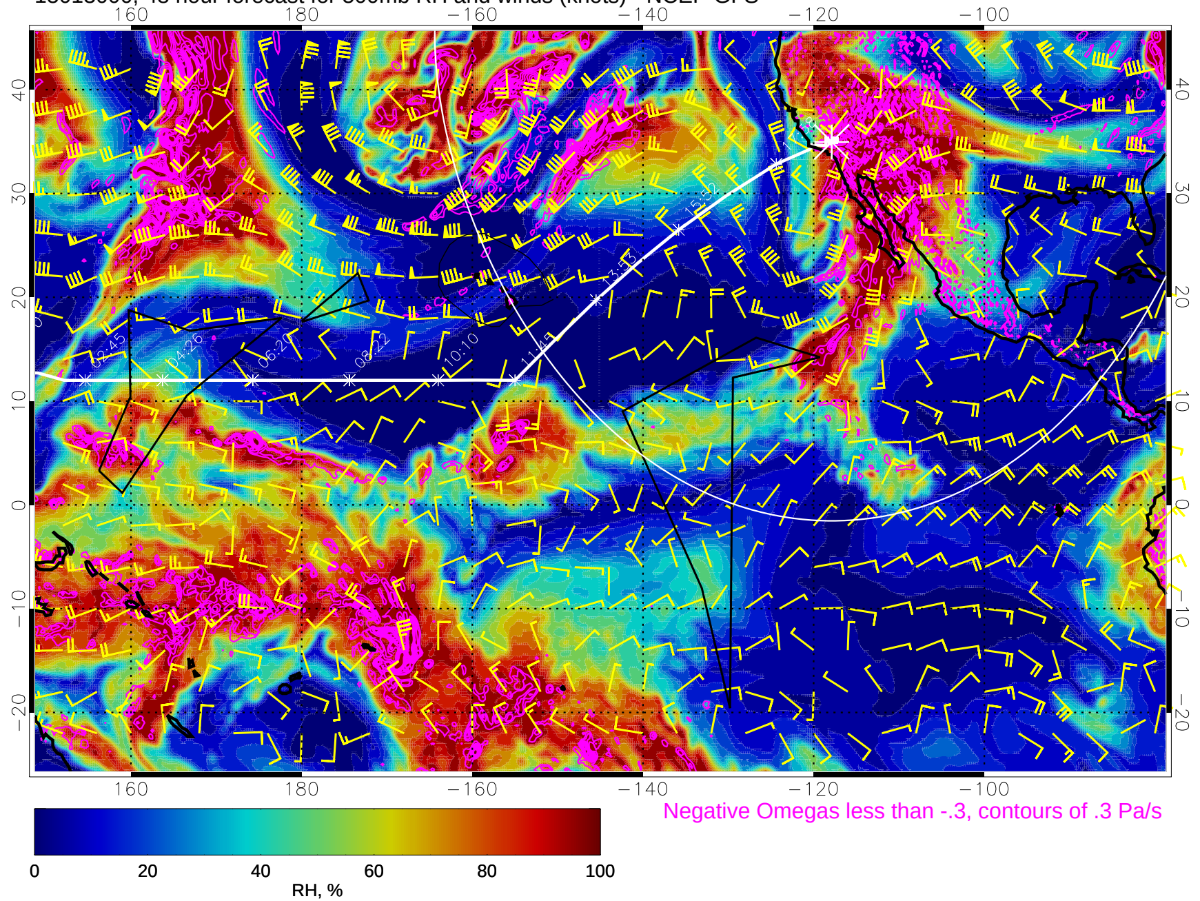
15013000, 48 hour forecast for 500mb RH and winds (knots) - NCEP GFS
