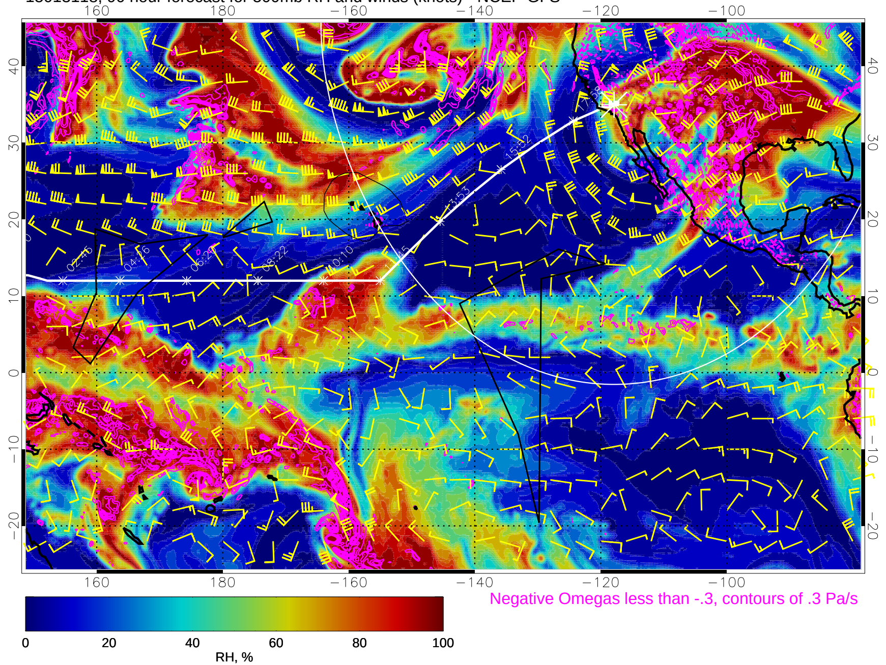
15013118, 90 hour forecast for 500mb RH and winds (knots) - NCEP GFS
