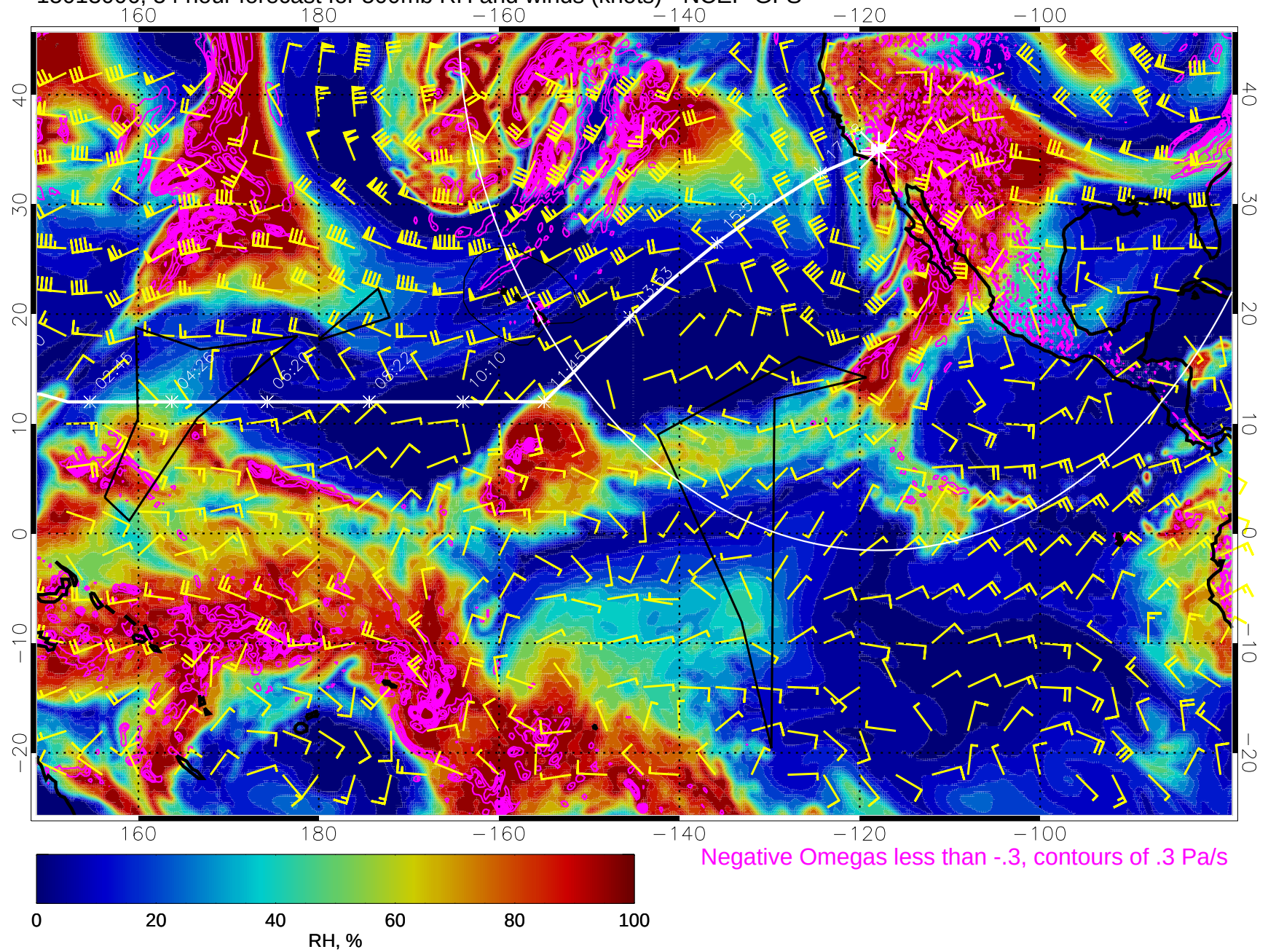
15013006, 54 hour forecast for 500mb RH and winds (knots) - NCEP GFS
