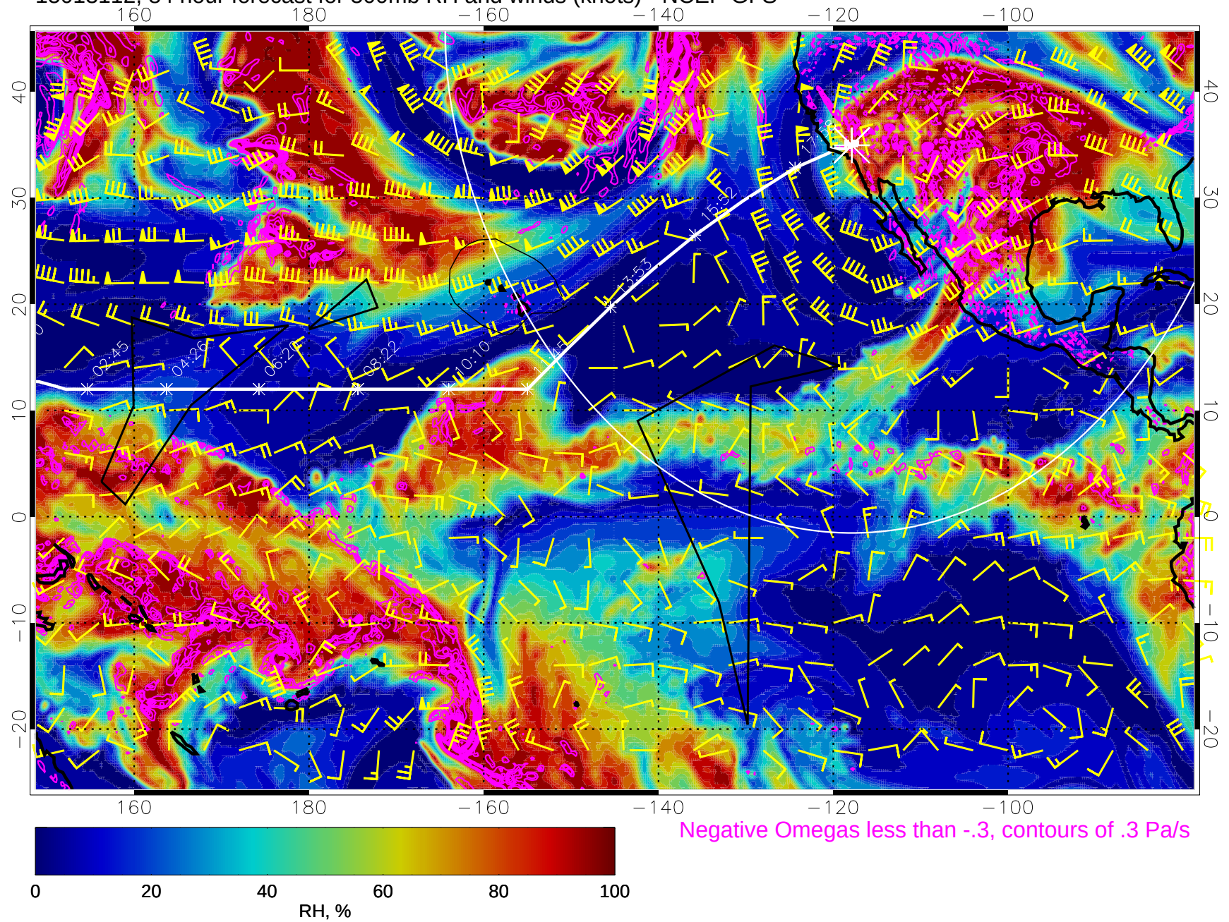
15013112, 84 hour forecast for 500mb RH and winds (knots) - NCEP GFS
