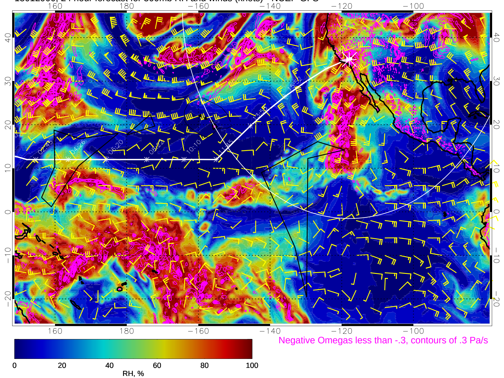
15012900, 24 hour forecast for 500mb RH and winds (knots) - NCEP GFS
