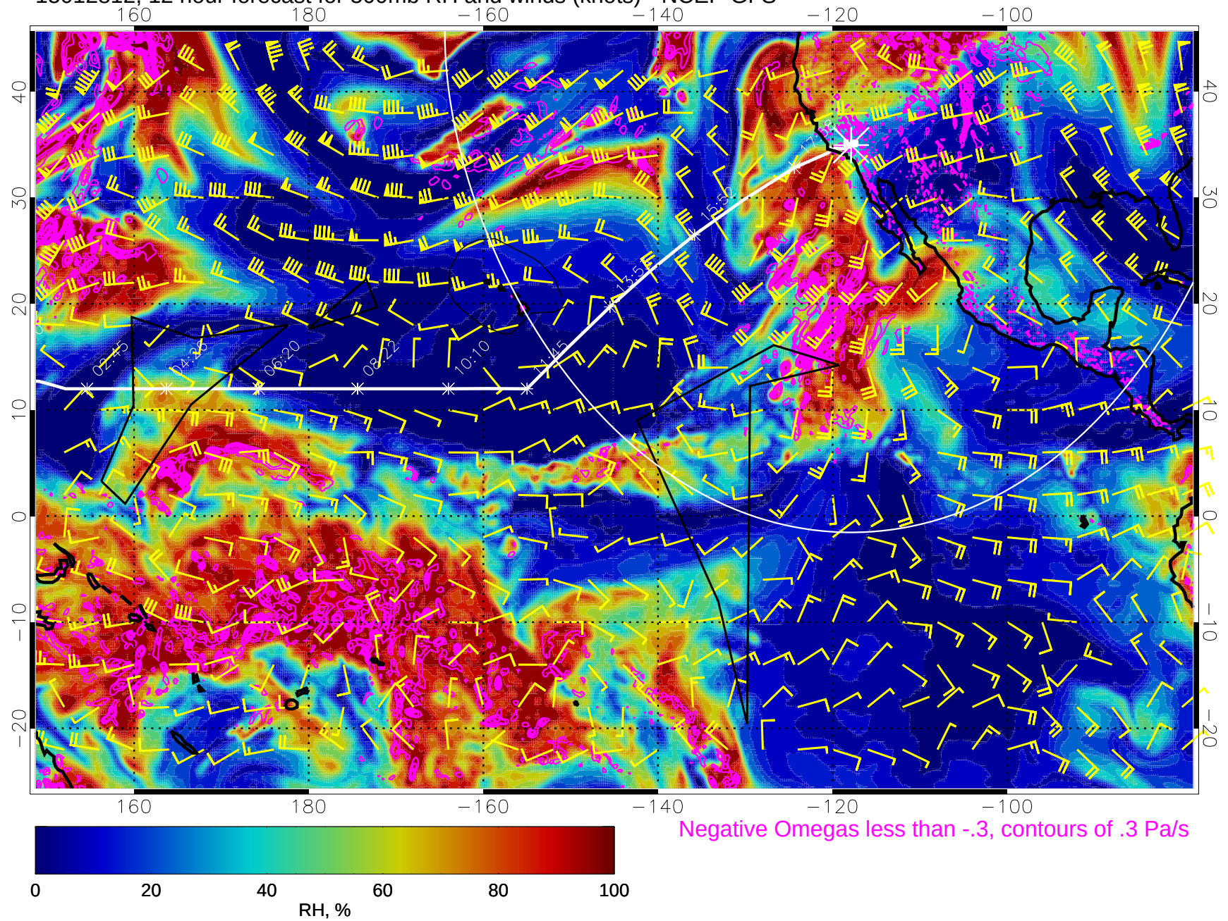
15012812, 12 hour forecast for 500mb RH and winds (knots) - NCEP GFS
