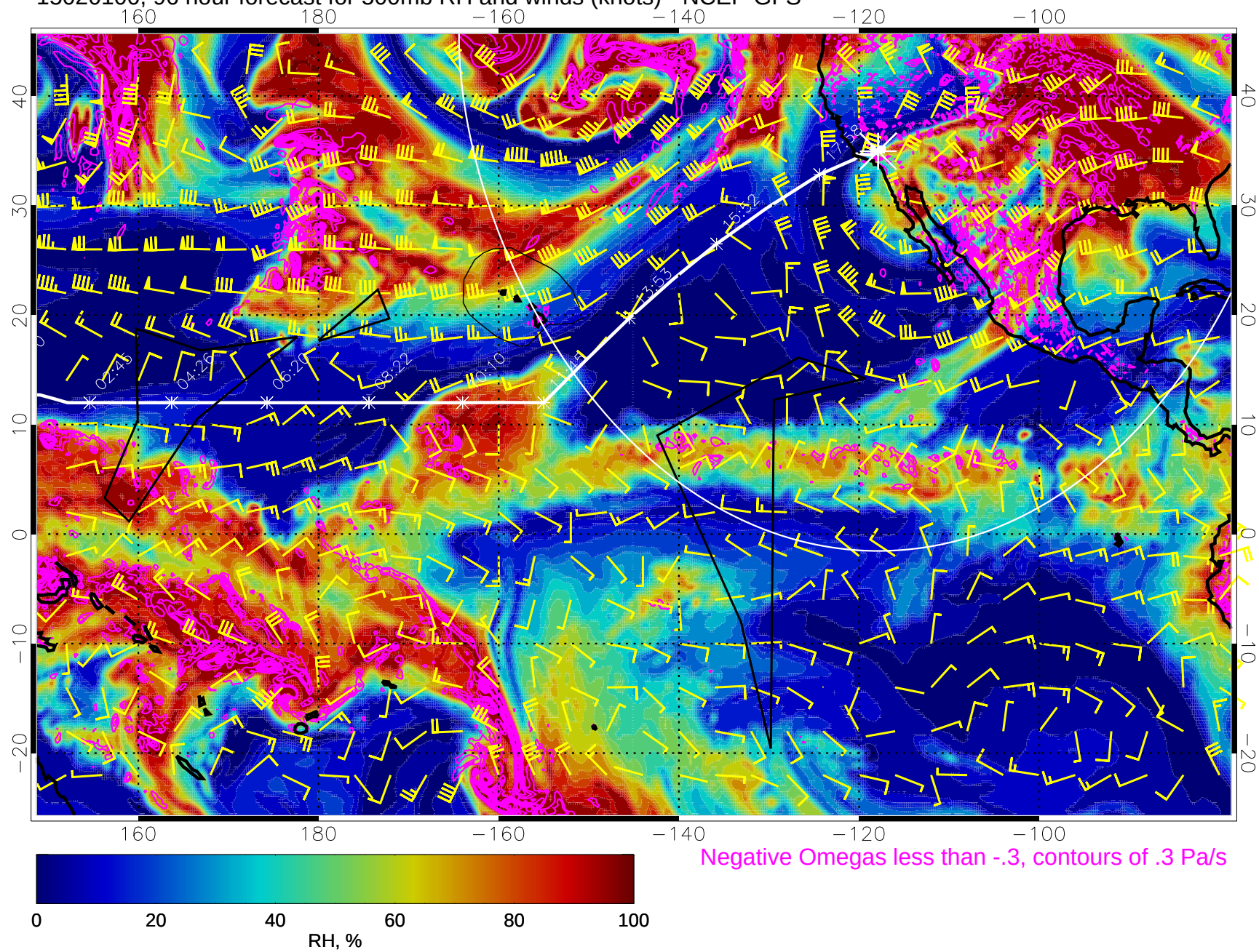
15020100, 96 hour forecast for 500mb RH and winds (knots) - NCEP GFS
