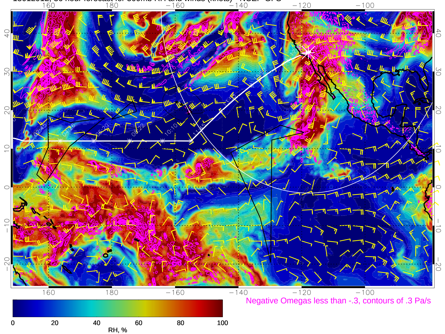
15012912, 36 hour forecast for 500mb RH and winds (knots) - NCEP GFS
