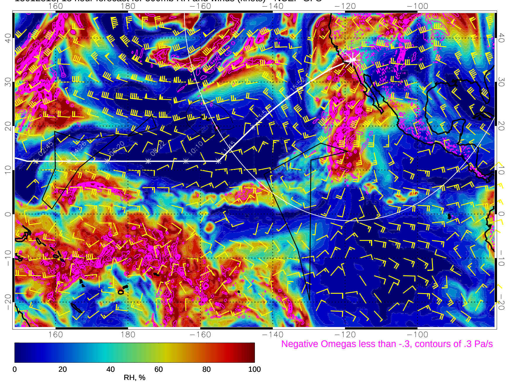
15012818, 18 hour forecast for 500mb RH and winds (knots) - NCEP GFS
