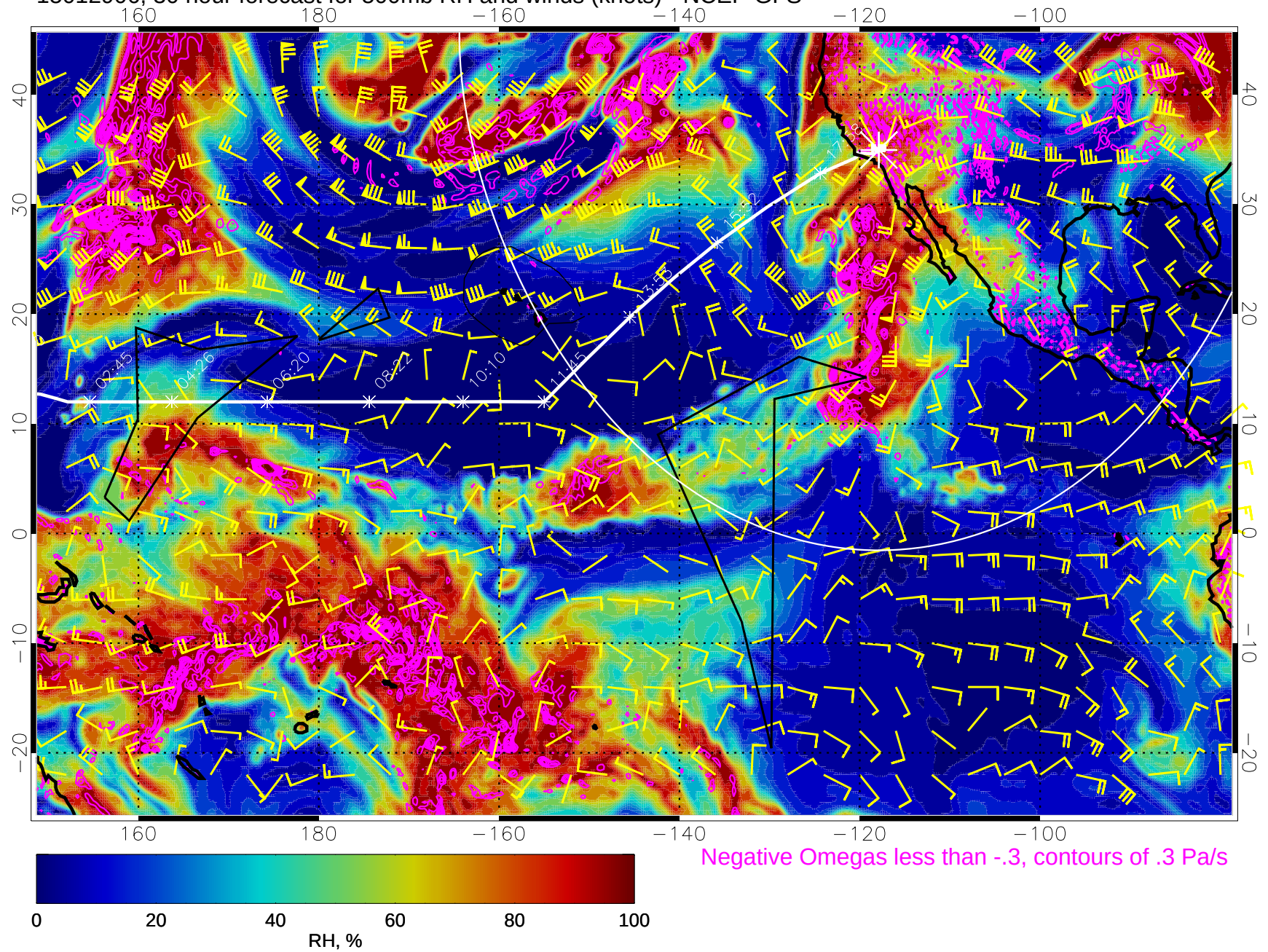
15012906, 30 hour forecast for 500mb RH and winds (knots) - NCEP GFS
