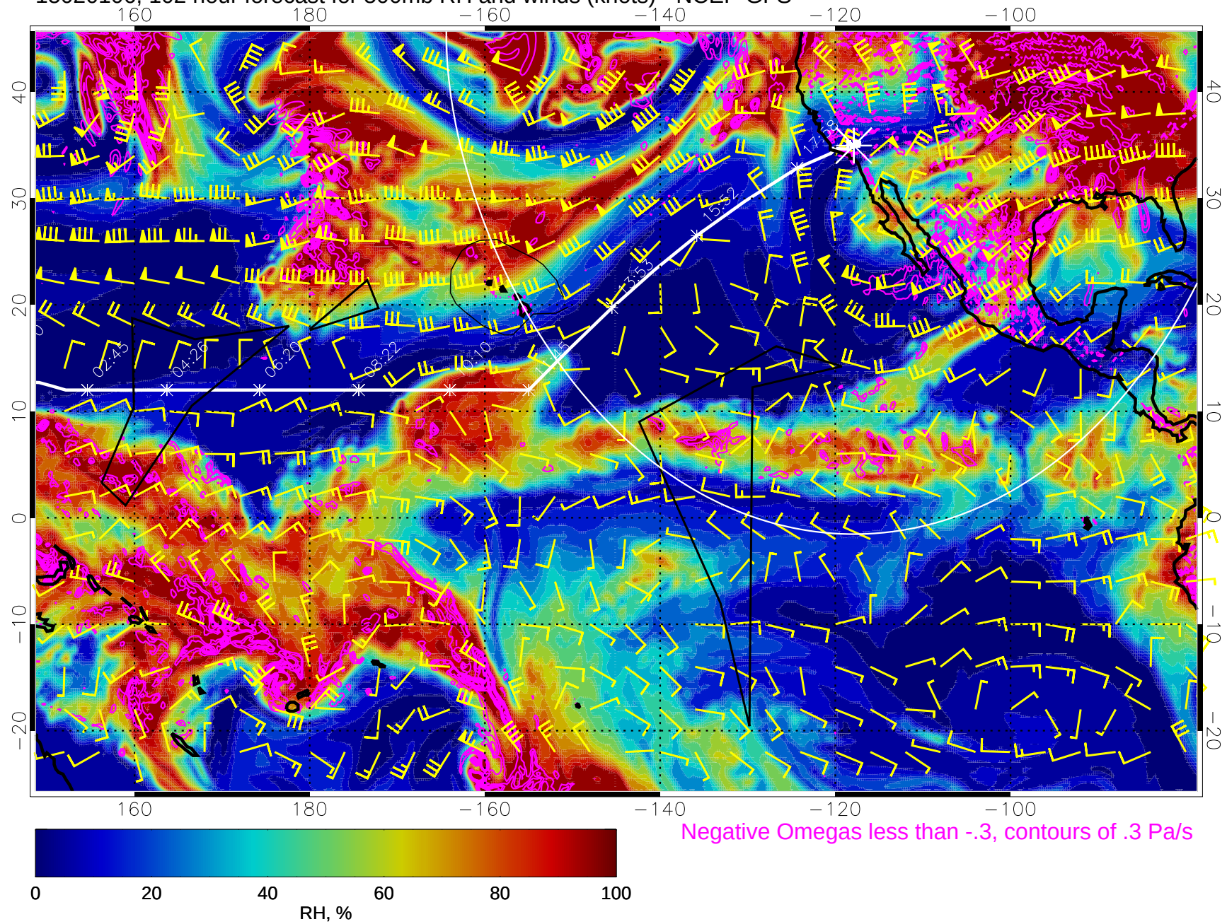
15020106, 102 hour forecast for 500mb RH and winds (knots) - NCEP GFS
