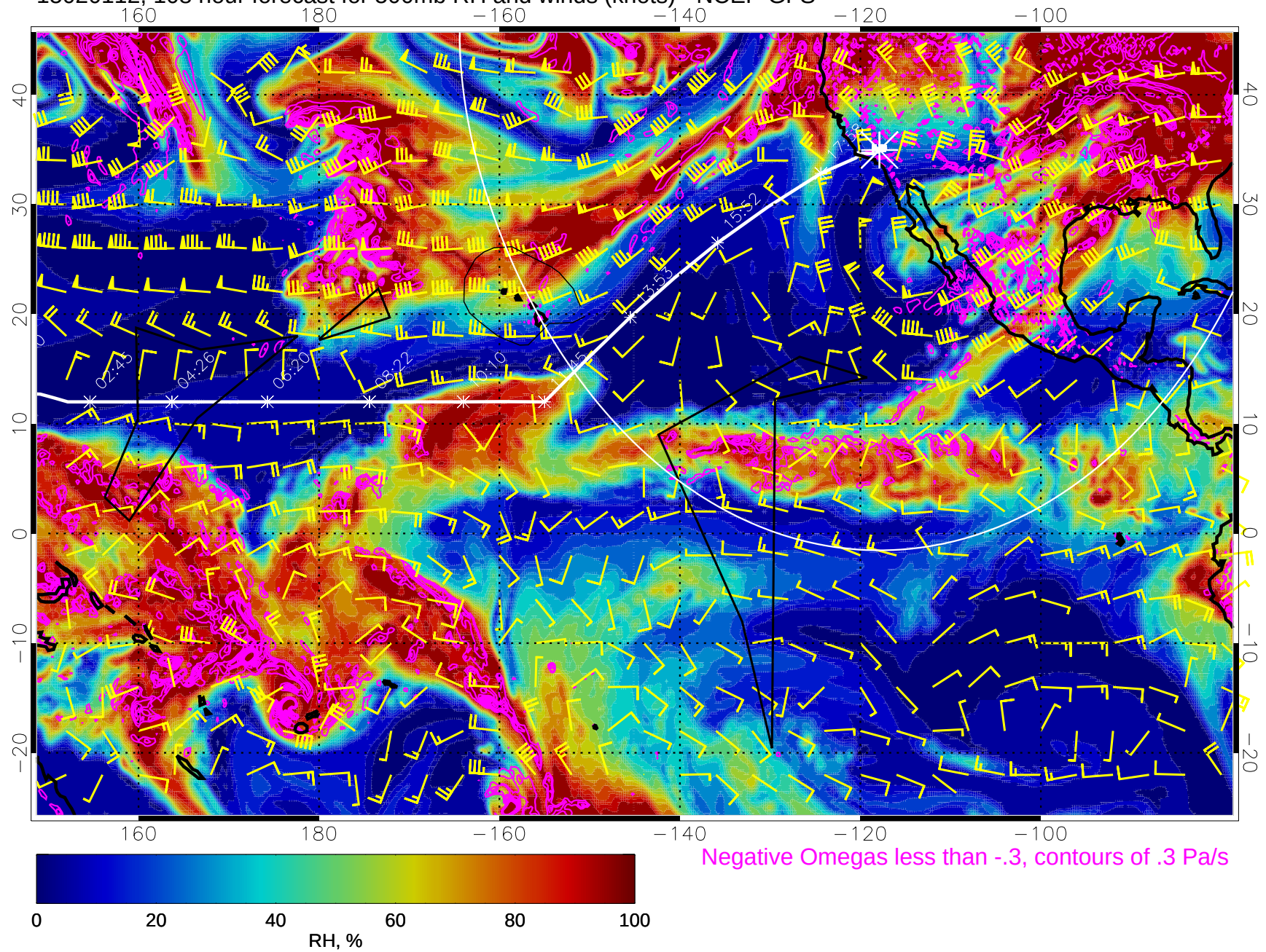
15020112, 108 hour forecast for 500mb RH and winds (knots) - NCEP GFS
