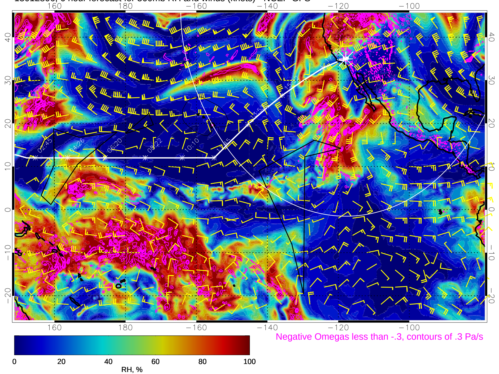
15012806, 6 hour forecast for 500mb RH and winds (knots) - NCEP GFS
