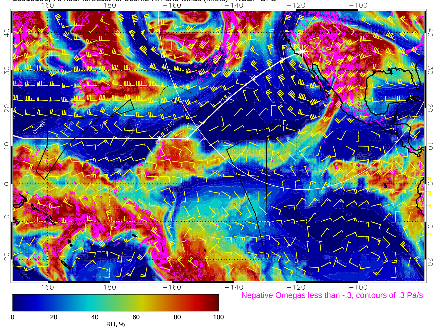
15013106, 78 hour forecast for 500mb RH and winds (knots) - NCEP GFS
