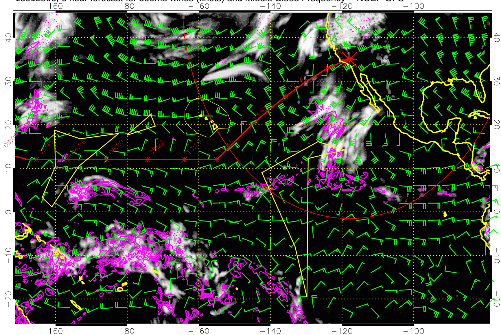
15012806, 6 hour forecast for 500mb winds (knots) and Middle Cloud Frequency -- NCEP GFS
