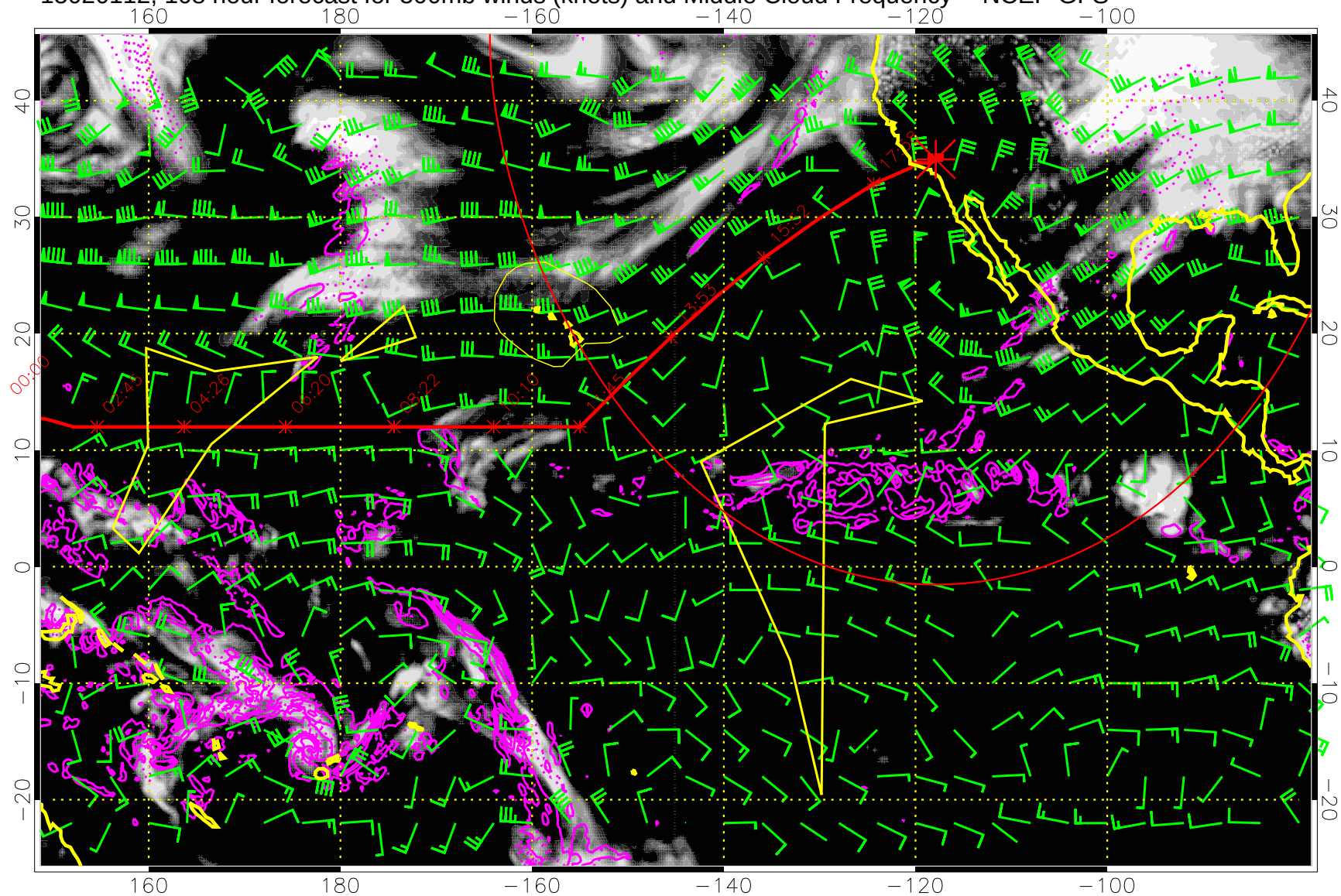
15020112, 108 hour forecast for 500mb winds (knots) and Middle Cloud Frequency -- NCEP GFS
