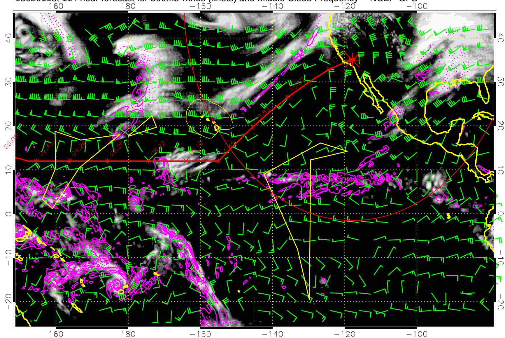
15020118, 114 hour forecast for 500mb winds (knots) and Middle Cloud Frequency -- NCEP GFS
