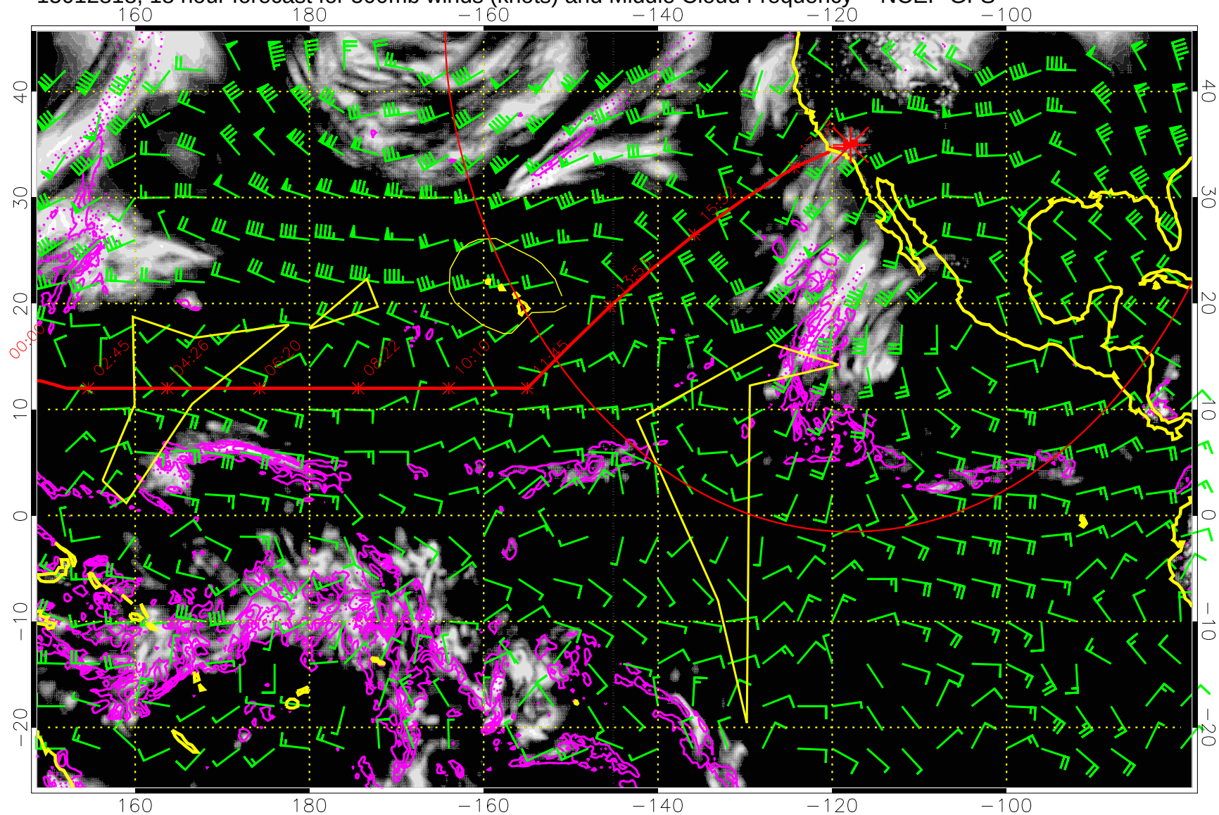
15012818, 18 hour forecast for 500mb winds (knots) and Middle Cloud Frequency -- NCEP GFS
