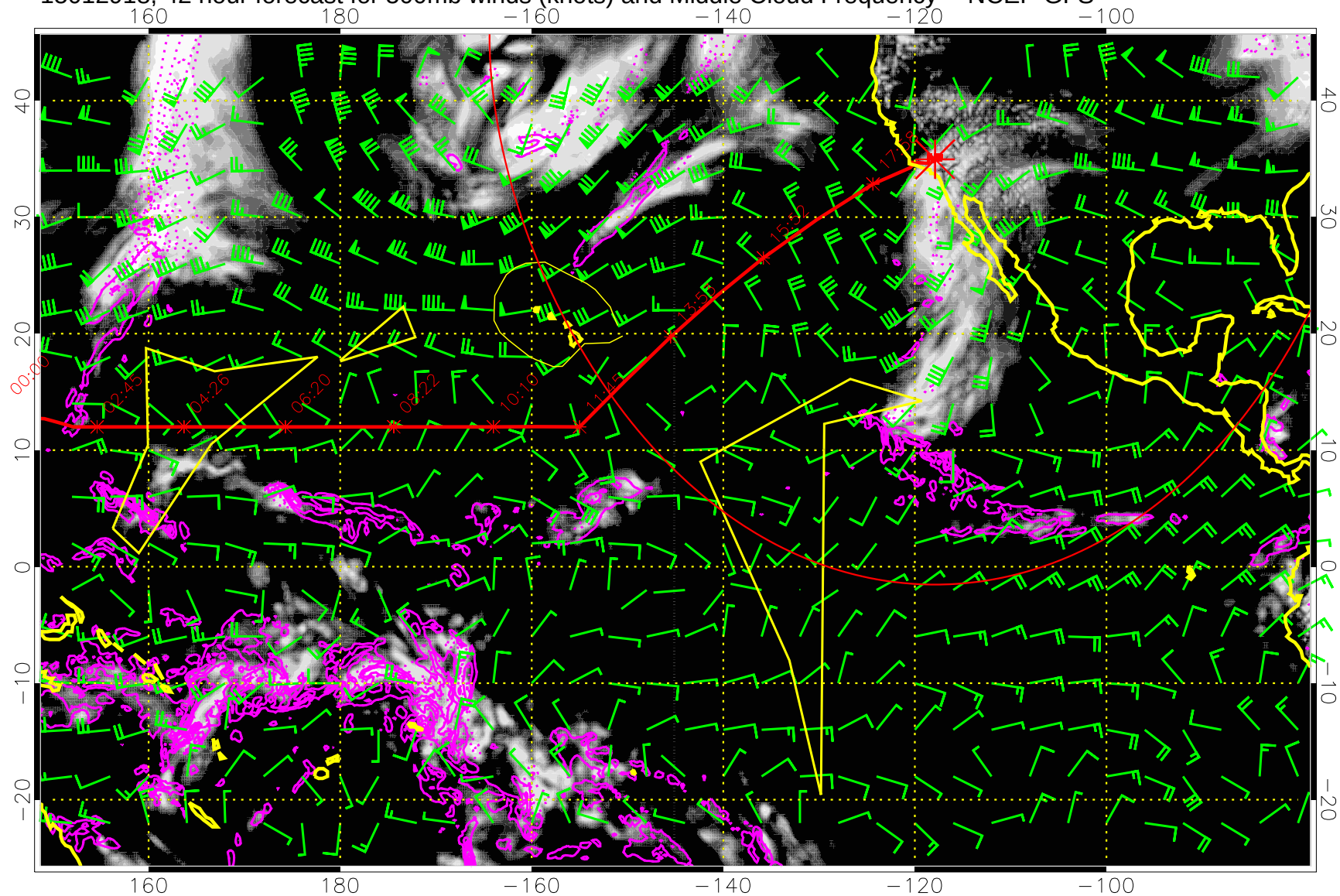
15012918, 42 hour forecast for 500mb winds (knots) and Middle Cloud Frequency -- NCEP GFS
