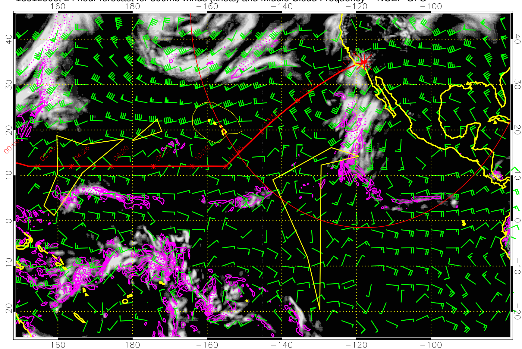
15012900, 24 hour forecast for 500mb winds (knots) and Middle Cloud Frequency -- NCEP GFS
