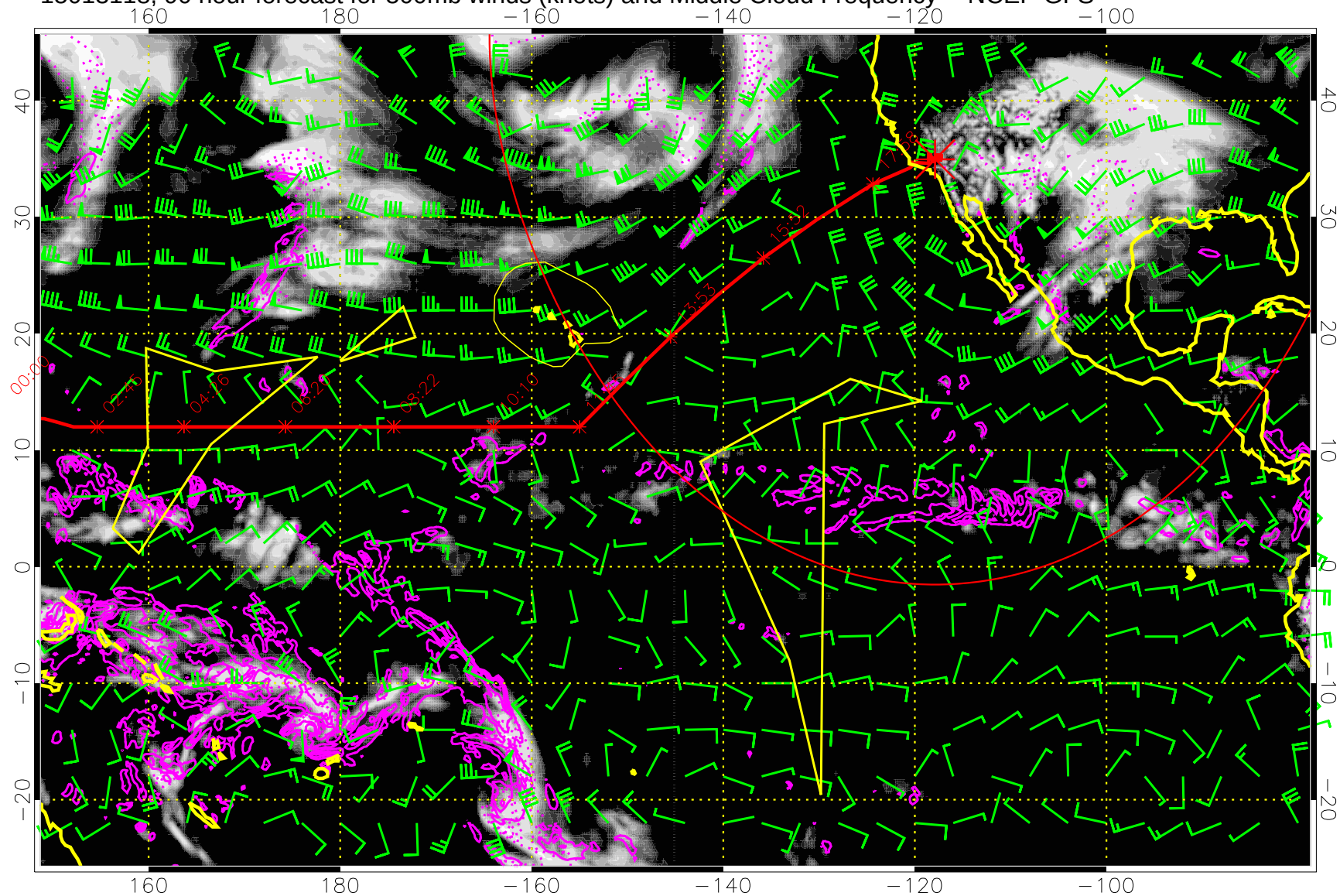
15013118, 90 hour forecast for 500mb winds (knots) and Middle Cloud Frequency -- NCEP GFS
