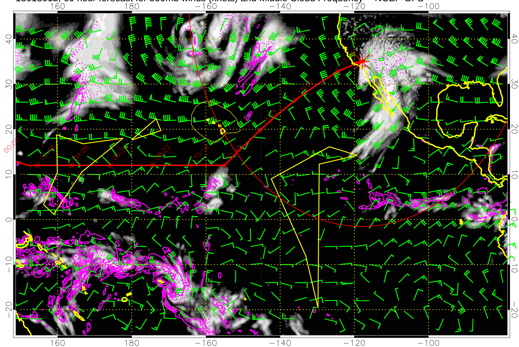
15013012, 60 hour forecast for 500mb winds (knots) and Middle Cloud Frequency -- NCEP GFS
