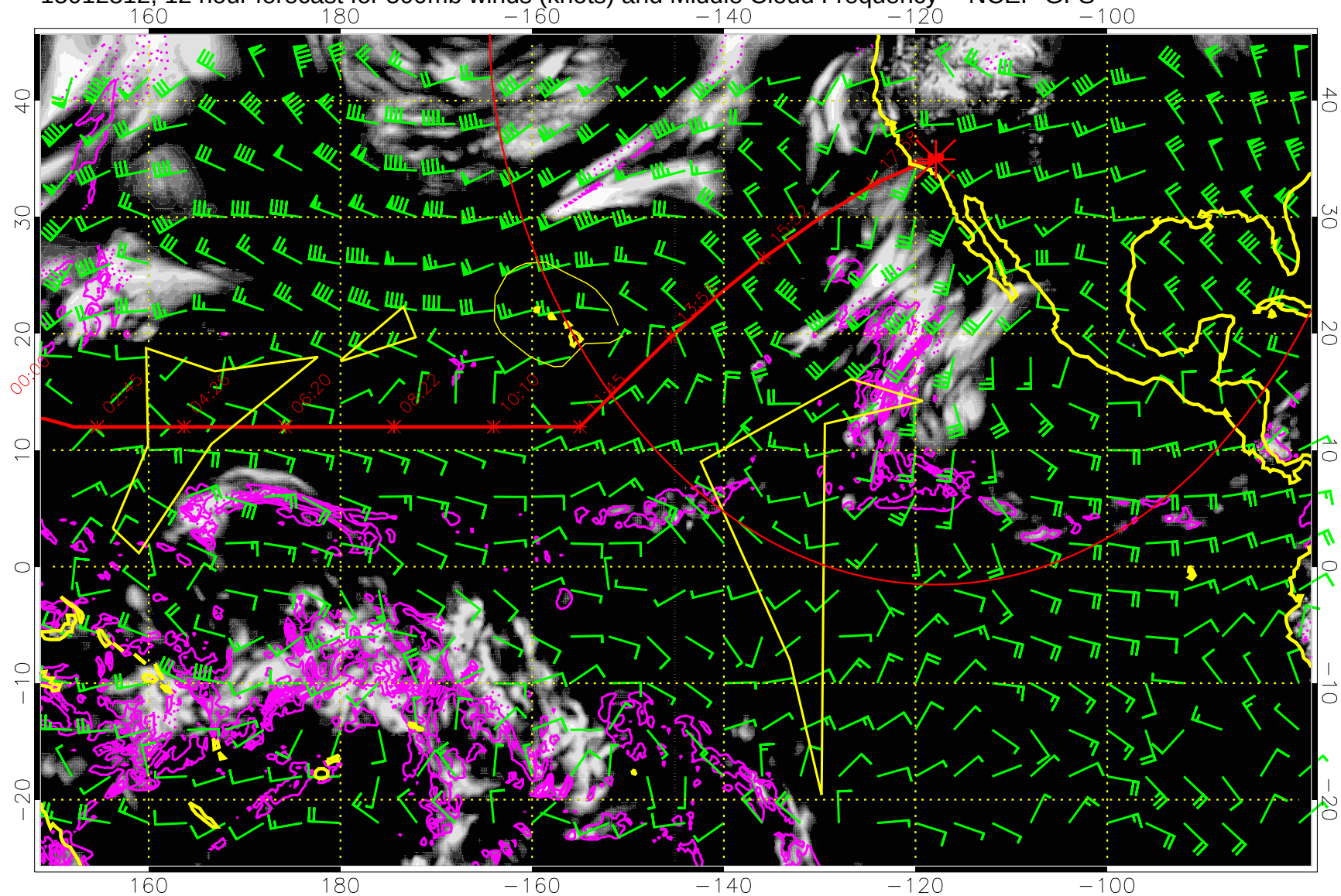
15012812, 12 hour forecast for 500mb winds (knots) and Middle Cloud Frequency -- NCEP GFS
