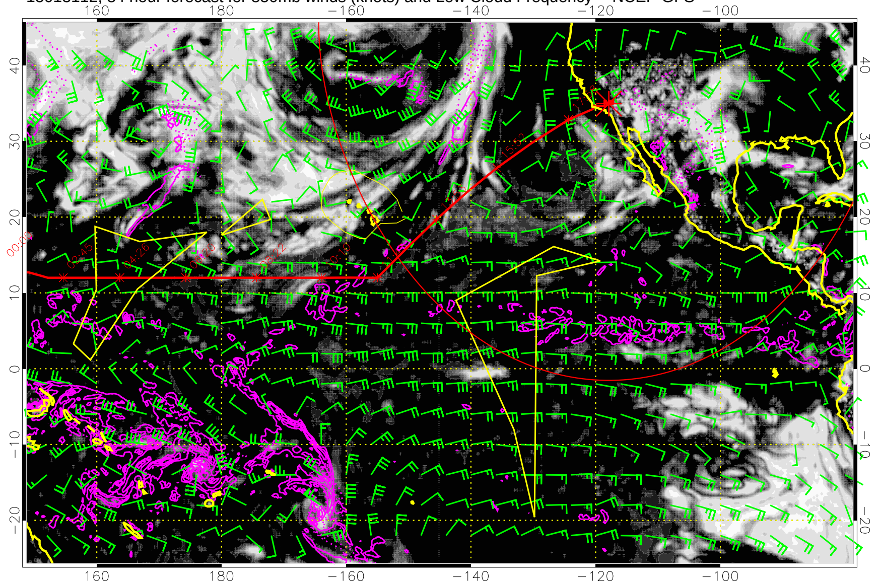
15013112, 84 hour forecast for 850mb winds (knots) and Low Cloud Frequency -- NCEP GFS
