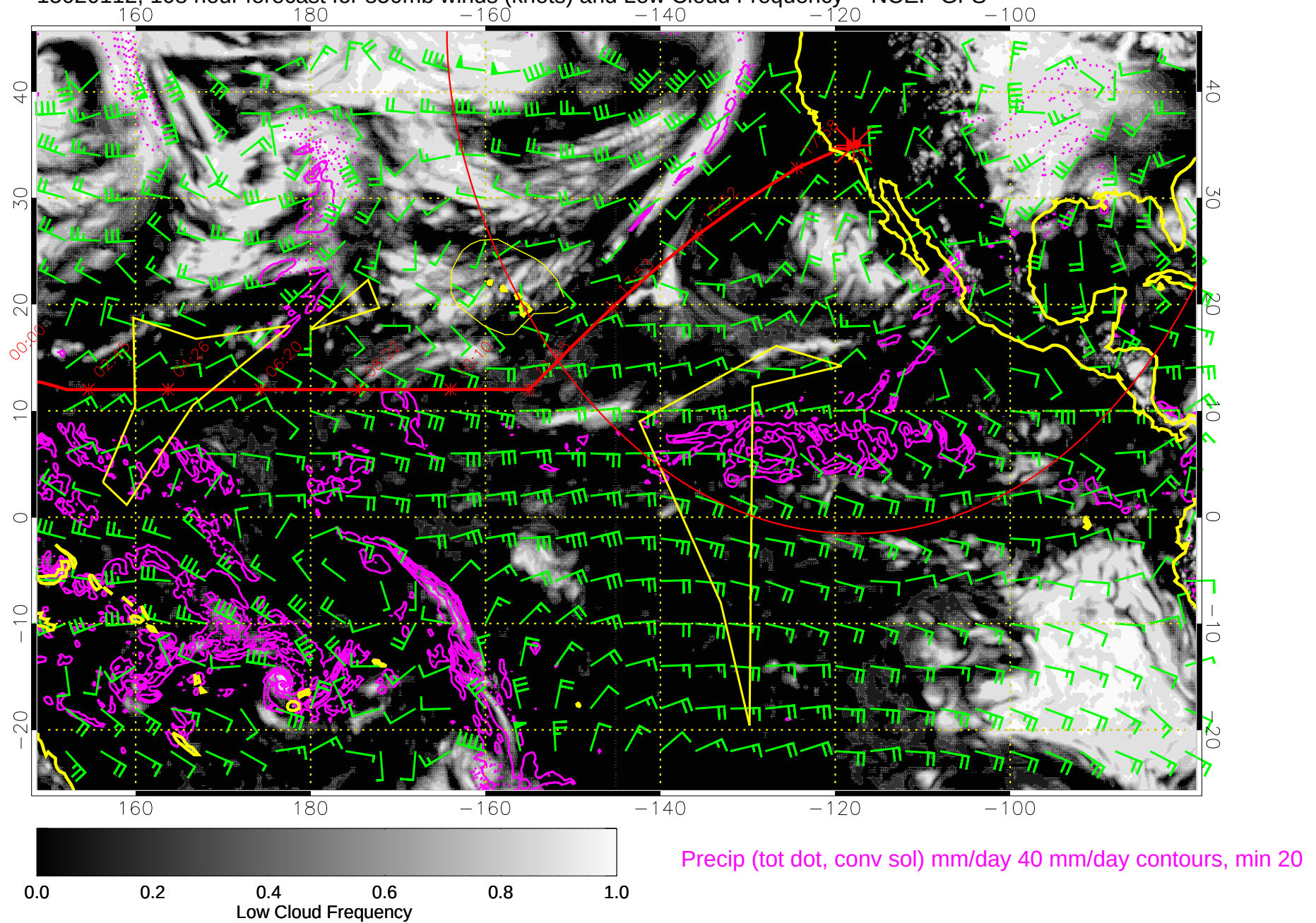
15020112, 108 hour forecast for 850mb winds (knots) and Low Cloud Frequency -- NCEP GFS
