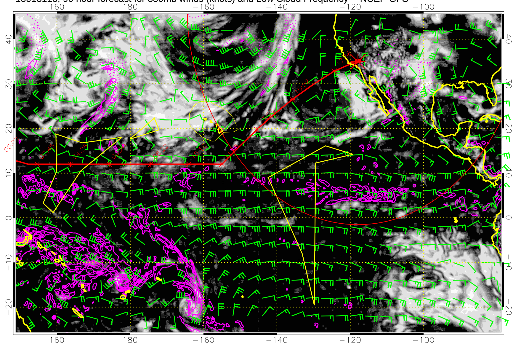
15013118, 90 hour forecast for 850mb winds (knots) and Low Cloud Frequency -- NCEP GFS
