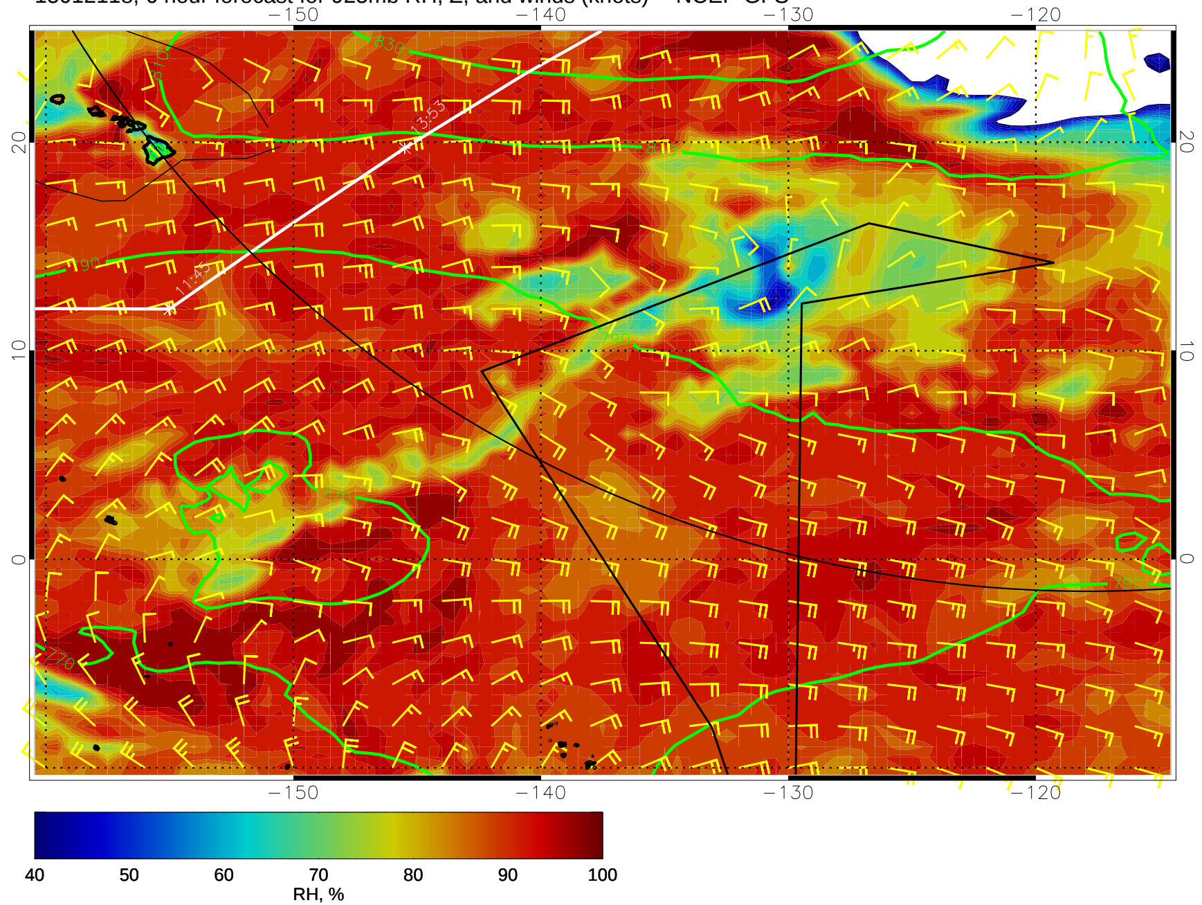
15012118, 6 hour forecast for 925mb RH, Z, and winds (knots) -- NCEP GFS
