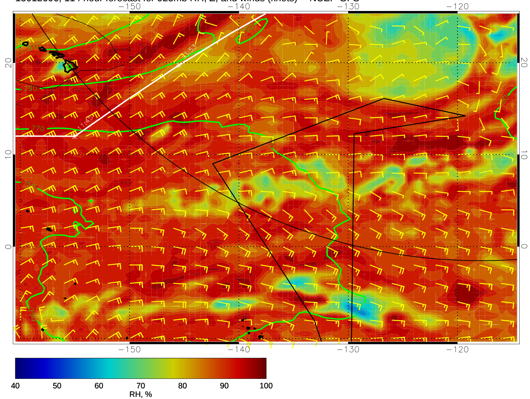
15012606, 114 hour forecast for 925mb RH, Z, and winds (knots) -- NCEP GFS
