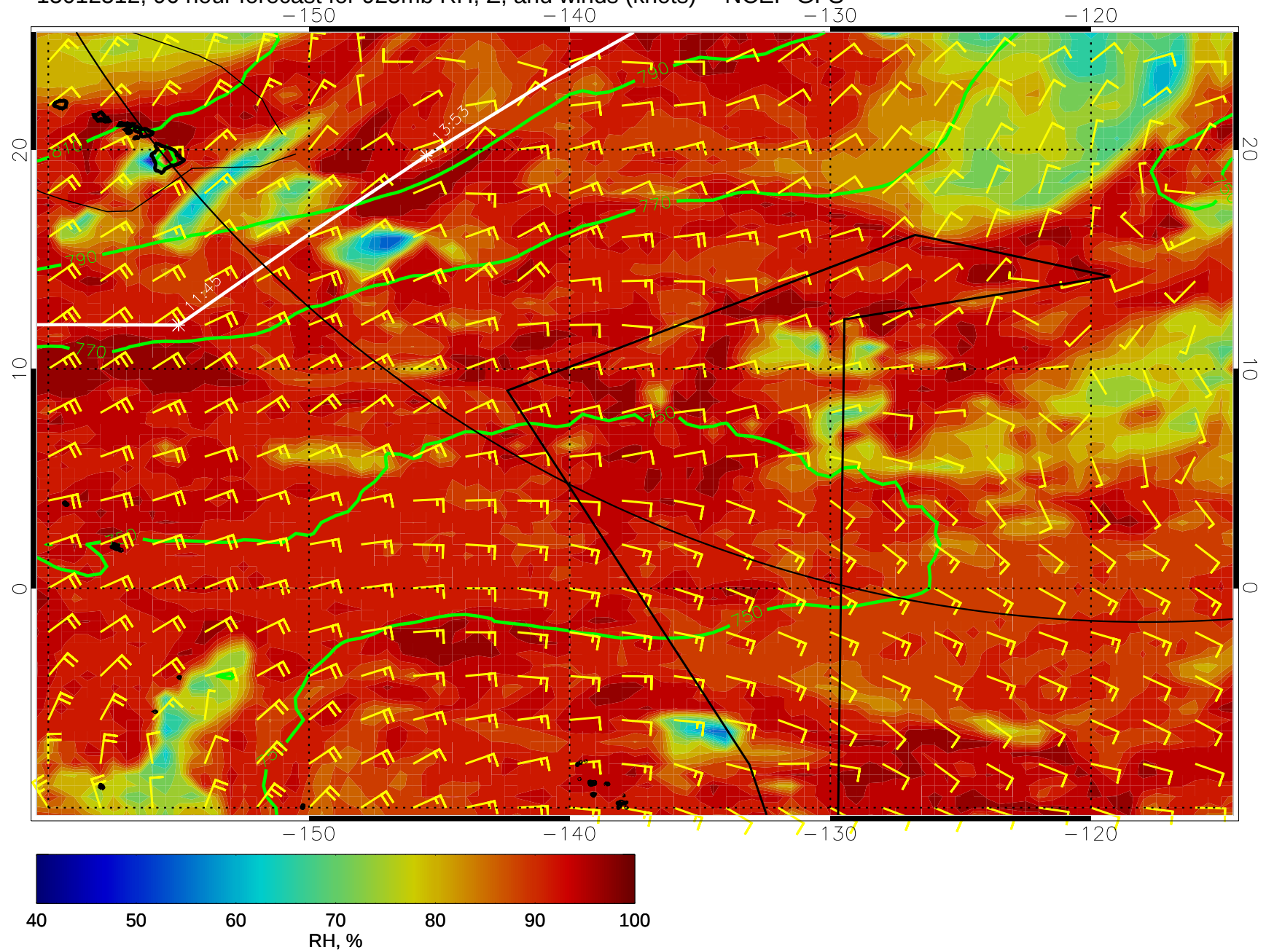
15012512, 96 hour forecast for 925mb RH, Z, and winds (knots) -- NCEP GFS
