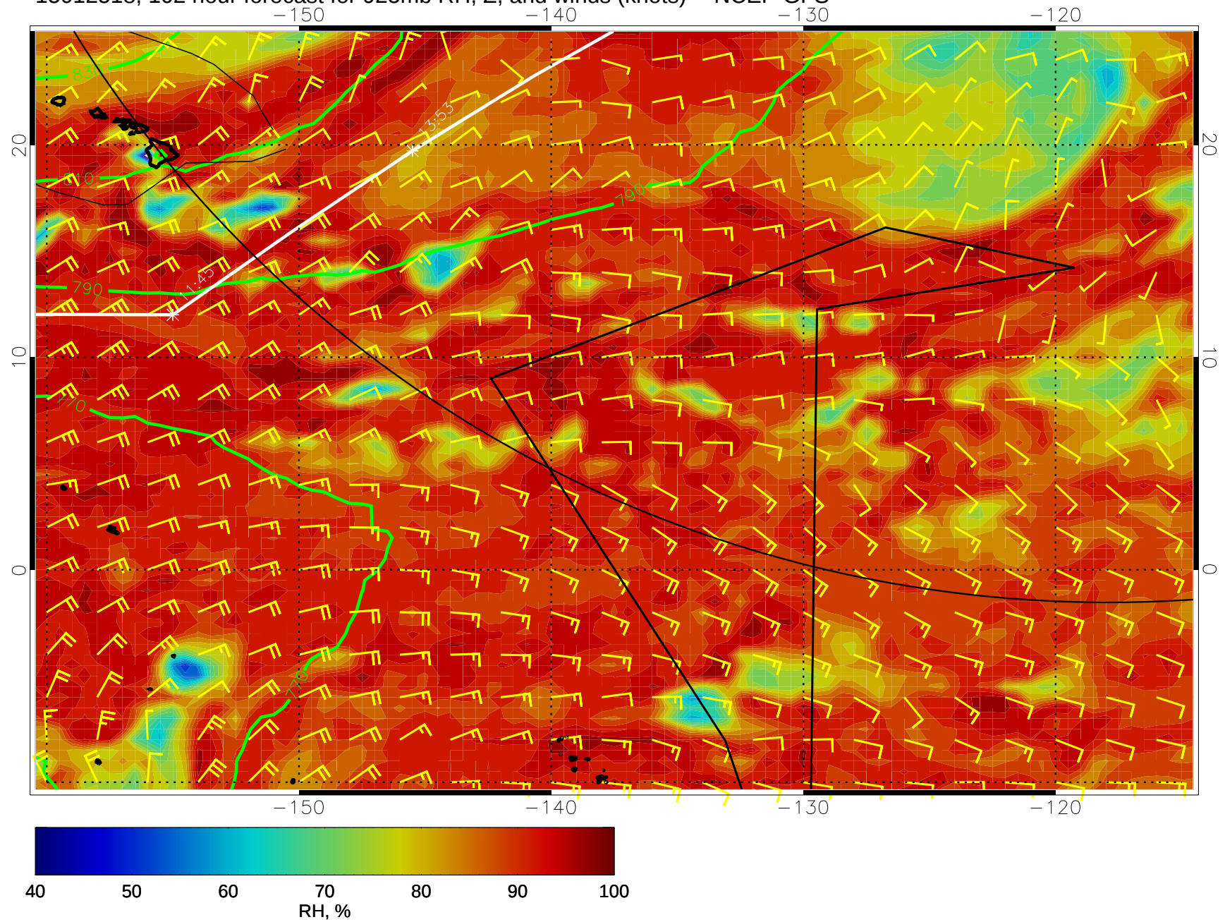
15012518, 102 hour forecast for 925mb RH, Z, and winds (knots) -- NCEP GFS
