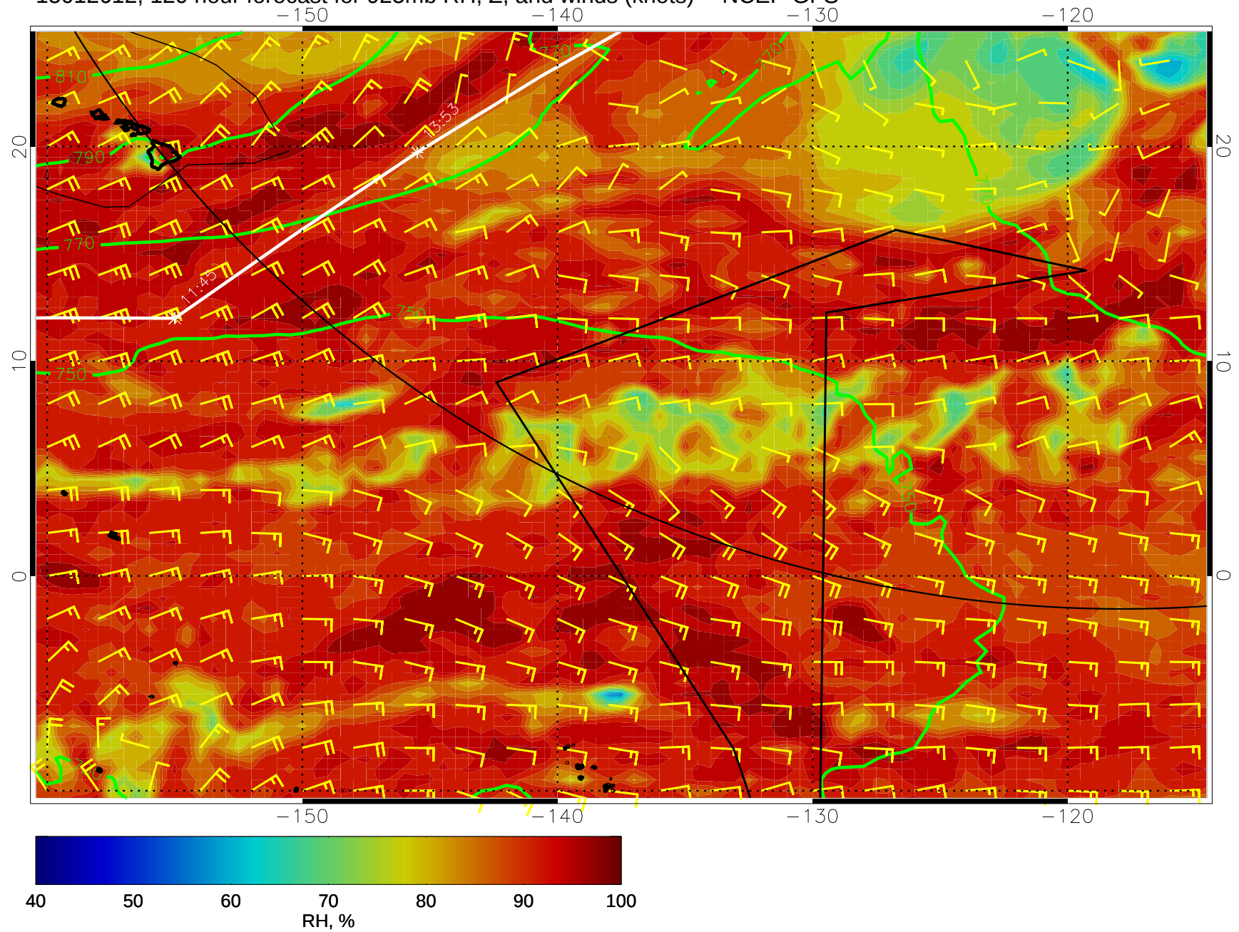
15012612, 120 hour forecast for 925mb RH, Z, and winds (knots) -- NCEP GFS
