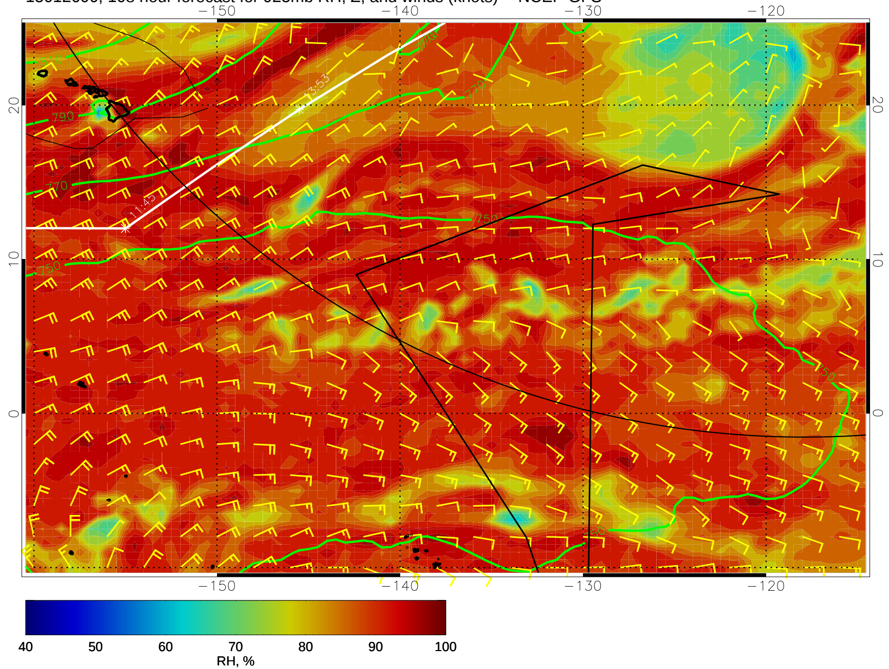
15012600, 108 hour forecast for 925mb RH, Z, and winds (knots) -- NCEP GFS
