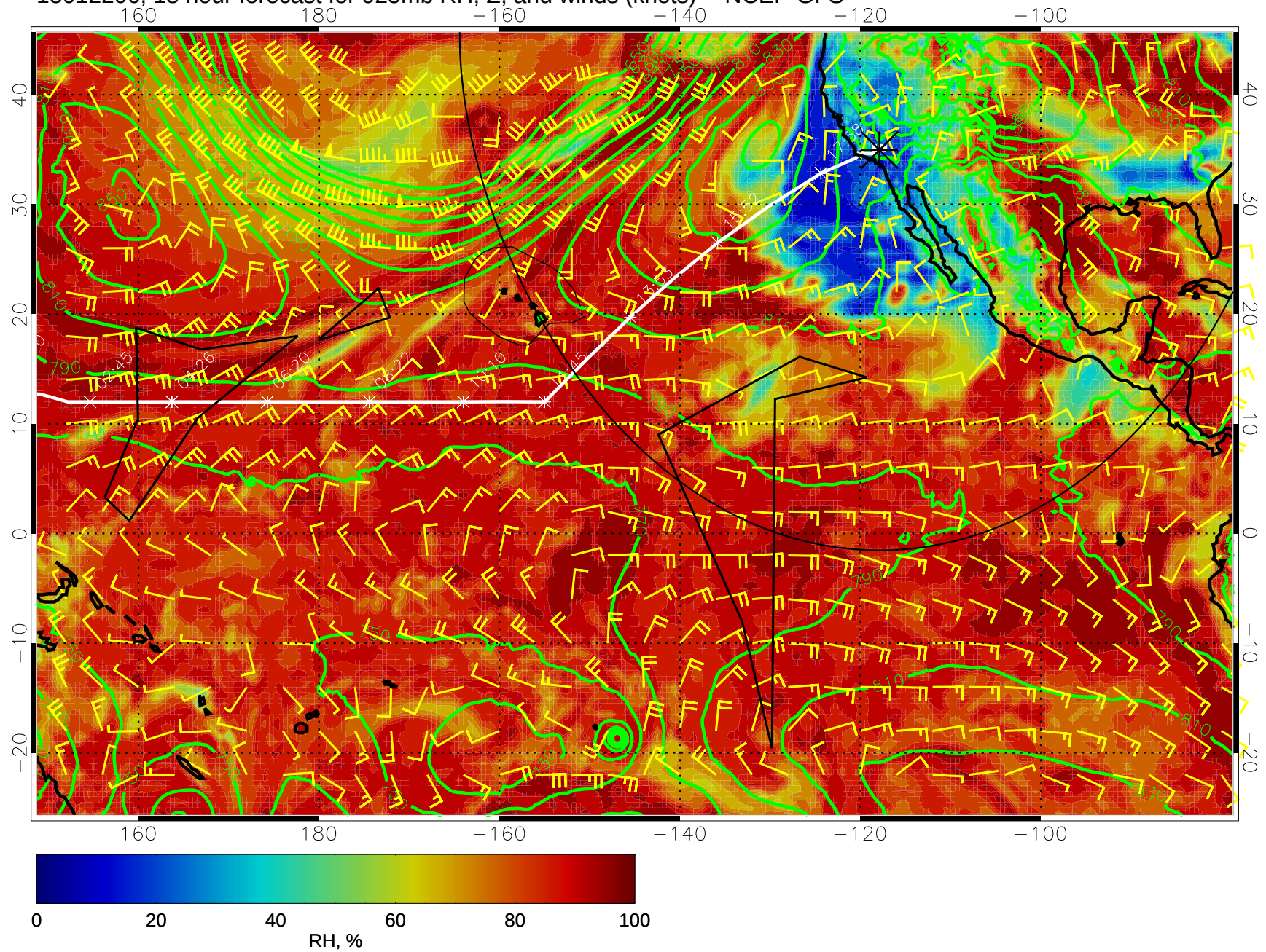
15012206, 18 hour forecast for 925mb RH, Z, and winds (knots) -- NCEP GFS
