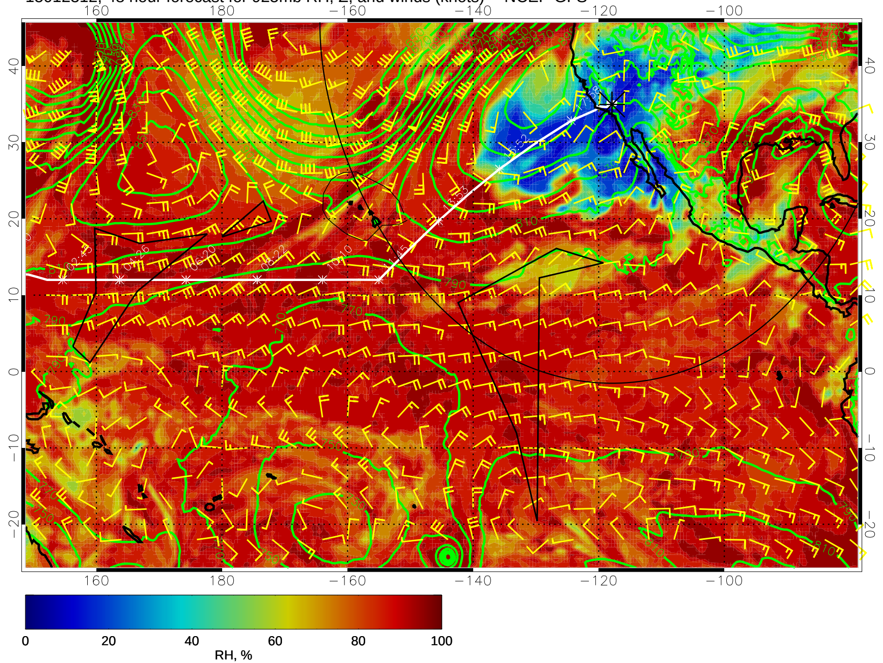
15012312, 48 hour forecast for 925mb RH, Z, and winds (knots) -- NCEP GFS
