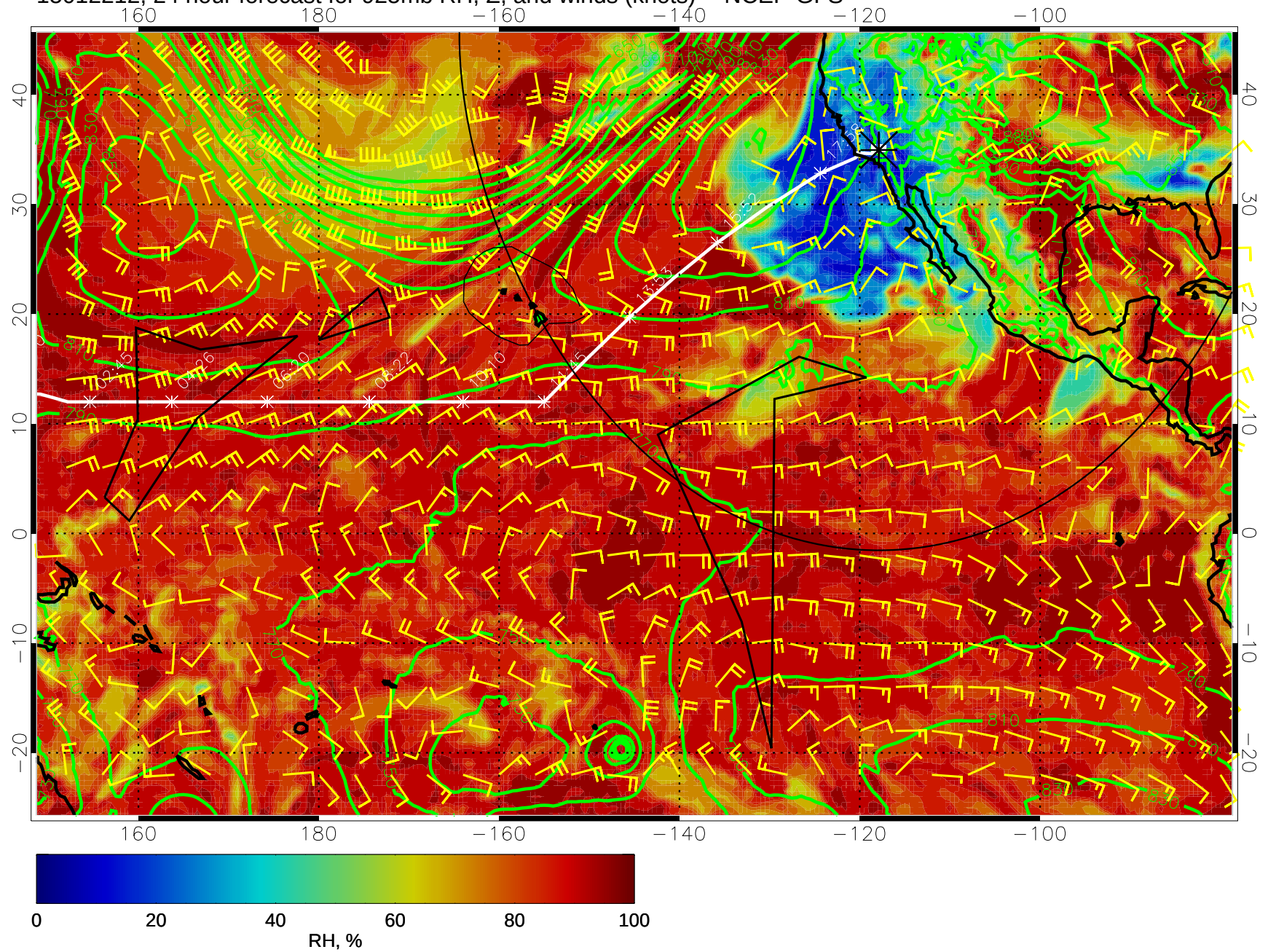
15012212, 24 hour forecast for 925mb RH, Z, and winds (knots) -- NCEP GFS
