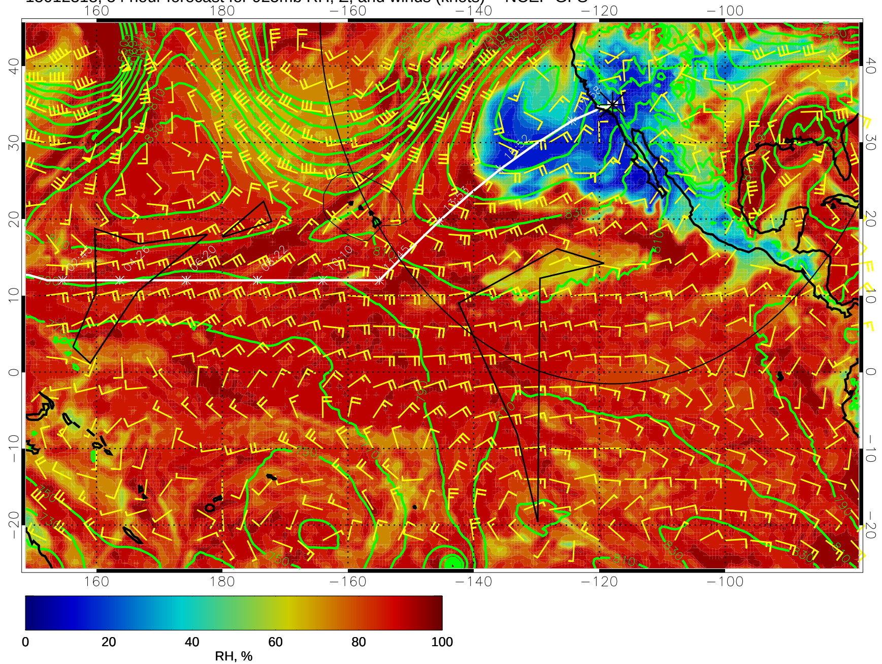
15012318, 54 hour forecast for 925mb RH, Z, and winds (knots) -- NCEP GFS
