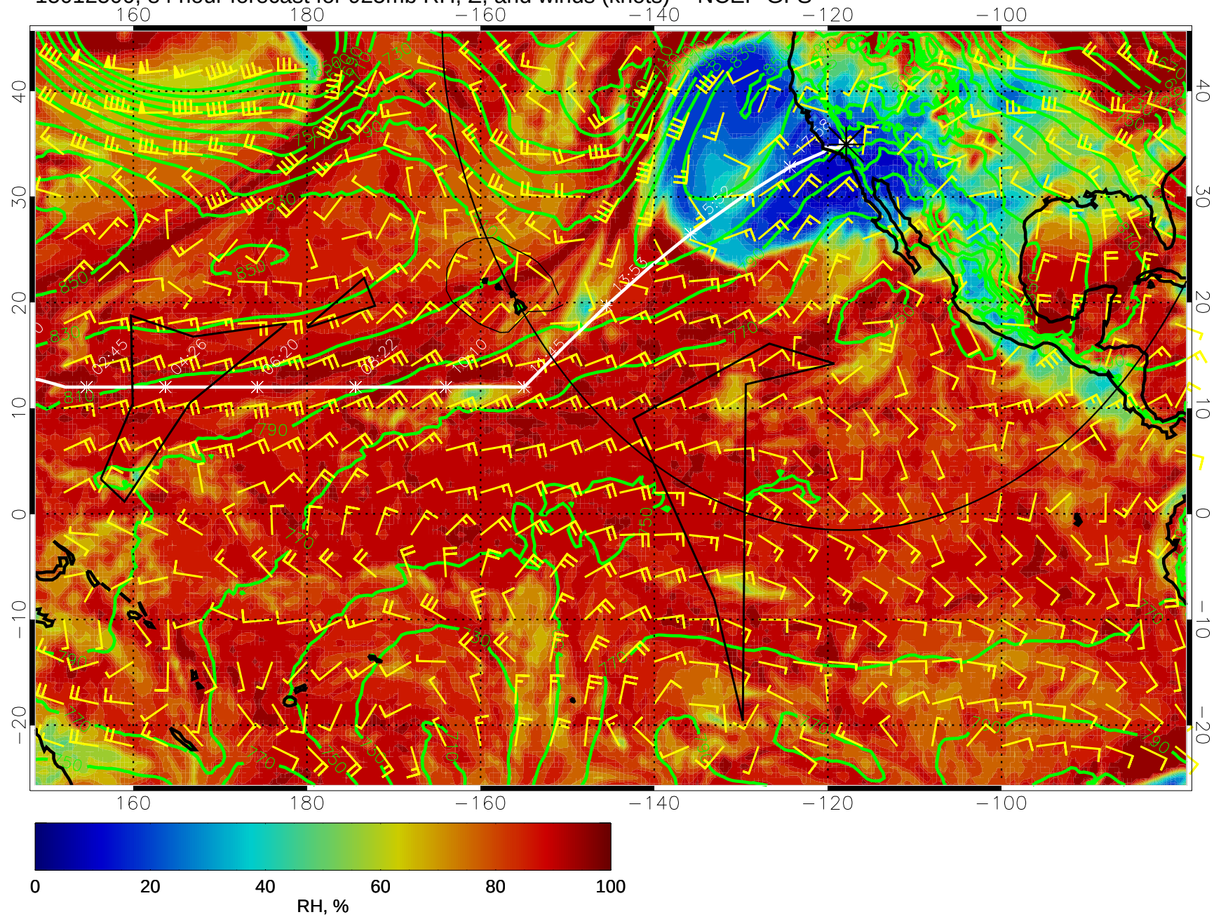
15012500, 84 hour forecast for 925mb RH, Z, and winds (knots) -- NCEP GFS
