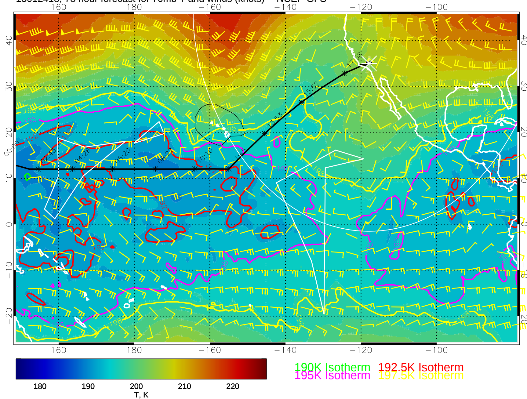
15012418, 78 hour forecast for 70mb T and winds (knots) -- NCEP GFS
