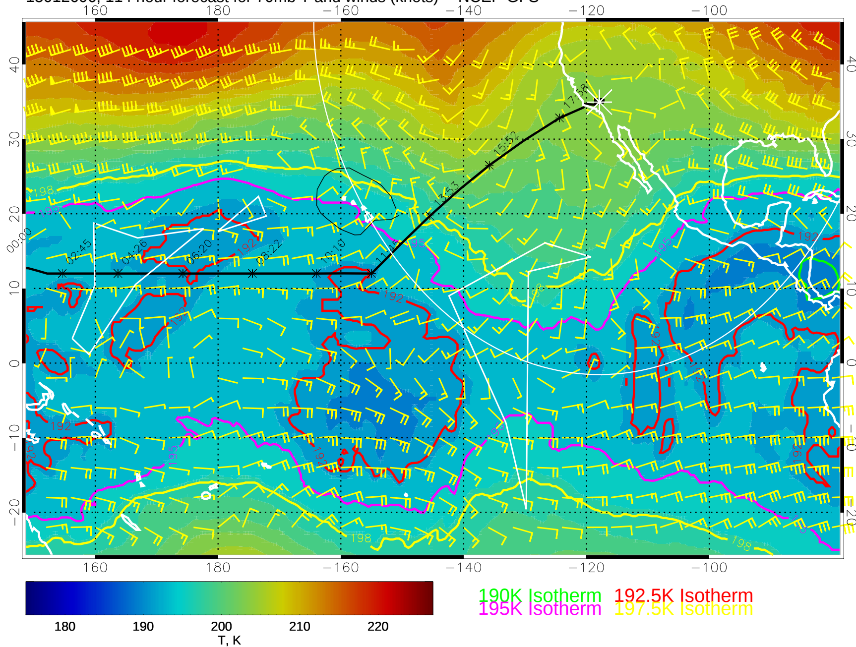
15012606, 114 hour forecast for 70mb T and winds (knots) -- NCEP GFS
