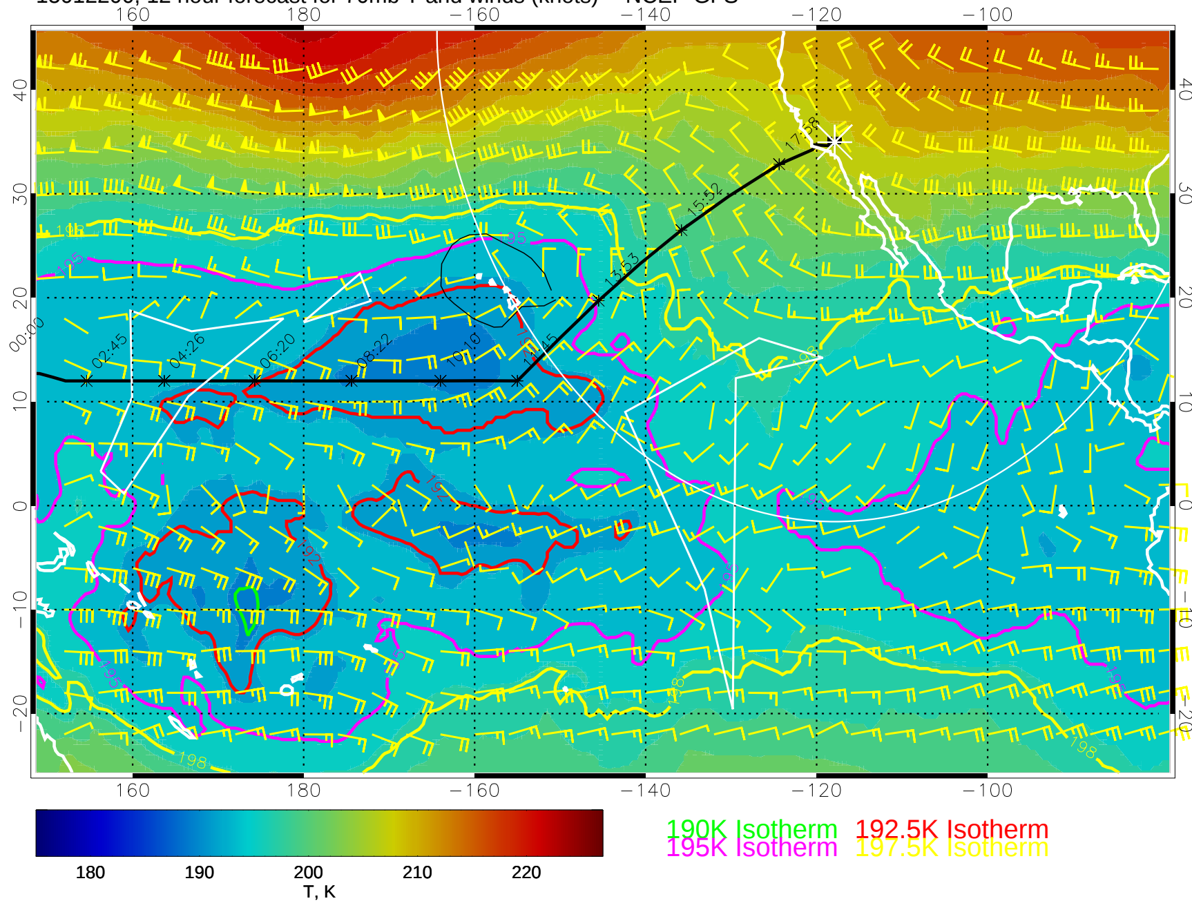
15012200, 12 hour forecast for 70mb T and winds (knots) -- NCEP GFS
