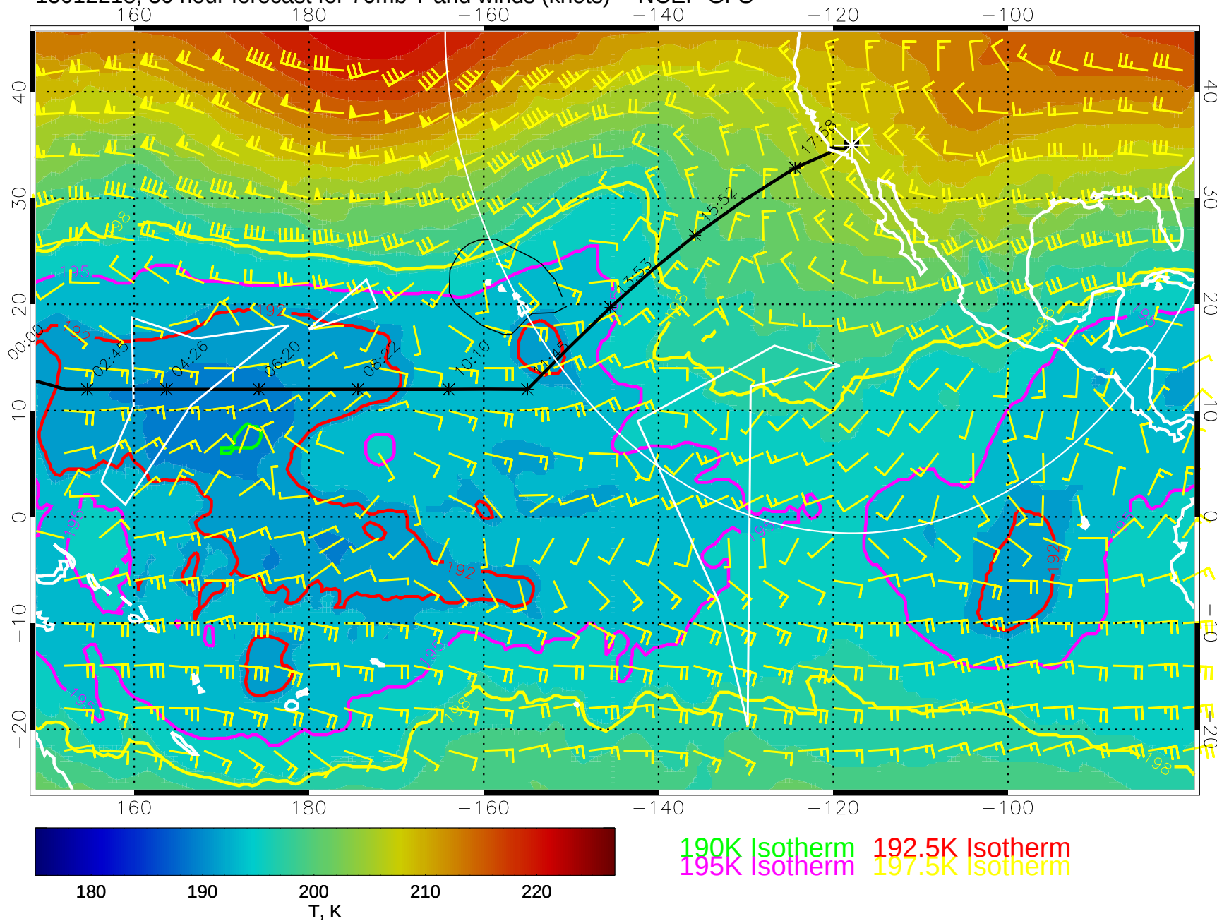
15012218, 30 hour forecast for 70mb T and winds (knots) -- NCEP GFS
