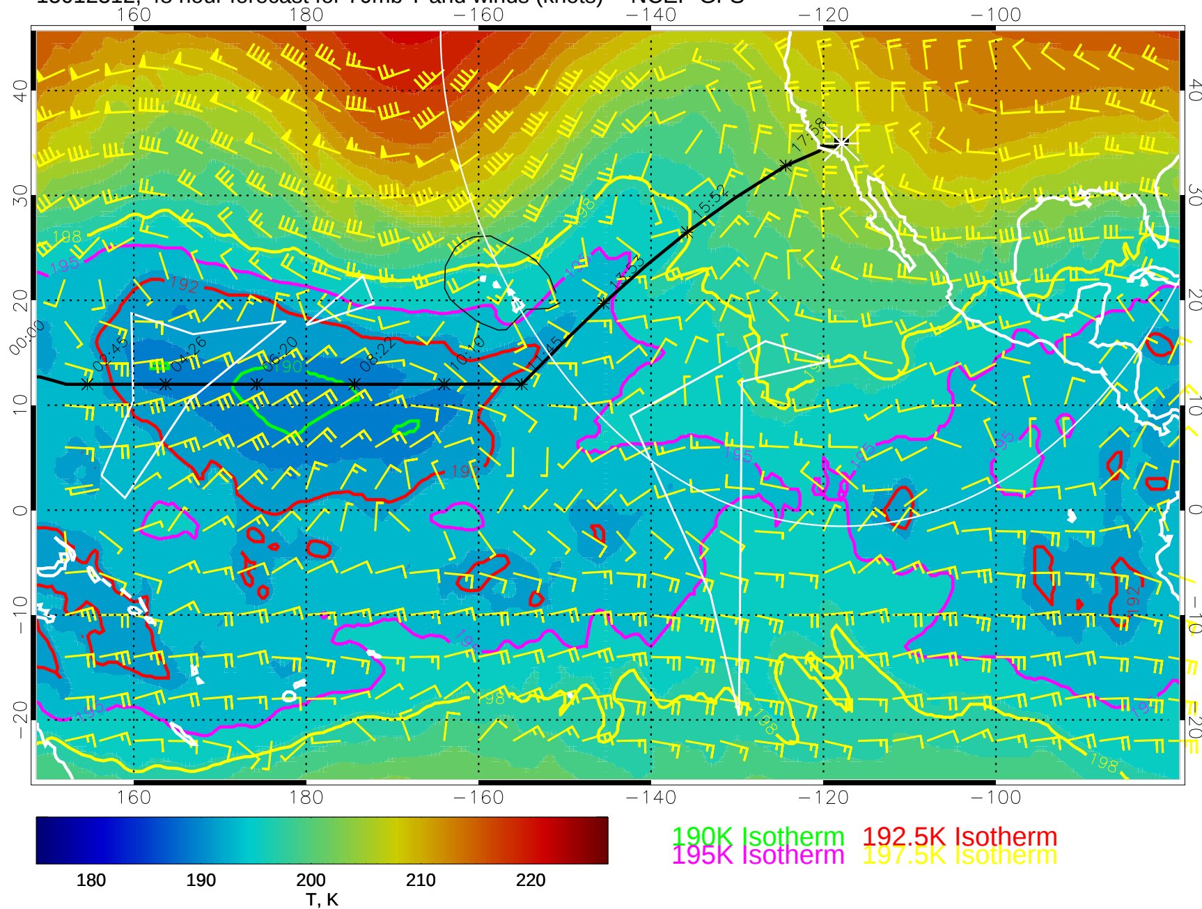
15012312, 48 hour forecast for 70mb T and winds (knots) -- NCEP GFS
