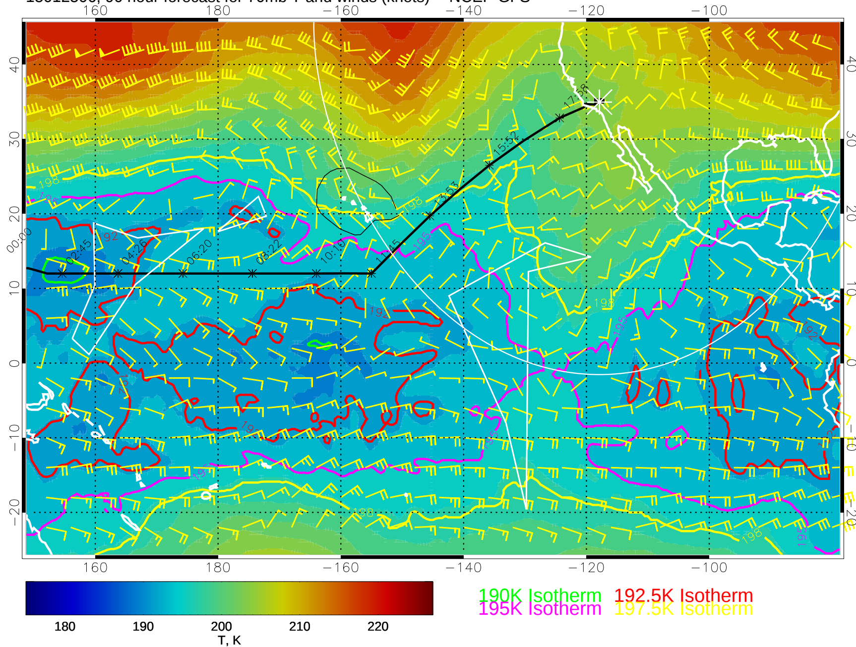
15012506, 90 hour forecast for 70mb T and winds (knots) -- NCEP GFS
