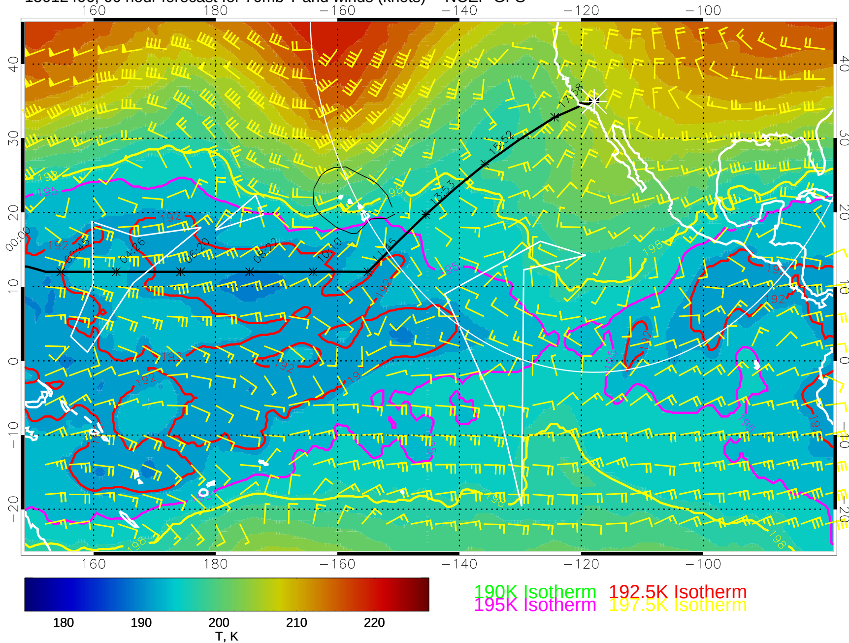
15012406, 66 hour forecast for 70mb T and winds (knots) -- NCEP GFS
