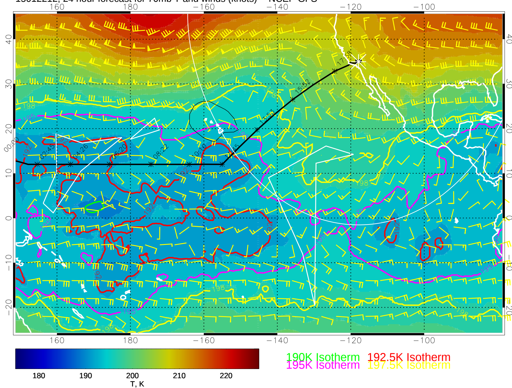
15012212, 24 hour forecast for 70mb T and winds (knots) -- NCEP GFS
