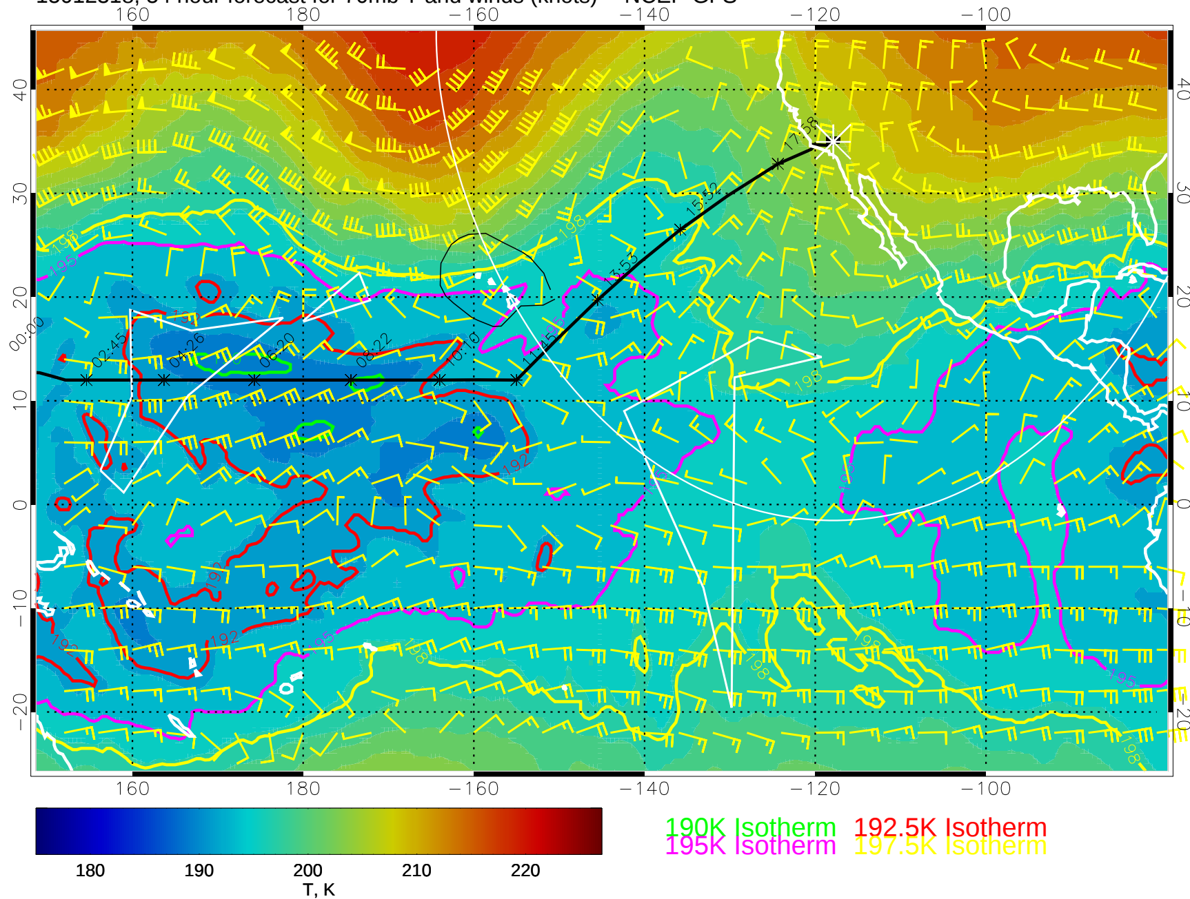
15012318, 54 hour forecast for 70mb T and winds (knots) -- NCEP GFS
