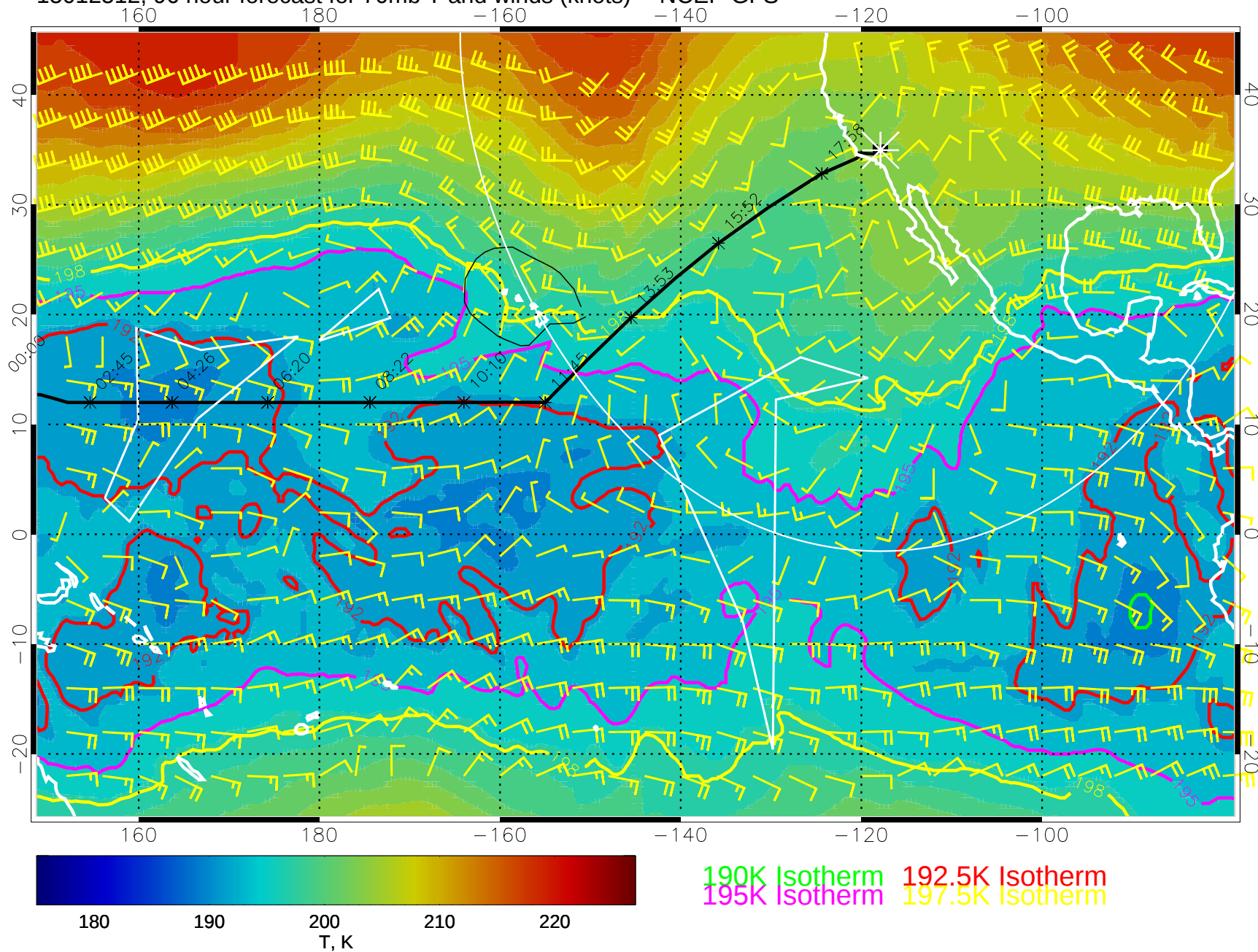
15012512, 96 hour forecast for 70mb T and winds (knots) -- NCEP GFS
