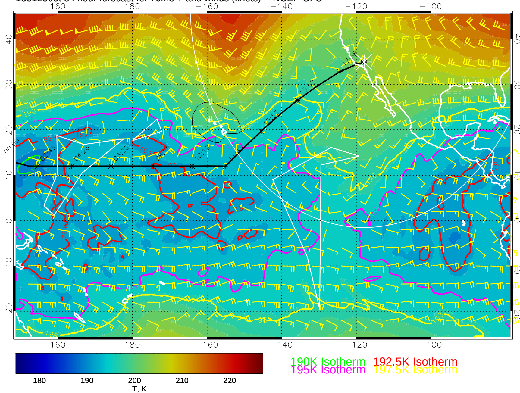
15012500, 84 hour forecast for 70mb T and winds (knots) -- NCEP GFS
