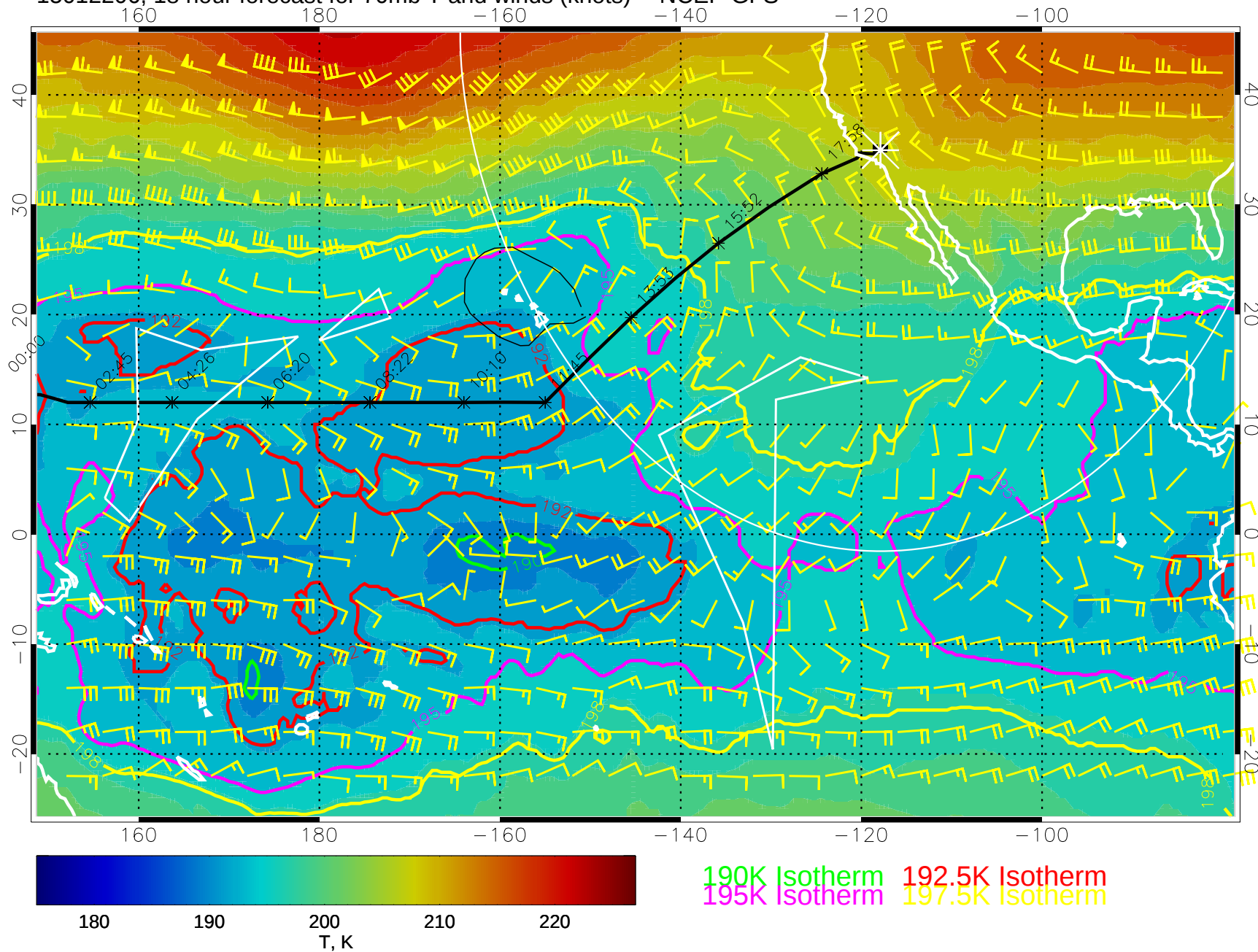
15012206, 18 hour forecast for 70mb T and winds (knots) -- NCEP GFS
