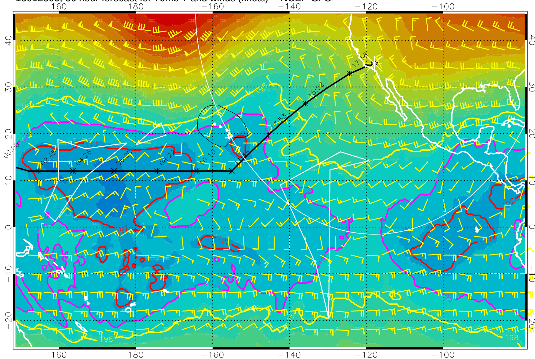
15012300, 36 hour forecast for 70mb T and winds (knots) -- NCEP GFS
