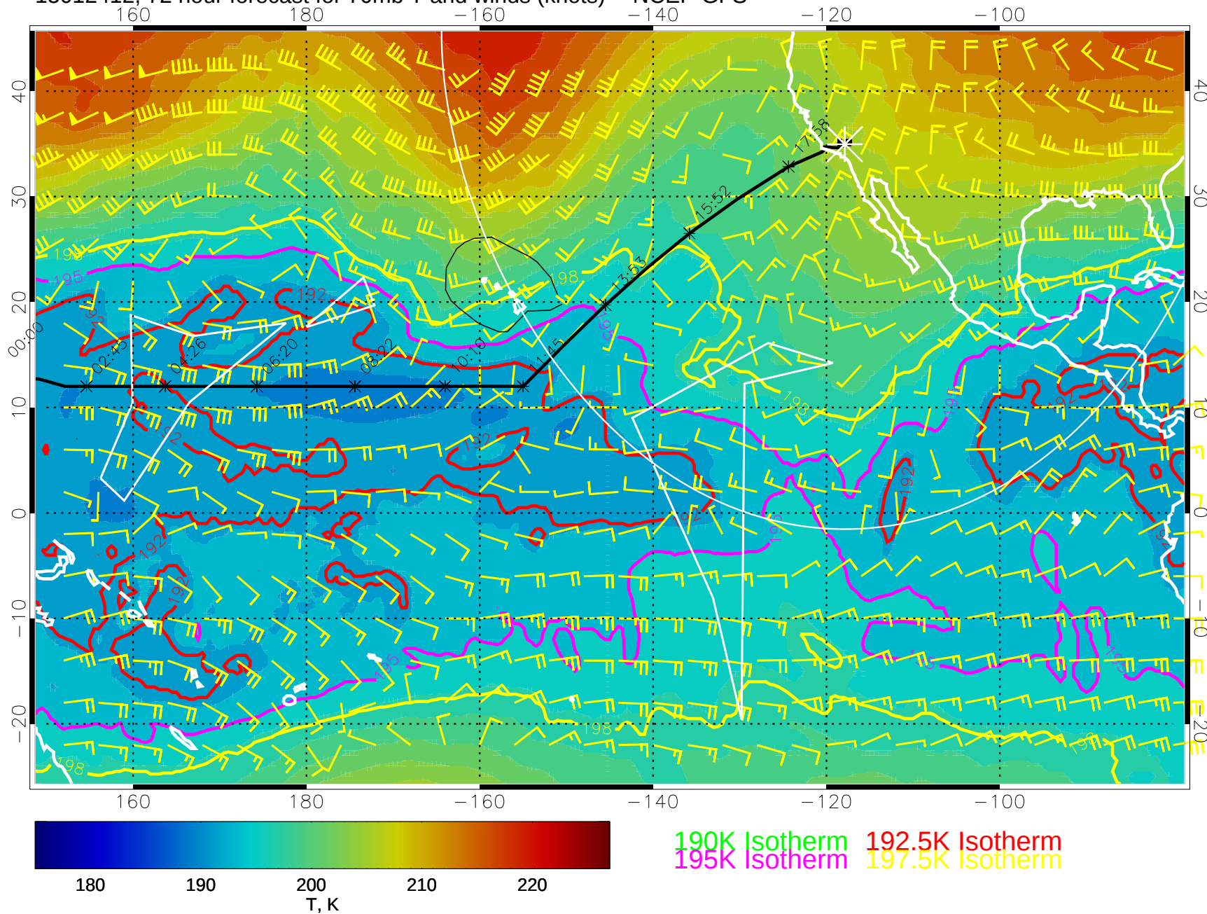
15012412, 72 hour forecast for 70mb T and winds (knots) -- NCEP GFS
