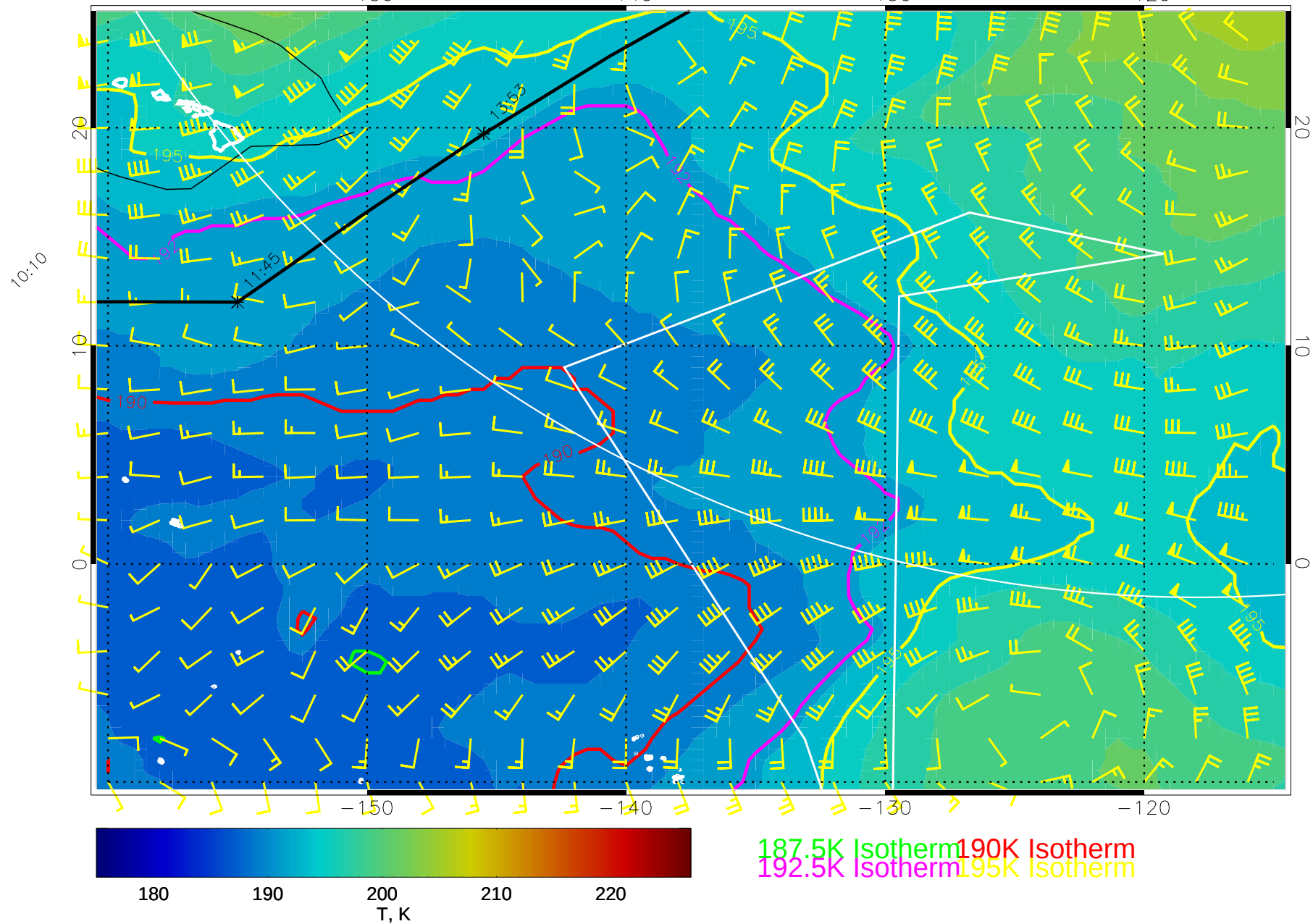
15012412, 72 hour forecast for 100mb T and winds (knots) -- NCEP GFS
