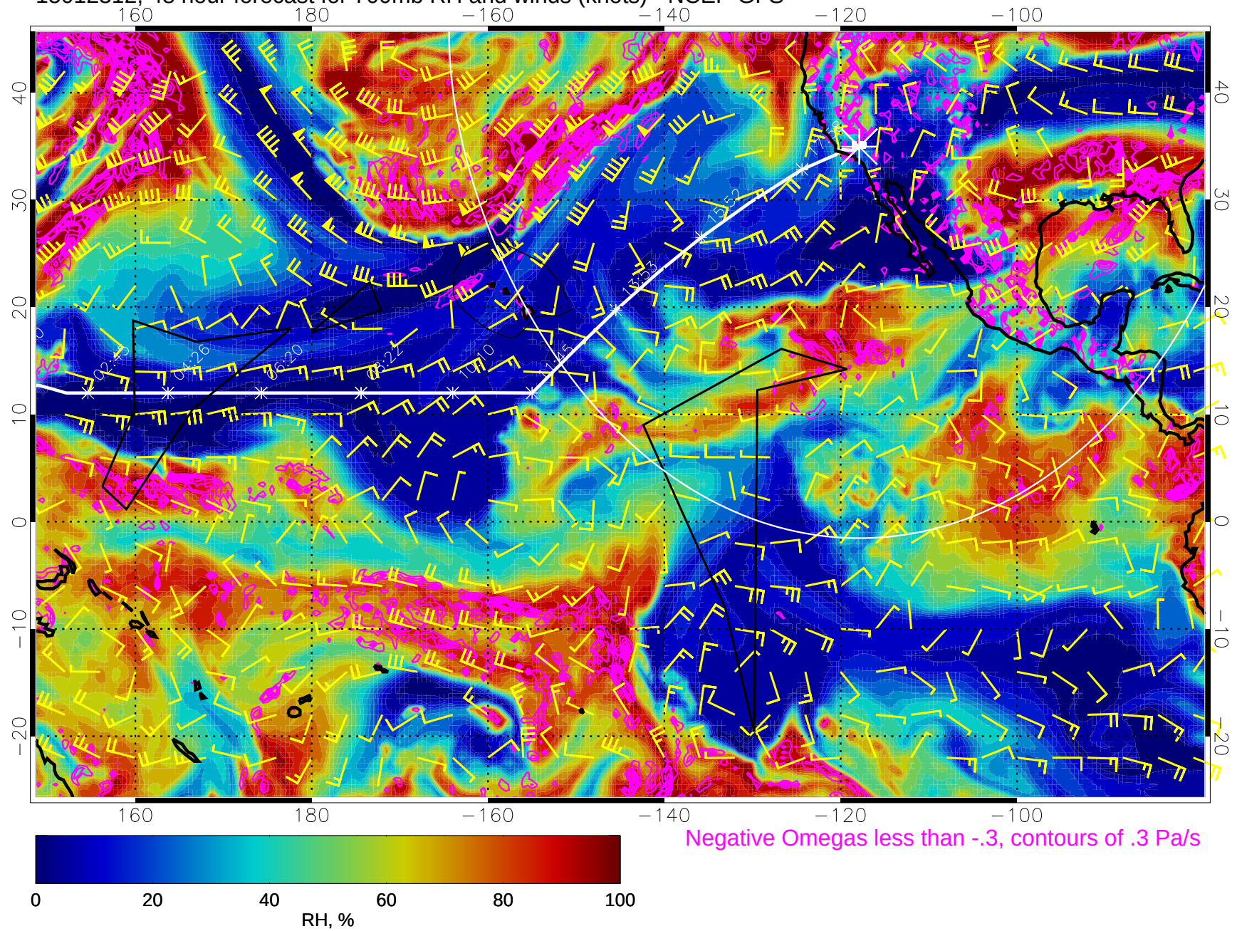
15012312, 48 hour forecast for 700mb RH and winds (knots) - NCEP GFS
