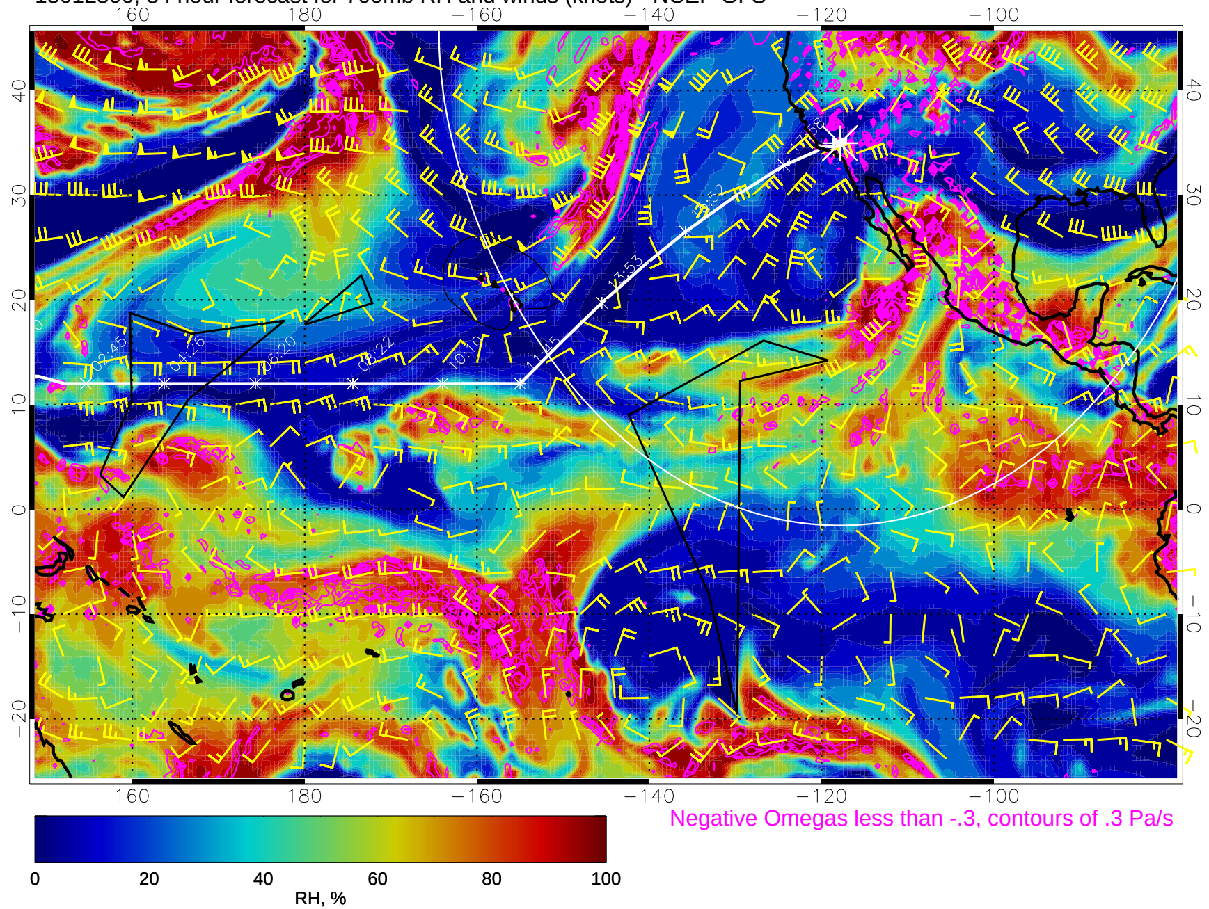
15012500, 84 hour forecast for 700mb RH and winds (knots) - NCEP GFS
