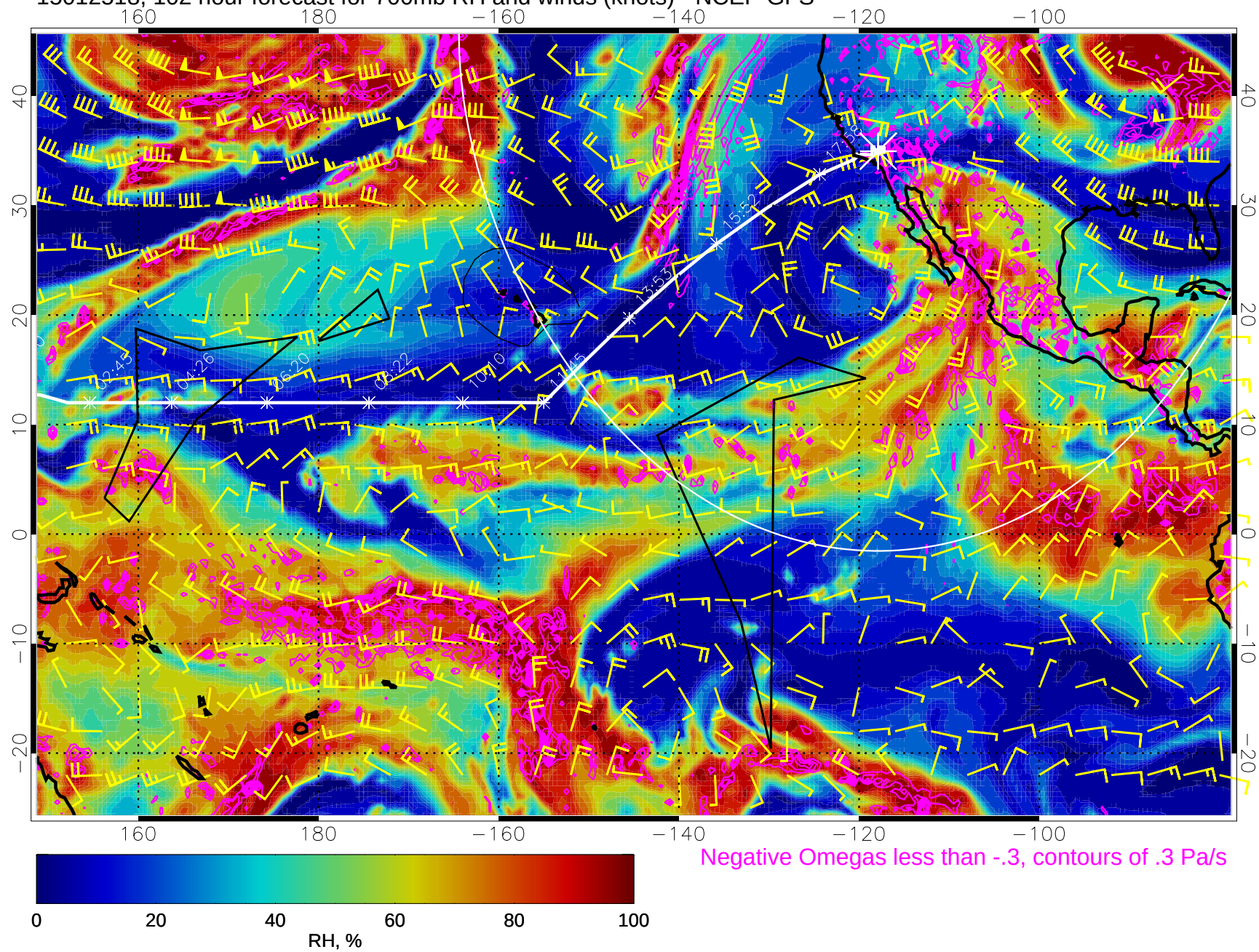
15012518, 102 hour forecast for 700mb RH and winds (knots) - NCEP GFS
