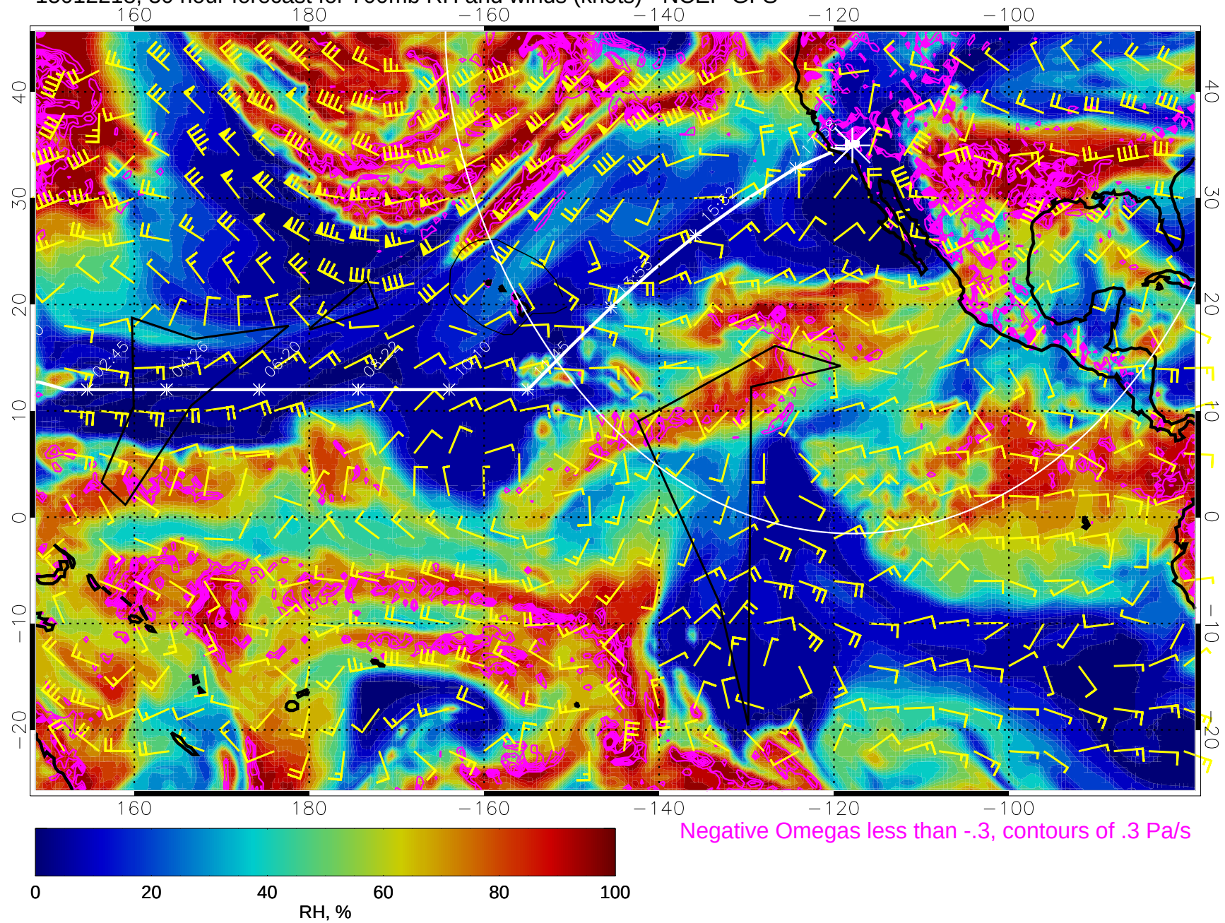
15012218, 30 hour forecast for 700mb RH and winds (knots) - NCEP GFS
