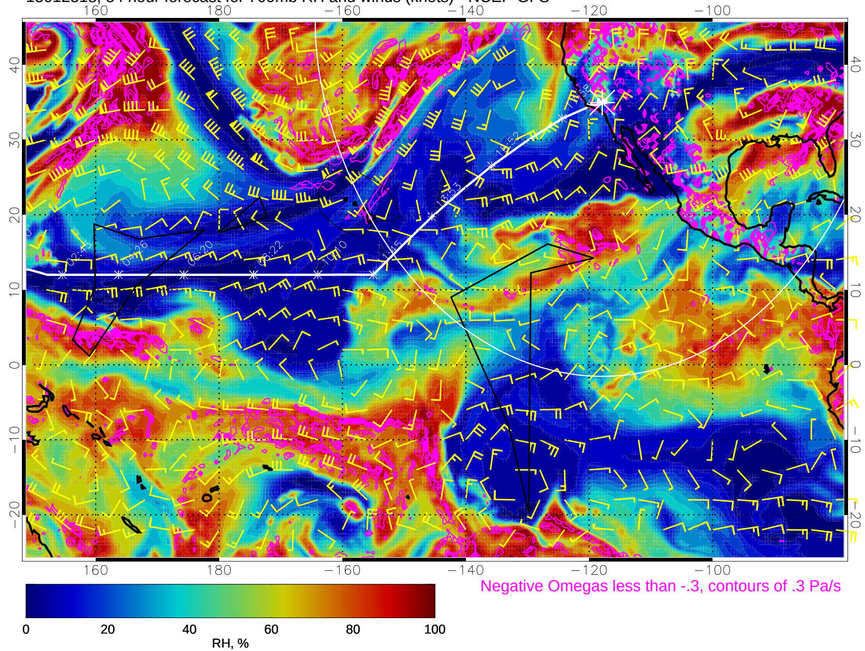
15012318, 54 hour forecast for 700mb RH and winds (knots) - NCEP GFS
