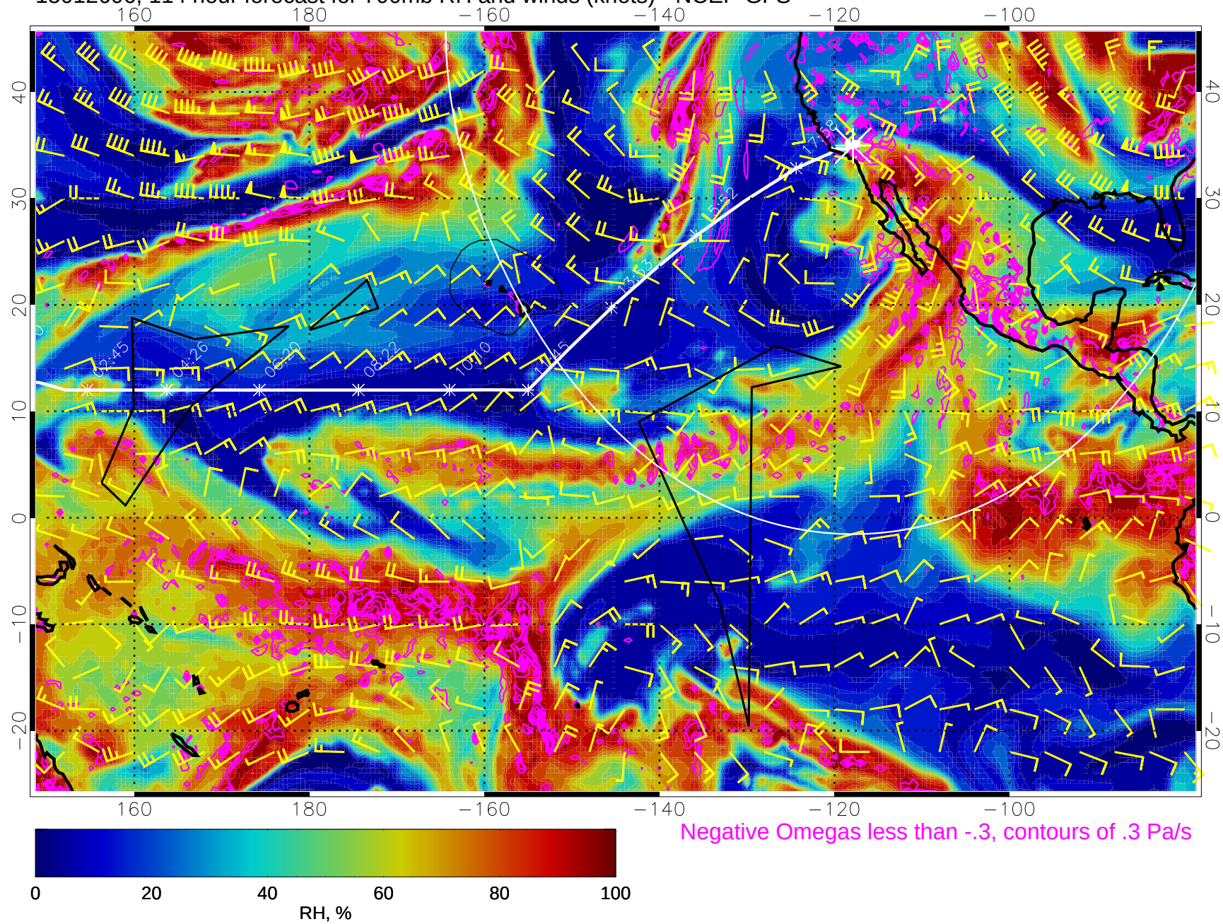
15012606, 114 hour forecast for 700mb RH and winds (knots) - NCEP GFS
