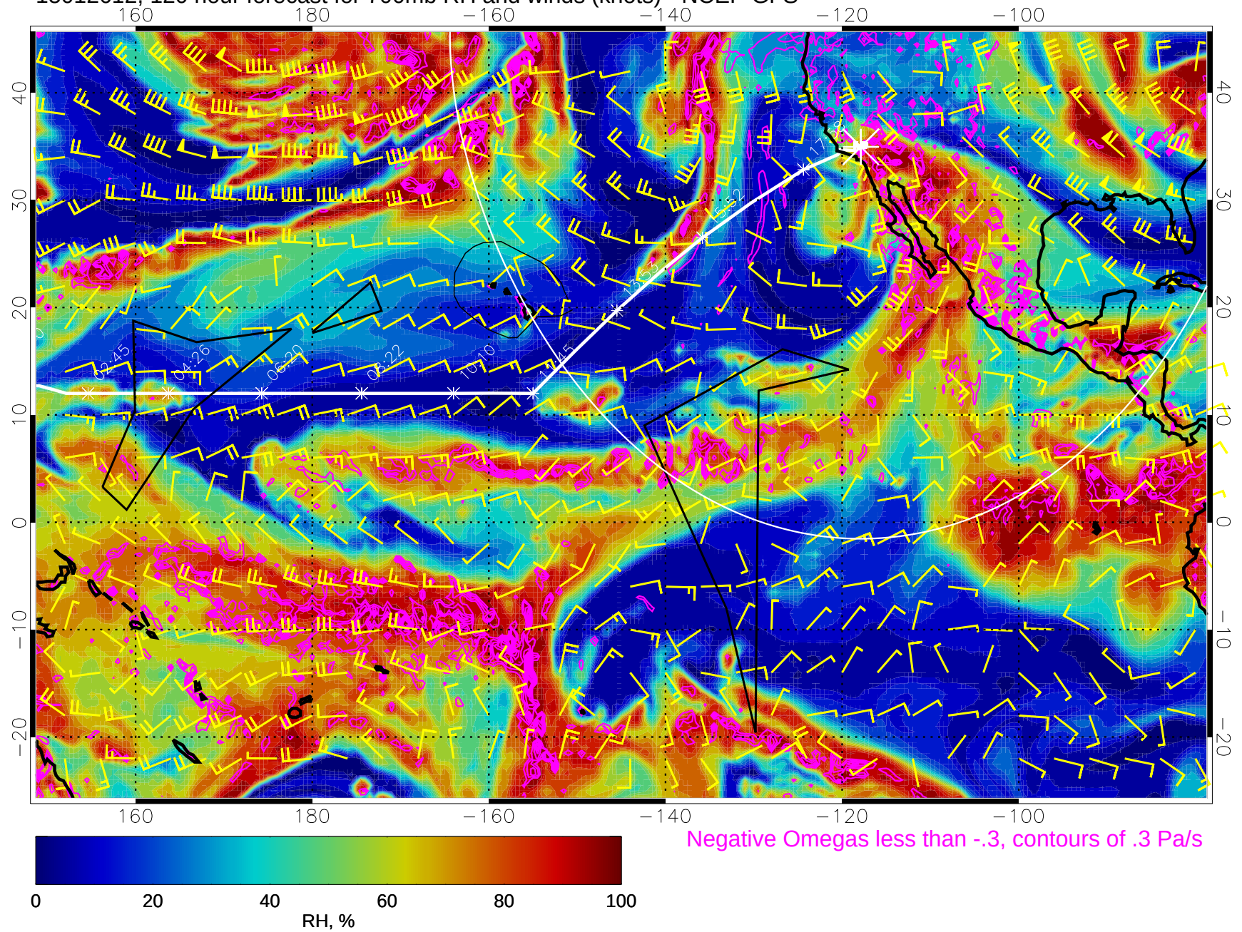
15012612, 120 hour forecast for 700mb RH and winds (knots) - NCEP GFS
