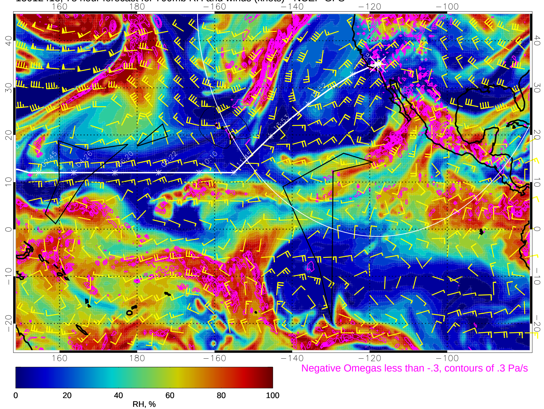
15012418, 78 hour forecast for 700mb RH and winds (knots) - NCEP GFS
