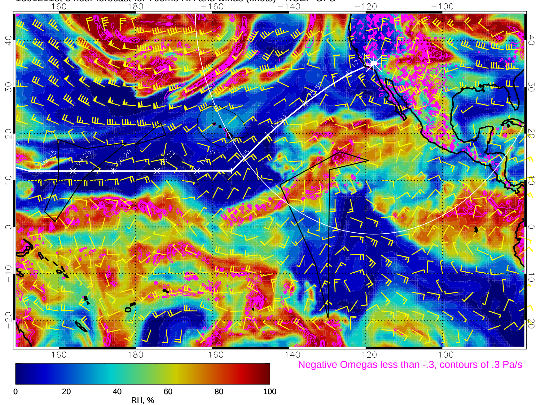
15012118, 6 hour forecast for 700mb RH and winds (knots) - NCEP GFS
