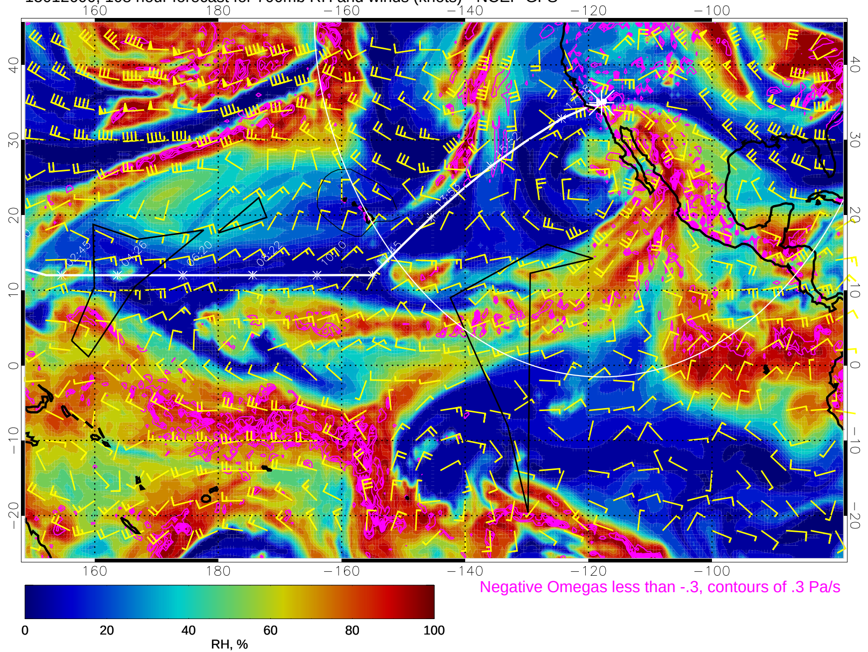
15012600, 108 hour forecast for 700mb RH and winds (knots) - NCEP GFS
