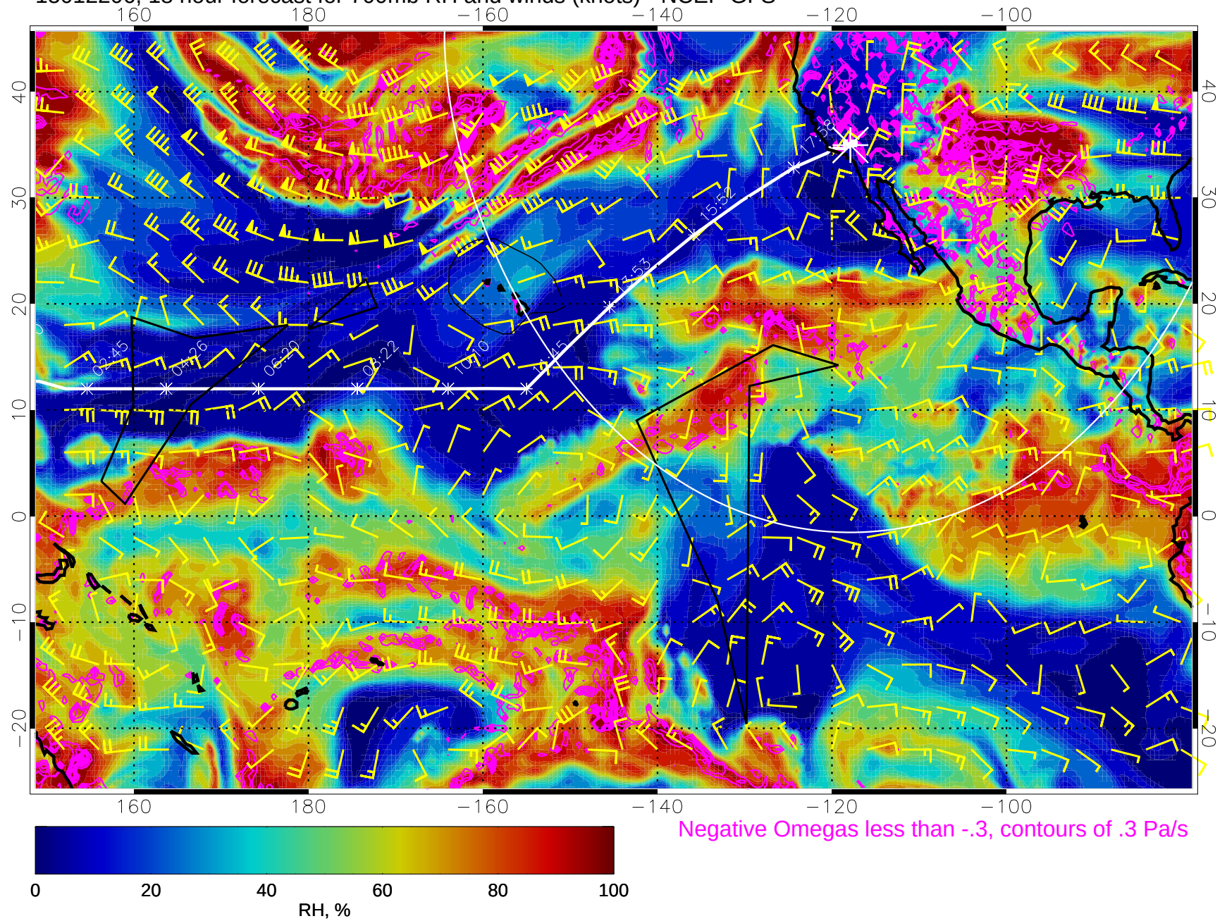
15012206, 18 hour forecast for 700mb RH and winds (knots) - NCEP GFS
