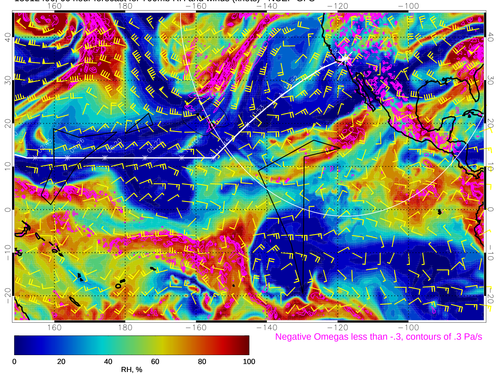
15012406, 66 hour forecast for 700mb RH and winds (knots) - NCEP GFS
