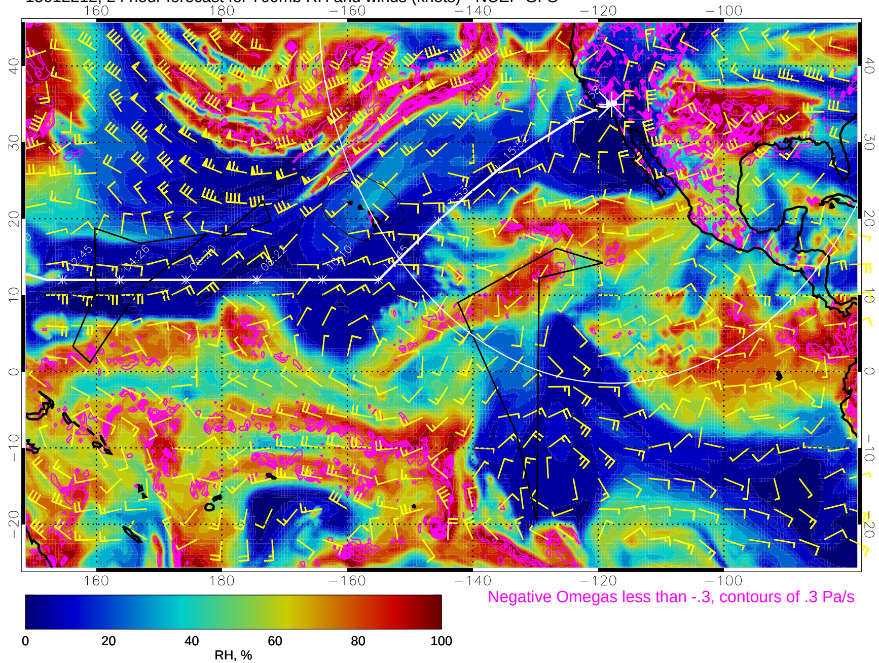
15012212, 24 hour forecast for 700mb RH and winds (knots) - NCEP GFS
