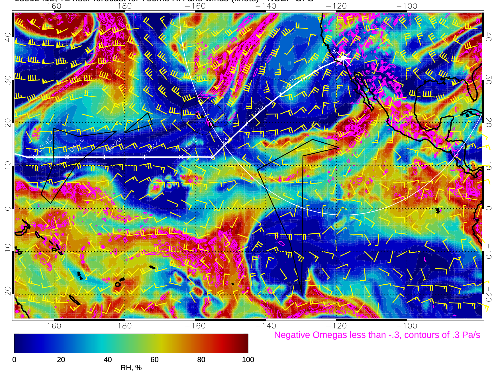
15012412, 72 hour forecast for 700mb RH and winds (knots) - NCEP GFS
