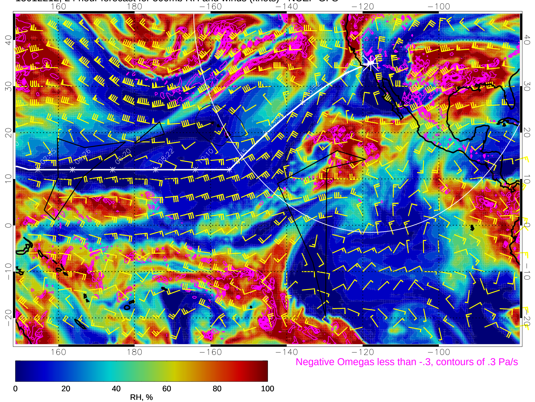
15012212, 24 hour forecast for 500mb RH and winds (knots) - NCEP GFS
