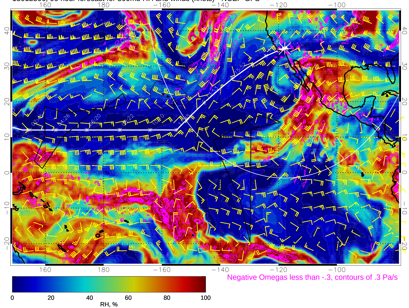
15012506, 90 hour forecast for 500mb RH and winds (knots) - NCEP GFS
