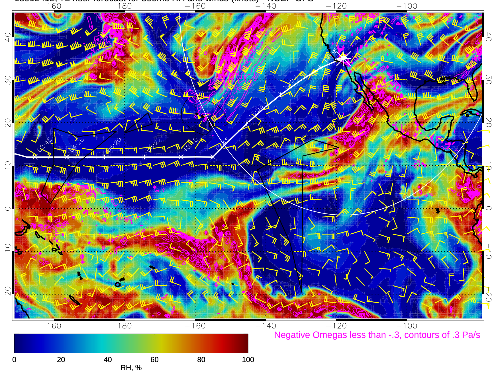
15012412, 72 hour forecast for 500mb RH and winds (knots) - NCEP GFS
