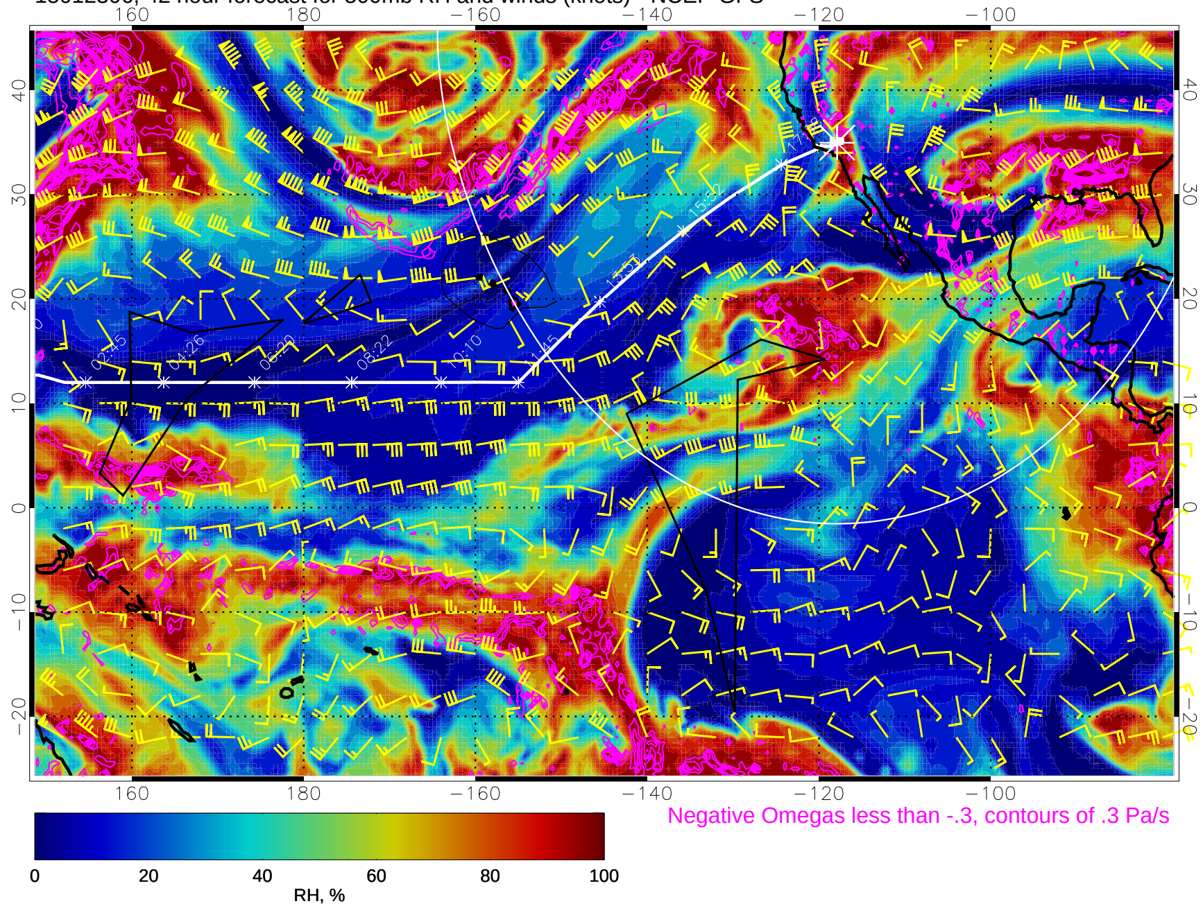
15012306, 42 hour forecast for 500mb RH and winds (knots) - NCEP GFS
