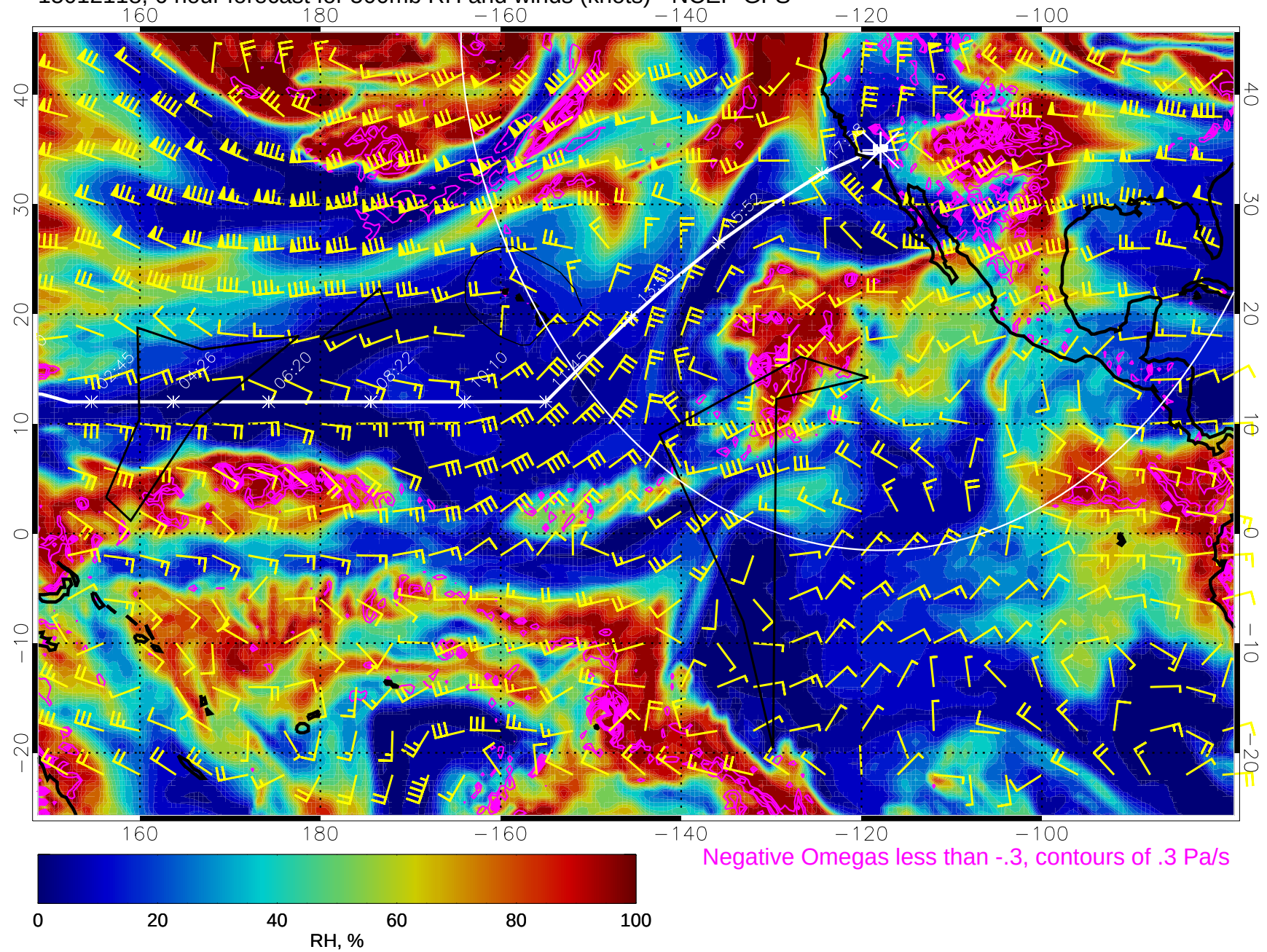
15012118, 6 hour forecast for 500mb RH and winds (knots) - NCEP GFS
