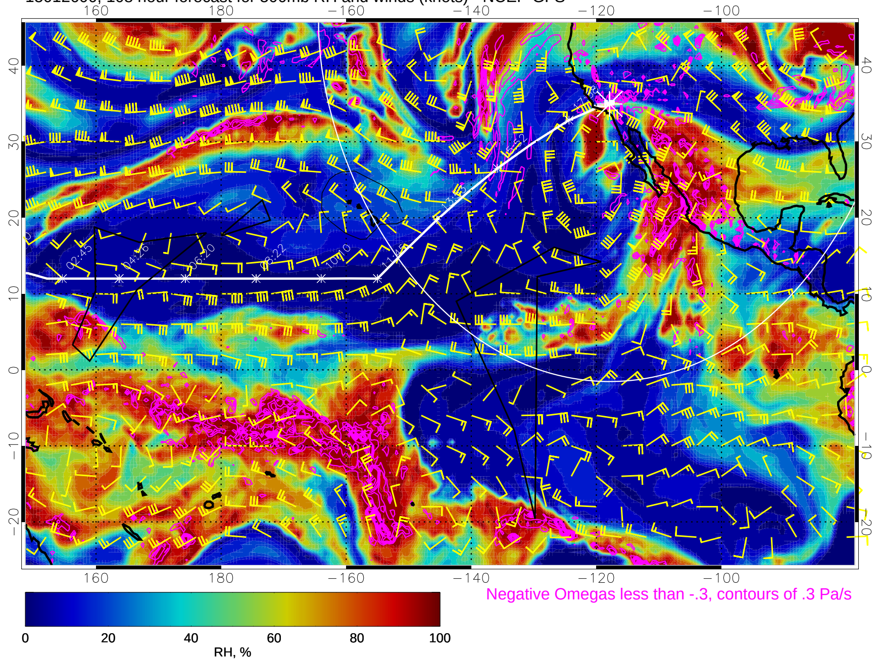
15012600, 108 hour forecast for 500mb RH and winds (knots) - NCEP GFS
