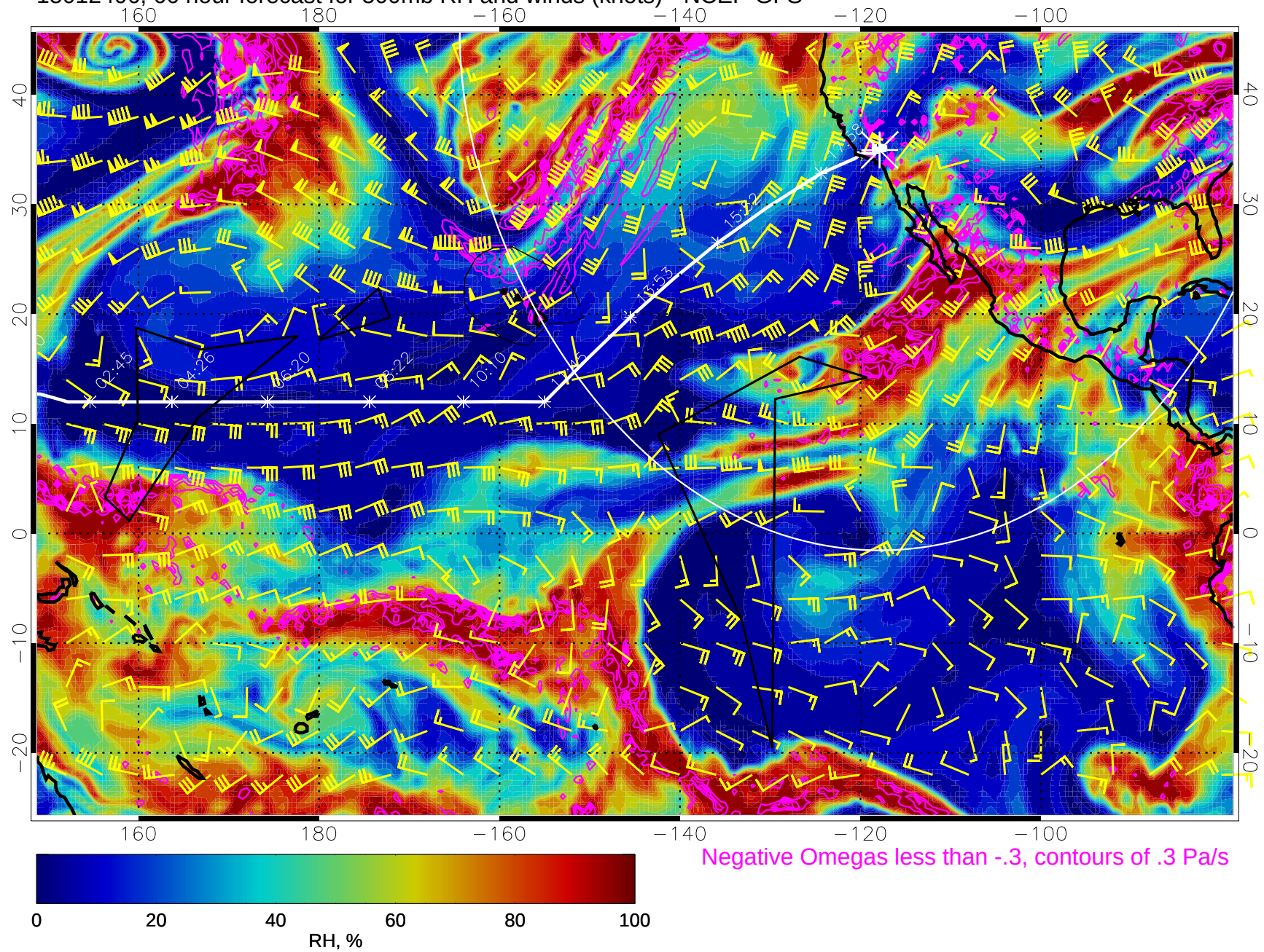
15012406, 66 hour forecast for 500mb RH and winds (knots) - NCEP GFS
