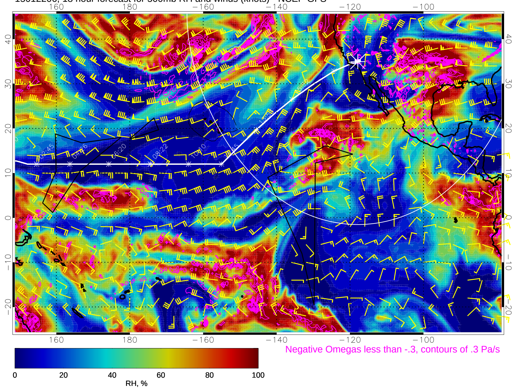
15012206, 18 hour forecast for 500mb RH and winds (knots) - NCEP GFS
