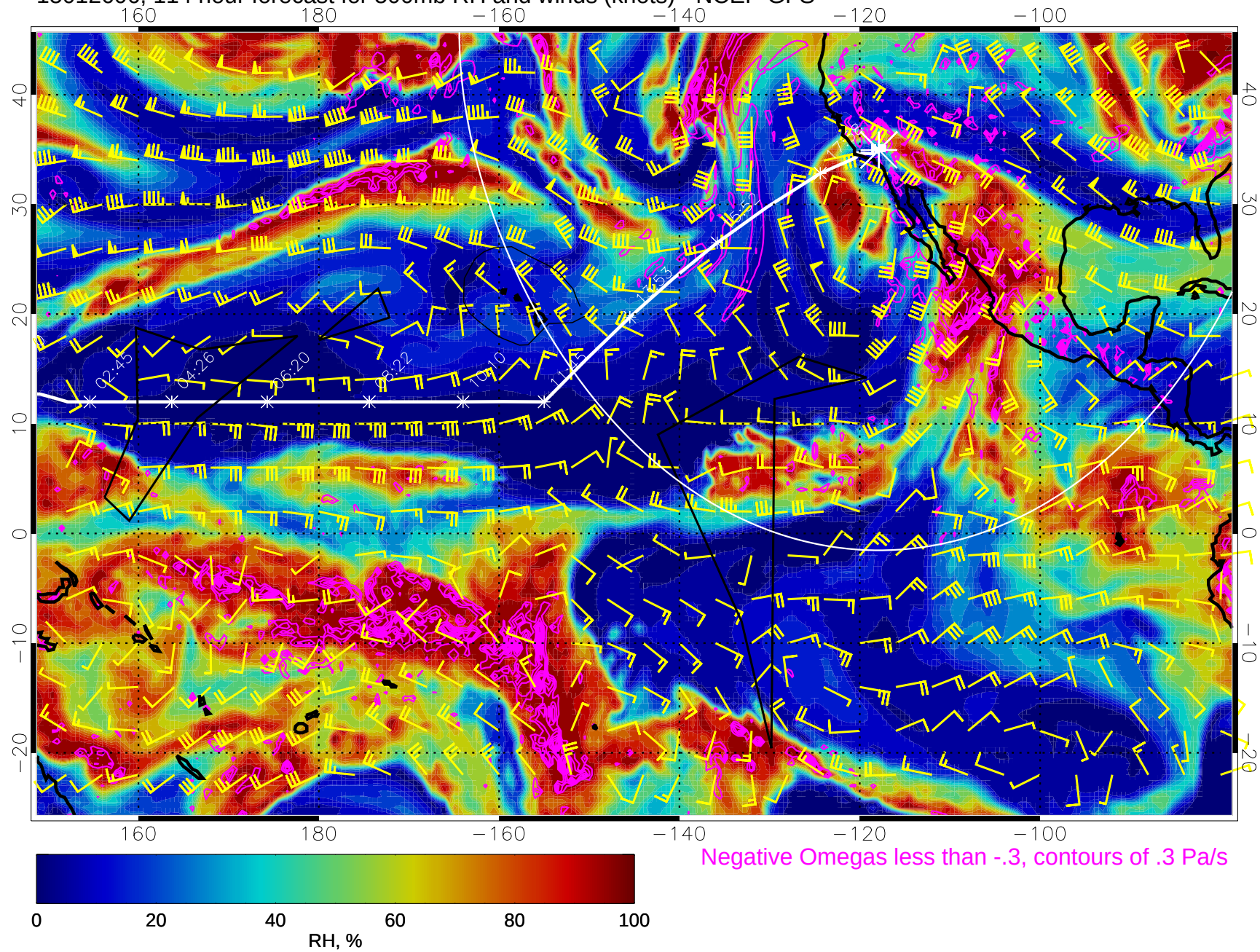
15012606, 114 hour forecast for 500mb RH and winds (knots) - NCEP GFS
