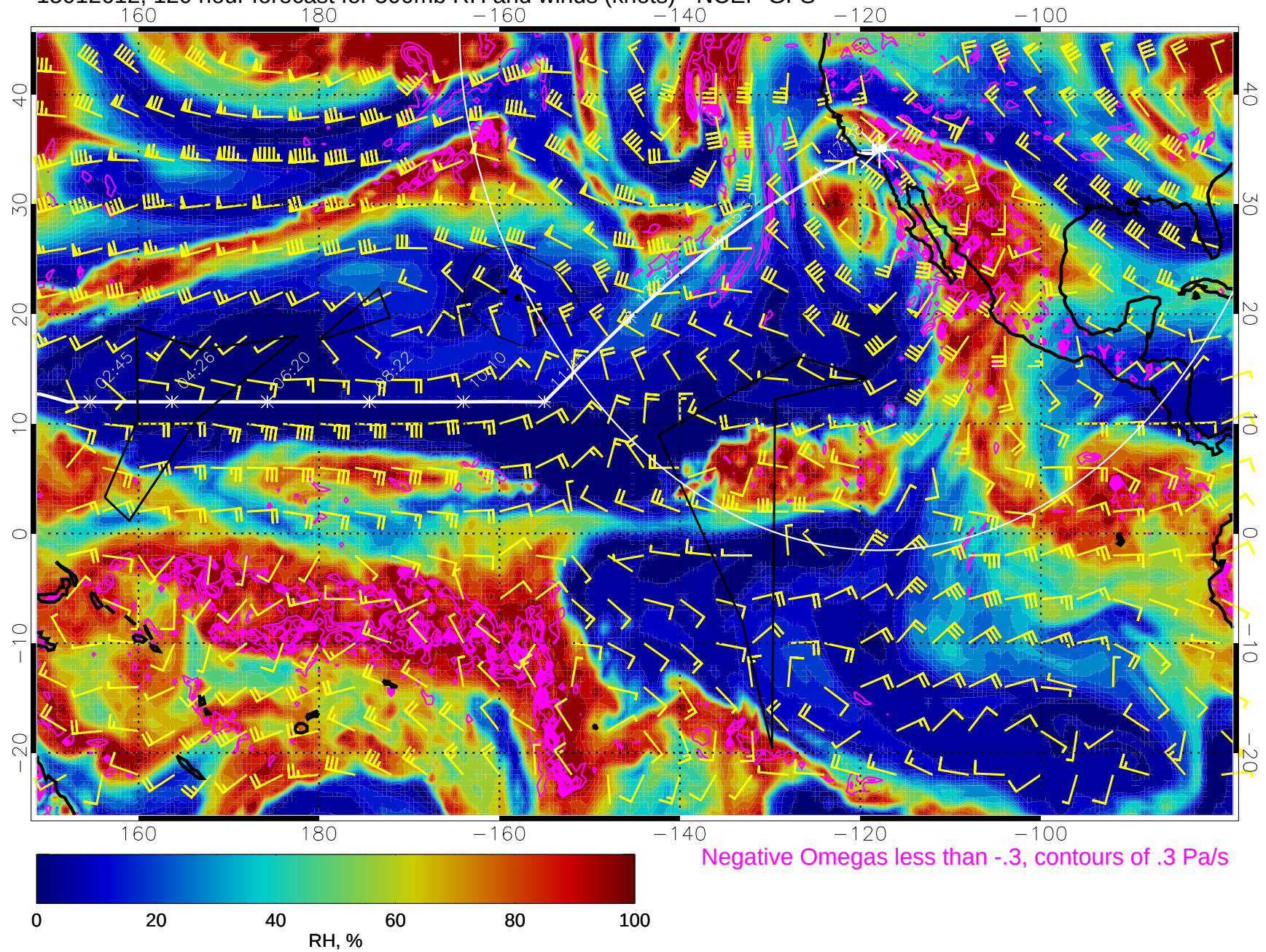
15012612, 120 hour forecast for 500mb RH and winds (knots) - NCEP GFS
