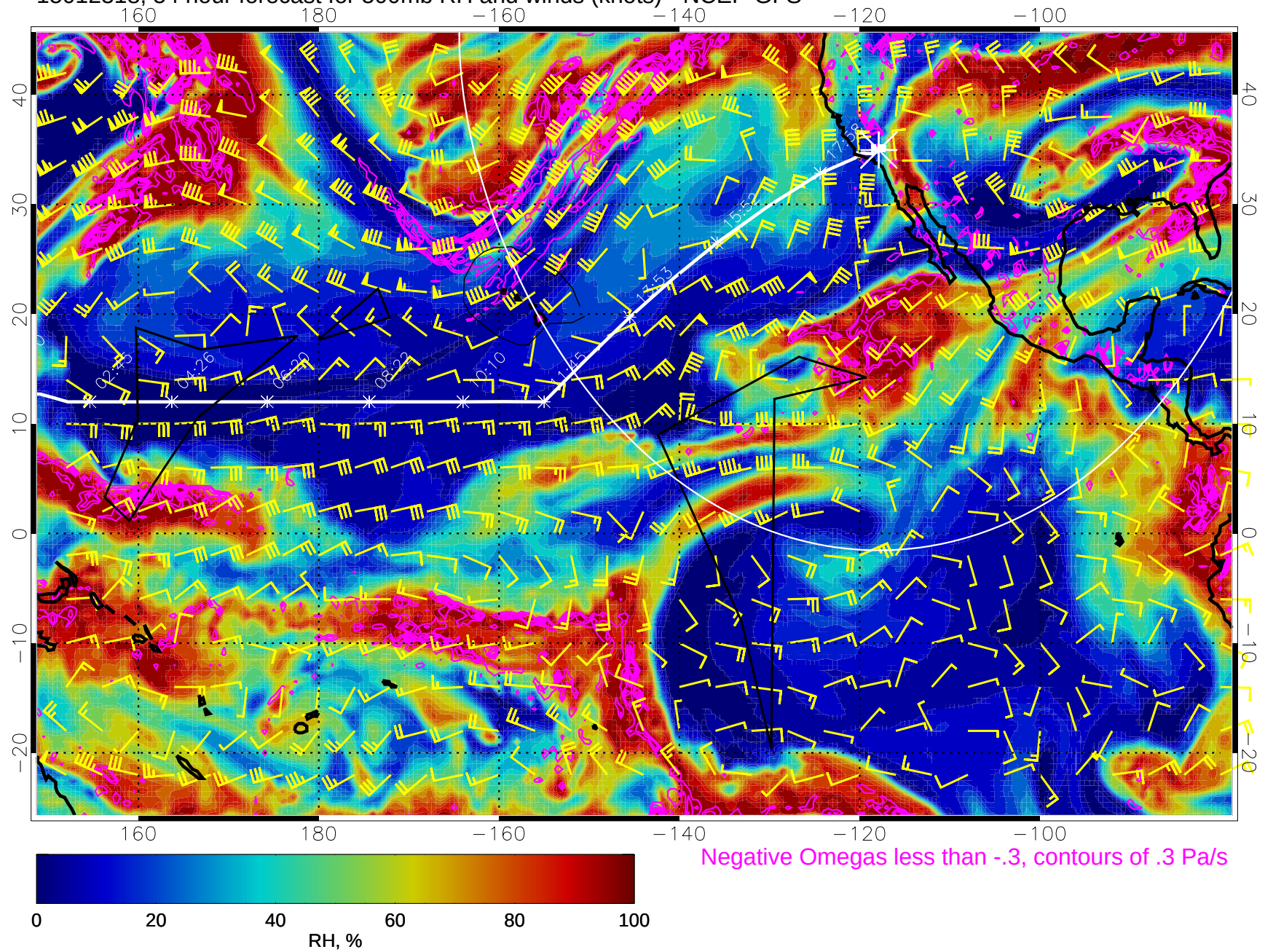
15012318, 54 hour forecast for 500mb RH and winds (knots) - NCEP GFS
