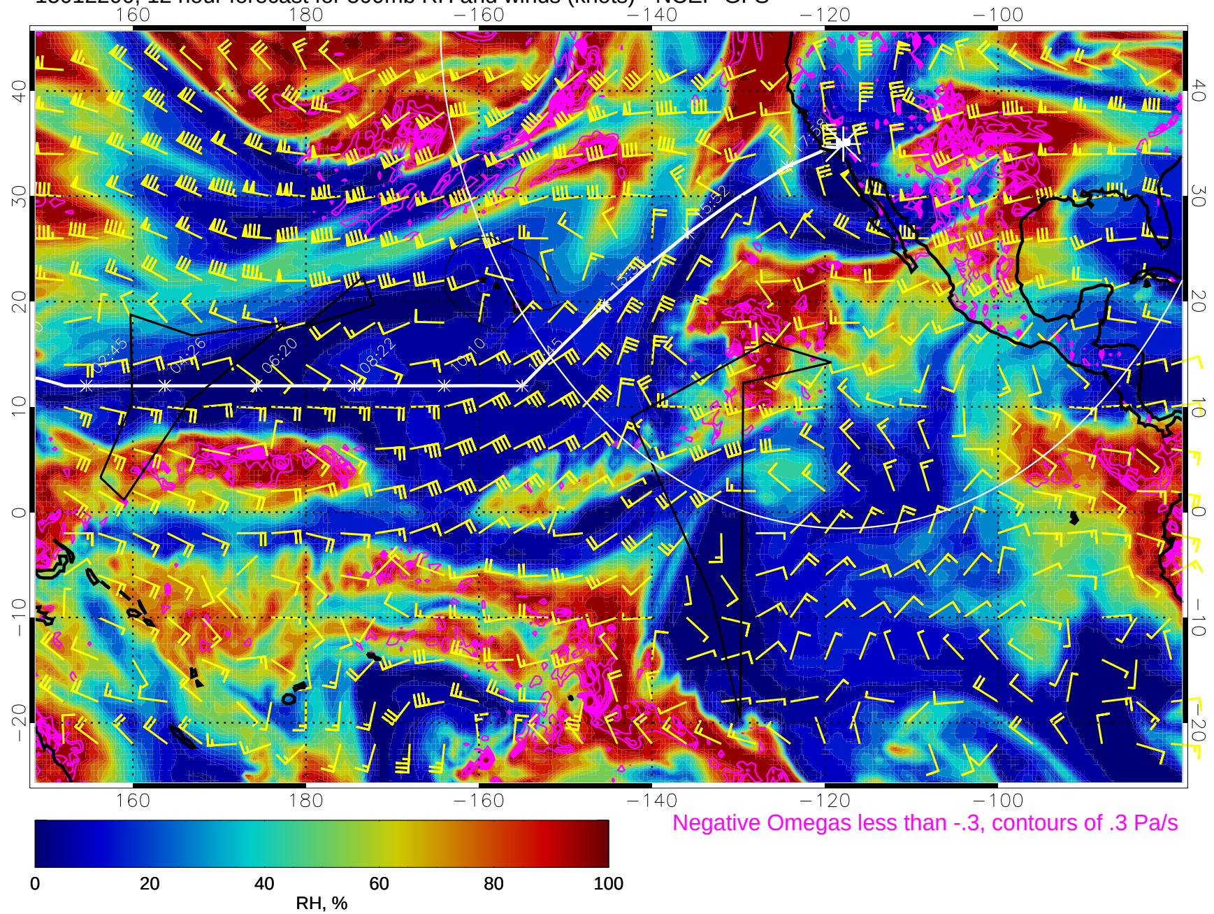
15012200, 12 hour forecast for 500mb RH and winds (knots) - NCEP GFS
