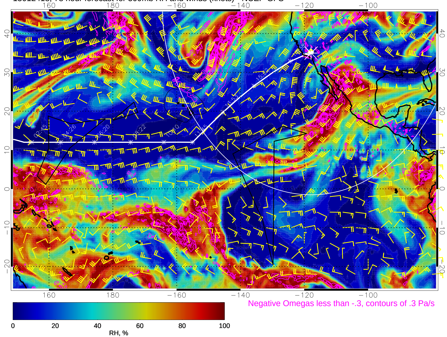
15012418, 78 hour forecast for 500mb RH and winds (knots) - NCEP GFS
