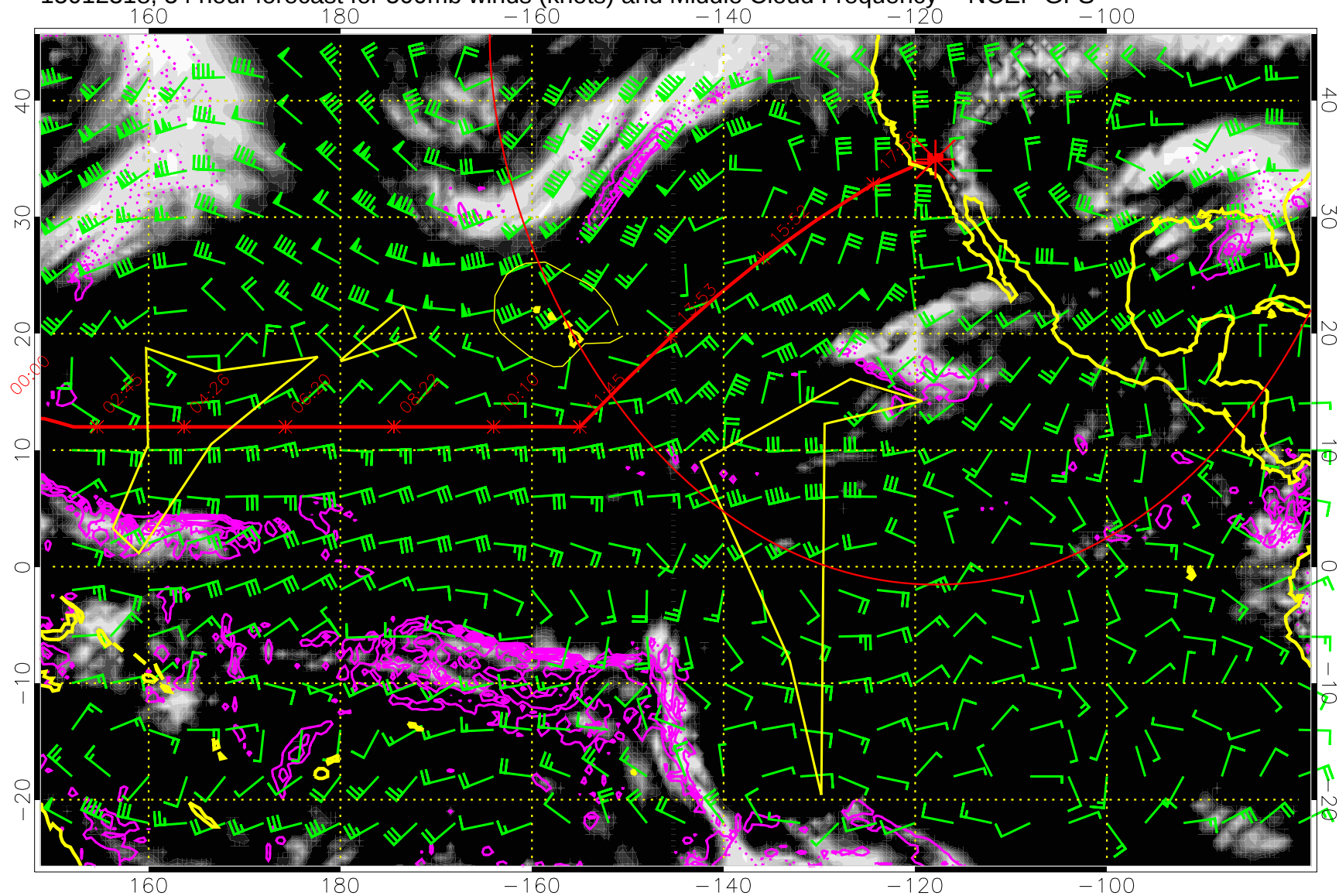
15012318, 54 hour forecast for 500mb winds (knots) and Middle Cloud Frequency -- NCEP GFS
