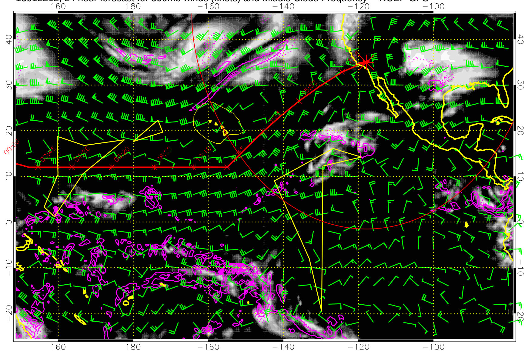
15012212, 24 hour forecast for 500mb winds (knots) and Middle Cloud Frequency -- NCEP GFS
