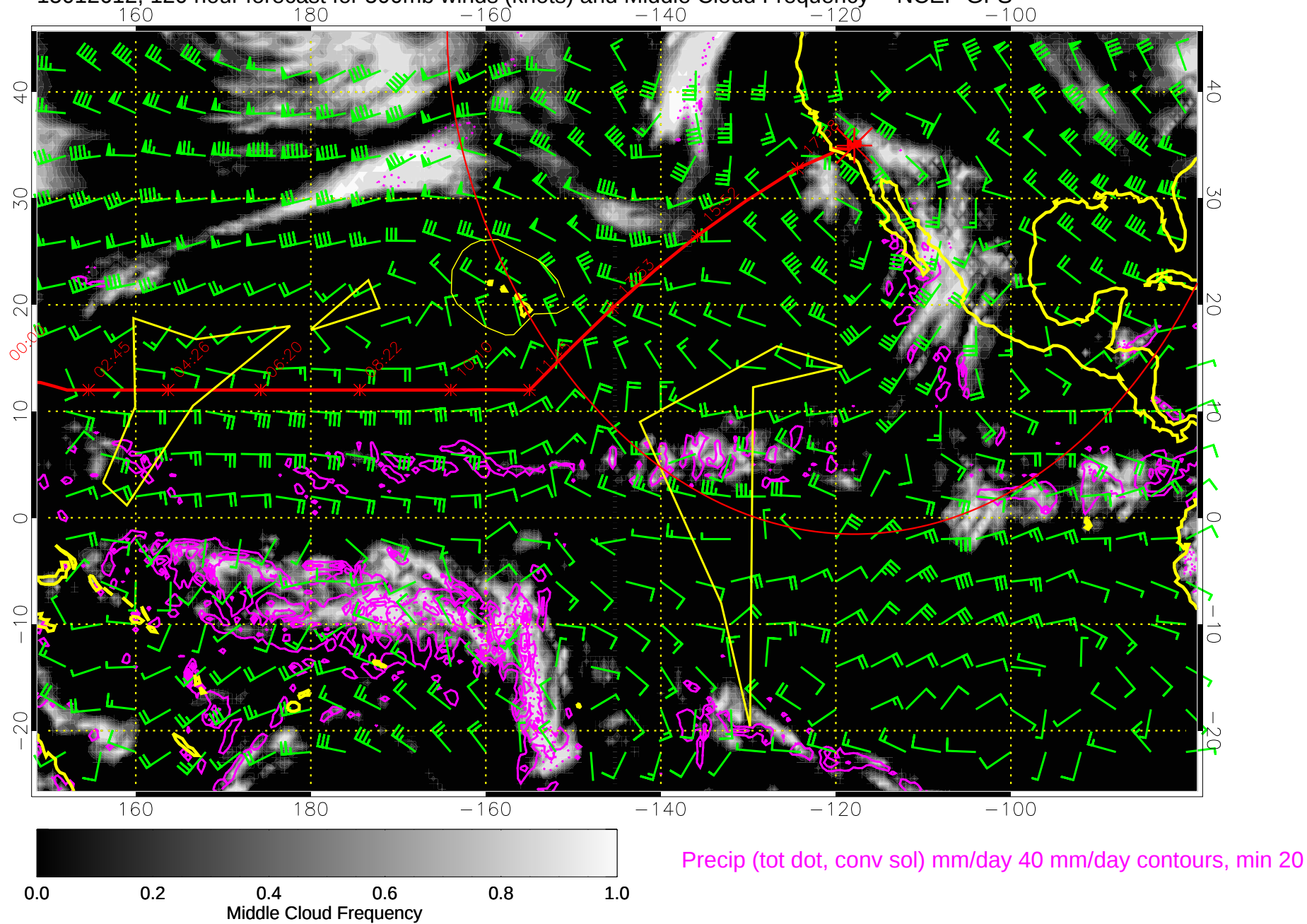
15012612, 120 hour forecast for 500mb winds (knots) and Middle Cloud Frequency -- NCEP GFS
