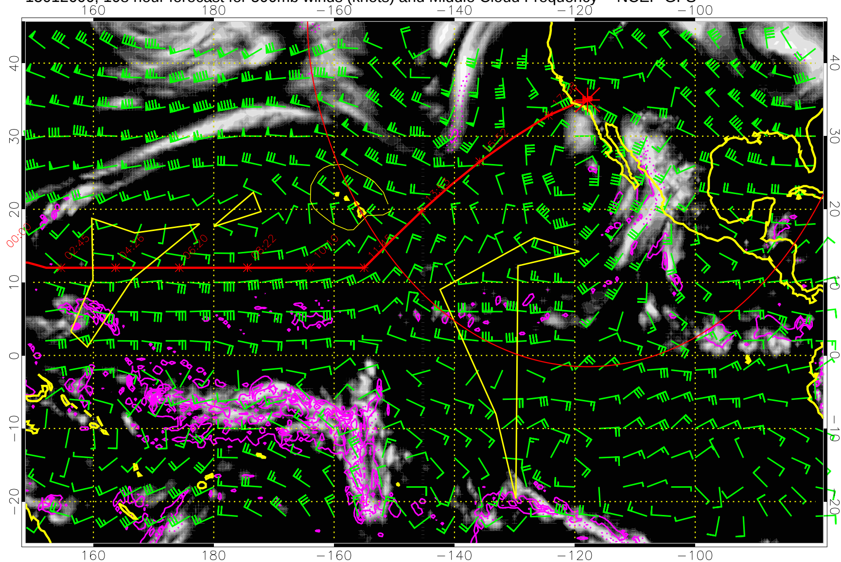
15012600, 108 hour forecast for 500mb winds (knots) and Middle Cloud Frequency -- NCEP GFS
