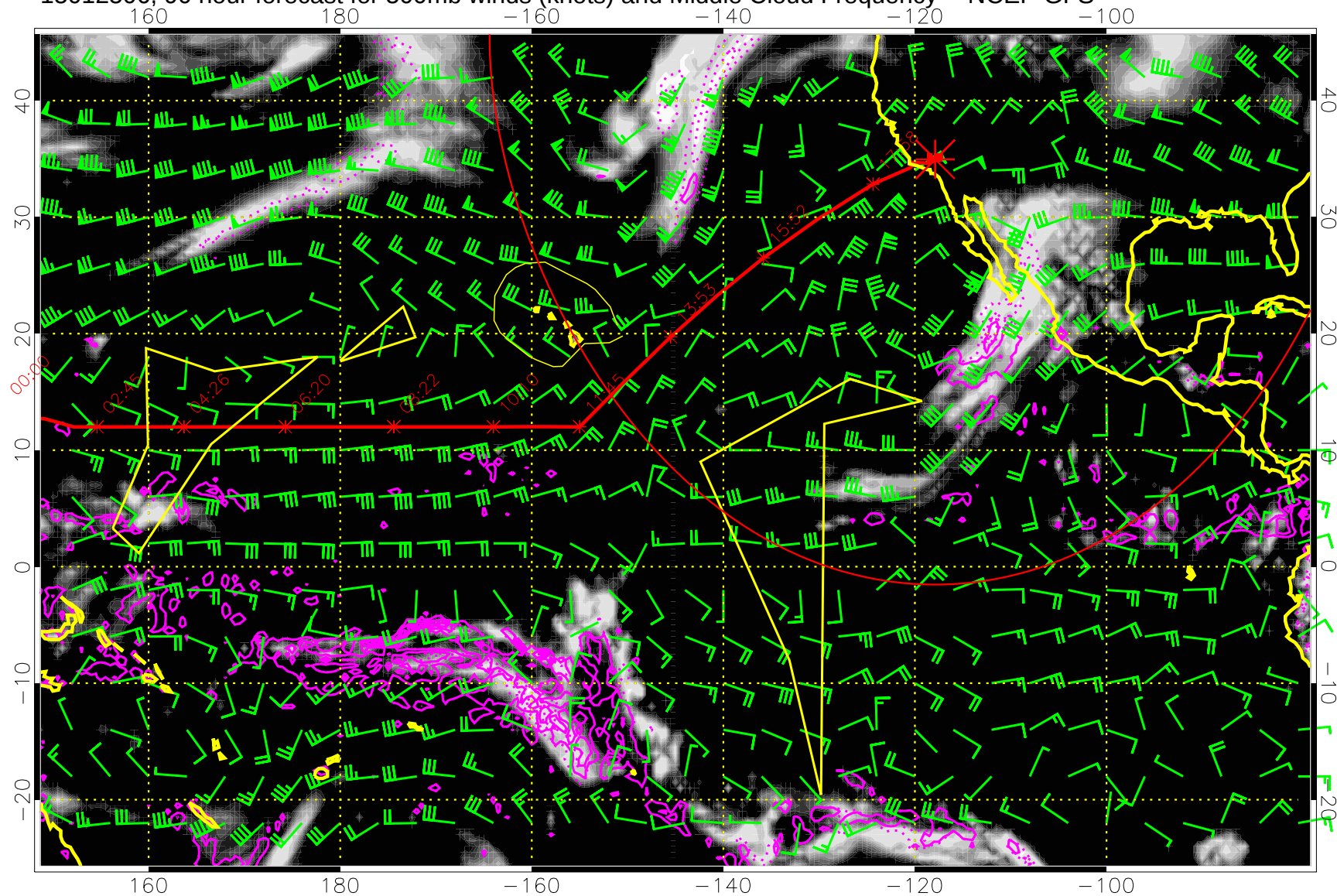
15012506, 90 hour forecast for 500mb winds (knots) and Middle Cloud Frequency -- NCEP GFS
