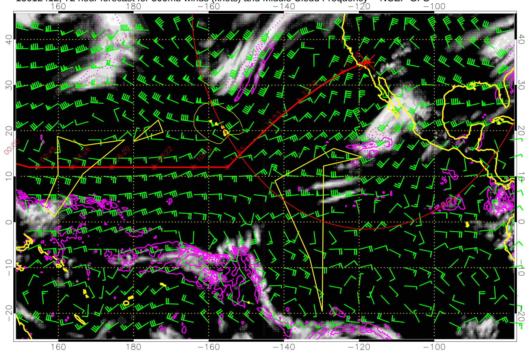
15012412, 72 hour forecast for 500mb winds (knots) and Middle Cloud Frequency -- NCEP GFS
