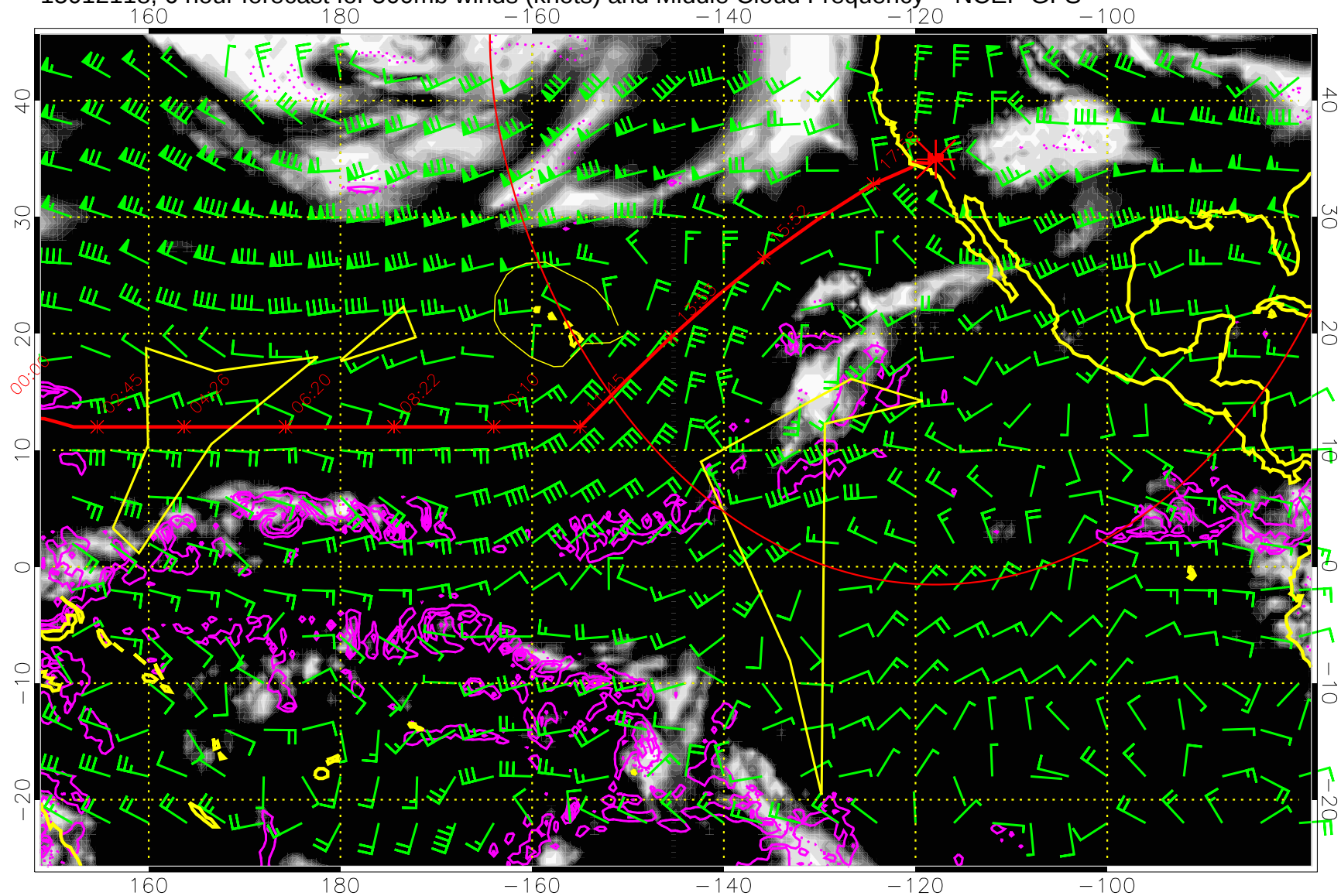
15012118, 6 hour forecast for 500mb winds (knots) and Middle Cloud Frequency -- NCEP GFS
