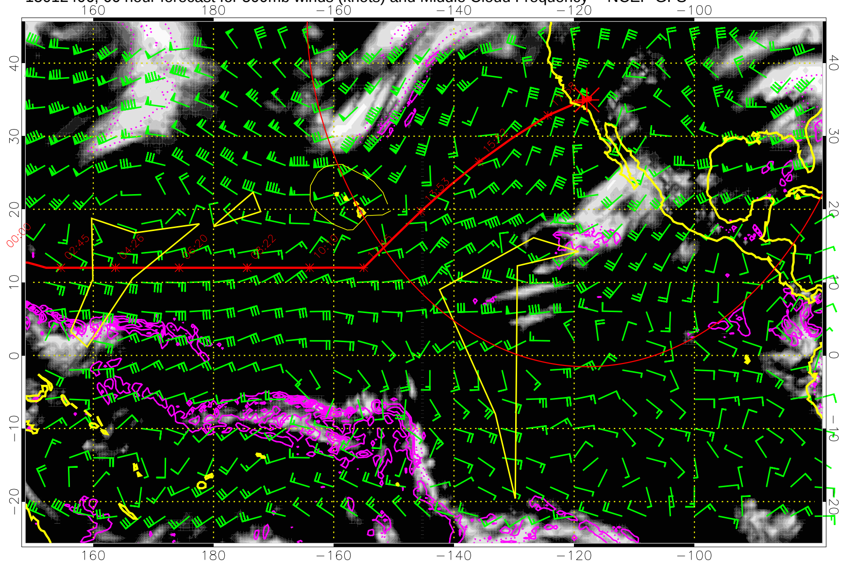
15012406, 66 hour forecast for 500mb winds (knots) and Middle Cloud Frequency -- NCEP GFS
