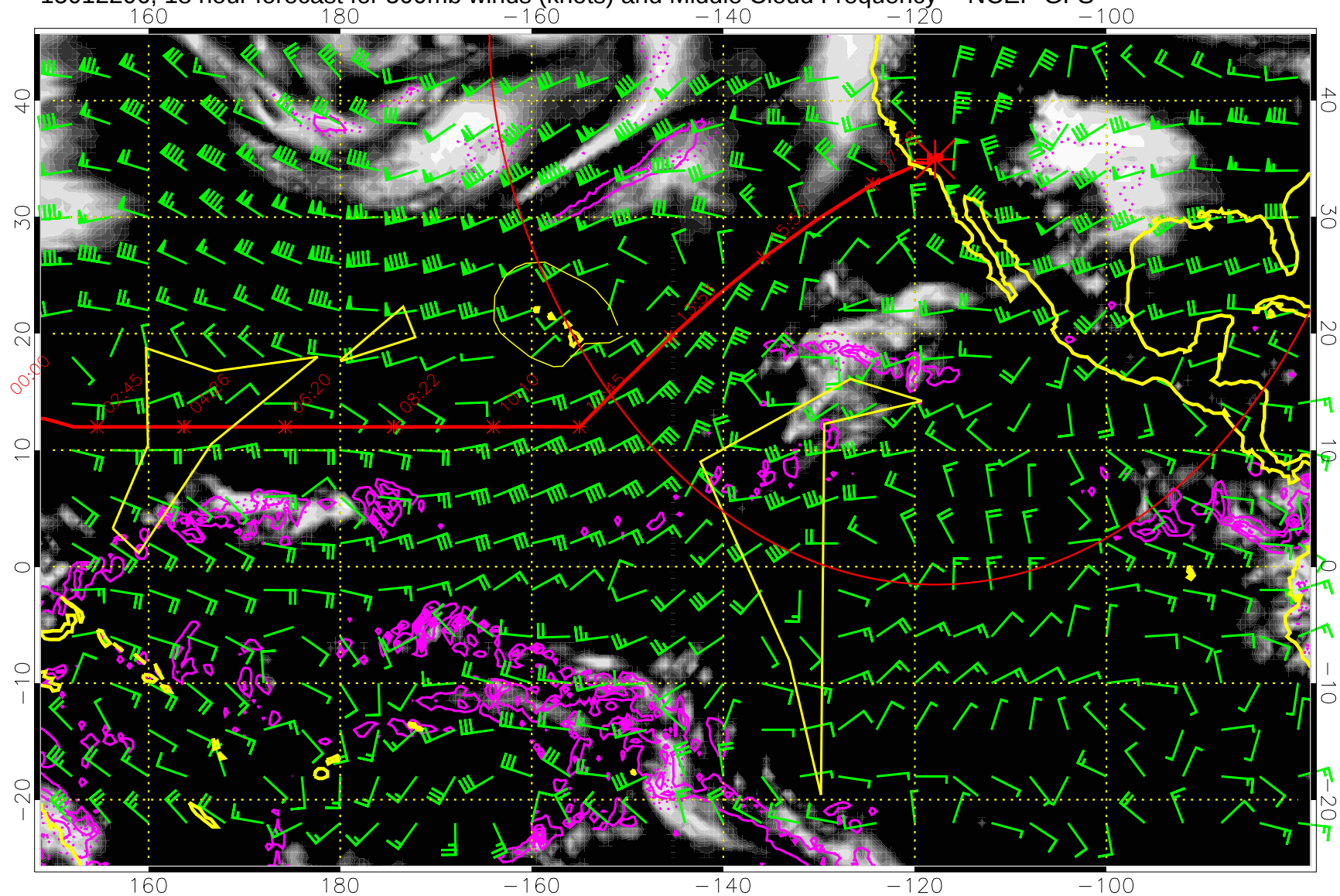
15012206, 18 hour forecast for 500mb winds (knots) and Middle Cloud Frequency -- NCEP GFS
