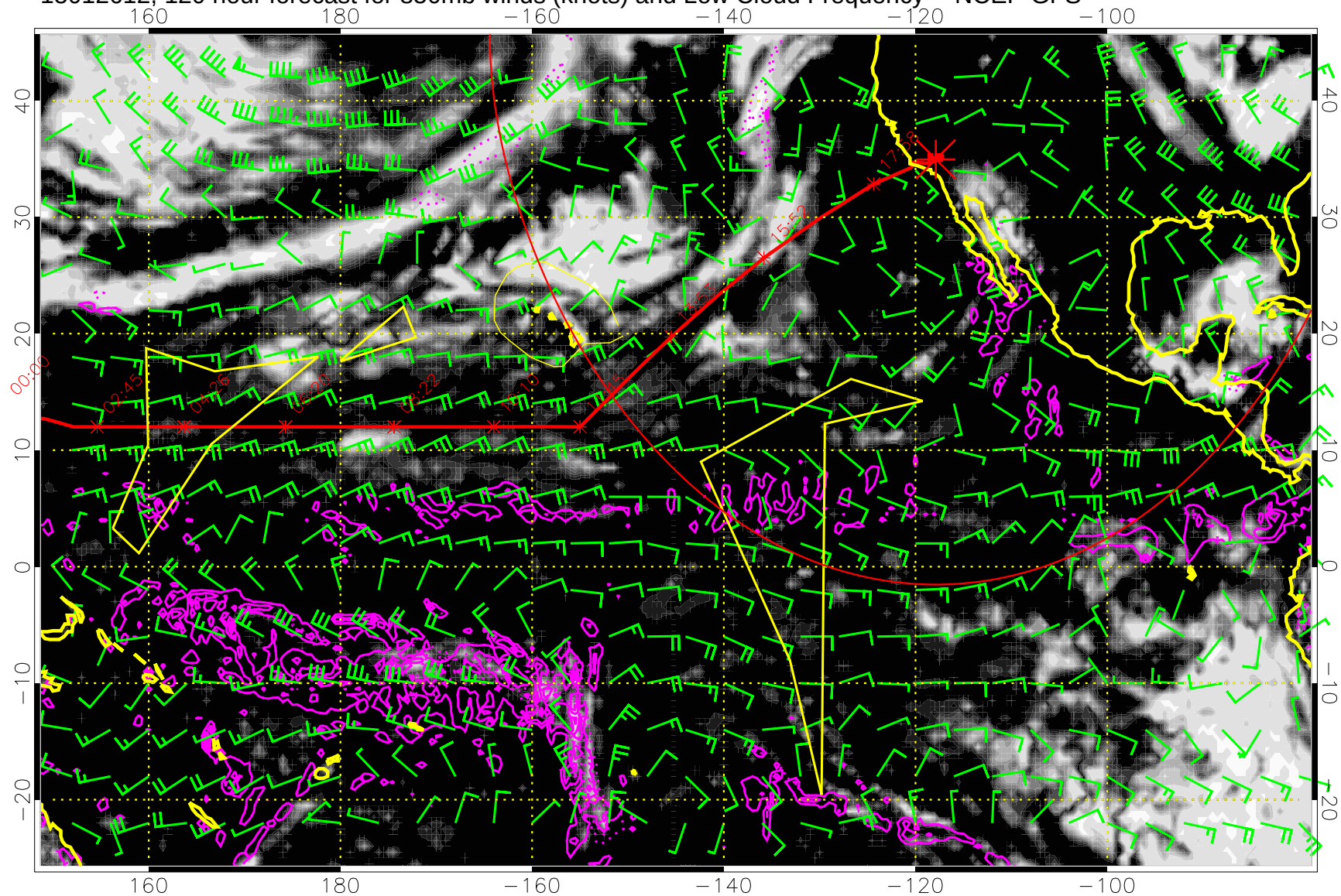
15012612, 120 hour forecast for 850mb winds (knots) and Low Cloud Frequency -- NCEP GFS
