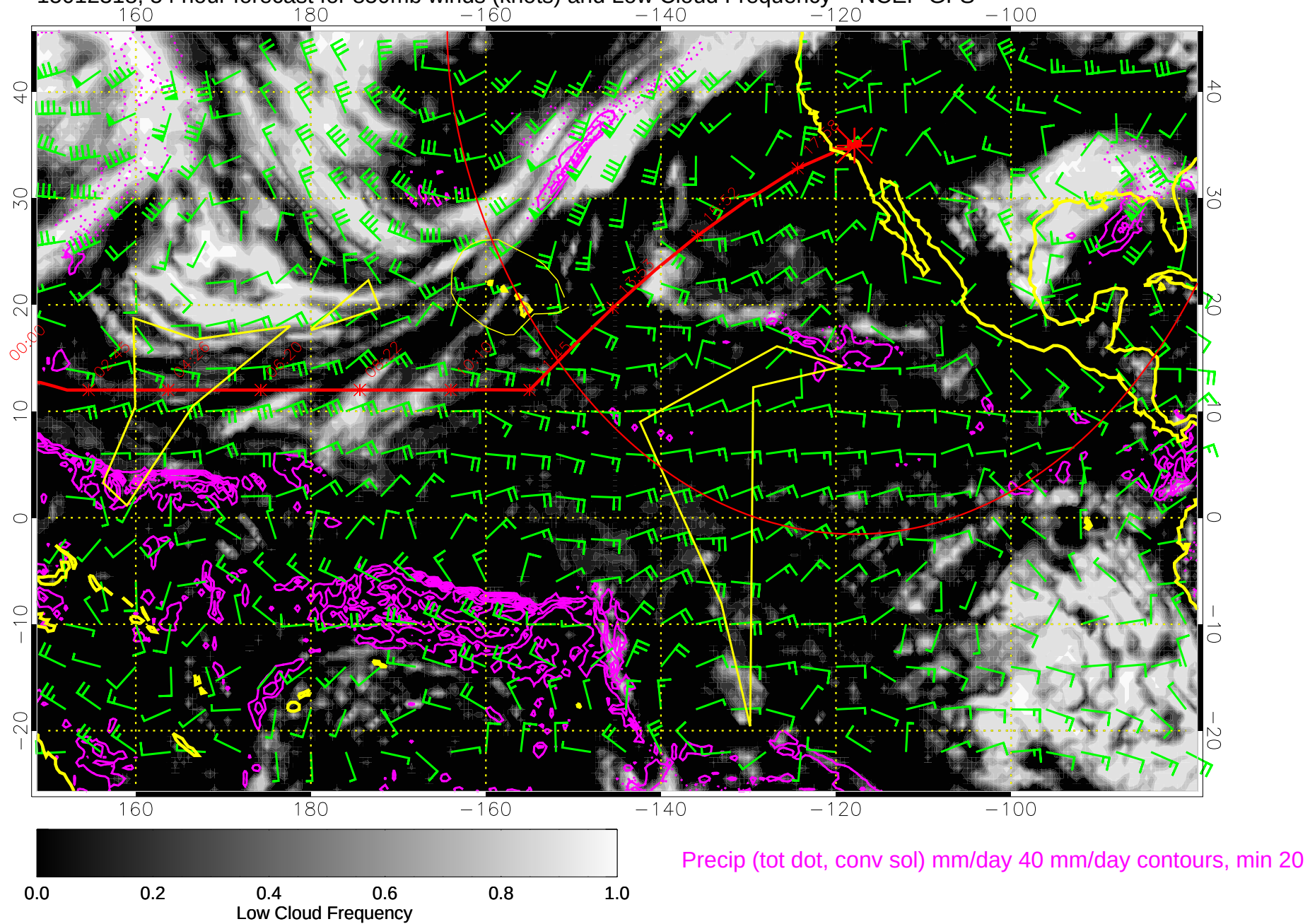
15012318, 54 hour forecast for 850mb winds (knots) and Low Cloud Frequency -- NCEP GFS
