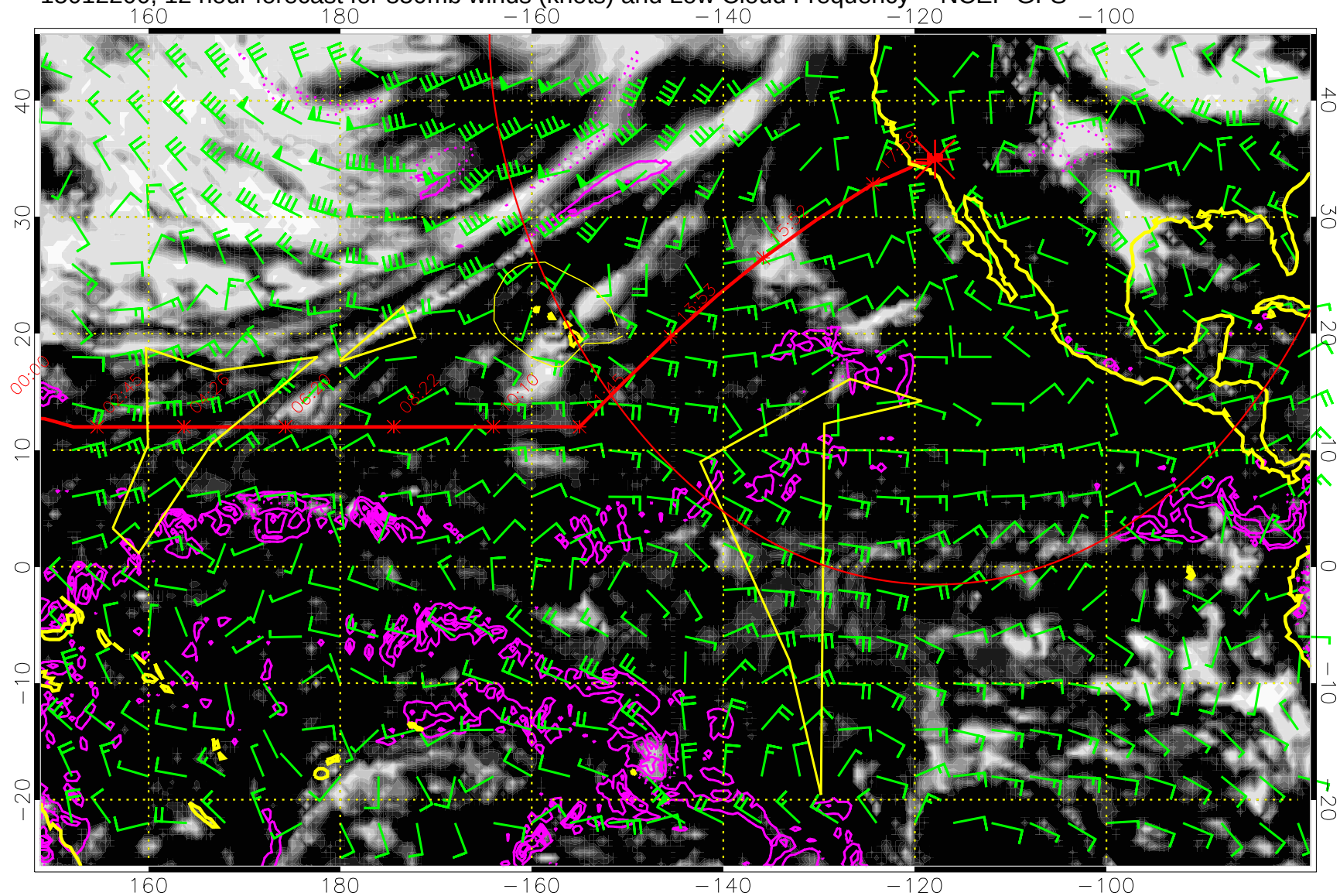
15012200, 12 hour forecast for 850mb winds (knots) and Low Cloud Frequency -- NCEP GFS
