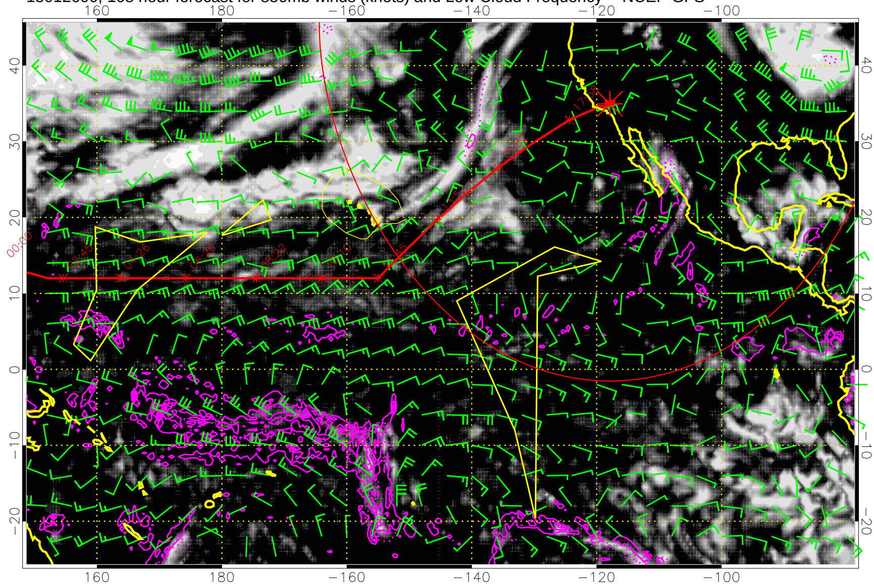
15012600, 108 hour forecast for 850mb winds (knots) and Low Cloud Frequency -- NCEP GFS
