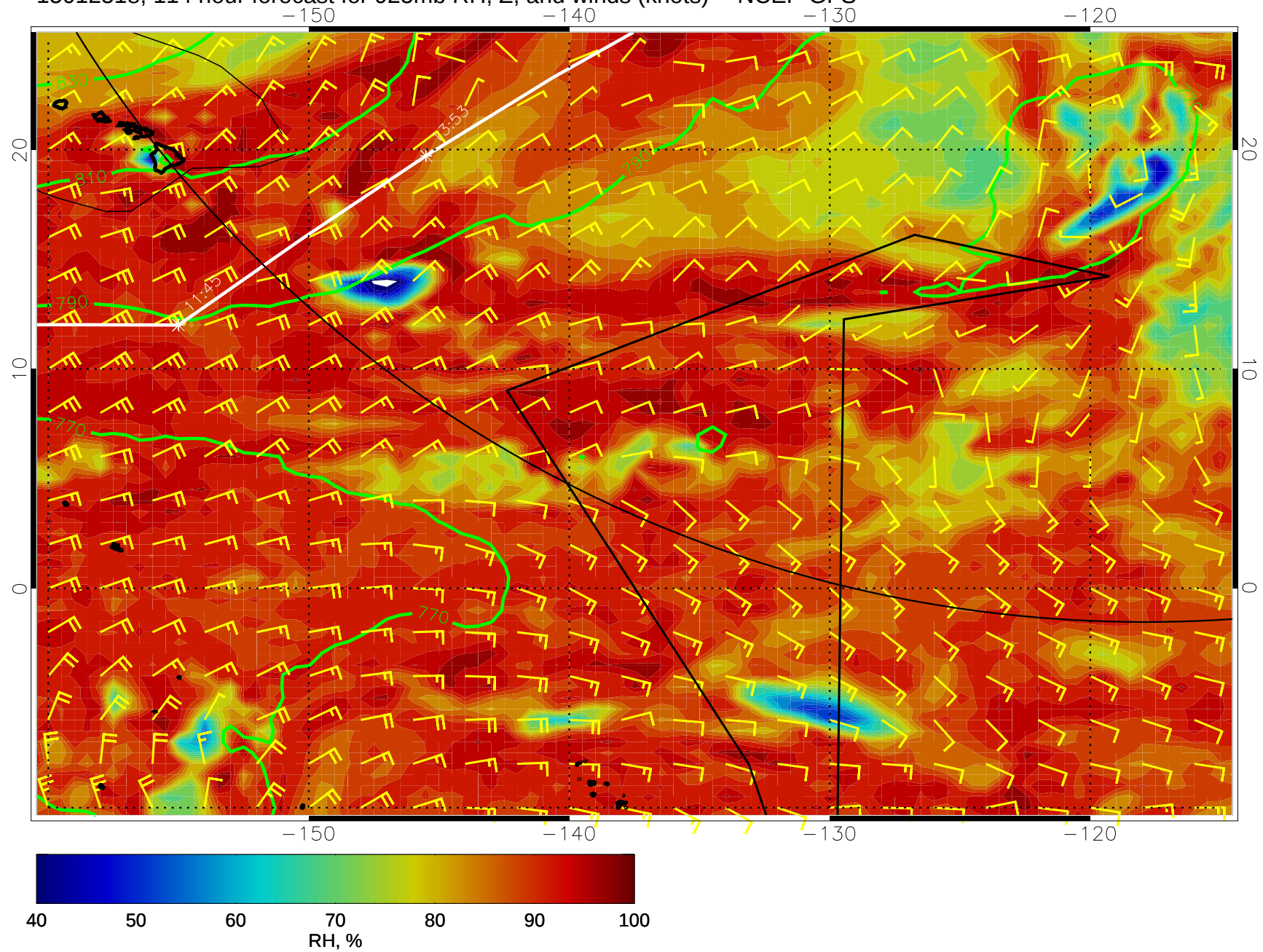
15012518, 114 hour forecast for 925mb RH, Z, and winds (knots) -- NCEP GFS
