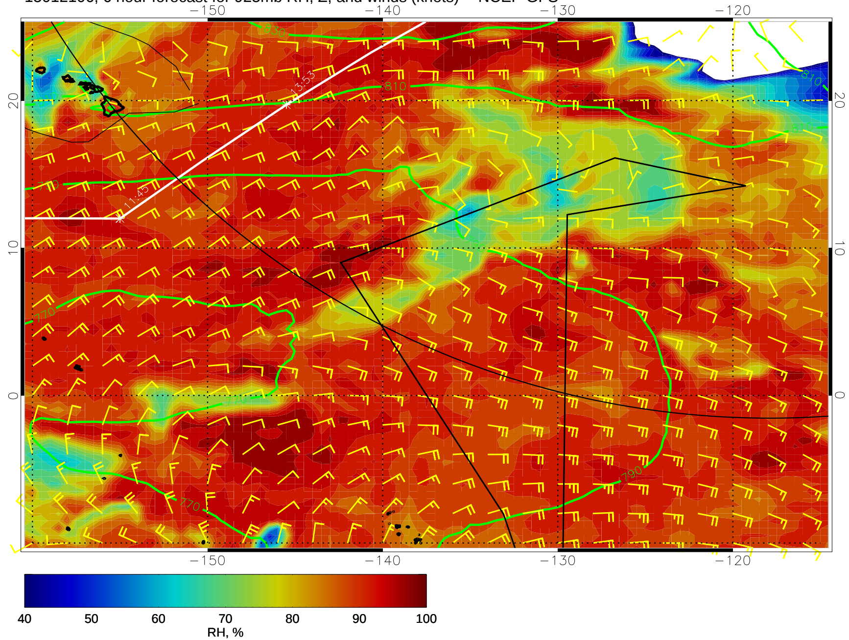
15012106, 6 hour forecast for 925mb RH, Z, and winds (knots) -- NCEP GFS
