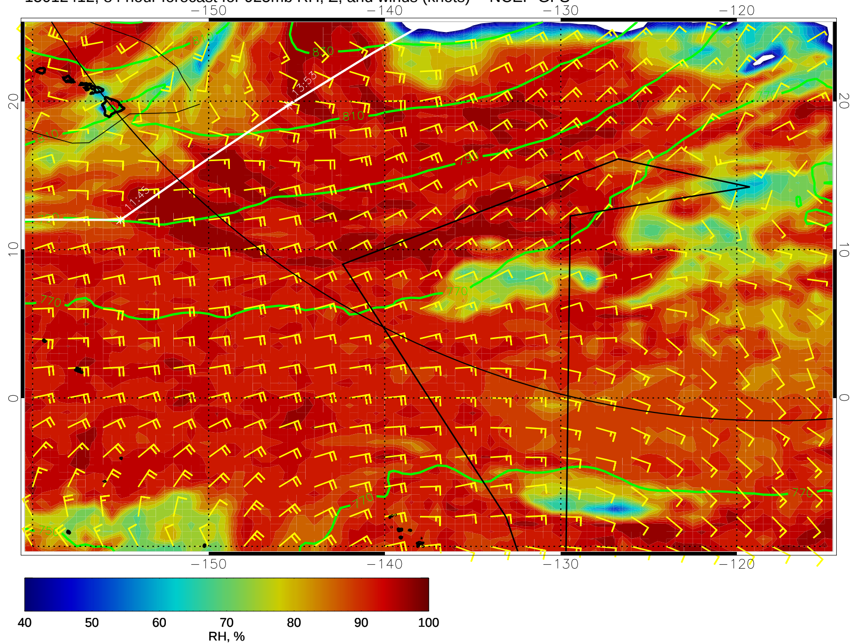
15012412, 84 hour forecast for 925mb RH, Z, and winds (knots) -- NCEP GFS
