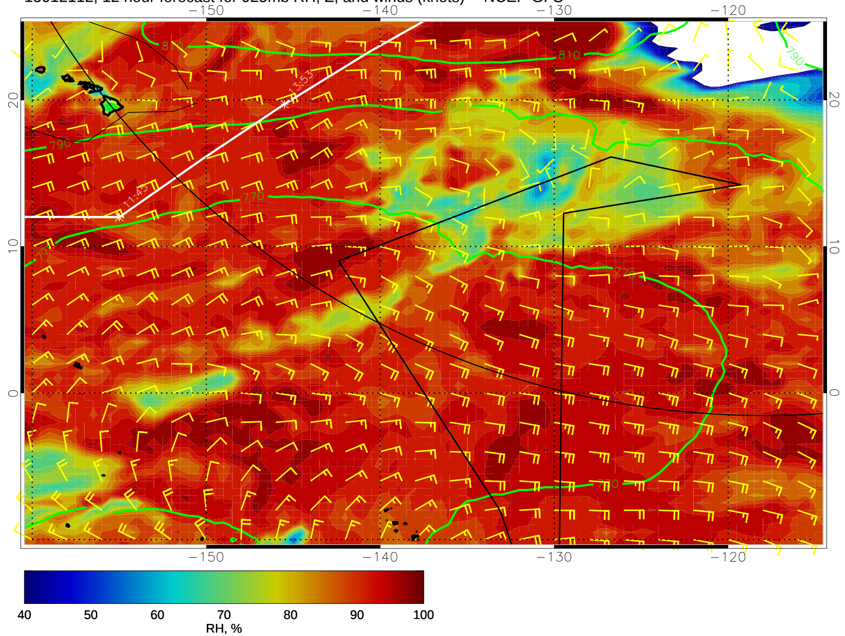
15012112, 12 hour forecast for 925mb RH, Z, and winds (knots) -- NCEP GFS
