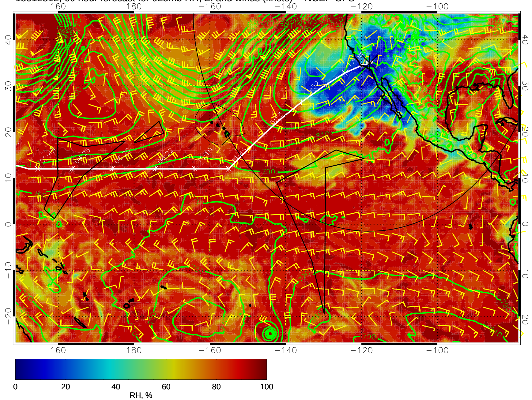
15012312, 60 hour forecast for 925mb RH, Z, and winds (knots) -- NCEP GFS
