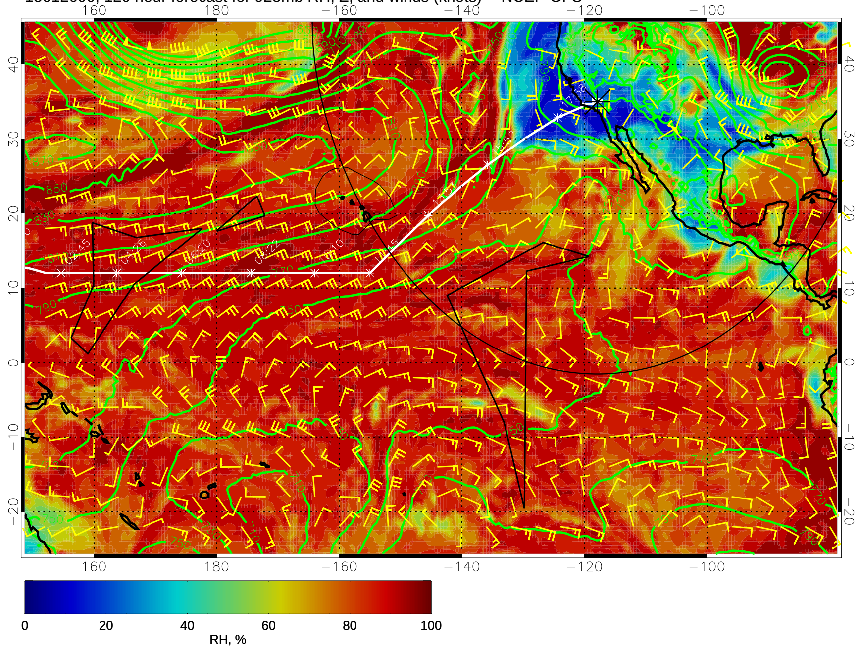
15012600, 120 hour forecast for 925mb RH, Z, and winds (knots) -- NCEP GFS
