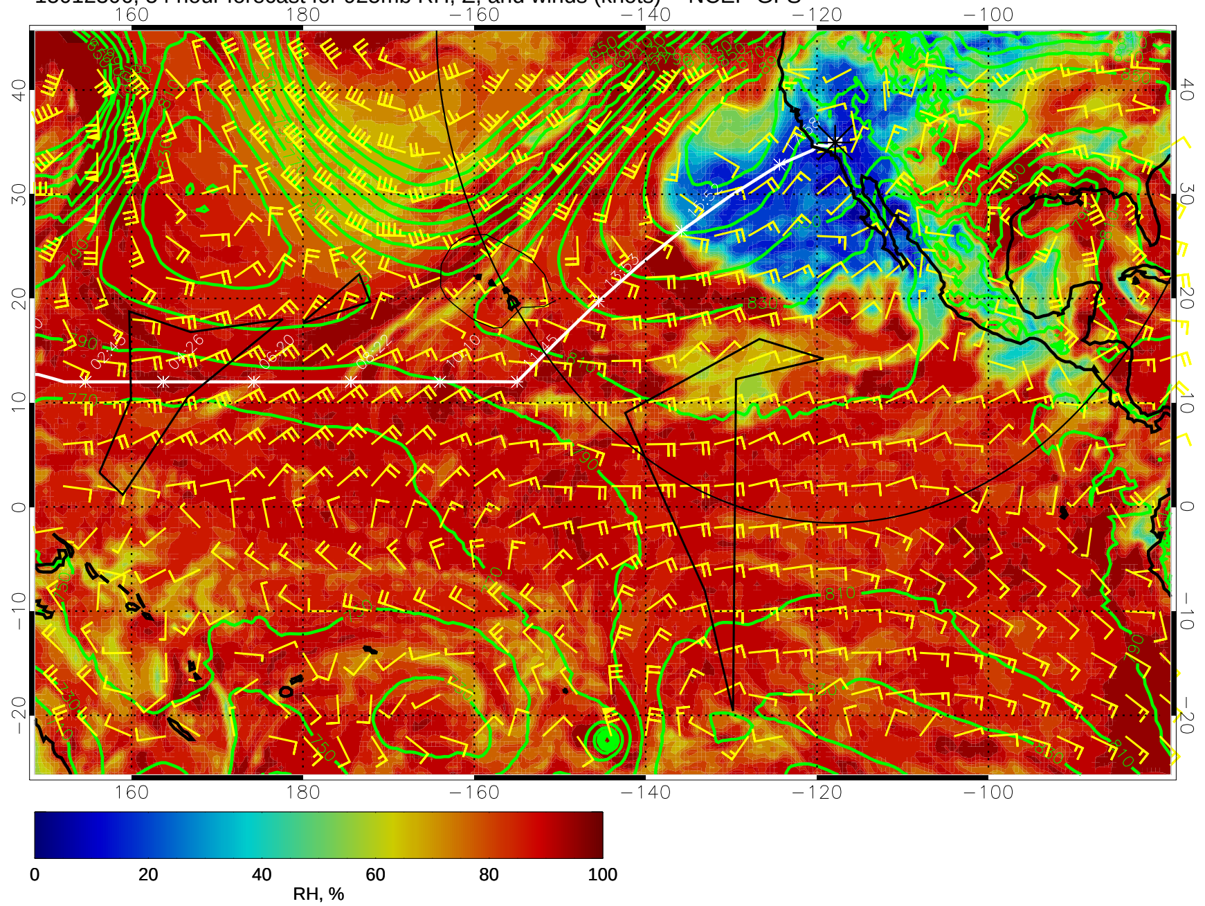
15012306, 54 hour forecast for 925mb RH, Z, and winds (knots) -- NCEP GFS
