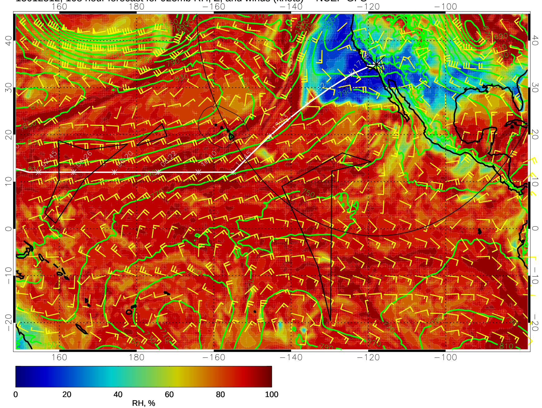
15012512, 108 hour forecast for 925mb RH, Z, and winds (knots) -- NCEP GFS
