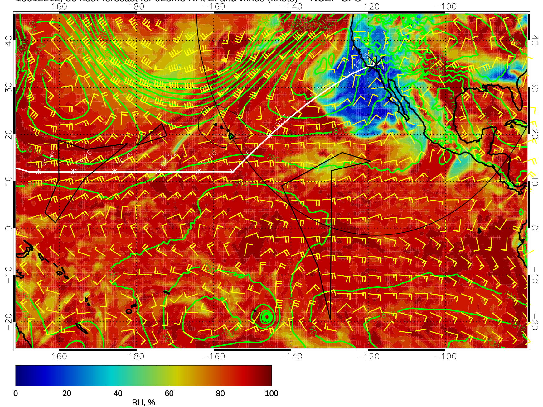
15012212, 36 hour forecast for 925mb RH, Z, and winds (knots) -- NCEP GFS
