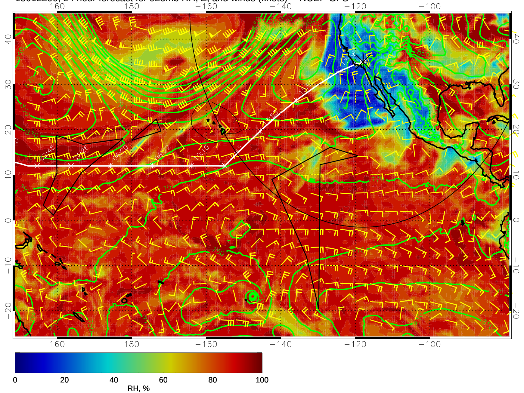
15012200, 24 hour forecast for 925mb RH, Z, and winds (knots) -- NCEP GFS
