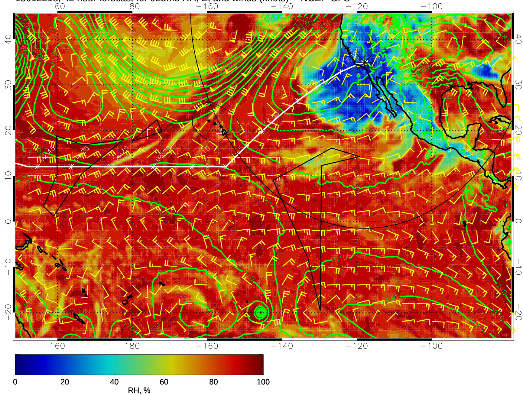
15012218, 42 hour forecast for 925mb RH, Z, and winds (knots) -- NCEP GFS
