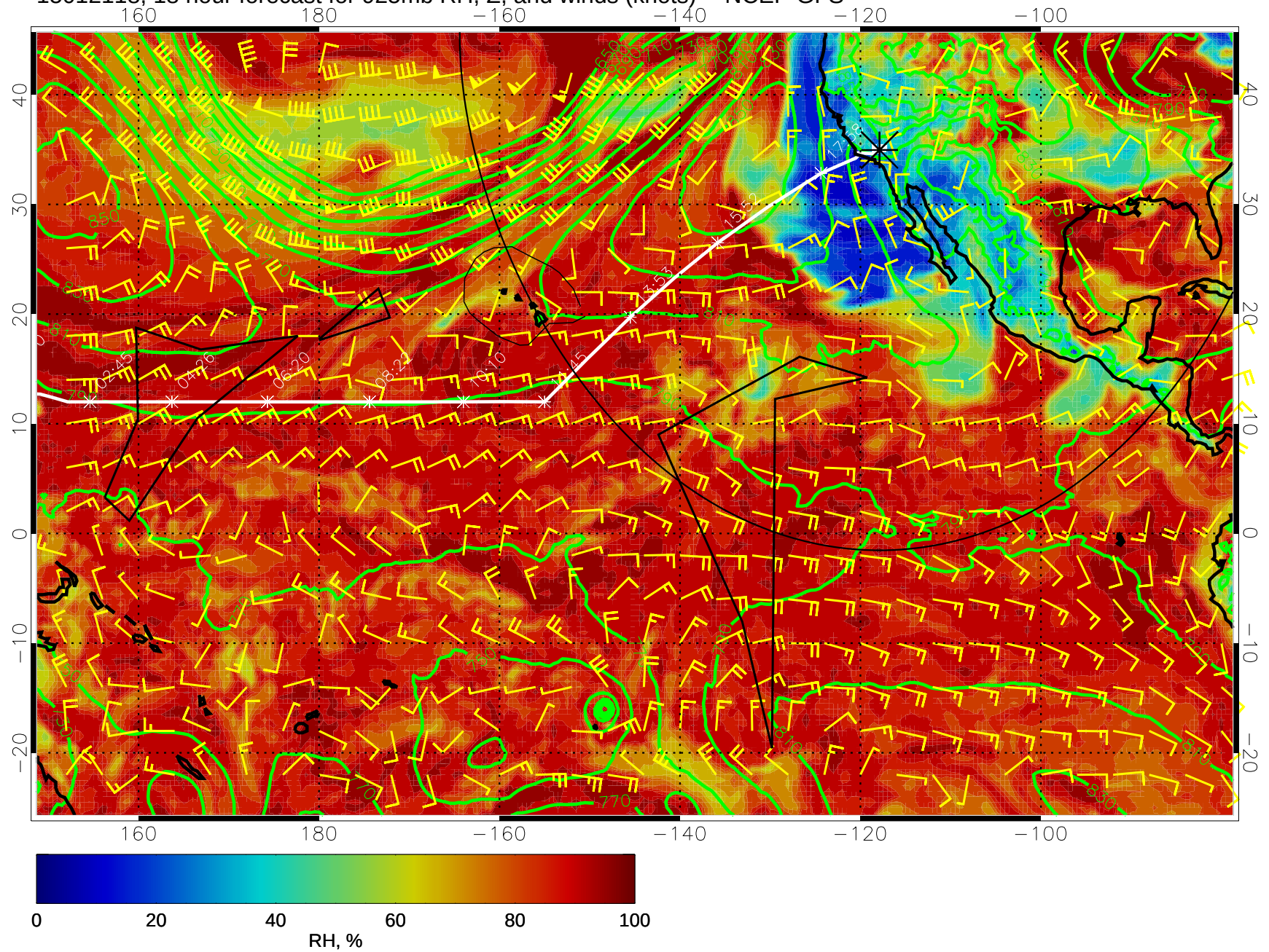
15012118, 18 hour forecast for 925mb RH, Z, and winds (knots) -- NCEP GFS
