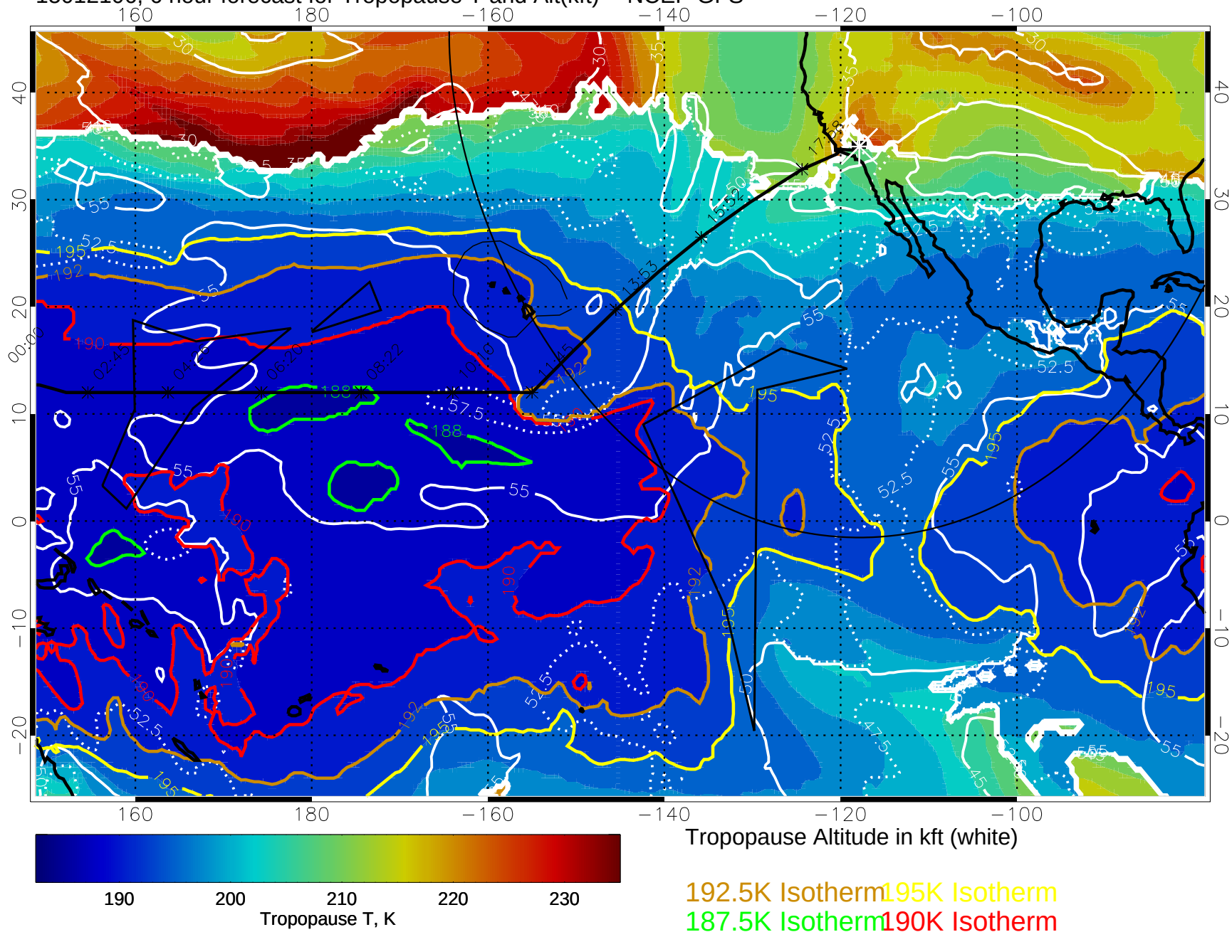
15012106, 6 hour forecast for Tropopause T and Alt(kft) -- NCEP GFS
