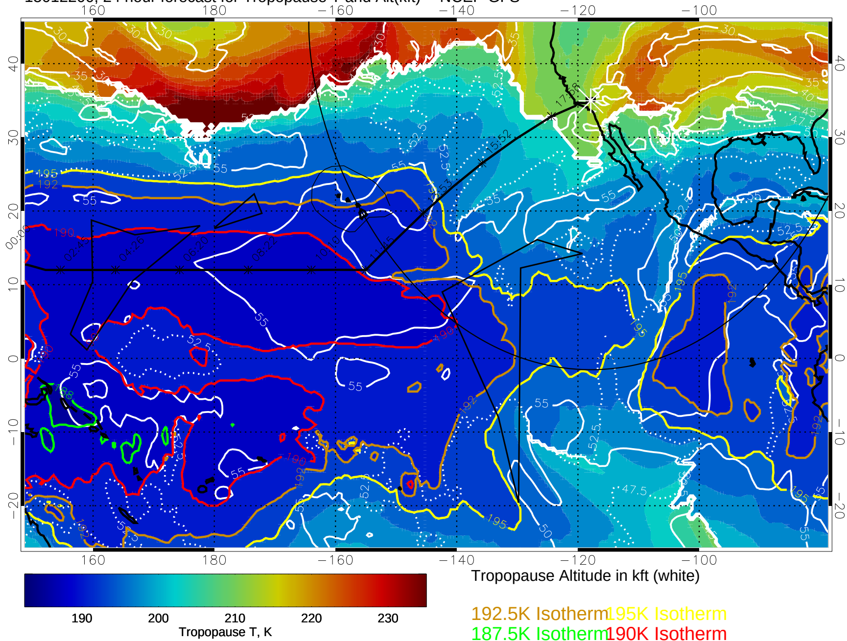
15012200, 24 hour forecast for Tropopause T and Alt(kft) -- NCEP GFS
