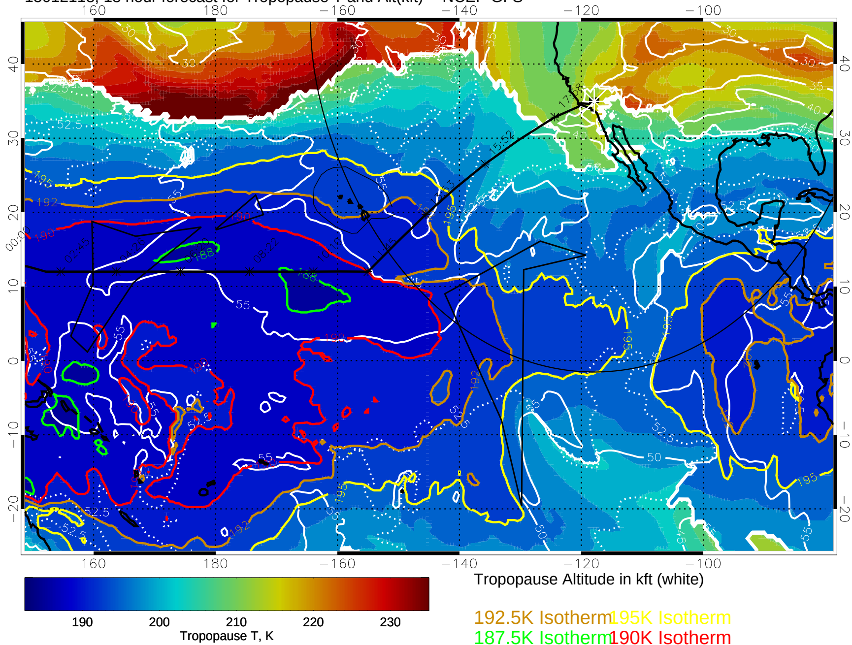
15012118, 18 hour forecast for Tropopause T and Alt(kft) -- NCEP GFS
