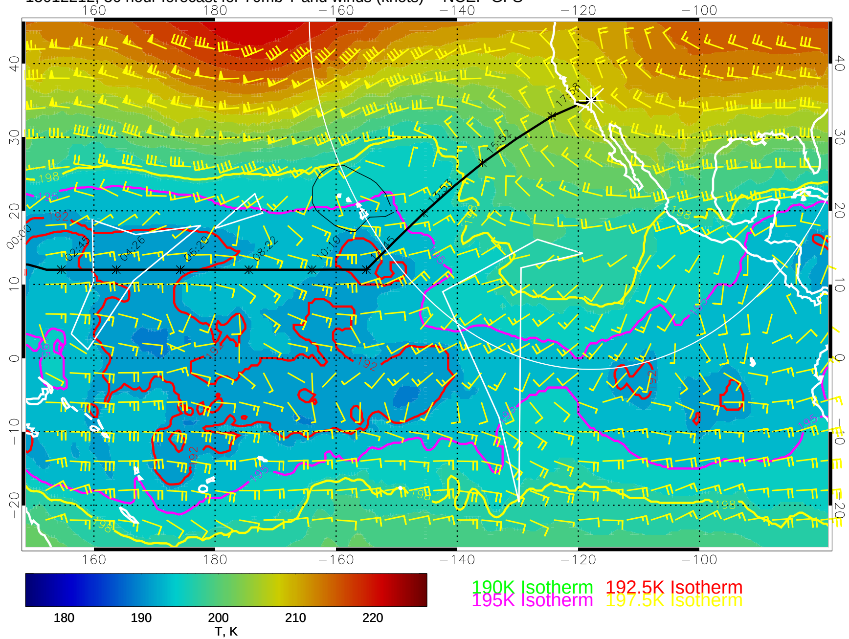
15012212, 36 hour forecast for 70mb T and winds (knots) -- NCEP GFS
