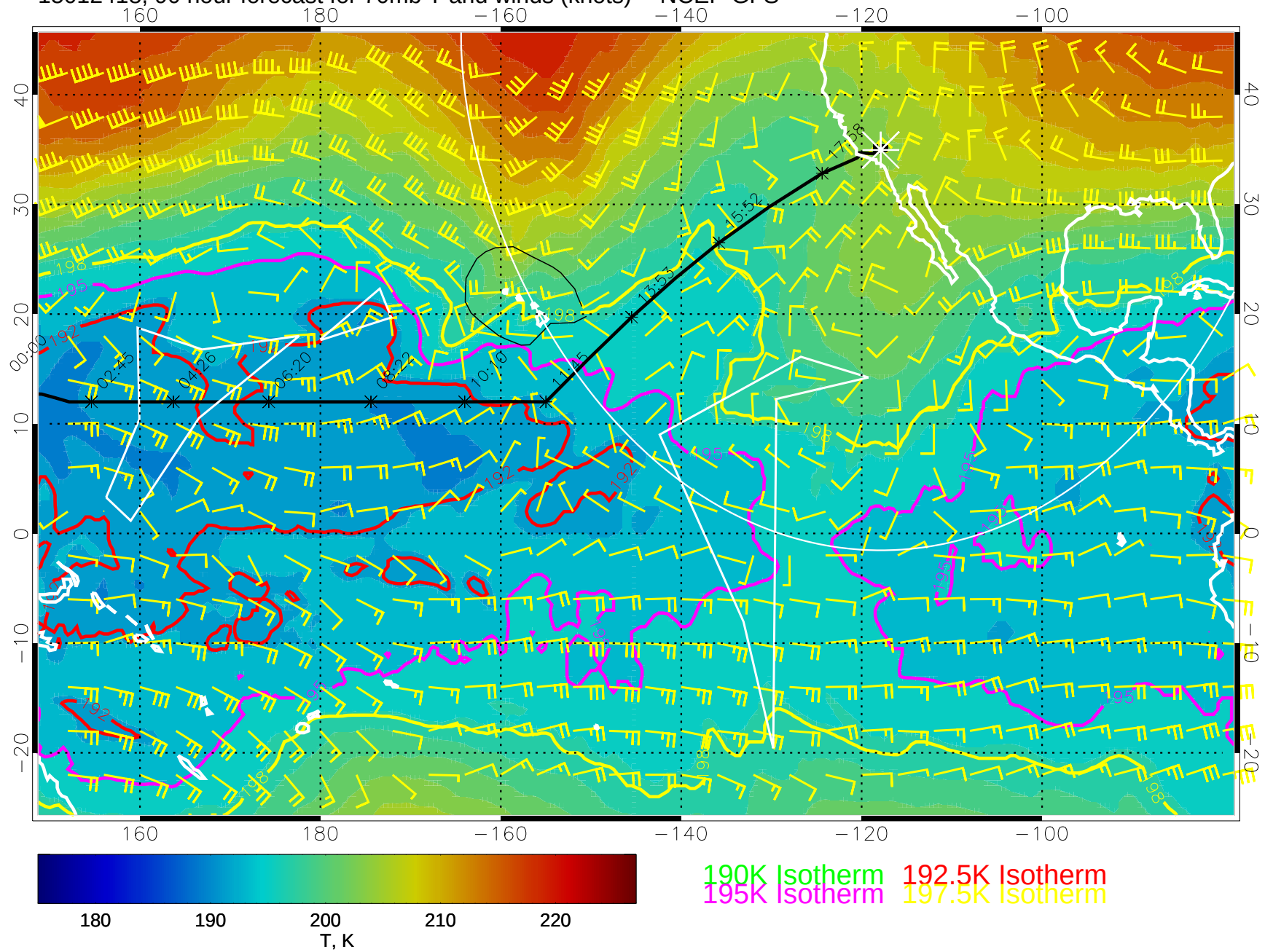
15012418, 90 hour forecast for 70mb T and winds (knots) -- NCEP GFS
