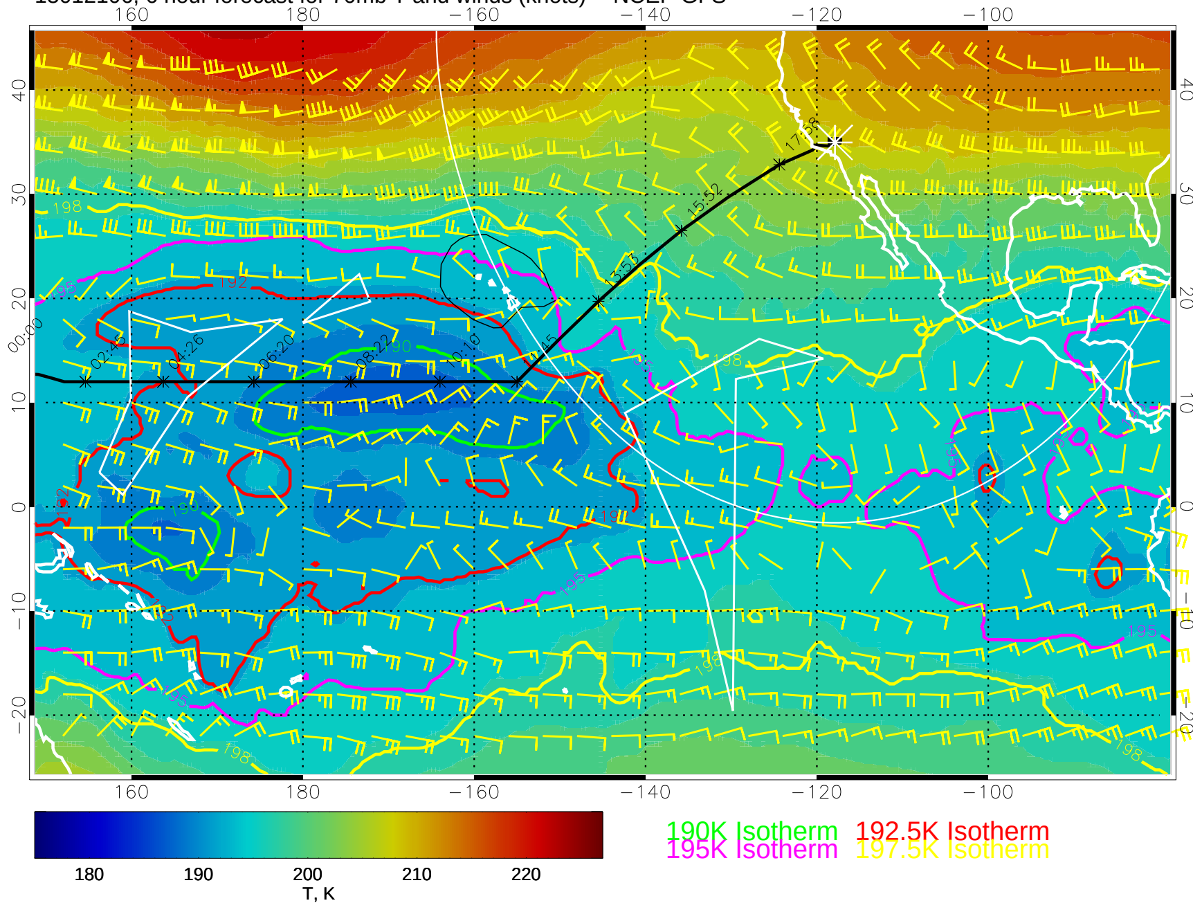
15012106, 6 hour forecast for 70mb T and winds (knots) -- NCEP GFS
