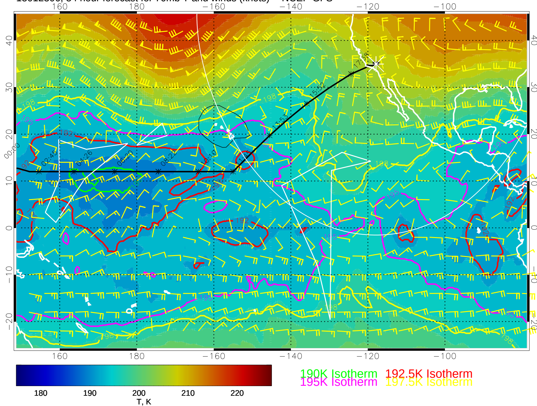
15012306, 54 hour forecast for 70mb T and winds (knots) -- NCEP GFS
