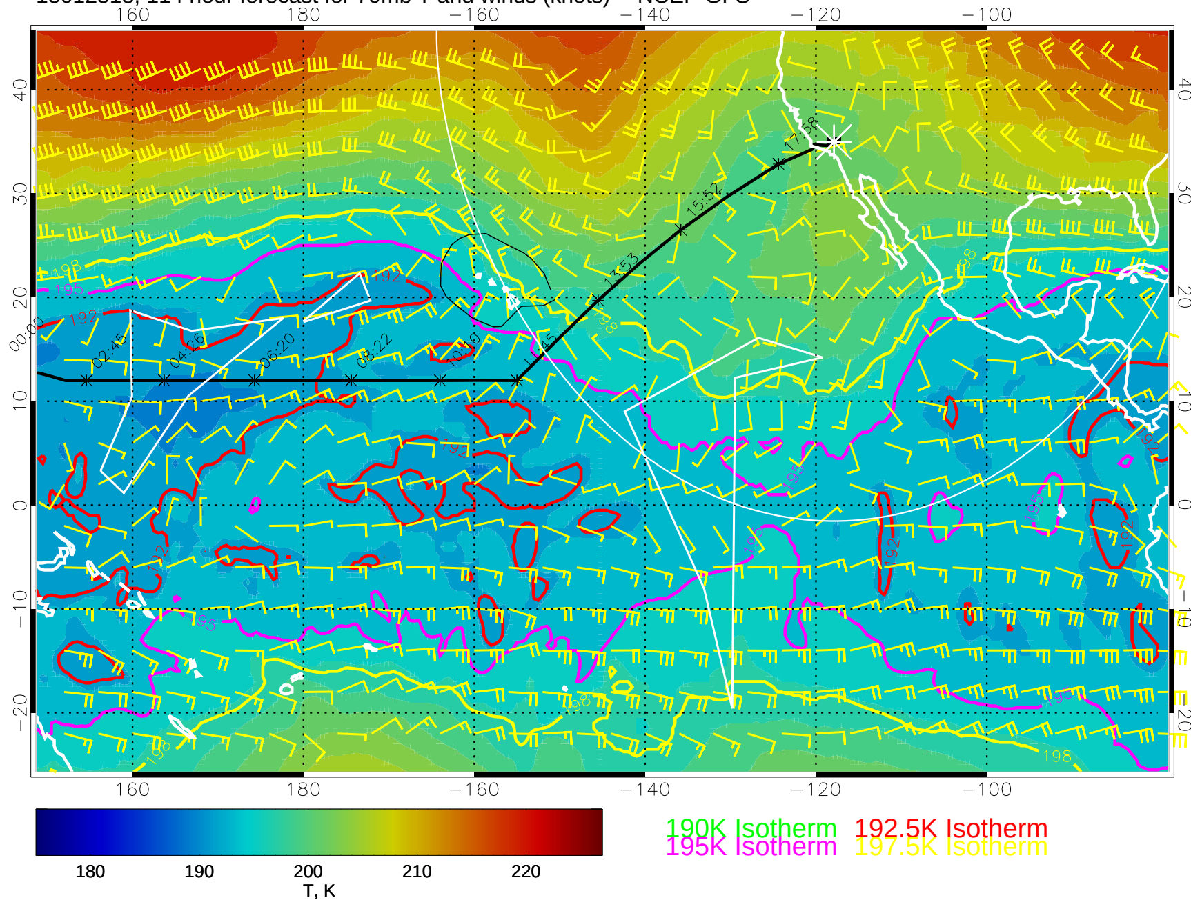
15012518, 114 hour forecast for 70mb T and winds (knots) -- NCEP GFS
