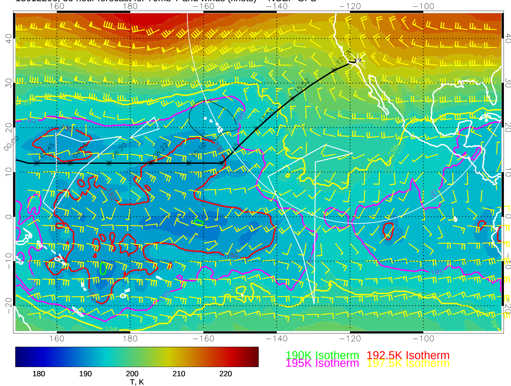
15012206, 30 hour forecast for 70mb T and winds (knots) -- NCEP GFS
