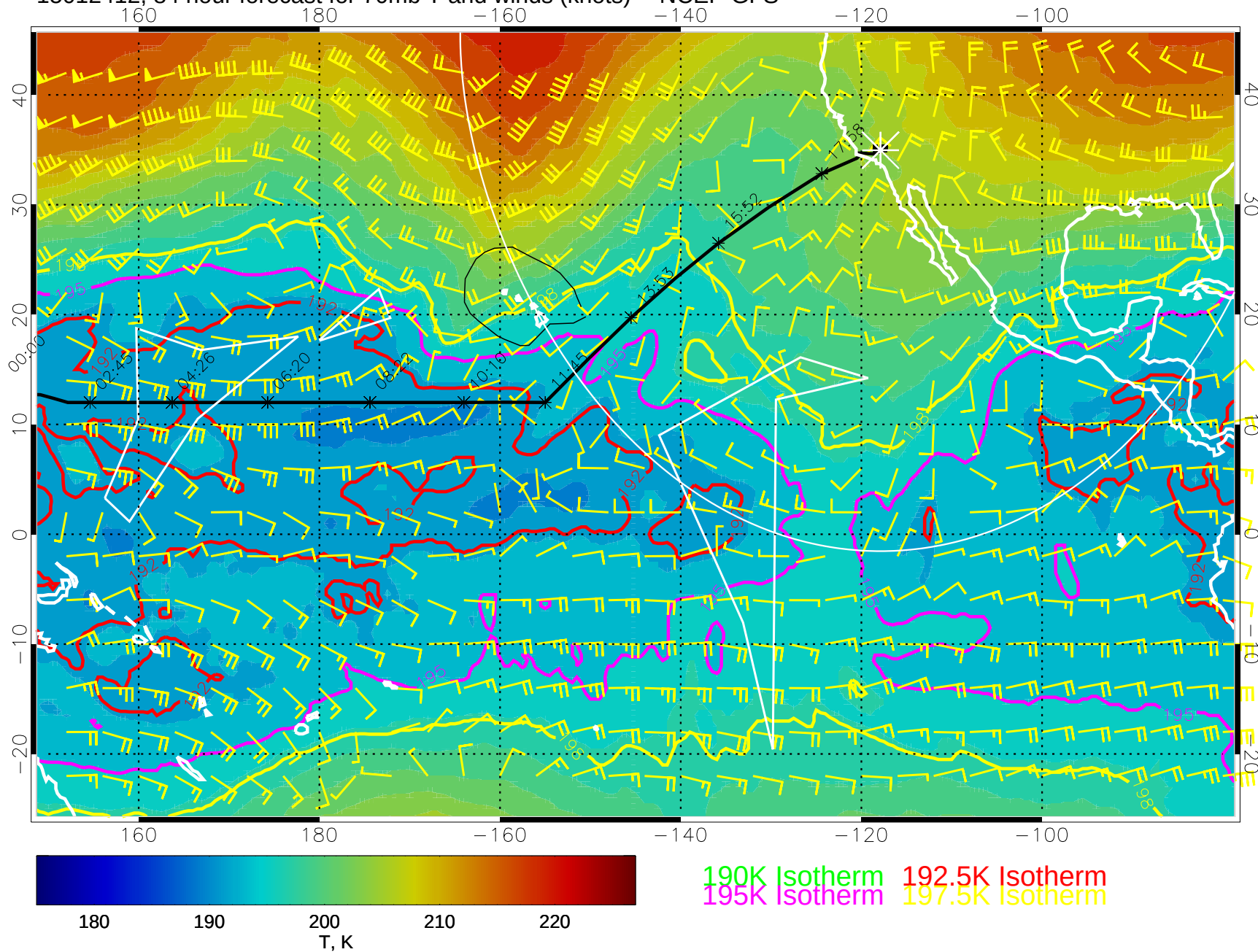
15012412, 84 hour forecast for 70mb T and winds (knots) -- NCEP GFS
