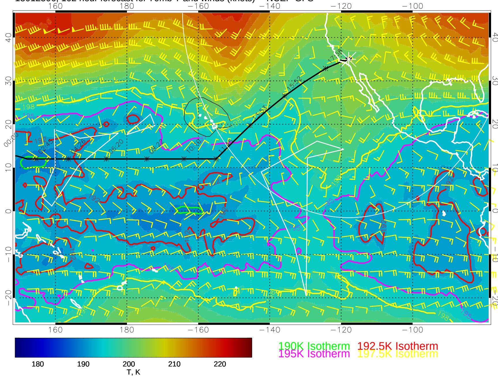
15012506, 102 hour forecast for 70mb T and winds (knots) -- NCEP GFS
