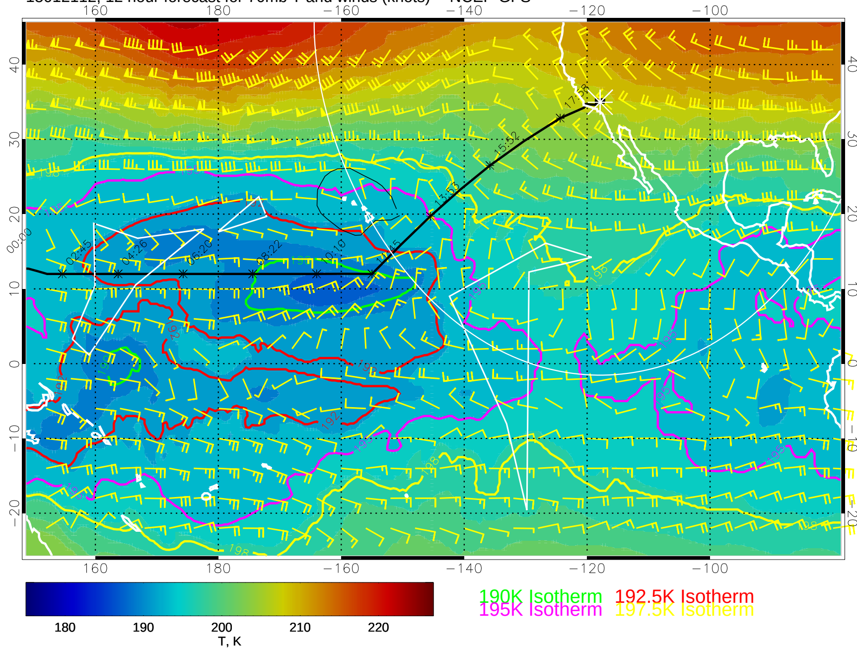
15012112, 12 hour forecast for 70mb T and winds (knots) -- NCEP GFS
