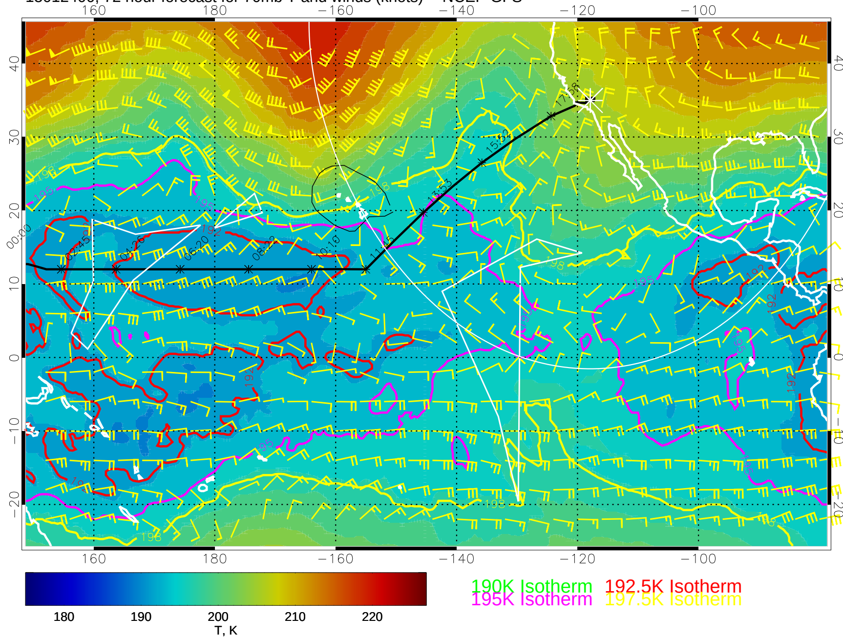
15012400, 72 hour forecast for 70mb T and winds (knots) -- NCEP GFS
