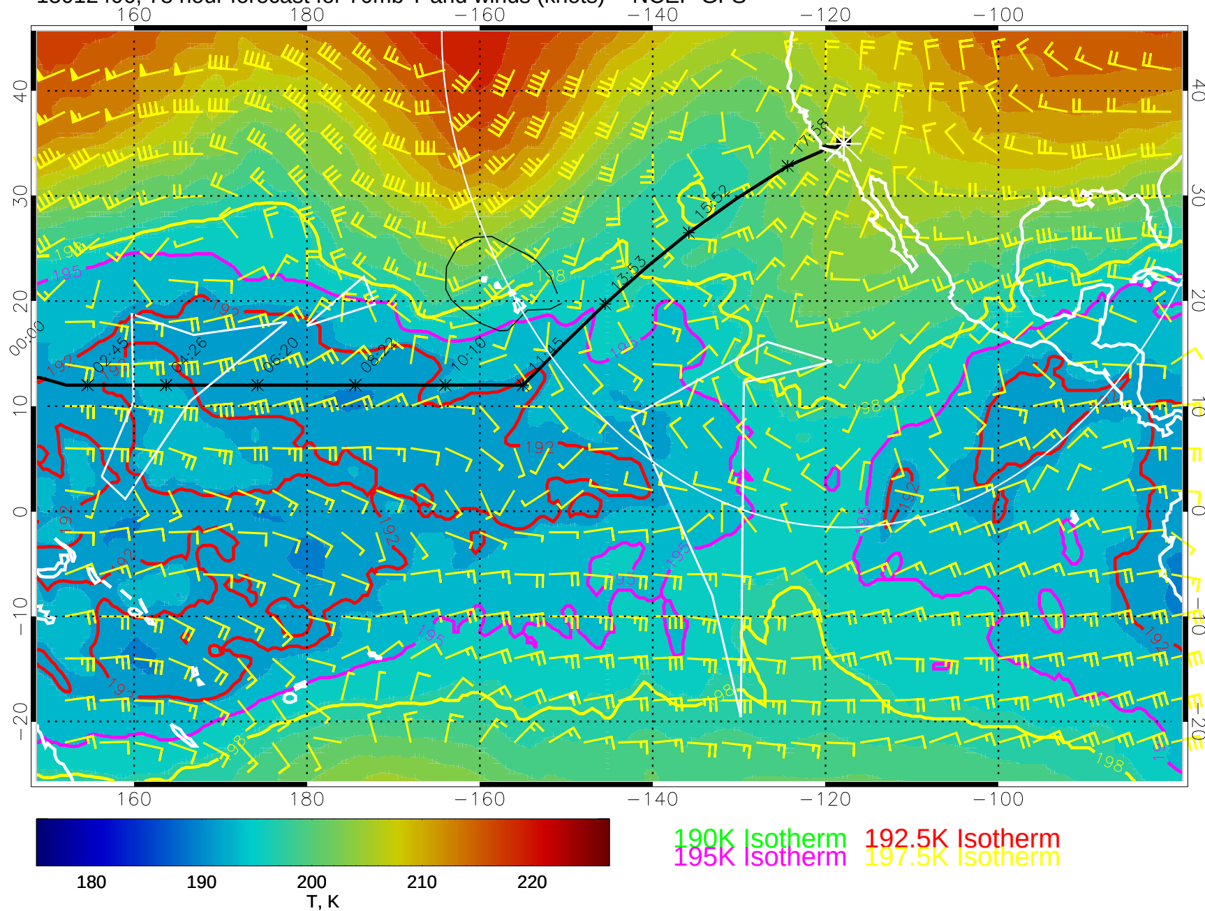
15012406, 78 hour forecast for 70mb T and winds (knots) -- NCEP GFS
