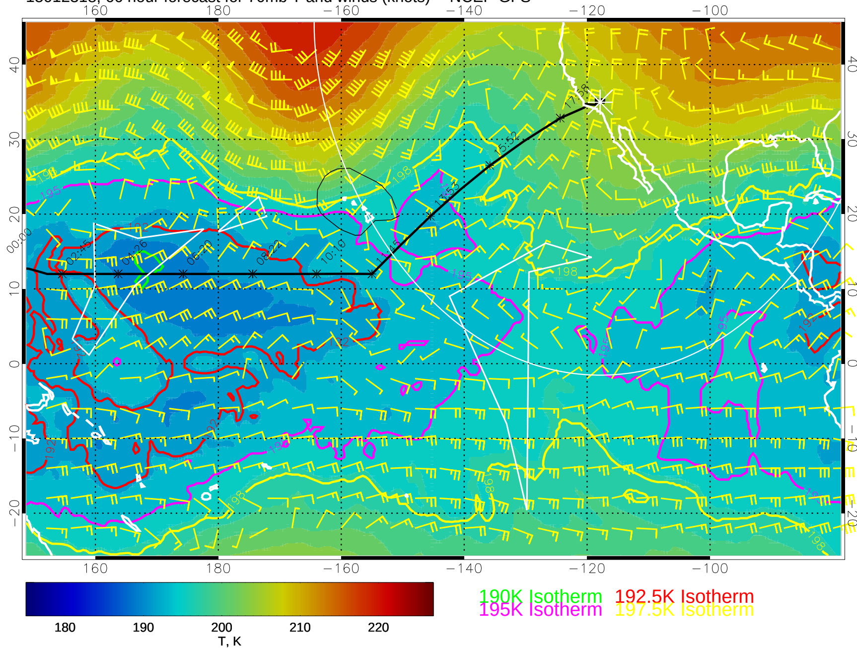
15012318, 66 hour forecast for 70mb T and winds (knots) -- NCEP GFS
