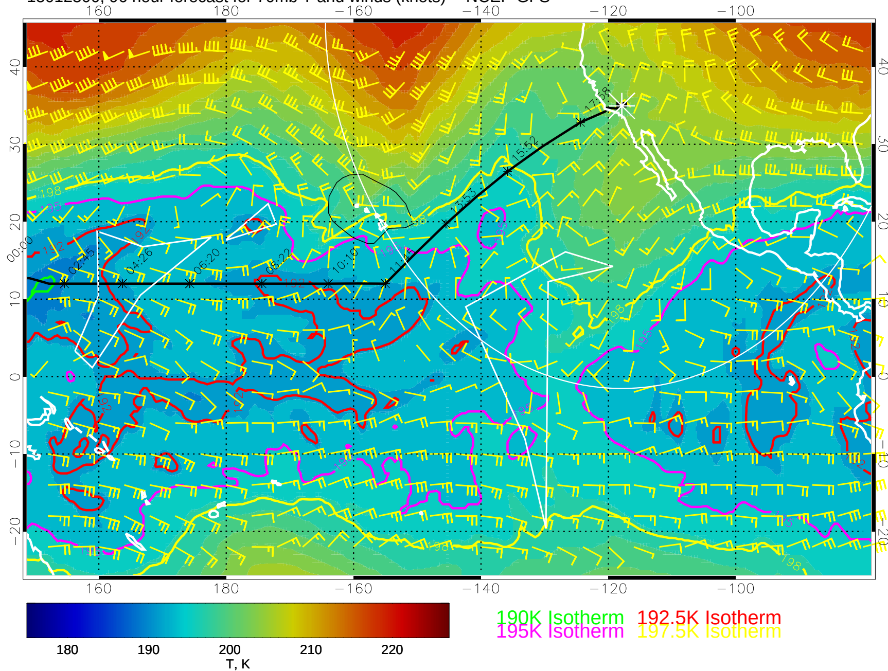
15012500, 96 hour forecast for 70mb T and winds (knots) -- NCEP GFS
