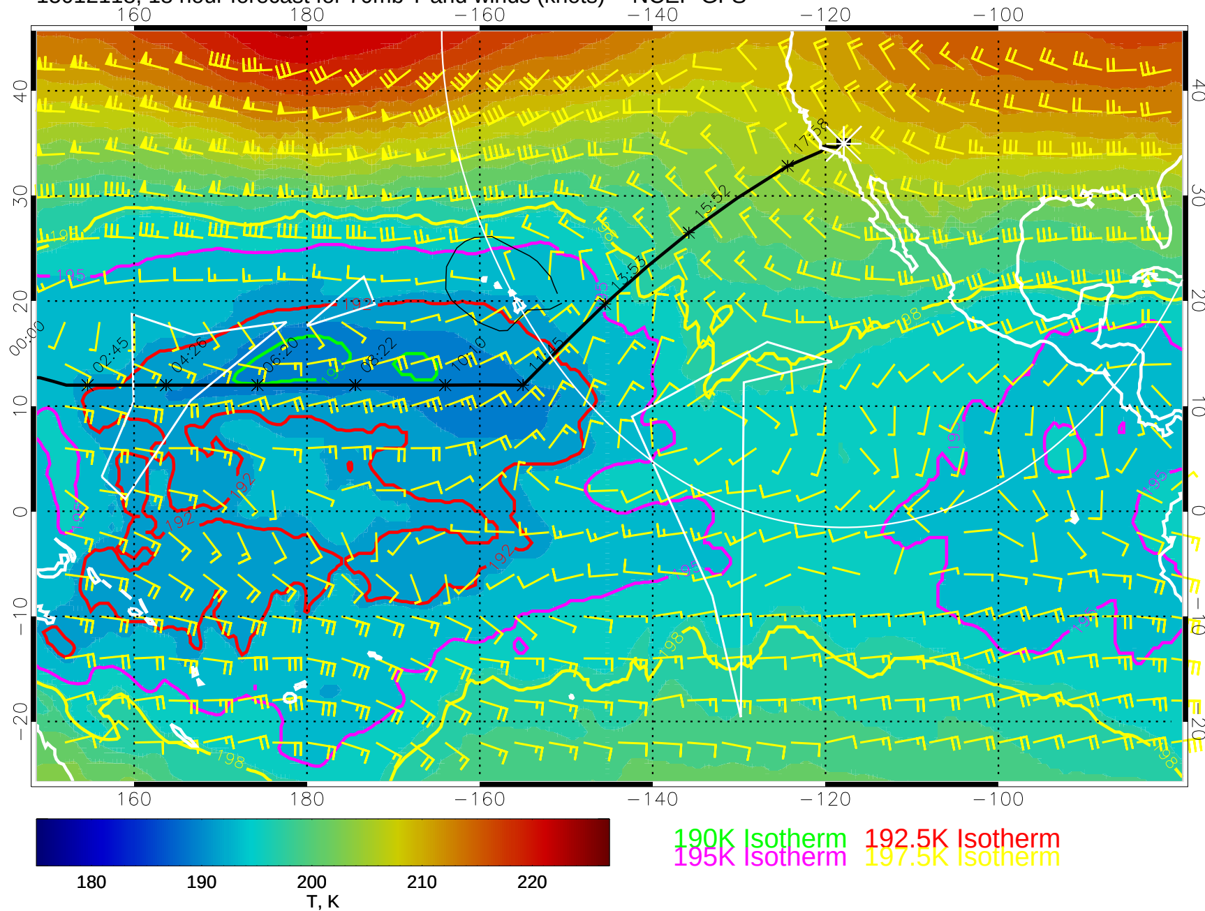
15012118, 18 hour forecast for 70mb T and winds (knots) -- NCEP GFS
