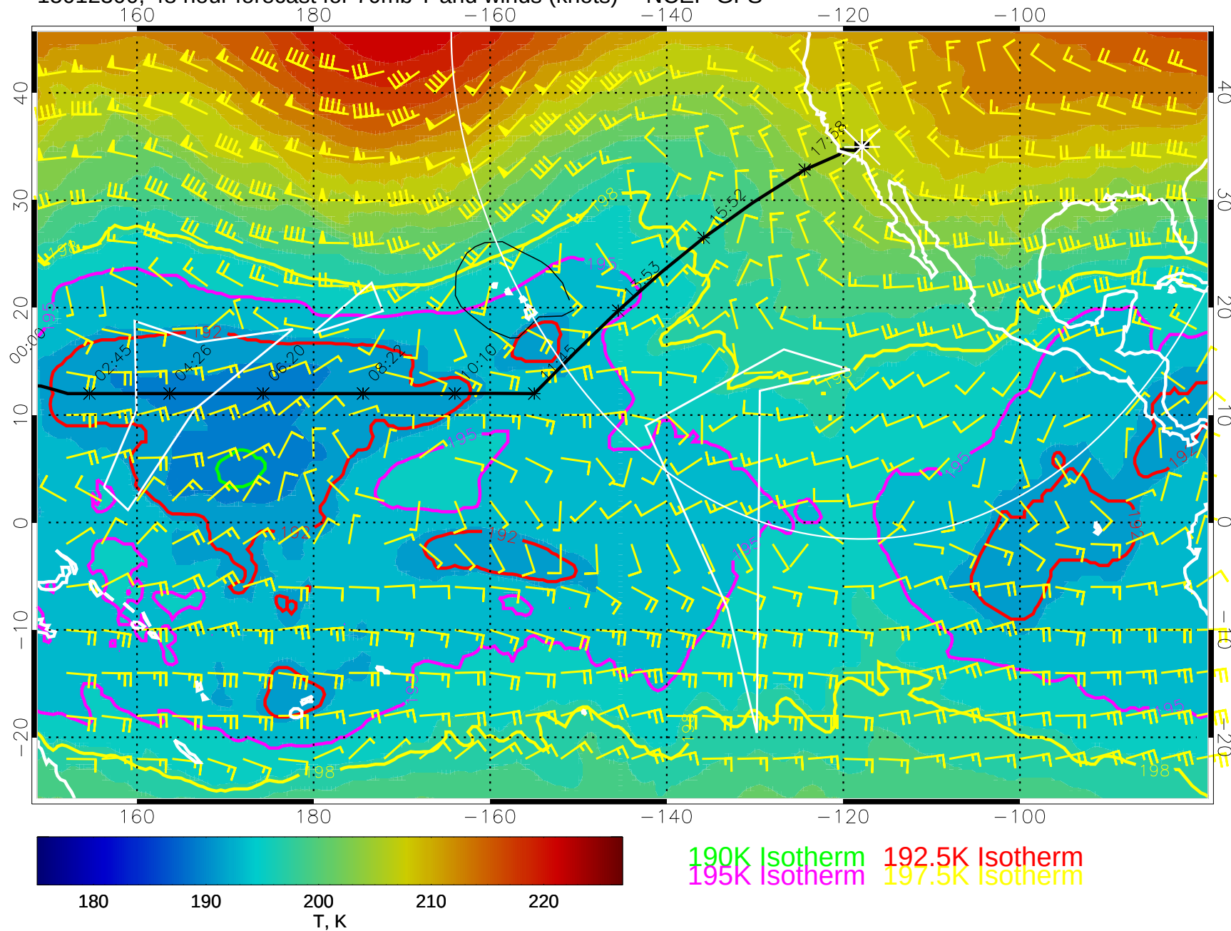
15012300, 48 hour forecast for 70mb T and winds (knots) -- NCEP GFS
