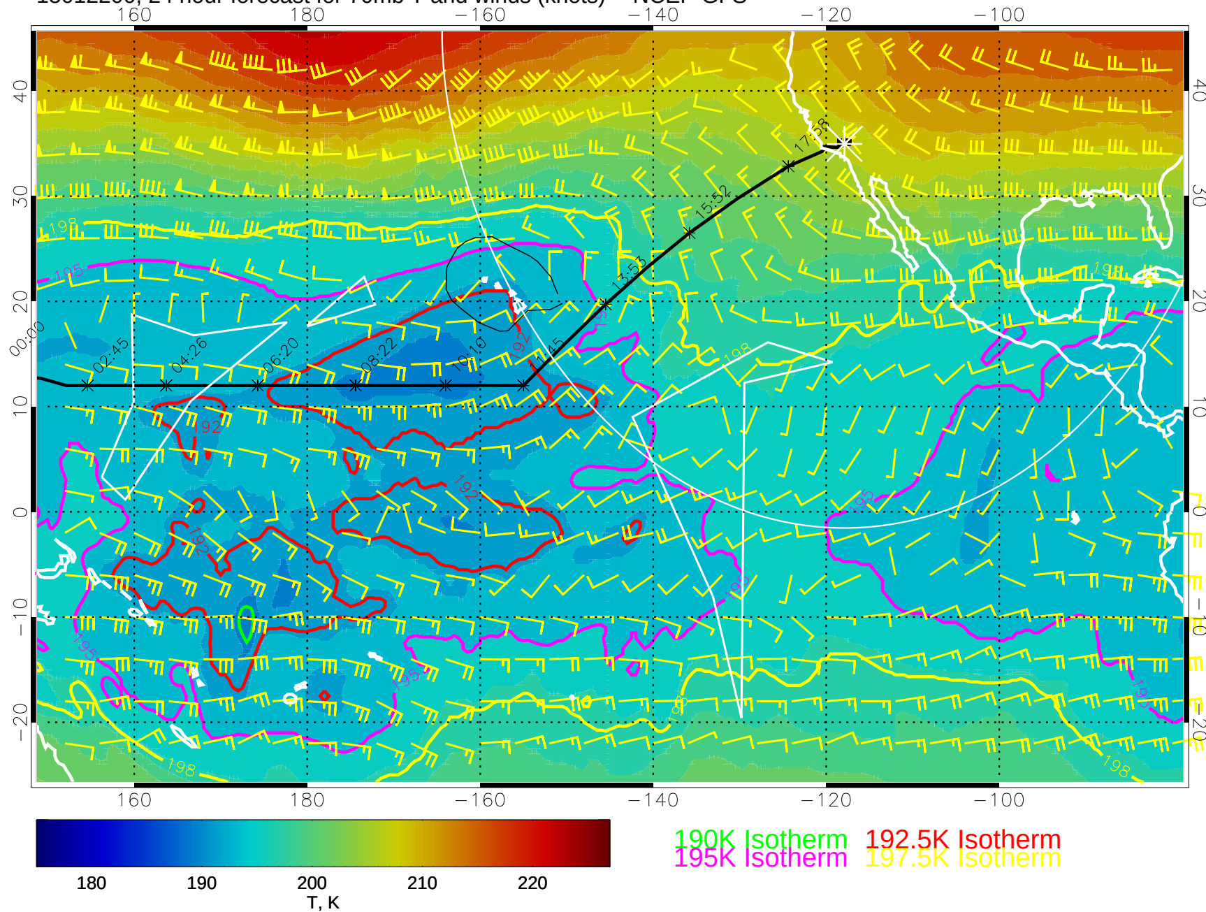
15012200, 24 hour forecast for 70mb T and winds (knots) -- NCEP GFS
