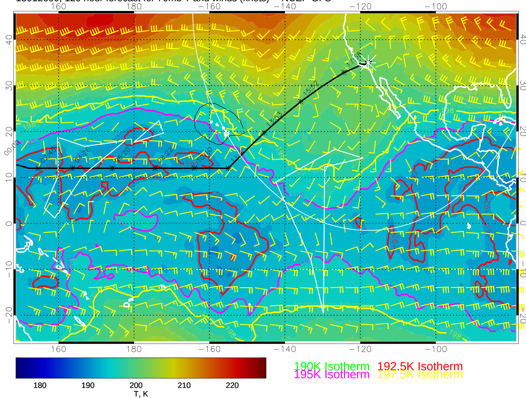
15012600, 120 hour forecast for 70mb T and winds (knots) -- NCEP GFS
