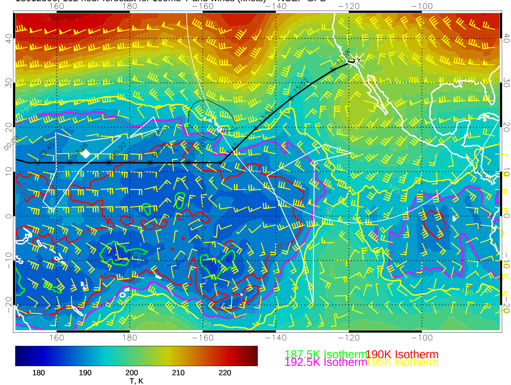
15012506, 102 hour forecast for 100mb T and winds (knots) -- NCEP GFS
