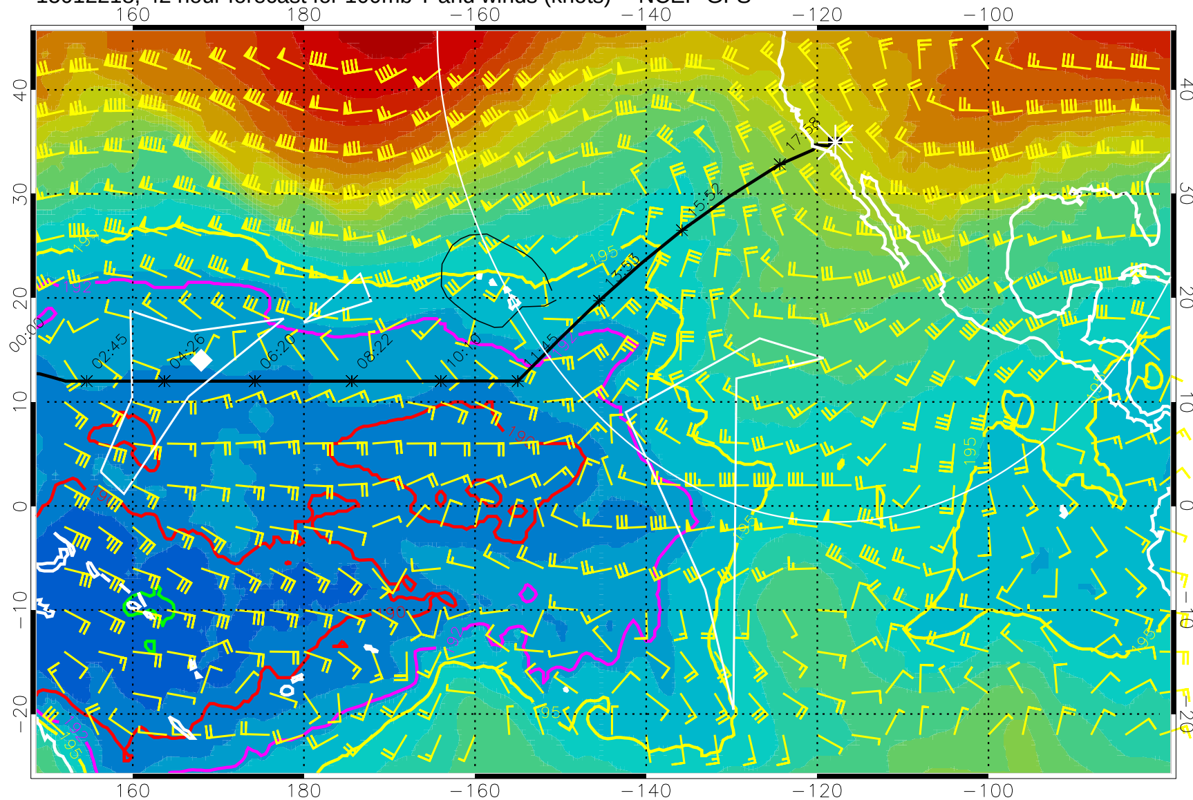
15012218, 42 hour forecast for 100mb T and winds (knots) -- NCEP GFS
