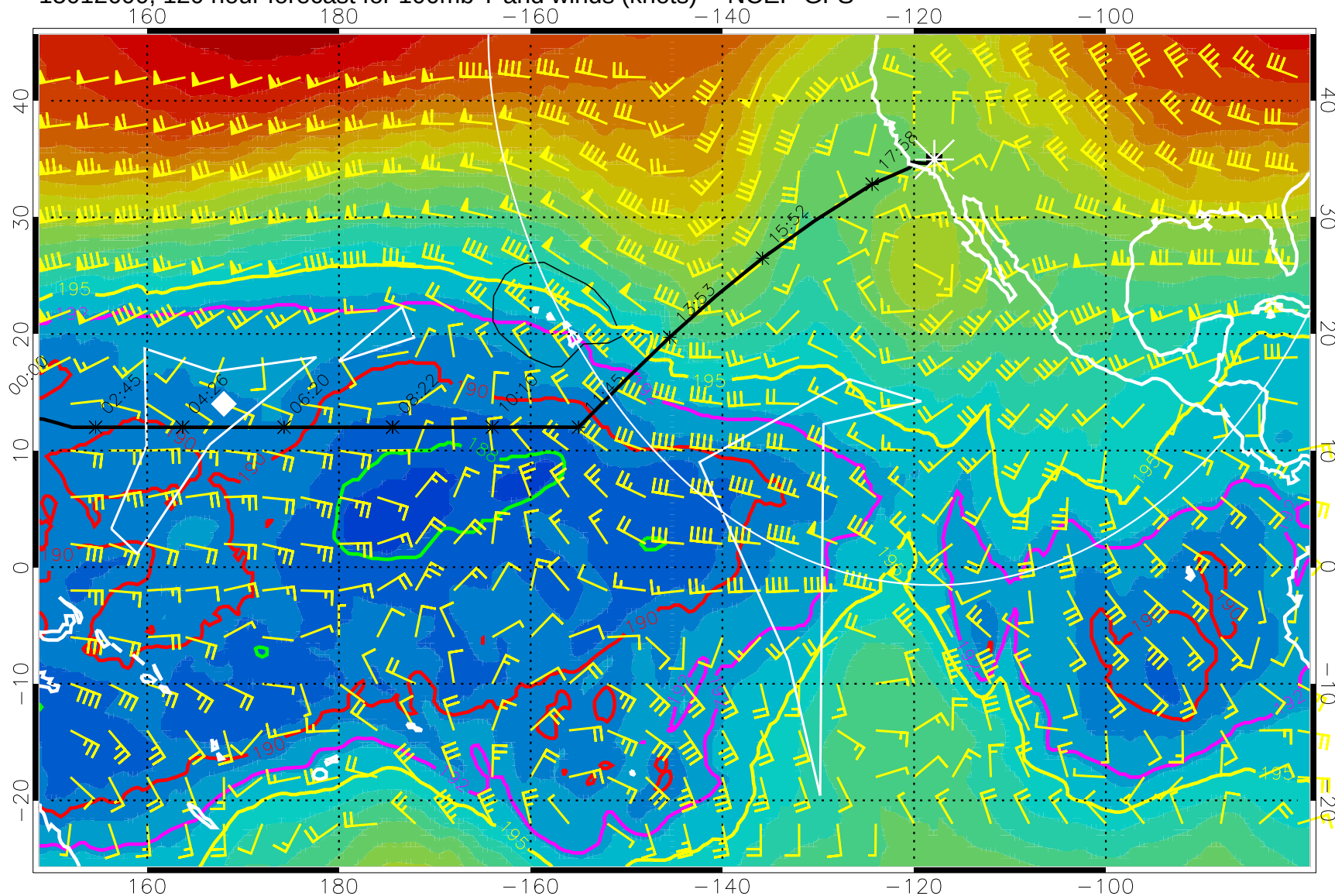
15012600, 120 hour forecast for 100mb T and winds (knots) -- NCEP GFS
