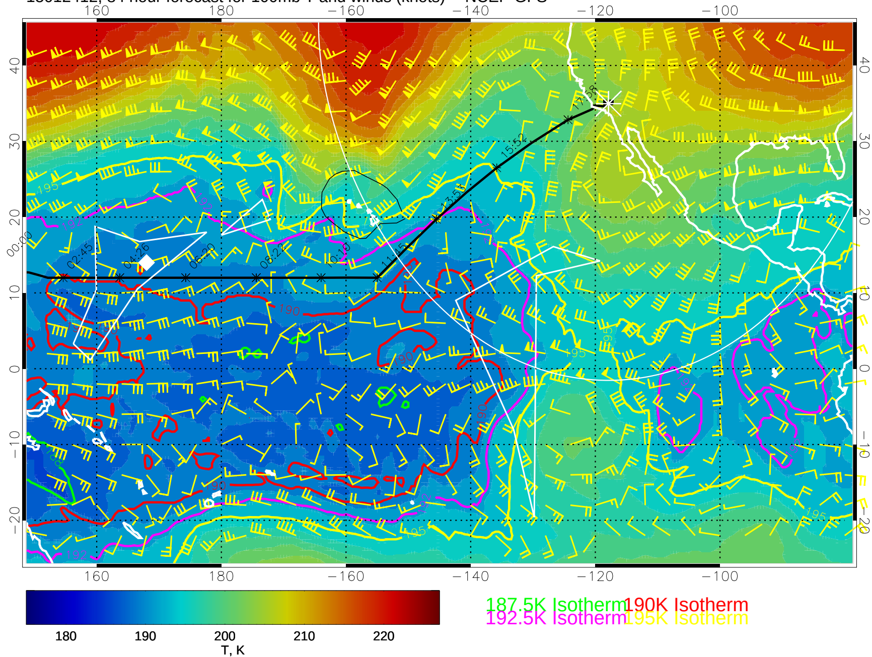
15012412, 84 hour forecast for 100mb T and winds (knots) -- NCEP GFS
