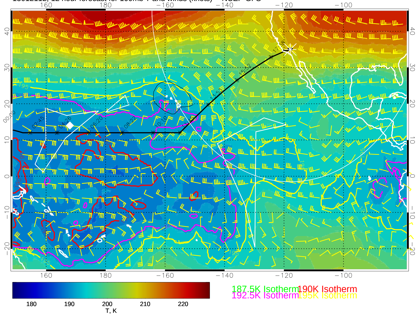
15012112, 12 hour forecast for 100mb T and winds (knots) -- NCEP GFS
