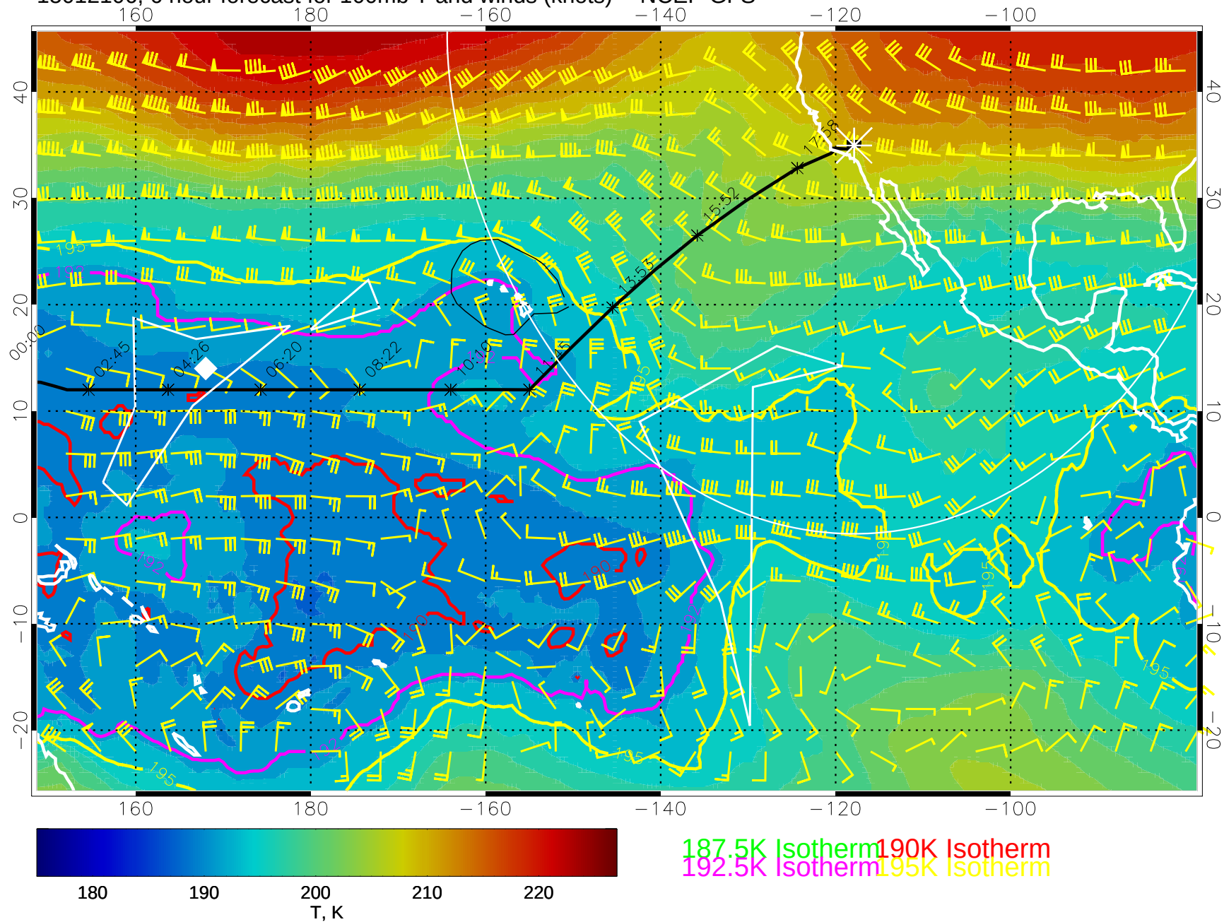
15012106, 6 hour forecast for 100mb T and winds (knots) -- NCEP GFS
