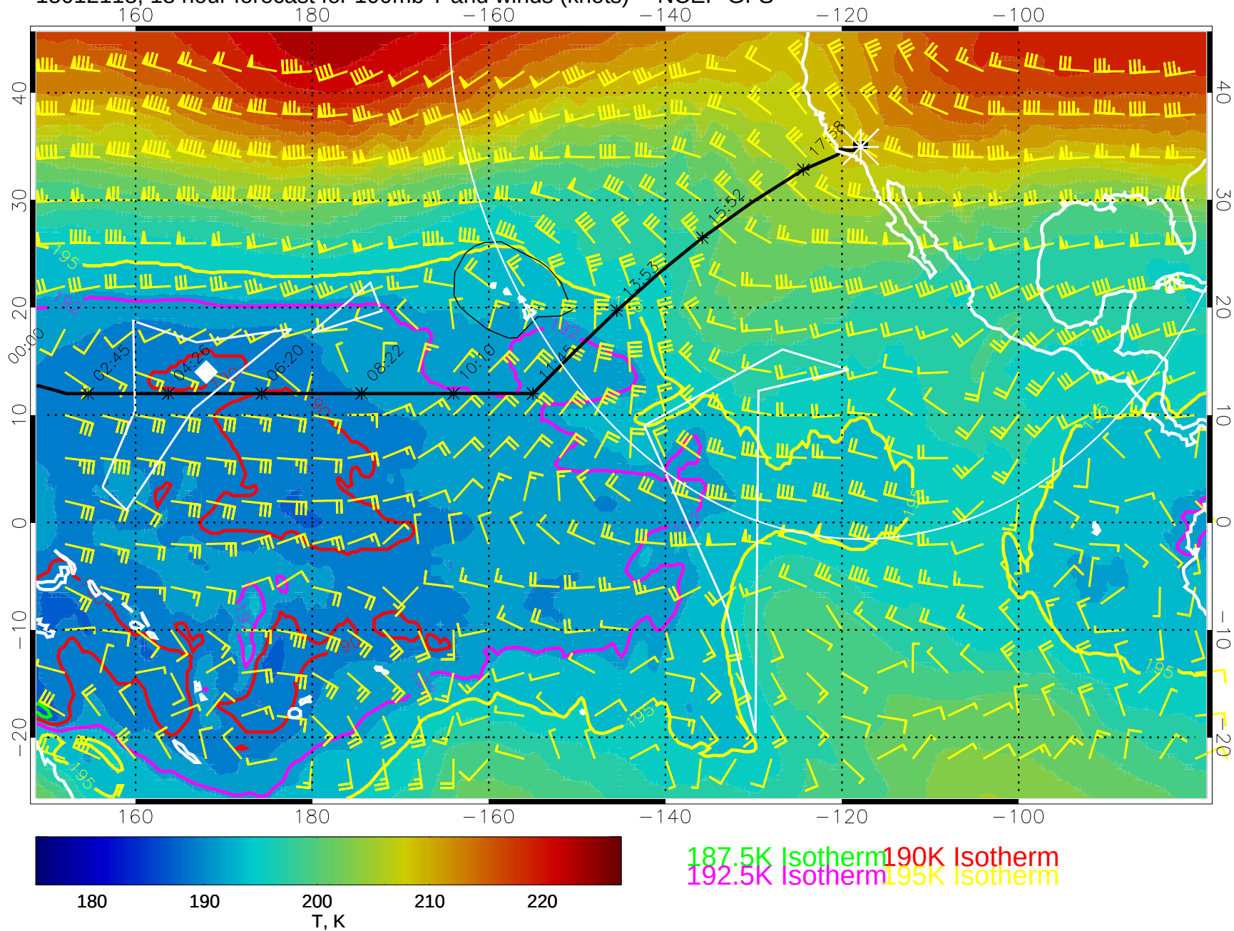
15012118, 18 hour forecast for 100mb T and winds (knots) -- NCEP GFS
