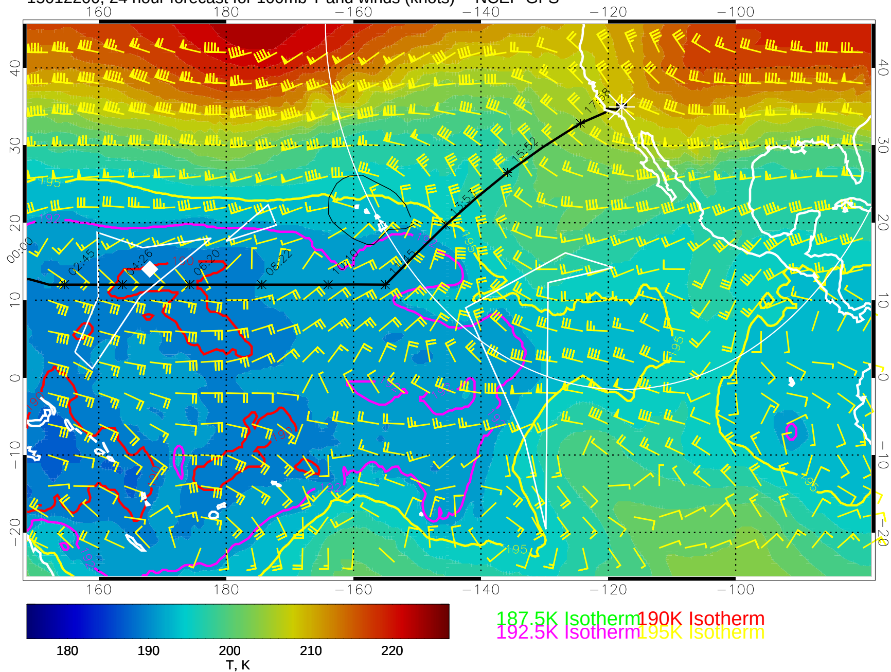
15012200, 24 hour forecast for 100mb T and winds (knots) -- NCEP GFS
