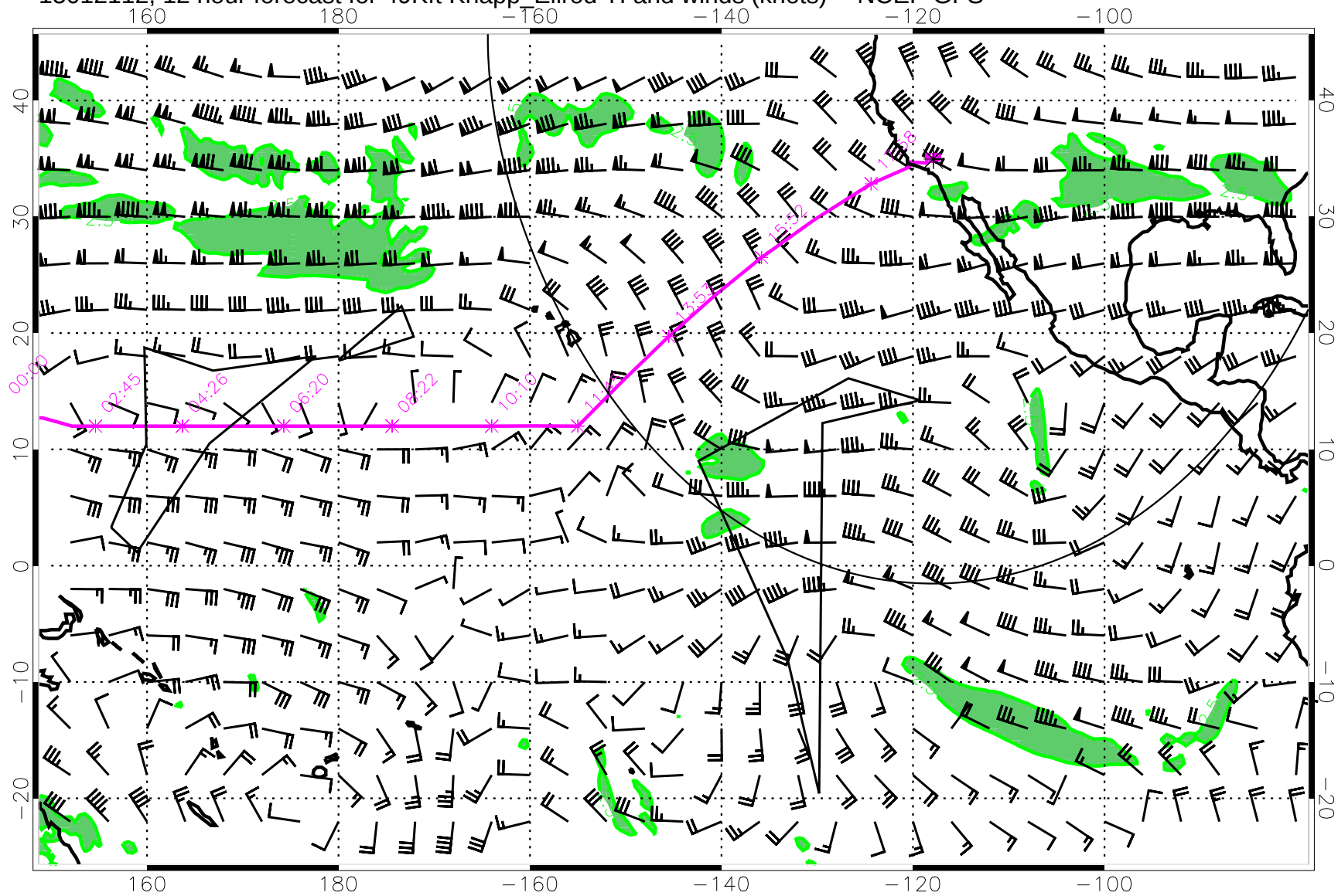
15012112, 12 hour forecast for 49Kft Knapp_Ellrod TI and winds (knots) -- NCEP GFS
