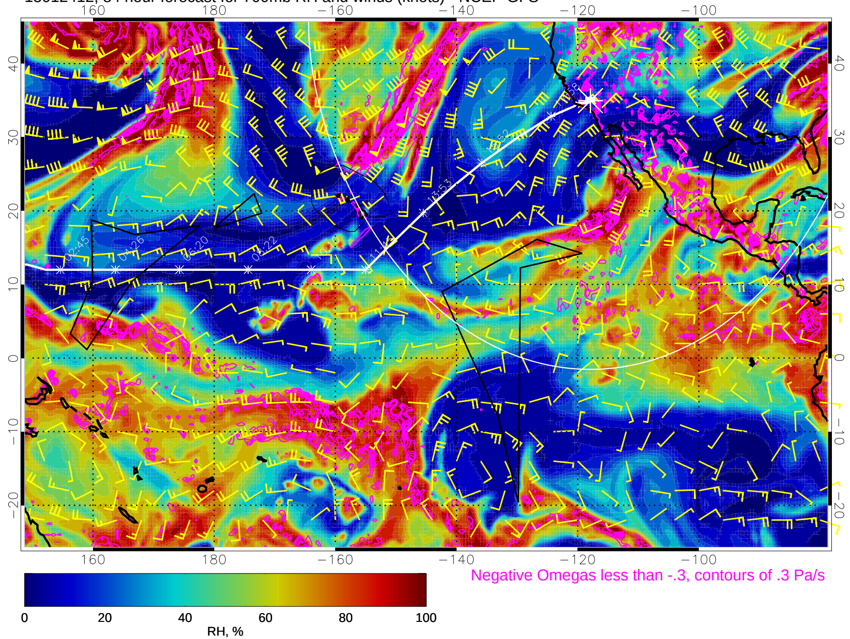
15012412, 84 hour forecast for 700mb RH and winds (knots) - NCEP GFS
