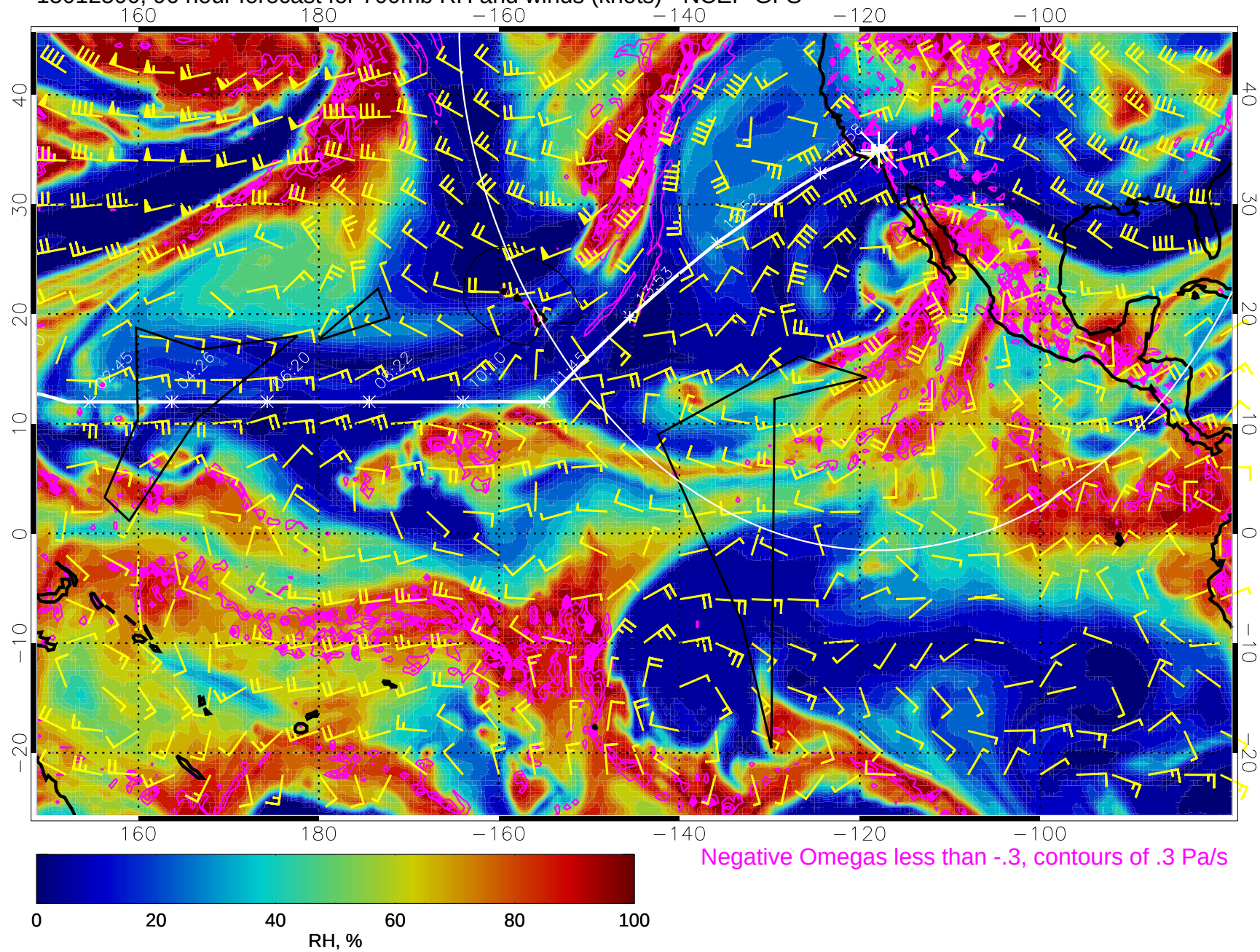
15012500, 96 hour forecast for 700mb RH and winds (knots) - NCEP GFS
