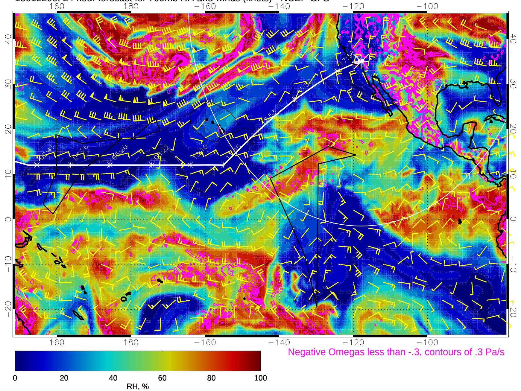
15012200, 24 hour forecast for 700mb RH and winds (knots) - NCEP GFS
