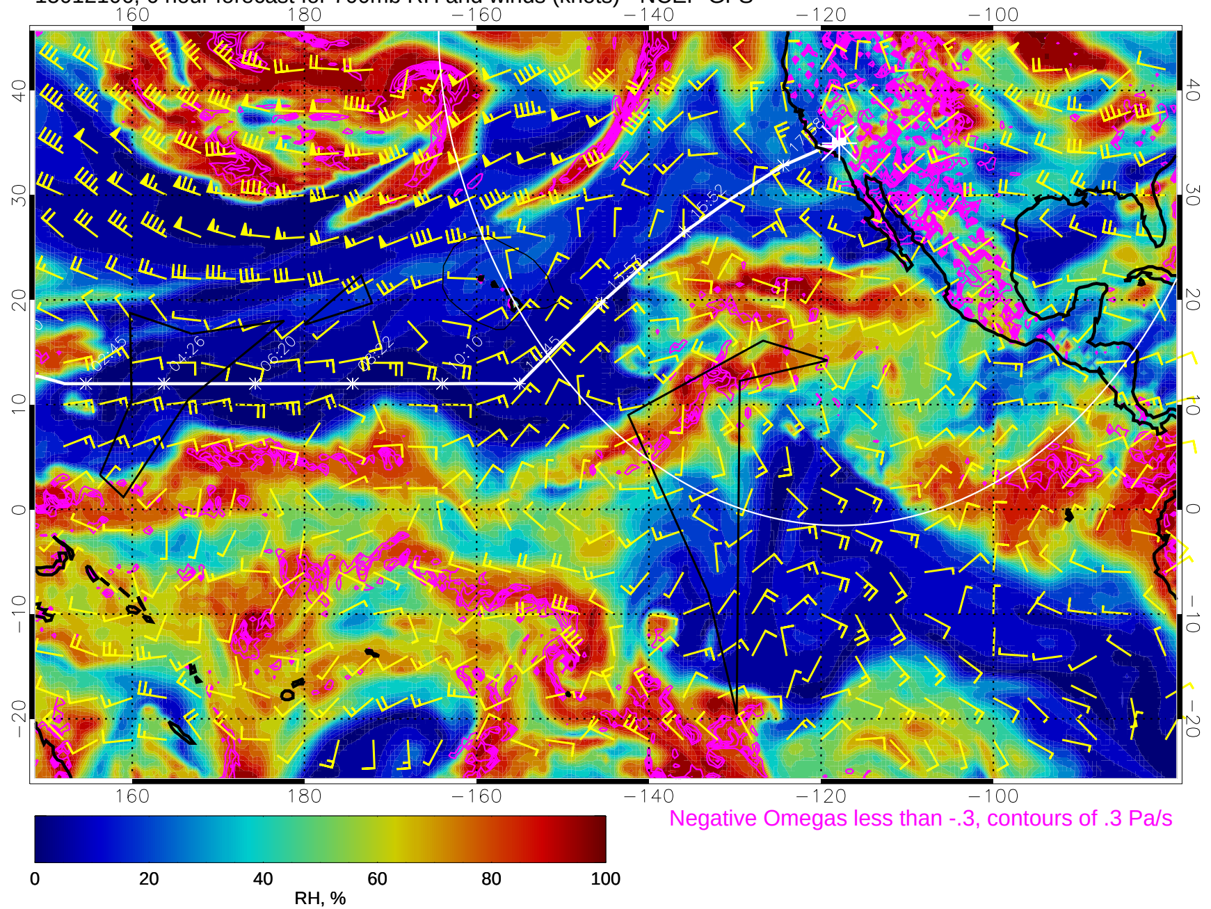
15012106, 6 hour forecast for 700mb RH and winds (knots) - NCEP GFS
