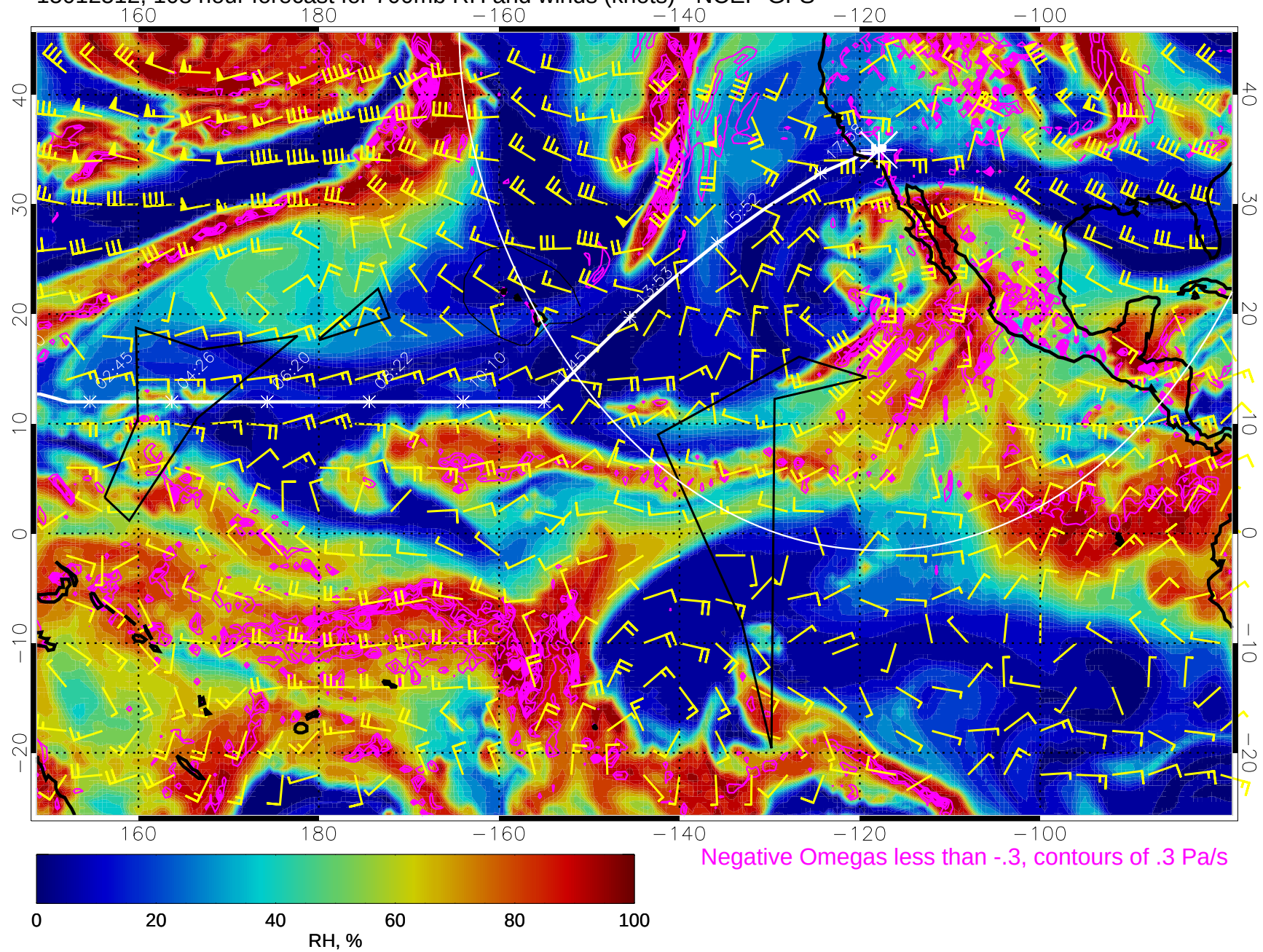
15012512, 108 hour forecast for 700mb RH and winds (knots) - NCEP GFS
