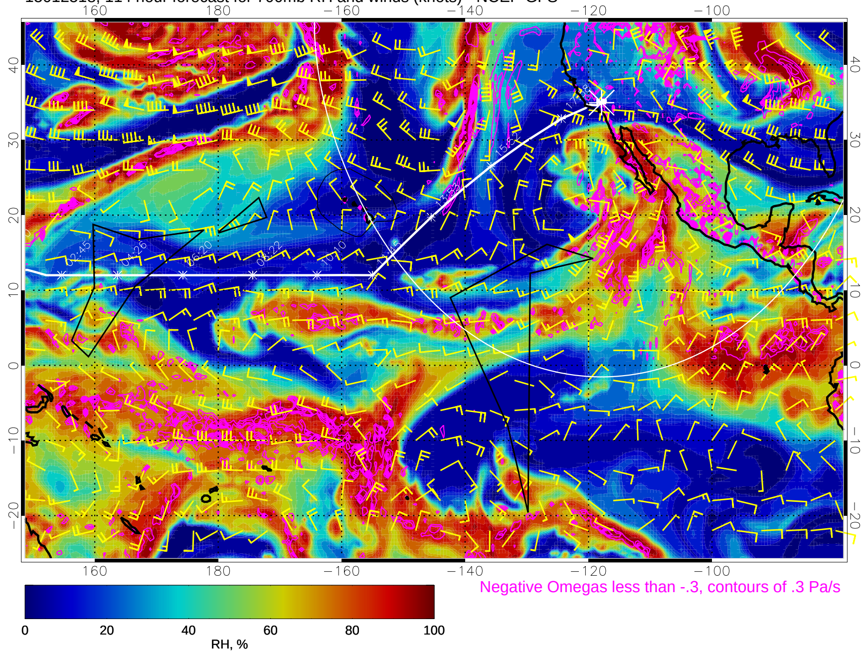
15012518, 114 hour forecast for 700mb RH and winds (knots) - NCEP GFS
