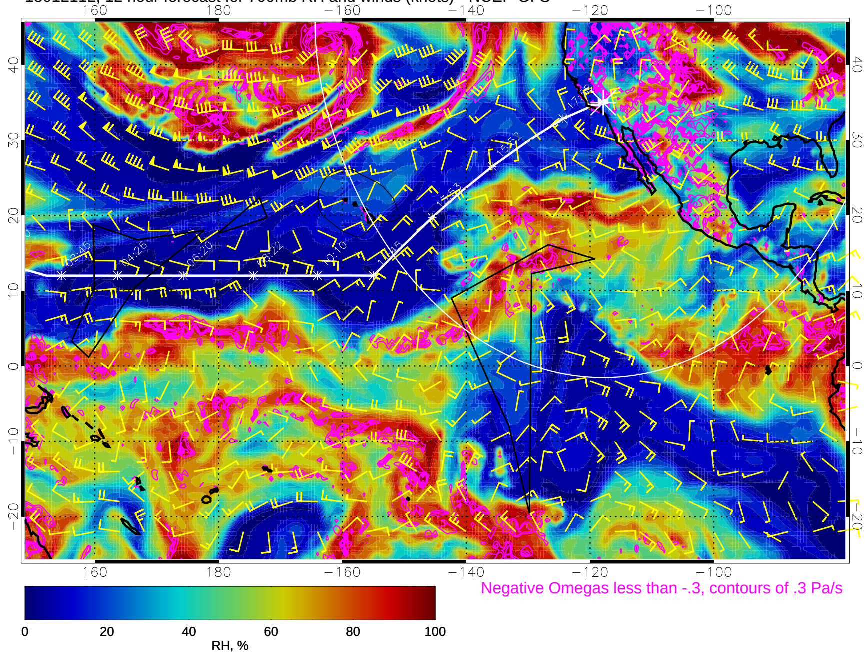
15012112, 12 hour forecast for 700mb RH and winds (knots) - NCEP GFS
