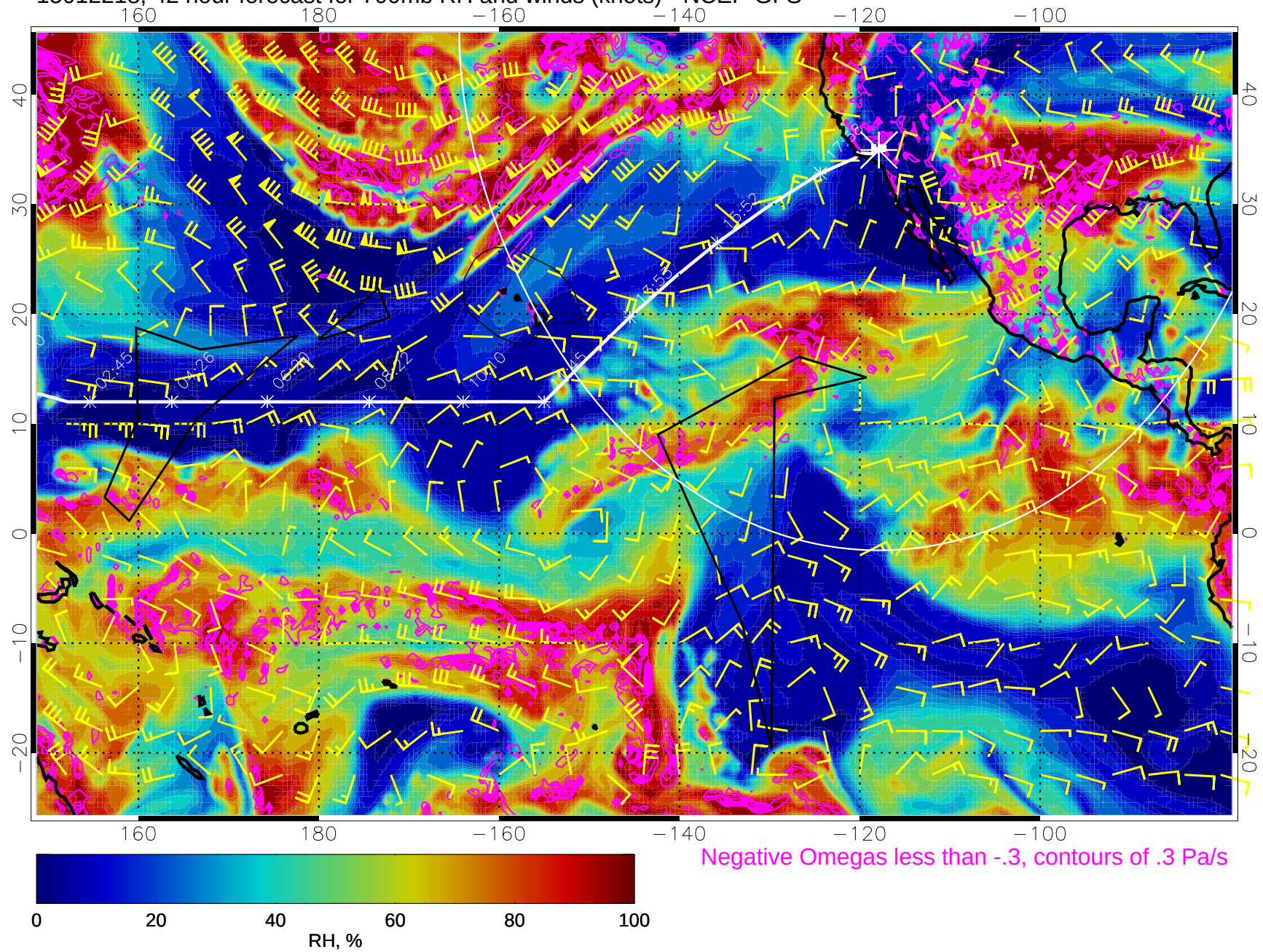
15012218, 42 hour forecast for 700mb RH and winds (knots) - NCEP GFS
