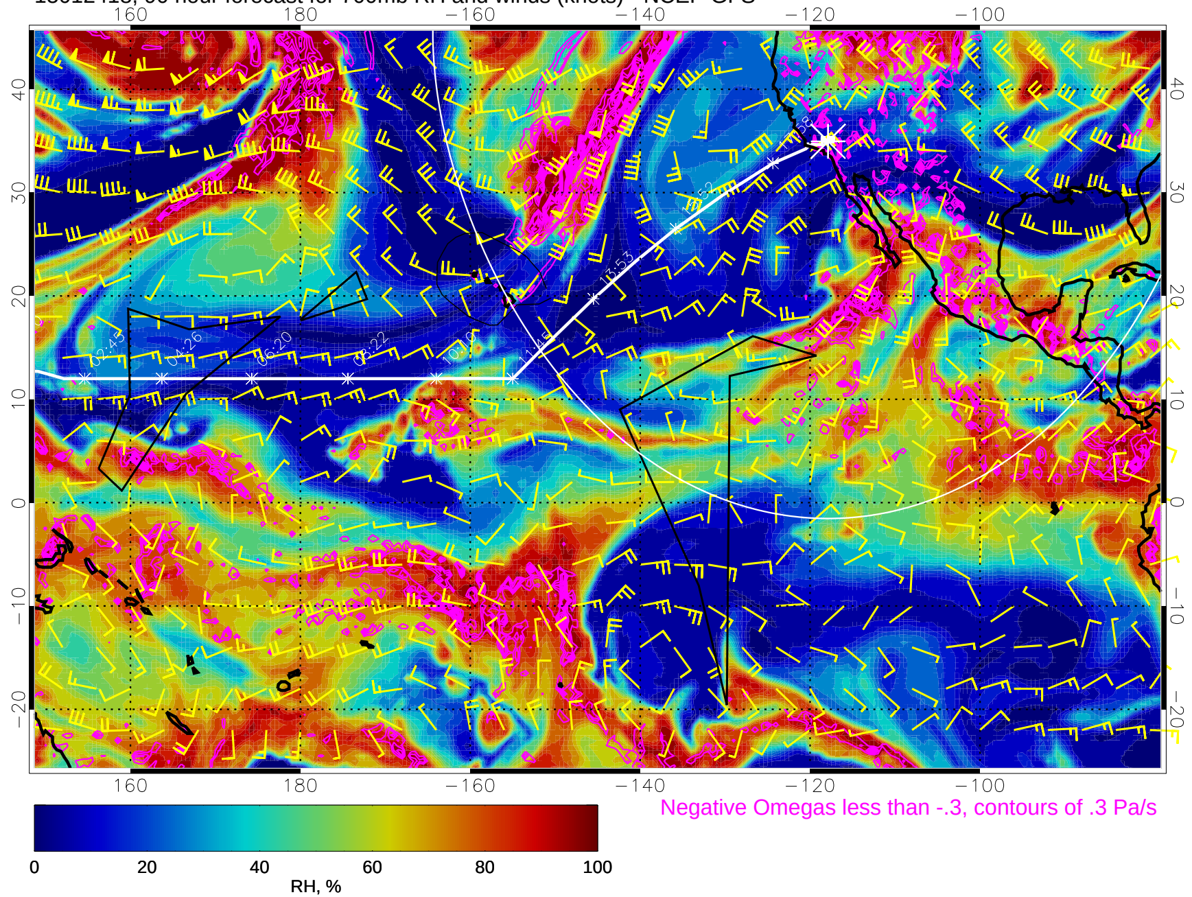
15012418, 90 hour forecast for 700mb RH and winds (knots) - NCEP GFS
