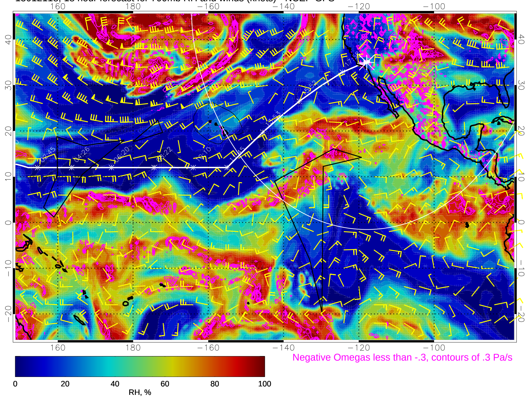
15012118, 18 hour forecast for 700mb RH and winds (knots) - NCEP GFS
