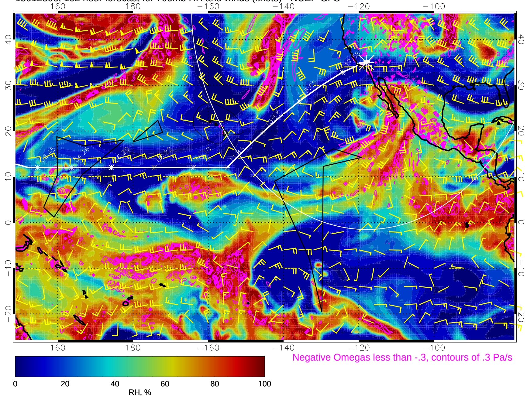
15012506, 102 hour forecast for 700mb RH and winds (knots) - NCEP GFS
