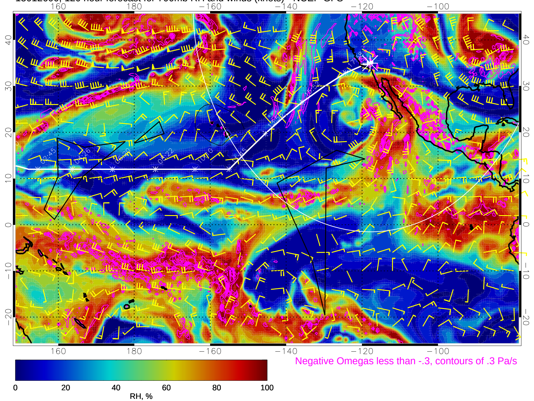
15012600, 120 hour forecast for 700mb RH and winds (knots) - NCEP GFS
