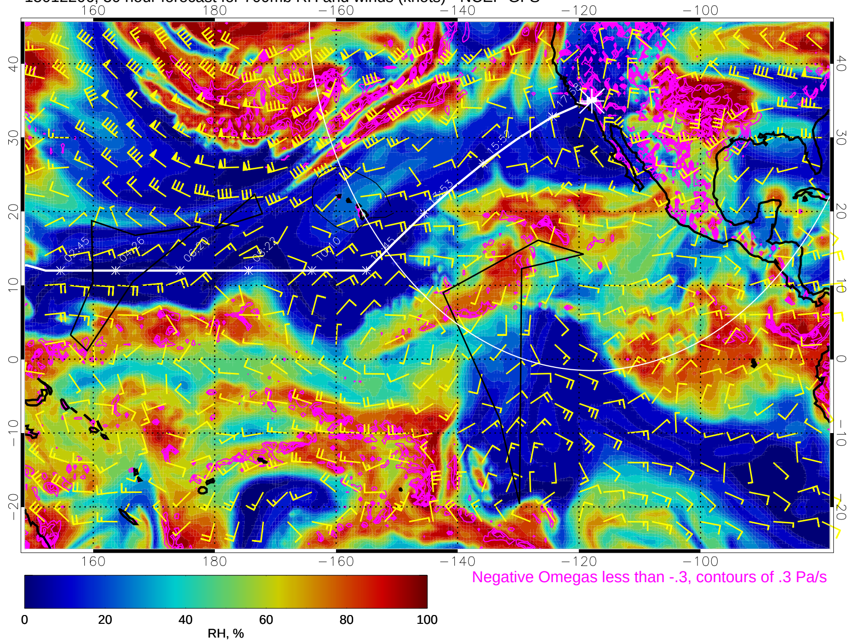
15012206, 30 hour forecast for 700mb RH and winds (knots) - NCEP GFS
