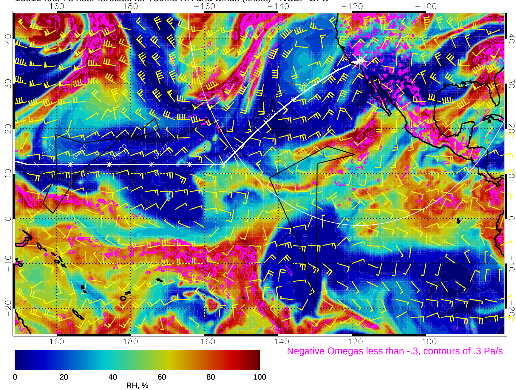
15012406, 78 hour forecast for 700mb RH and winds (knots) - NCEP GFS
