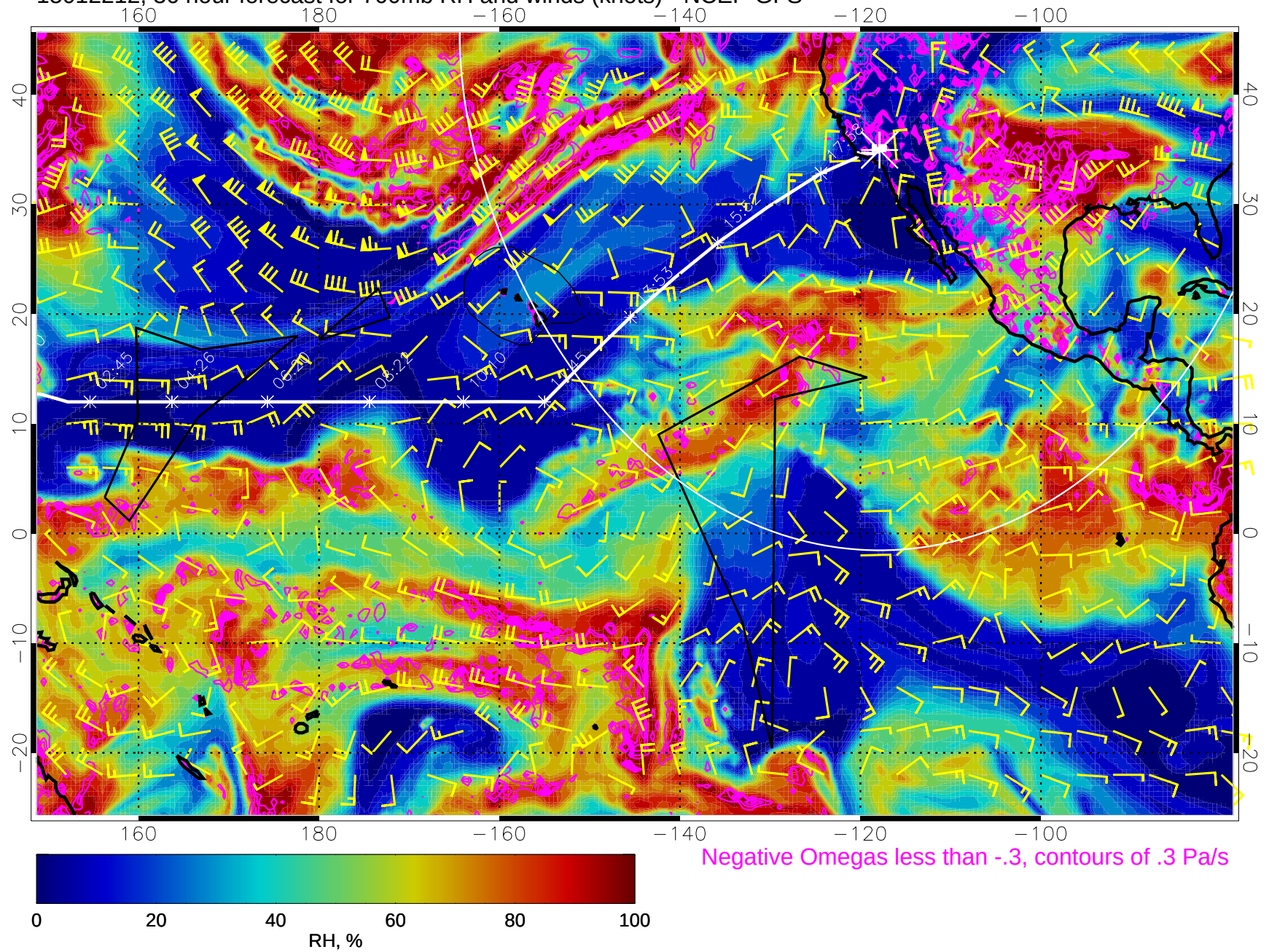
15012212, 36 hour forecast for 700mb RH and winds (knots) - NCEP GFS
