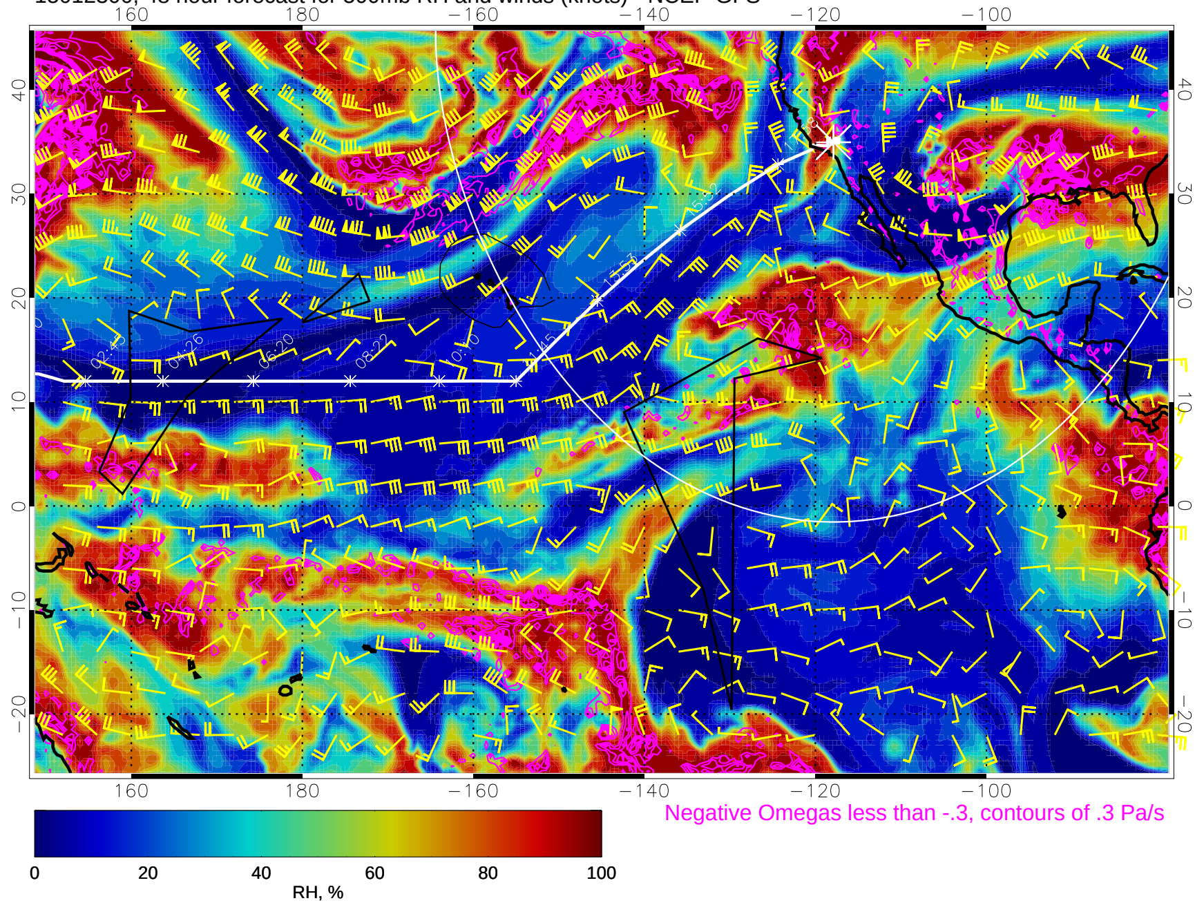
15012300, 48 hour forecast for 500mb RH and winds (knots) - NCEP GFS
