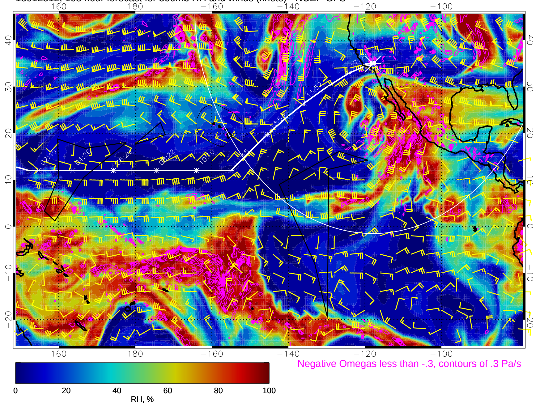
15012512, 108 hour forecast for 500mb RH and winds (knots) - NCEP GFS
