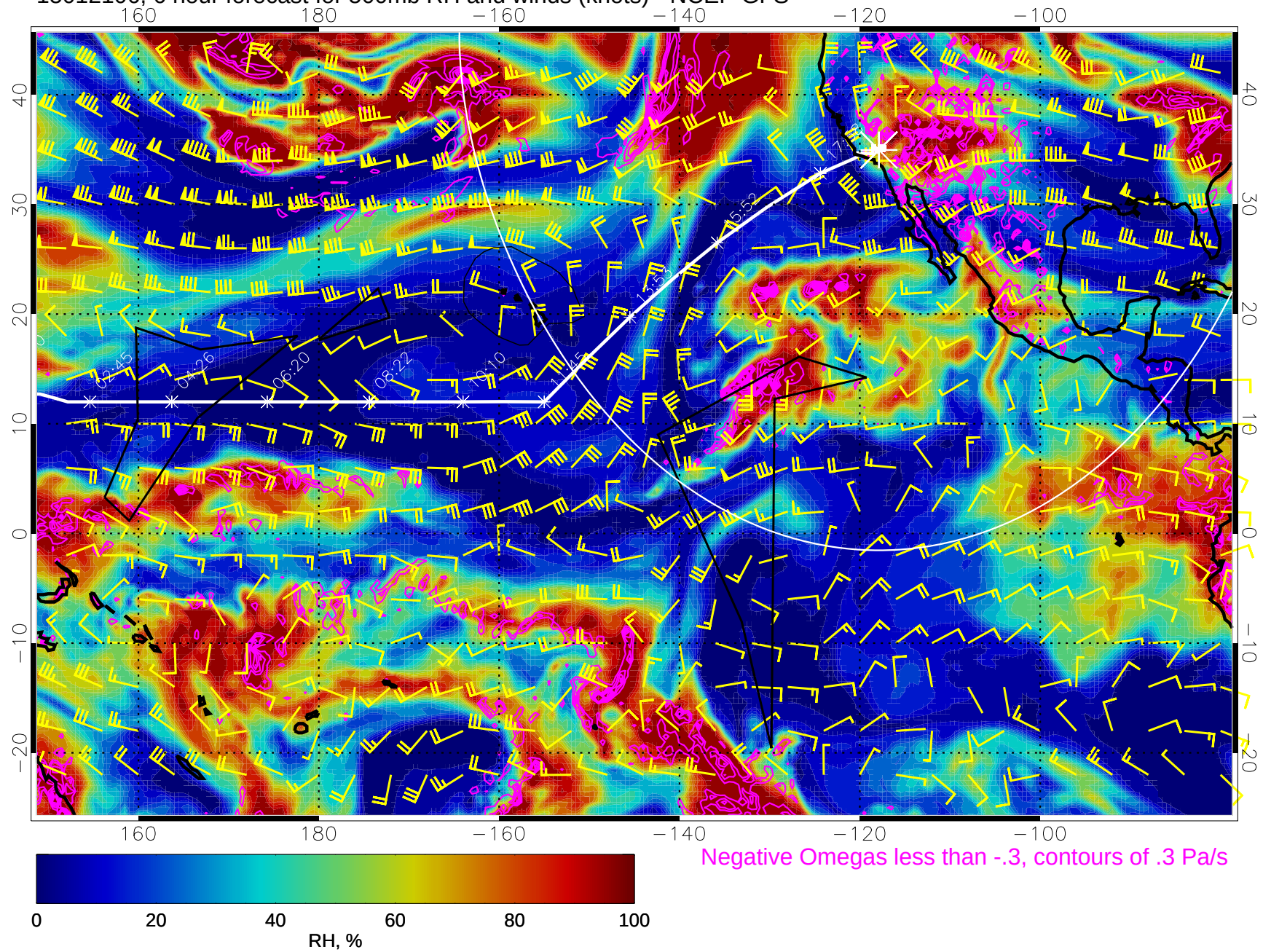
15012106, 6 hour forecast for 500mb RH and winds (knots) - NCEP GFS
