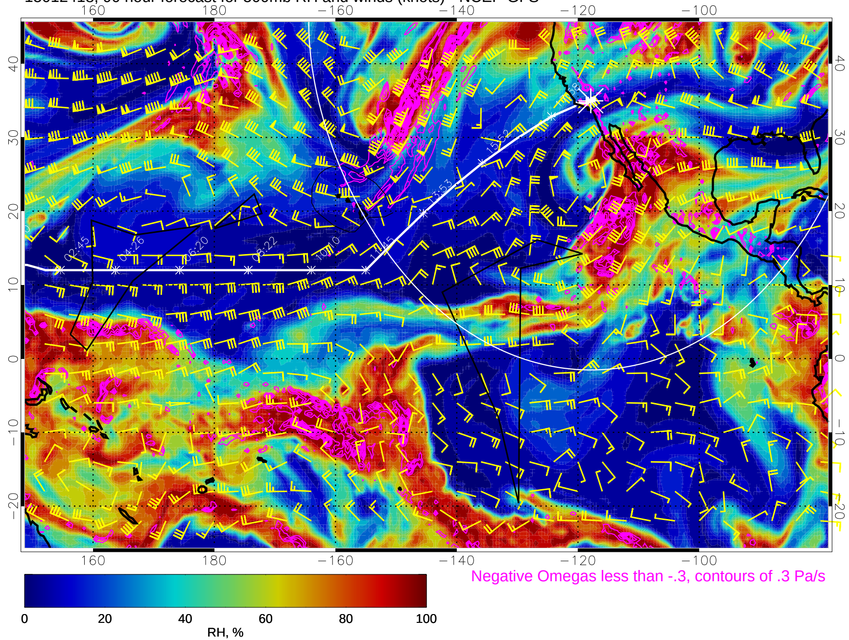
15012418, 90 hour forecast for 500mb RH and winds (knots) - NCEP GFS
