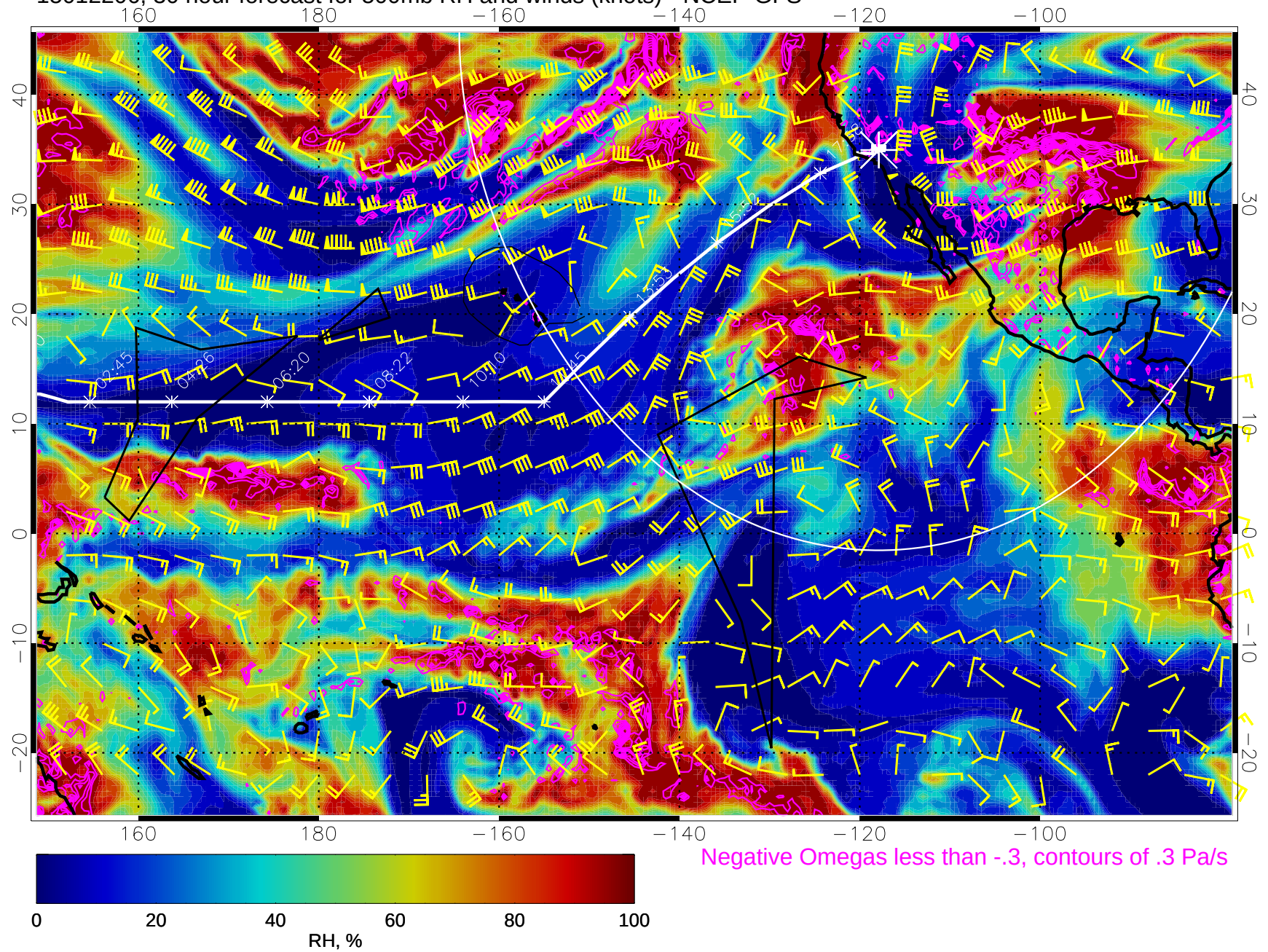
15012206, 30 hour forecast for 500mb RH and winds (knots) - NCEP GFS
