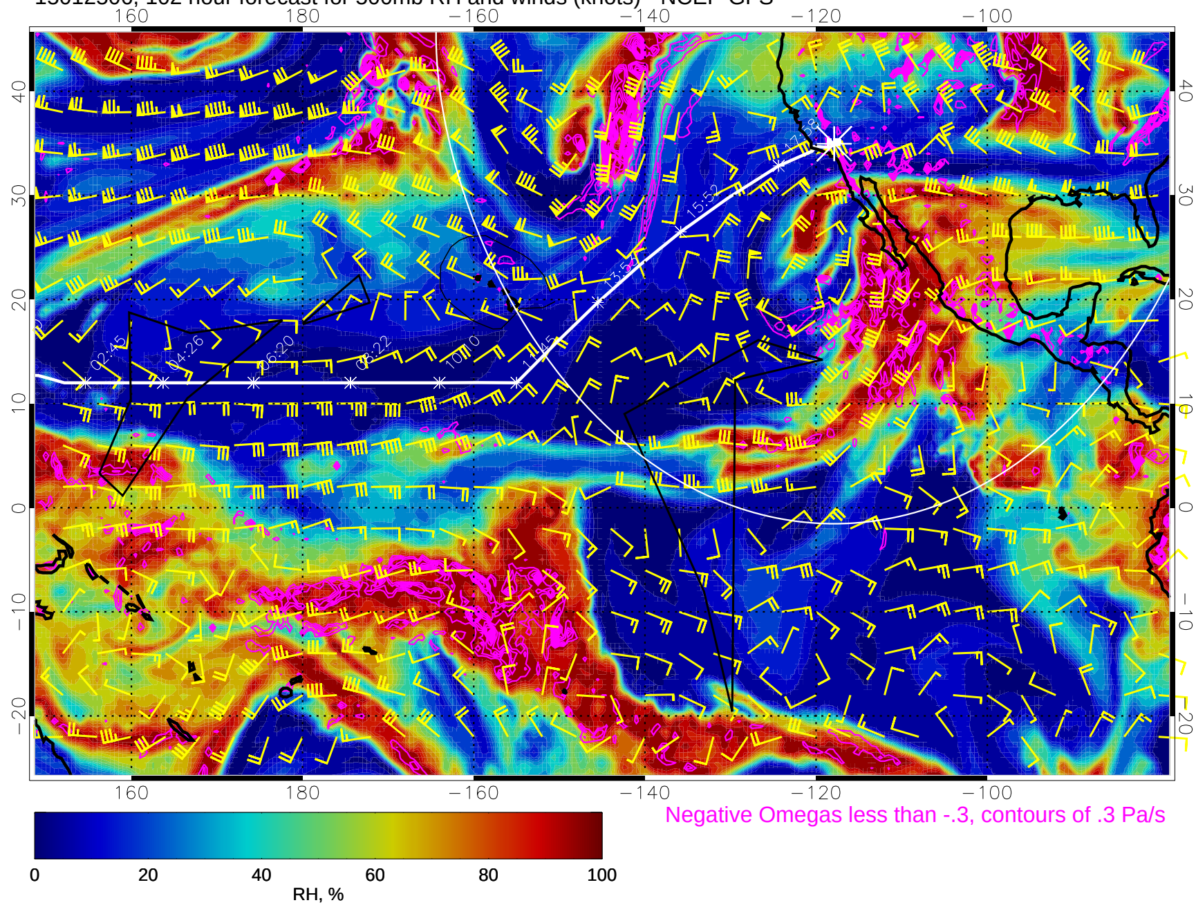
15012506, 102 hour forecast for 500mb RH and winds (knots) - NCEP GFS
