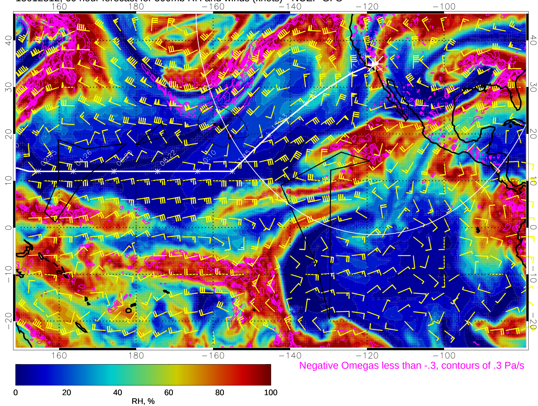
15012312, 60 hour forecast for 500mb RH and winds (knots) - NCEP GFS
