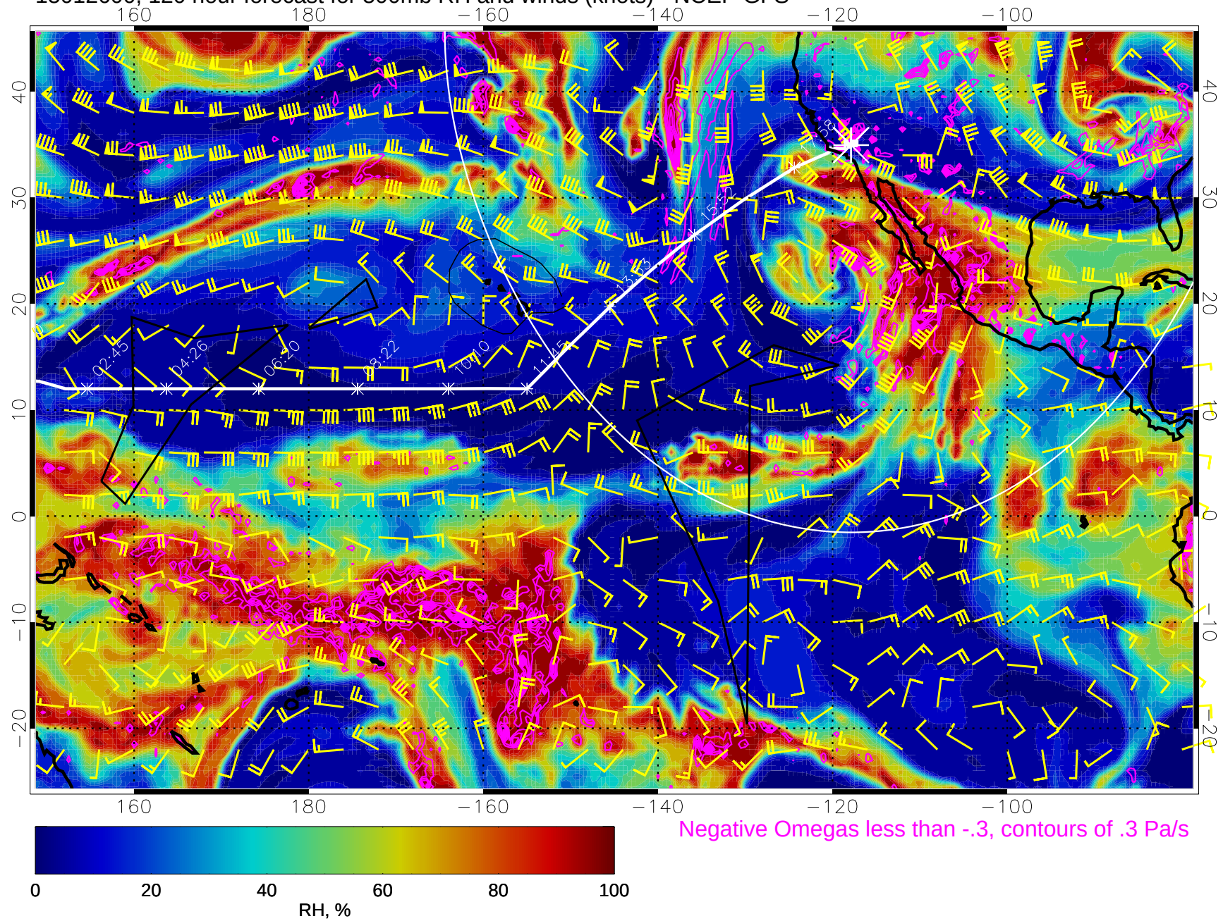
15012600, 120 hour forecast for 500mb RH and winds (knots) - NCEP GFS
