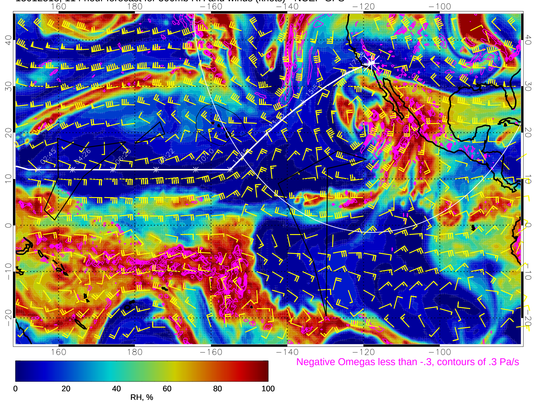
15012518, 114 hour forecast for 500mb RH and winds (knots) - NCEP GFS
