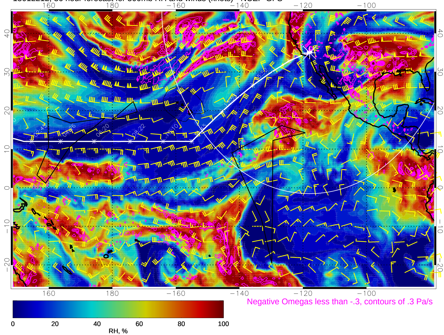
15012212, 36 hour forecast for 500mb RH and winds (knots) - NCEP GFS
