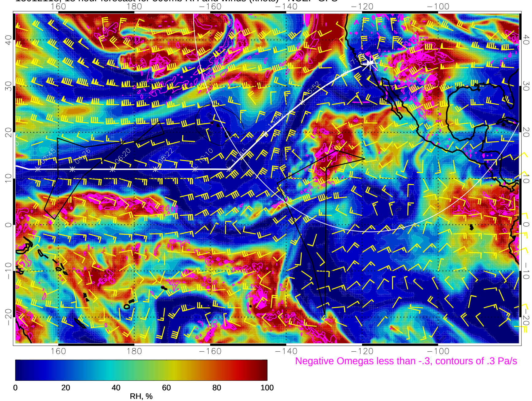
15012118, 18 hour forecast for 500mb RH and winds (knots) - NCEP GFS
