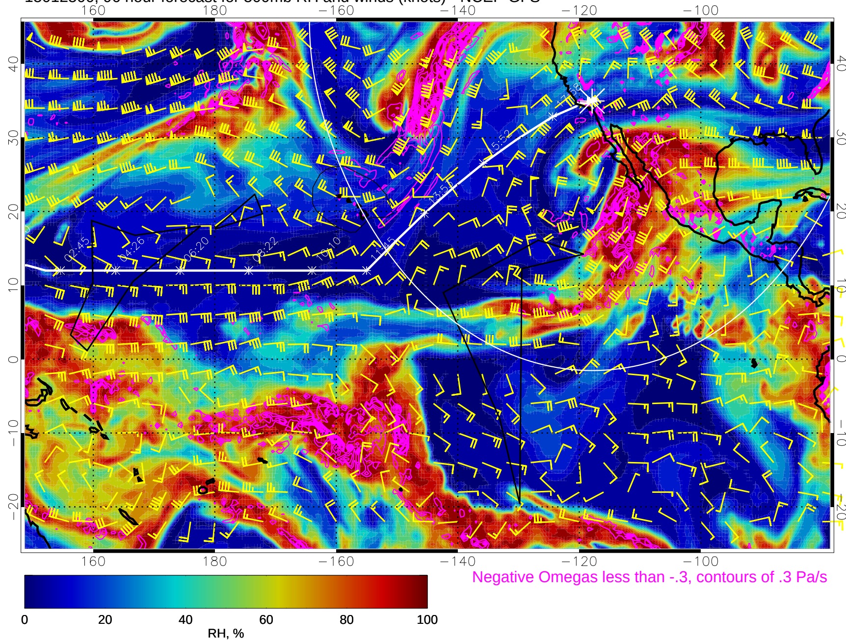
15012500, 96 hour forecast for 500mb RH and winds (knots) - NCEP GFS
