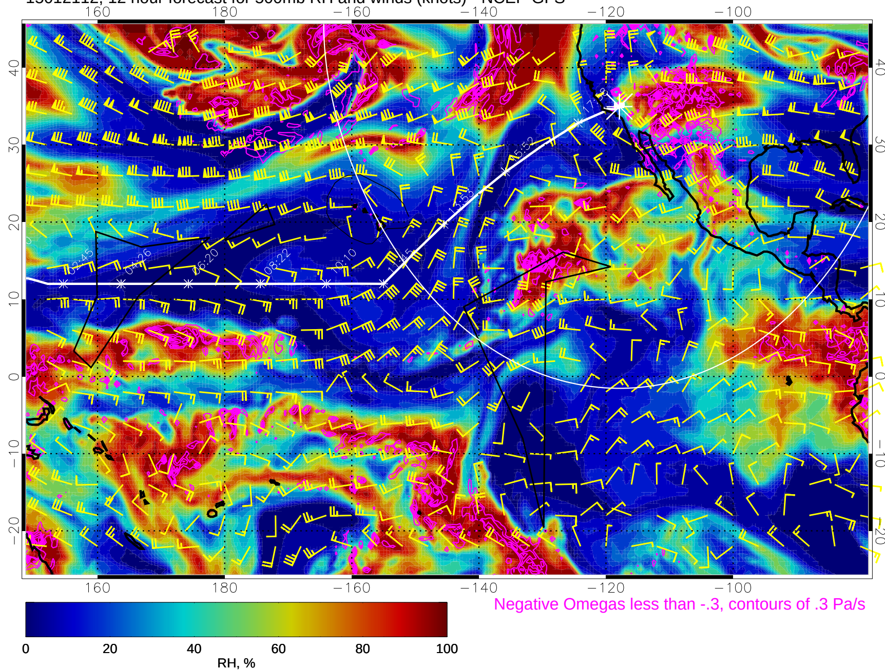
15012112, 12 hour forecast for 500mb RH and winds (knots) - NCEP GFS
