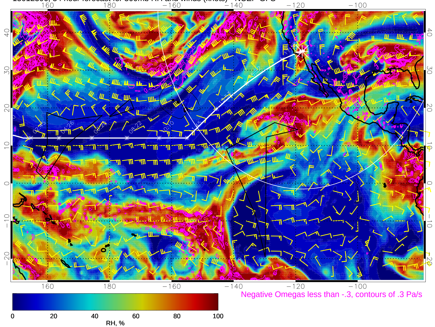
15012306, 54 hour forecast for 500mb RH and winds (knots) - NCEP GFS
