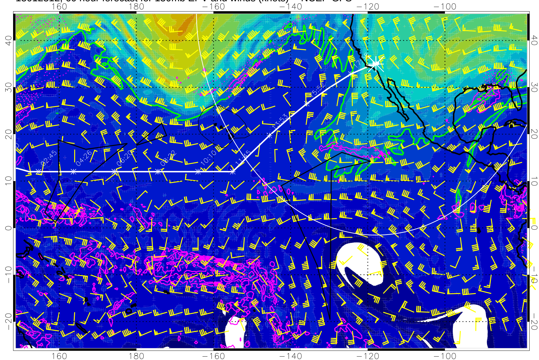
15012312, 60 hour forecast for 150mb EPV and winds (knots) -- NCEP GFS
