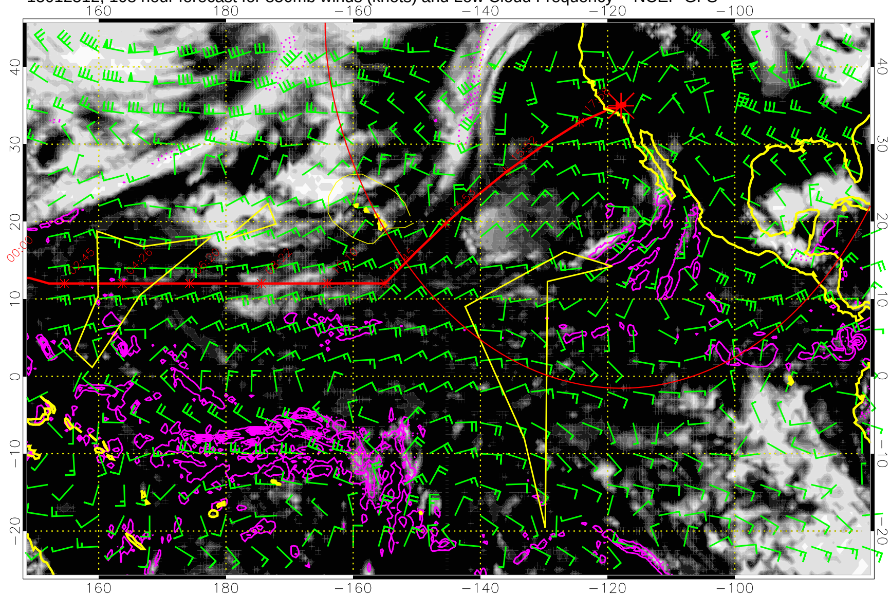
15012512, 108 hour forecast for 850mb winds (knots) and Low Cloud Frequency -- NCEP GFS
