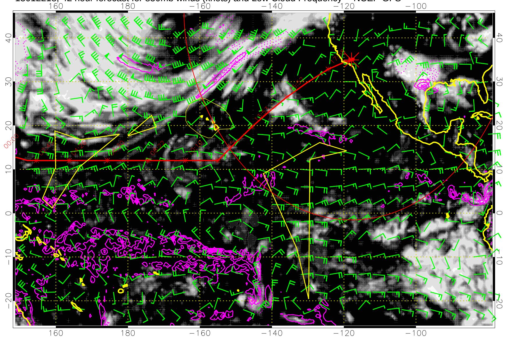
15012218, 42 hour forecast for 850mb winds (knots) and Low Cloud Frequency -- NCEP GFS
