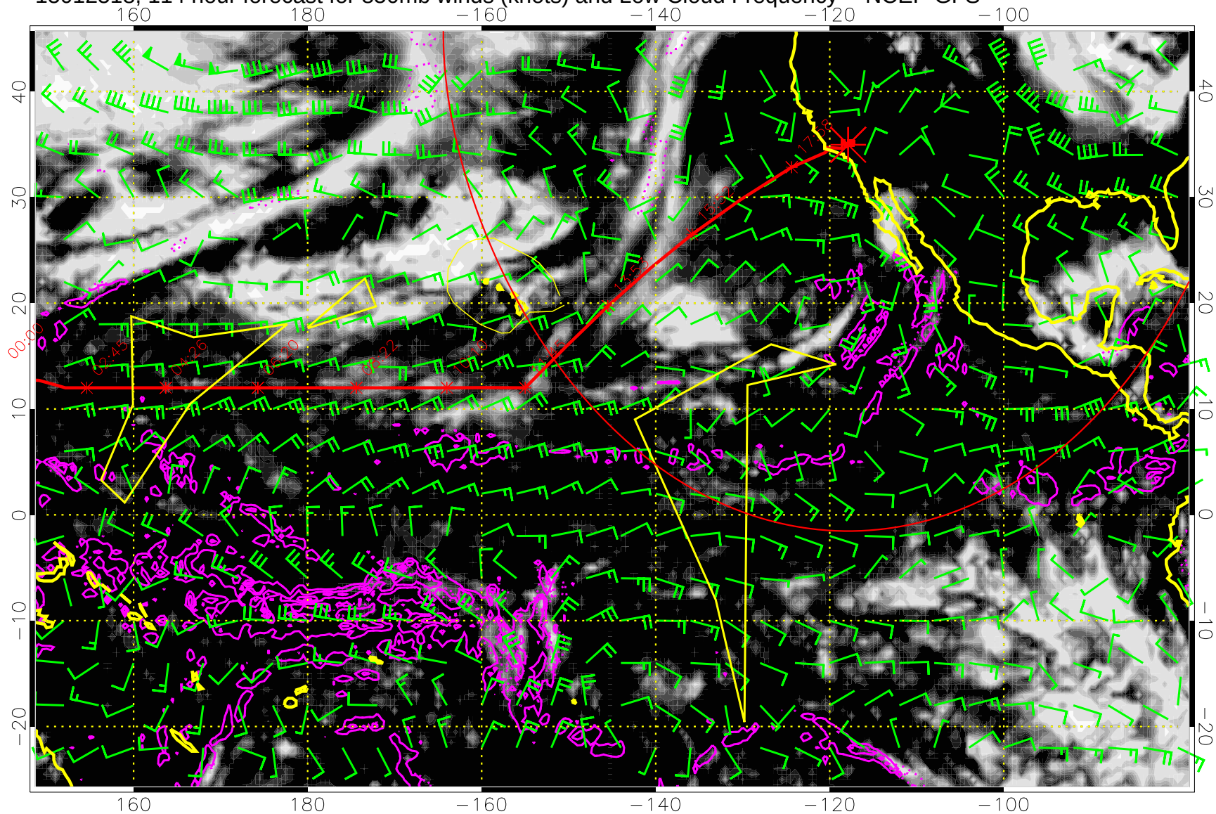
15012518, 114 hour forecast for 850mb winds (knots) and Low Cloud Frequency -- NCEP GFS
