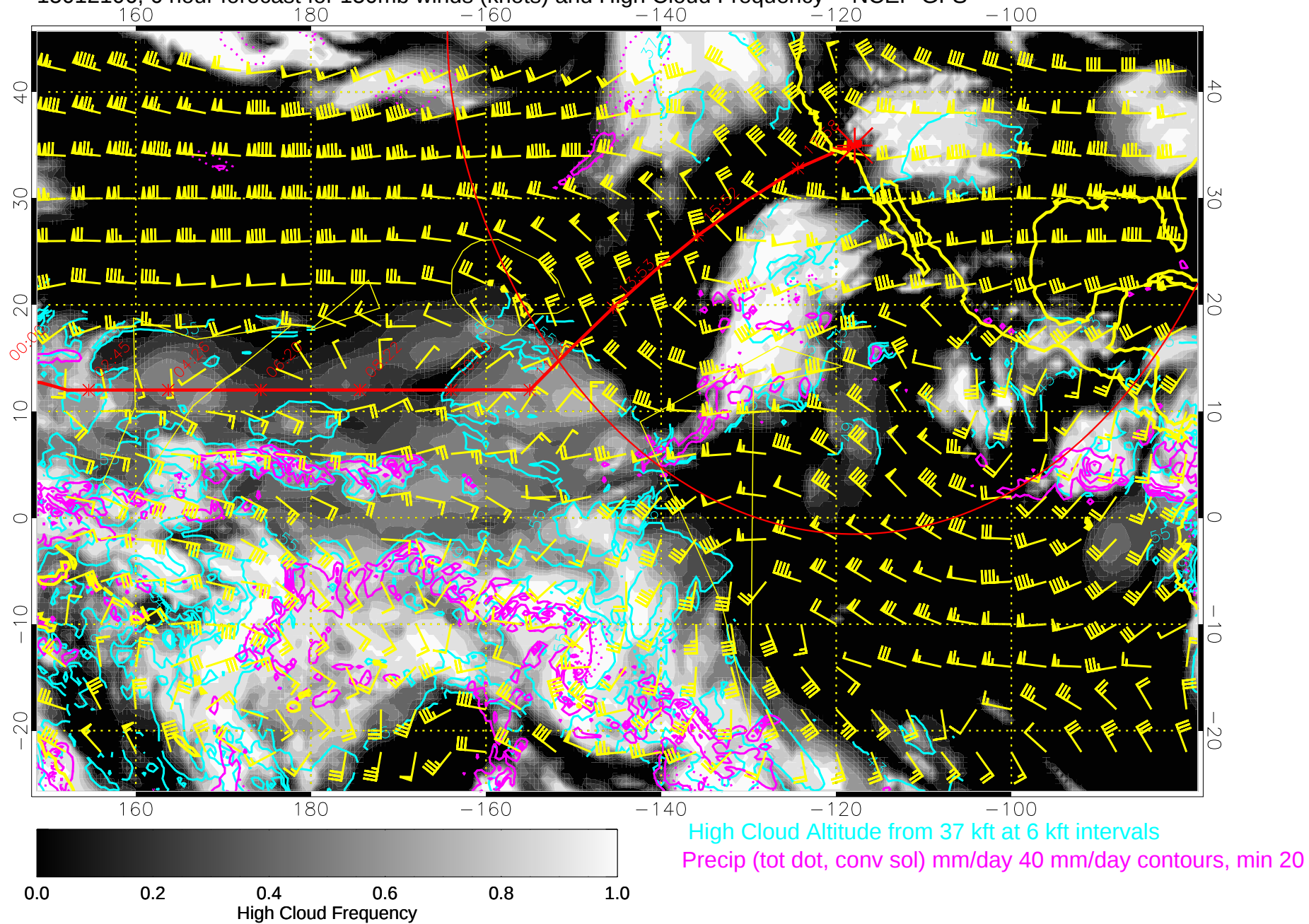
15012106, 6 hour forecast for 150mb winds (knots) and High Cloud Frequency -- NCEP GFS
