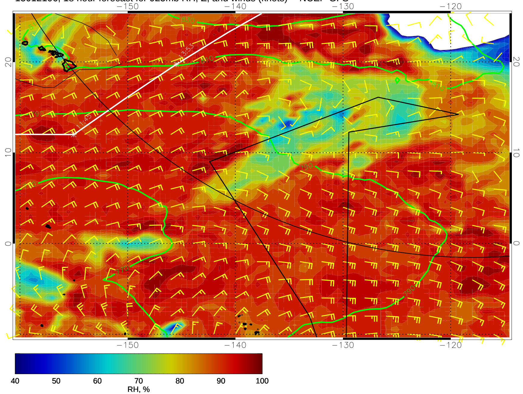
15012106, 18 hour forecast for 925mb RH, Z, and winds (knots) -- NCEP GFS
