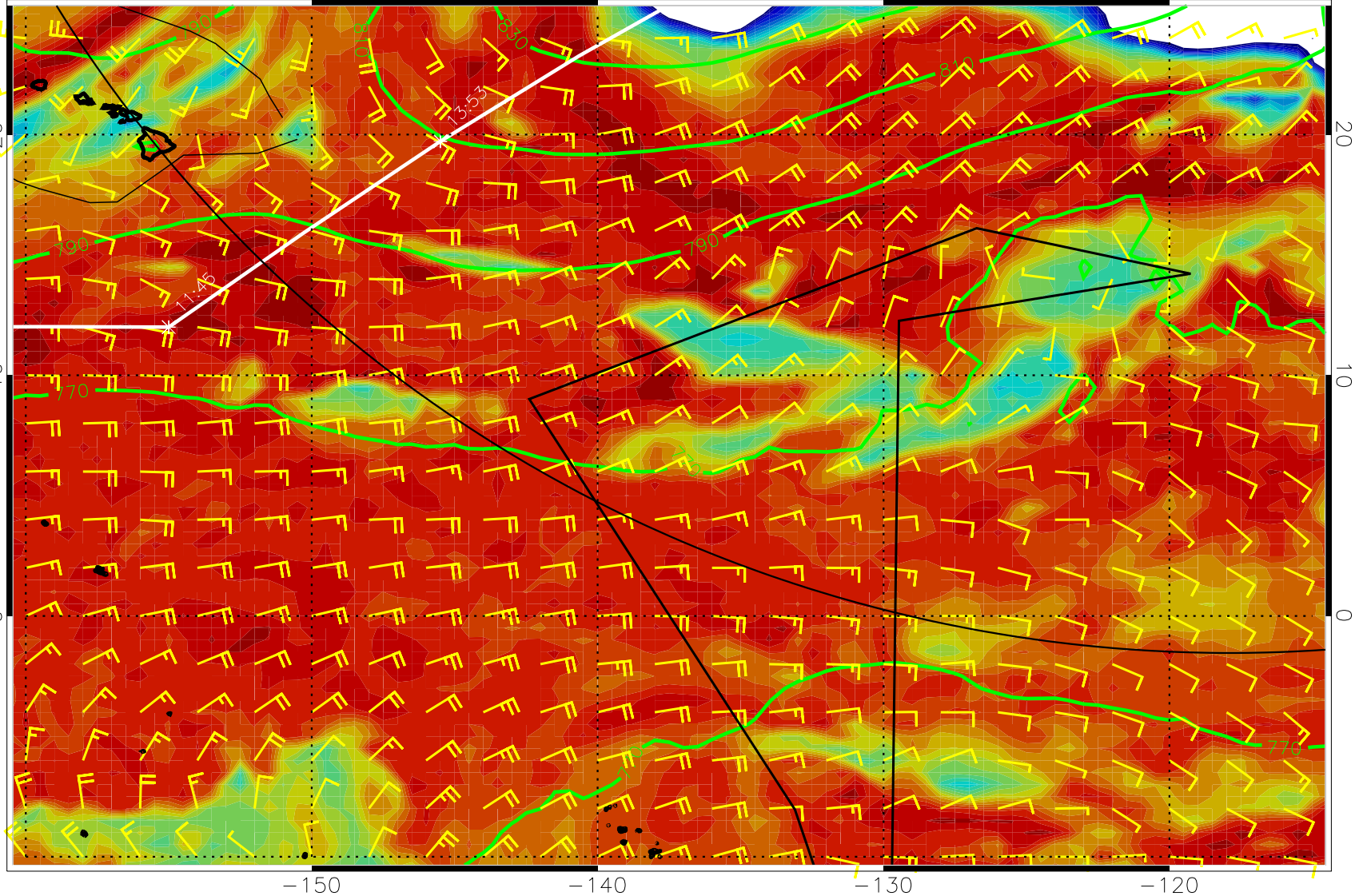
20022-100, 5 yr. lead forecast for: storms (in), \pm , and winds (knots) 2002 2003 2004 2005 -150 -140 -130 -120
