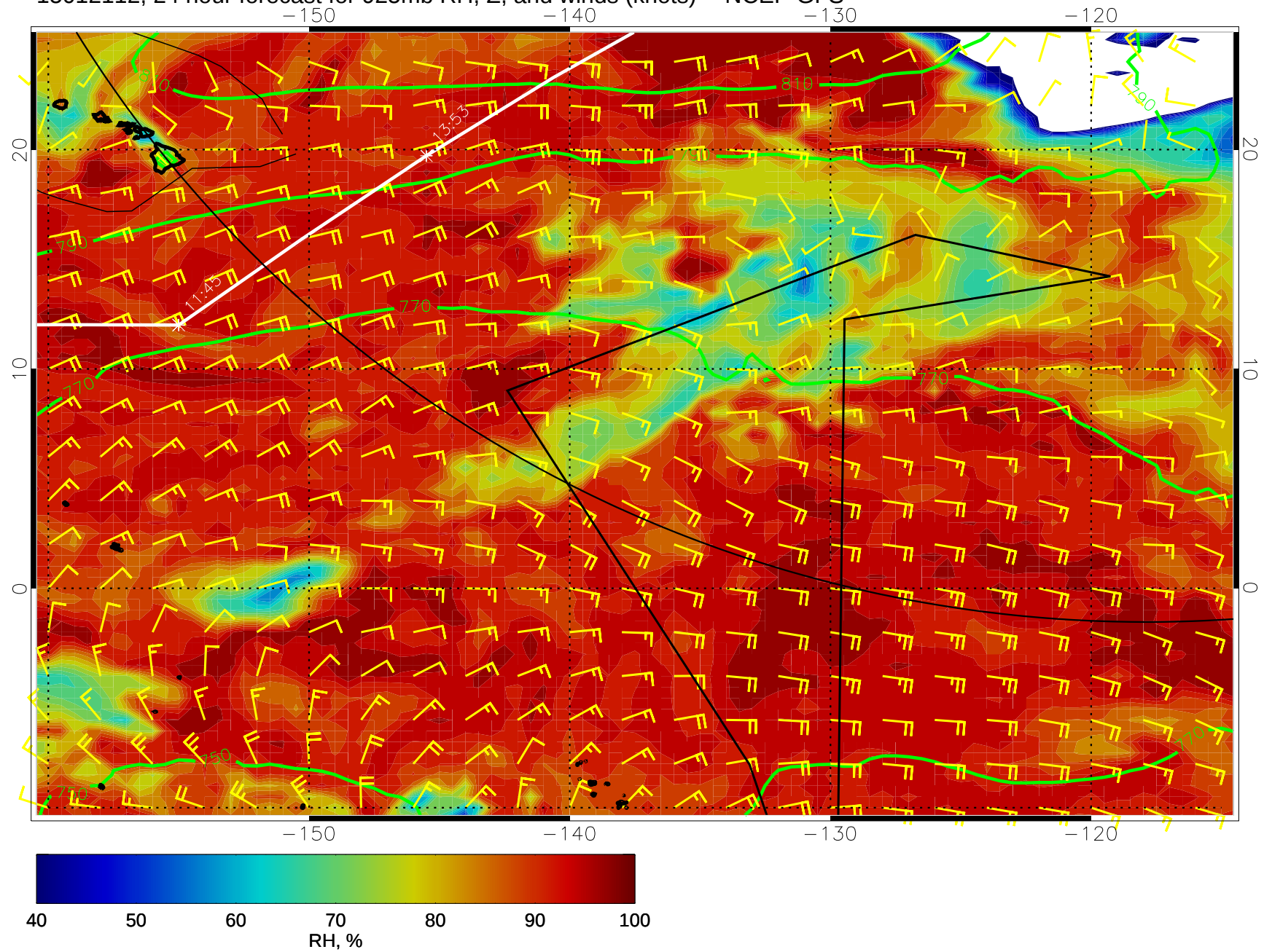
15012112, 24 hour forecast for 925mb RH, Z, and winds (knots) -- NCEP GFS
