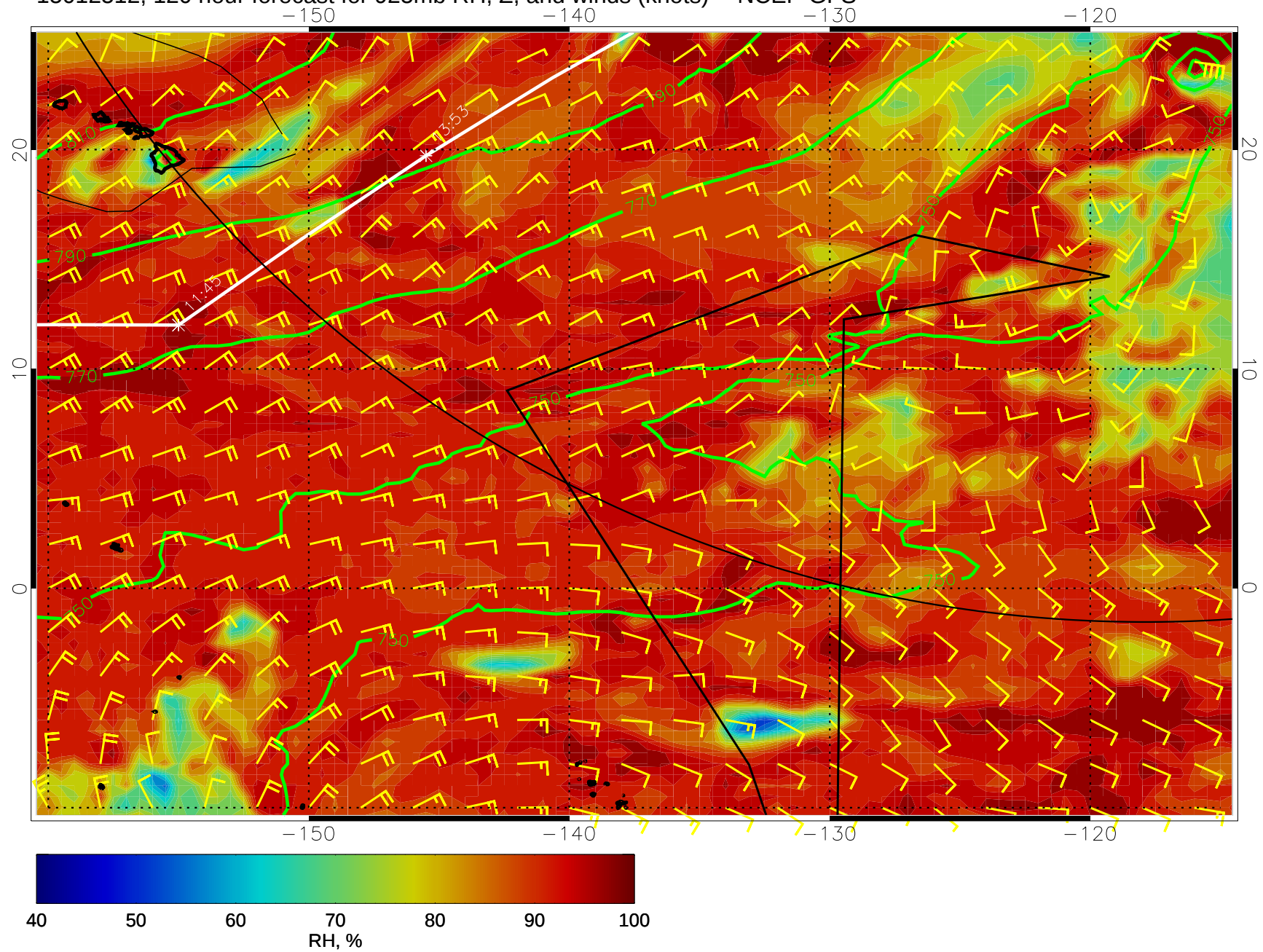
15012512, 120 hour forecast for 925mb RH, Z, and winds (knots) -- NCEP GFS
