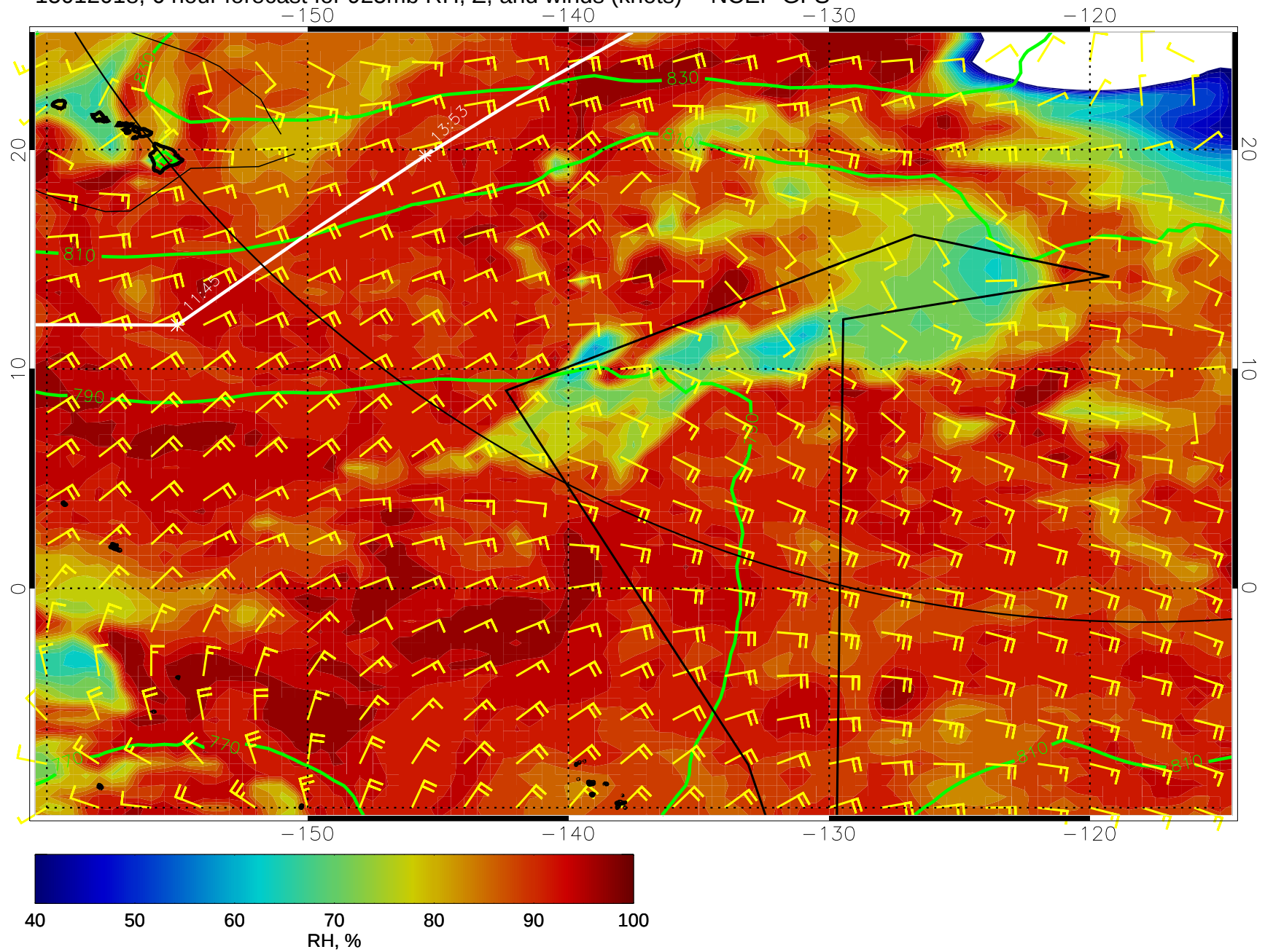
15012018, 6 hour forecast for 925mb RH, Z, and winds (knots) -- NCEP GFS
