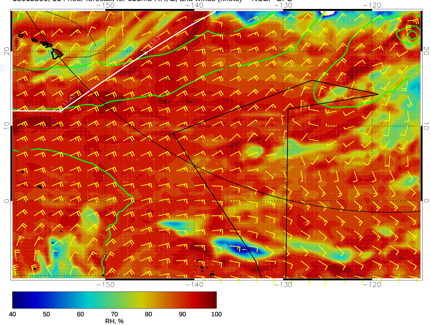
15012506, 114 hour forecast for 925mb RH, Z, and winds (knots) -- NCEP GFS
