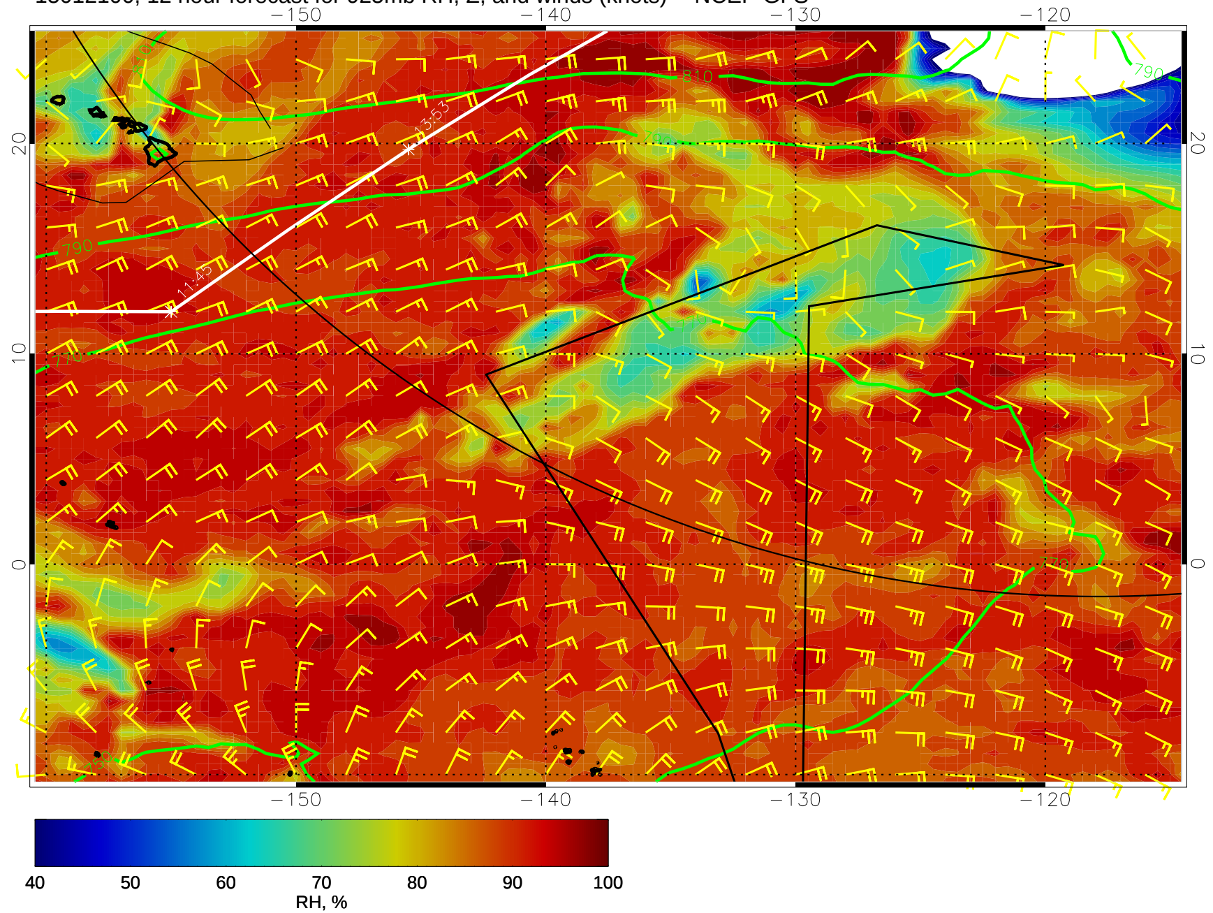
15012100, 12 hour forecast for 925mb RH, Z, and winds (knots) -- NCEP GFS
