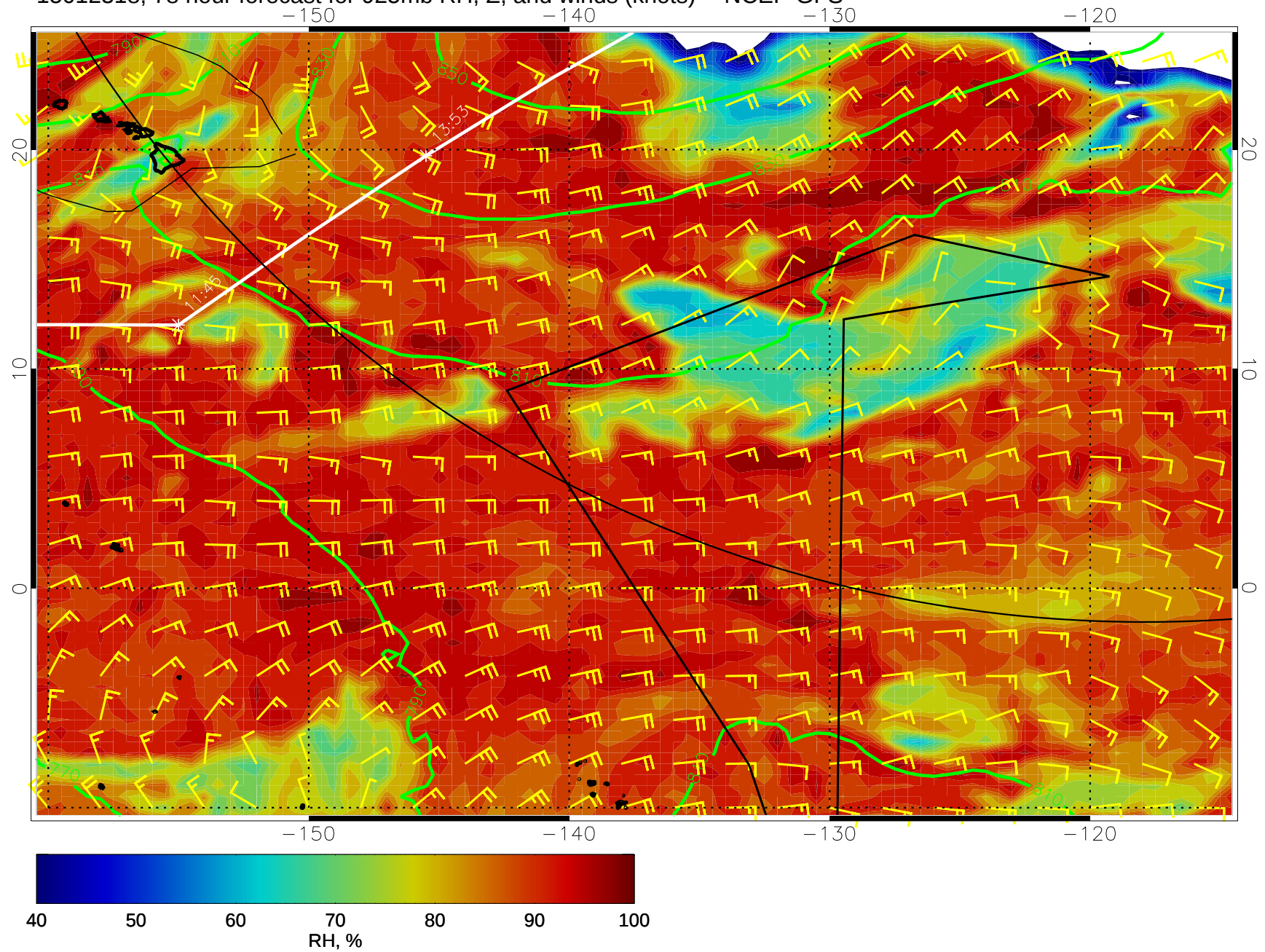
15012318, 78 hour forecast for 925mb RH, Z, and winds (knots) -- NCEP GFS
