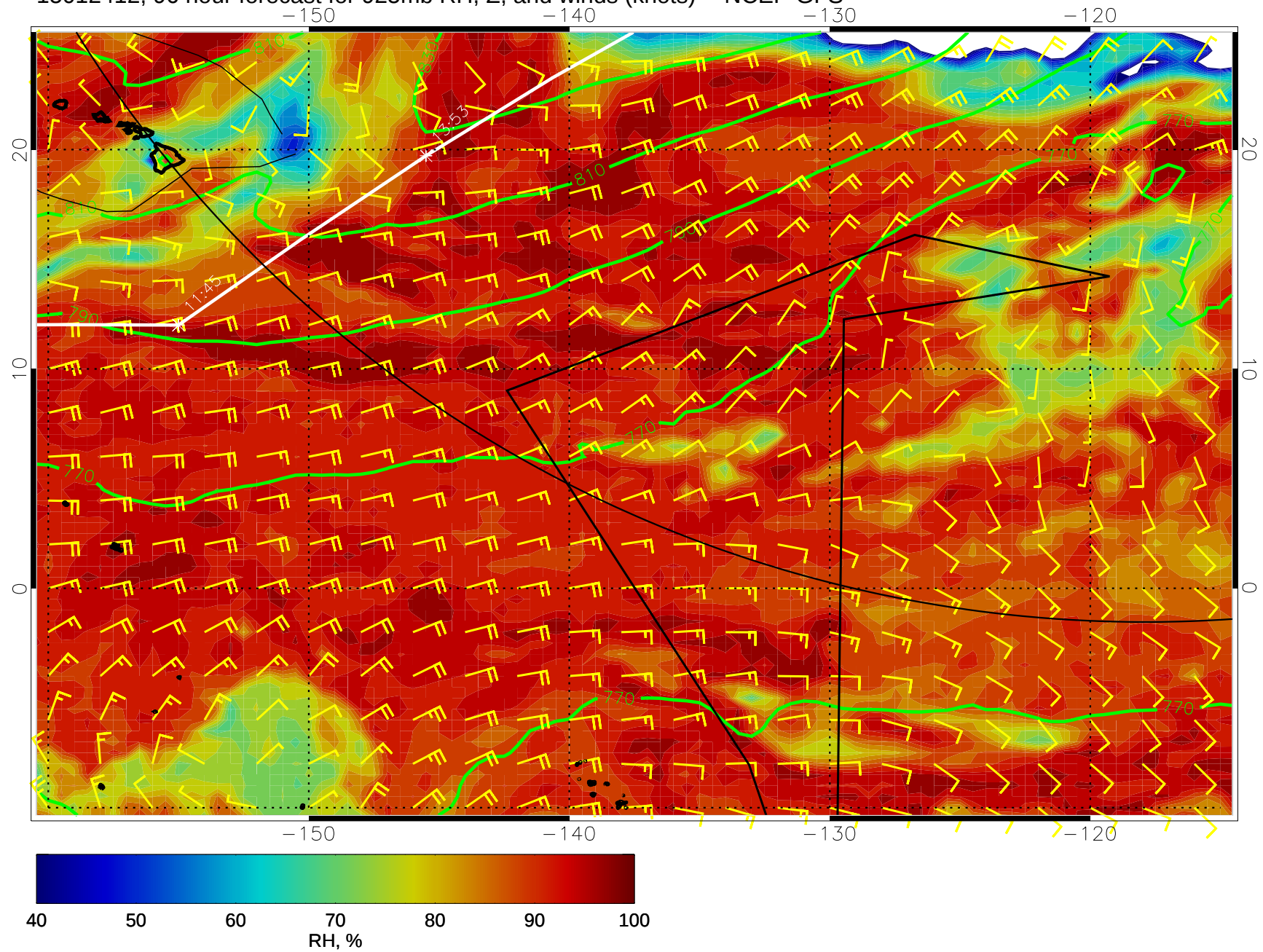
15012412, 96 hour forecast for 925mb RH, Z, and winds (knots) -- NCEP GFS
