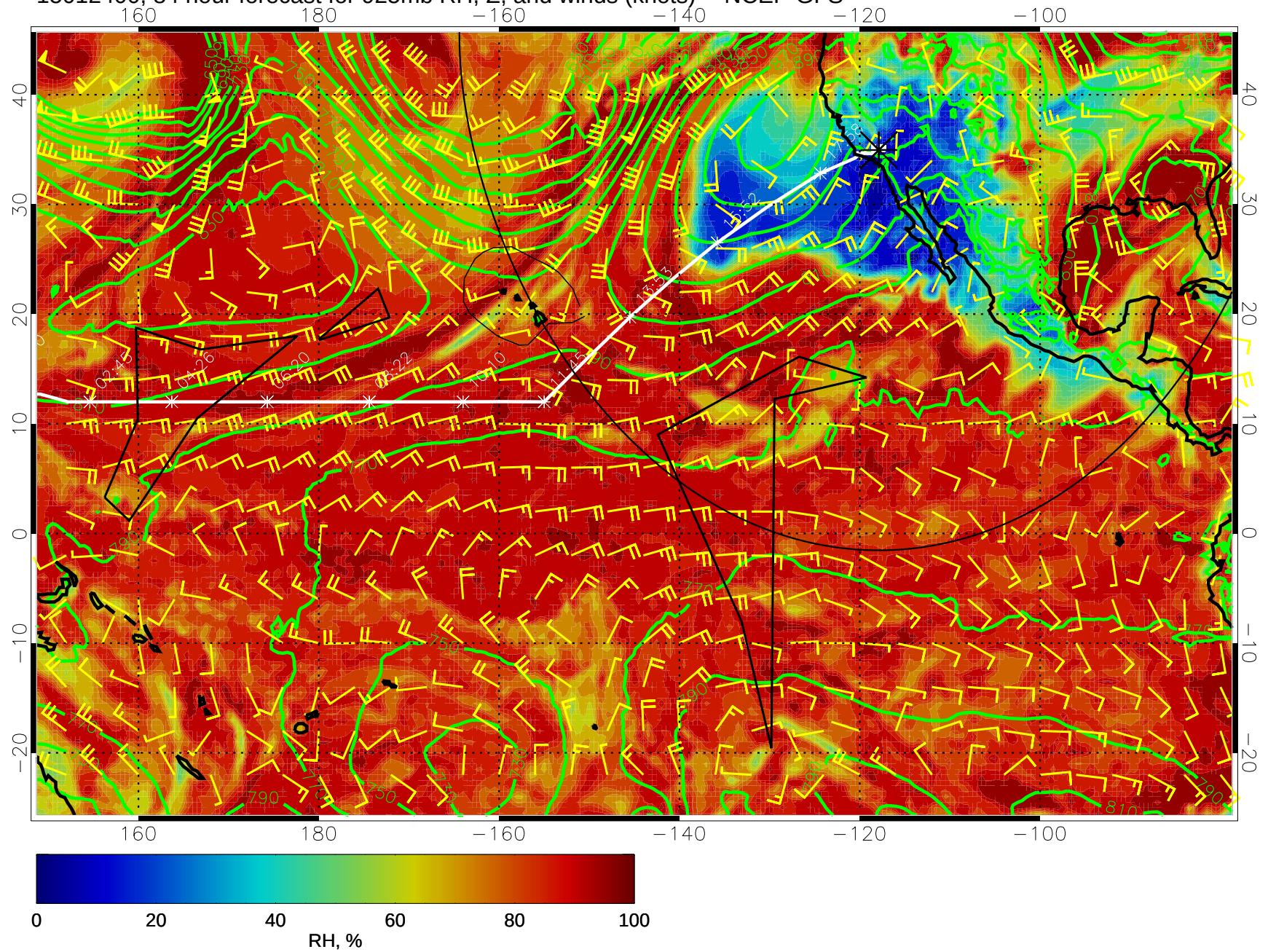
15012400, 84 hour forecast for 925mb RH, Z, and winds (knots) -- NCEP GFS
