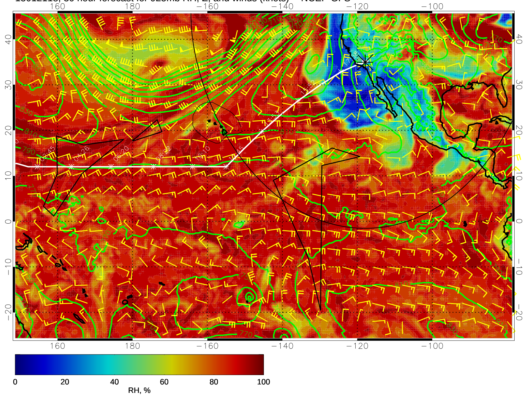
15012118, 30 hour forecast for 925mb RH, Z, and winds (knots) -- NCEP GFS
