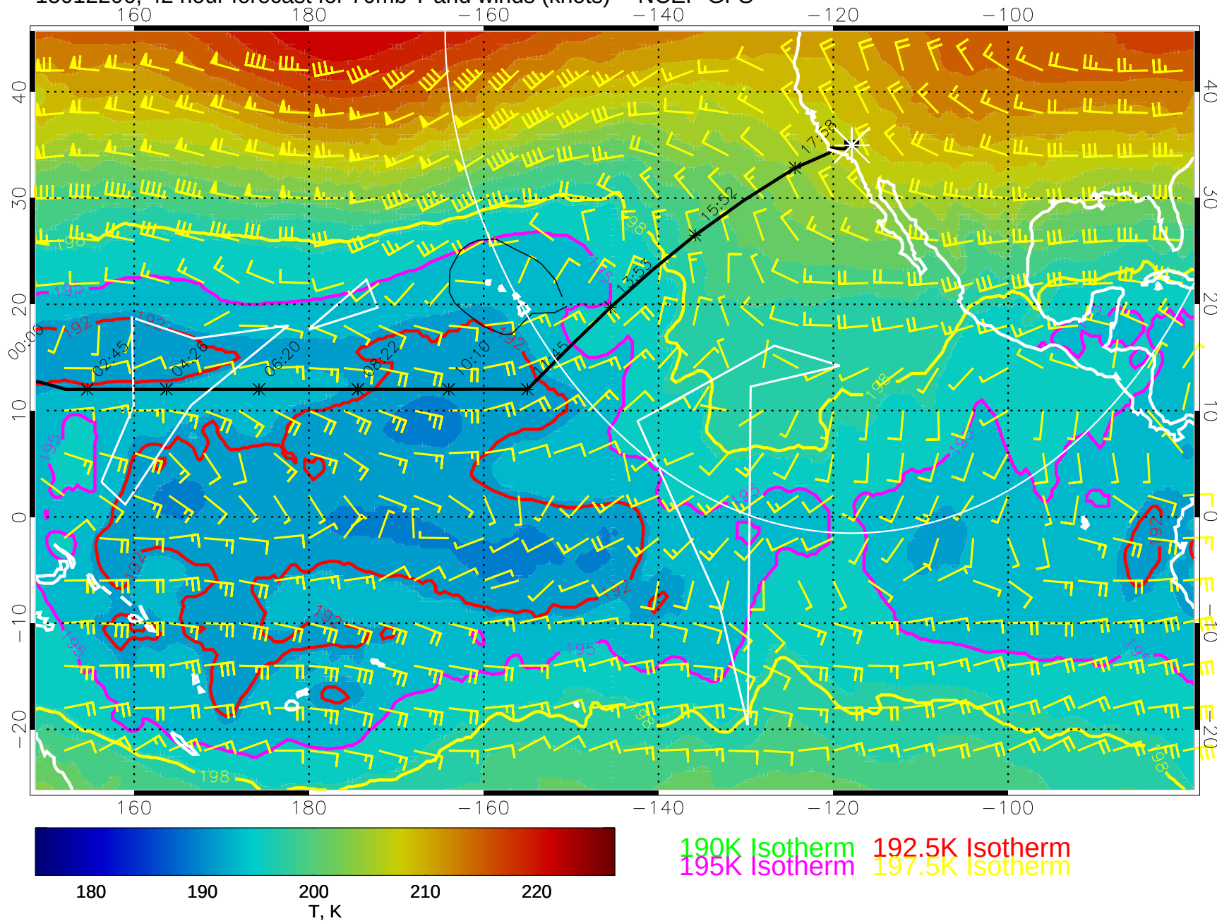
15012206, 42 hour forecast for 70mb T and winds (knots) -- NCEP GFS
