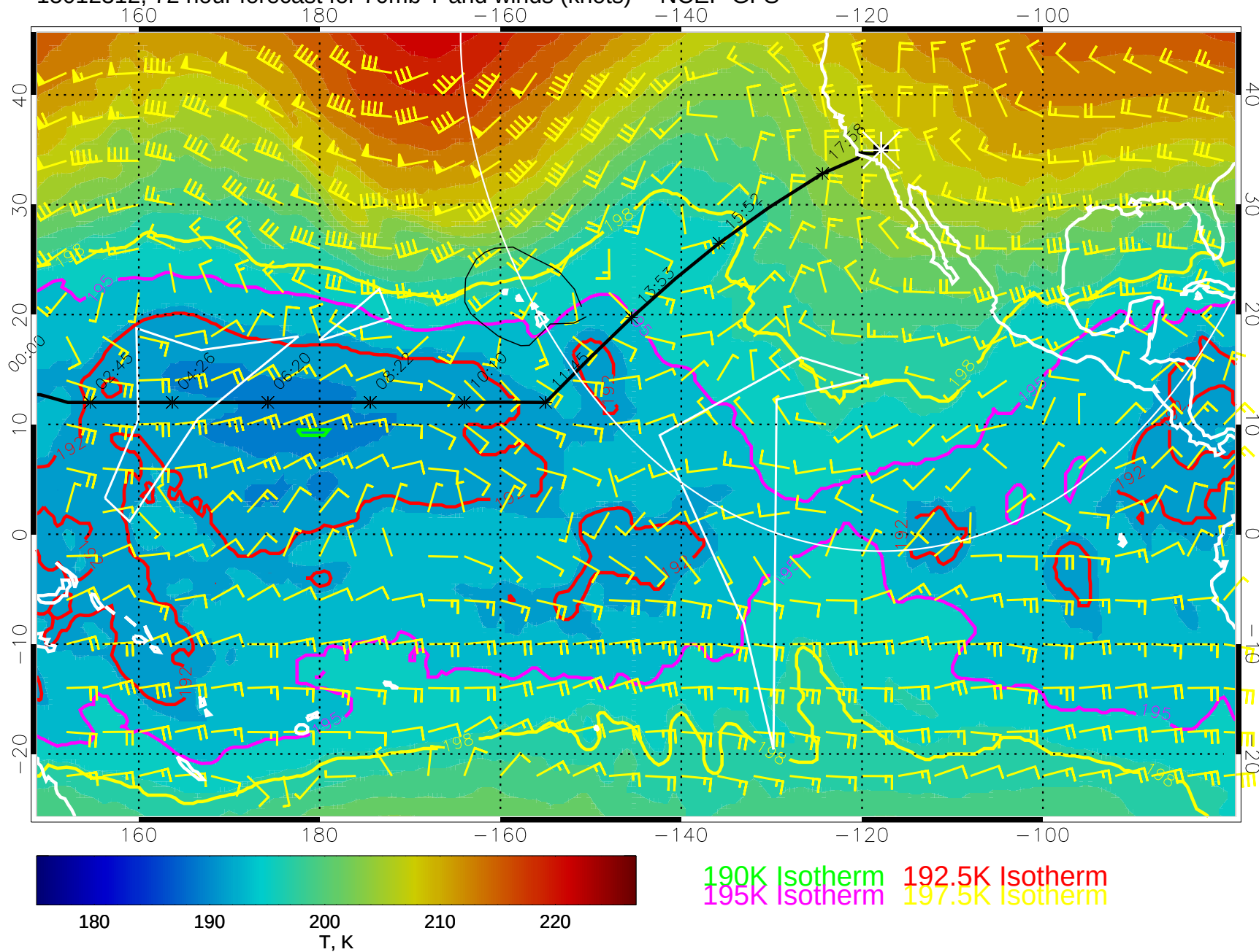
15012312, 72 hour forecast for 70mb T and winds (knots) -- NCEP GFS
