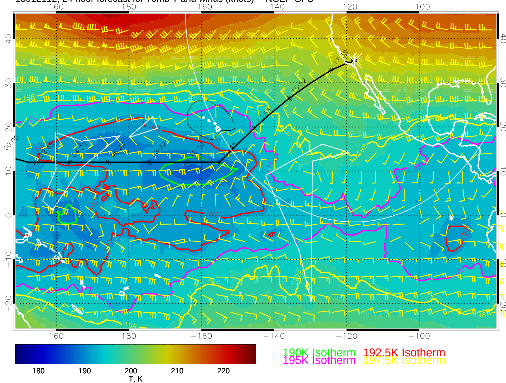
15012112, 24 hour forecast for 70mb T and winds (knots) -- NCEP GFS
