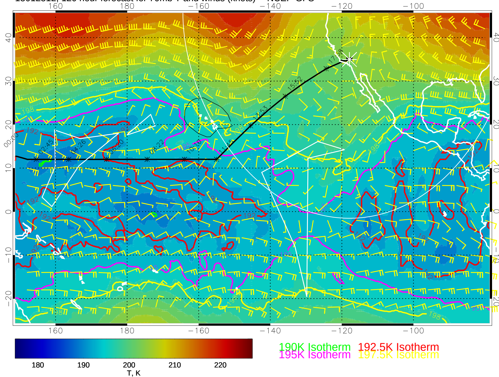
15012512, 120 hour forecast for 70mb T and winds (knots) -- NCEP GFS
