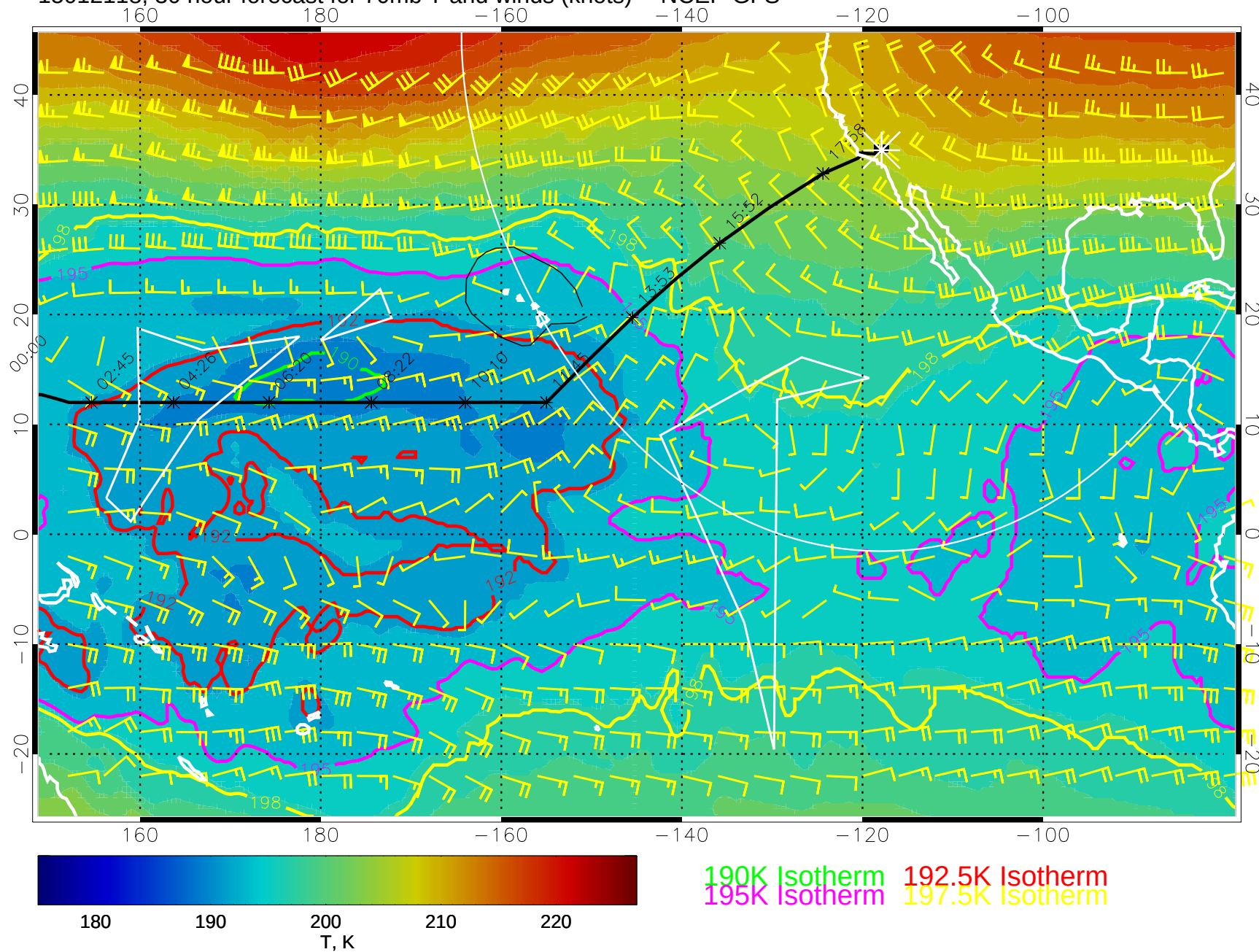
15012118, 30 hour forecast for 70mb T and winds (knots) -- NCEP GFS
