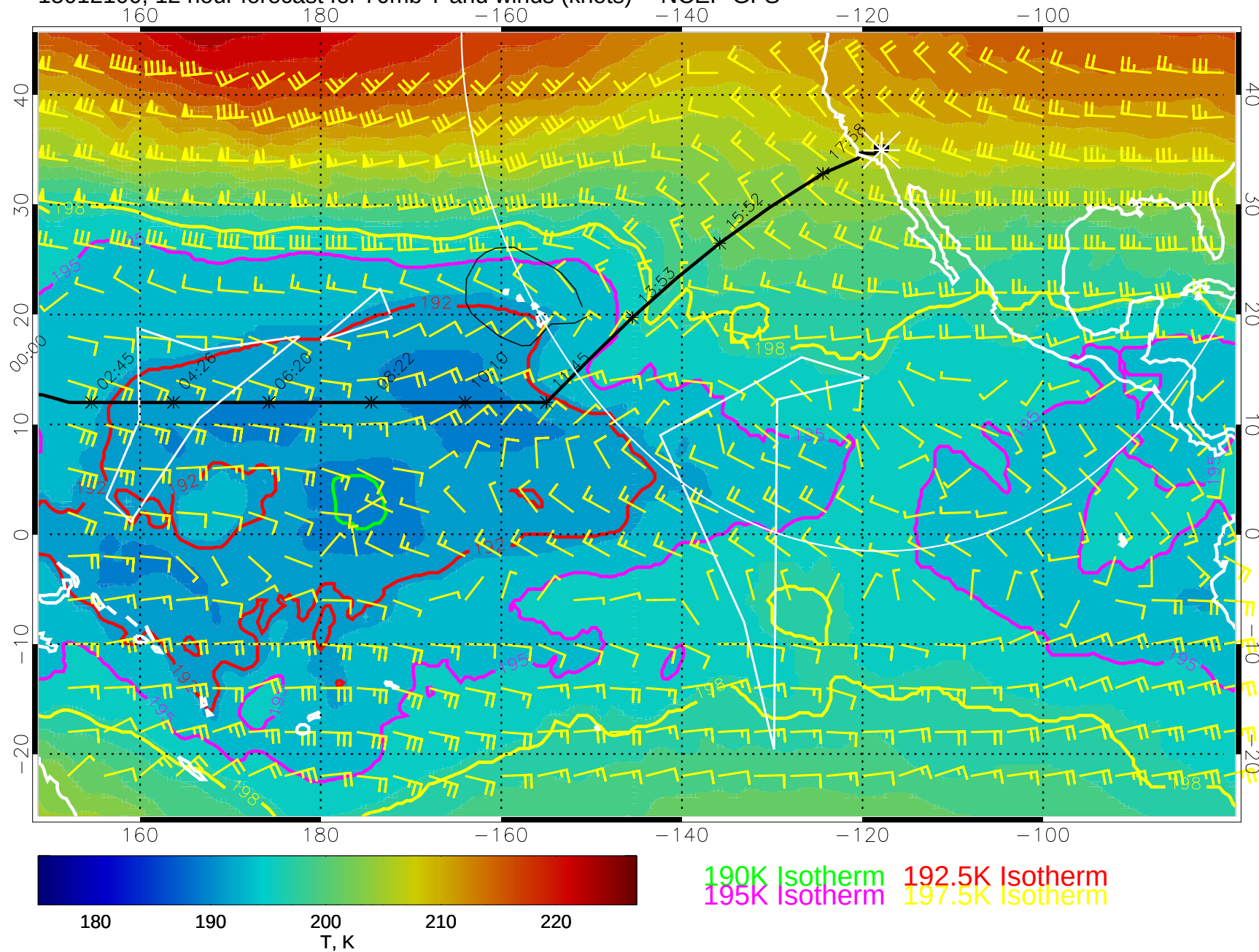
15012100, 12 hour forecast for 70mb T and winds (knots) -- NCEP GFS
