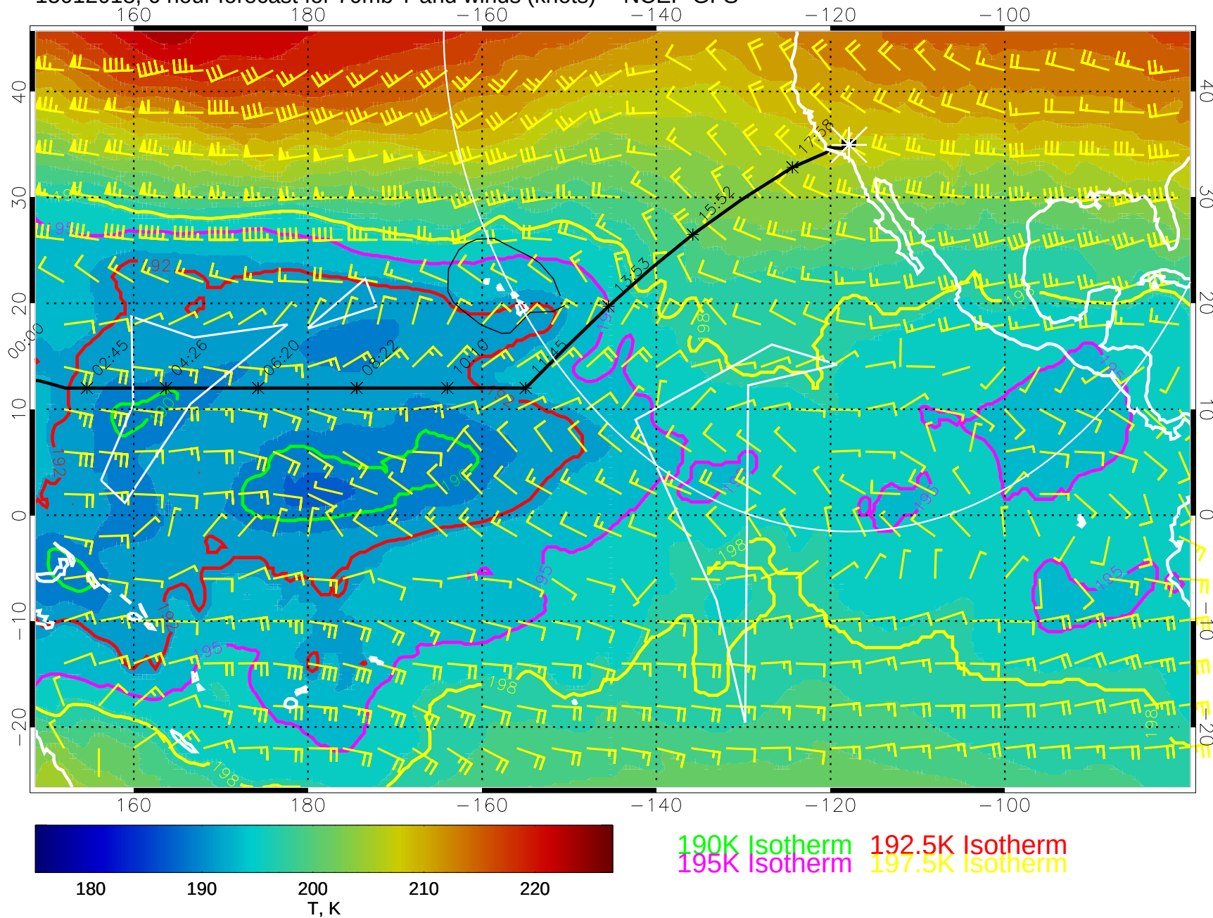
15012018, 6 hour forecast for 70mb T and winds (knots) -- NCEP GFS
