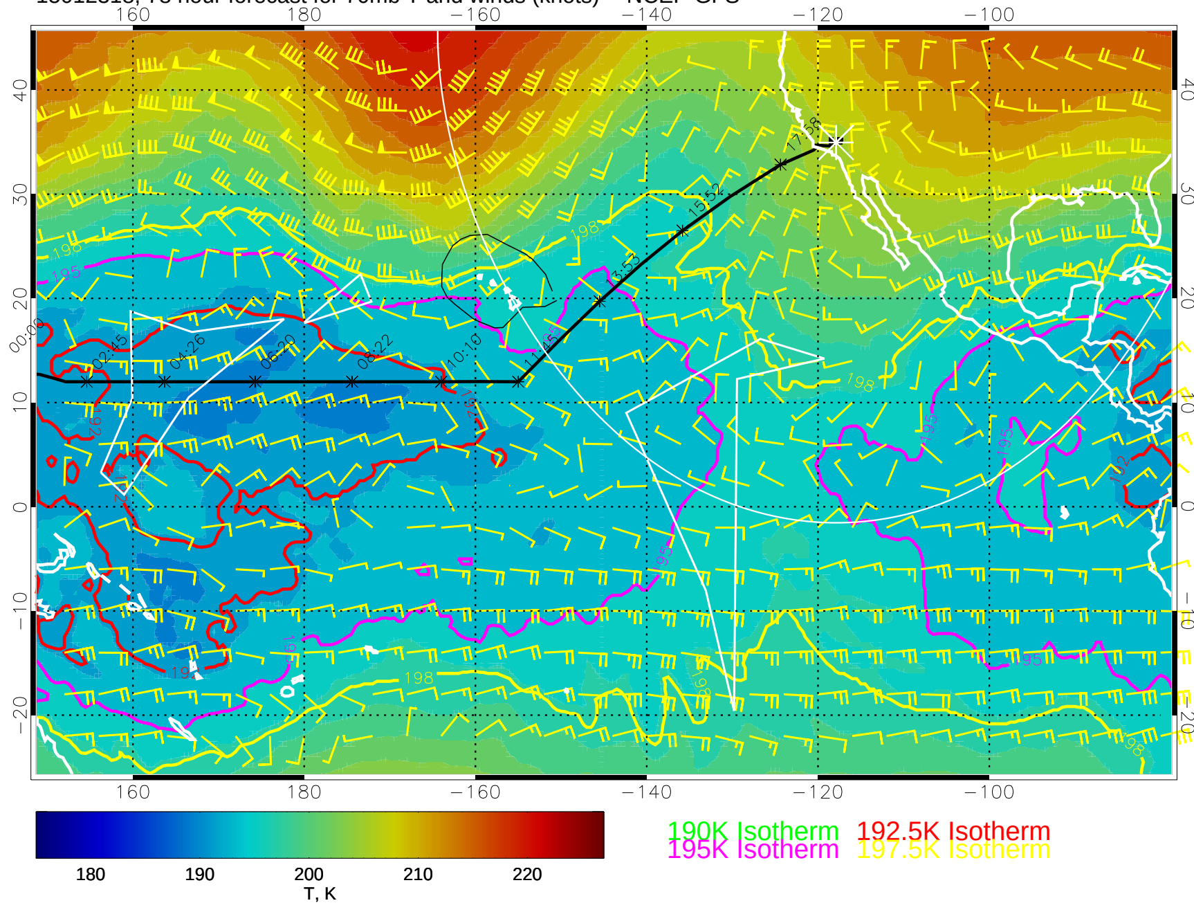
15012318, 78 hour forecast for 70mb T and winds (knots) -- NCEP GFS
