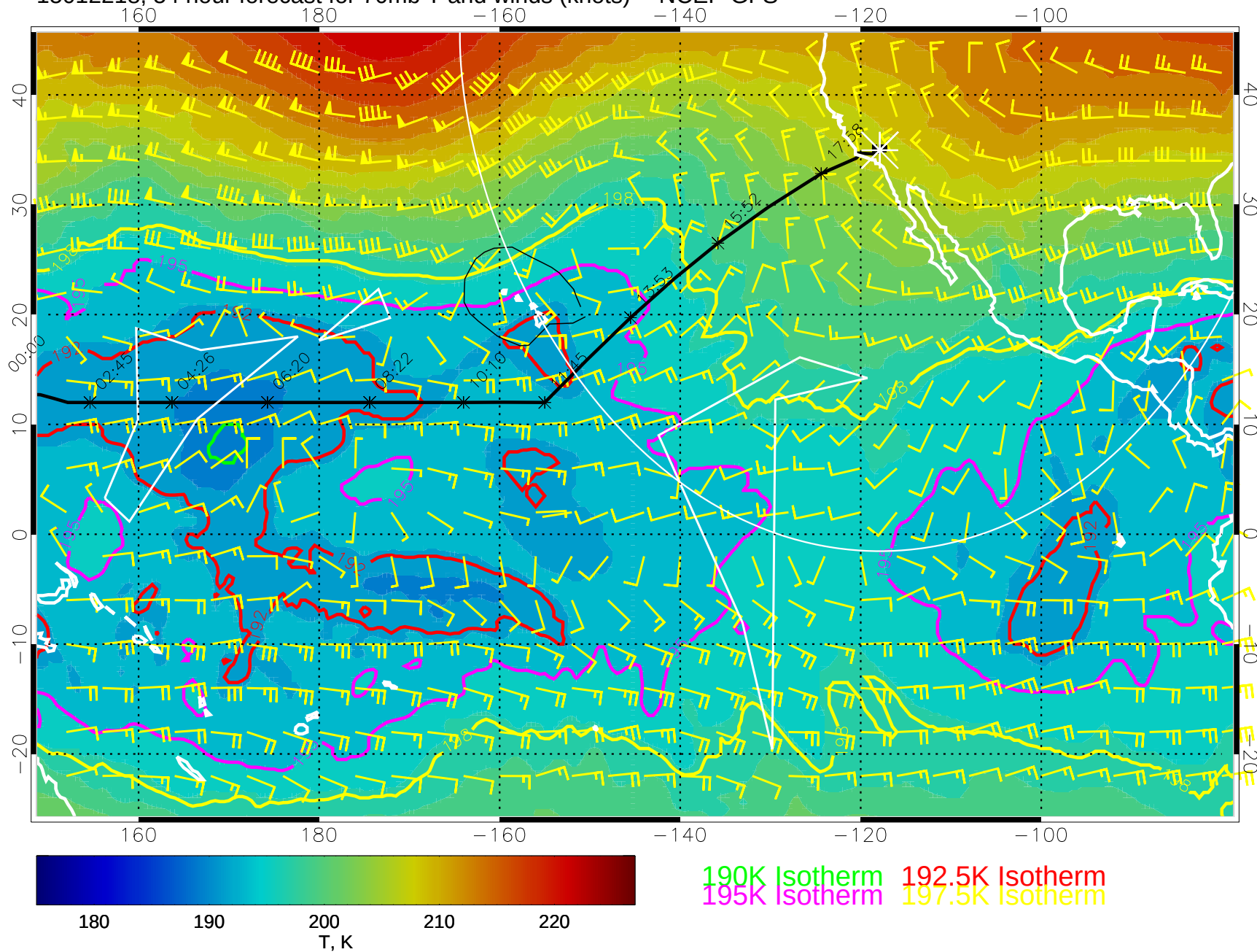
15012218, 54 hour forecast for 70mb T and winds (knots) -- NCEP GFS
