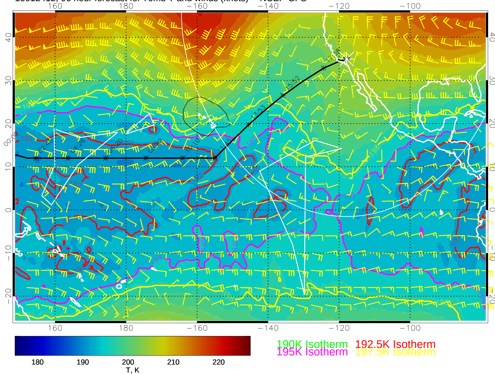
15012412, 96 hour forecast for 70mb T and winds (knots) -- NCEP GFS
