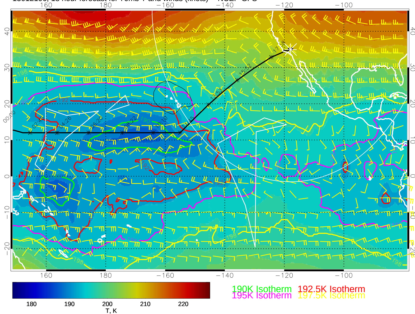
15012106, 18 hour forecast for 70mb T and winds (knots) -- NCEP GFS
