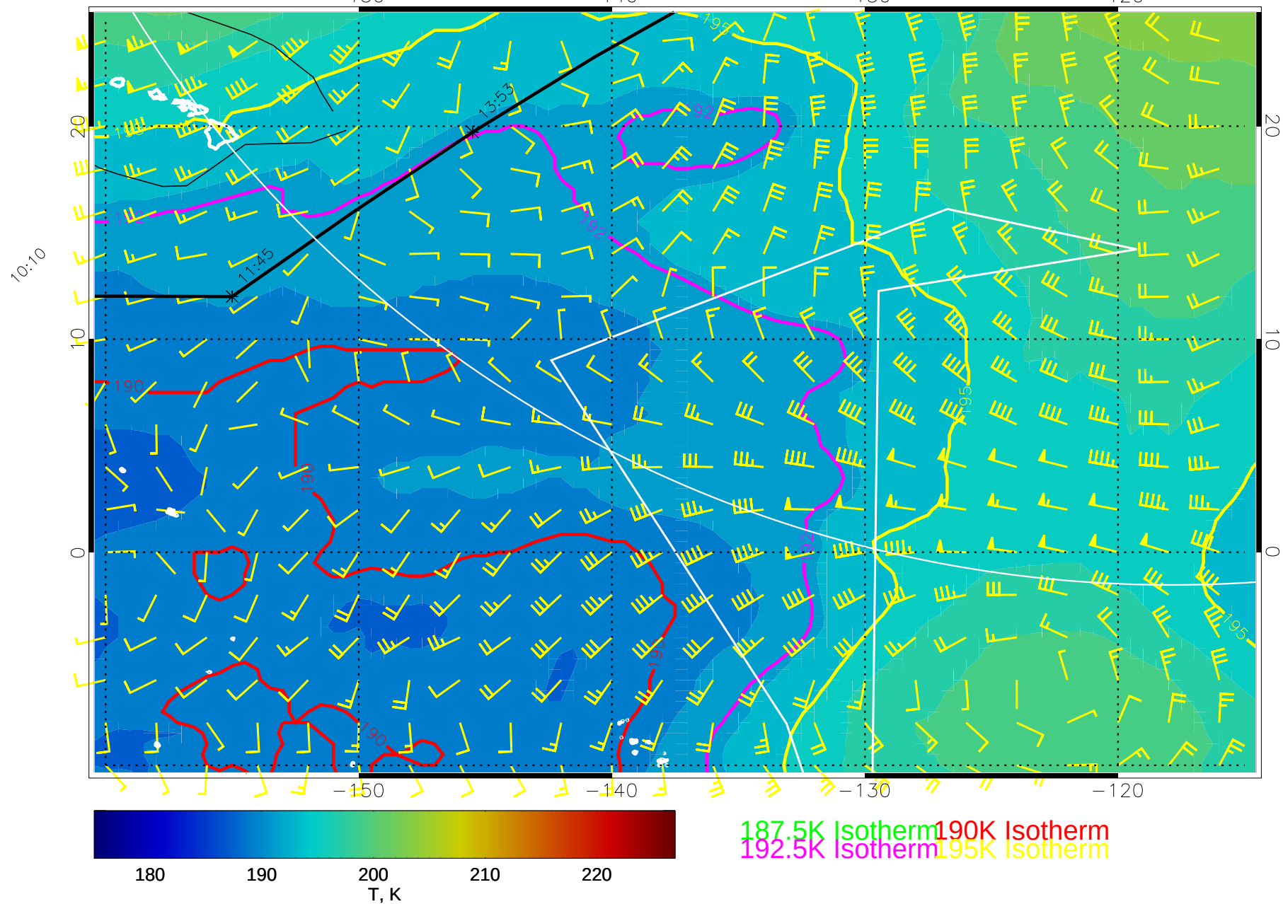
15012400, 84 hour forecast for 100mb T and winds (knots) -- NCEP GFS
