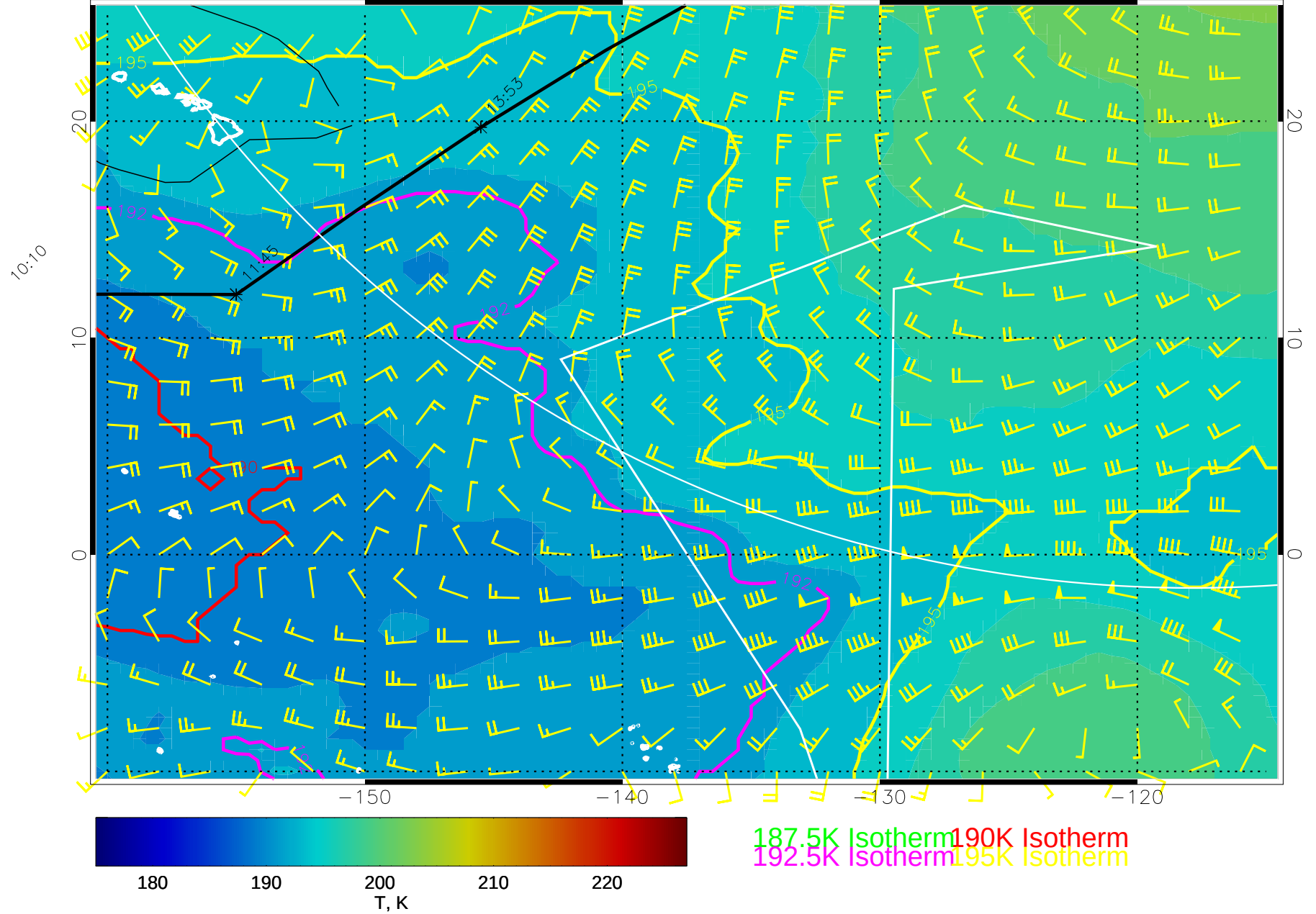
15012218, 54 hour forecast for 100mb T and winds (knots) -- NCEP GFS
