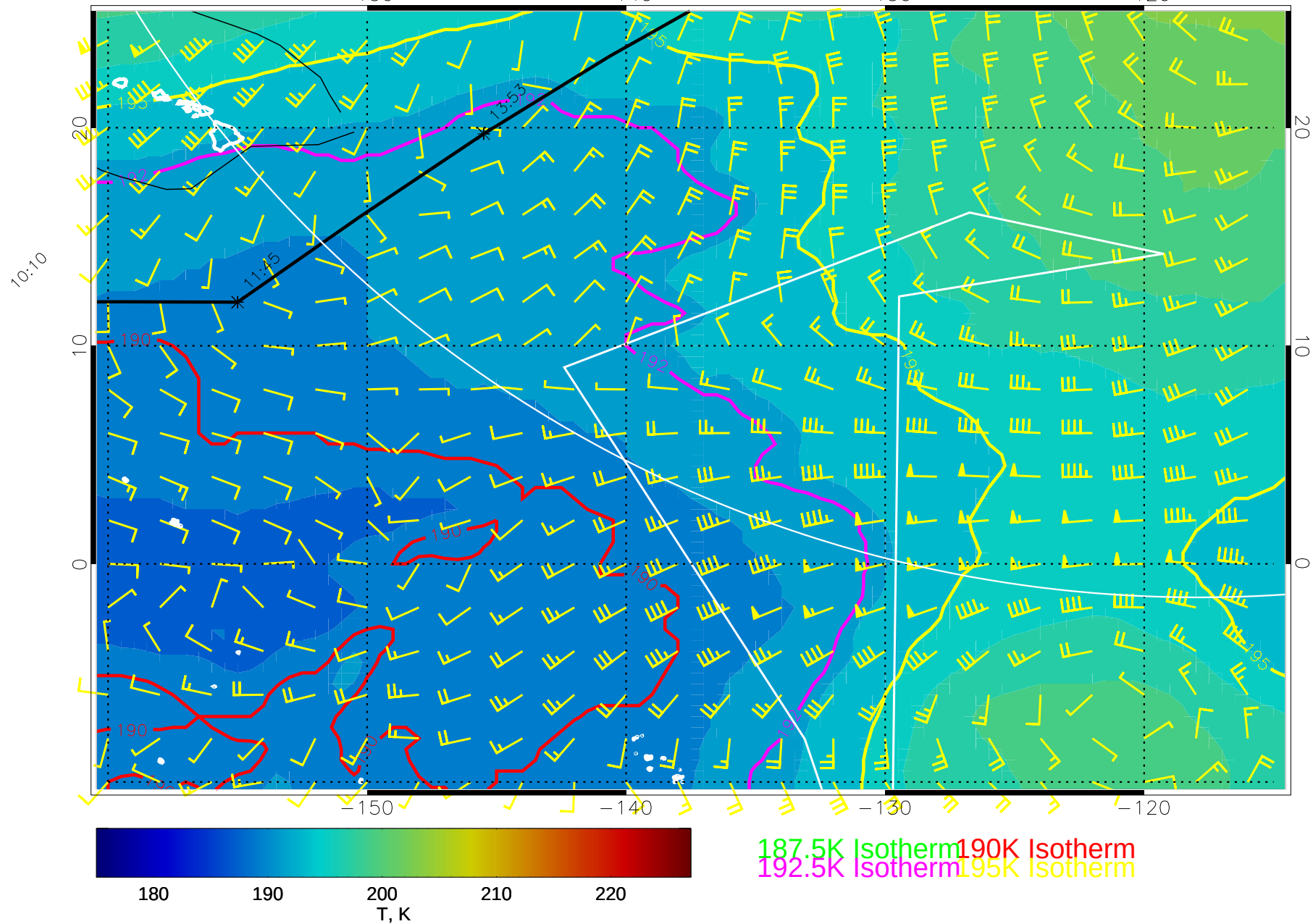
15012312, 72 hour forecast for 100mb T and winds (knots) -- NCEP GFS
