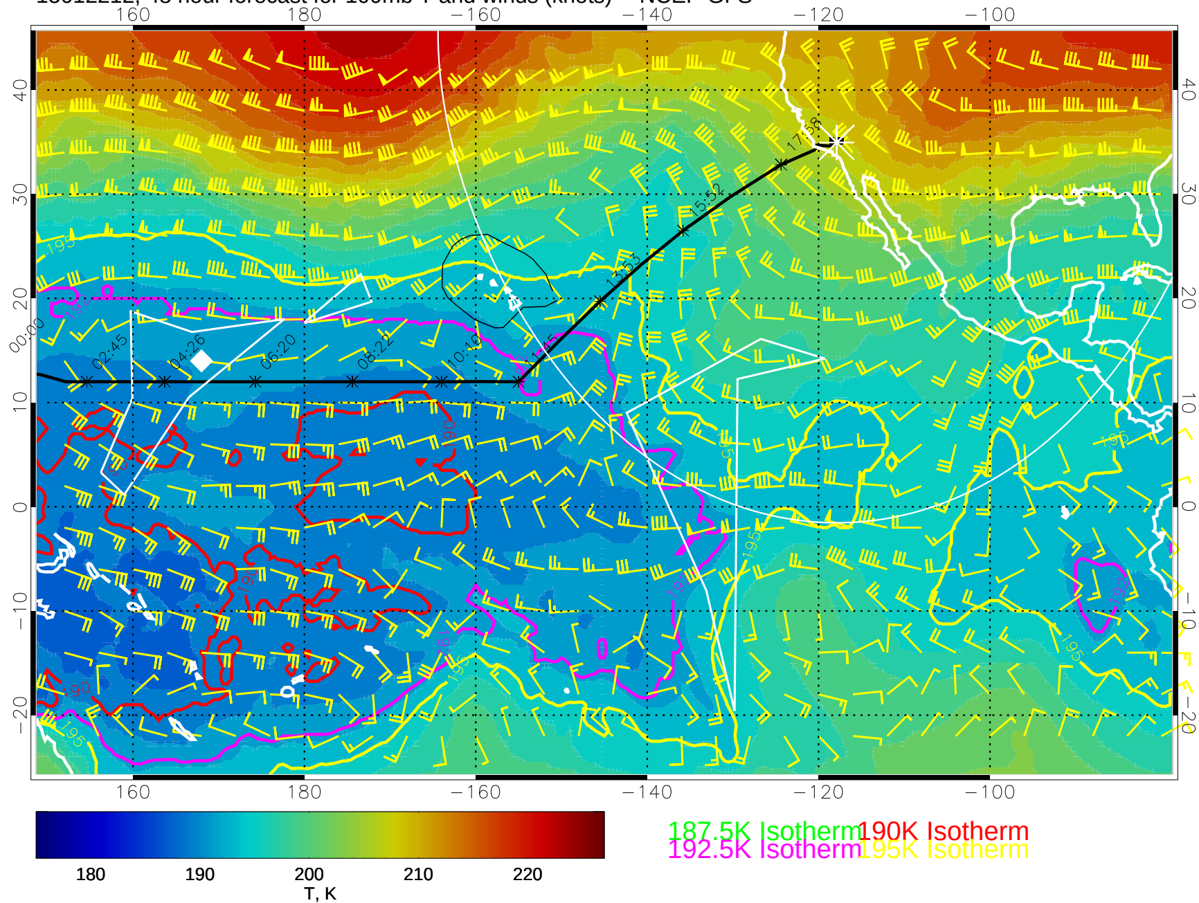
15012212, 48 hour forecast for 100mb T and winds (knots) -- NCEP GFS
