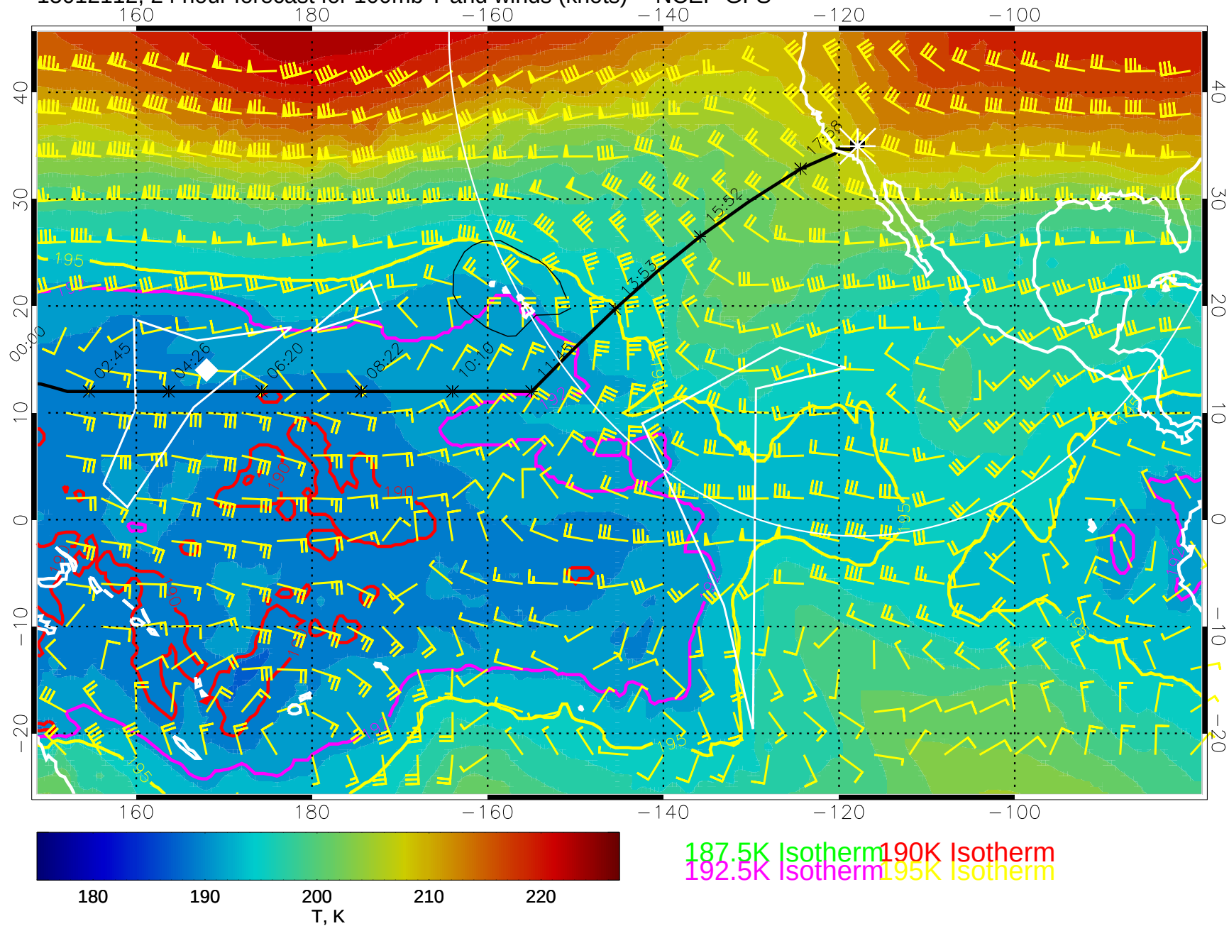
15012112, 24 hour forecast for 100mb T and winds (knots) -- NCEP GFS
