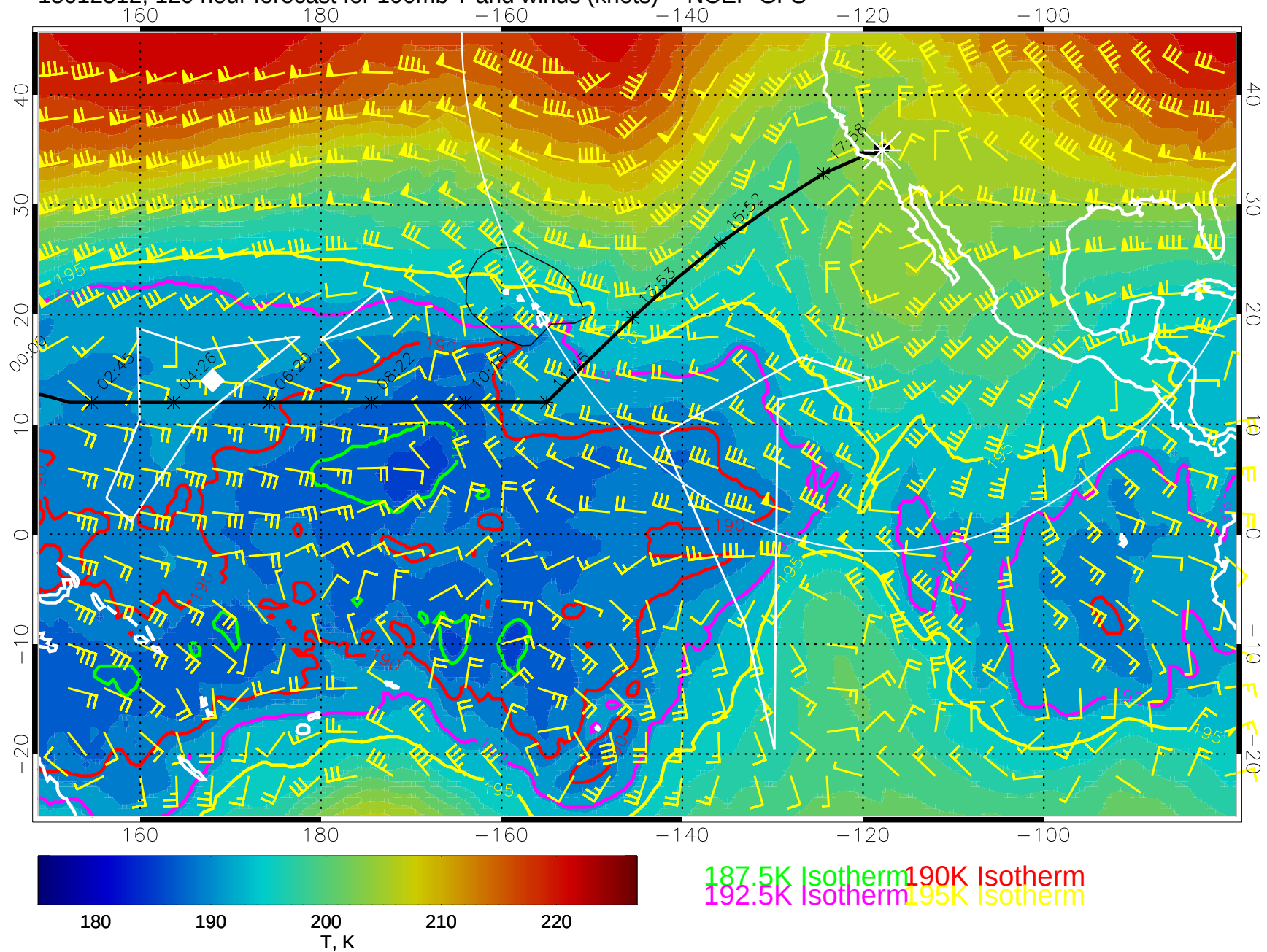
15012512, 120 hour forecast for 100mb T and winds (knots) -- NCEP GFS
