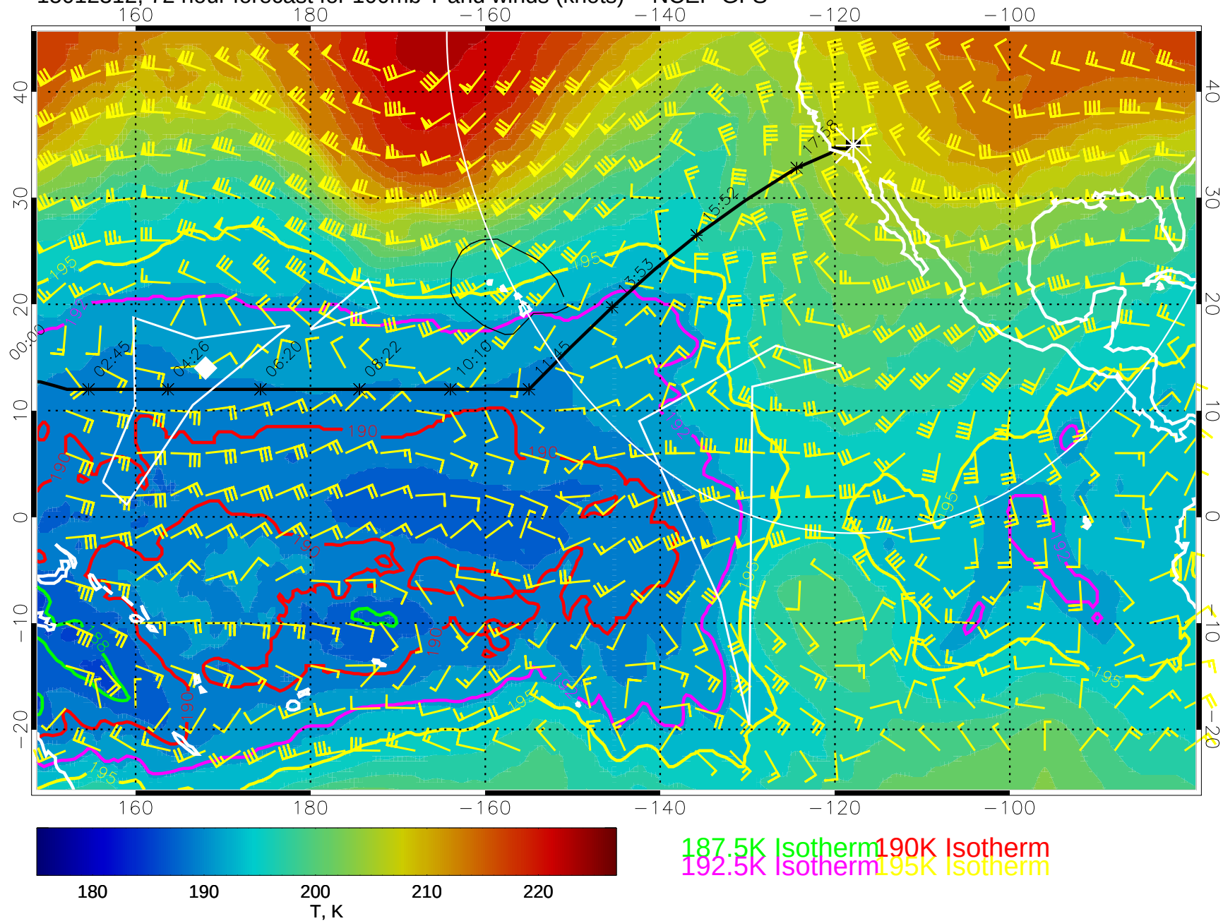
15012312, 72 hour forecast for 100mb T and winds (knots) -- NCEP GFS
