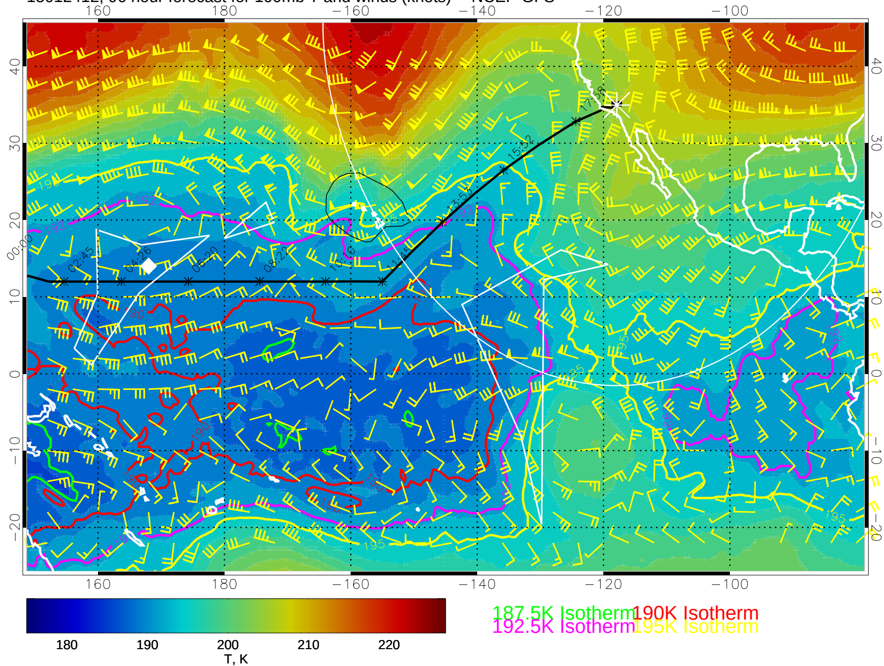
15012412, 96 hour forecast for 100mb T and winds (knots) -- NCEP GFS
