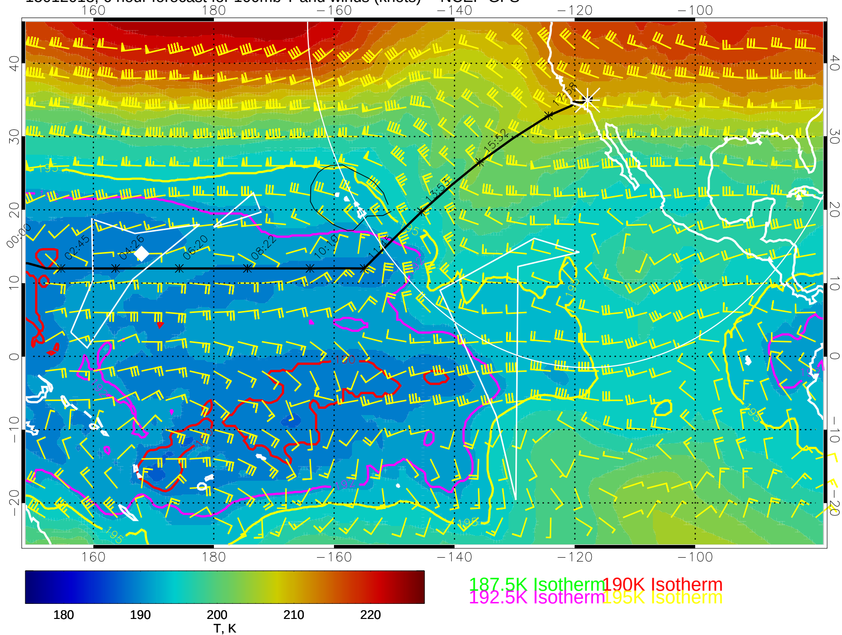
15012018, 6 hour forecast for 100mb T and winds (knots) -- NCEP GFS
