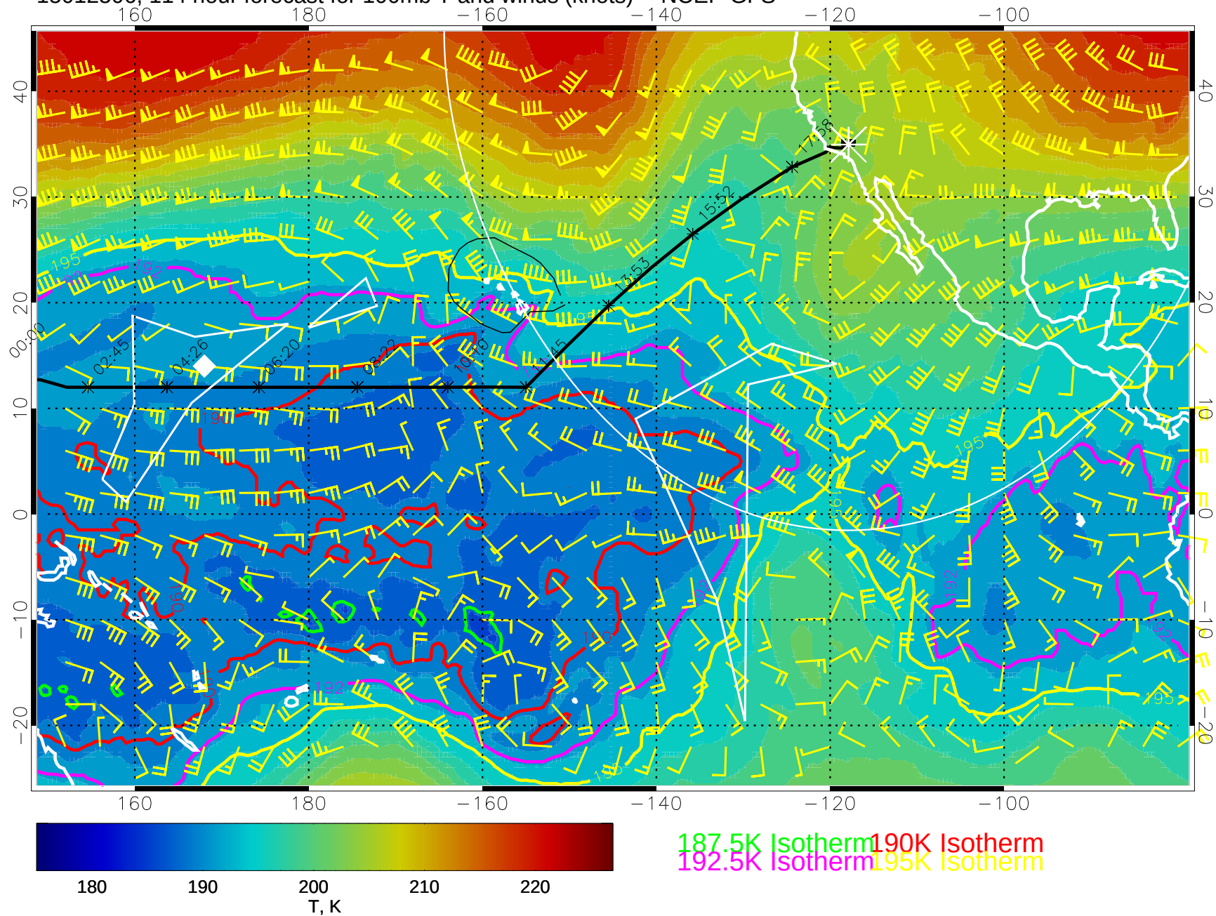
15012506, 114 hour forecast for 100mb T and winds (knots) -- NCEP GFS
