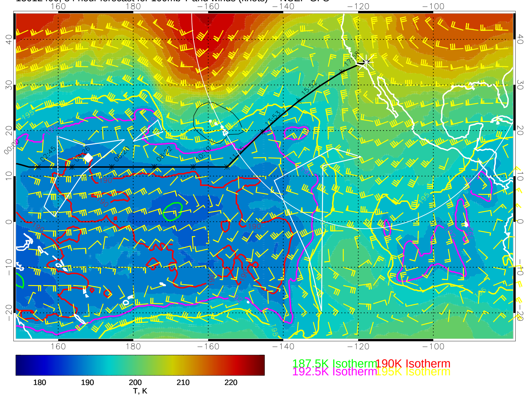
15012400, 84 hour forecast for 100mb T and winds (knots) -- NCEP GFS
