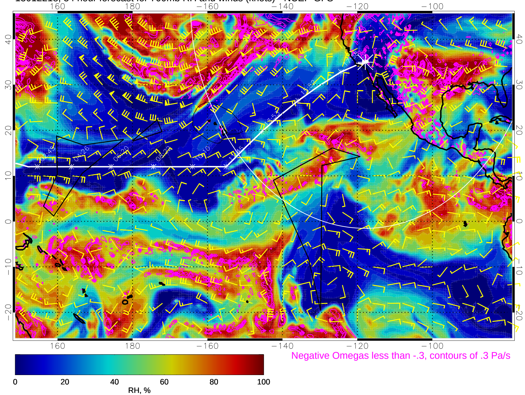
15012218, 54 hour forecast for 700mb RH and winds (knots) - NCEP GFS
