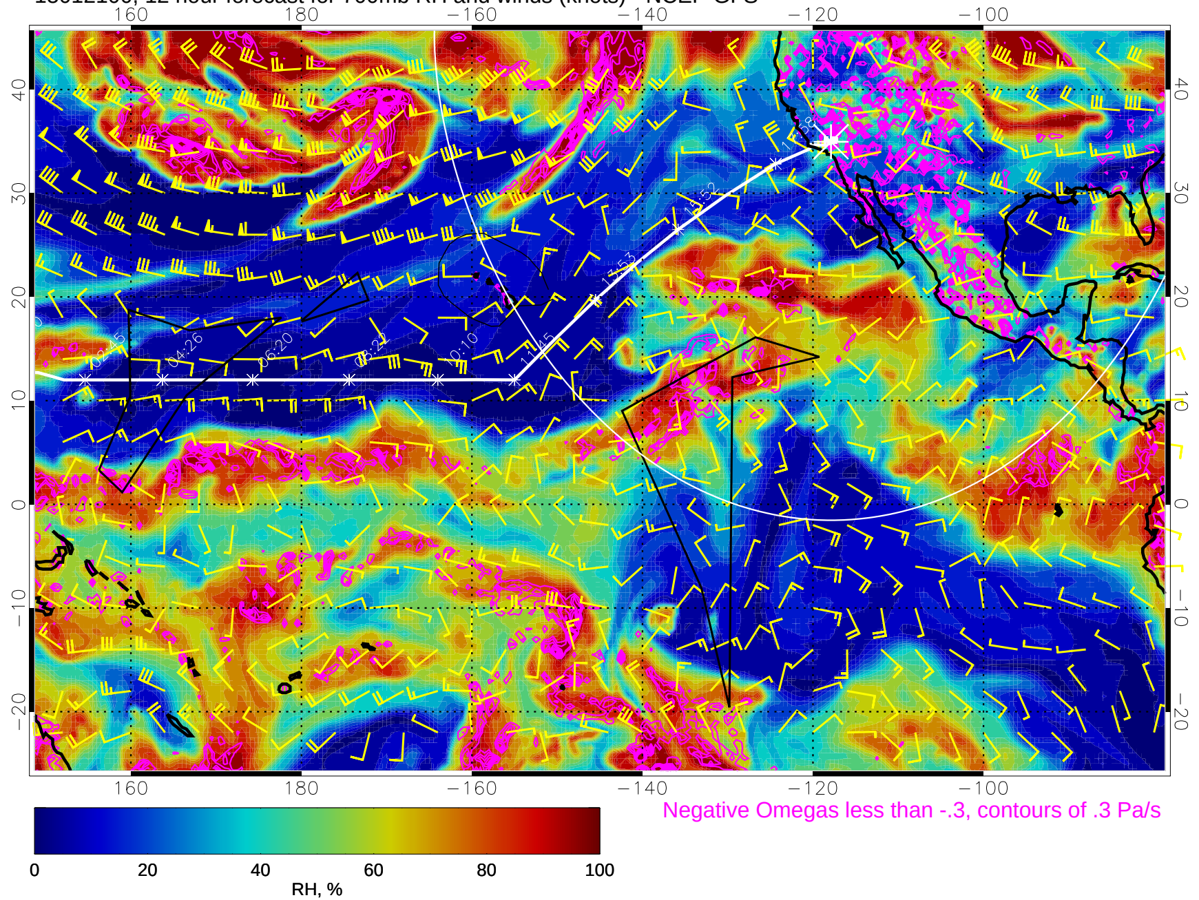
15012100, 12 hour forecast for 700mb RH and winds (knots) - NCEP GFS
