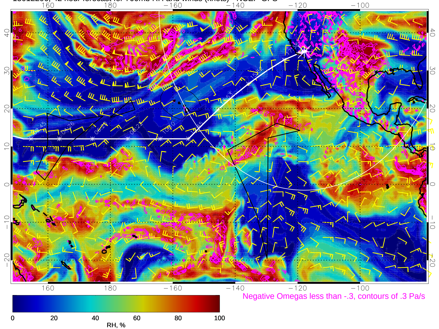
15012206, 42 hour forecast for 700mb RH and winds (knots) - NCEP GFS
