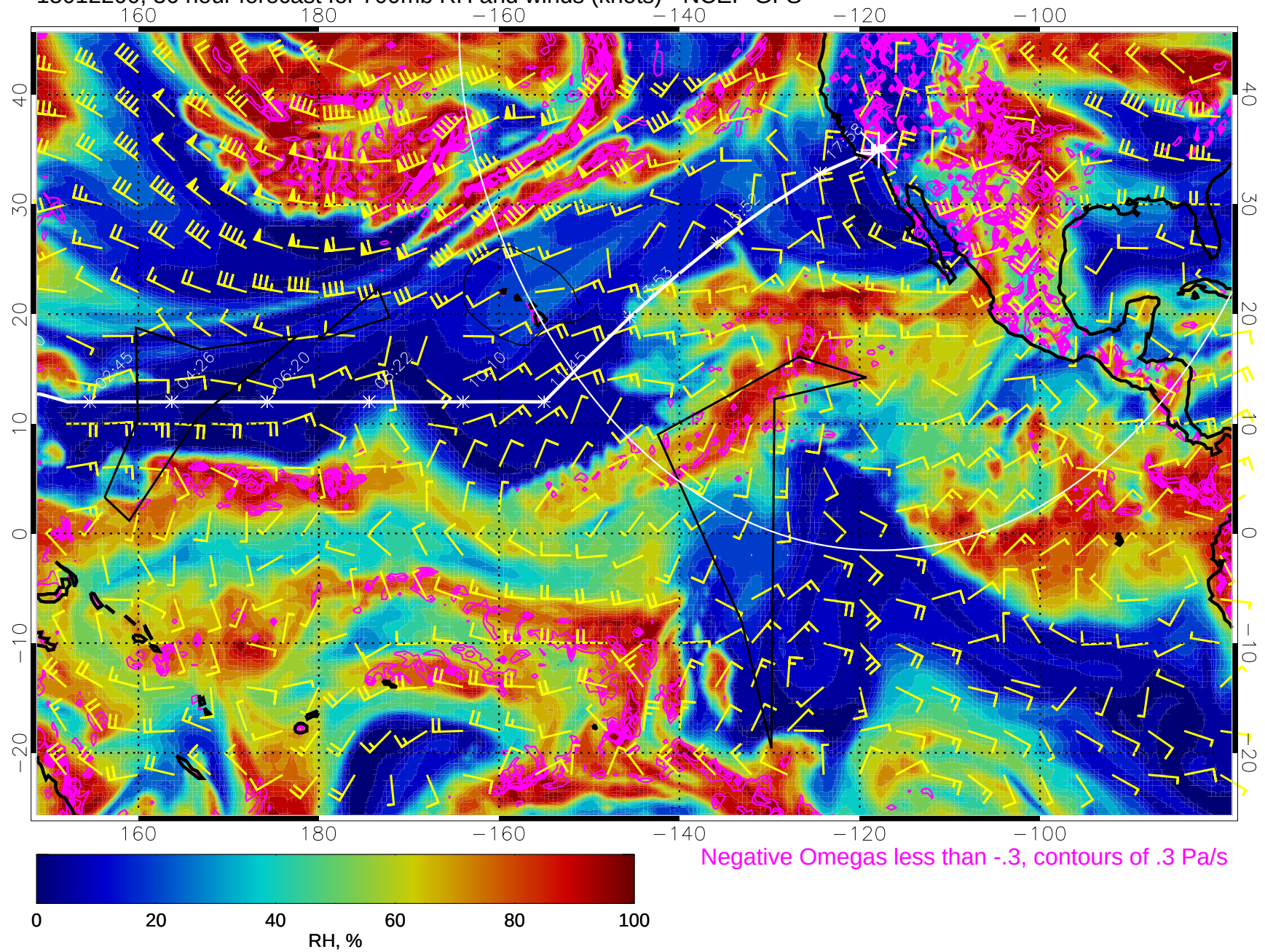
15012200, 36 hour forecast for 700mb RH and winds (knots) - NCEP GFS
