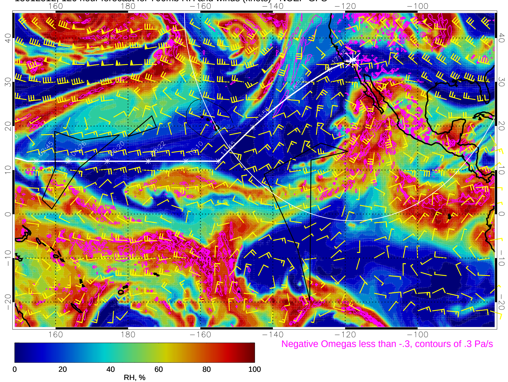
15012512, 120 hour forecast for 700mb RH and winds (knots) - NCEP GFS
