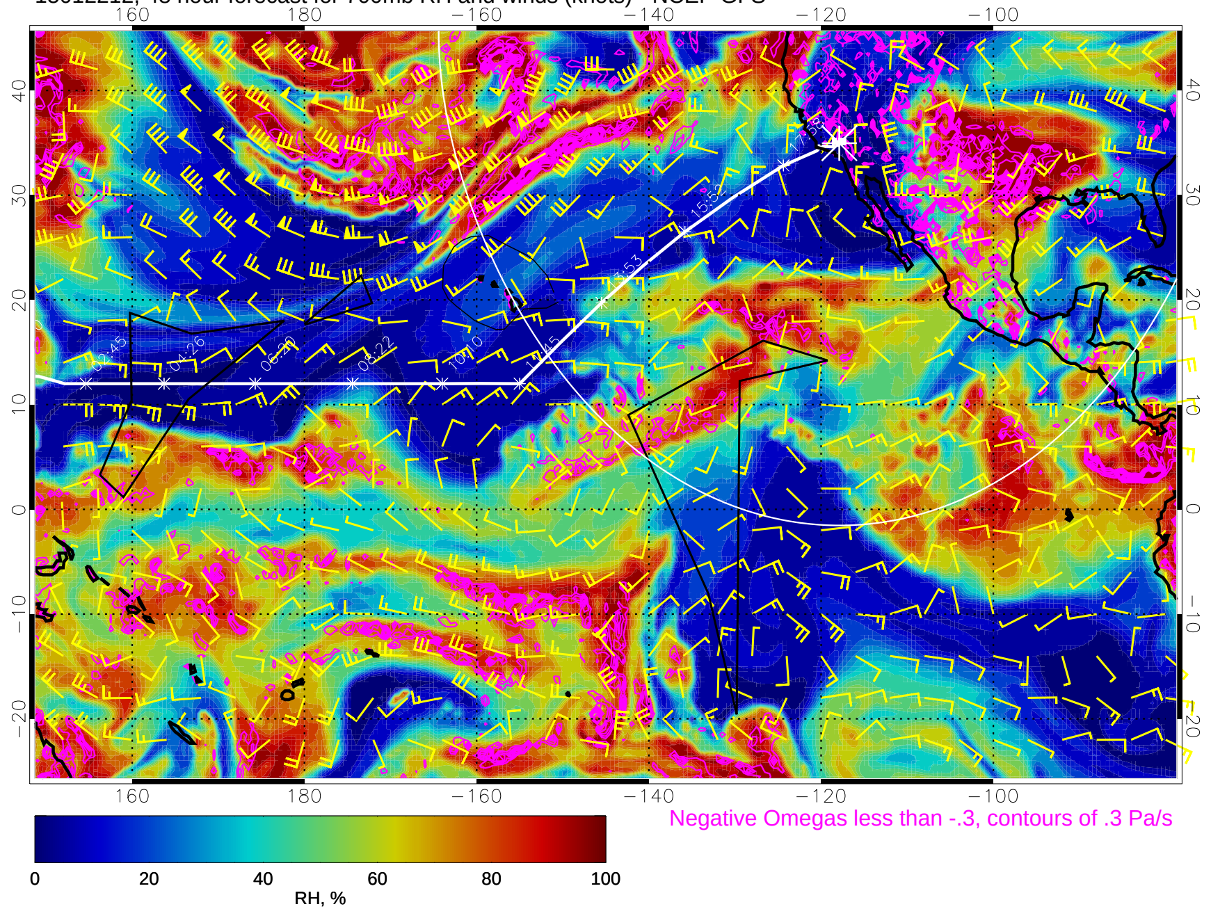
15012212, 48 hour forecast for 700mb RH and winds (knots) - NCEP GFS
