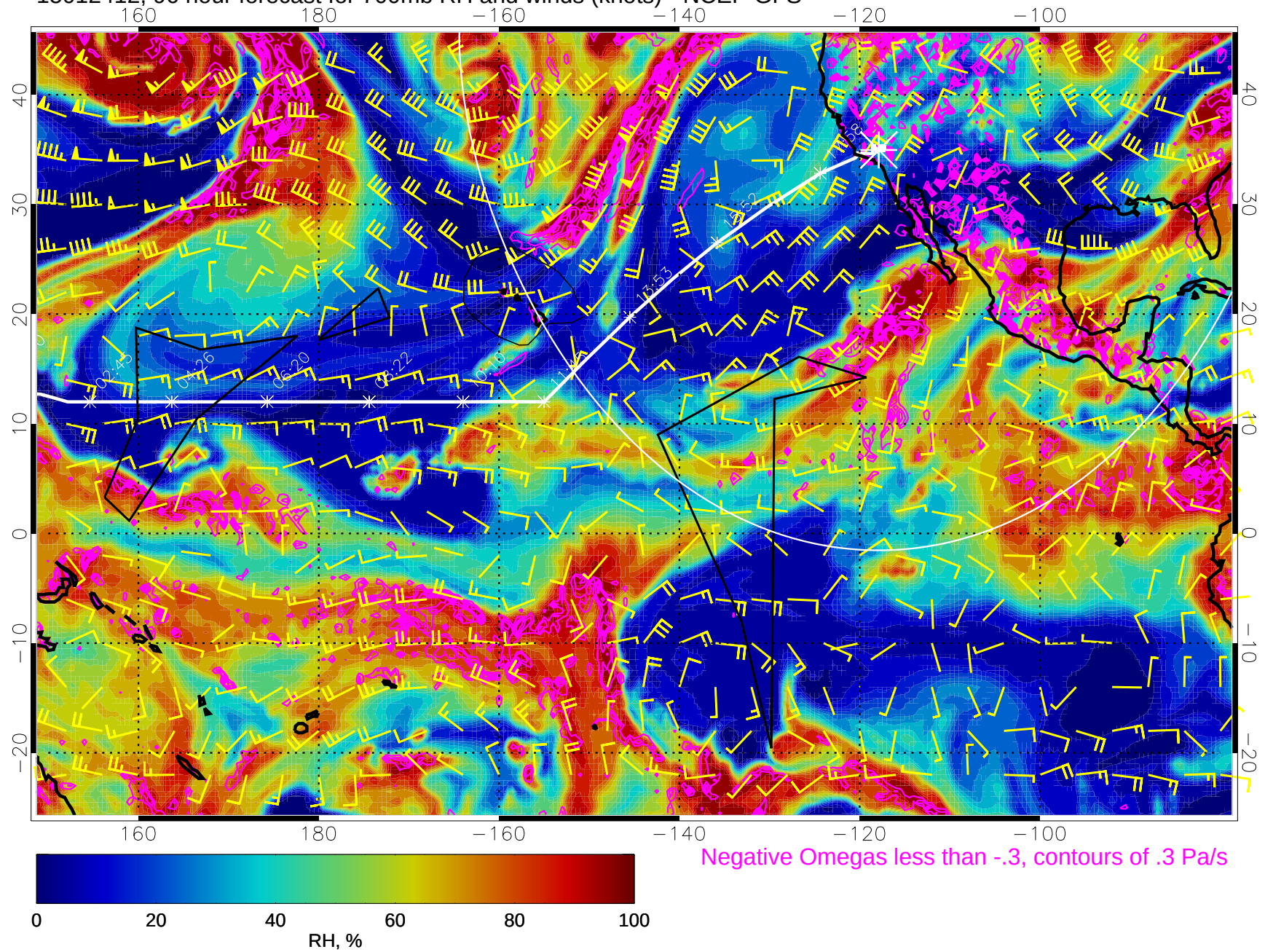
15012412, 96 hour forecast for 700mb RH and winds (knots) - NCEP GFS
