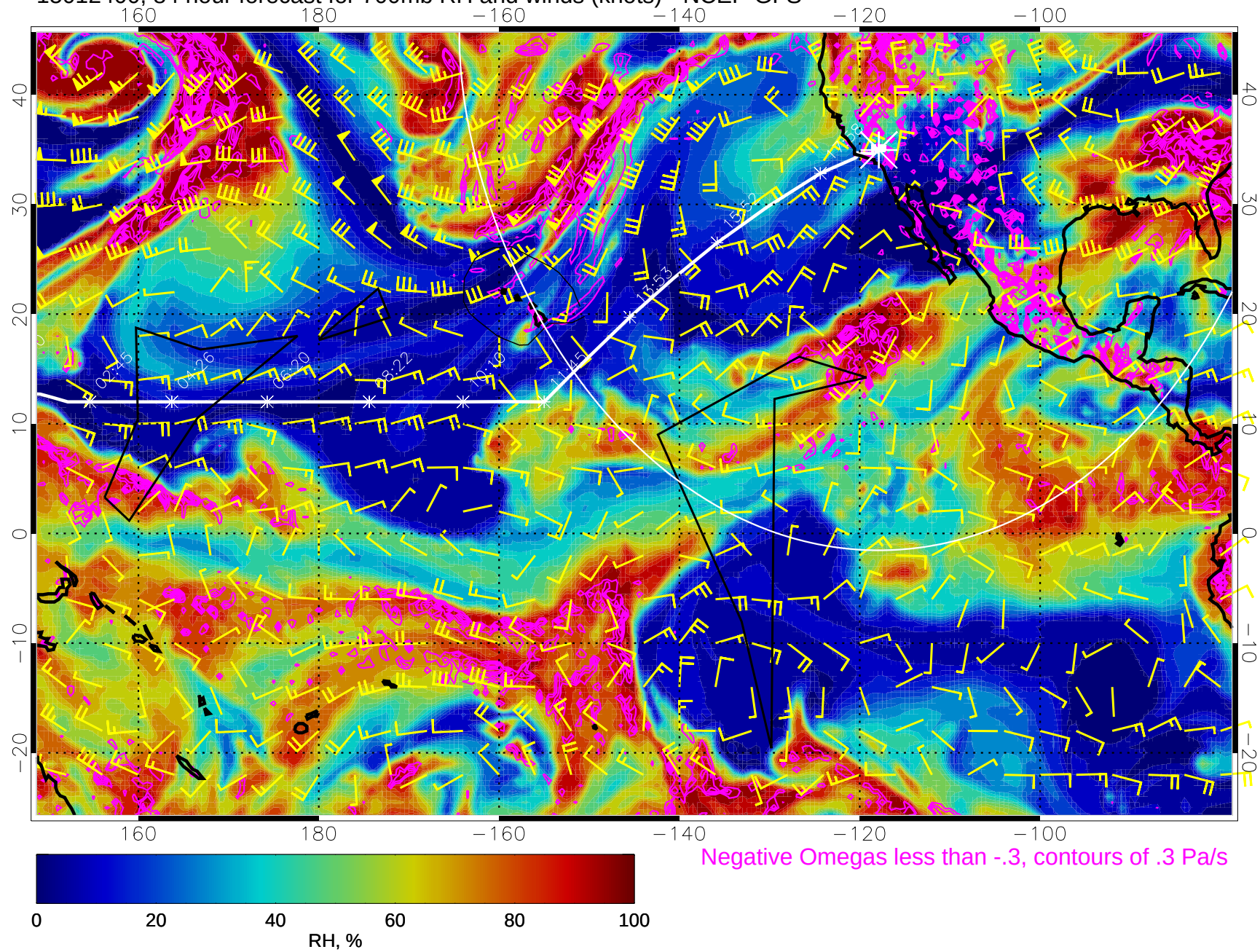
15012400, 84 hour forecast for 700mb RH and winds (knots) - NCEP GFS
