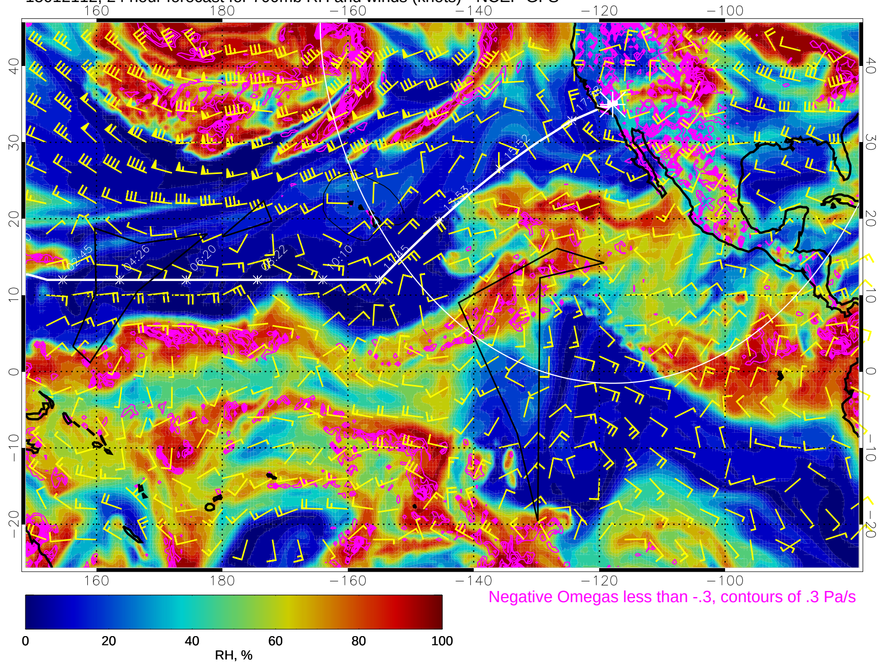
15012112, 24 hour forecast for 700mb RH and winds (knots) - NCEP GFS
