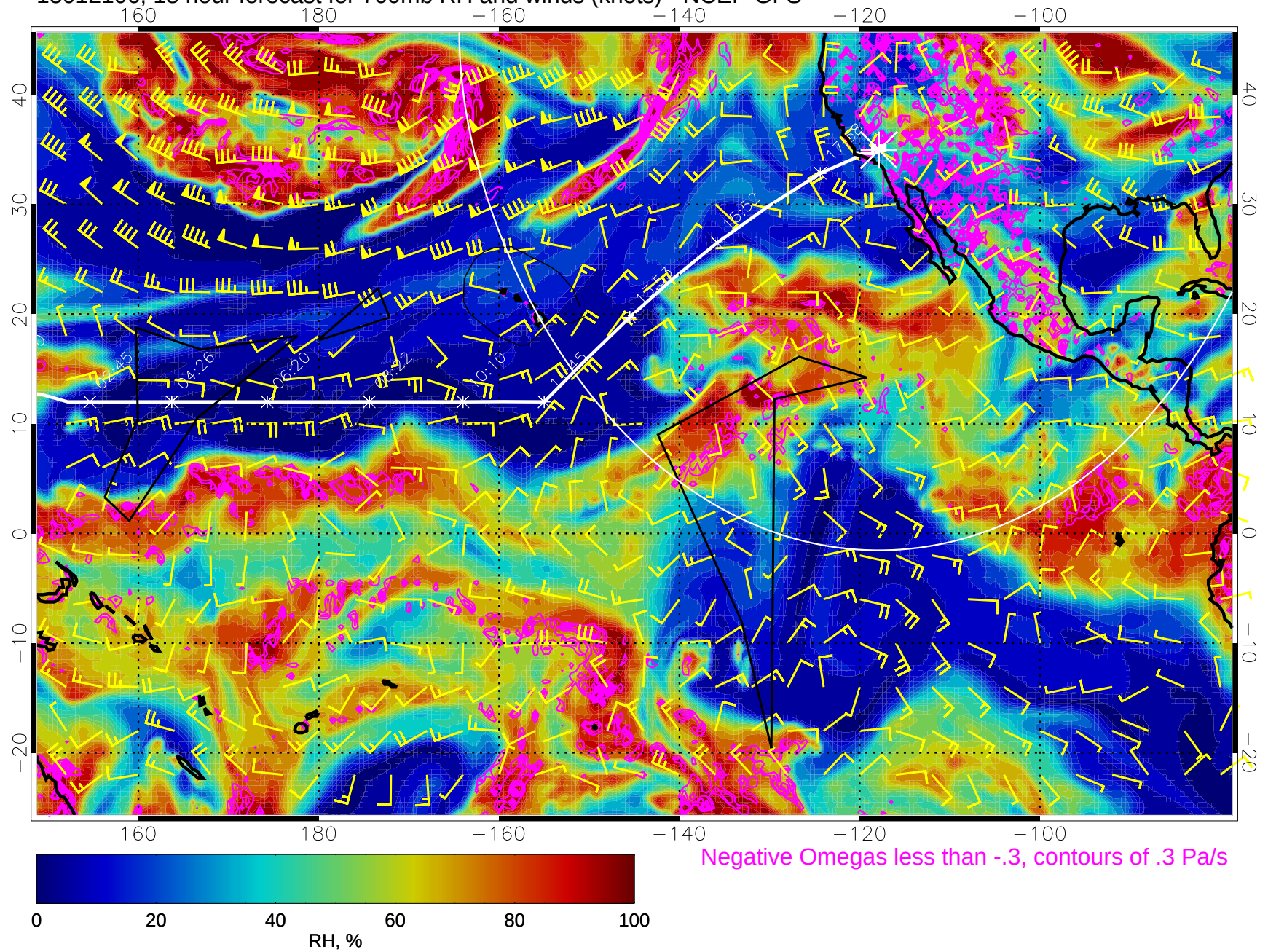
15012106, 18 hour forecast for 700mb RH and winds (knots) - NCEP GFS
