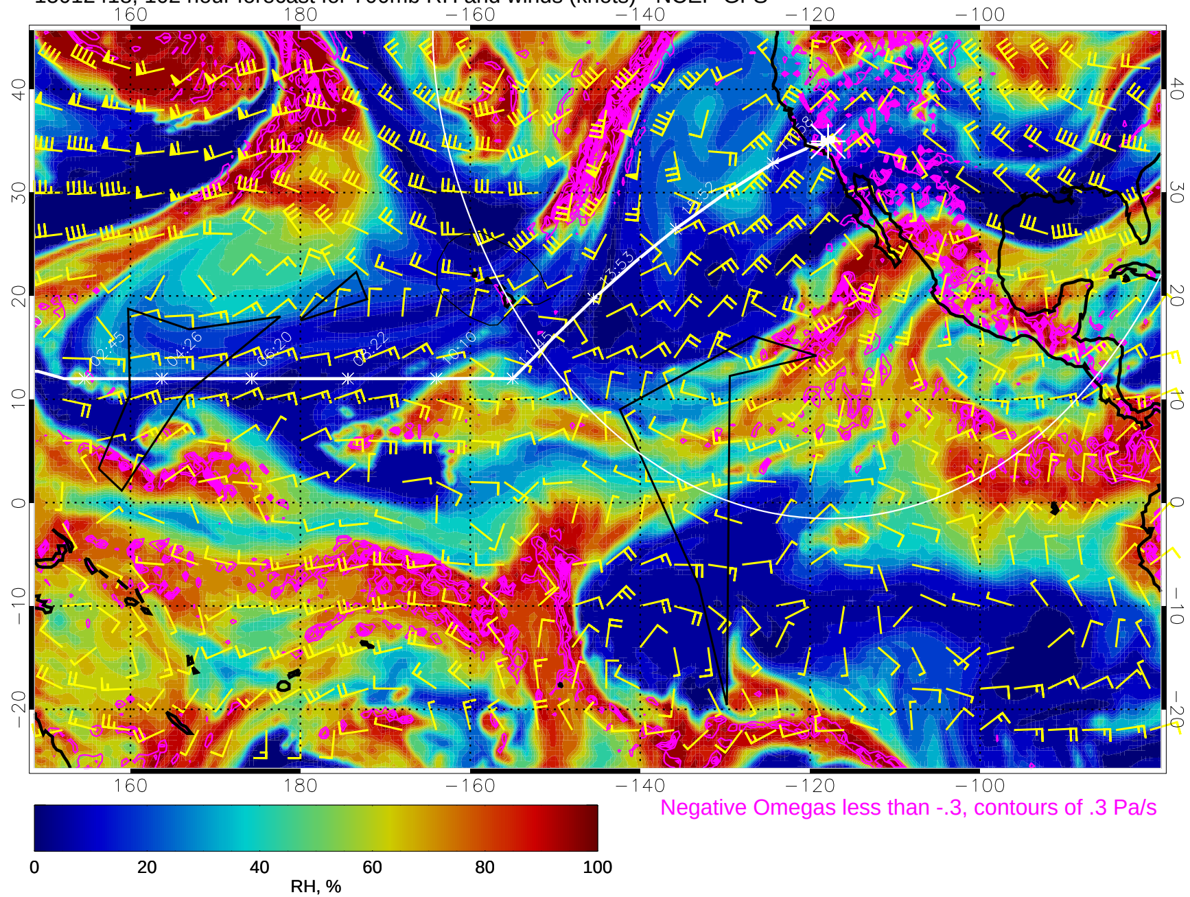
15012418, 102 hour forecast for 700mb RH and winds (knots) - NCEP GFS
