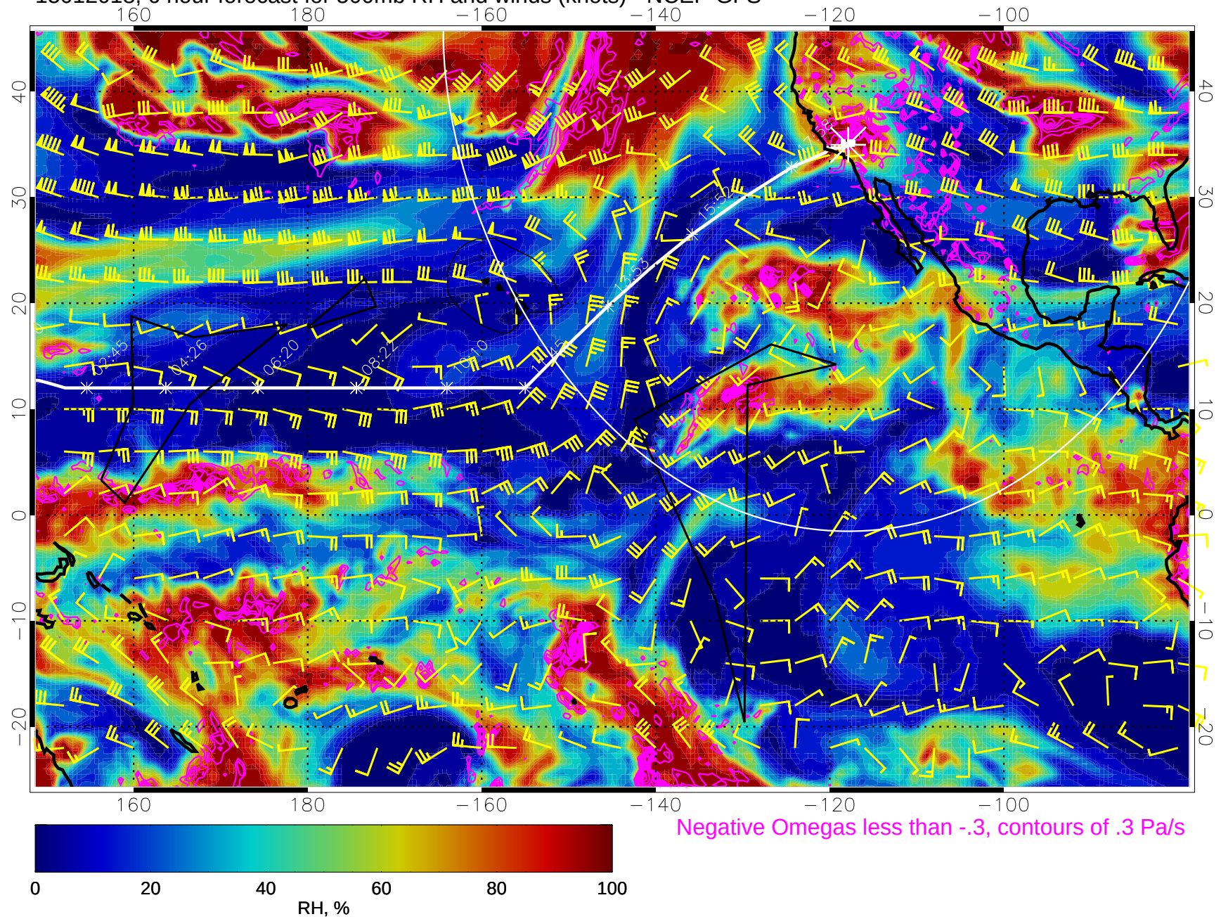
15012018, 6 hour forecast for 500mb RH and winds (knots) - NCEP GFS
