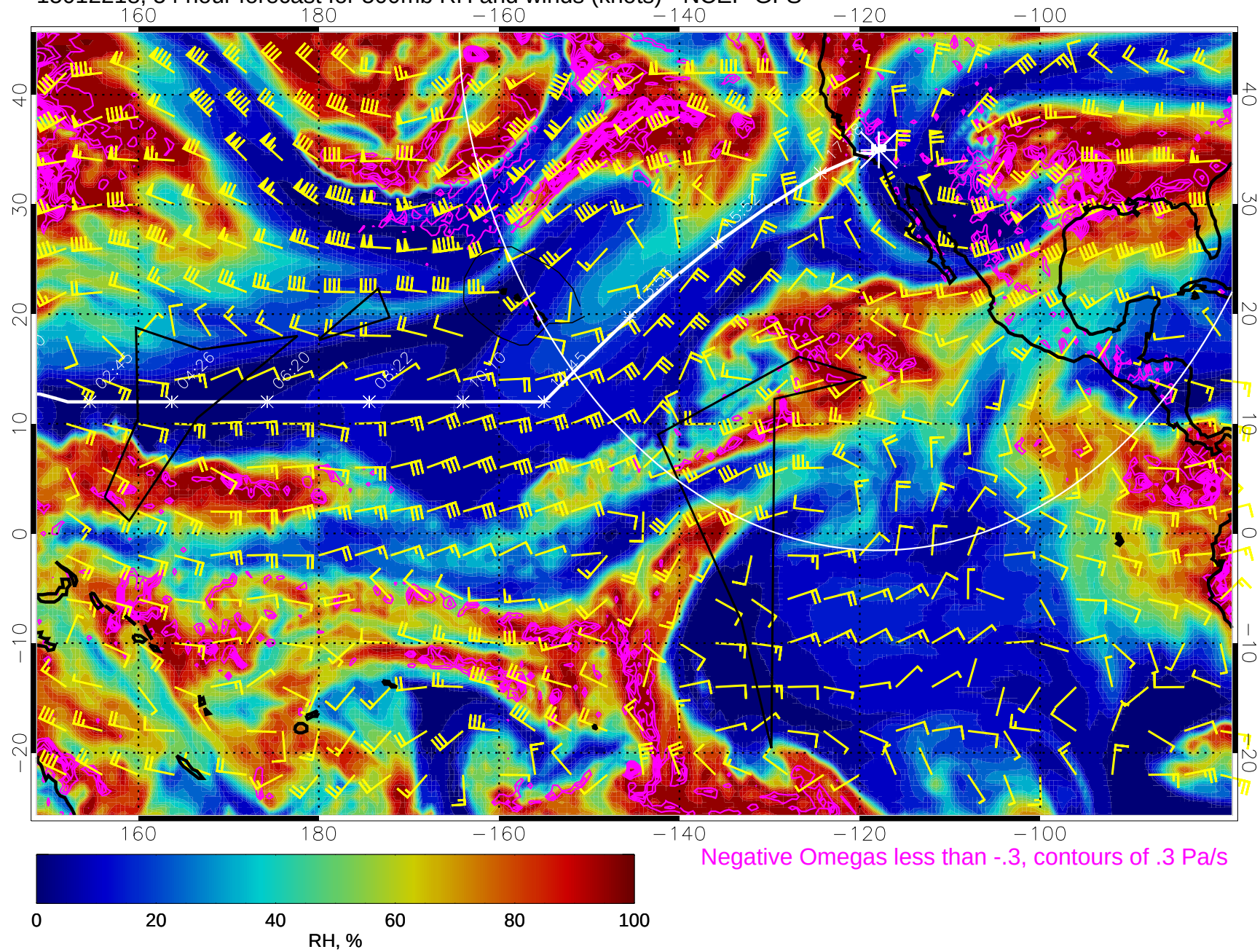
15012218, 54 hour forecast for 500mb RH and winds (knots) - NCEP GFS
