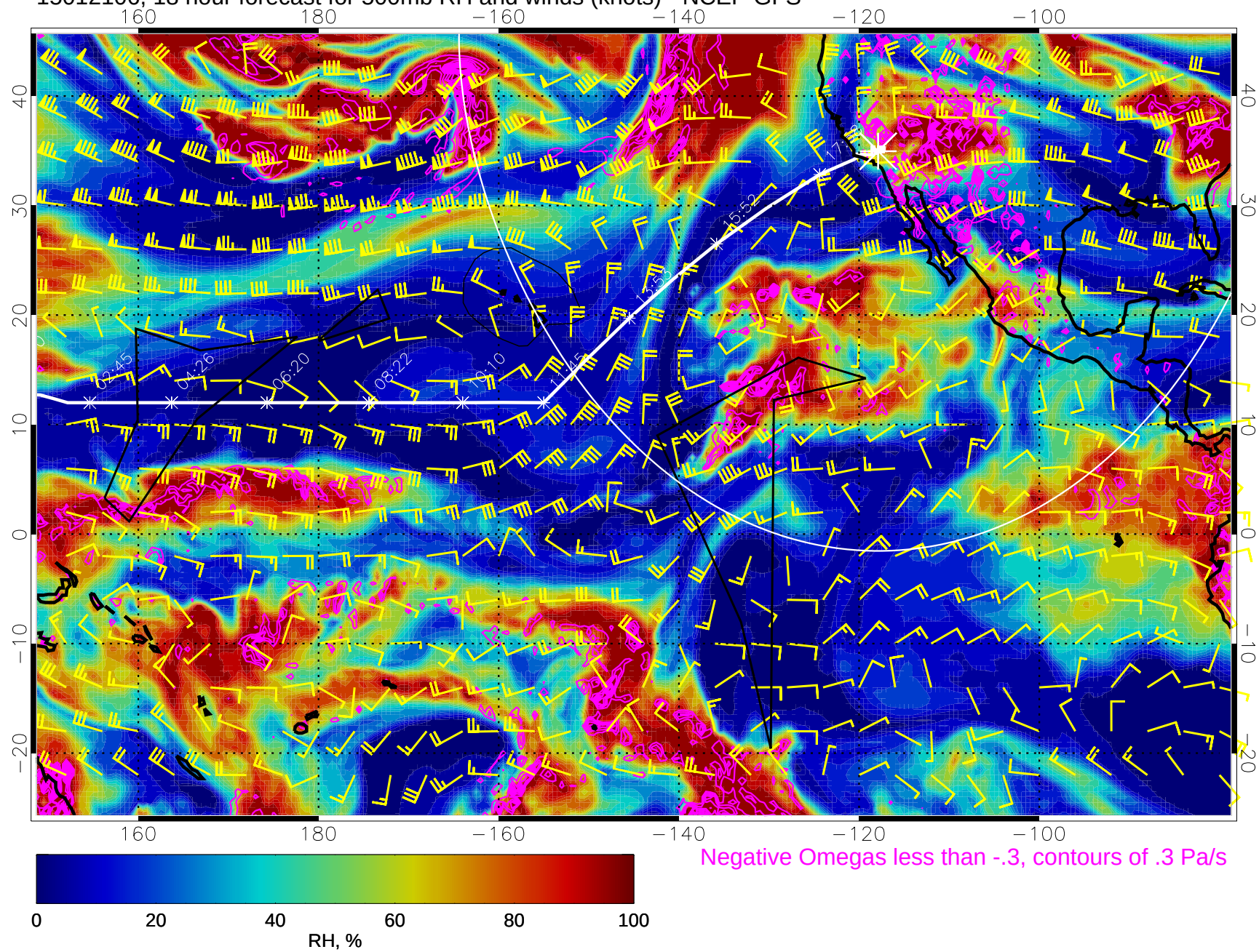
15012106, 18 hour forecast for 500mb RH and winds (knots) - NCEP GFS
