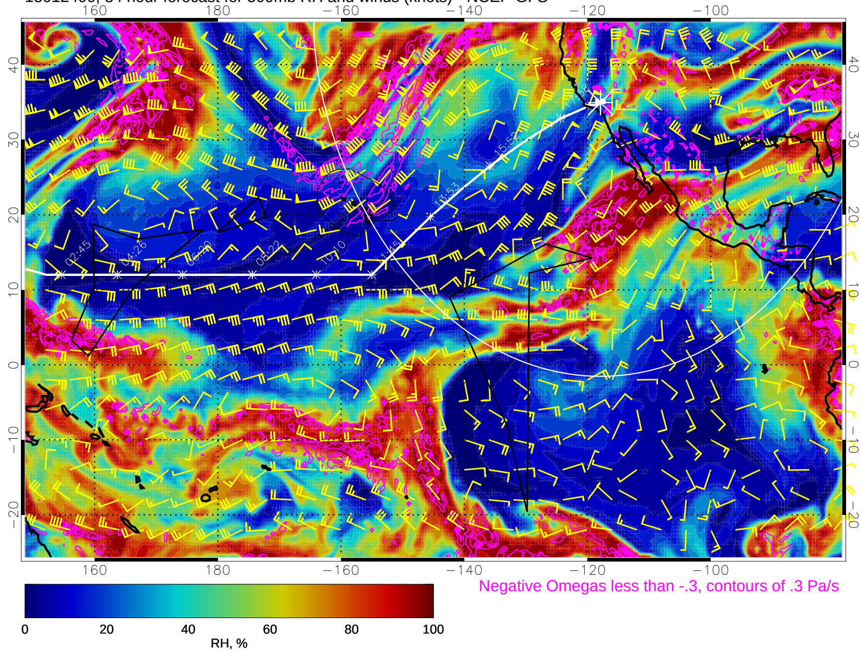
15012400, 84 hour forecast for 500mb RH and winds (knots) - NCEP GFS
