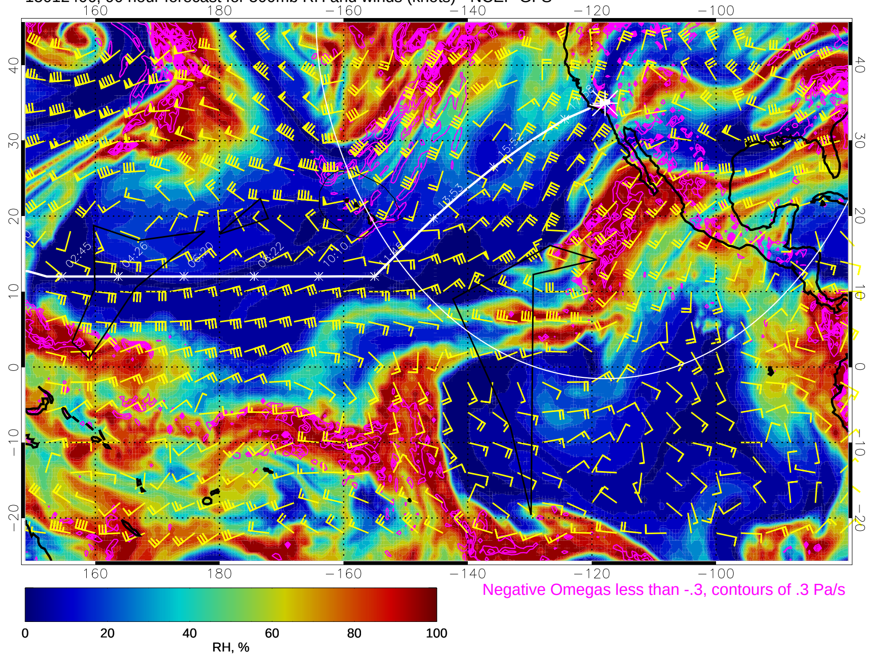
15012406, 90 hour forecast for 500mb RH and winds (knots) - NCEP GFS
