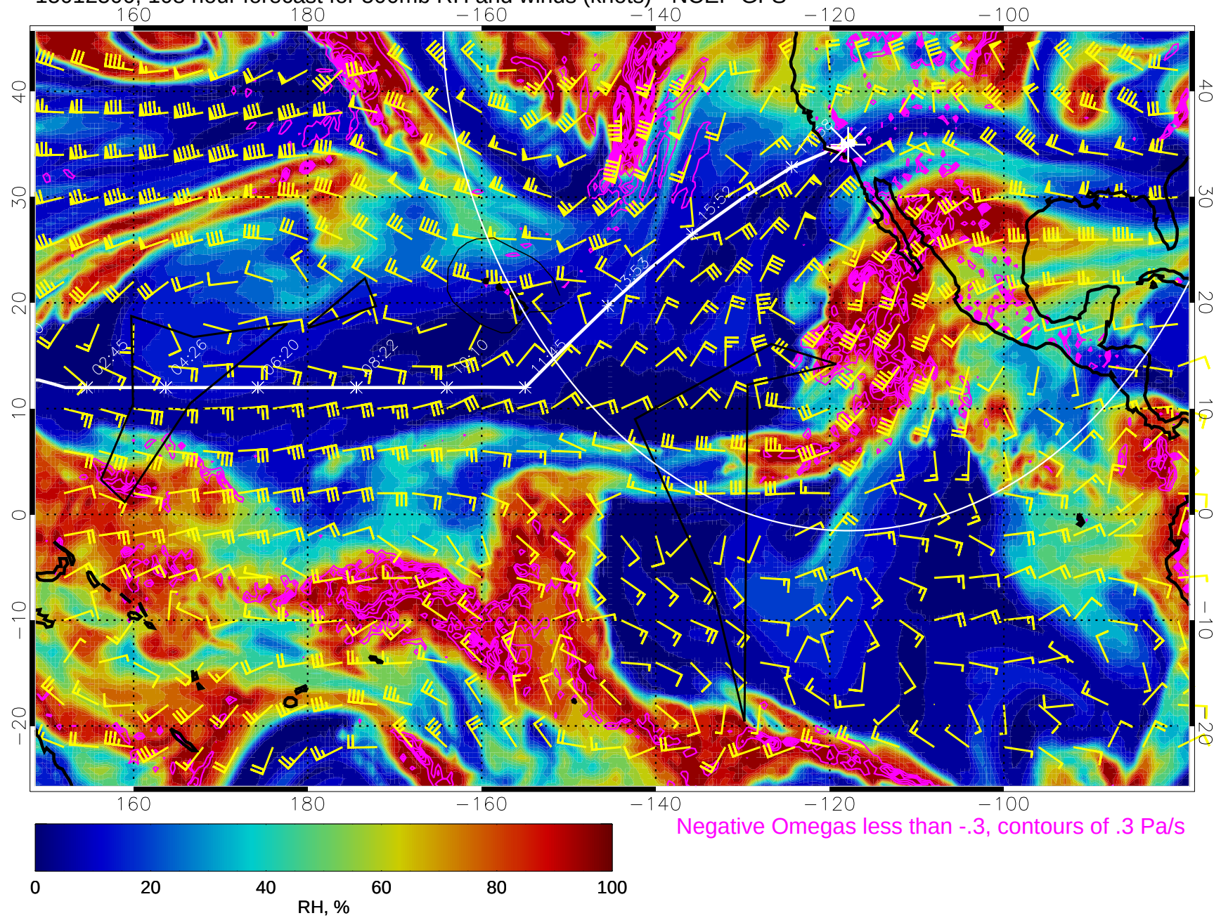
15012500, 108 hour forecast for 500mb RH and winds (knots) - NCEP GFS
