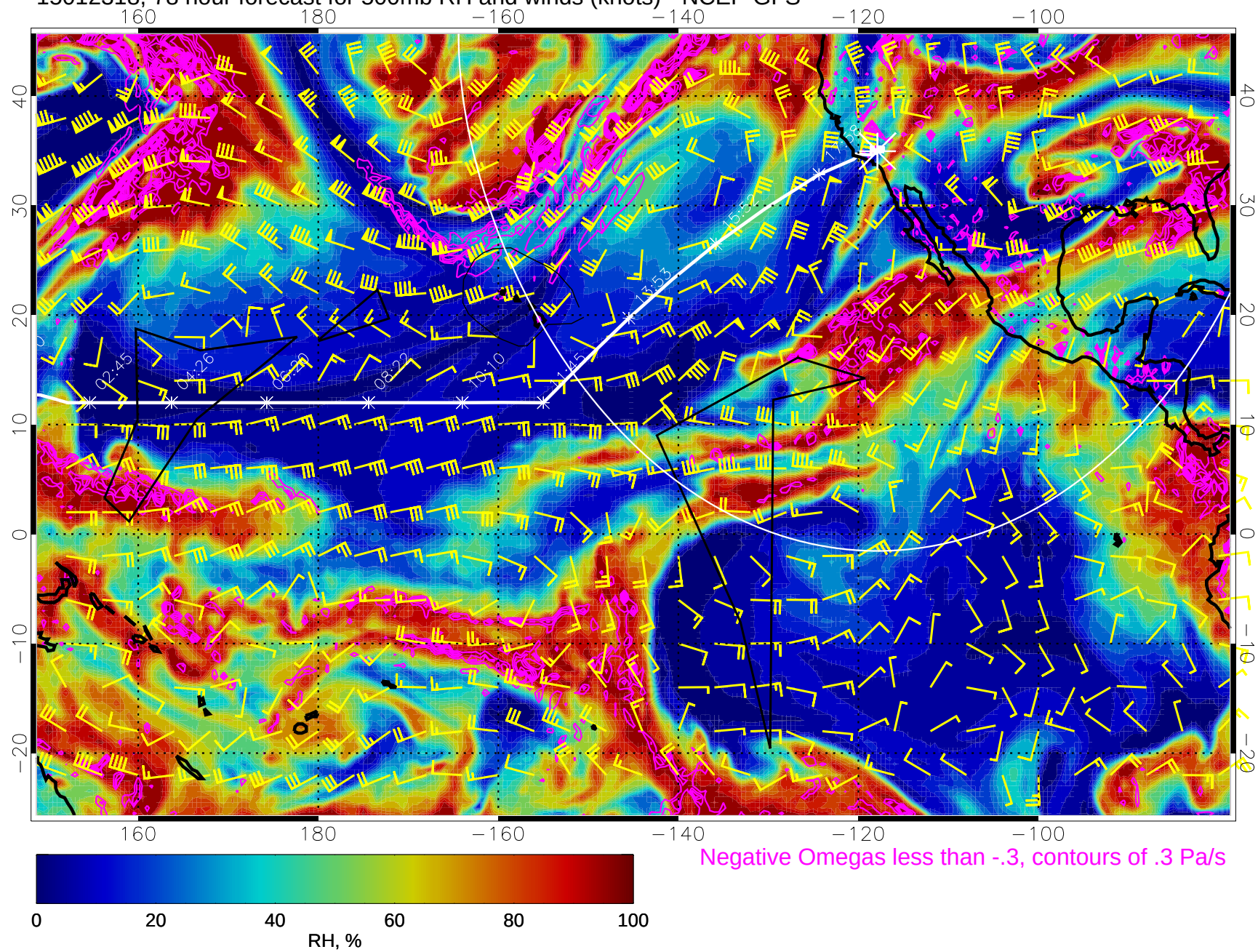
15012318, 78 hour forecast for 500mb RH and winds (knots) - NCEP GFS
