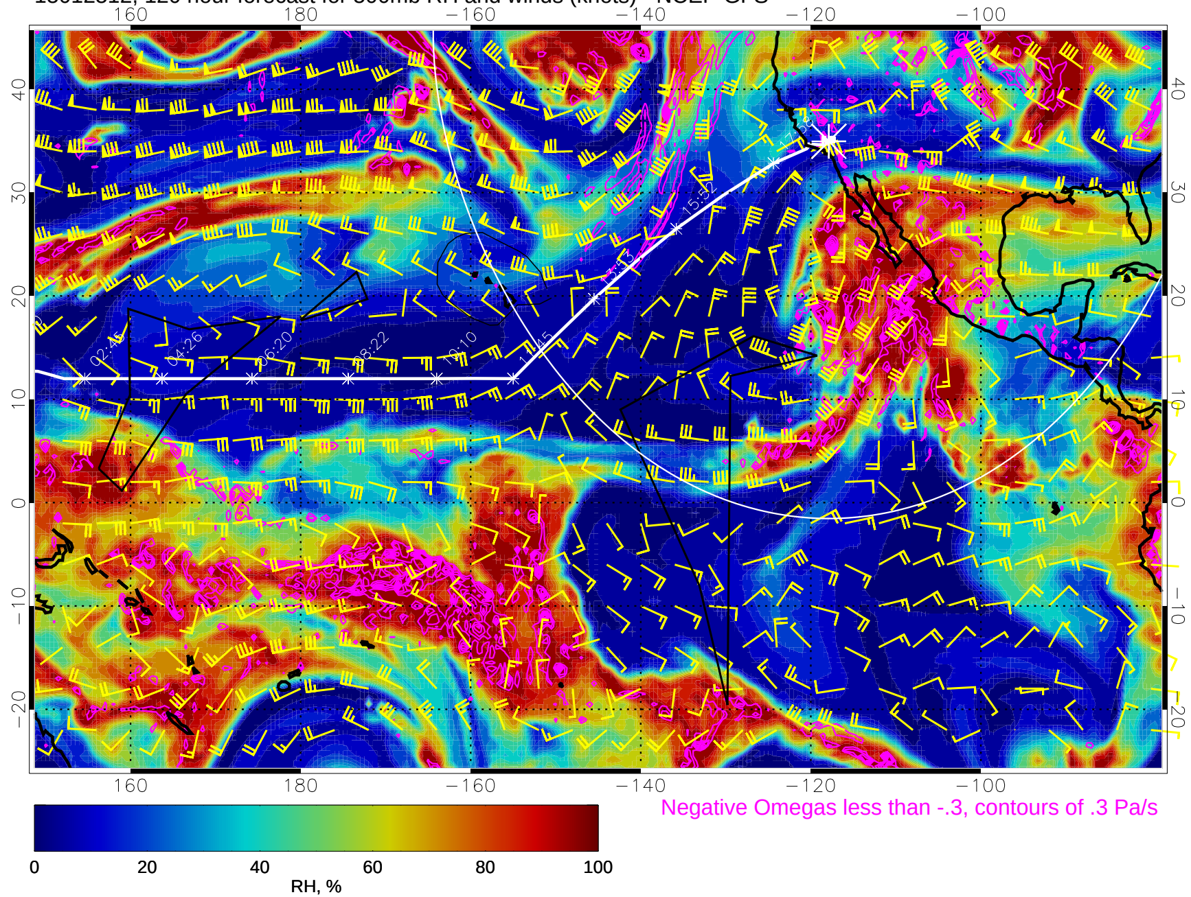
15012512, 120 hour forecast for 500mb RH and winds (knots) - NCEP GFS
