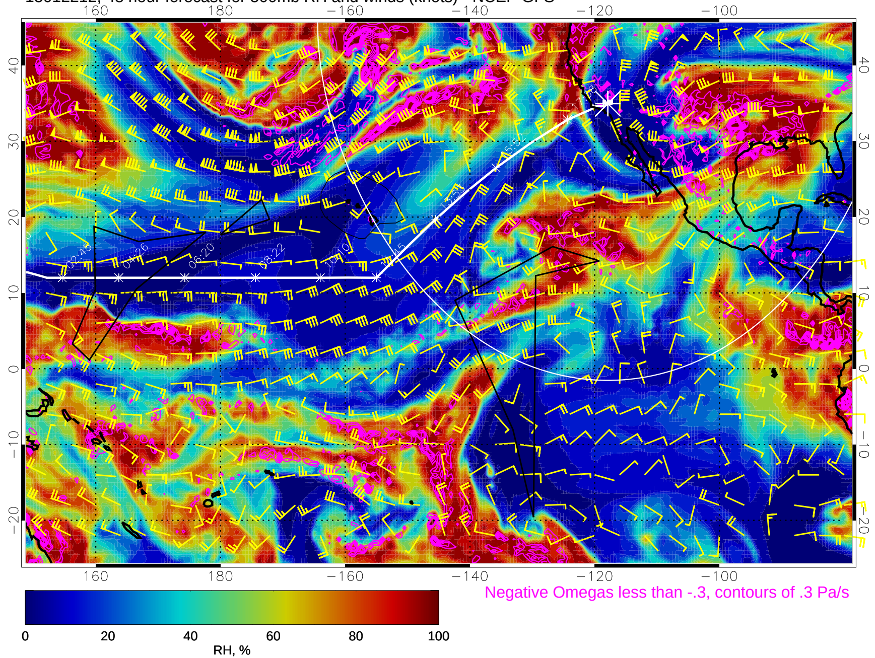
15012212, 48 hour forecast for 500mb RH and winds (knots) - NCEP GFS
