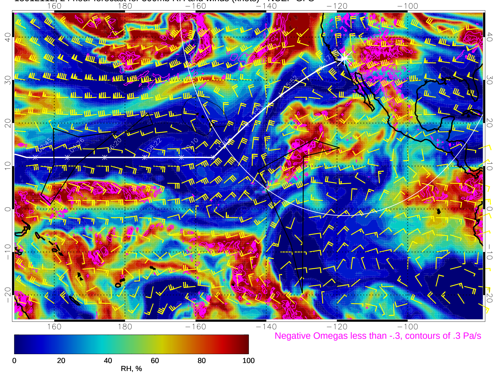
15012112, 24 hour forecast for 500mb RH and winds (knots) - NCEP GFS
