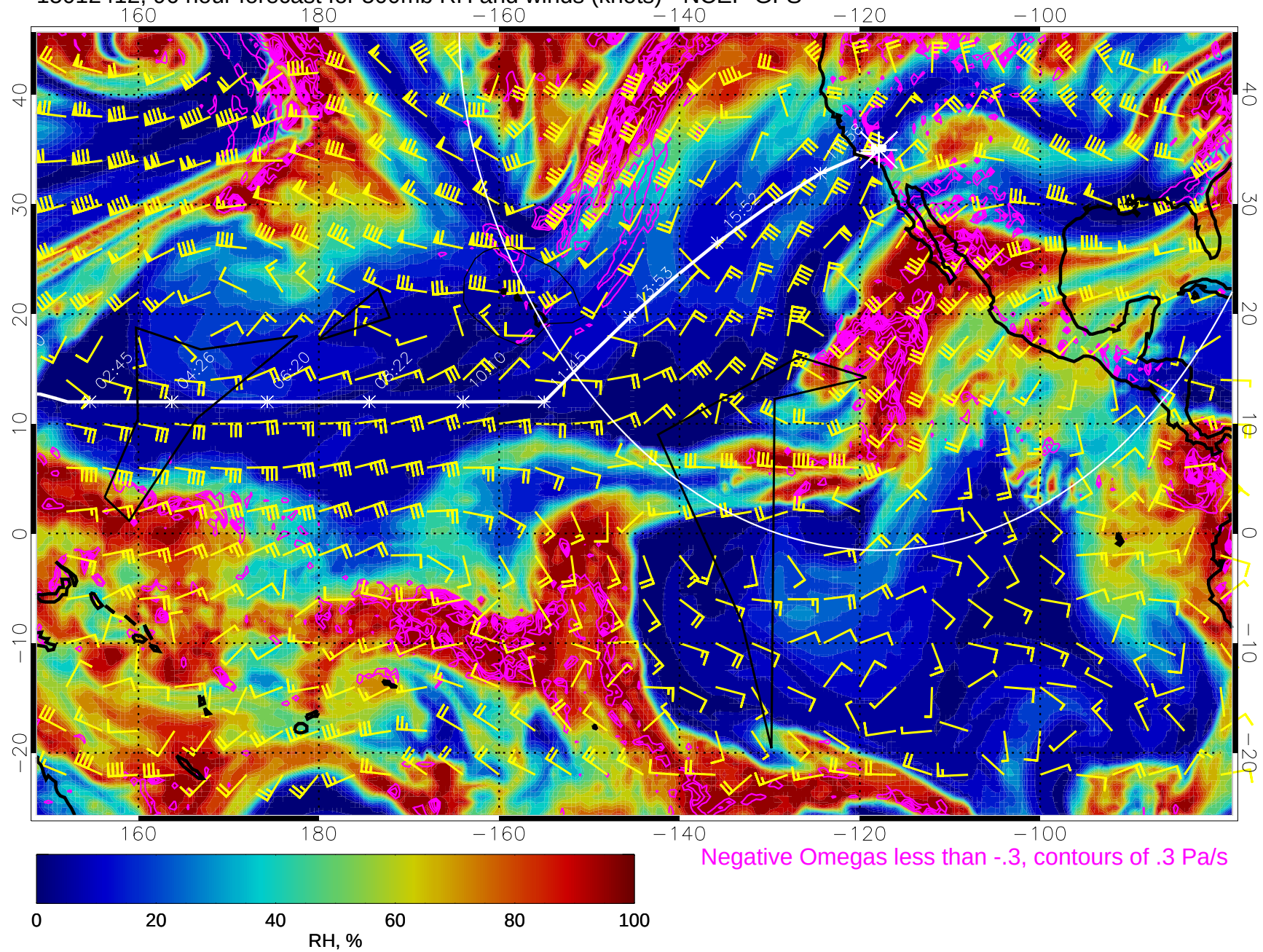
15012412, 96 hour forecast for 500mb RH and winds (knots) - NCEP GFS
