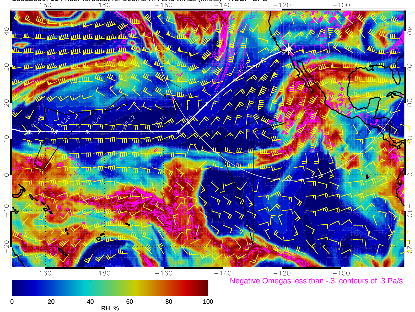
15012506, 114 hour forecast for 500mb RH and winds (knots) - NCEP GFS
