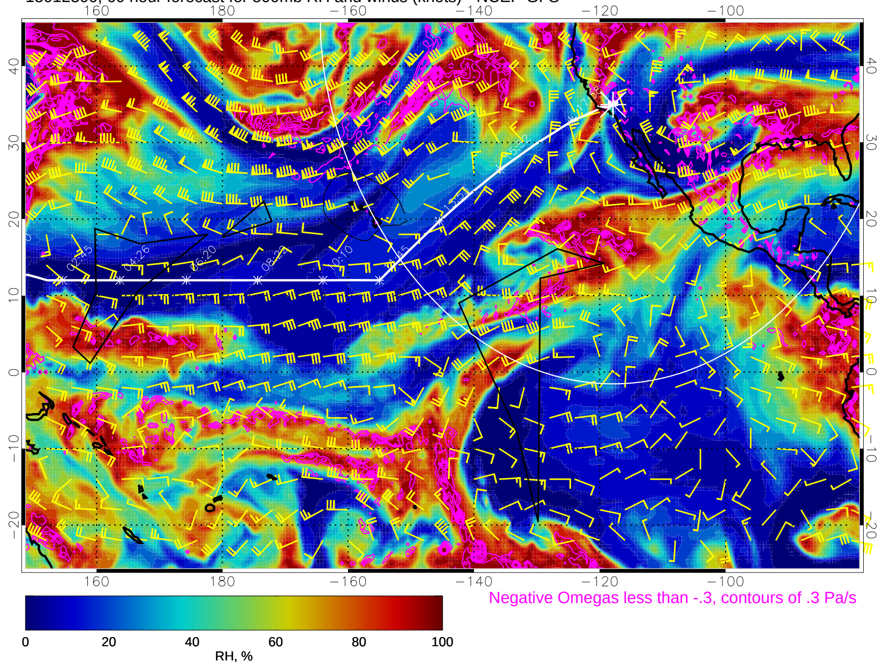
15012300, 60 hour forecast for 500mb RH and winds (knots) - NCEP GFS
