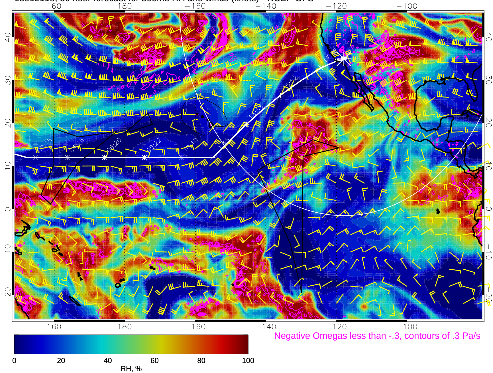
15012118, 30 hour forecast for 500mb RH and winds (knots) - NCEP GFS
