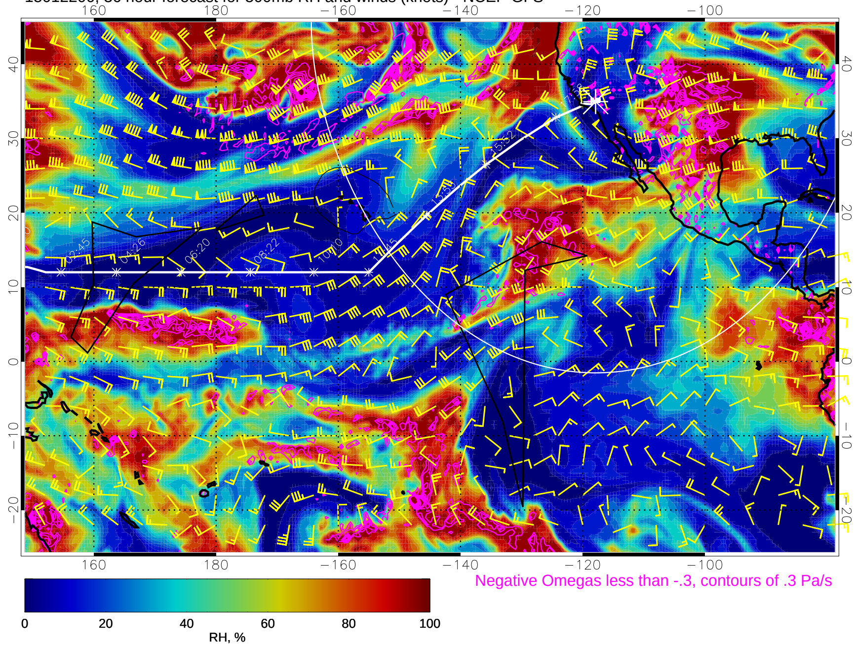
15012200, 36 hour forecast for 500mb RH and winds (knots) - NCEP GFS
