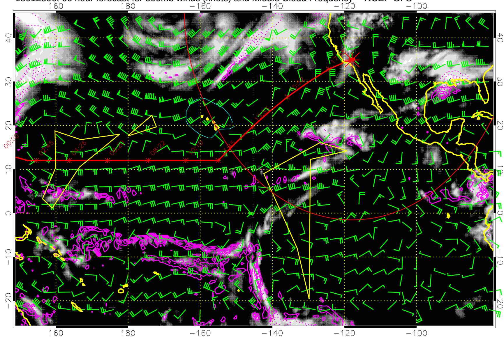
15012306, 66 hour forecast for 500mb winds (knots) and Middle Cloud Frequency -- NCEP GFS
