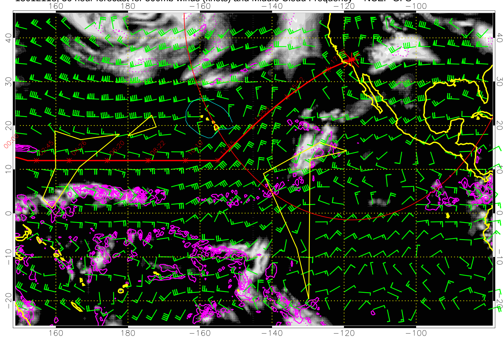
15012118, 30 hour forecast for 500mb winds (knots) and Middle Cloud Frequency -- NCEP GFS
