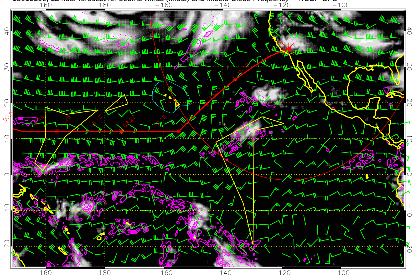
15012100, 12 hour forecast for 500mb winds (knots) and Middle Cloud Frequency -- NCEP GFS
