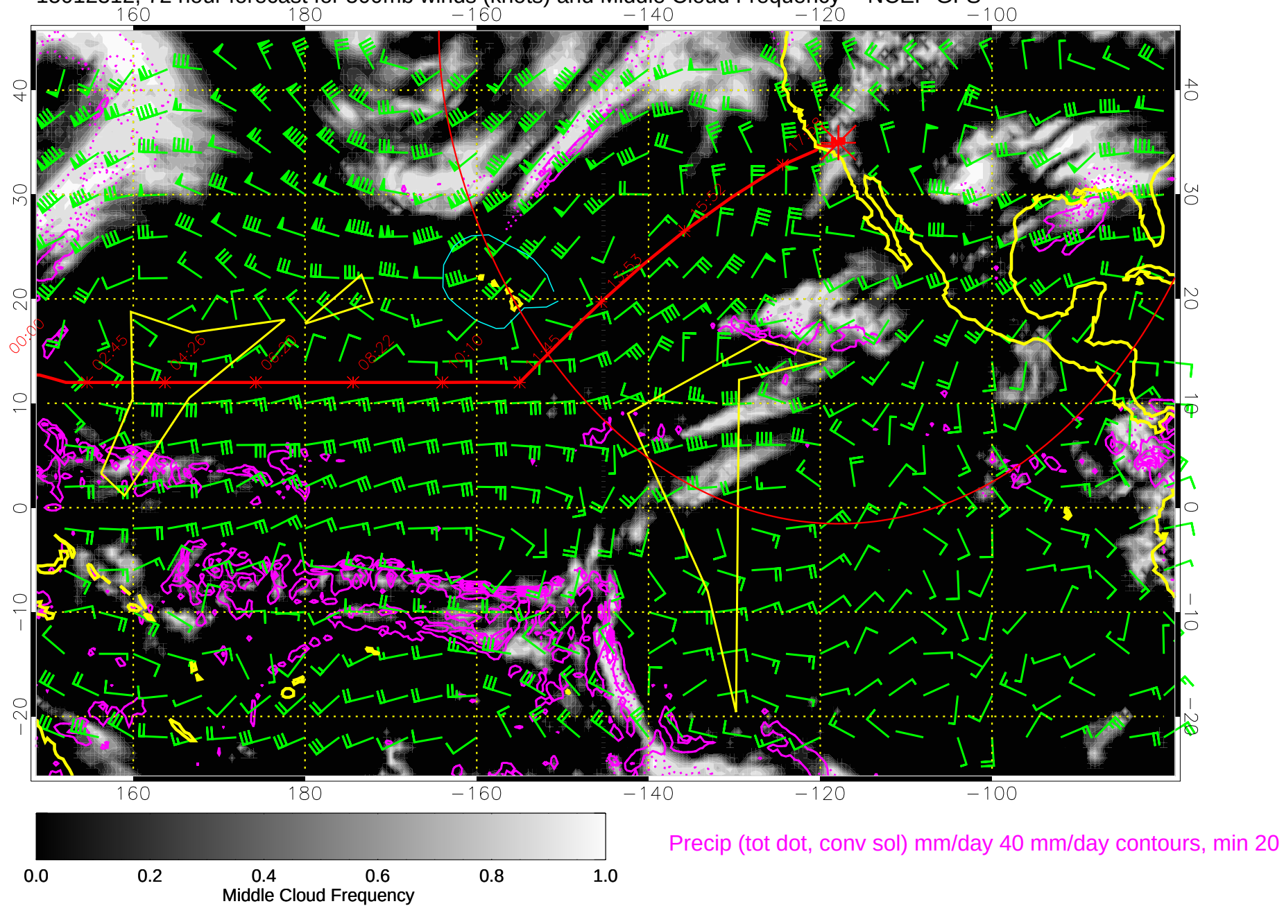
15012312, 72 hour forecast for 500mb winds (knots) and Middle Cloud Frequency -- NCEP GFS
