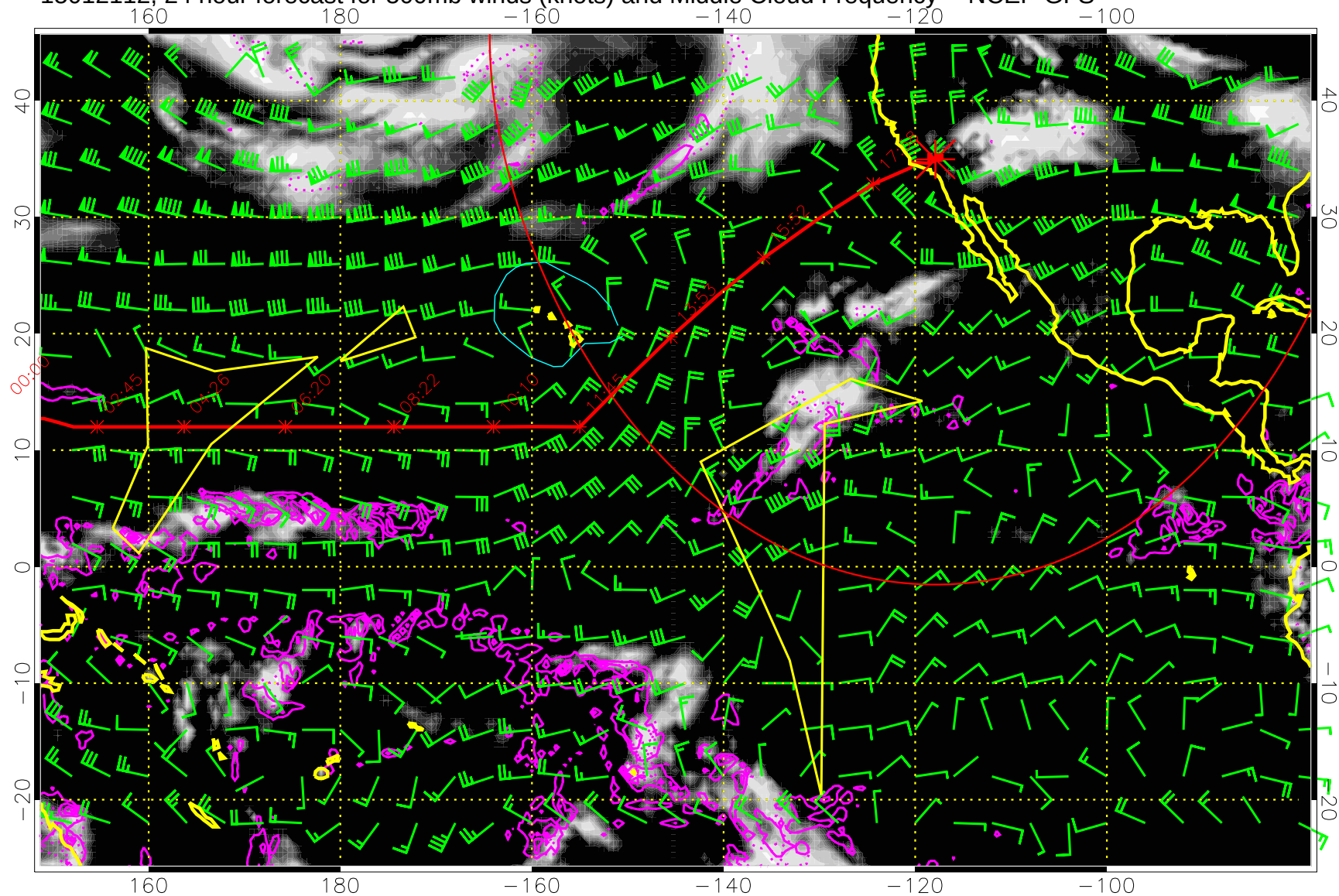
15012112, 24 hour forecast for 500mb winds (knots) and Middle Cloud Frequency -- NCEP GFS
