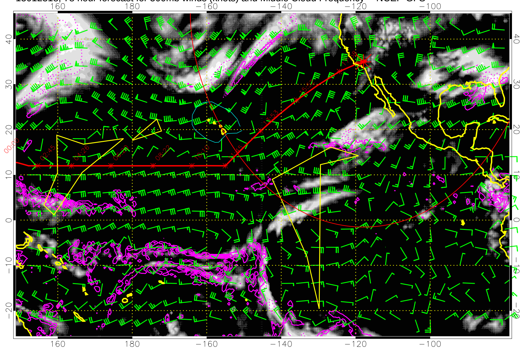
15012318, 78 hour forecast for 500mb winds (knots) and Middle Cloud Frequency -- NCEP GFS
