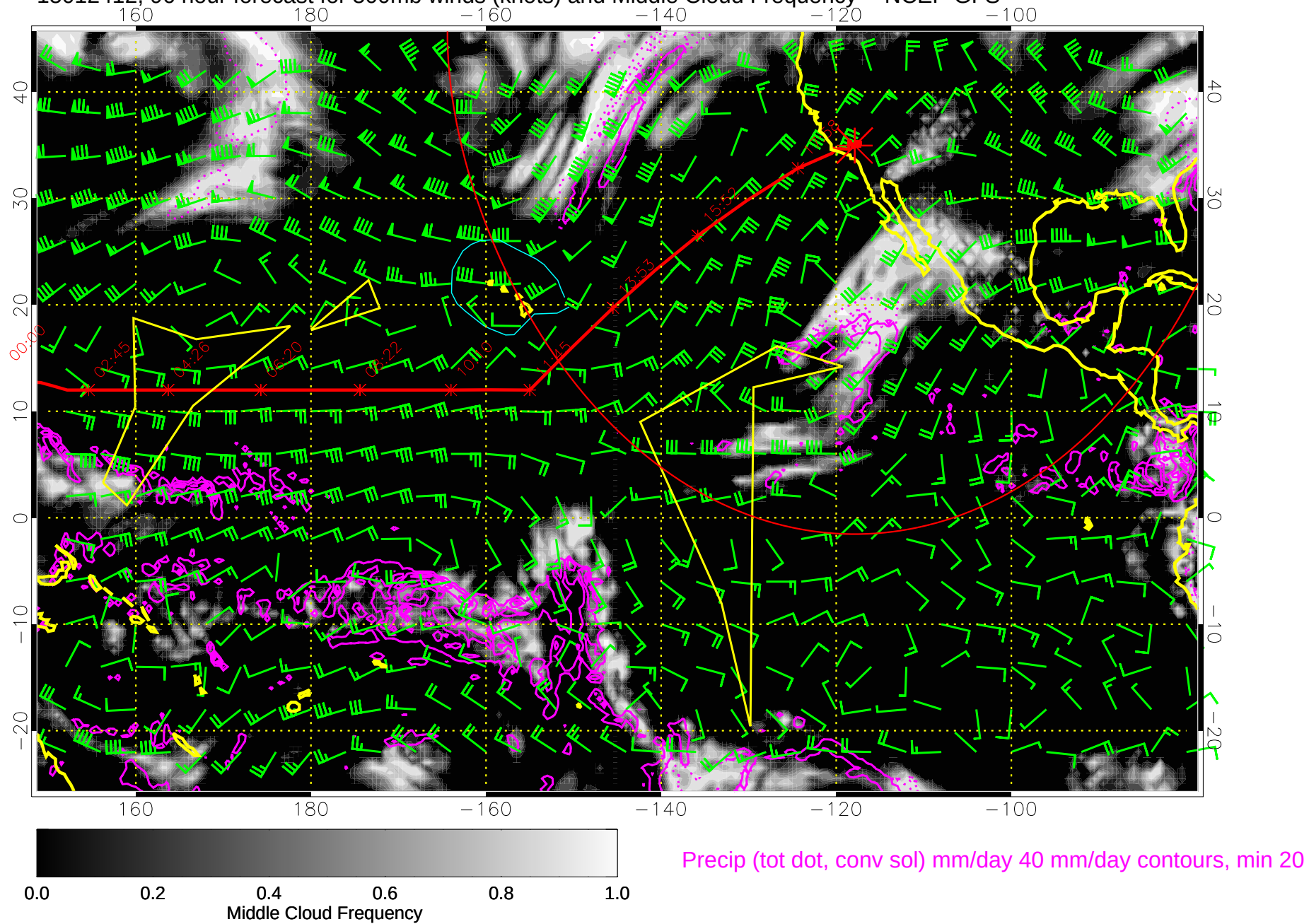
15012412, 96 hour forecast for 500mb winds (knots) and Middle Cloud Frequency -- NCEP GFS
