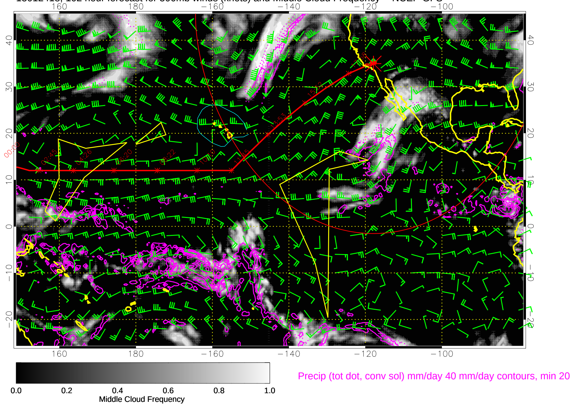
15012418, 102 hour forecast for 500mb winds (knots) and Middle Cloud Frequency -- NCEP GFS
