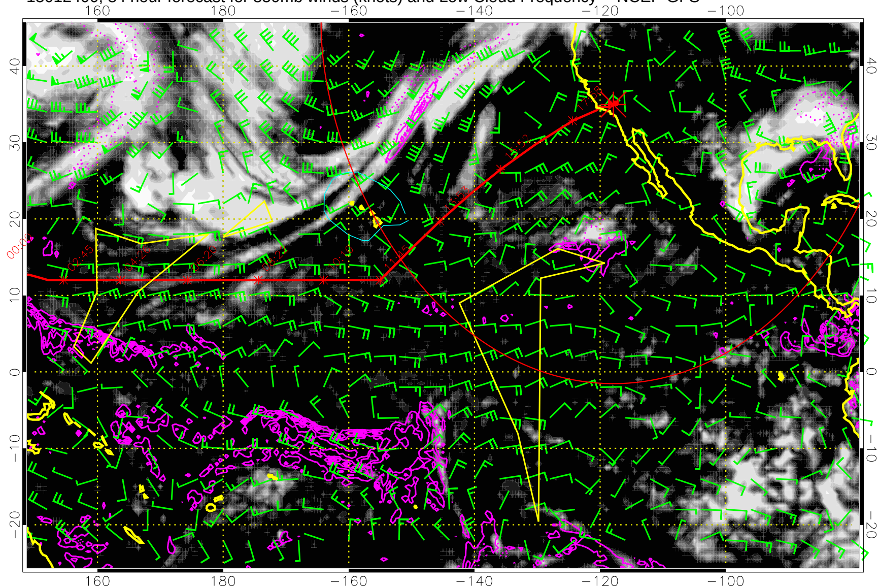
15012400, 84 hour forecast for 850mb winds (knots) and Low Cloud Frequency -- NCEP GFS
