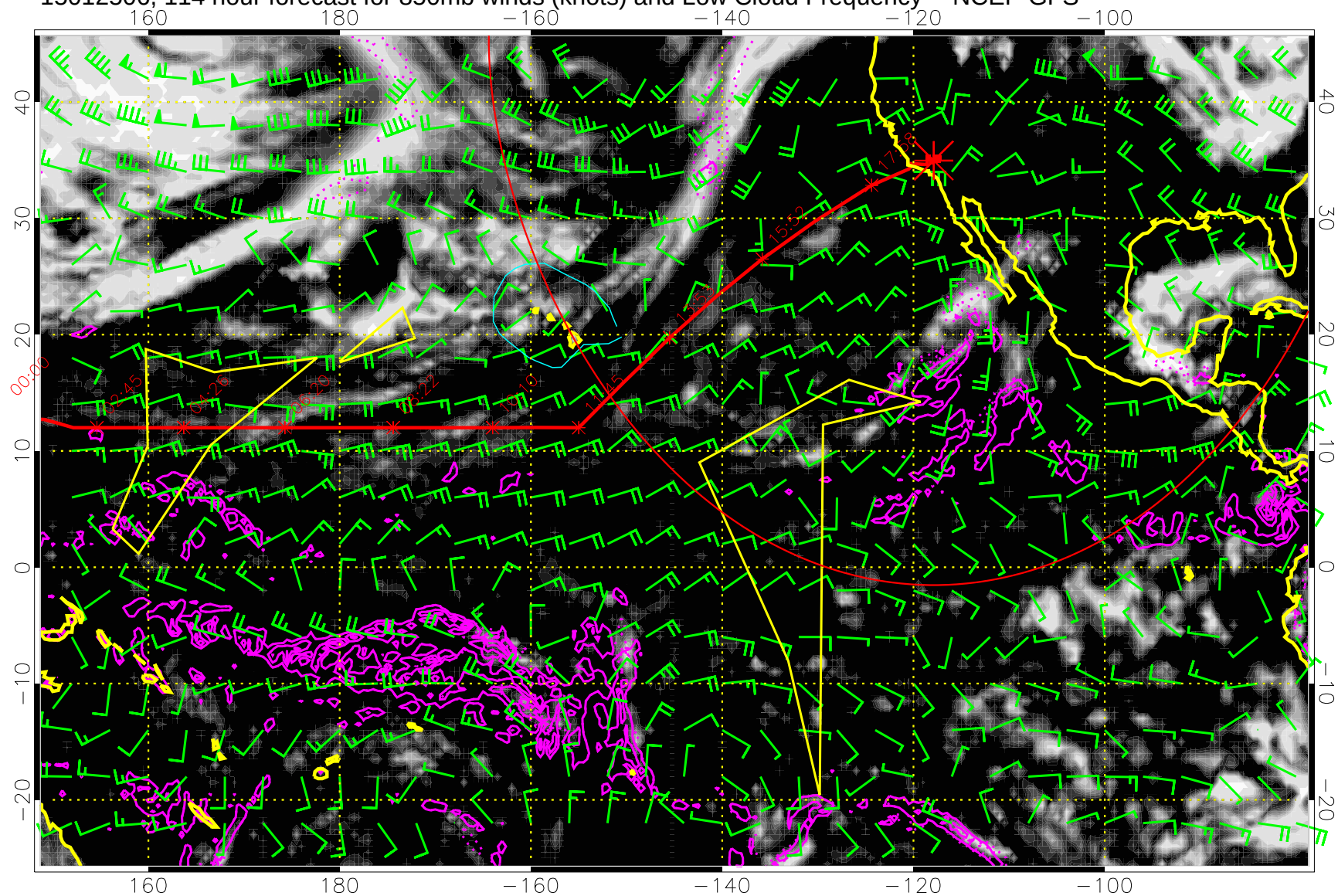
15012506, 114 hour forecast for 850mb winds (knots) and Low Cloud Frequency -- NCEP GFS
