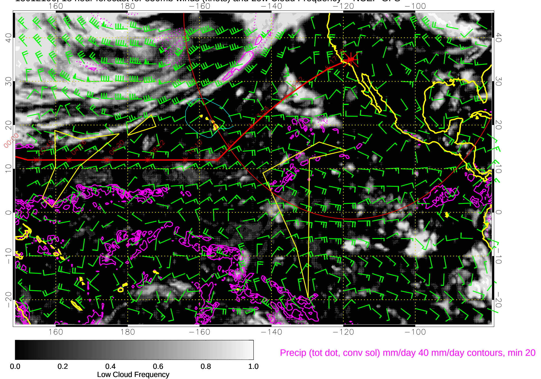
15012106, 18 hour forecast for 850mb winds (knots) and Low Cloud Frequency -- NCEP GFS
