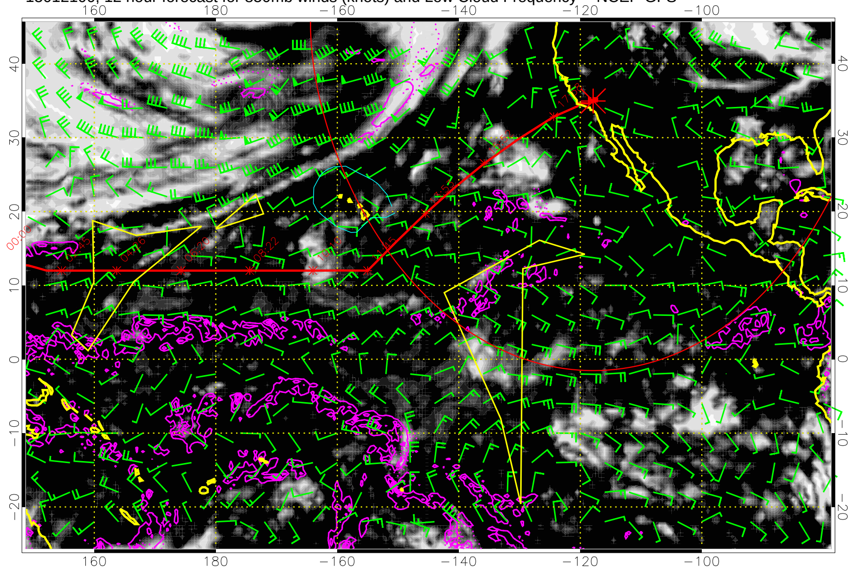
15012100, 12 hour forecast for 850mb winds (knots) and Low Cloud Frequency -- NCEP GFS
