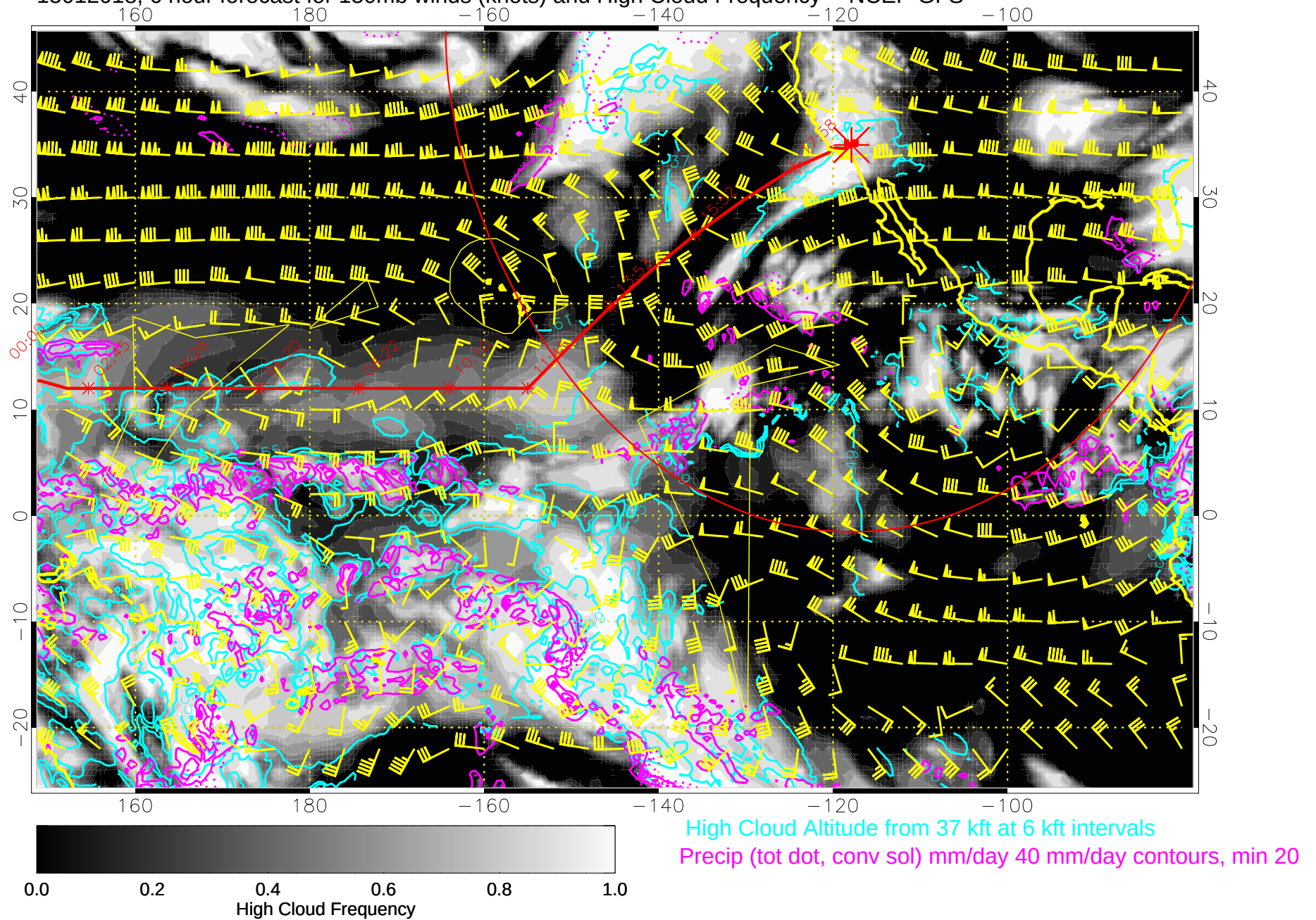
15012018, 6 hour forecast for 150mb winds (knots) and High Cloud Frequency -- NCEP GFS
