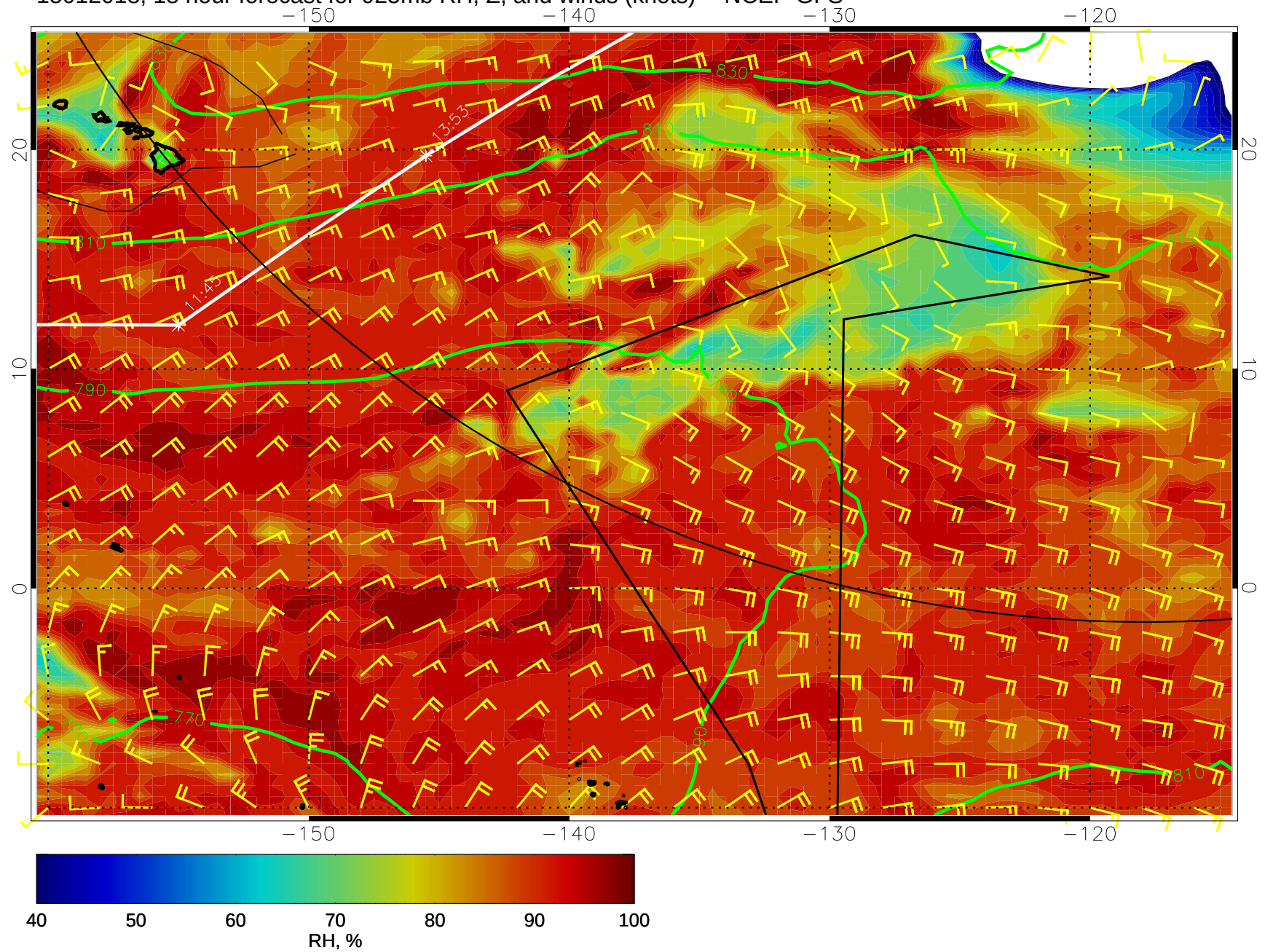
15012018, 18 hour forecast for 925mb RH, Z, and winds (knots) -- NCEP GFS
