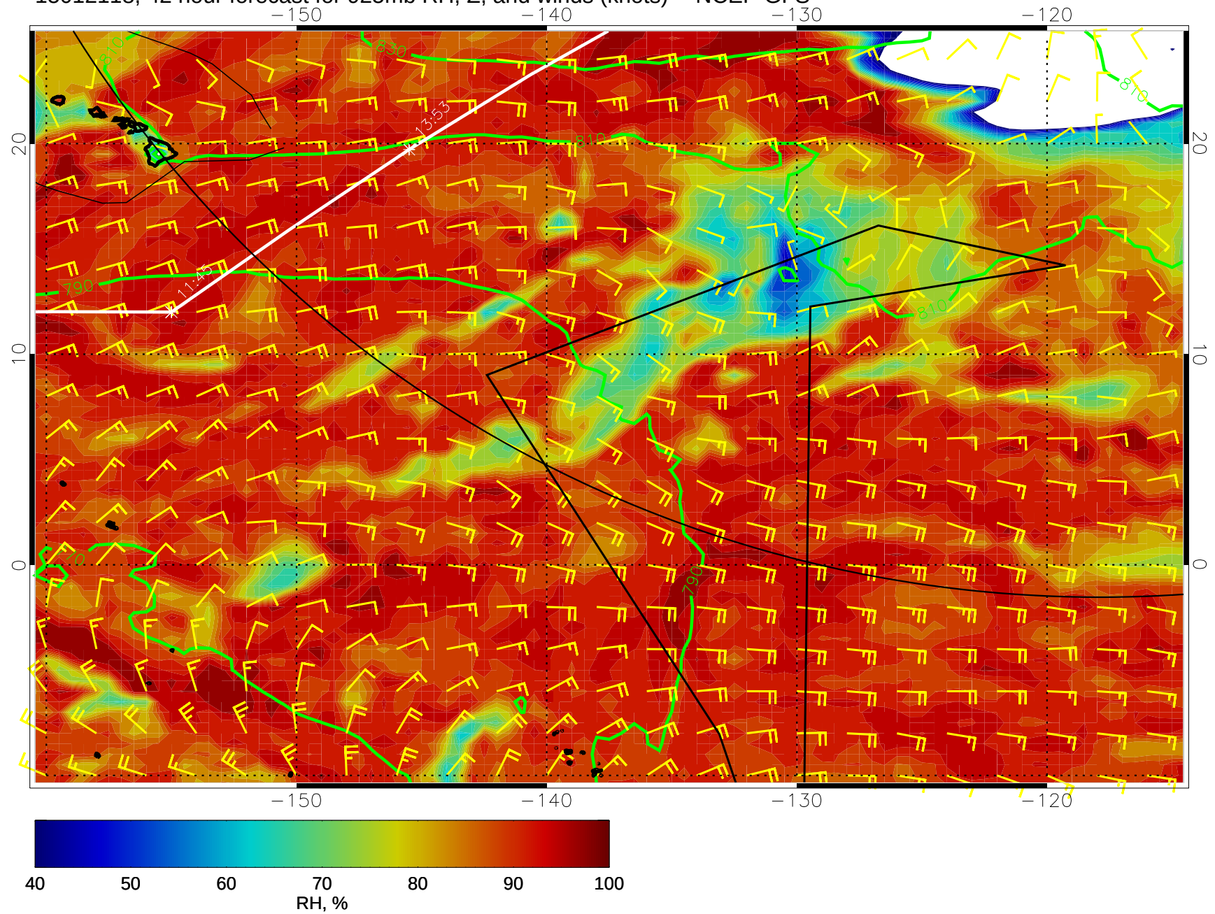
15012118, 42 hour forecast for 925mb RH, Z, and winds (knots) -- NCEP GFS
