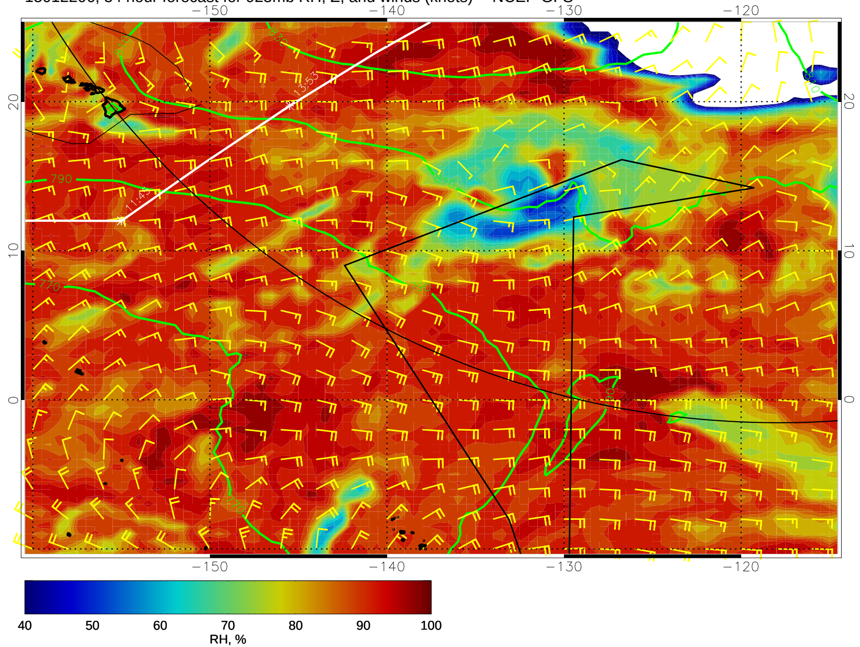
15012206, 54 hour forecast for 925mb RH, Z, and winds (knots) -- NCEP GFS
