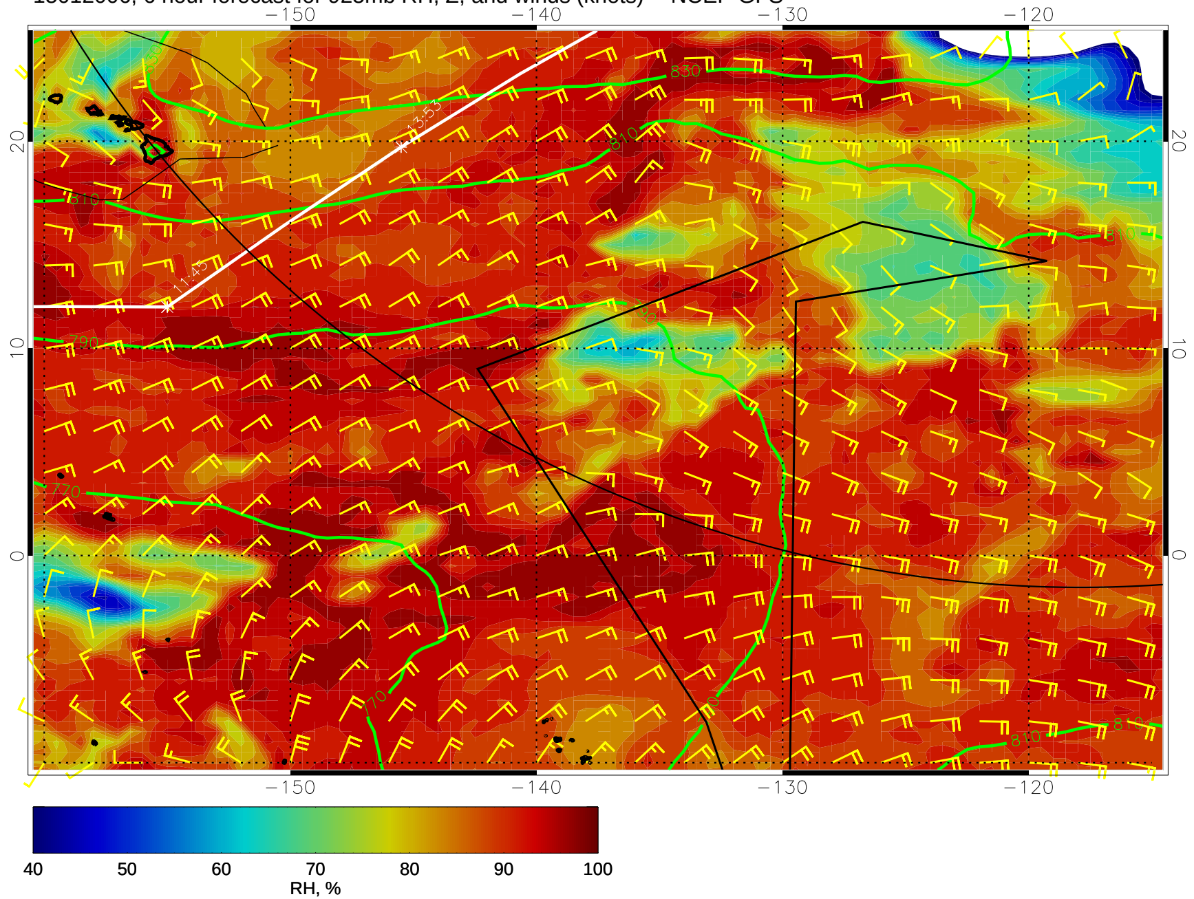
15012006, 6 hour forecast for 925mb RH, Z, and winds (knots) -- NCEP GFS
