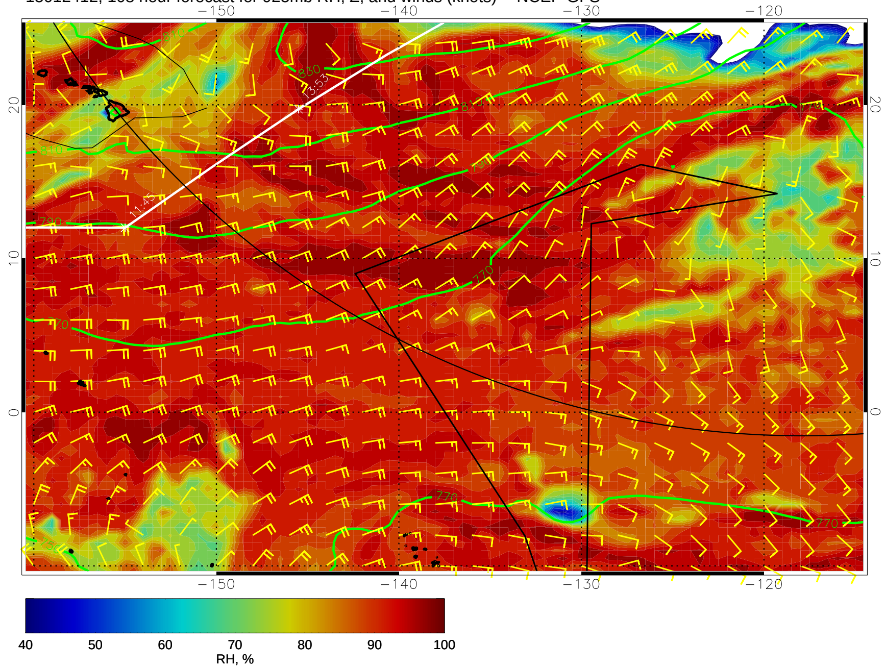
15012412, 108 hour forecast for 925mb RH, Z, and winds (knots) -- NCEP GFS
