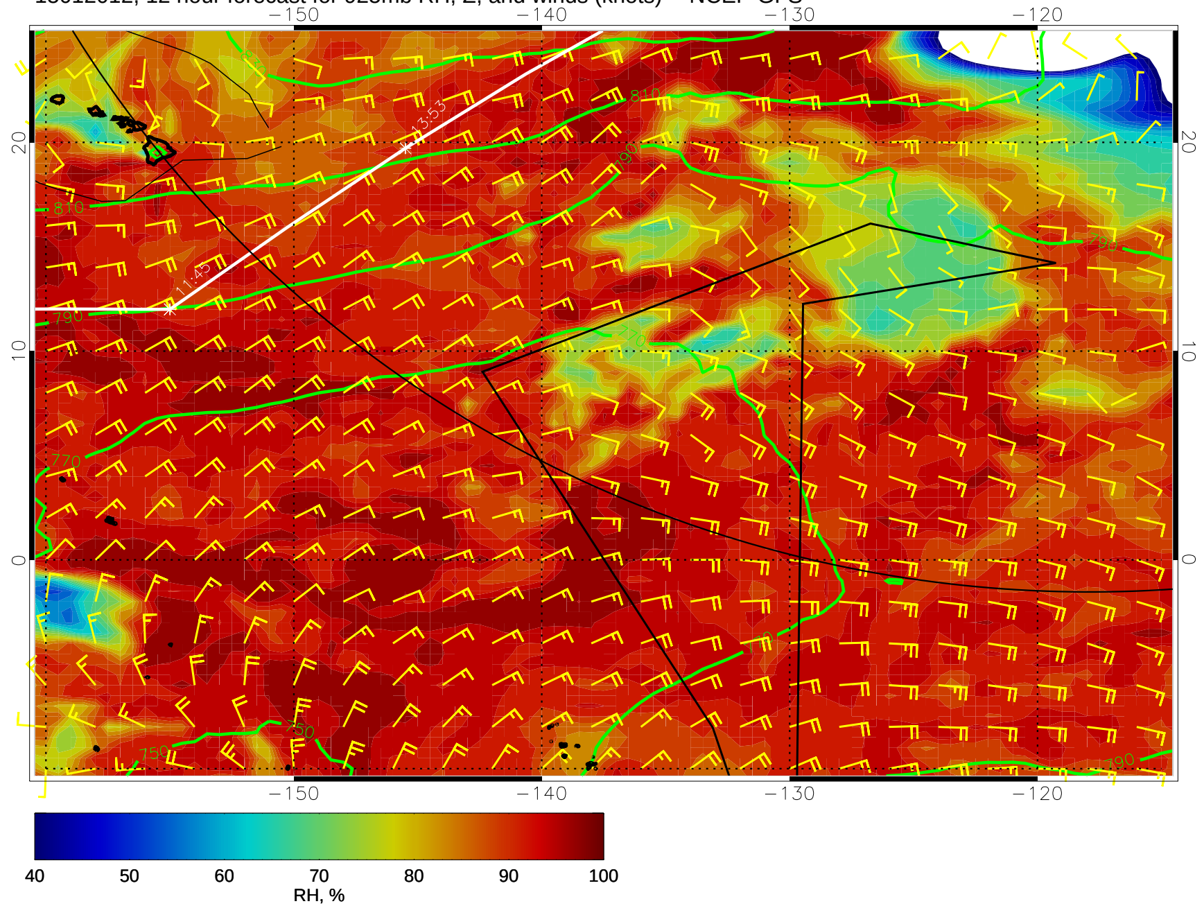
15012012, 12 hour forecast for 925mb RH, Z, and winds (knots) -- NCEP GFS
