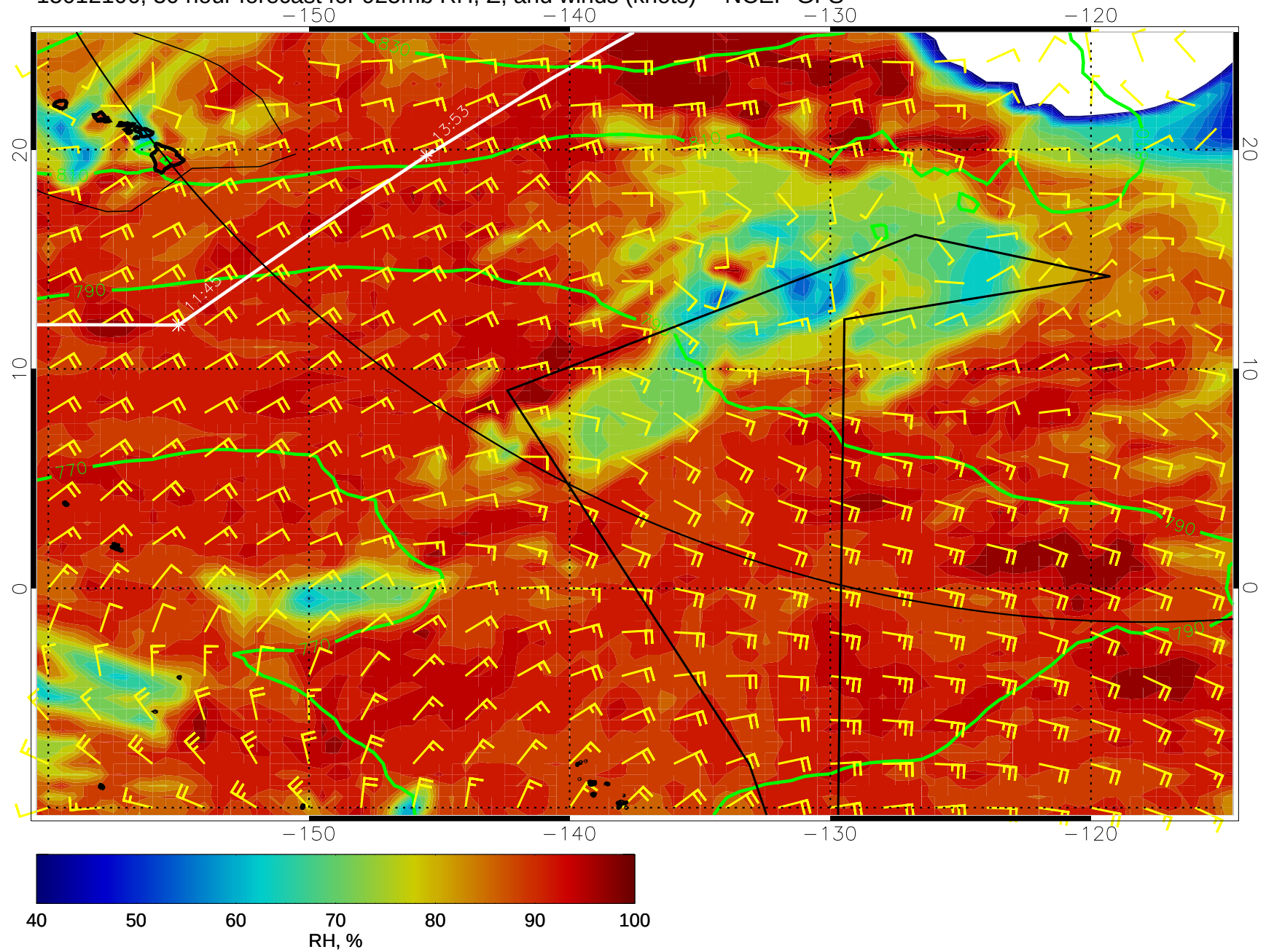
15012106, 30 hour forecast for 925mb RH, Z, and winds (knots) -- NCEP GFS
