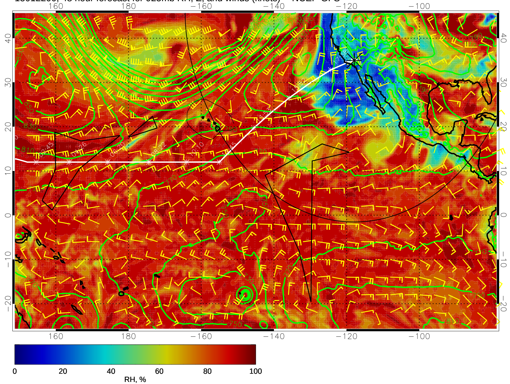
15012200, 48 hour forecast for 925mb RH, Z, and winds (knots) -- NCEP GFS
