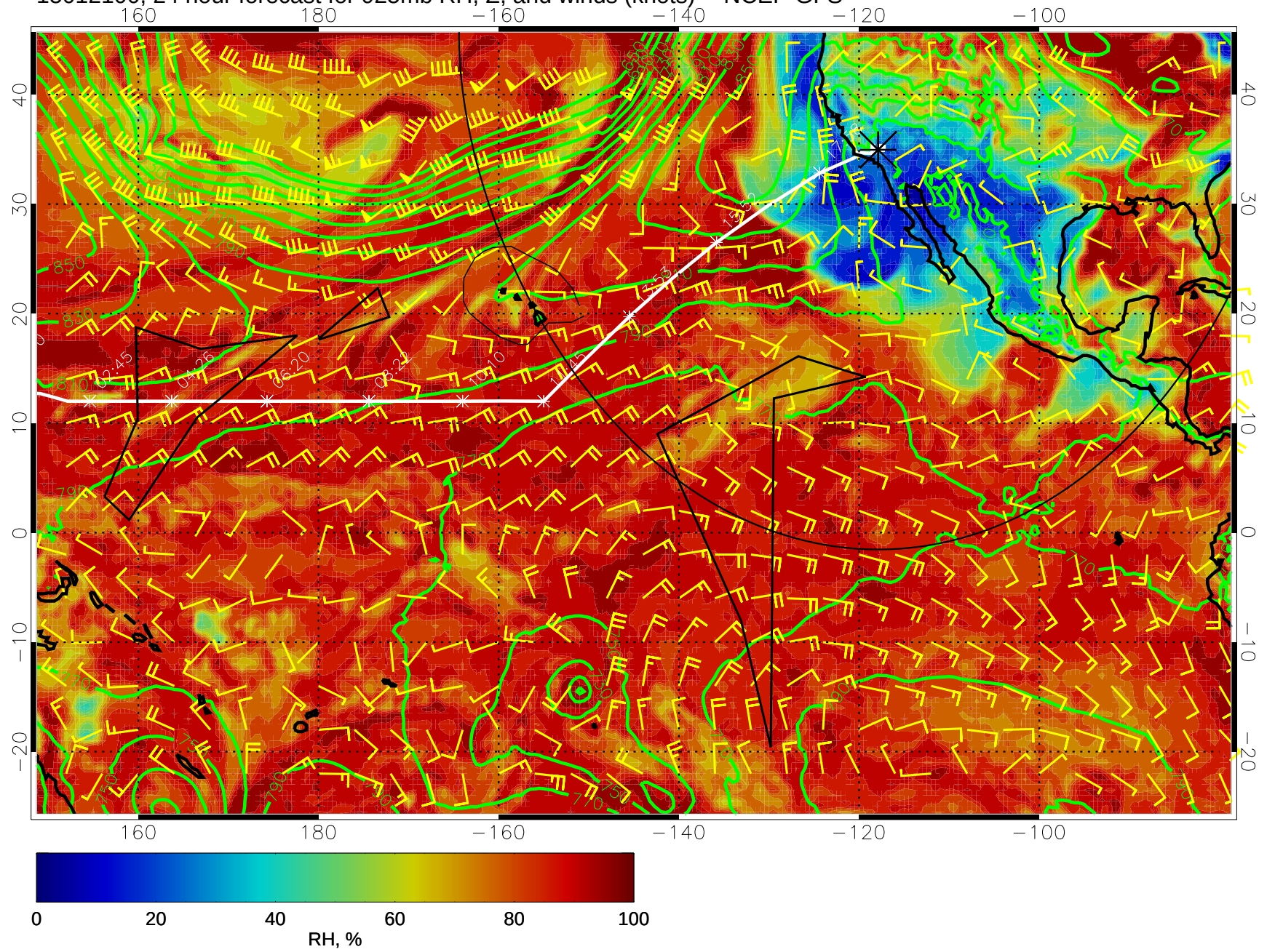
15012100, 24 hour forecast for 925mb RH, Z, and winds (knots) -- NCEP GFS
