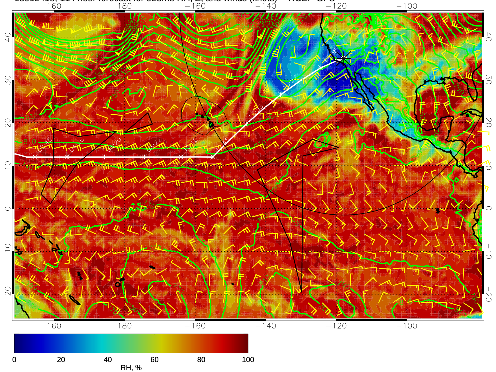
15012418, 114 hour forecast for 925mb RH, Z, and winds (knots) -- NCEP GFS
