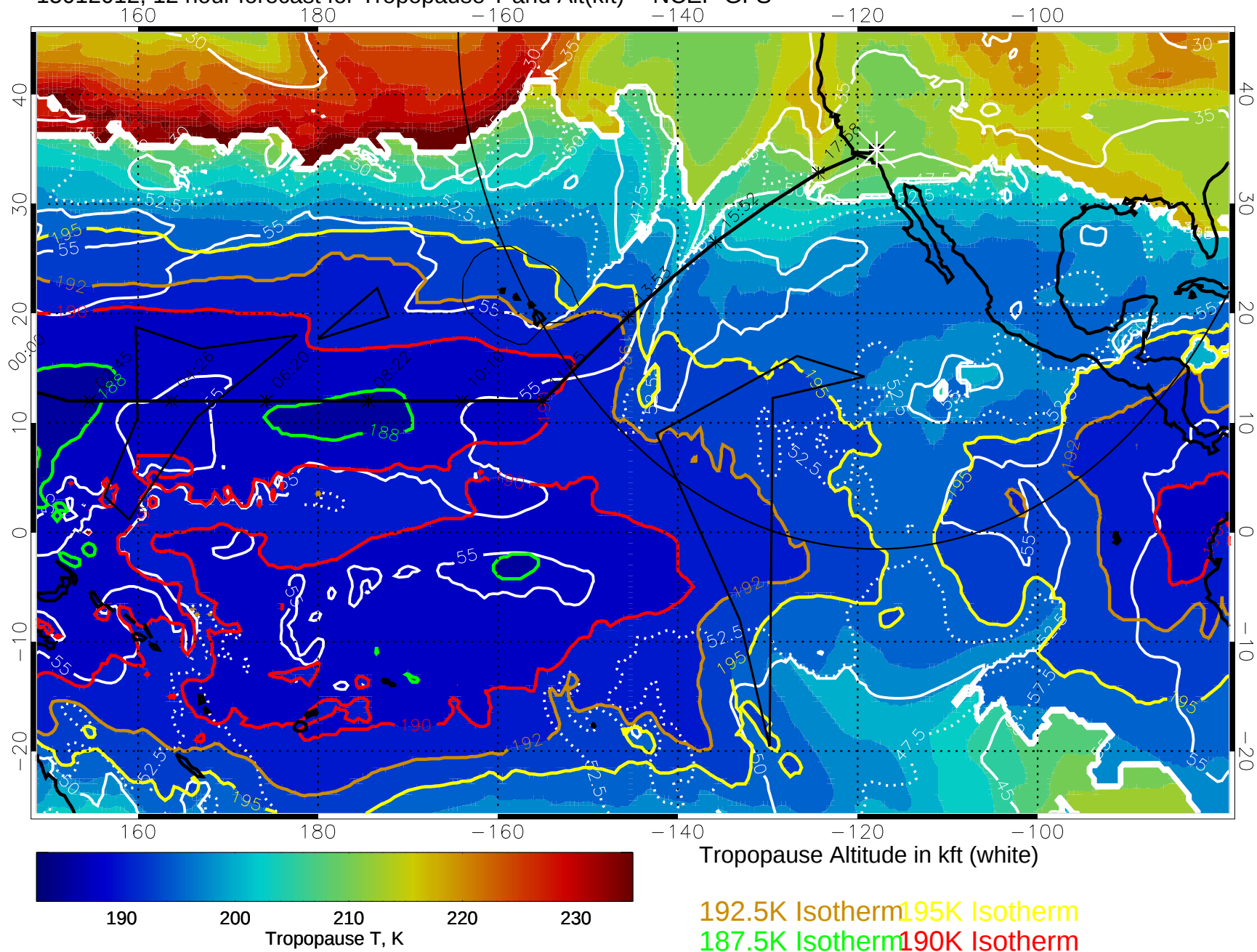
15012012, 12 hour forecast for Tropopause T and Alt(kft) -- NCEP GFS
