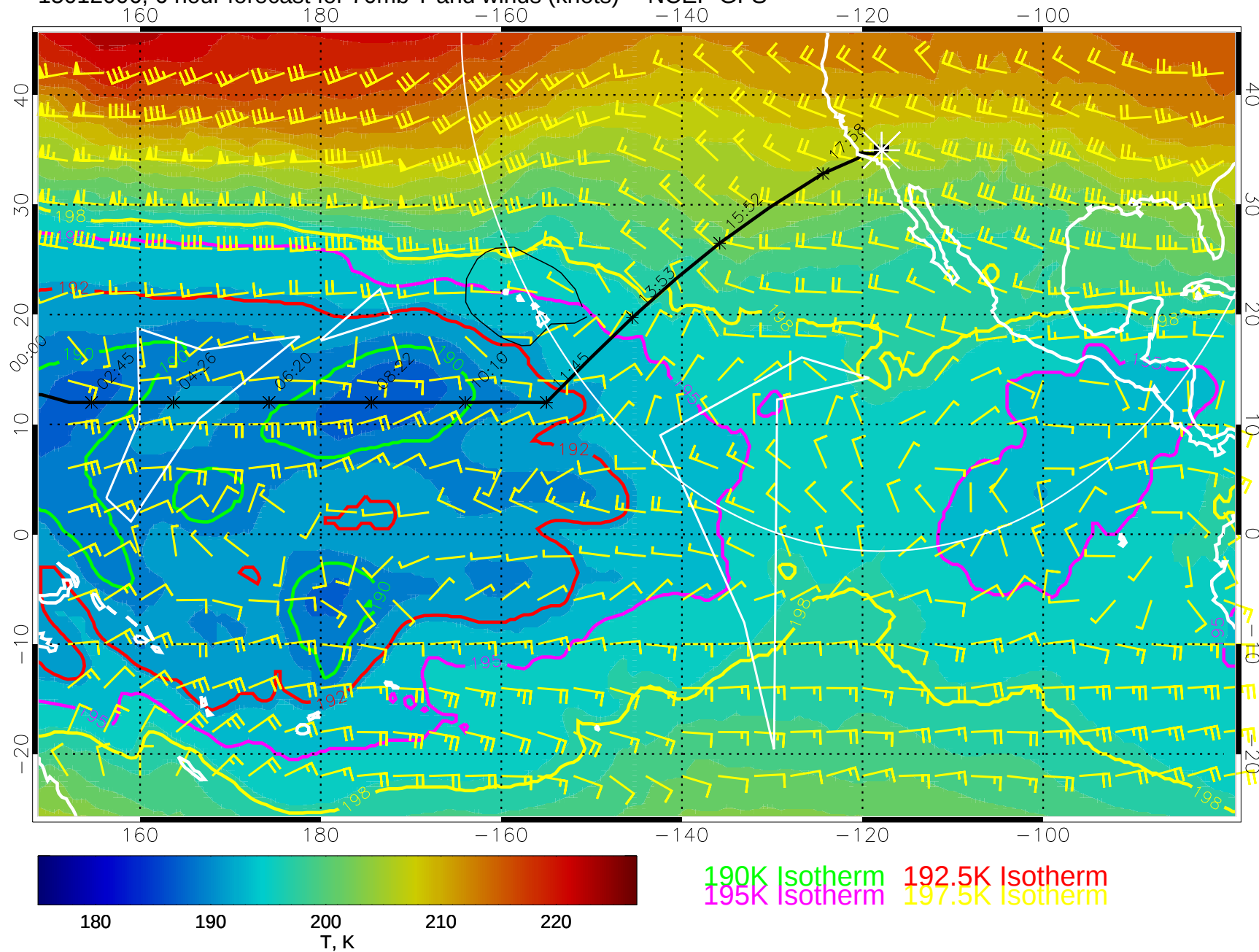
15012006, 6 hour forecast for 70mb T and winds (knots) -- NCEP GFS
