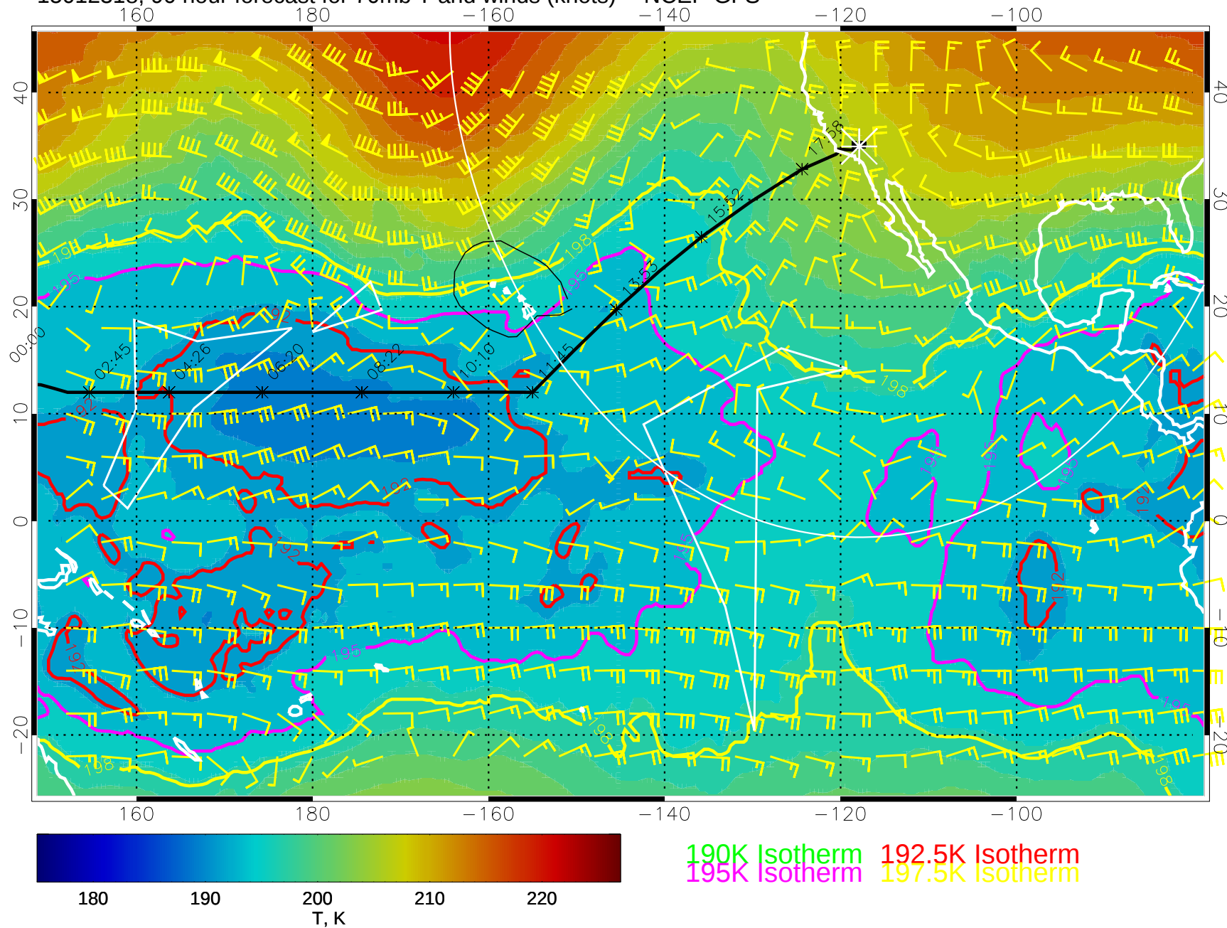
15012318, 90 hour forecast for 70mb T and winds (knots) -- NCEP GFS
