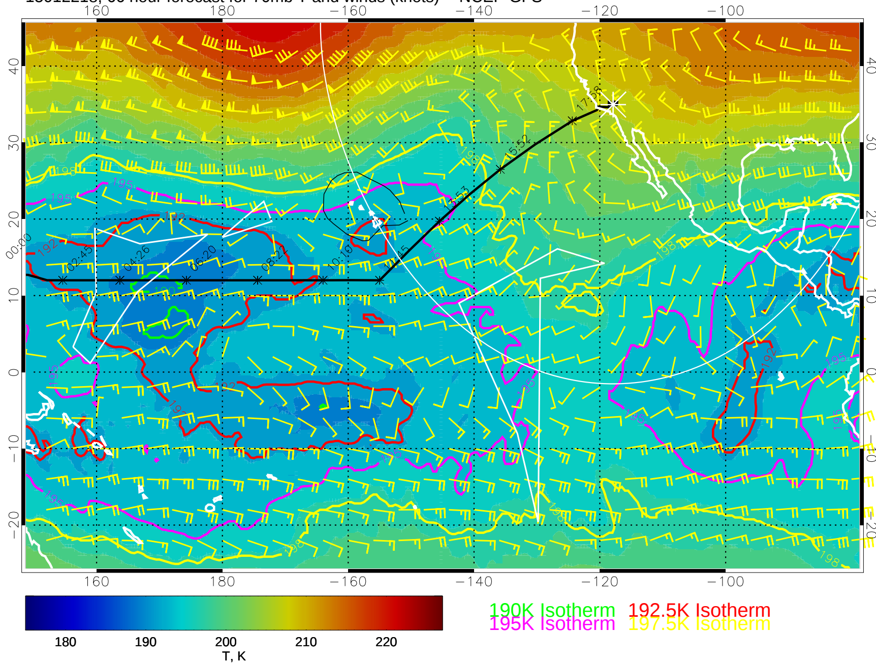
15012218, 66 hour forecast for 70mb T and winds (knots) -- NCEP GFS
