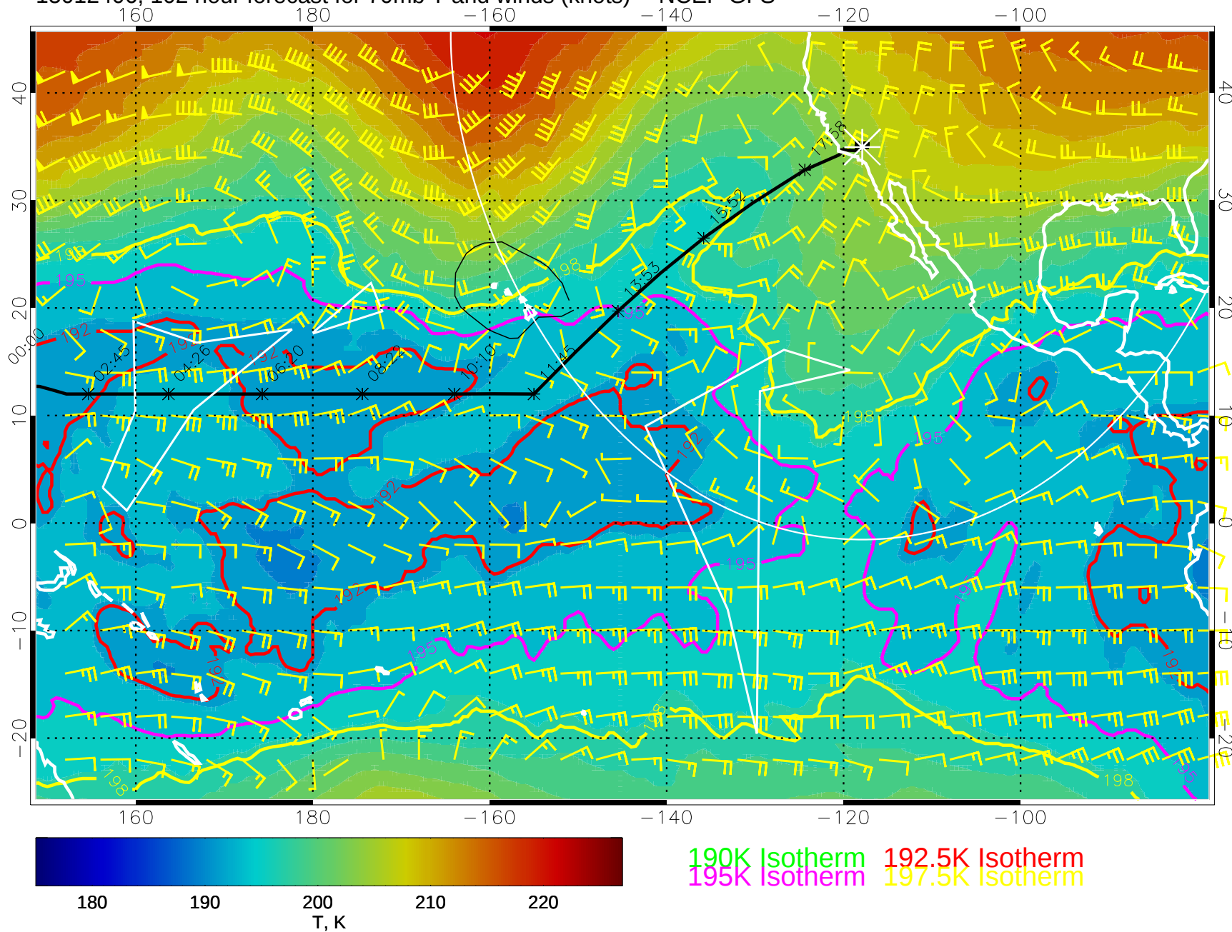
15012406, 102 hour forecast for 70mb T and winds (knots) -- NCEP GFS
