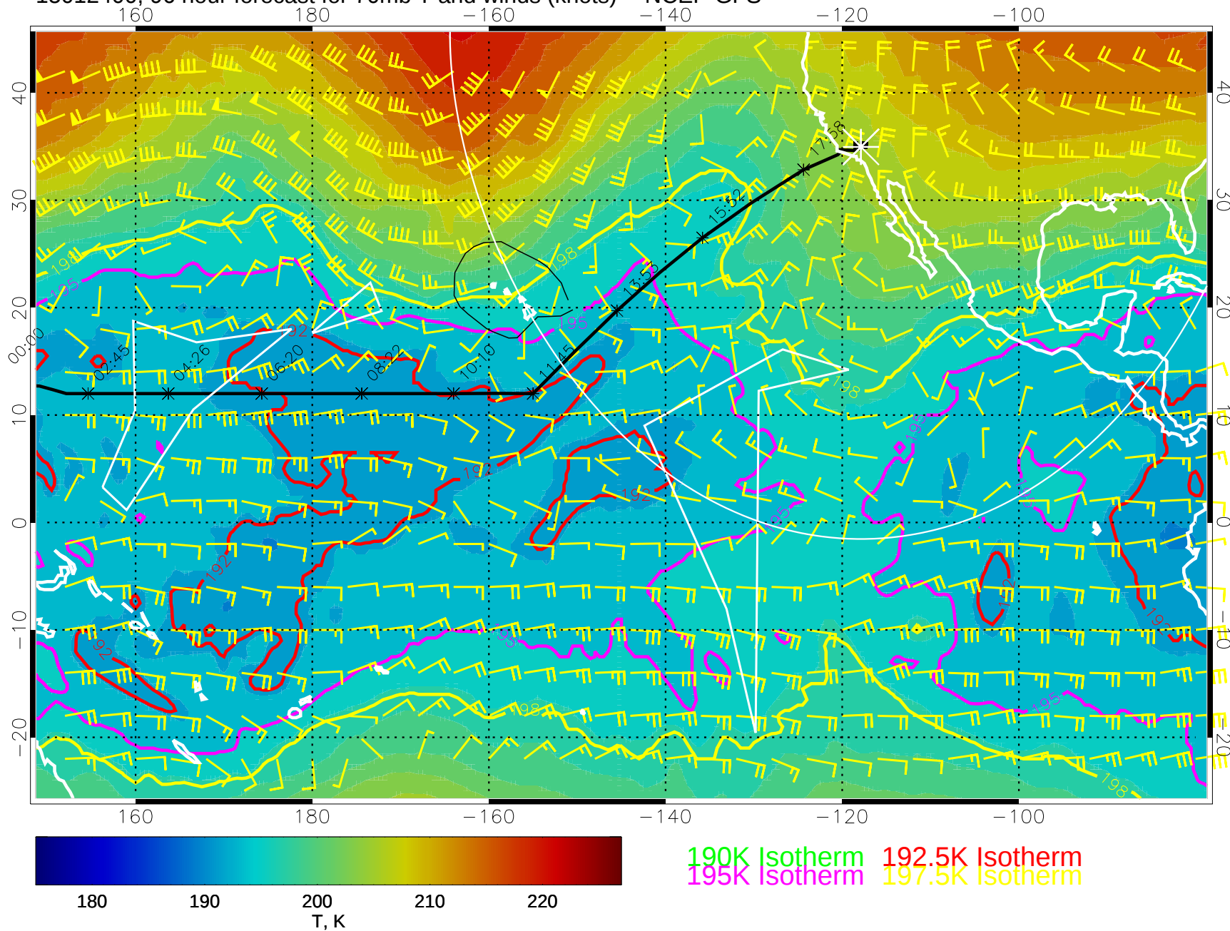
15012400, 96 hour forecast for 70mb T and winds (knots) -- NCEP GFS
