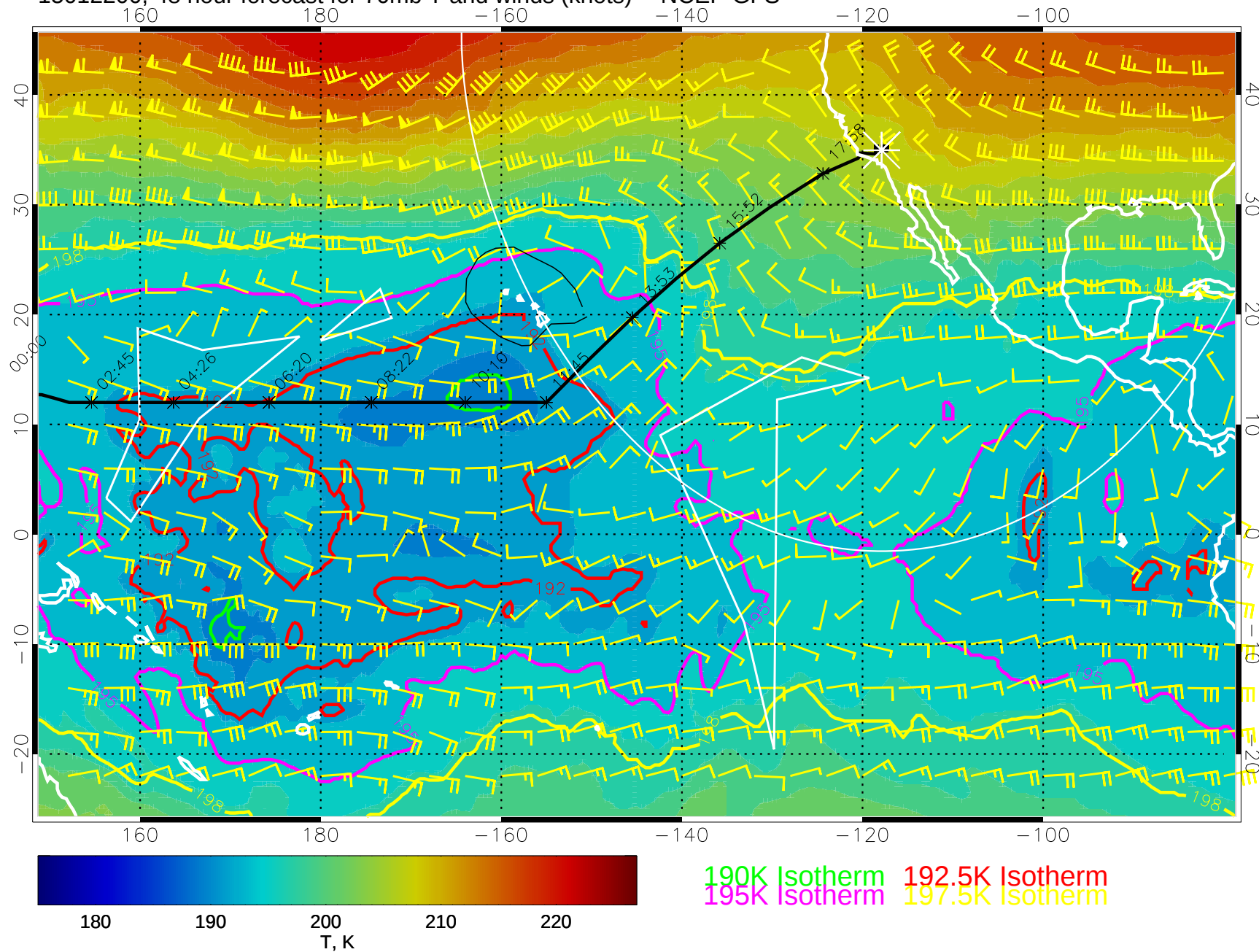
15012200, 48 hour forecast for 70mb T and winds (knots) -- NCEP GFS
