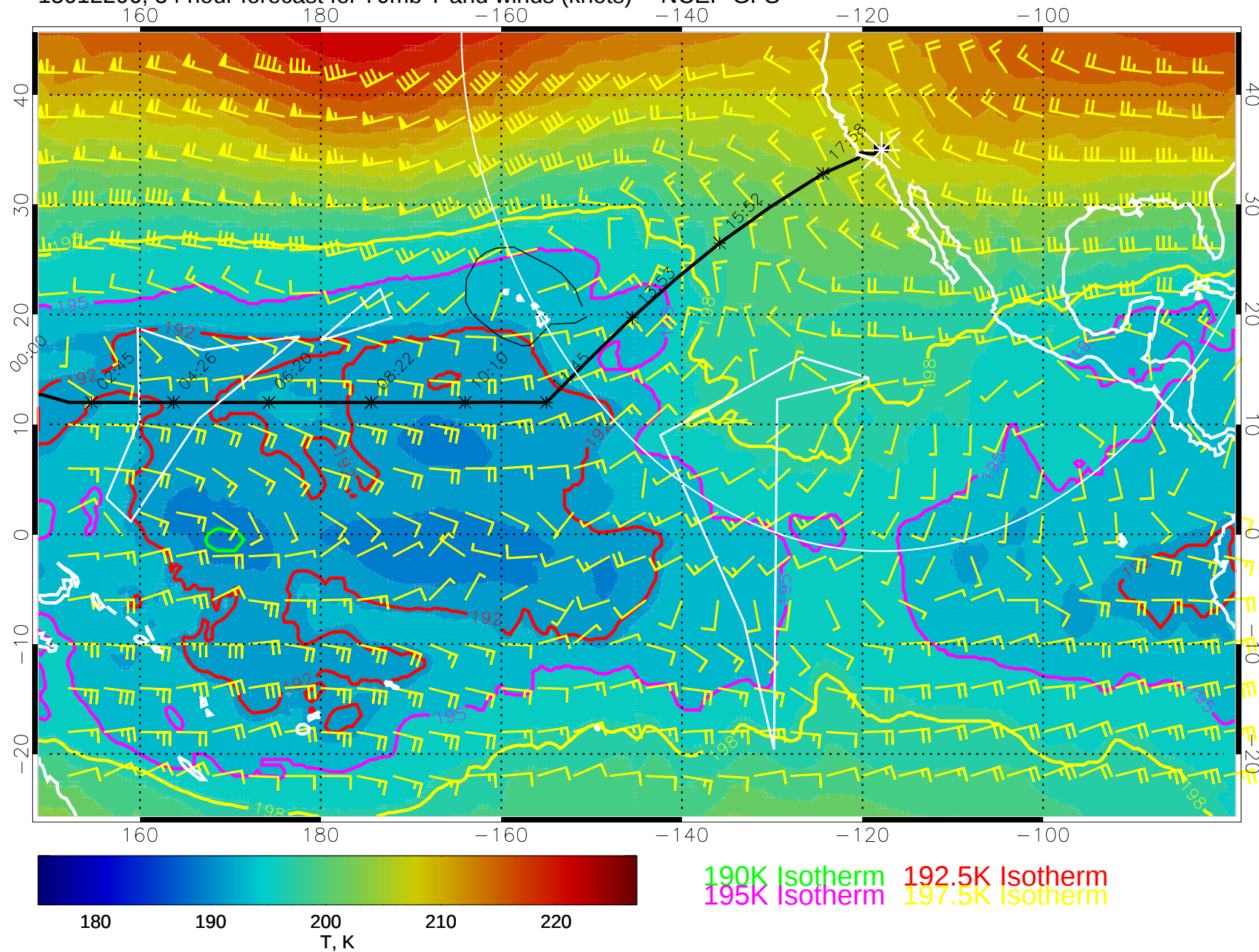
15012206, 54 hour forecast for 70mb T and winds (knots) -- NCEP GFS
