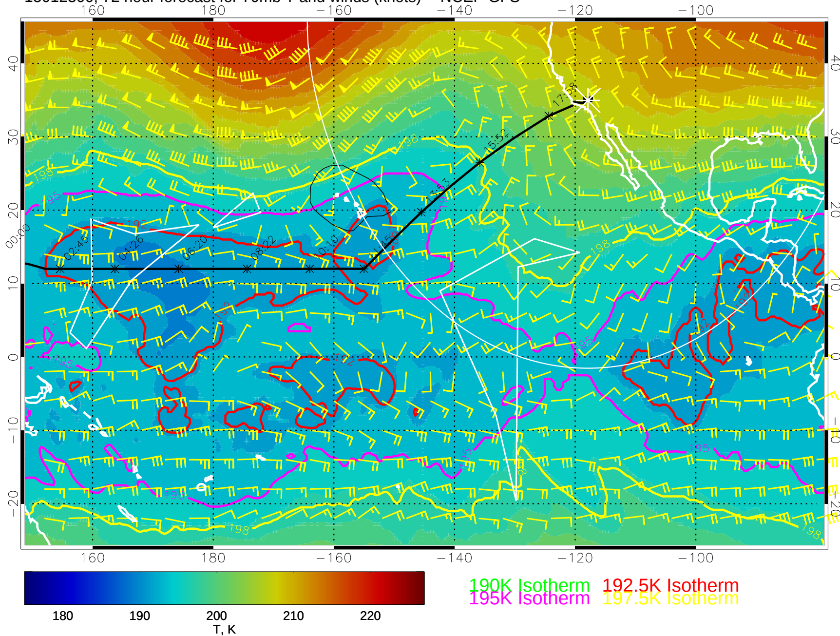
15012300, 72 hour forecast for 70mb T and winds (knots) -- NCEP GFS
