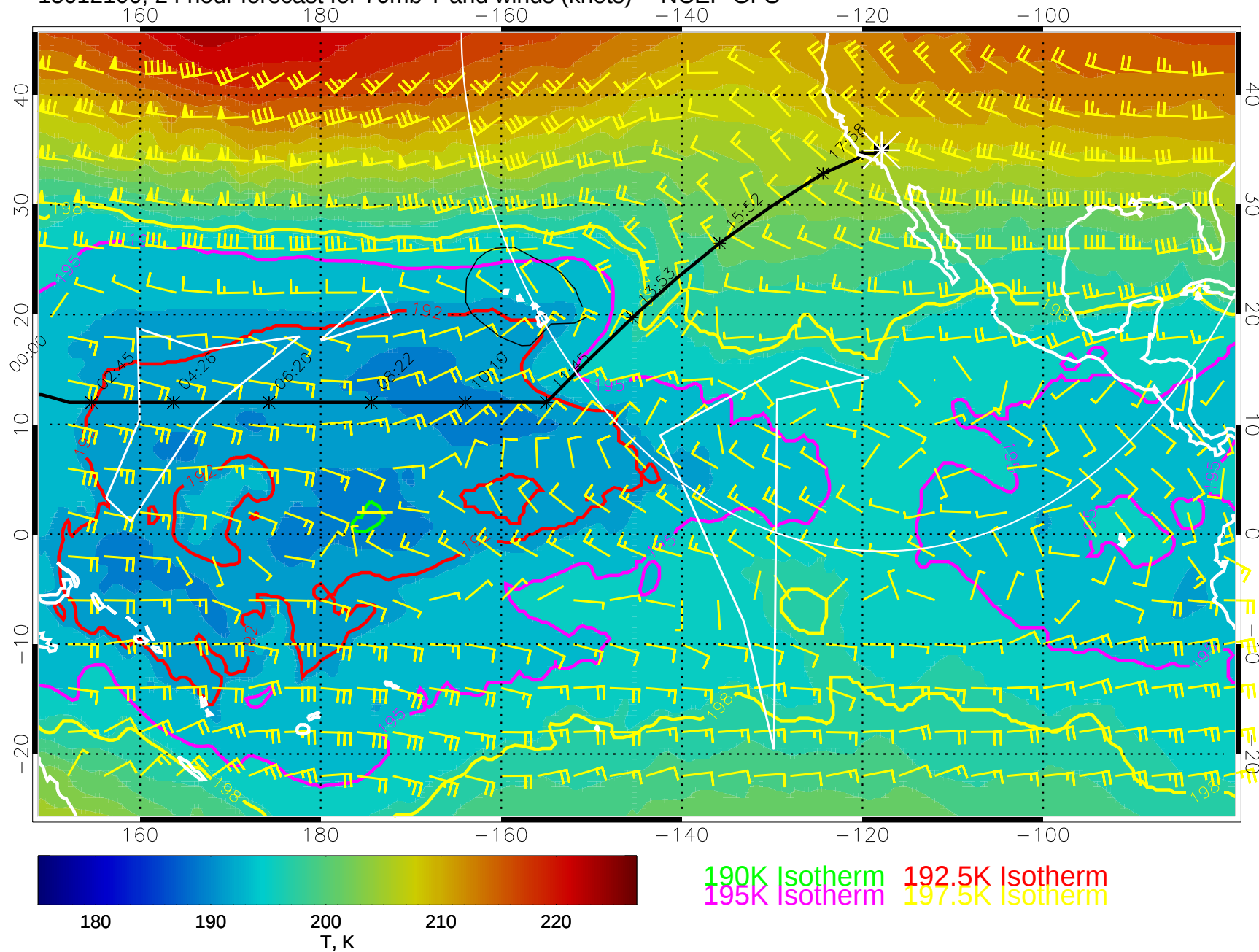
15012100, 24 hour forecast for 70mb T and winds (knots) -- NCEP GFS
