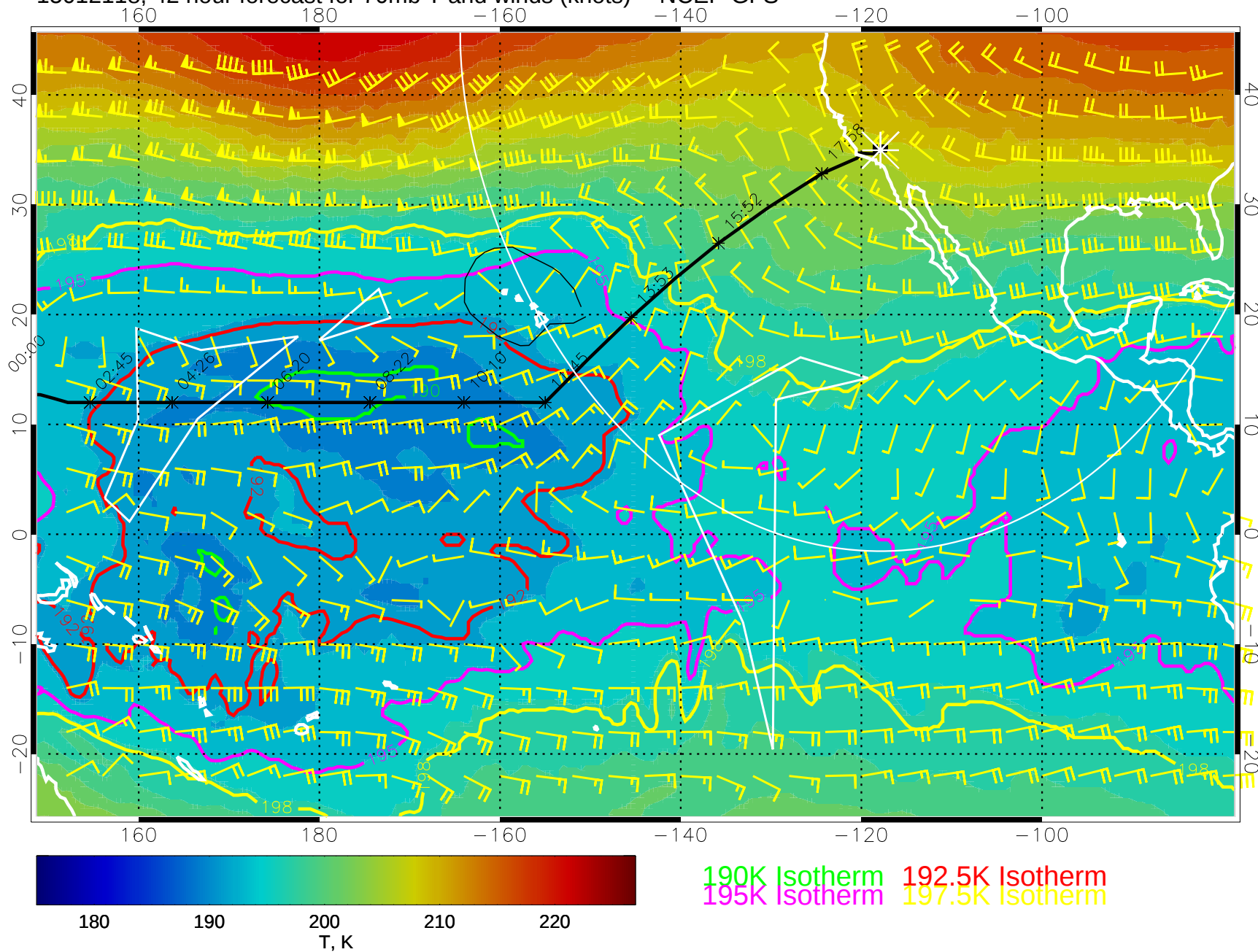
15012118, 42 hour forecast for 70mb T and winds (knots) -- NCEP GFS
