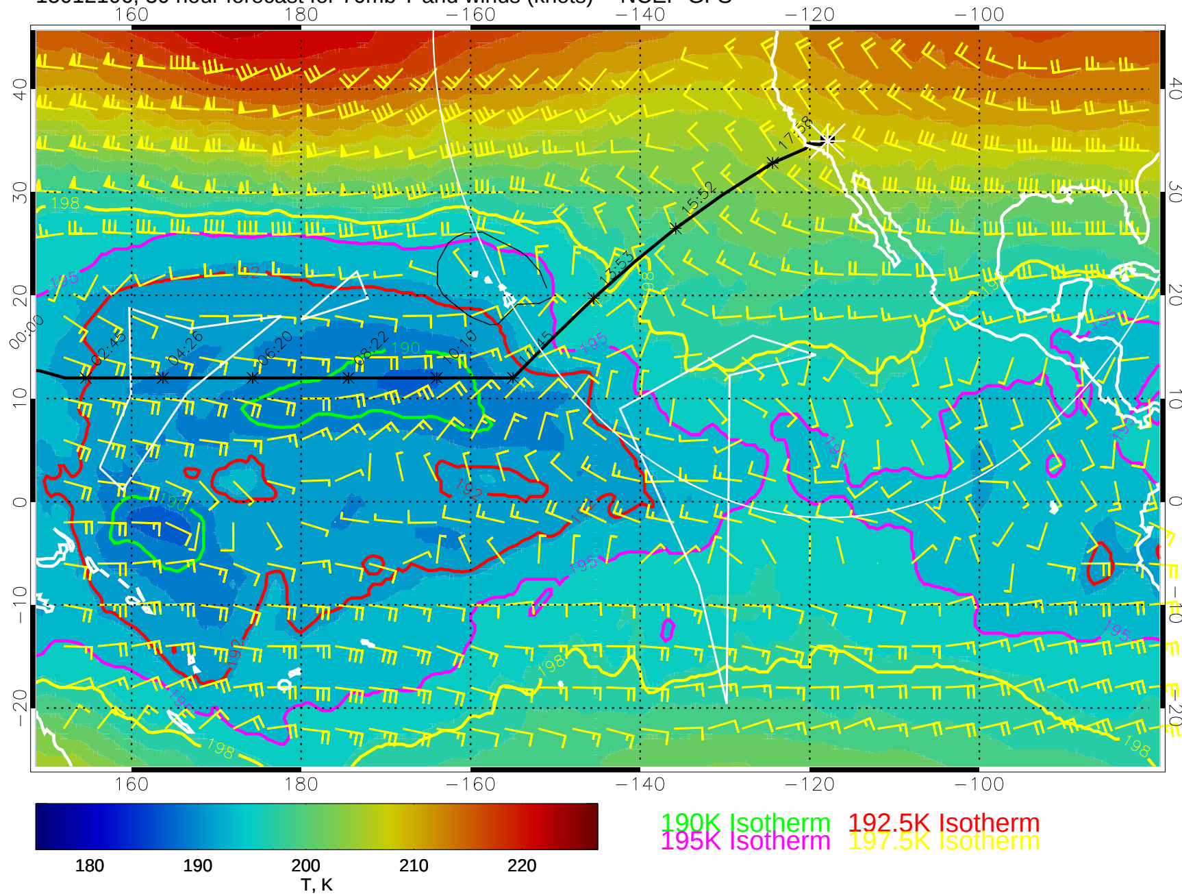
15012106, 30 hour forecast for 70mb T and winds (knots) -- NCEP GFS
