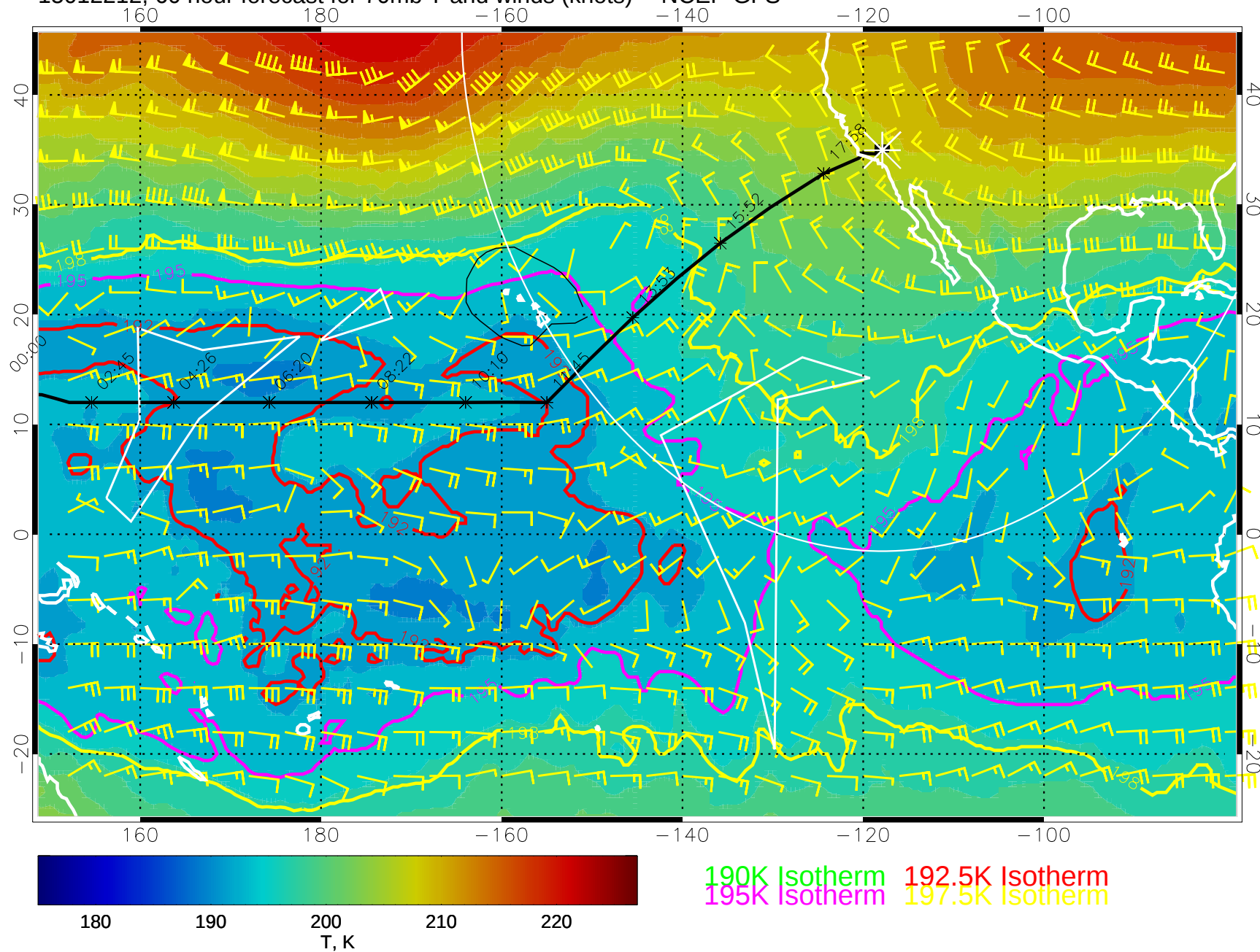
15012212, 60 hour forecast for 70mb T and winds (knots) -- NCEP GFS
