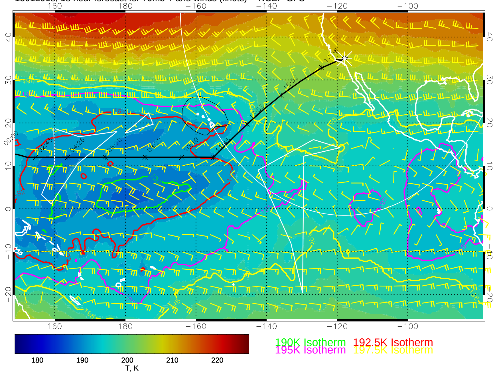
15012018, 18 hour forecast for 70mb T and winds (knots) -- NCEP GFS
