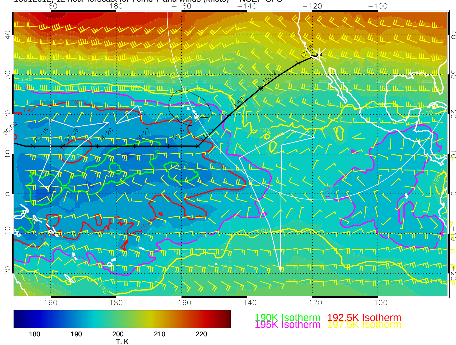
15012012, 12 hour forecast for 70mb T and winds (knots) -- NCEP GFS
