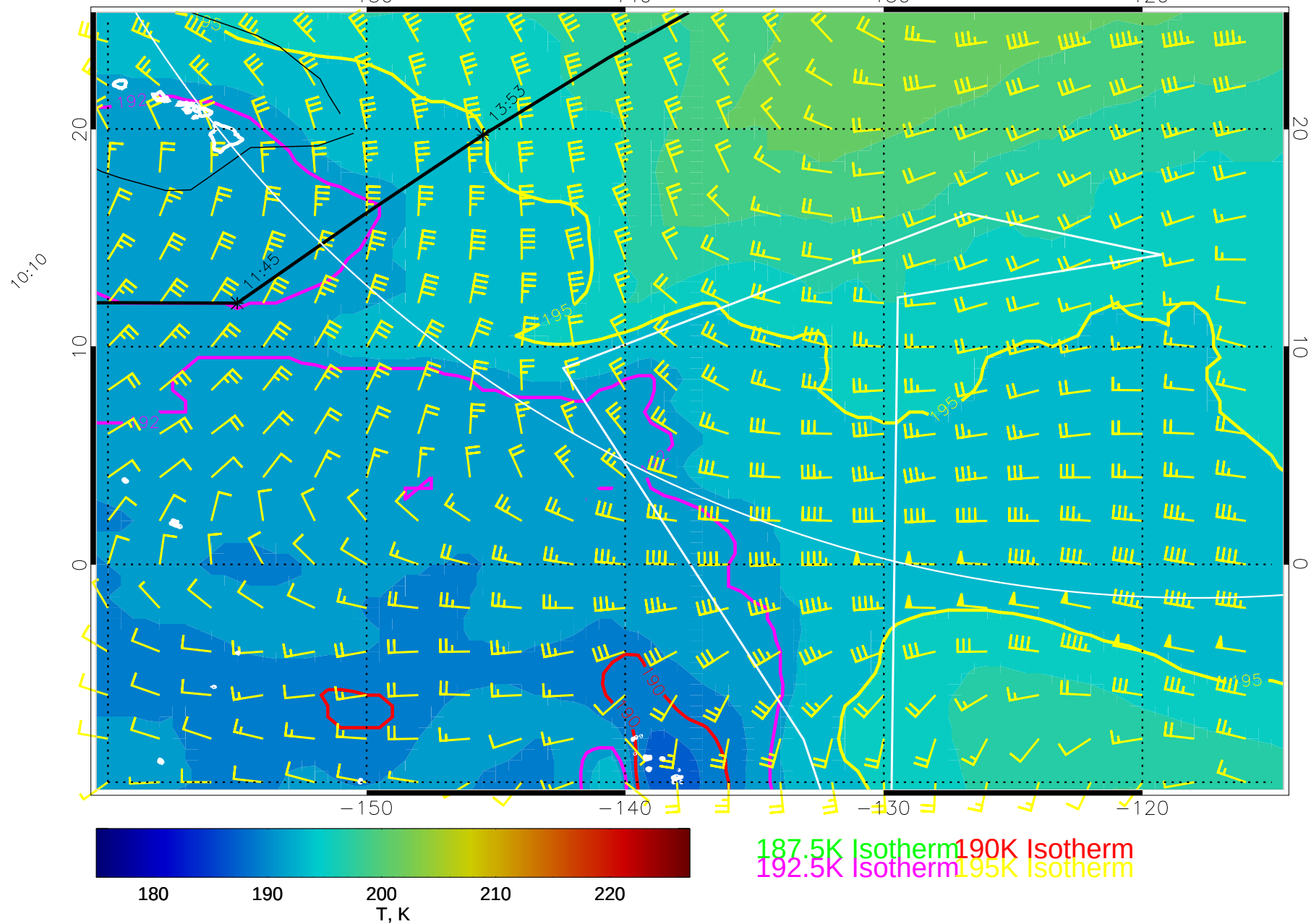
15012112, 36 hour forecast for 100mb T and winds (knots) -- NCEP GFS
