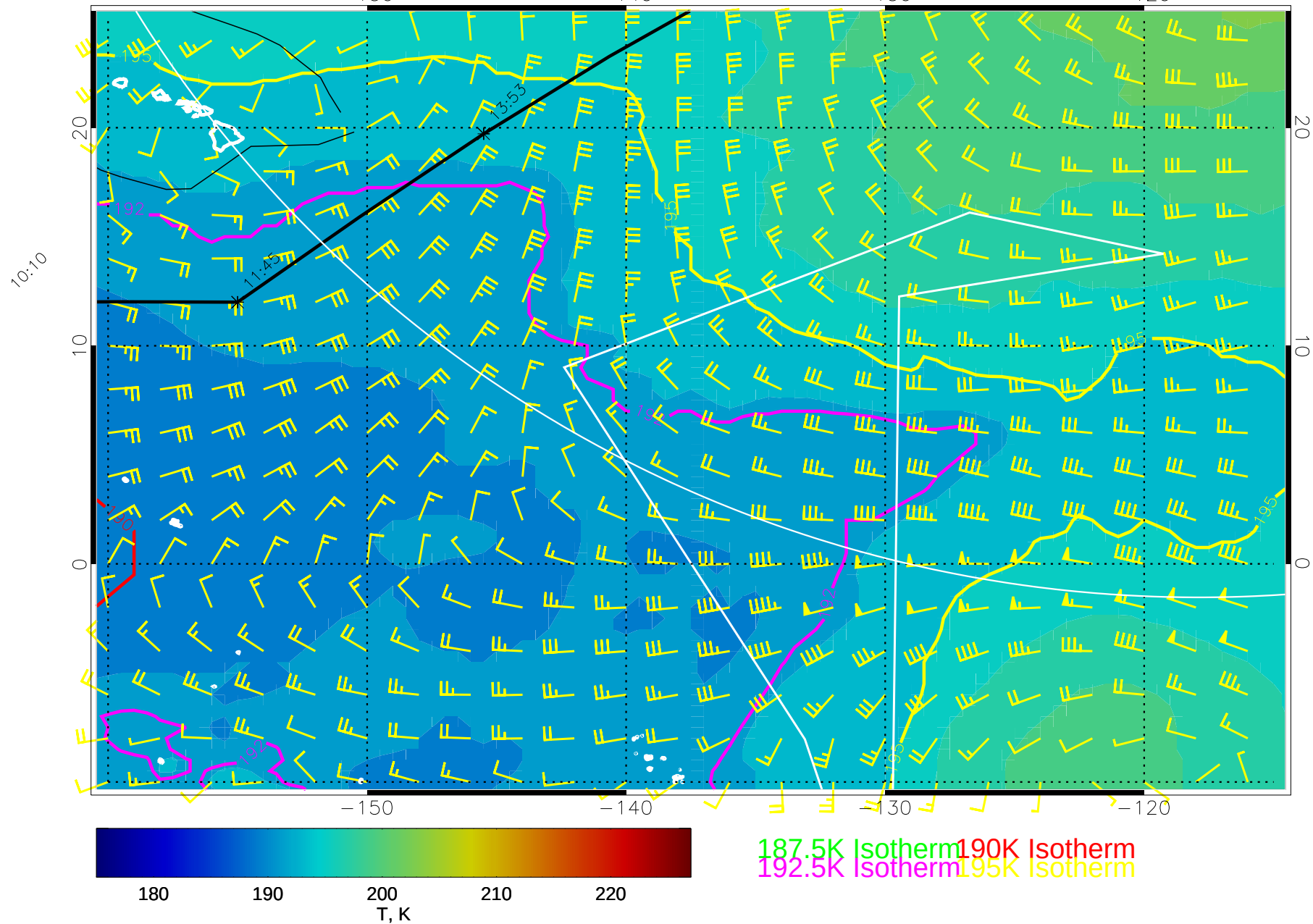
15012212, 60 hour forecast for 100mb T and winds (knots) -- NCEP GFS
