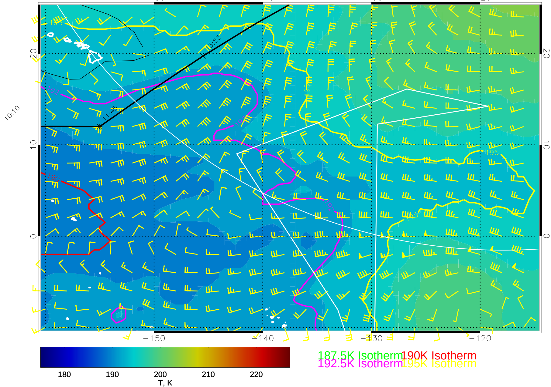
15012218, 66 hour forecast for 100mb T and winds (knots) -- NCEP GFS
