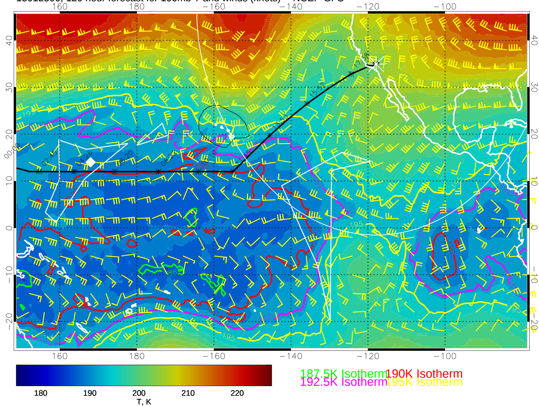
15012500, 120 hour forecast for 100mb T and winds (knots) -- NCEP GFS
