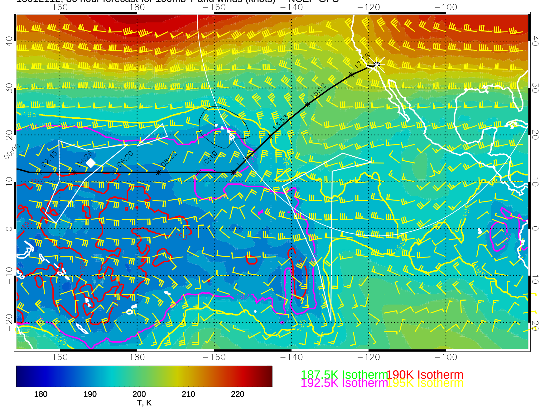
15012112, 36 hour forecast for 100mb T and winds (knots) -- NCEP GFS
