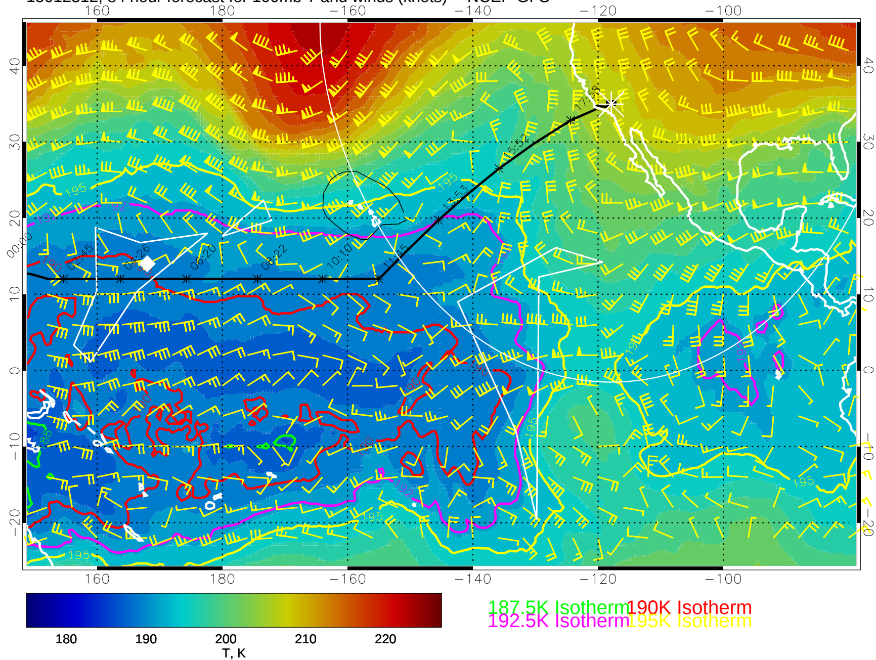
15012312, 84 hour forecast for 100mb T and winds (knots) -- NCEP GFS
