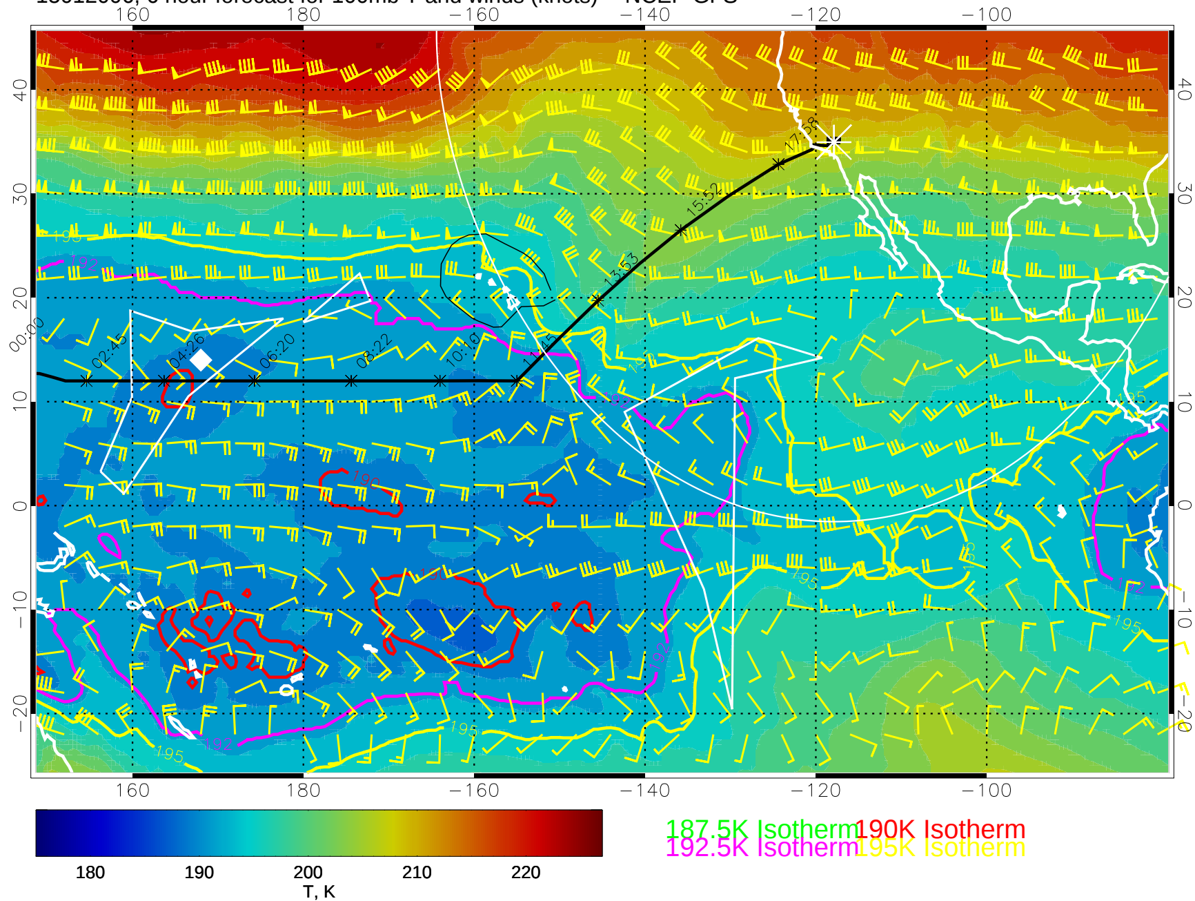
15012006, 6 hour forecast for 100mb T and winds (knots) -- NCEP GFS
