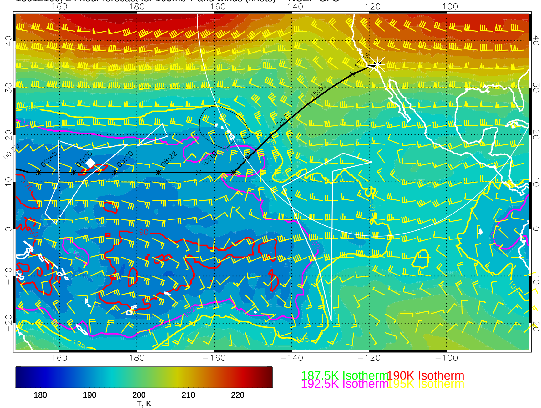
15012100, 24 hour forecast for 100mb T and winds (knots) -- NCEP GFS
