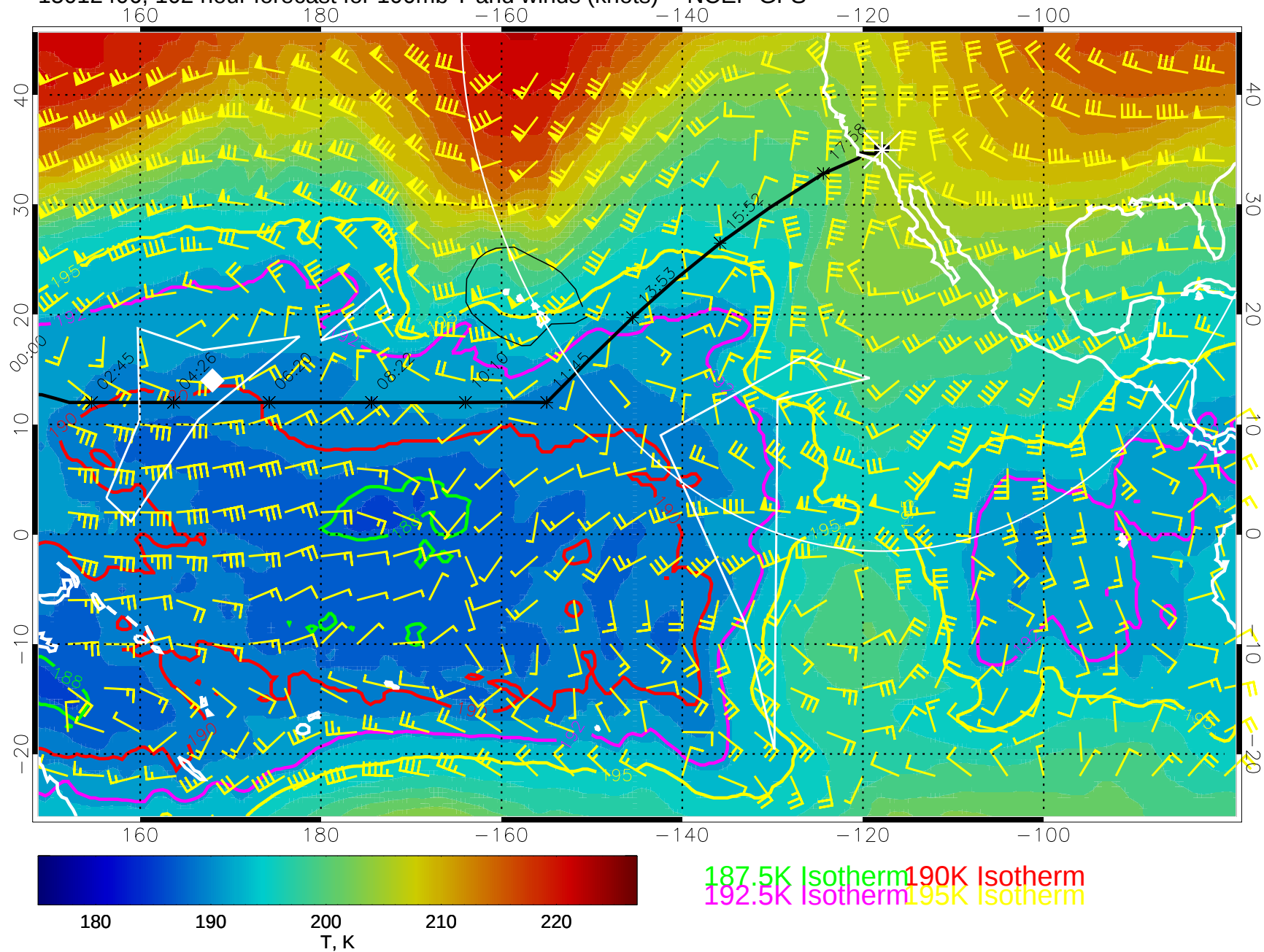
15012406, 102 hour forecast for 100mb T and winds (knots) -- NCEP GFS
