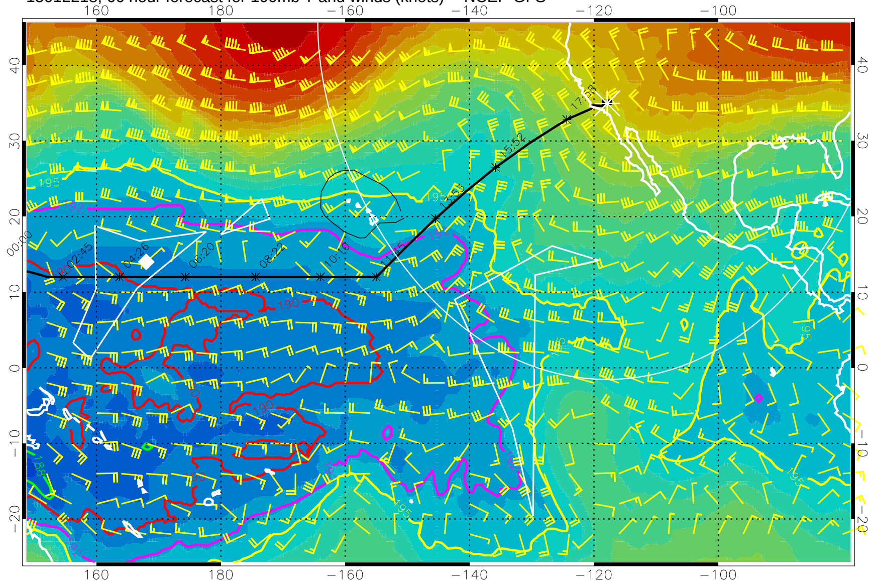
15012218, 66 hour forecast for 100mb T and winds (knots) -- NCEP GFS
