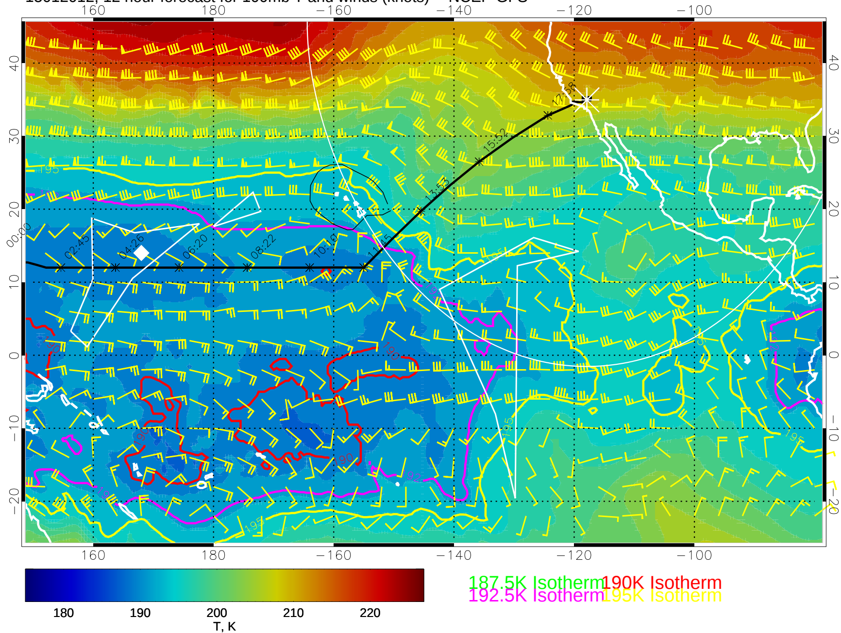
15012012, 12 hour forecast for 100mb T and winds (knots) -- NCEP GFS
