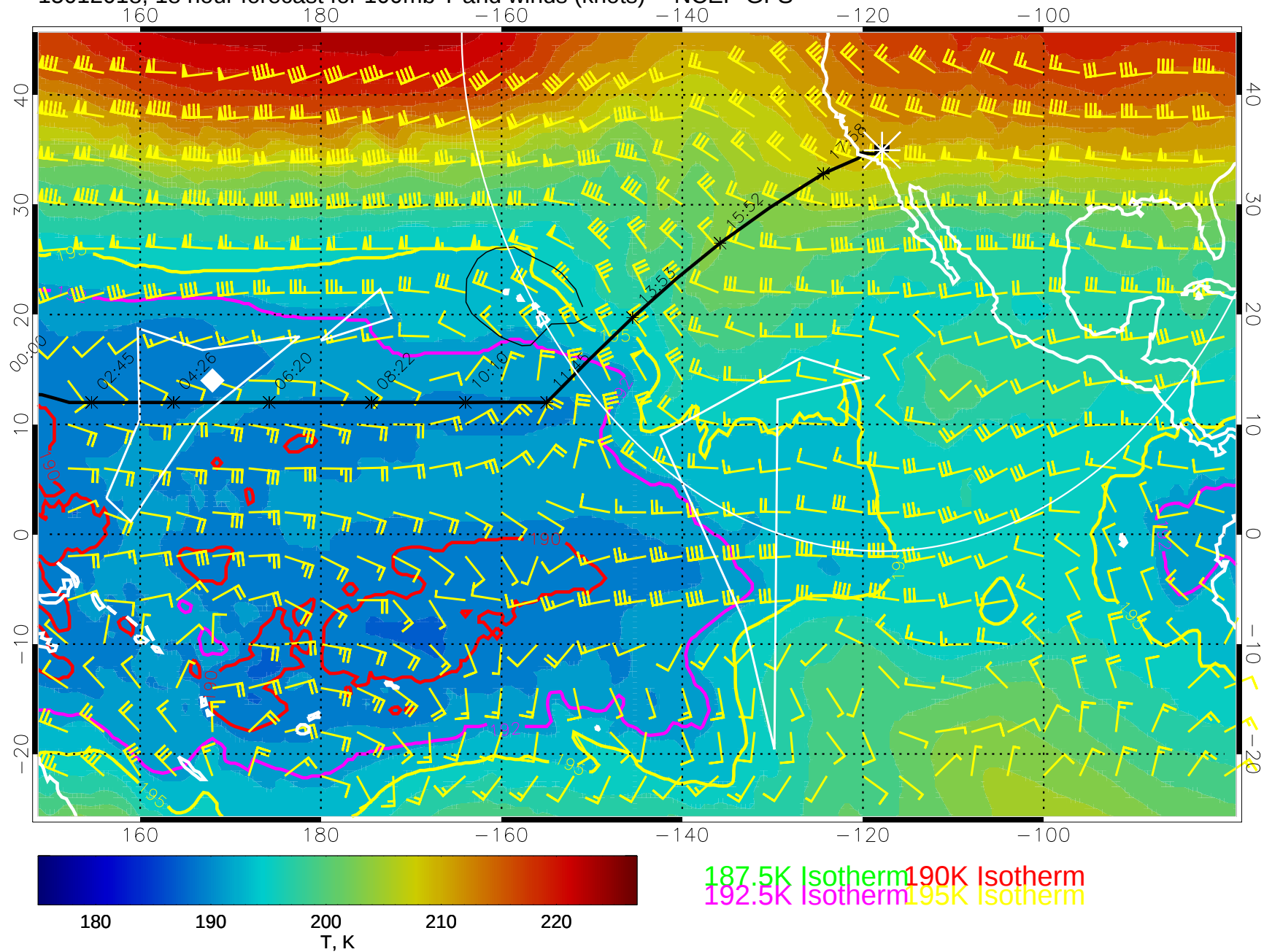
15012018, 18 hour forecast for 100mb T and winds (knots) -- NCEP GFS
