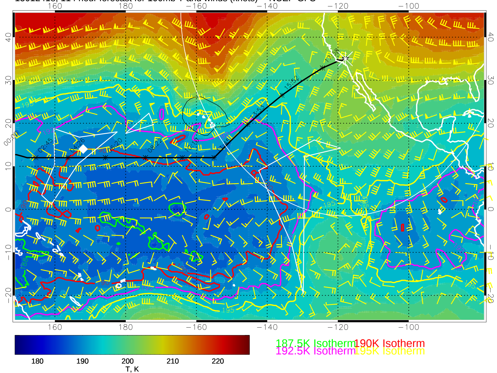
15012418, 114 hour forecast for 100mb T and winds (knots) -- NCEP GFS
