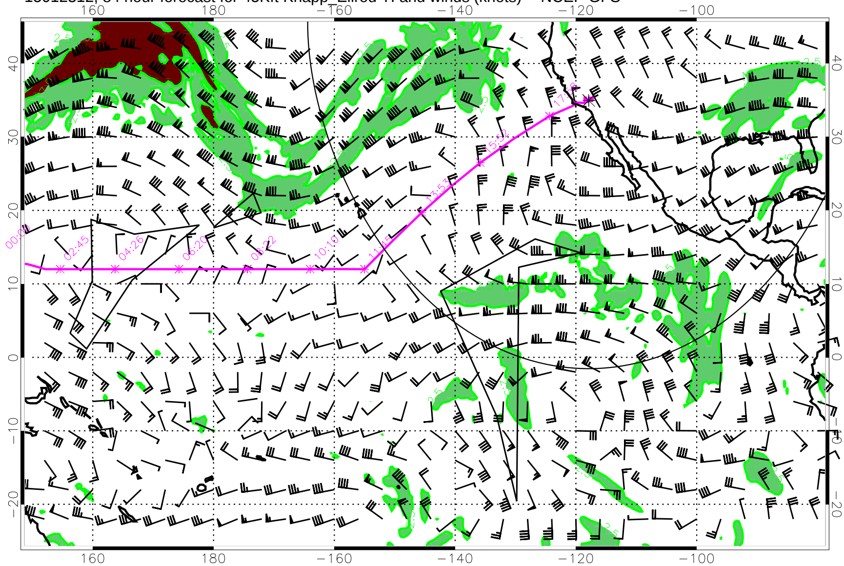
15012312, 84 hour forecast for 45Kft Knapp_Ellrod TI and winds (knots) -- NCEP GFS
