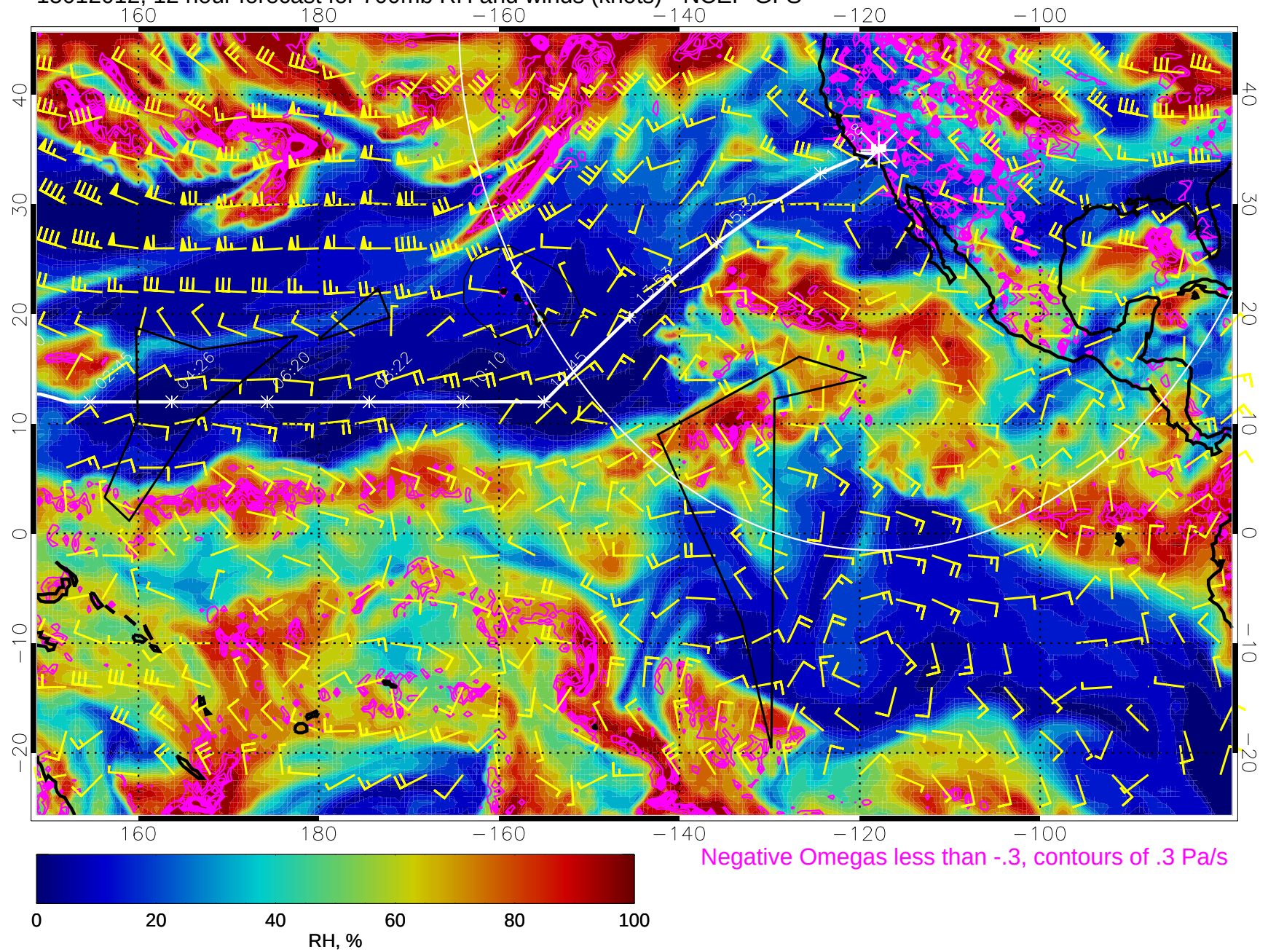
15012012, 12 hour forecast for 700mb RH and winds (knots) - NCEP GFS
