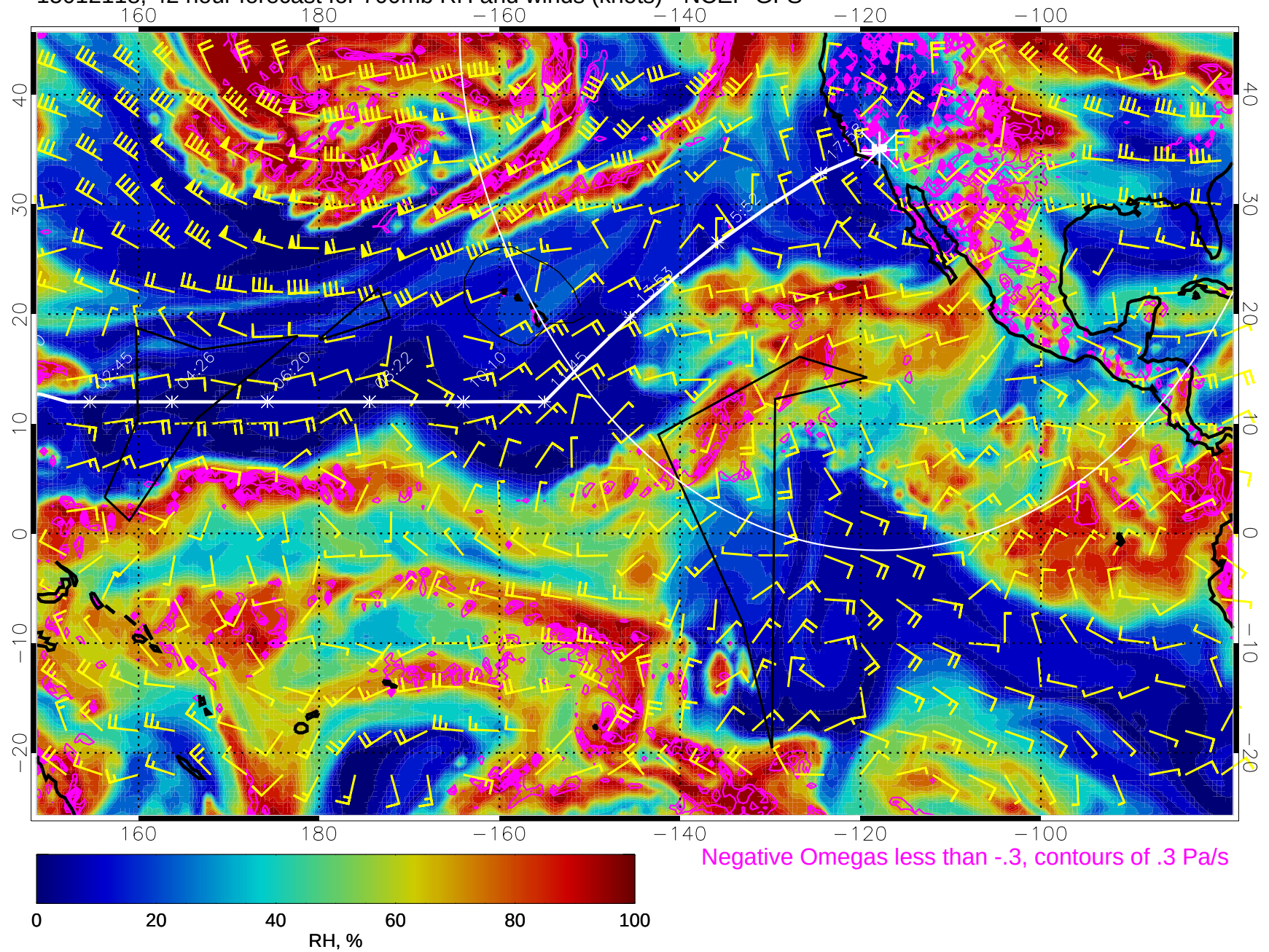
15012118, 42 hour forecast for 700mb RH and winds (knots) - NCEP GFS
