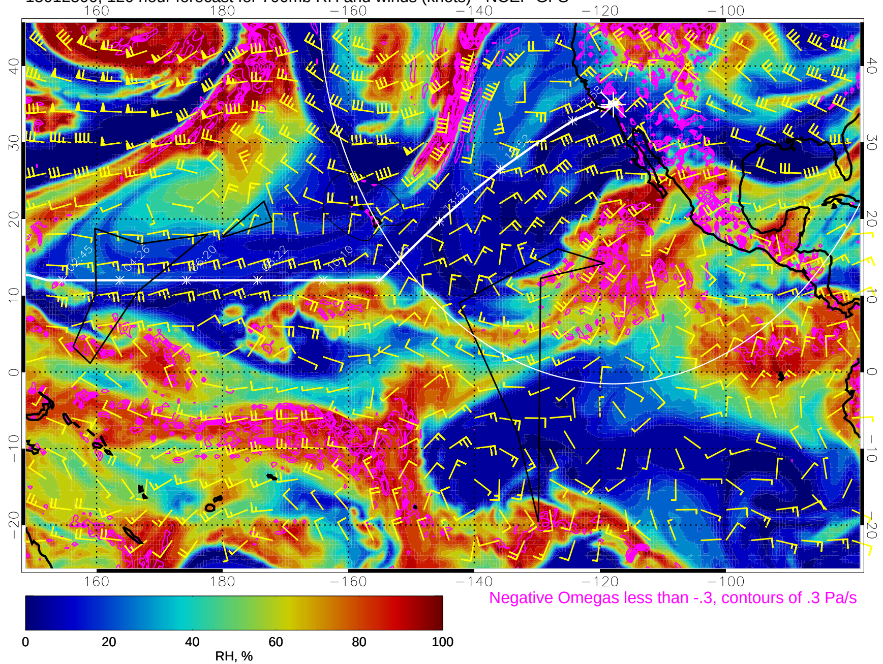
15012500, 120 hour forecast for 700mb RH and winds (knots) - NCEP GFS
