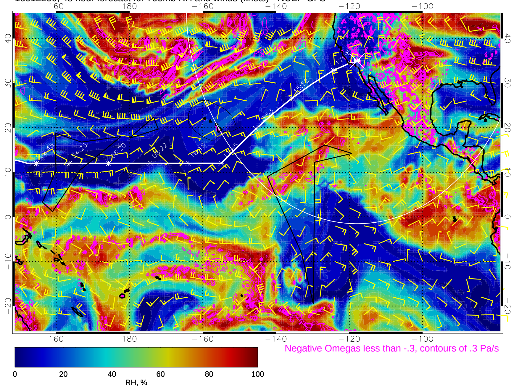
15012200, 48 hour forecast for 700mb RH and winds (knots) - NCEP GFS
