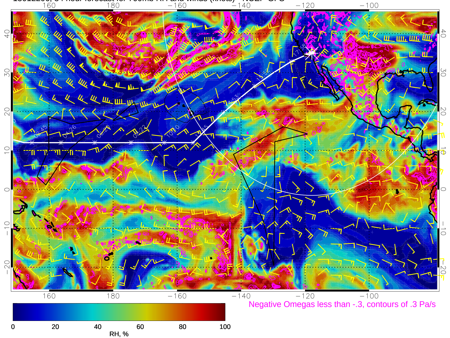
15012206, 54 hour forecast for 700mb RH and winds (knots) - NCEP GFS
