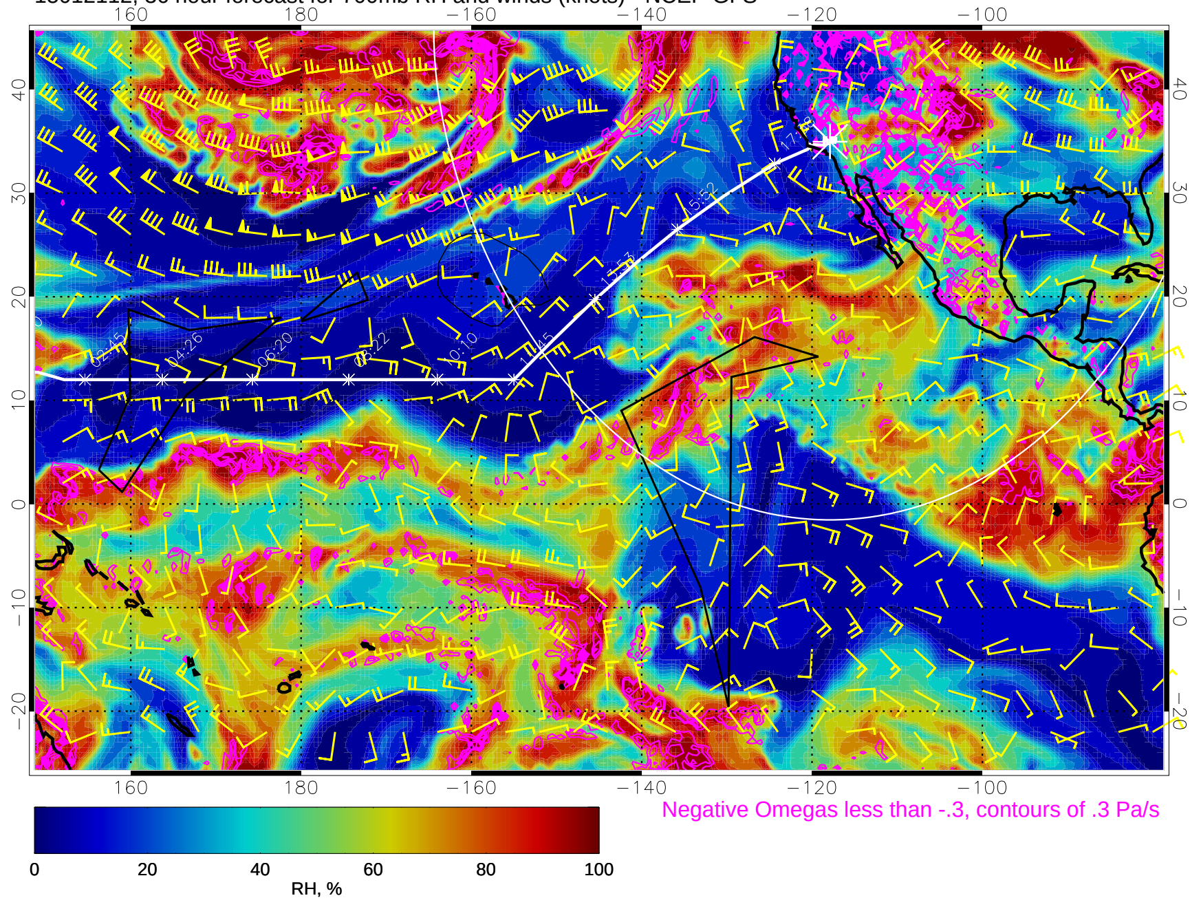
15012112, 36 hour forecast for 700mb RH and winds (knots) - NCEP GFS
