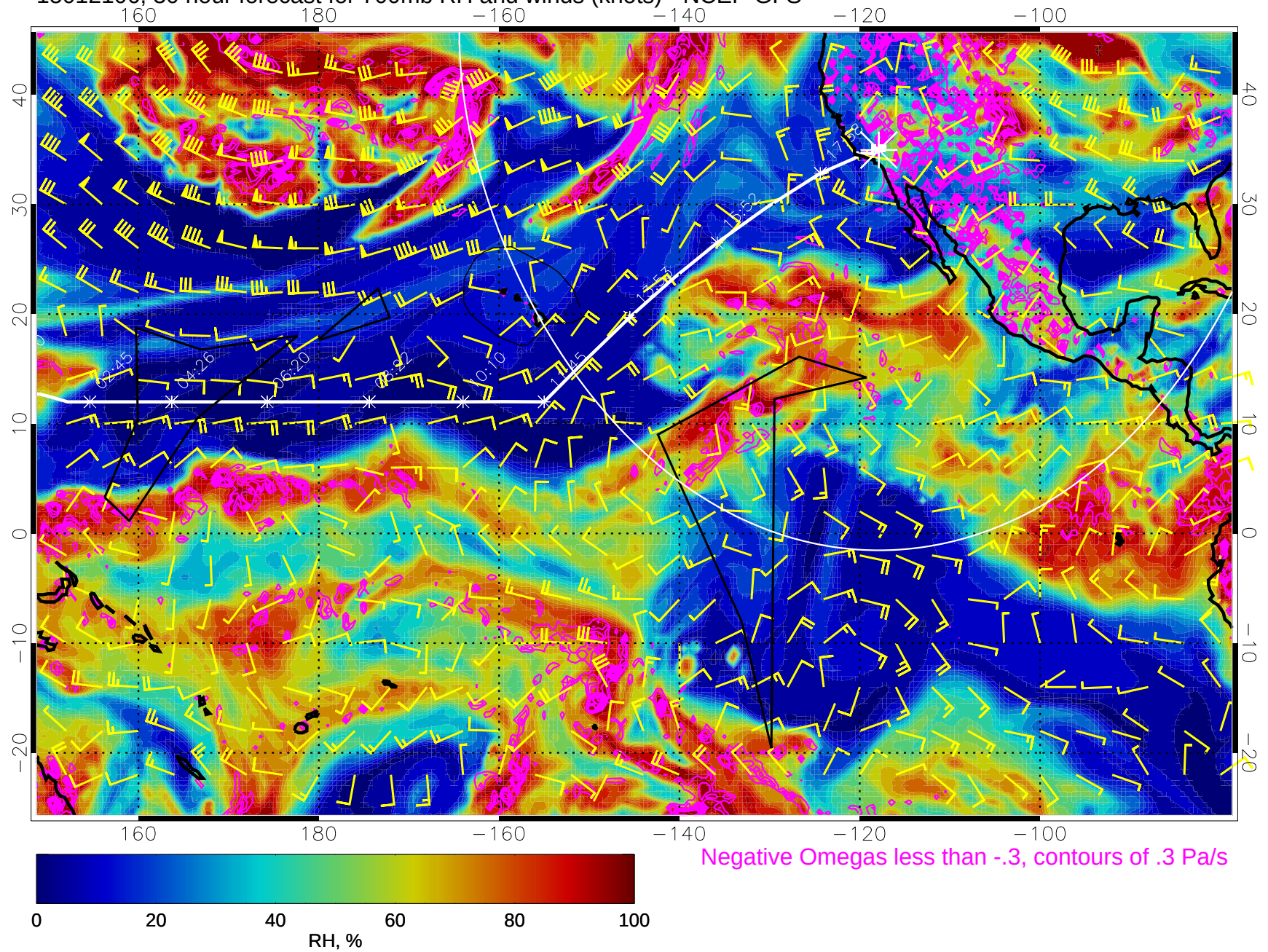
15012106, 30 hour forecast for 700mb RH and winds (knots) - NCEP GFS
