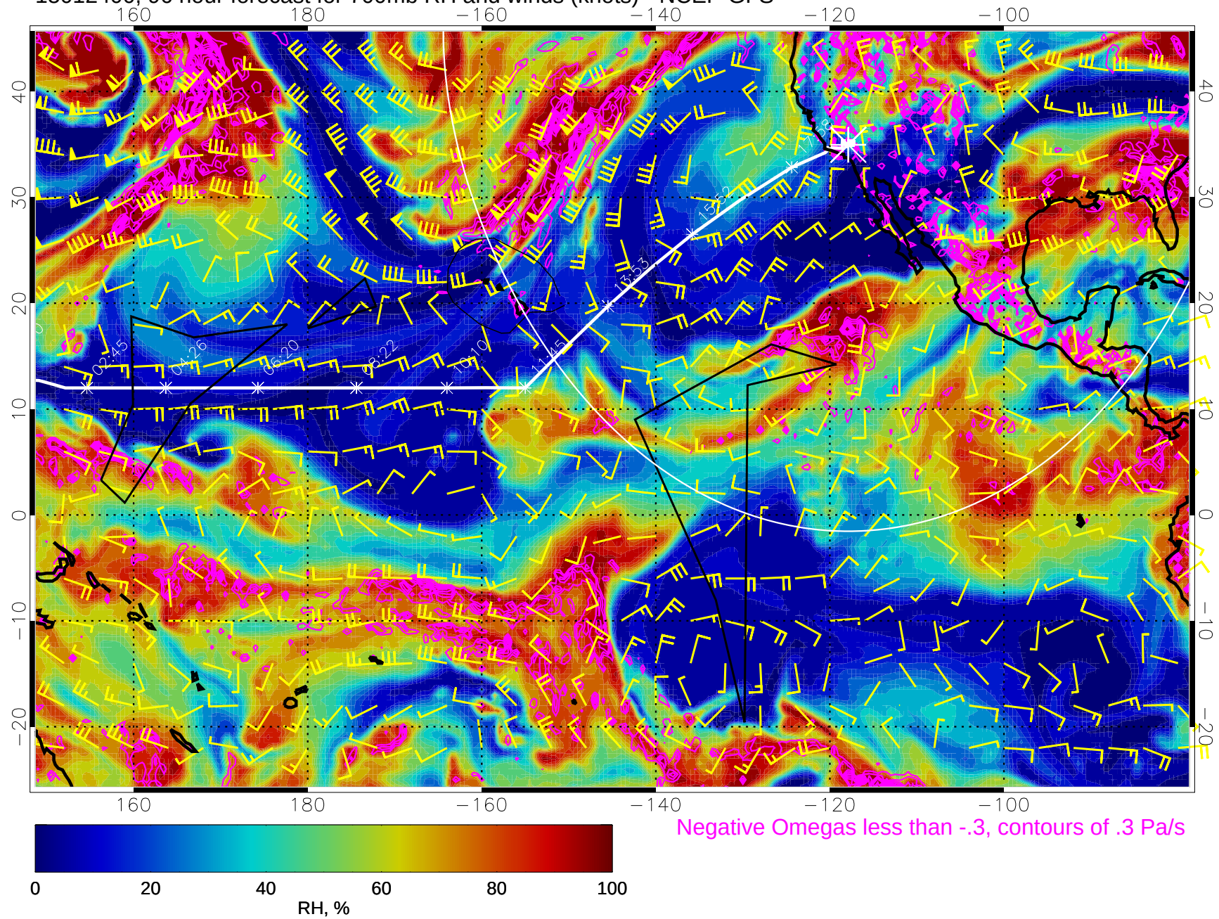
15012400, 96 hour forecast for 700mb RH and winds (knots) - NCEP GFS
