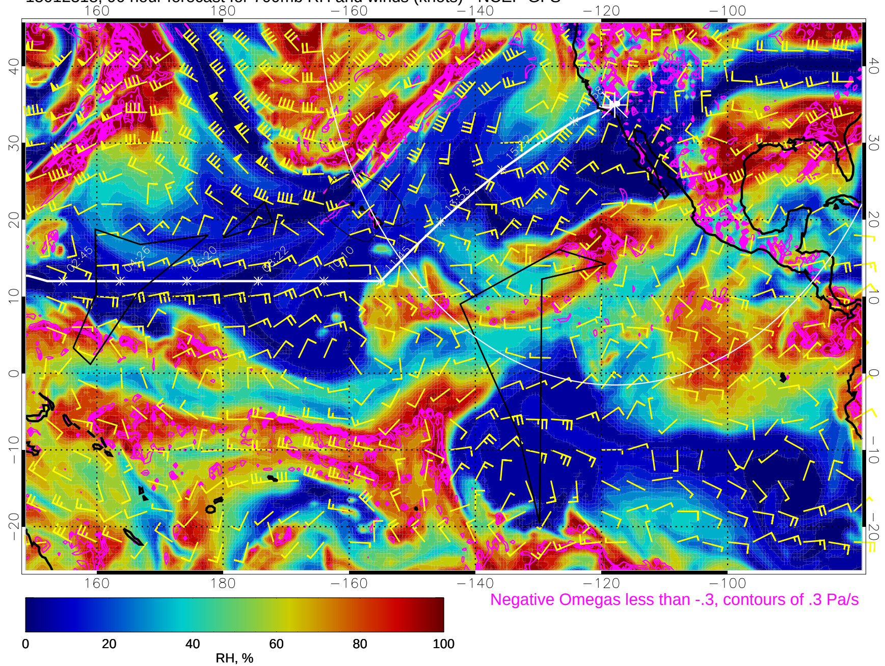
15012318, 90 hour forecast for 700mb RH and winds (knots) - NCEP GFS
