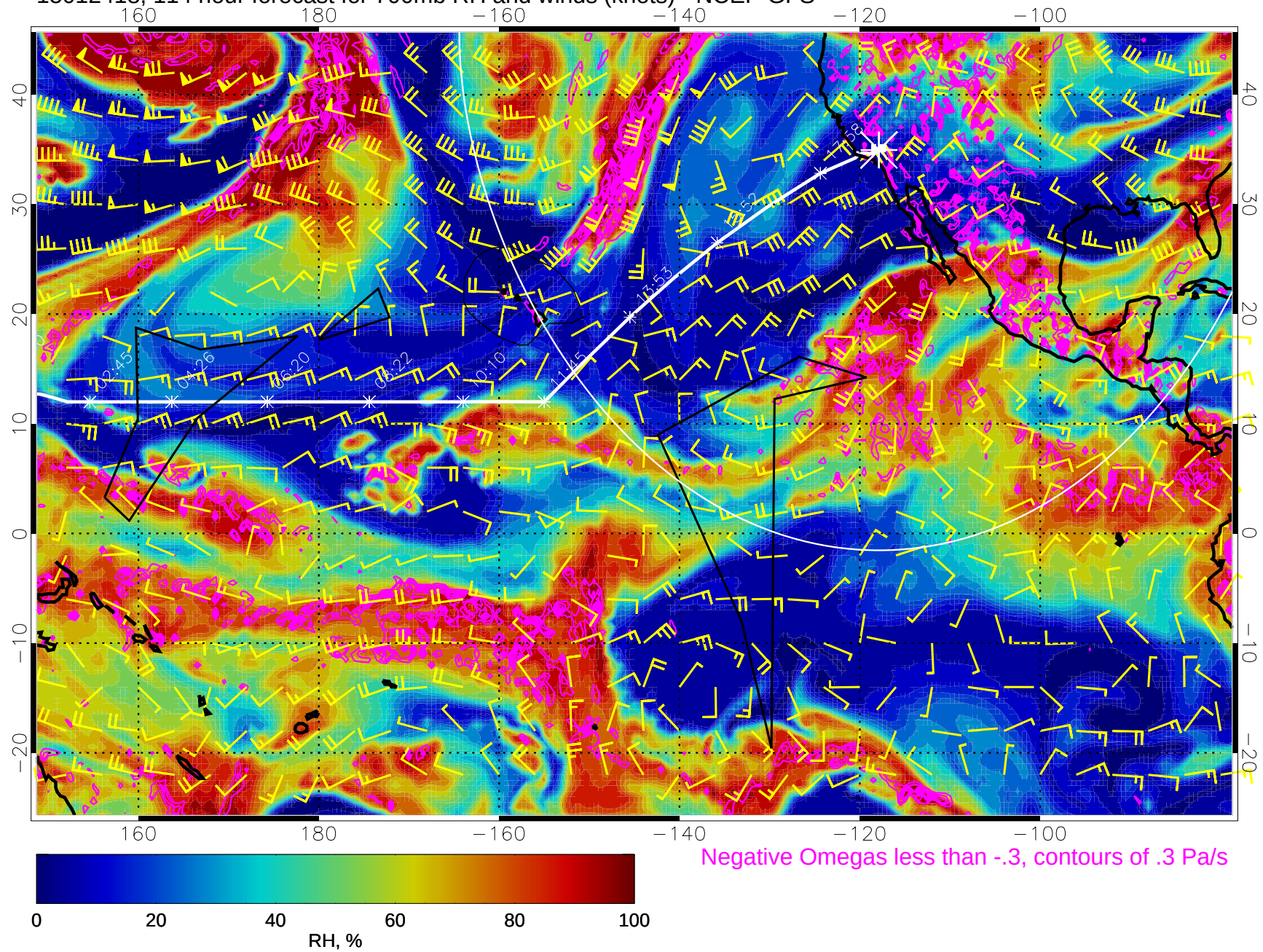
15012418, 114 hour forecast for 700mb RH and winds (knots) - NCEP GFS
