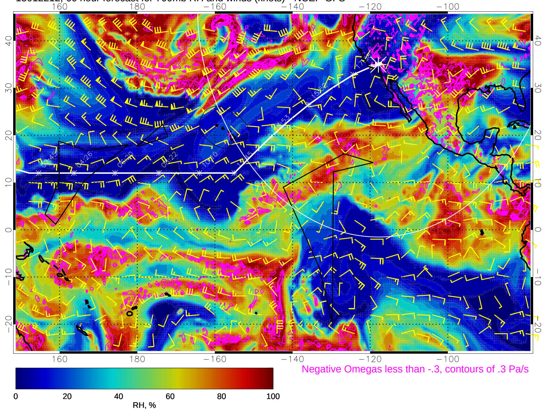
15012212, 60 hour forecast for 700mb RH and winds (knots) - NCEP GFS
