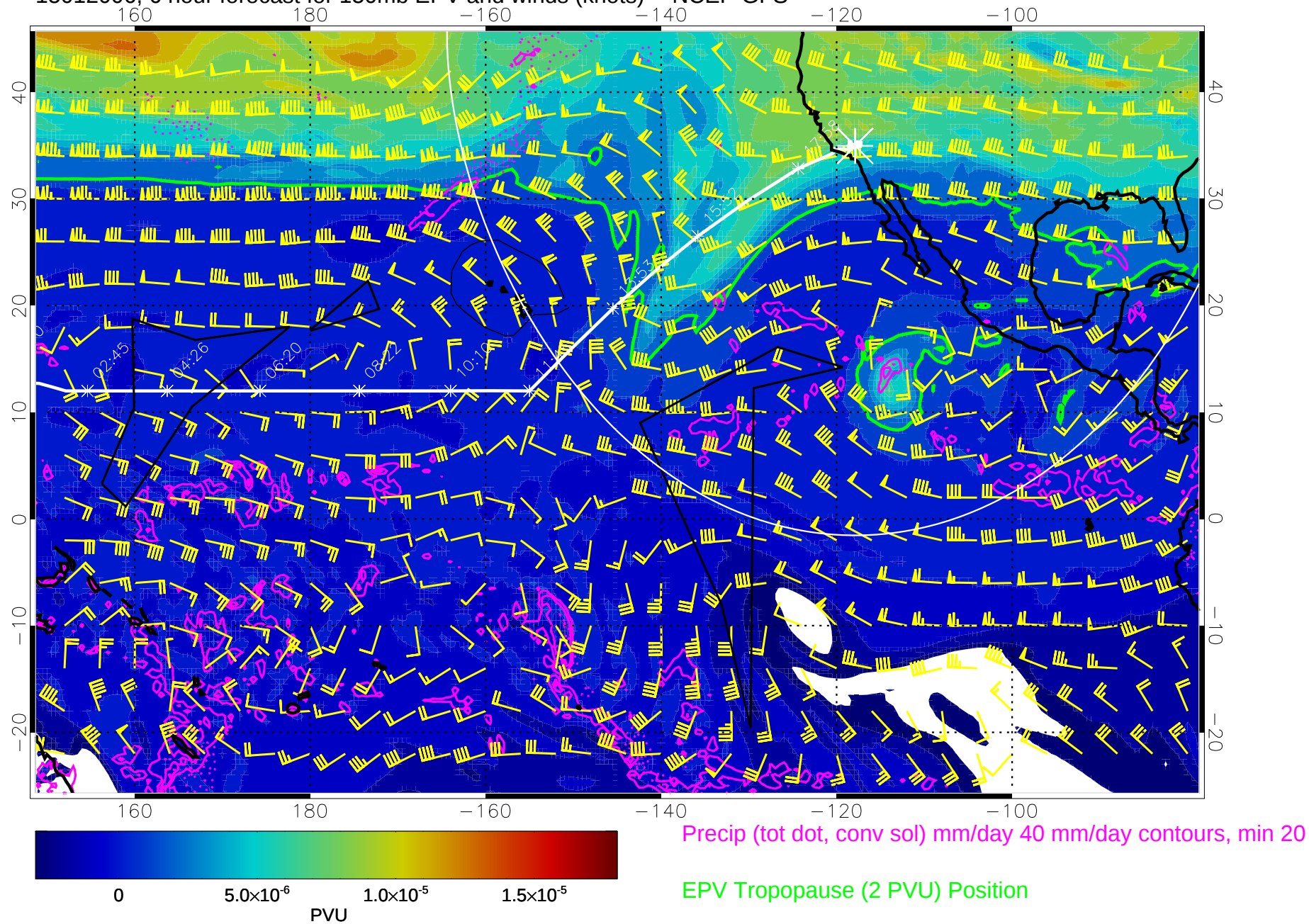
15012006, 6 hour forecast for 150mb EPV and winds (knots) -- NCEP GFS
