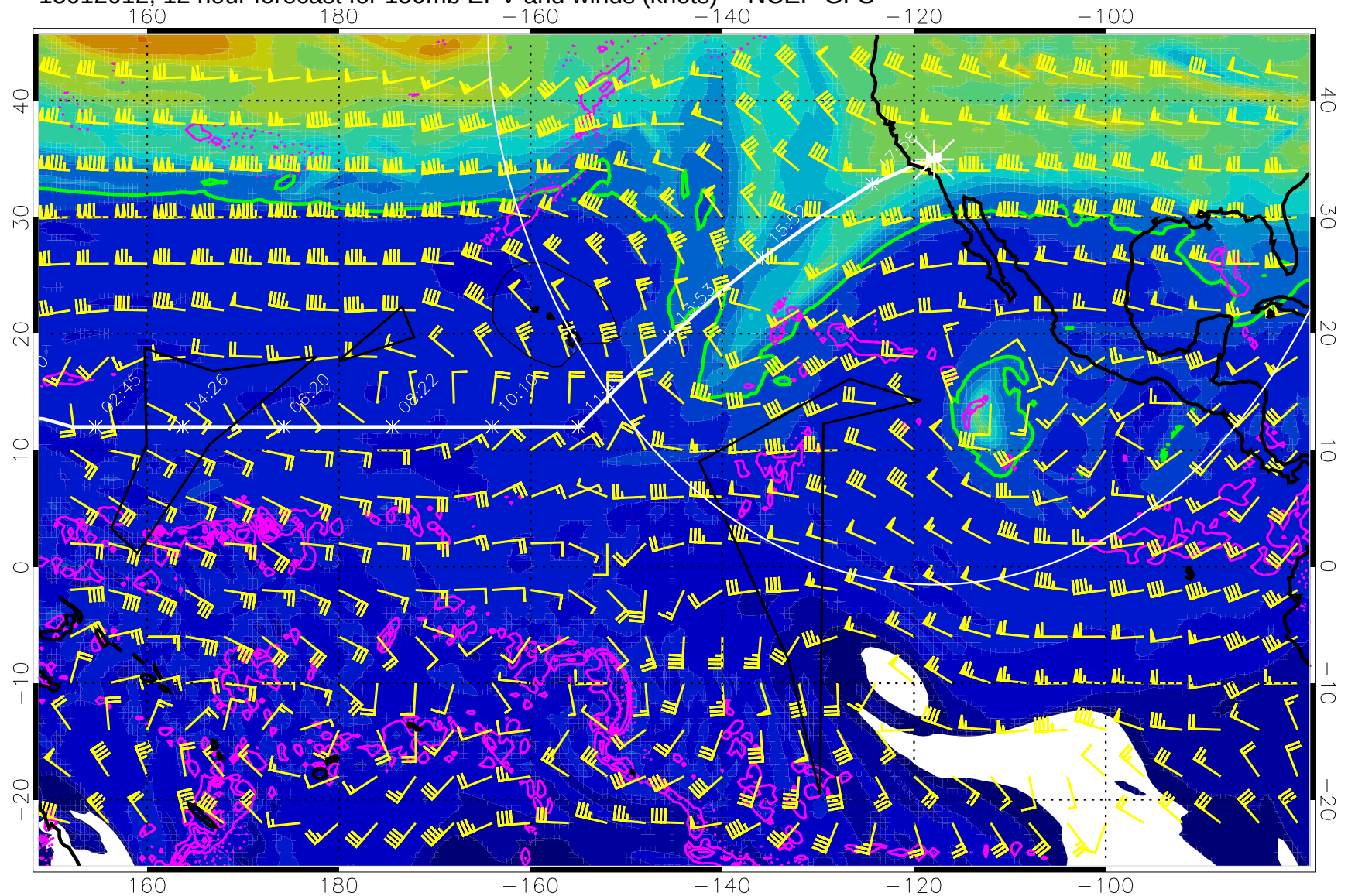
15012012, 12 hour forecast for 150mb EPV and winds (knots) -- NCEP GFS
