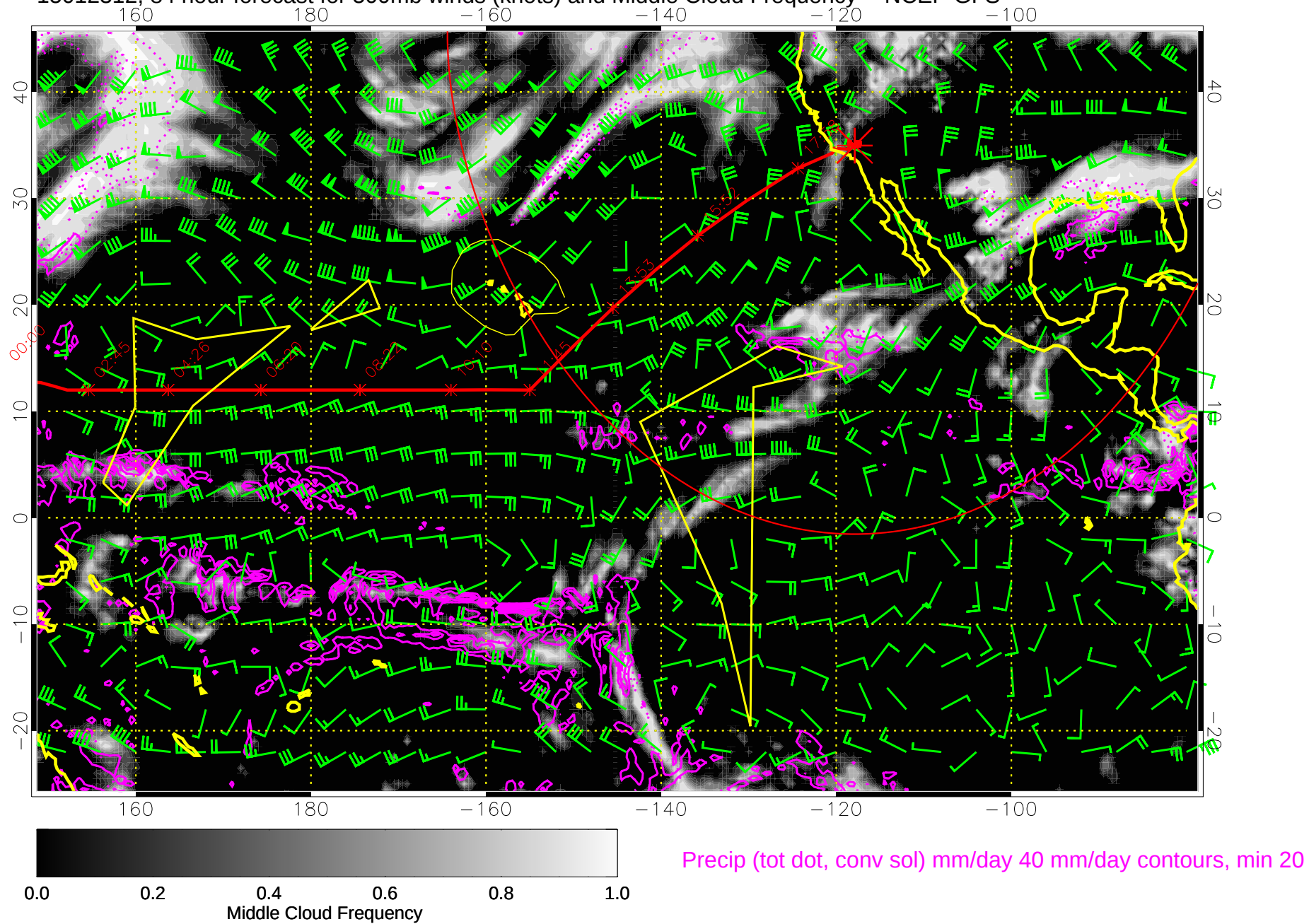
15012312, 84 hour forecast for 500mb winds (knots) and Middle Cloud Frequency -- NCEP GFS
