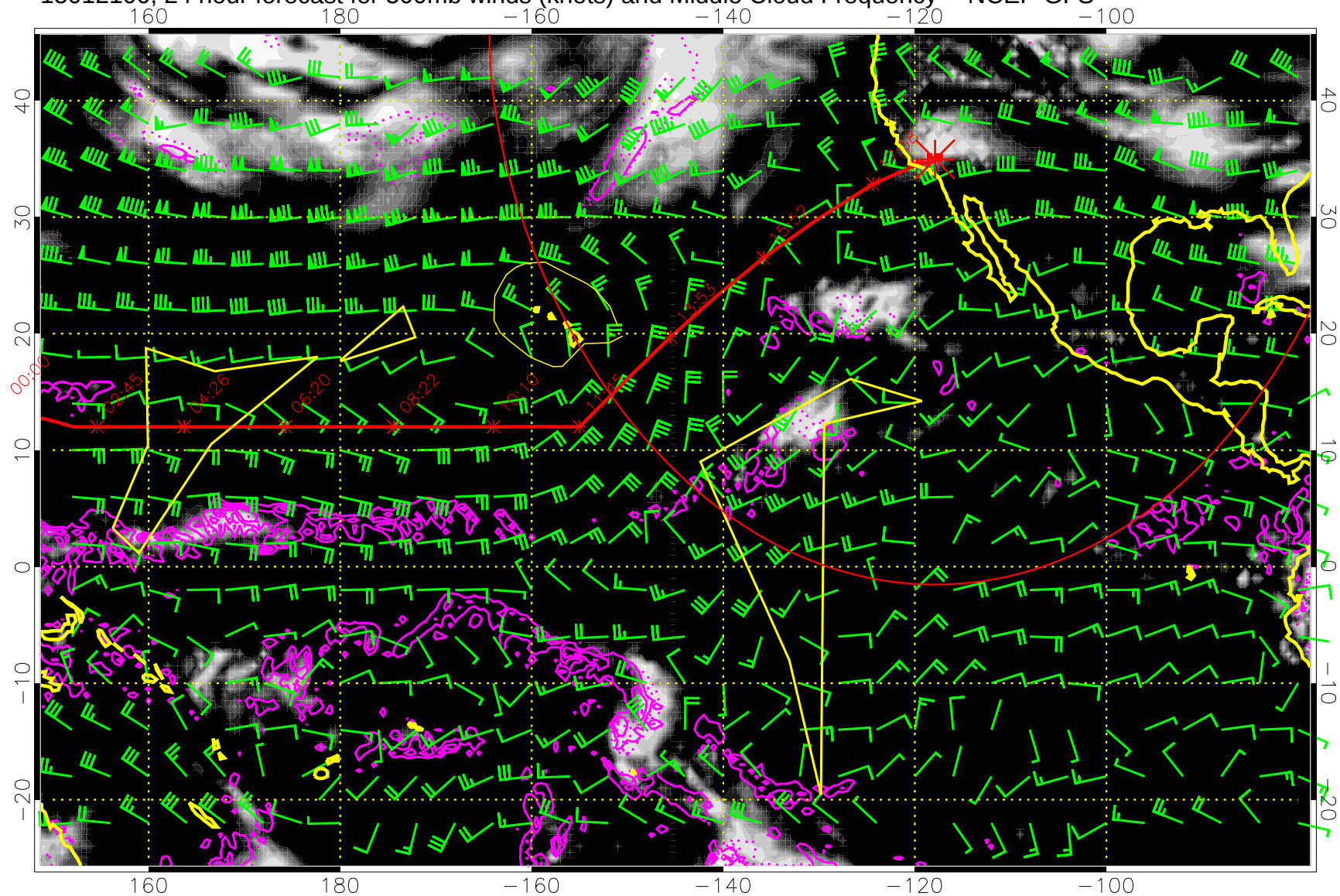
15012100, 24 hour forecast for 500mb winds (knots) and Middle Cloud Frequency -- NCEP GFS
