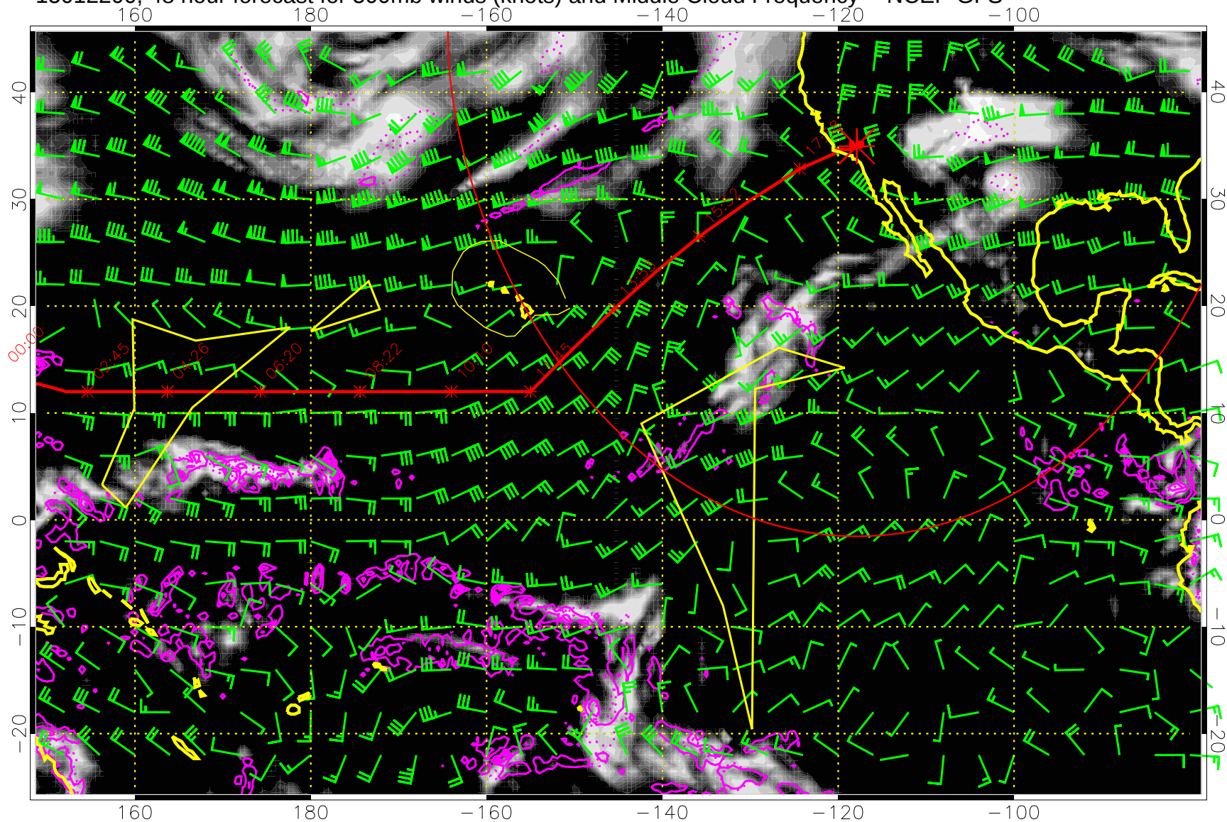
15012200, 48 hour forecast for 500mb winds (knots) and Middle Cloud Frequency -- NCEP GFS
