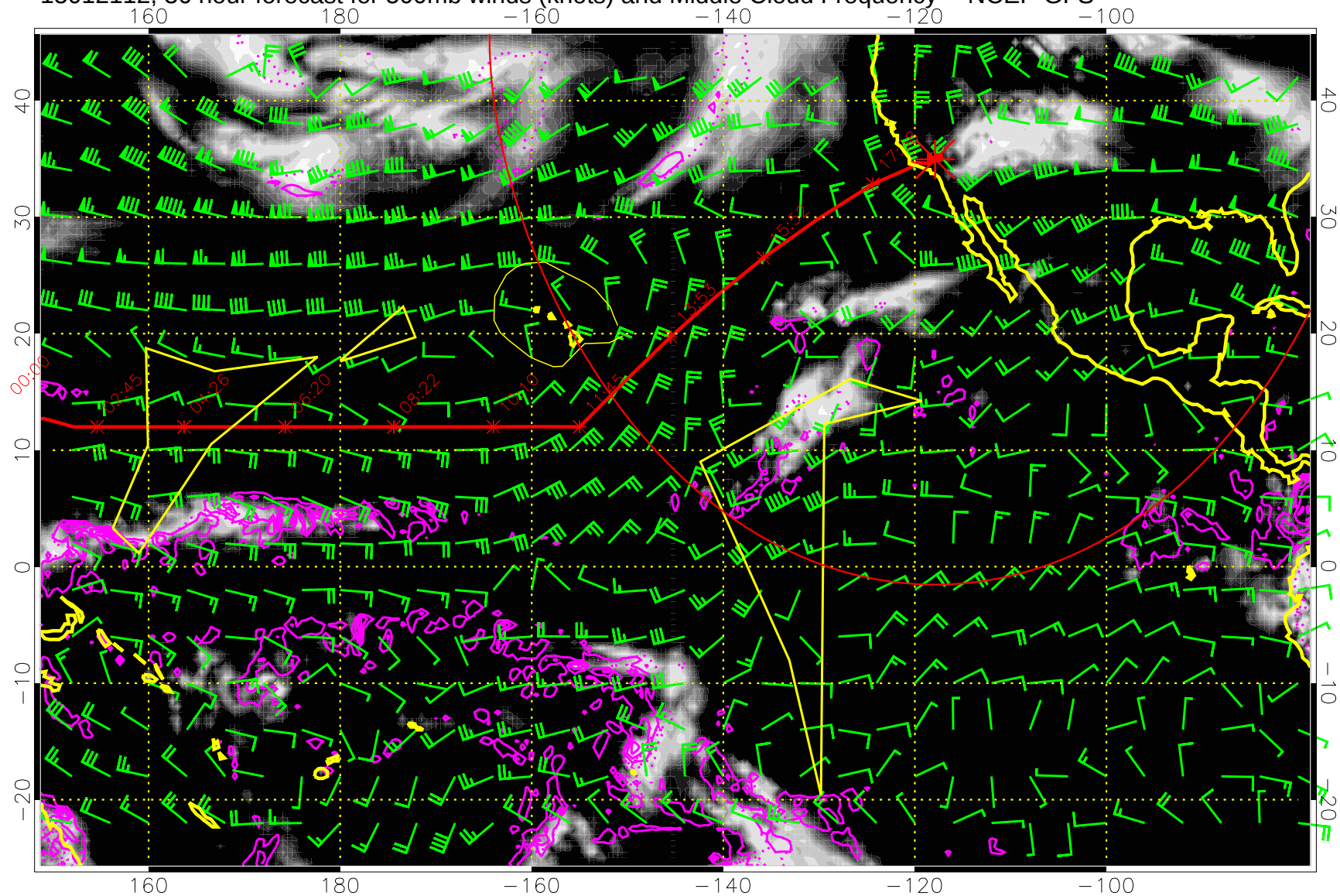
15012112, 36 hour forecast for 500mb winds (knots) and Middle Cloud Frequency -- NCEP GFS
