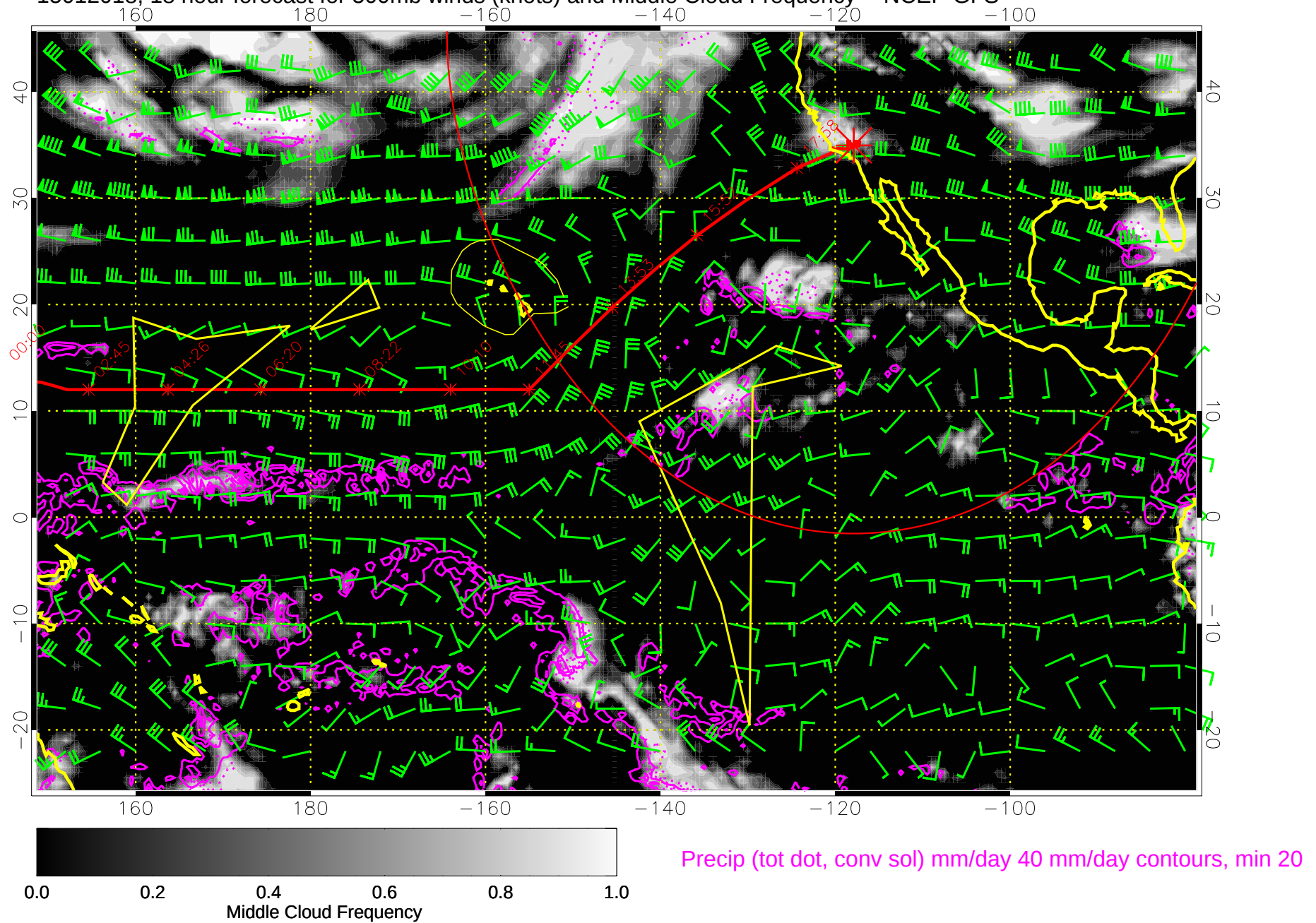
15012018, 18 hour forecast for 500mb winds (knots) and Middle Cloud Frequency -- NCEP GFS
