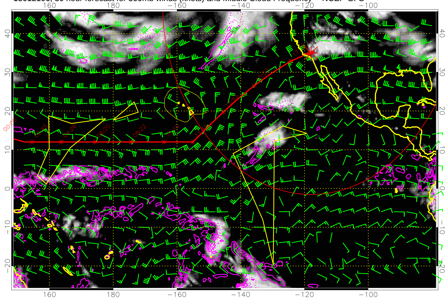
15012106, 30 hour forecast for 500mb winds (knots) and Middle Cloud Frequency -- NCEP GFS
