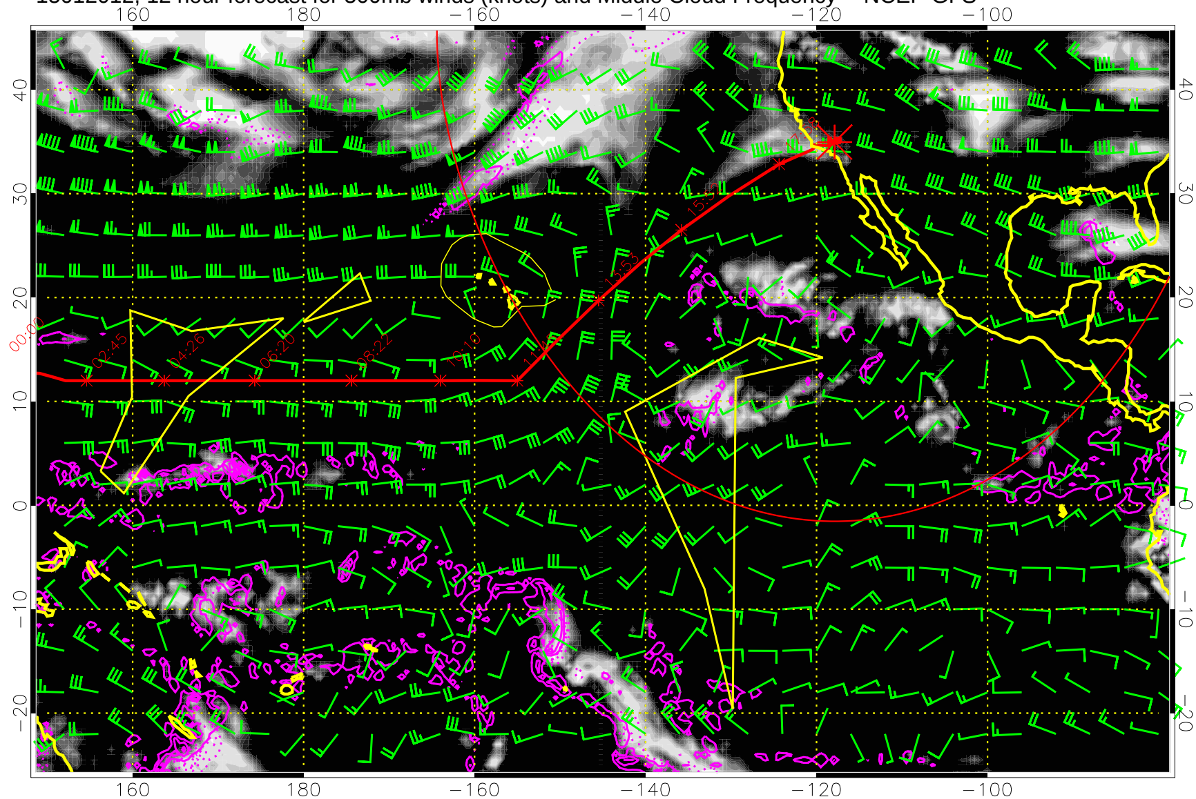
15012012, 12 hour forecast for 500mb winds (knots) and Middle Cloud Frequency -- NCEP GFS
