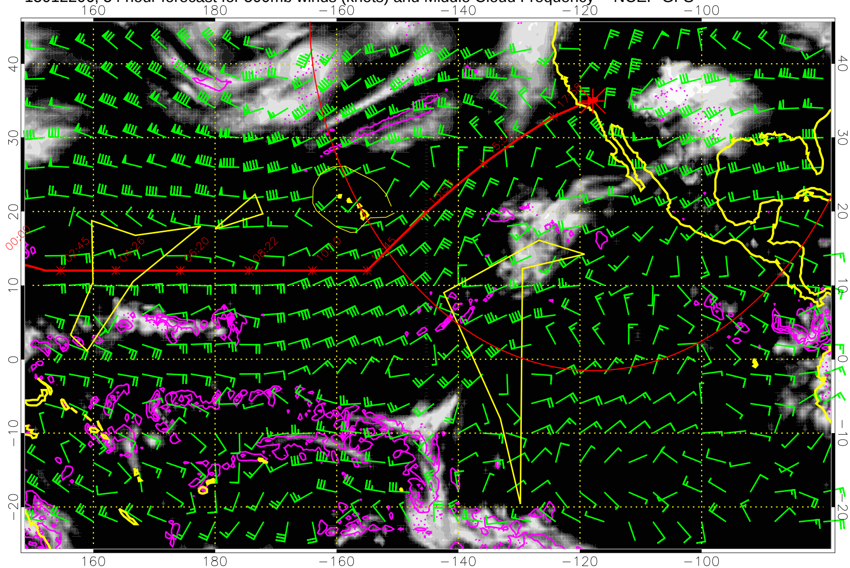
15012206, 54 hour forecast for 500mb winds (knots) and Middle Cloud Frequency -- NCEP GFS
