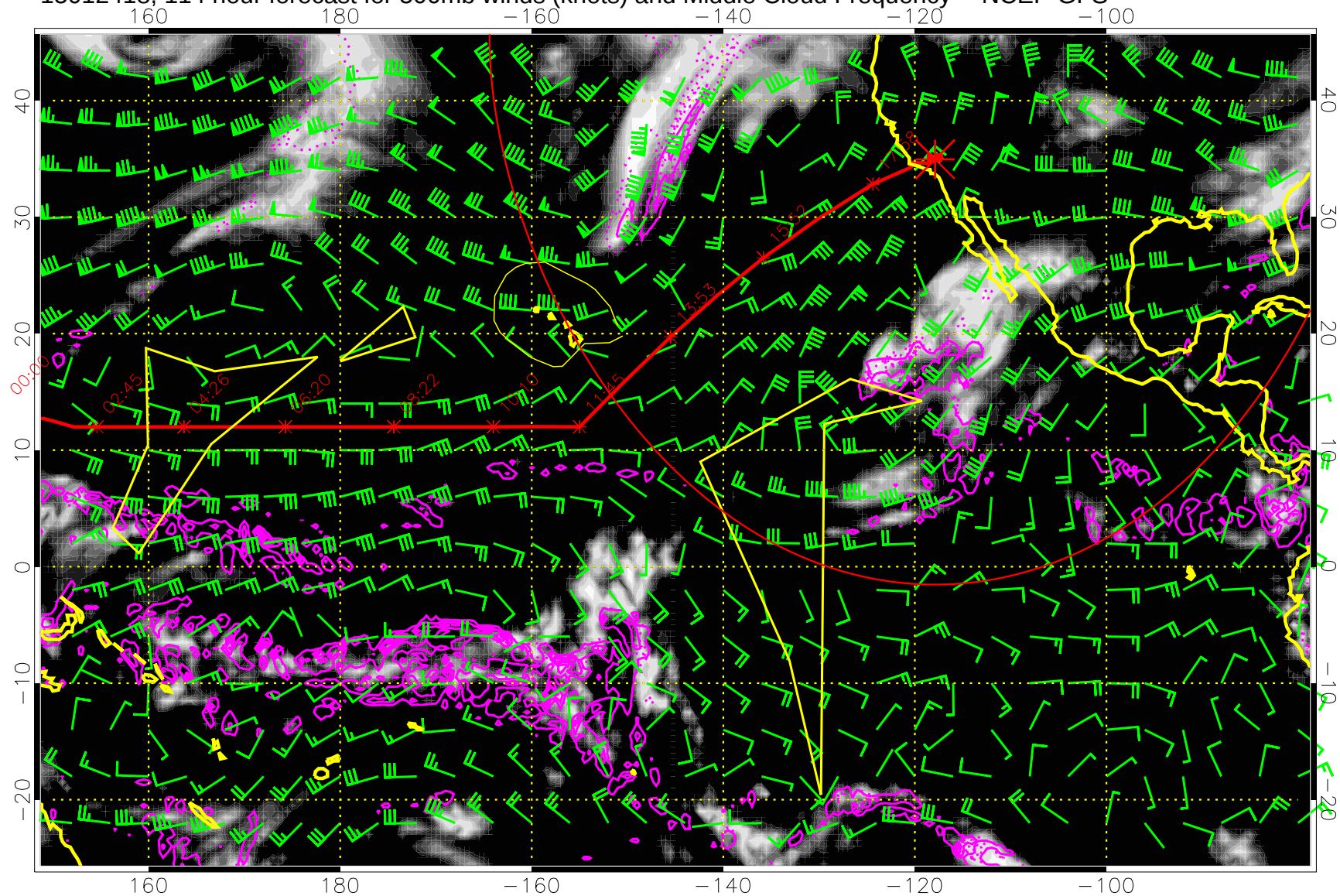
15012418, 114 hour forecast for 500mb winds (knots) and Middle Cloud Frequency -- NCEP GFS
