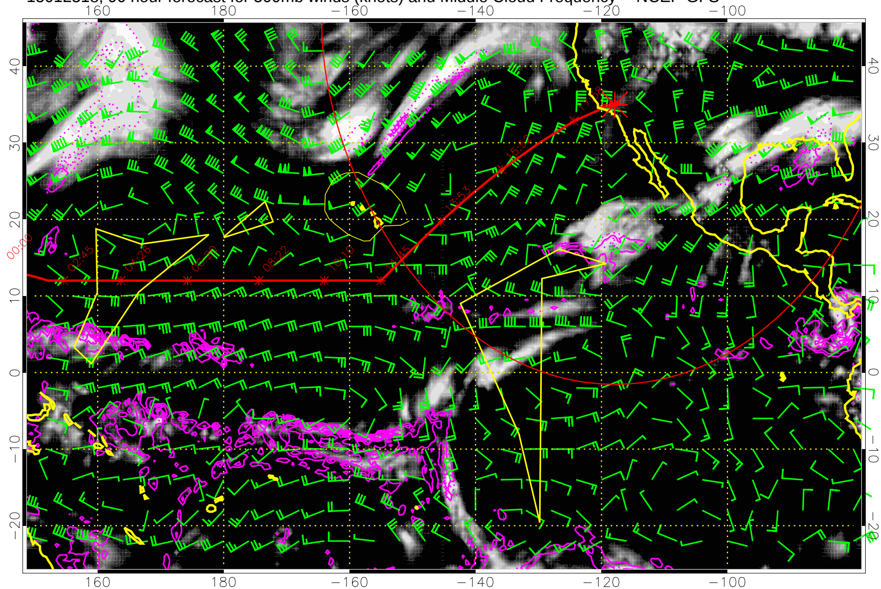
15012318, 90 hour forecast for 500mb winds (knots) and Middle Cloud Frequency -- NCEP GFS
