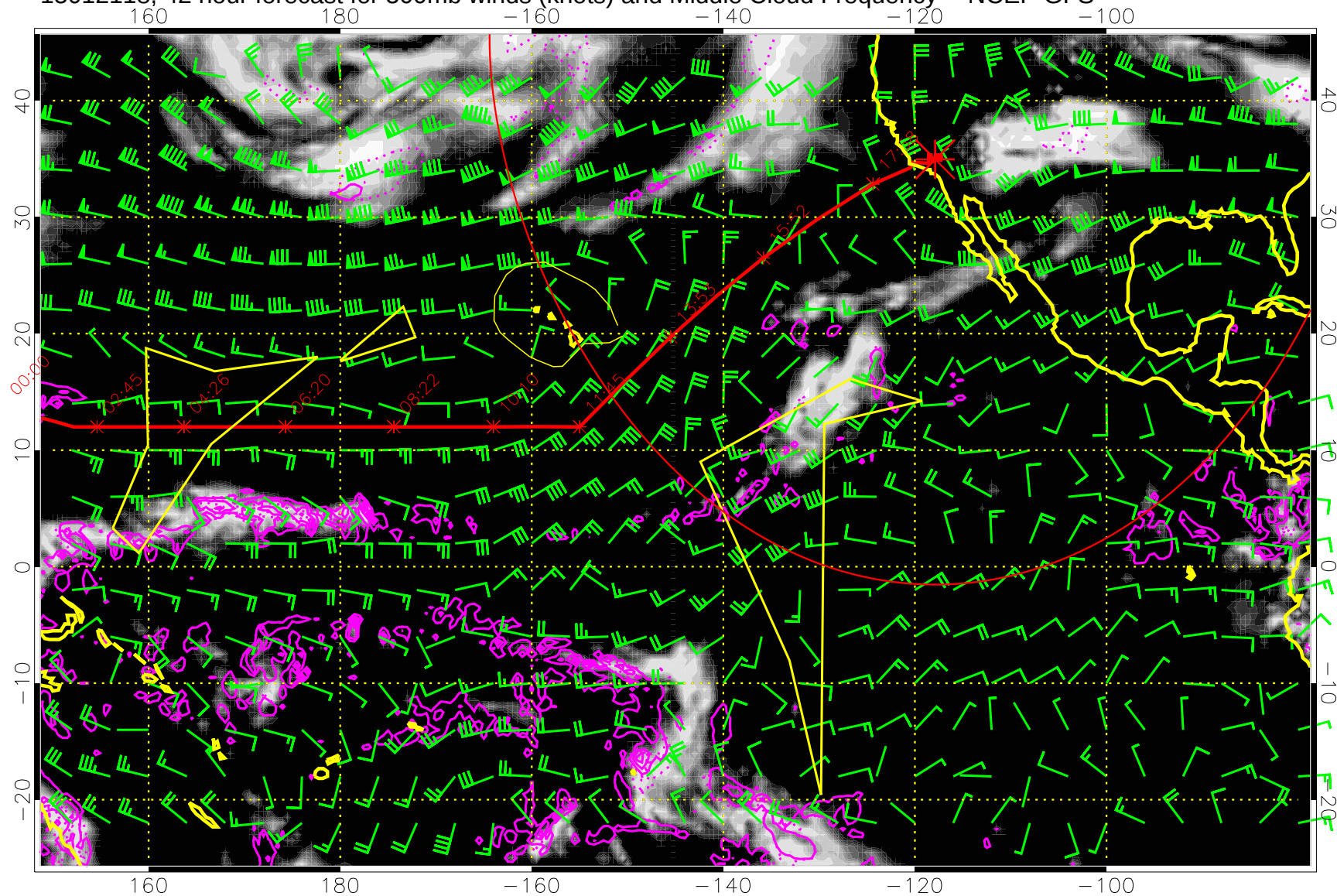
15012118, 42 hour forecast for 500mb winds (knots) and Middle Cloud Frequency -- NCEP GFS
