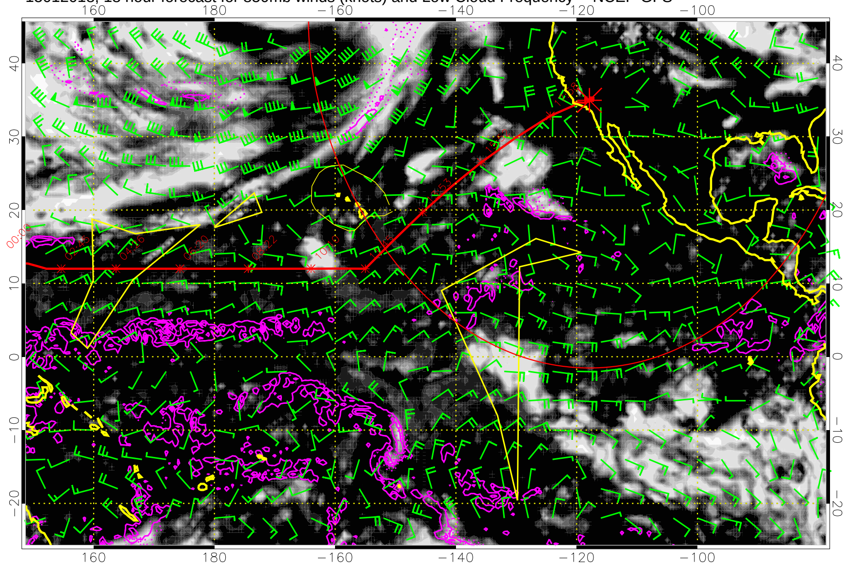
15012018, 18 hour forecast for 850mb winds (knots) and Low Cloud Frequency -- NCEP GFS
