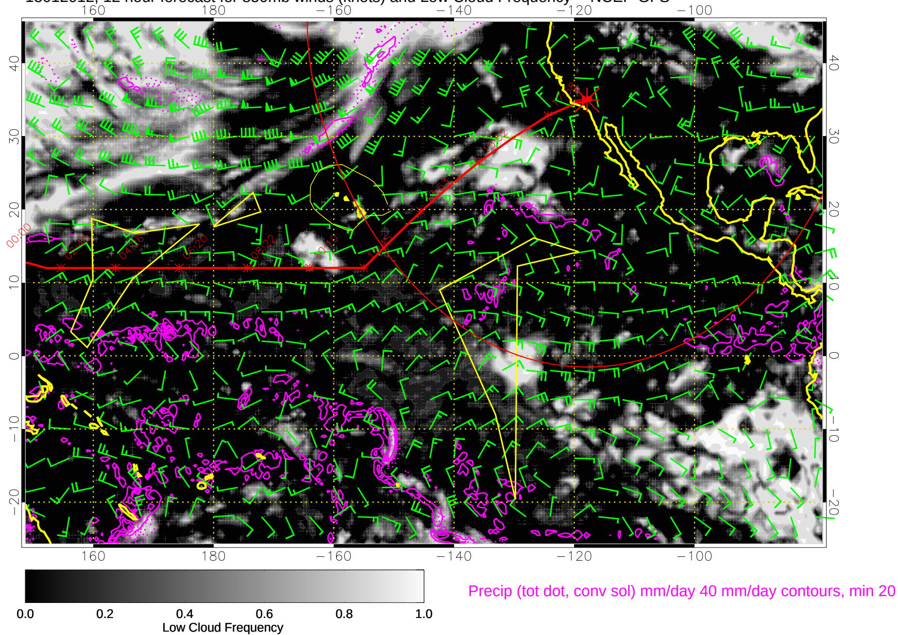
15012012, 12 hour forecast for 850mb winds (knots) and Low Cloud Frequency -- NCEP GFS
