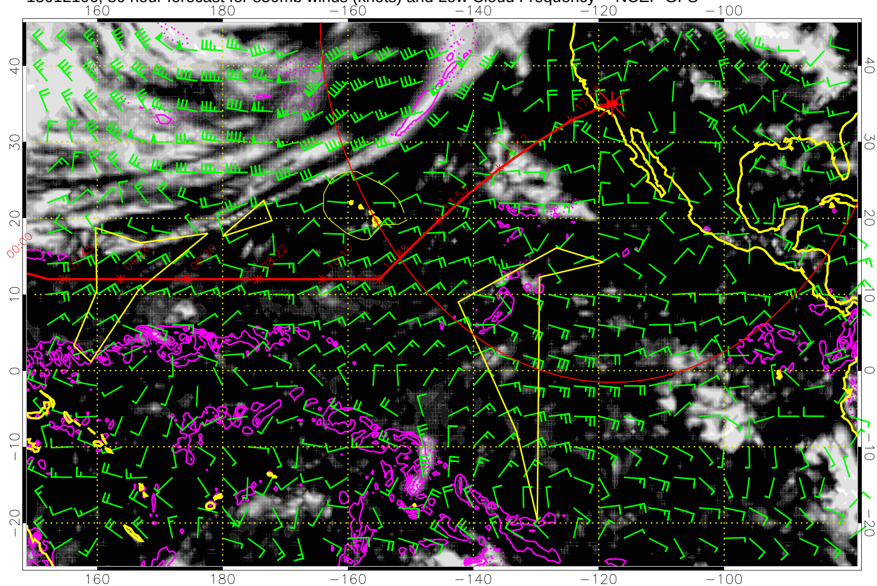
15012106, 30 hour forecast for 850mb winds (knots) and Low Cloud Frequency -- NCEP GFS
