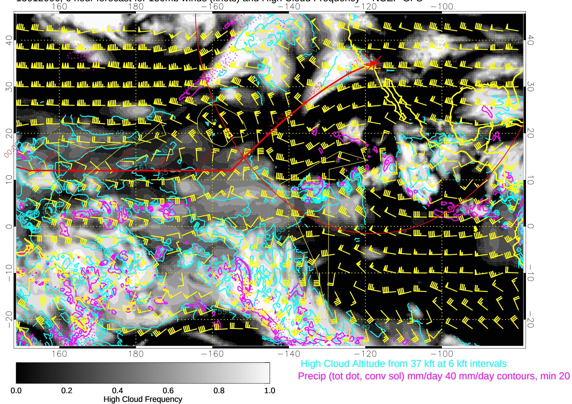
15012006, 6 hour forecast for 150mb winds (knots) and High Cloud Frequency -- NCEP GFS
