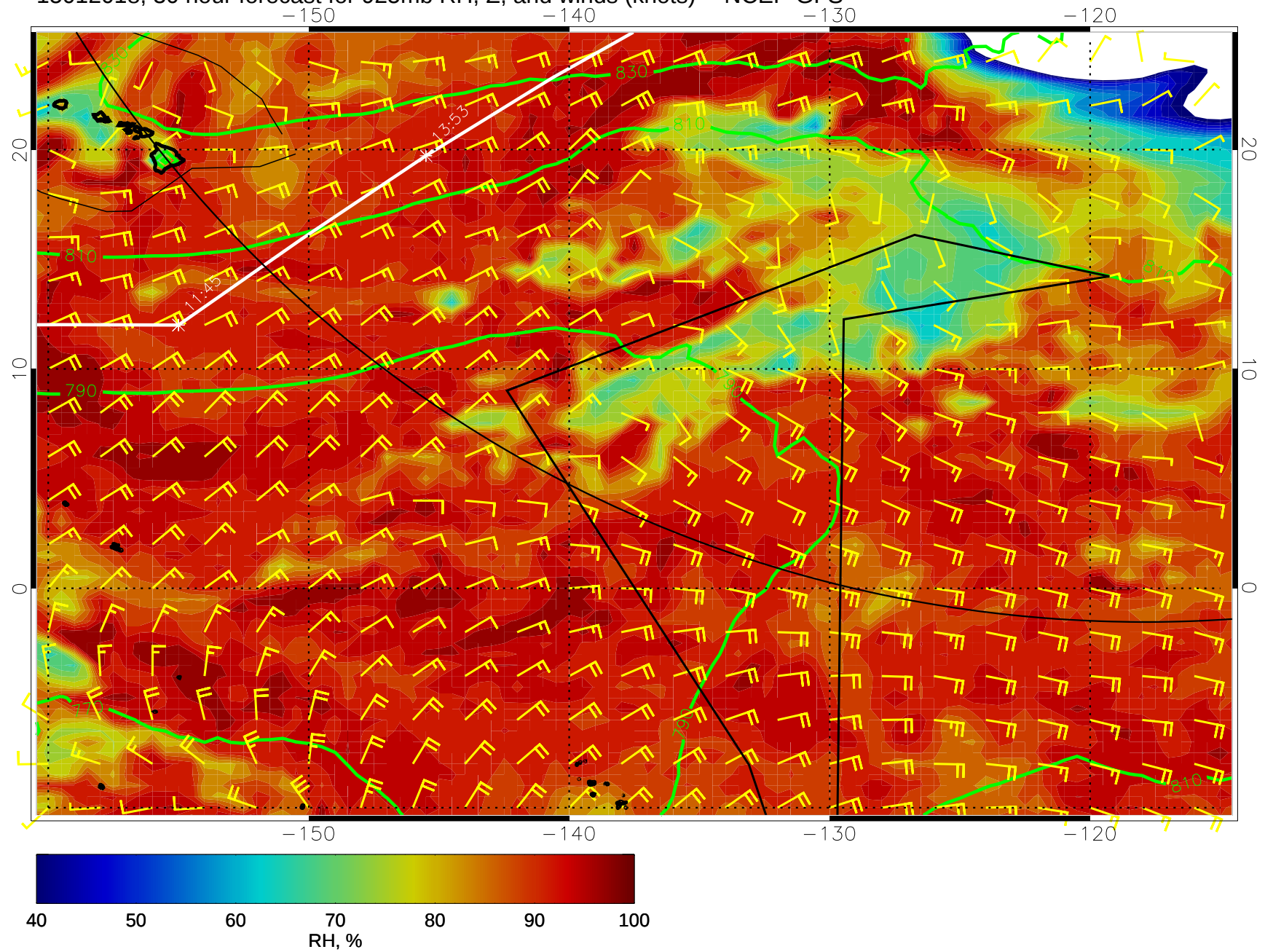
15012018, 30 hour forecast for 925mb RH, Z, and winds (knots) -- NCEP GFS
