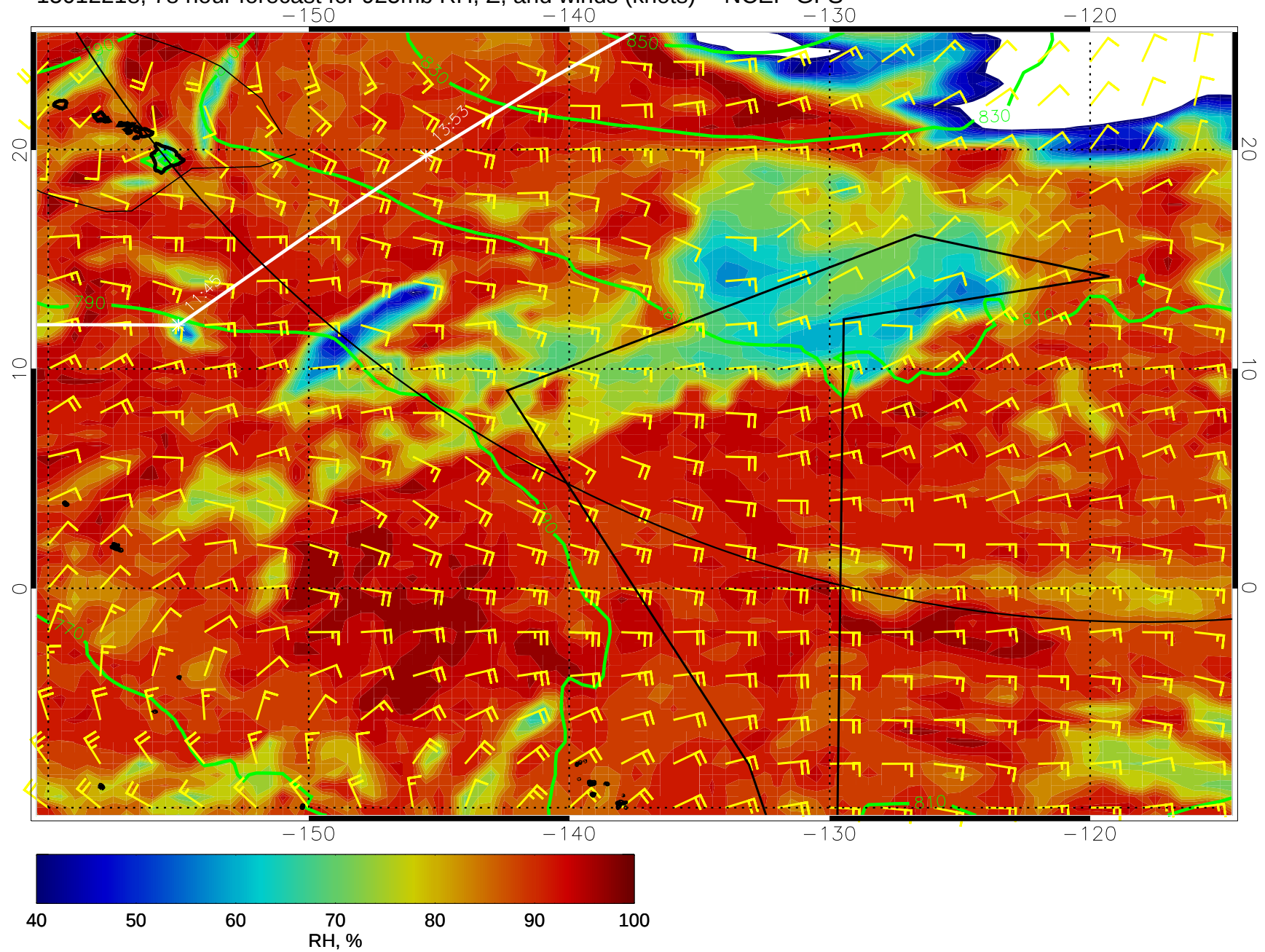
15012218, 78 hour forecast for 925mb RH, Z, and winds (knots) -- NCEP GFS
