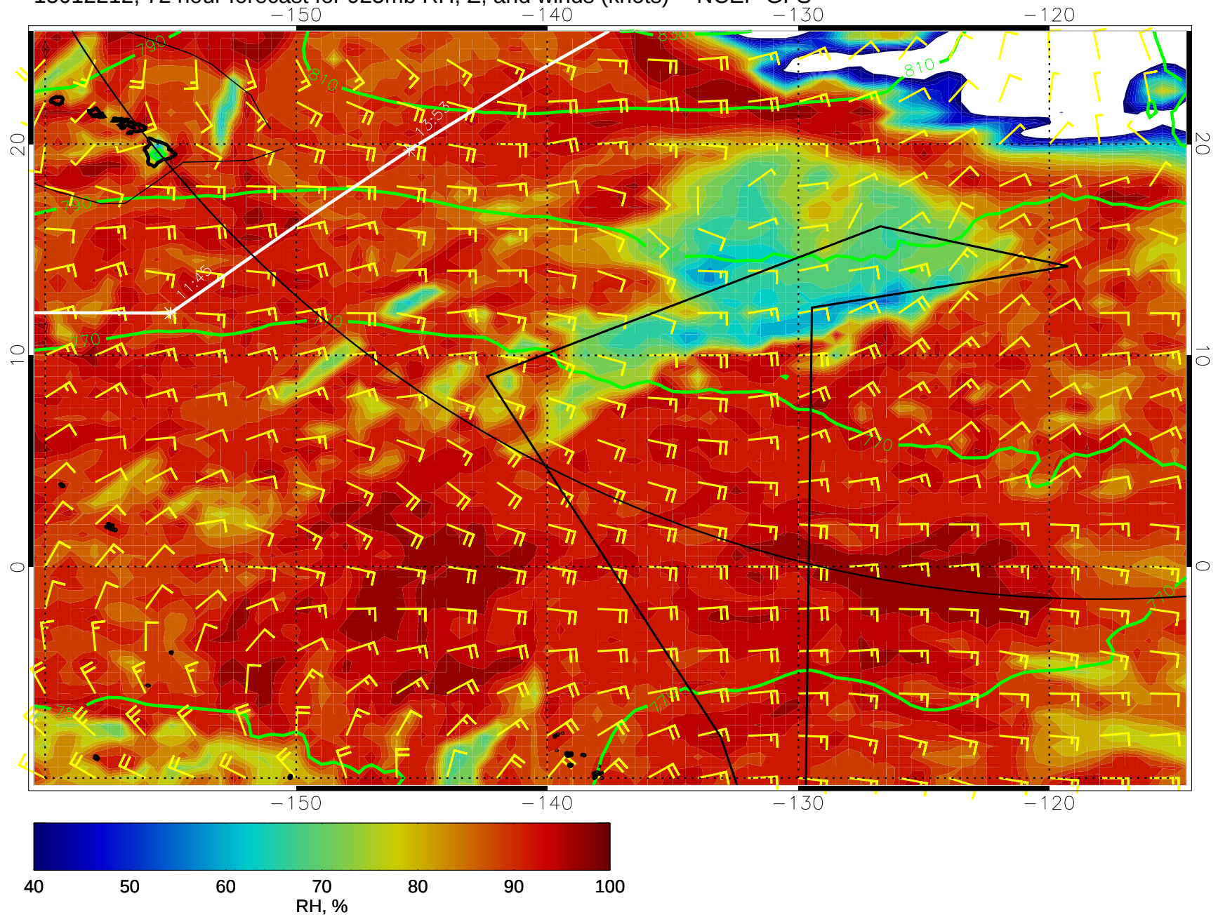
15012212, 72 hour forecast for 925mb RH, Z, and winds (knots) -- NCEP GFS
