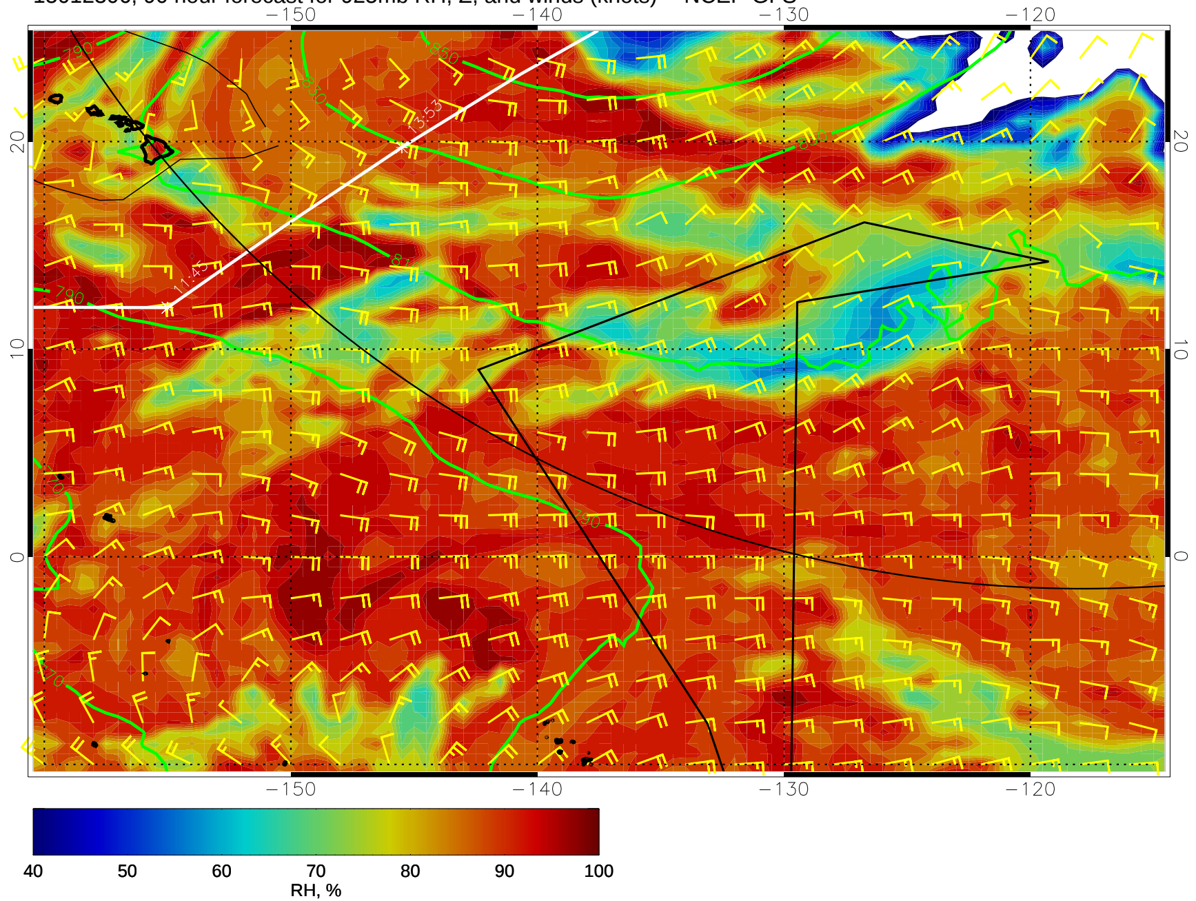
15012306, 90 hour forecast for 925mb RH, Z, and winds (knots) -- NCEP GFS
