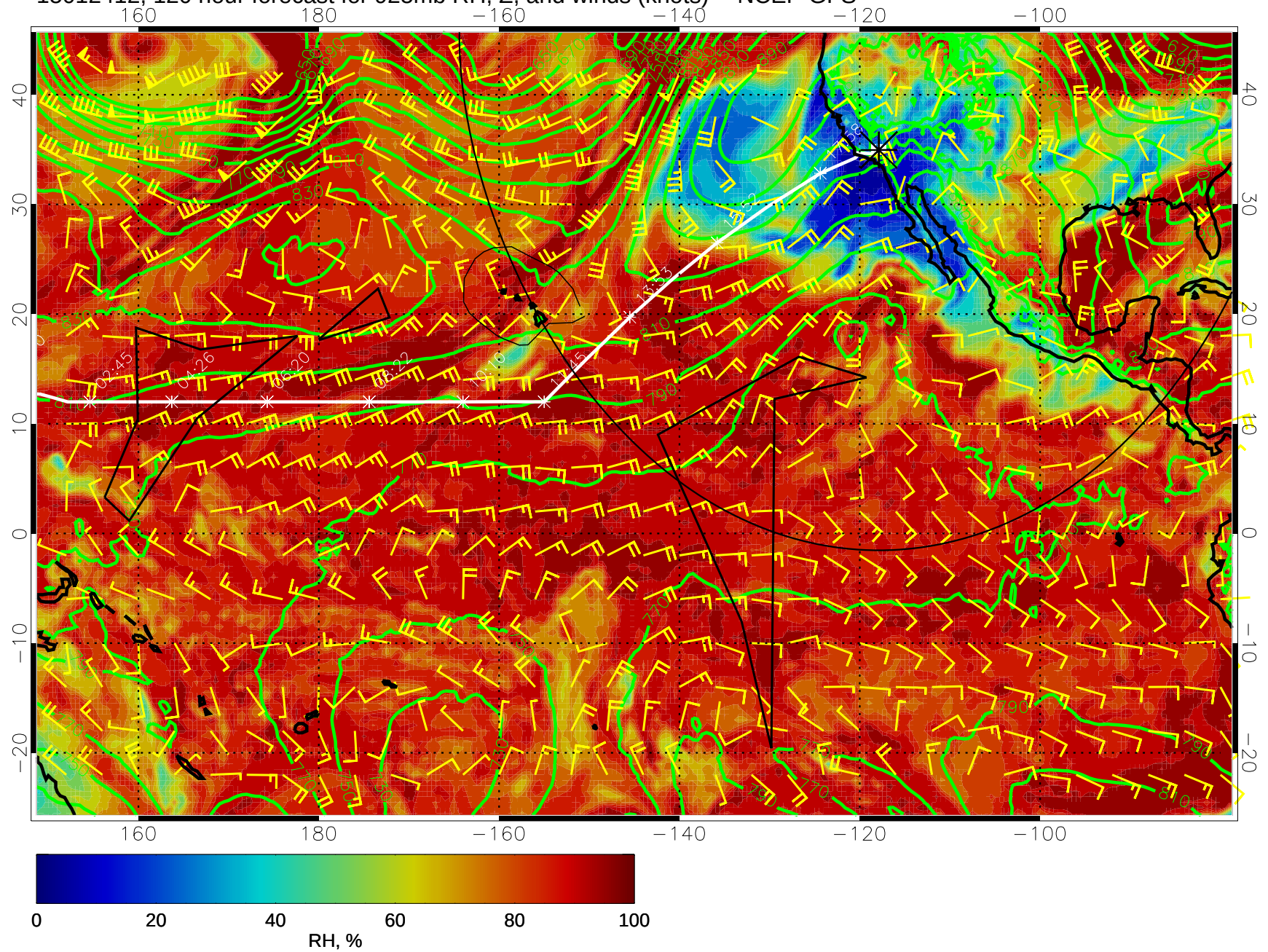
15012412, 120 hour forecast for 925mb RH, Z, and winds (knots) -- NCEP GFS
