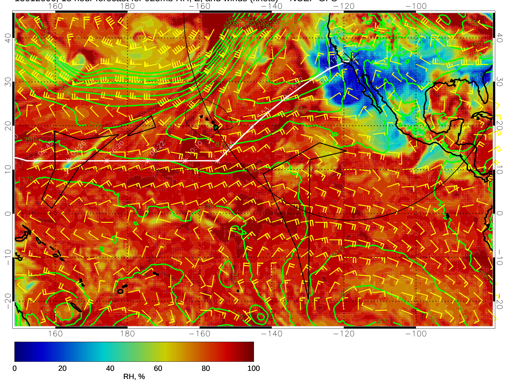
15012006, 18 hour forecast for 925mb RH, Z, and winds (knots) -- NCEP GFS
