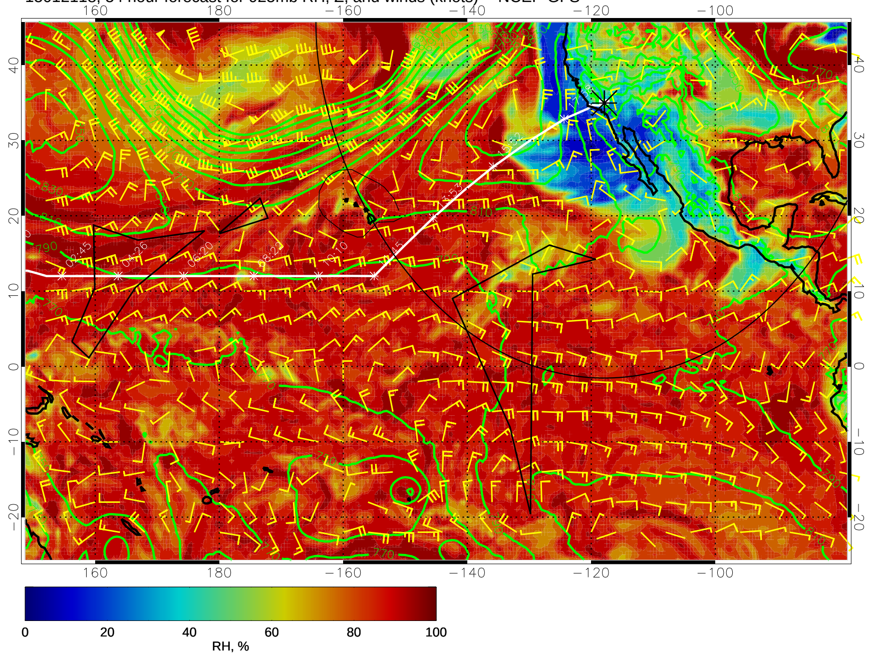
15012118, 54 hour forecast for 925mb RH, Z, and winds (knots) -- NCEP GFS
