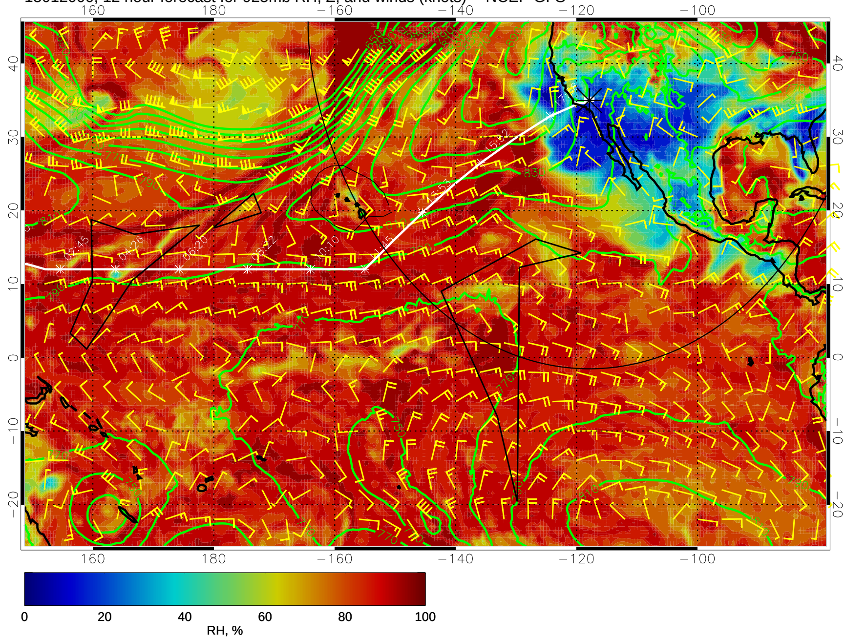
15012000, 12 hour forecast for 925mb RH, Z, and winds (knots) -- NCEP GFS
