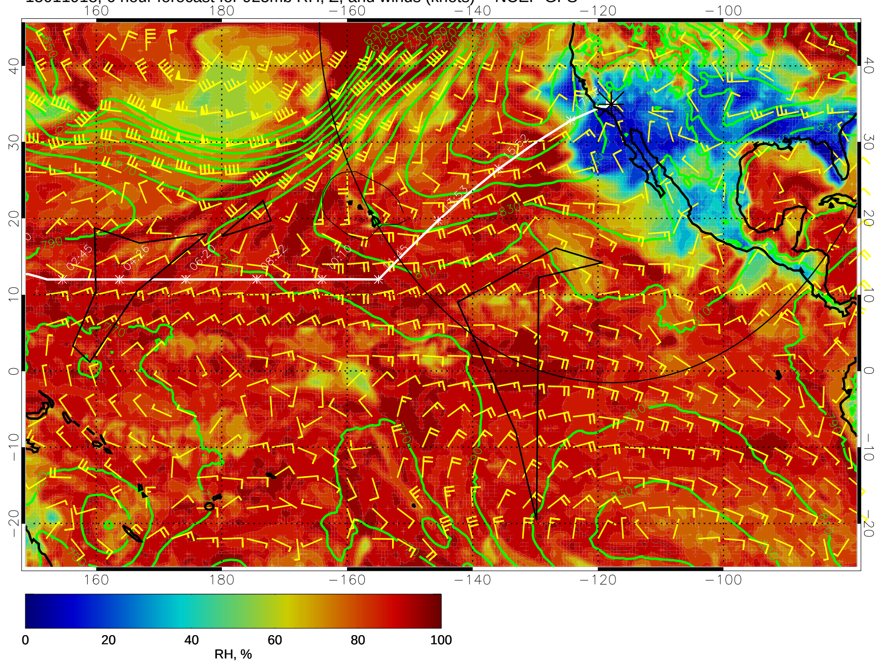
15011918, 6 hour forecast for 925mb RH, Z, and winds (knots) -- NCEP GFS
