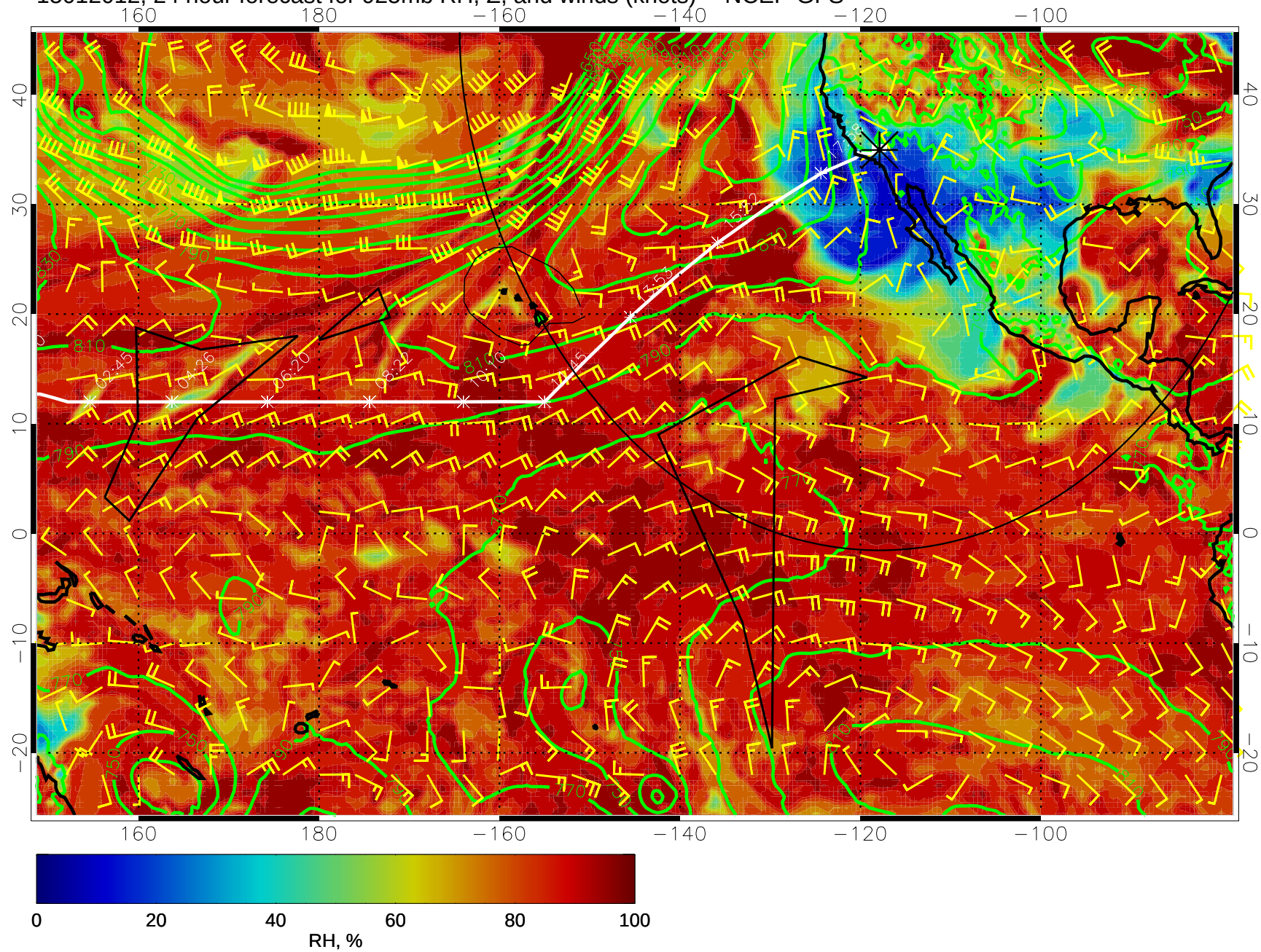
15012012, 24 hour forecast for 925mb RH, Z, and winds (knots) -- NCEP GFS
