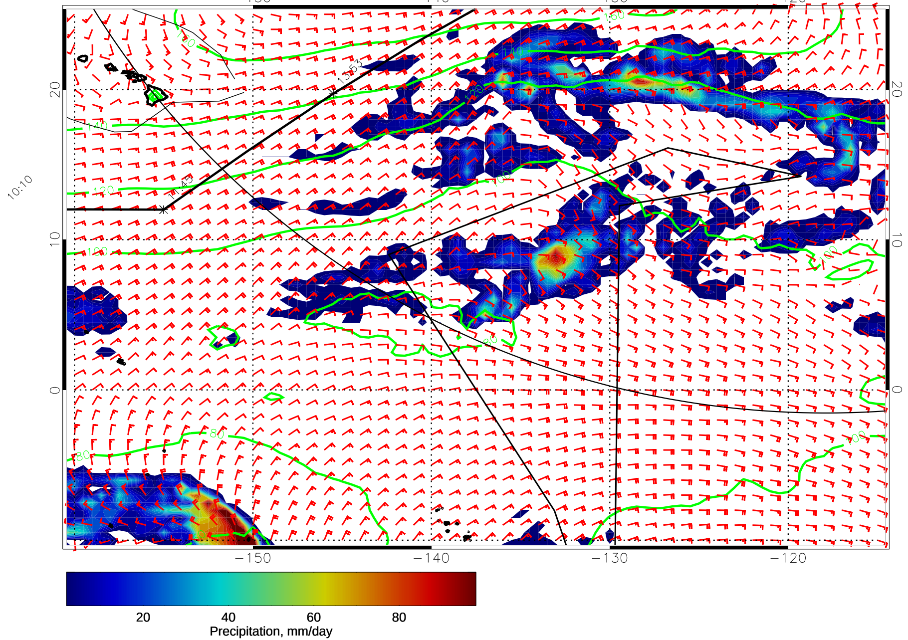
15012012, 24 hour forecast for precip, 1000mb Z, and winds (knots) -- NCEP GFS
